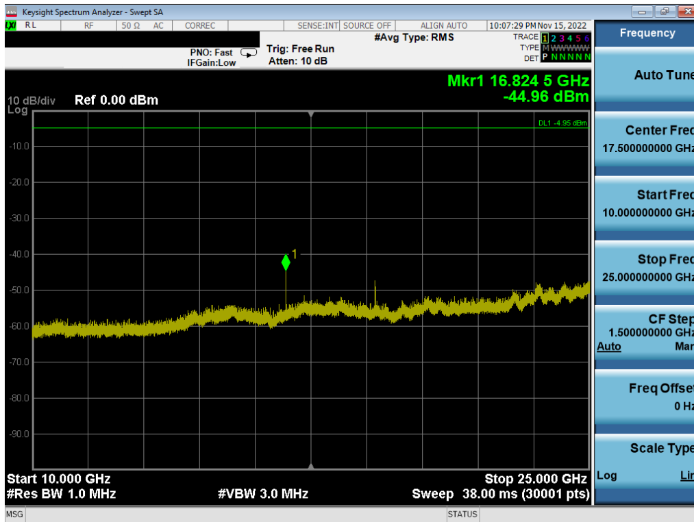
Plot 7-18. Conducted Spurious Plot (Bluetooth (LE), 2Mbps – Ch. 0)
