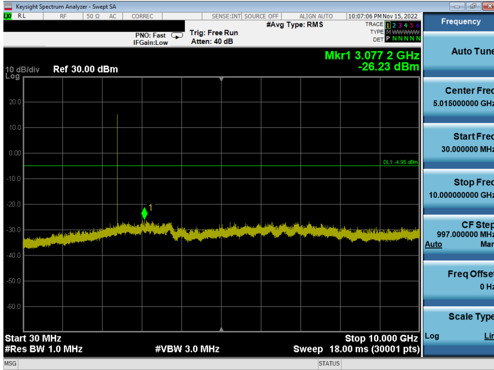
Plot 7-17. Conducted Spurious Plot (Bluetooth (LE), 2Mbps – Ch. 0)
