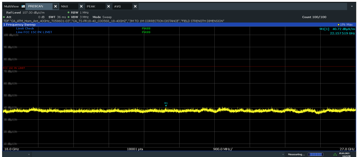
Plot 7-27. Radiated Spurious Emissions Above 18GHz V Polarity (2Mbps – Ch. 19)
