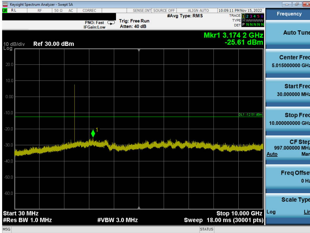
Plot 7-19. Conducted Spurious Plot (Bluetooth (LE), 2Mbps – Ch. 19)
