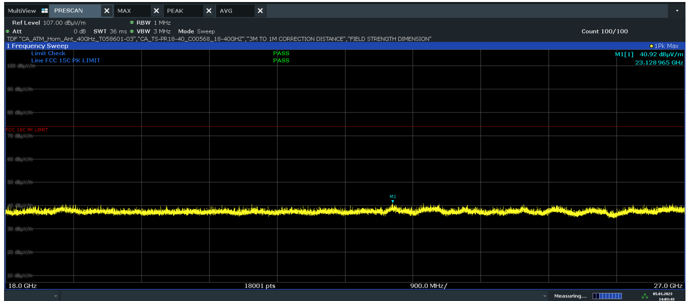
Plot 7-26. Radiated Spurious Emissions Above 18GHz H Polarity (2Mbps – Ch. 19)
