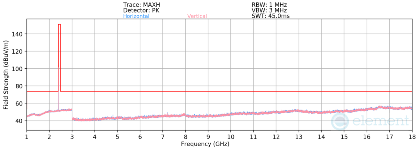
Plot 7-23. Radiated Spurious Emissions 1-18GHz (2Mbps – Ch. 1)
