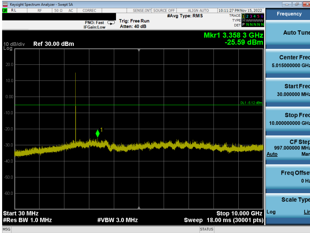
Plot 7-21. Conducted Spurious Plot (Bluetooth (LE), 2Mbps – Ch. 39)
