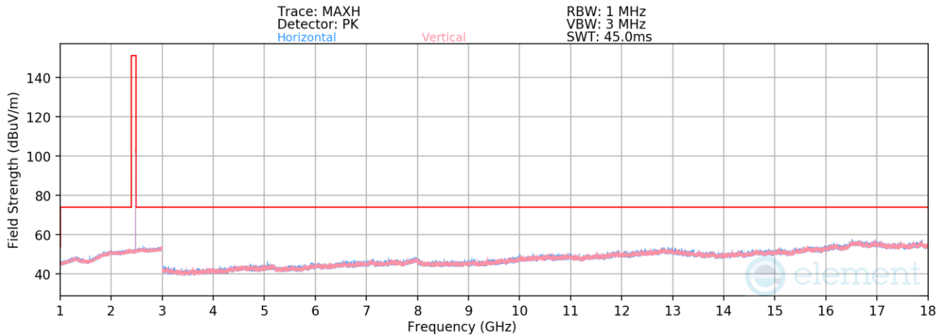
Plot 7-25. Radiated Spurious Emissions 1-18GHz (2Mbps – Ch. 38)
