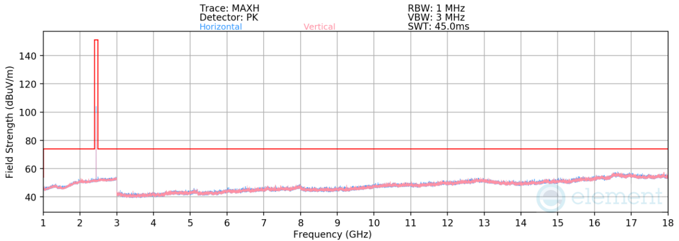
Plot 7-24. Radiated Spurious Emissions 1-18GHz (2Mbps – Ch. 19)
