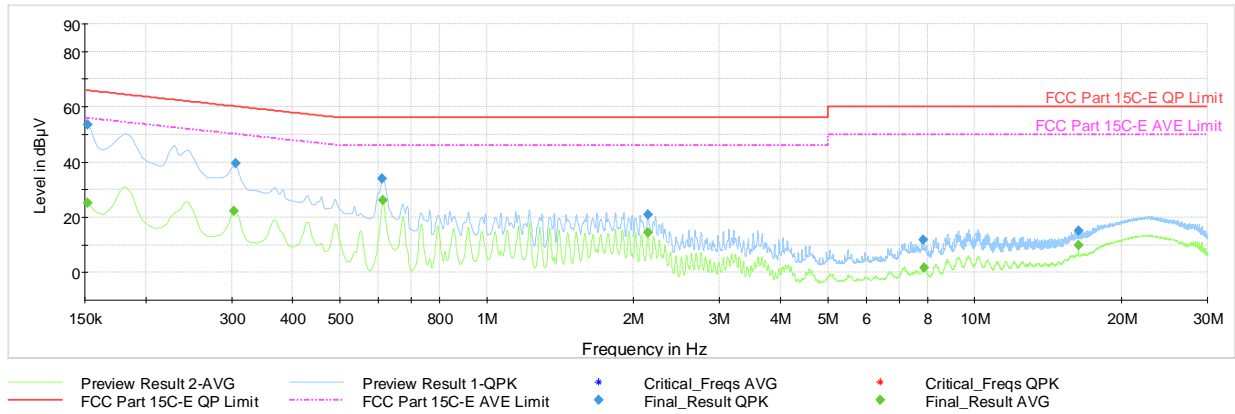
Plot 7-33. AC Line Conducted Plot with Bluetooth LE (L1, 2Mbps – Ch.19 with Laptop)
