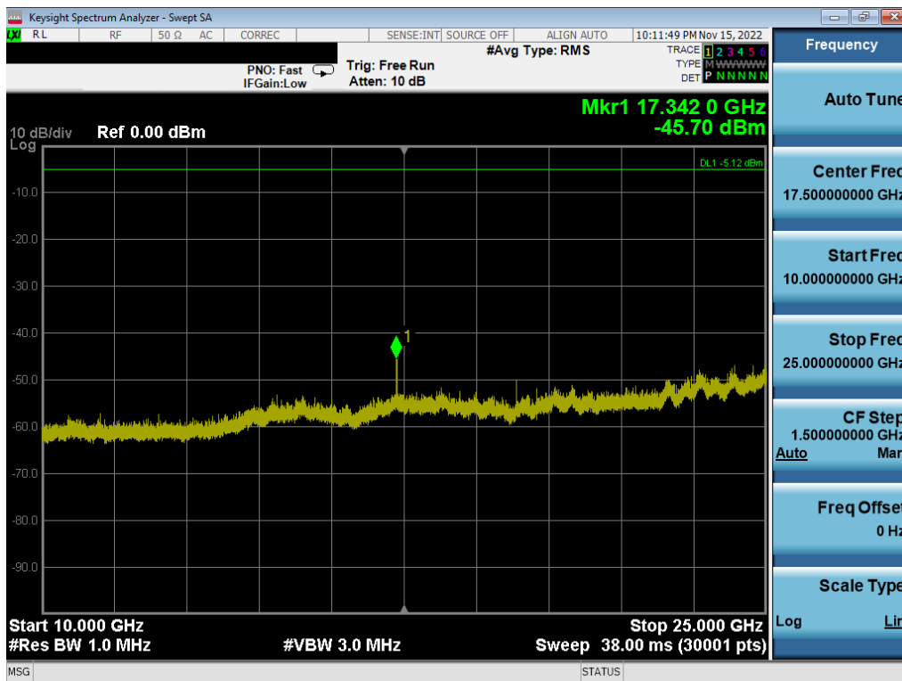
Plot 7-22. Conducted Spurious Plot (Bluetooth (LE), 2Mbps – Ch. 39)
