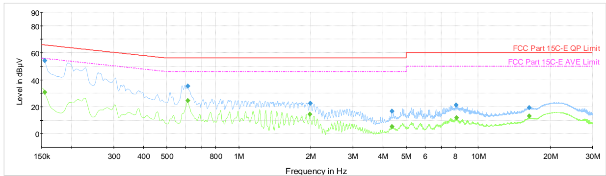
Plot 7-34. AC Line Conducted Plot with Bluetooth LE (N, 2Mbps – Ch.0, with Laptop)
