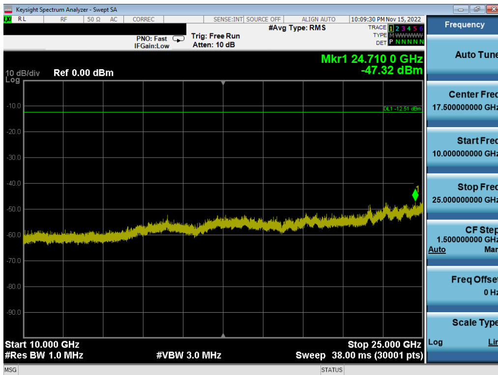
Plot 7-20. Conducted Spurious Plot (Bluetooth (LE), 2Mbps – Ch. 19)
