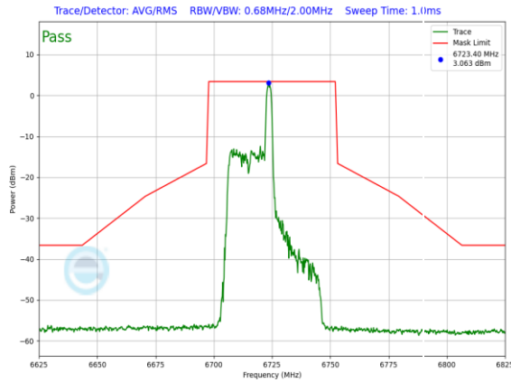
Plot 7-1067. SP In-Band Emission Plot CDD Diversity Antenna WF5B (40MHz 802.11ax RU26 (UNII Band 7) – Ch. 155)
