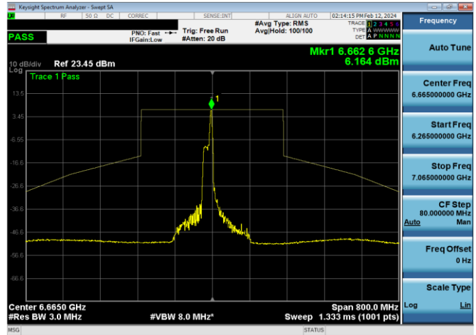
Plot 7-1083. SP In-Band Emission Plot CDD Diversity Antenna WF5B (160MHz 802.11ax RU26 (UNII Band 7) – Ch. 143)
