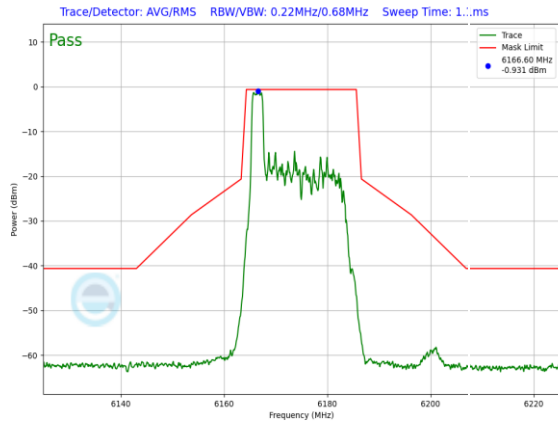
Plot 7-962. SP In-Band Emission Plot CDD Primary Antenna 4a (20MHz 802.11ax RU26 (UNII Band 5) – Ch. 45)
