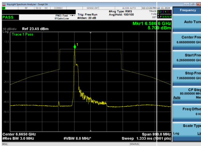
Plot 7-1081. SP In-Band Emission Plot CDD Diversity Antenna WF5B (160MHz 802.11ax RU26 (UNII Band 7) – Ch. 143)
