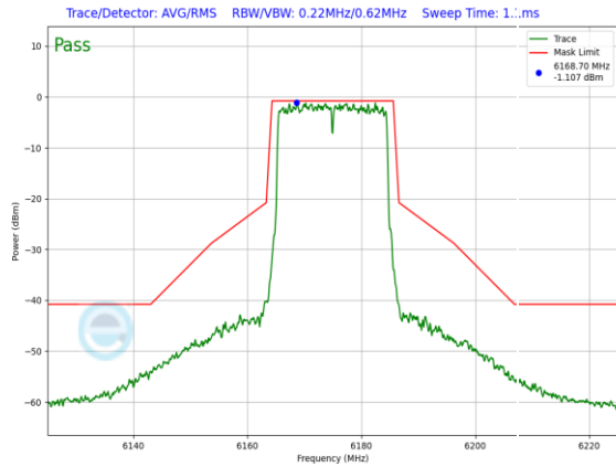
Plot 7-1031. SP In-Band Emission Plot CDD Diversity Antenna WF5B (20MHz 802.11ax RU242 (UNII Band 5) – Ch. 45)
