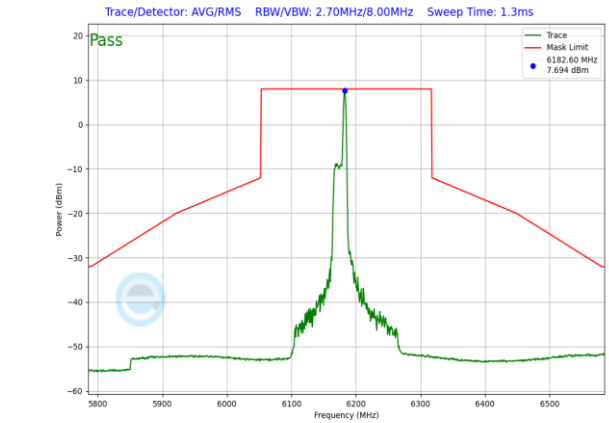
Plot 7-1052. SP In-Band Emission Plot CDD Diversity Antenna 2a (160MHz 802.11ax RU26 (UNII Band 5) – Ch. 47)
