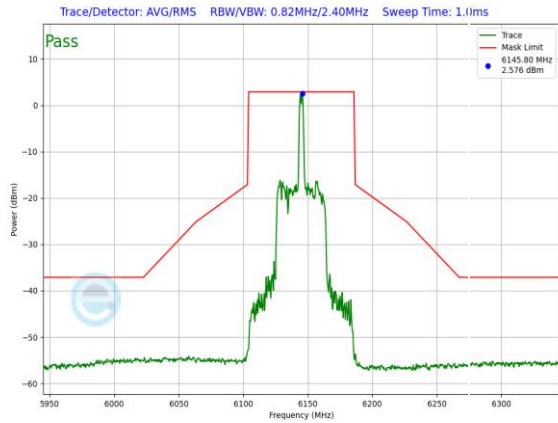
Plot 7-1043. SP In-Band Emission Plot CDD Diversity Antenna WF5B (80MHz 802.11ax RU26 (UNII Band 5) – Ch. 39)
