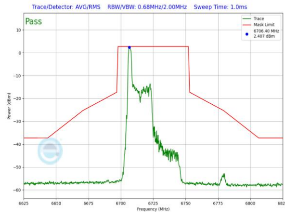
Plot 7-1065. SP In-Band Emission Plot CDD Diversity Antenna WF5B (40MHz 802.11ax RU26 (UNII Band 7) – Ch. 155)
