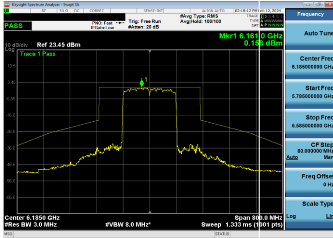
Plot 7-991. SP In-Band Emission Plot CDD Primary Antenna WF5B (160MHz 802.11ax RU996x2 (UNII Band 5) – Ch. 47)
