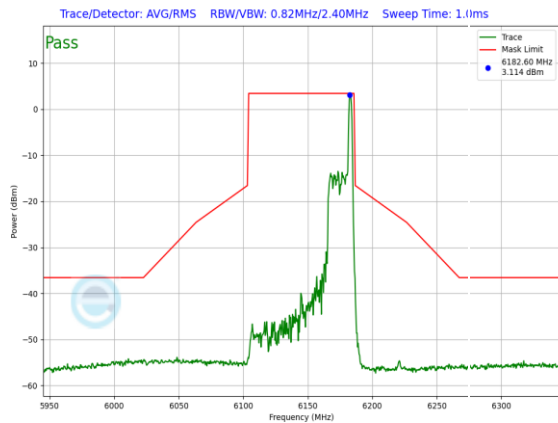
Plot 7-1045. SP In-Band Emission Plot CDD Diversity Antenna WF5B (80MHz 802.11ax RU26 (UNII Band 5) – Ch. 39)
