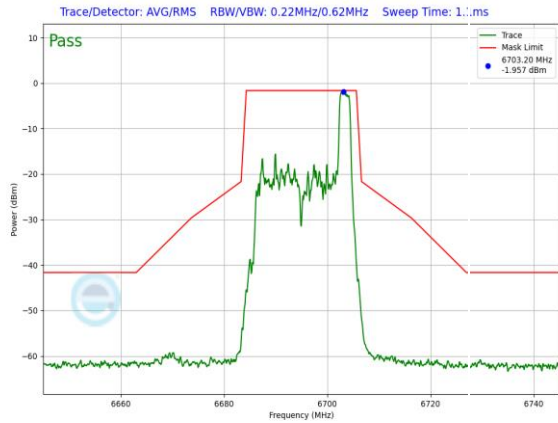
Plot 7-1061. SP In-Band Emission Plot CDD Diversity Antenna WF5B (20MHz 802.11ax RU26 (UNII Band 7) – Ch. 149)
