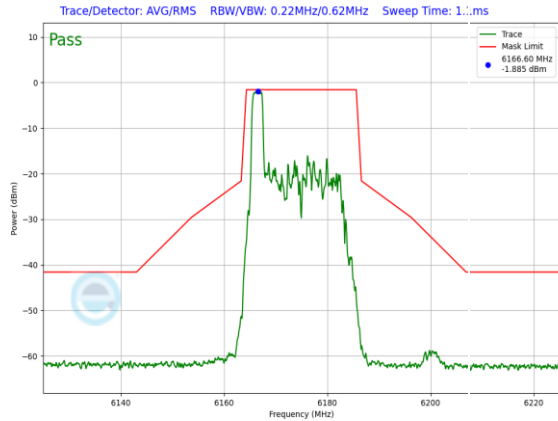
Plot 7-1025. SP In-Band Emission Plot CDD Diversity Antenna WF5B (20MHz 802.11ax RU26 (UNII Band 5) – Ch. 45)
