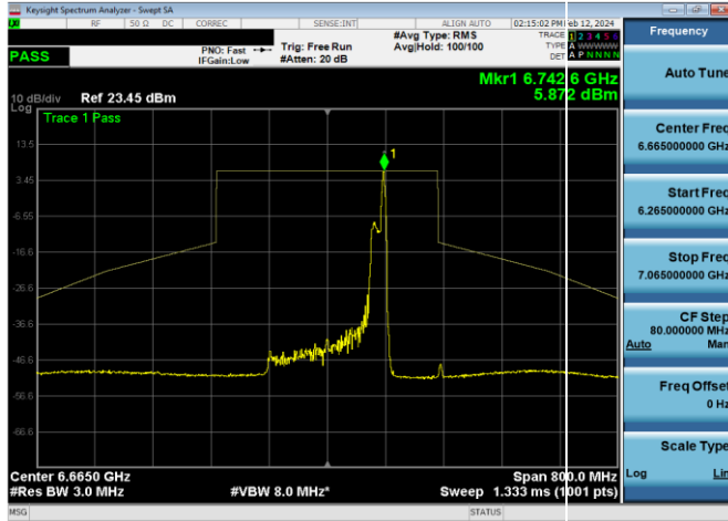
Plot 7-1021. SP In-Band Emission Plot CDD Primary Antenna WF5B (160MHz 802.11ax RU26 (UNII Band 7) – Ch. 143)
