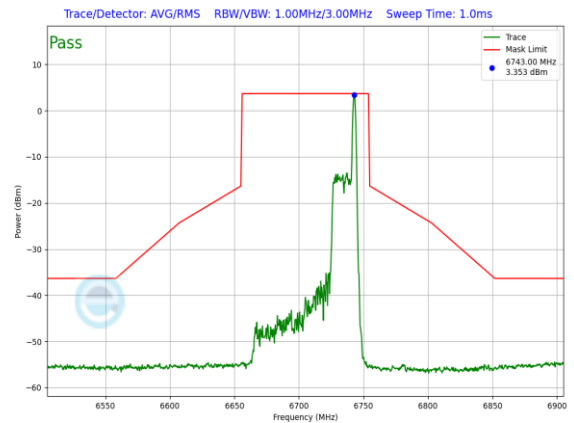
Plot 7-1077. SP In-Band Emission Plot CDD Diversity Antenna WF5B (80MHz 802.11ax RU26 (UNII Band 7) – Ch. 151)
