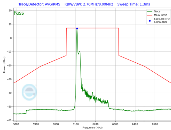
Plot 7-1050. SP In-Band Emission Plot CDD Diversity Antenna 2a (160MHz 802.11ax RU26 (UNII Band 5) – Ch. 47)
