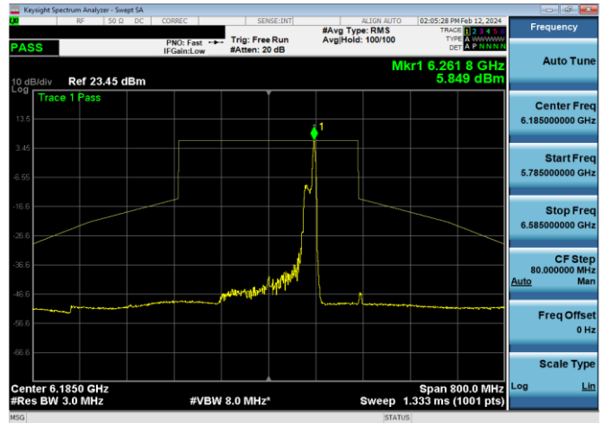
Plot 7-989. SP In-Band Emission Plot CDD Primary Antenna WF5B (160MHz 802.11ax RU26 (UNII Band 5) – Ch. 47)
