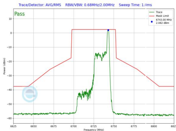
Plot 7-1069. SP In-Band Emission Plot CDD Diversity Antenna WF5B (40MHz 802.11ax RU26 (UNII Band 7) – Ch. 155)
