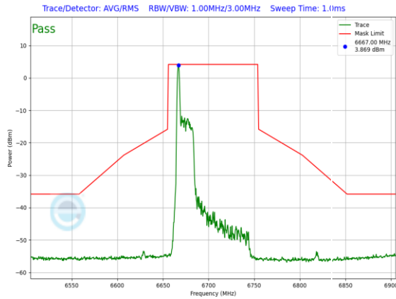
Plot 7-1073. SP In-Band Emission Plot CDD Diversity Antenna WF5B (80MHz 802.11ax RU26 (UNII Band 7) – Ch. 151)
