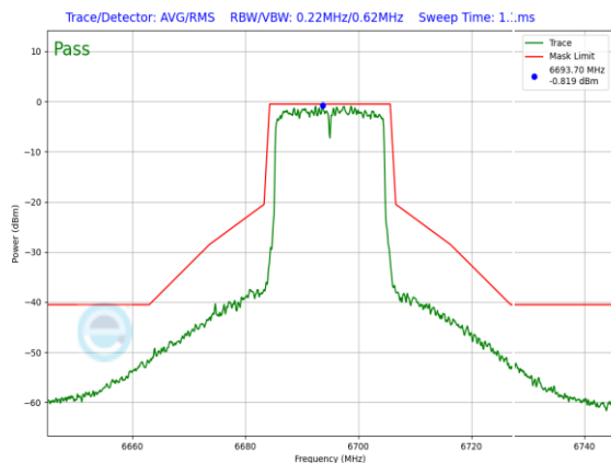
Plot 7-1063. SP In-Band Emission Plot CDD Diversity Antenna WF5B (20MHz 802.11ax RU242 (UNII Band 7) – Ch. 149)
