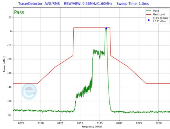
Plot 7-1037. SP In-Band Emission Plot CDD Diversity Antenna WF5B (40MHz 802.11ax RU26 (UNII Band 5) – Ch. 43)
