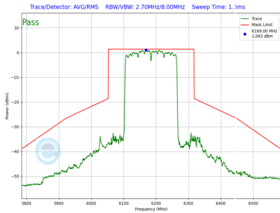
Plot 7-1056. SP In-Band Emission Plot CDD Diversity Antenna 2a (160MHz 802.11ax RU996x2 (UNII Band 5) – Ch. 47)
