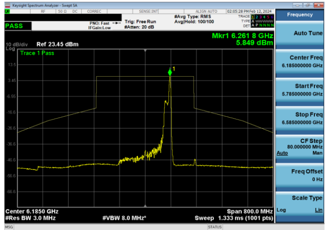
Plot 7-1053. SP In-Band Emission Plot CDD Diversity Antenna WF5B (160MHz 802.11ax RU26 (UNII Band 5) – Ch. 47)
