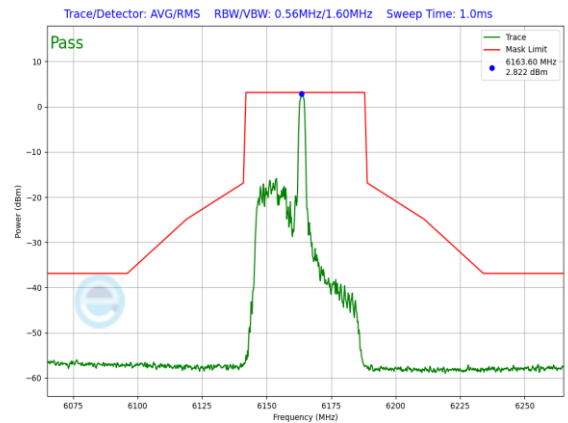
Plot 7-1035. SP In-Band Emission Plot CDD Diversity Antenna WF5B (40MHz 802.11ax RU26 (UNII Band 5) – Ch. 43)
