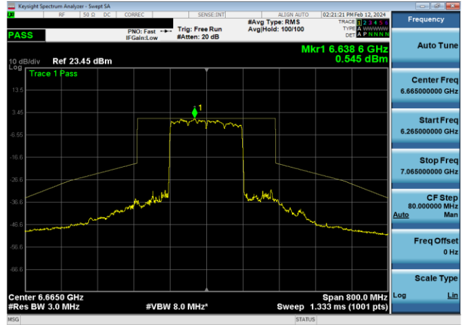
Plot 7-1023. SP In-Band Emission Plot CDD Primary Antenna WF5B (160MHz 802.11ax RU996x2 (UNII Band 7) – Ch. 143)
