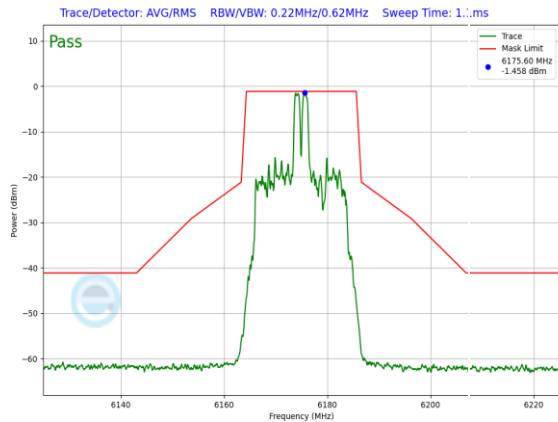
Plot 7-1027. SP In-Band Emission Plot CDD Diversity Antenna WF5B (20MHz 802.11ax RU26 (UNII Band 5) – Ch. 45)
