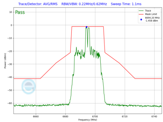
Plot 7-1059. SP In-Band Emission Plot CDD Diversity Antenna WF5B (20MHz 802.11ax RU26 (UNII Band 7) – Ch. 149)
