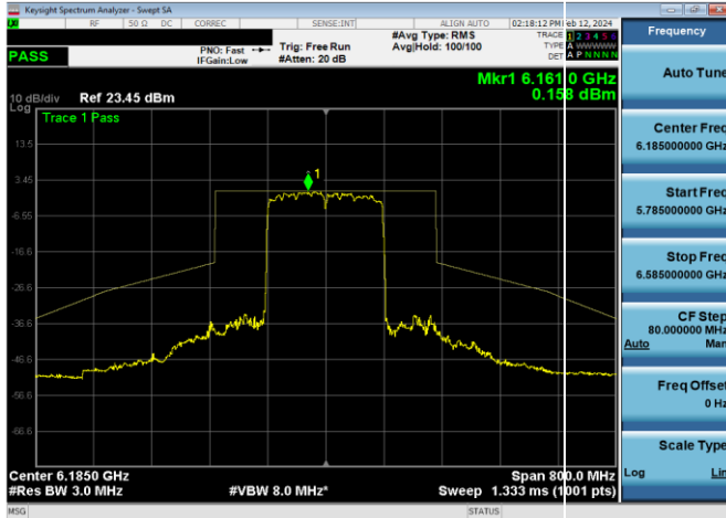
Plot 7-1055. SP In-Band Emission Plot CDD Diversity Antenna WF5B (160MHz 802.11ax RU996x2 (UNII Band 5) – Ch. 47)
