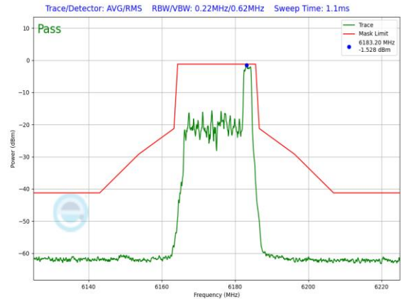
Plot 7-1029. SP In-Band Emission Plot CDD Diversity Antenna WF5B (20MHz 802.11ax RU26 (UNII Band 5) – Ch. 45)
