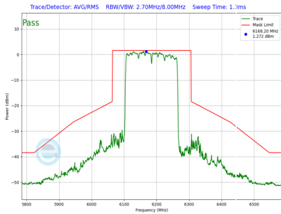
Plot 7-992. SP In-Band Emission Plot CDD Primary Antenna 4a (160MHz 802.11ax RU996x2 (UNII Band 5) – Ch. 47)
