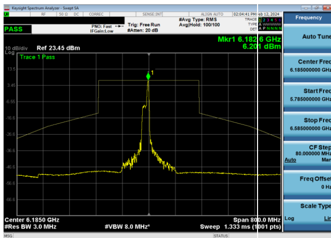
Plot 7-1051. SP In-Band Emission Plot CDD Diversity Antenna WF5B (160MHz 802.11ax RU26 (UNII Band 5) – Ch. 47)
