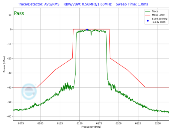
Plot 7-1039. SP In-Band Emission Plot CDD Diversity Antenna WF5B (40MHz 802.11ax RU484 (UNII Band 5) – Ch. 43)
