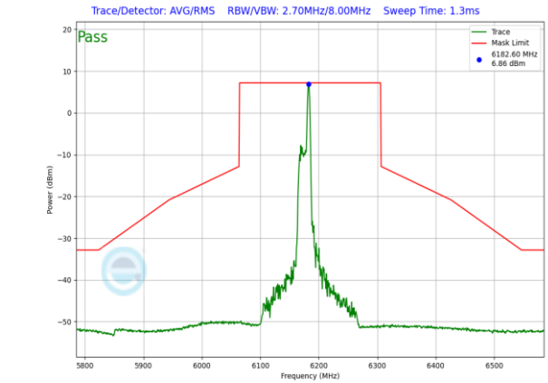
Plot 7-988. SP In-Band Emission Plot CDD Primary Antenna 4a (160MHz 802.11ax RU26 (UNII Band 5) – Ch. 47)
