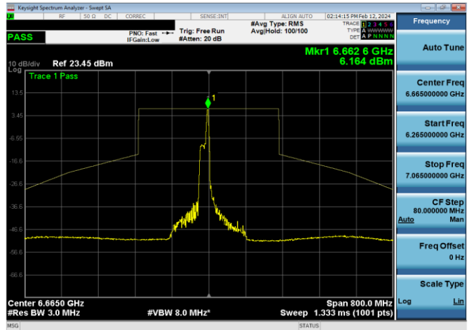
Plot 7-1019. SP In-Band Emission Plot CDD Primary Antenna WF5B (160MHz 802.11ax RU26 (UNII Band 7) – Ch. 143)
