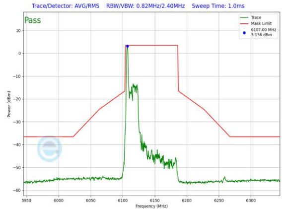
Plot 7-1041. SP In-Band Emission Plot CDD Diversity Antenna WF5B (80MHz 802.11ax RU26 (UNII Band 5) – Ch. 39)
