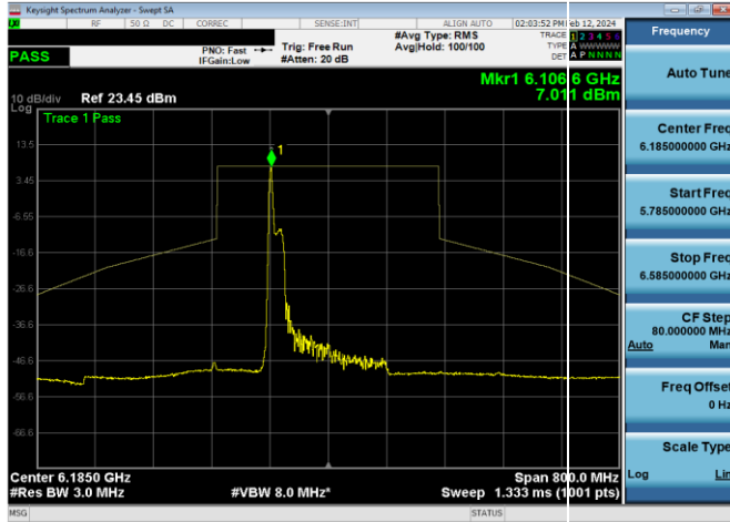
Plot 7-985. SP In-Band Emission Plot CDD Primary Antenna WF5B (160MHz 802.11ax RU26 (UNII Band 5) – Ch. 47)
