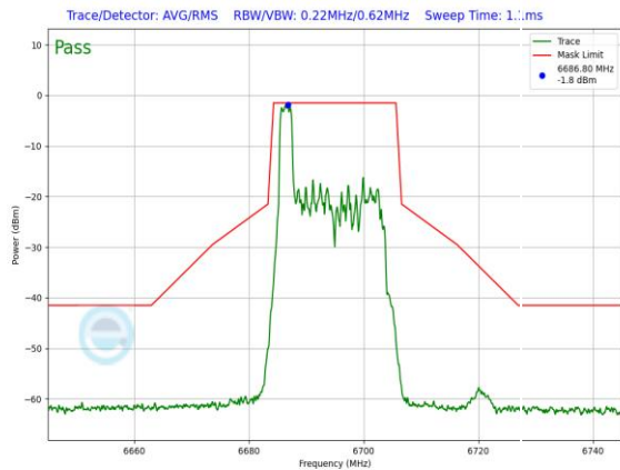
Plot 7-1057. SP In-Band Emission Plot CDD Diversity Antenna WF5B (20MHz 802.11ax RU26 (UNII Band 7) – Ch. 149)
