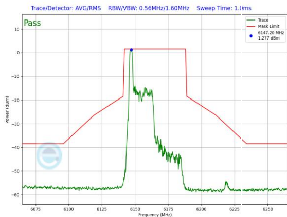
Plot 7-1033. SP In-Band Emission Plot CDD Diversity Antenna WF5B (40MHz 802.11ax RU26 (UNII Band 5) – Ch. 43)
