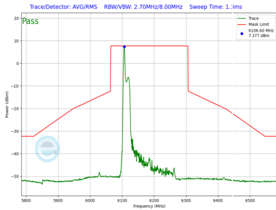
Plot 7-986. SP In-Band Emission Plot CDD Primary Antenna 4a (160MHz 802.11ax RU26 (UNII Band 5) – Ch. 47)
