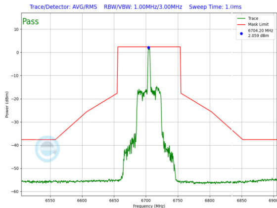
Plot 7-1075. SP In-Band Emission Plot CDD Diversity Antenna WF5B (80MHz 802.11ax RU26 (UNII Band 7) – Ch. 151)
