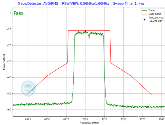
Plot 7-1126. LPI In-Band Emission Plot SDM Diversity Antenna 4a (40MHz 802.11ax (UNII Band 8) – Ch. 211, MCS11)
