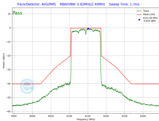
Plot 7-1147. SP In-Band Emission Plot SDM Diversity Antenna 4a (80MHz 802.11ax (UNII Band 5) – Ch. 39, MCS11)
