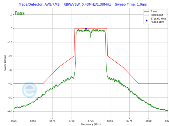
Plot 7-1150. SP In-Band Emission Plot SDM Diversity Antenna 4a (40MHz 802.11ax (UNII Band 7) – Ch. 155, MCS11)
