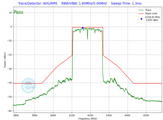
Plot 7-1148. SP In-Band Emission Plot SDM Diversity Antenna 4a (160MHz 802.11ax (UNII Band 5) – Ch. 47, MCS11)
