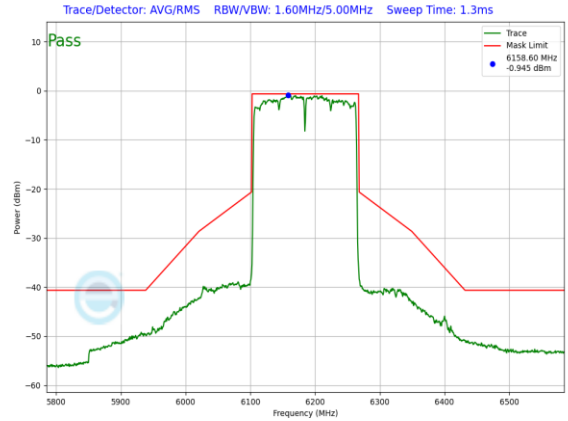
Plot 7-1140. SP In-Band Emission Plot SDM Diversity Antenna 4a (160MHz 802.11ax (UNII Band 5) – Ch. 47, MCS4)
