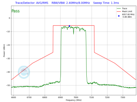
Plot 7-1128. LPI In-Band Emission Plot SDM Diversity Antenna 4a (160MHz 802.11ax (UNII Band 8) – Ch. 207, MCS11)
