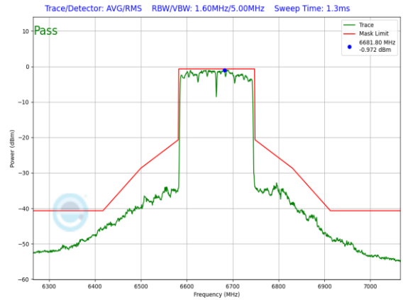
Plot 7-1152. SP In-Band Emission Plot SDM Diversity Antenna 4a (160MHz 802.11ax (UNII Band 7) – Ch. 143, MCS11)
