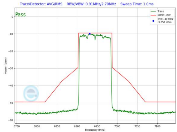
Plot 7-1127. LPI In-Band Emission Plot SDM Diversity Antenna 4a (80MHz 802.11ax (UNII Band 8) – Ch. 199, MCS11)
