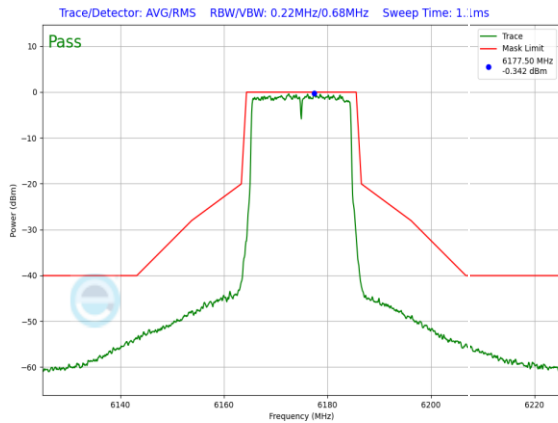
Plot 7-1129. SP In-Band Emission Plot SDM Diversity Antenna 4a (20MHz 802.11ax (UNII Band 5) – Ch. 45, MCS2)
