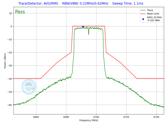
Plot 7-1141. SP In-Band Emission Plot SDM Diversity Antenna 4a (20MHz 802.11ax (UNII Band 7) – Ch. 149, MCS4)
