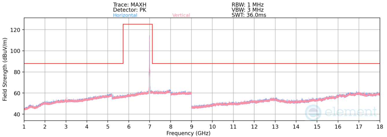
Plot 7-1211. Radiated Spurious Emissions above 1GHz Antenna 4a (802.11ax – Ch. 209, MCS0)
