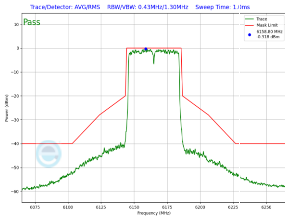
Plot 7-1146. SP In-Band Emission Plot SDM Diversity Antenna 4a (40MHz 802.11ax (UNII Band 5) – Ch. 43, MCS11)
