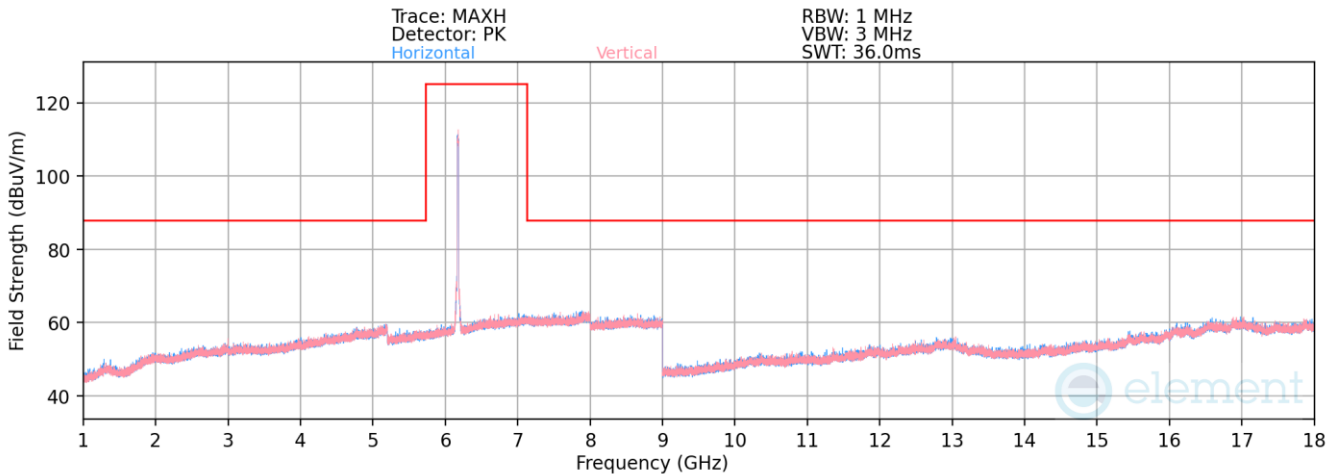
Plot 7-1214. Radiated Spurious Emissions above 1GHz Antenna 2a (802.11ax – Ch. 45, MCS0)
