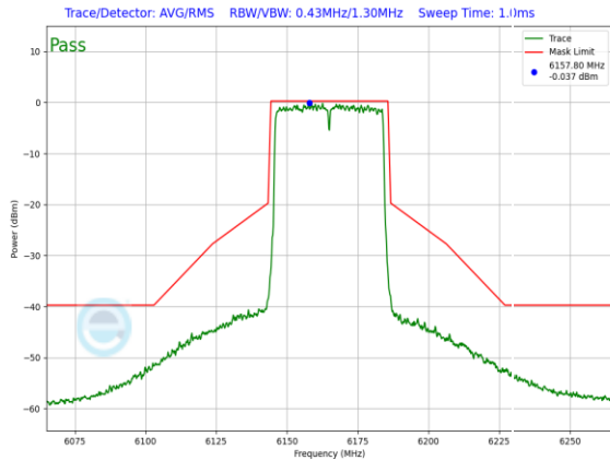
Plot 7-1138. SP In-Band Emission Plot SDM Diversity Antenna 4a (40MHz 802.11ax (UNII Band 5) – Ch. 43, MCS4)
