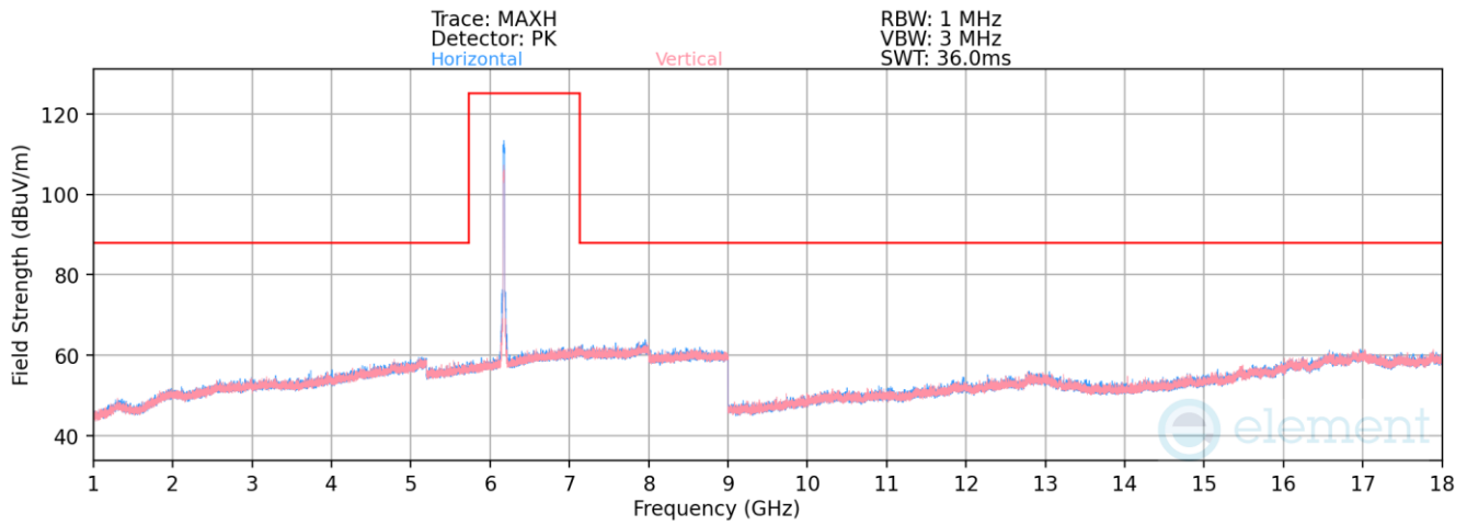
Plot 7-1190. Radiated Spurious Emissions above 1GHz Antenna WF5B (802.11ax – Ch. 45, MCS0)
