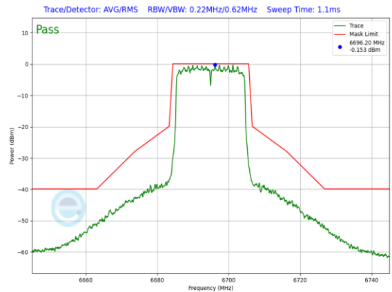
Plot 7-1149. SP In-Band Emission Plot SDM Diversity Antenna 4a (20MHz 802.11ax (UNII Band 7) – Ch. 149, MCS11)
