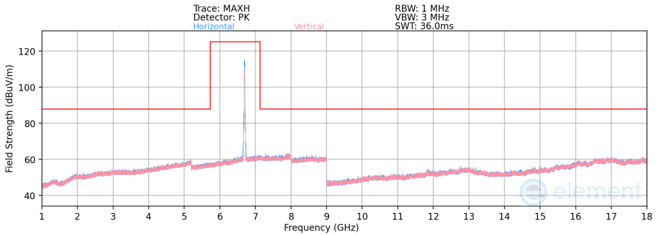
Plot 7-1196. Radiated Spurious Emissions above 1GHz Antenna WF5B (802.11ax – Ch. 149, MCS0)
