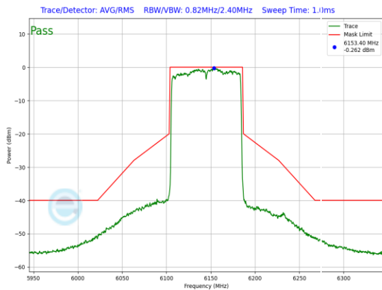
Plot 7-1139. SP In-Band Emission Plot SDM Diversity Antenna 4a (80MHz 802.11ax (UNII Band 5) – Ch. 39, MCS4)
