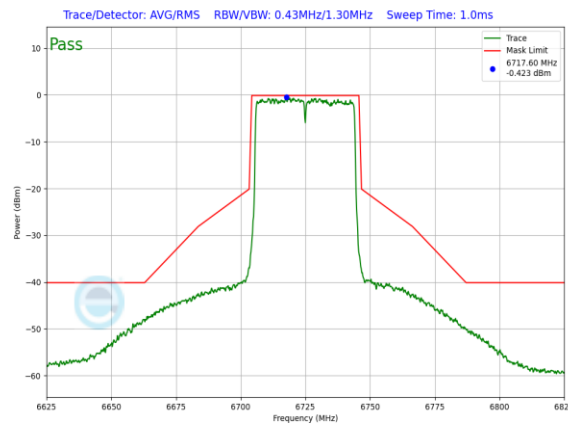
Plot 7-1134. SP In-Band Emission Plot SDM Diversity Antenna 4a (40MHz 802.11ax (UNII Band 7) – Ch. 155, MCS2)
