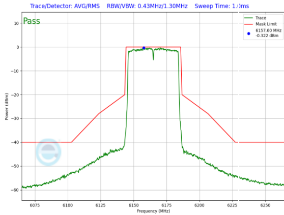
Plot 7-1130. SP In-Band Emission Plot SDM Diversity Antenna 4a (40MHz 802.11ax (UNII Band 5) – Ch. 43, MCS2)
