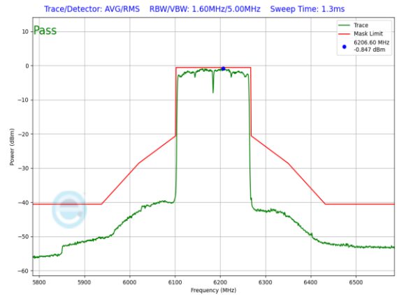
Plot 7-1132. SP In-Band Emission Plot SDM Diversity Antenna 4a (160MHz 802.11ax (UNII Band 5) – Ch. 47, MCS2)
