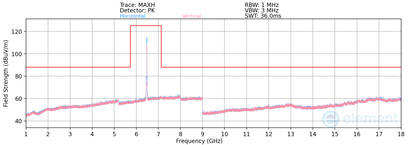
Plot 7-1193. Radiated Spurious Emissions above 1GHz Antenna WF5B (802.11ax – Ch. 105, MCS0)
