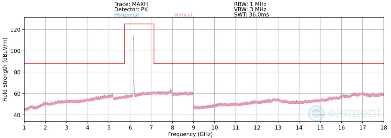
Plot 7-1202. Radiated Spurious Emissions above 1GHz Antenna 4a (802.11ax – Ch. 45, MCS0)
