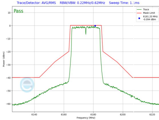
Plot 7-1137. SP In-Band Emission Plot SDM Diversity Antenna 4a (20MHz 802.11ax (UNII Band 5) – Ch. 45, MCS4)
