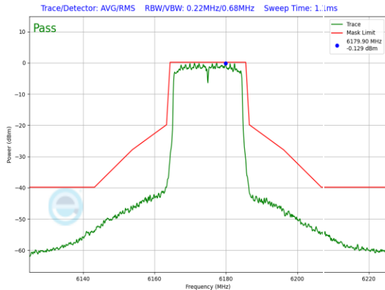
Plot 7-1145. SP In-Band Emission Plot SDM Diversity Antenna 4a (20MHz 802.11ax (UNII Band 5) – Ch. 45, MCS11)
