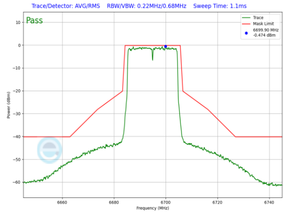
Plot 7-1133. SP In-Band Emission Plot SDM Diversity Antenna 4a (20MHz 802.11ax (UNII Band 7) – Ch. 149, MCS2)
