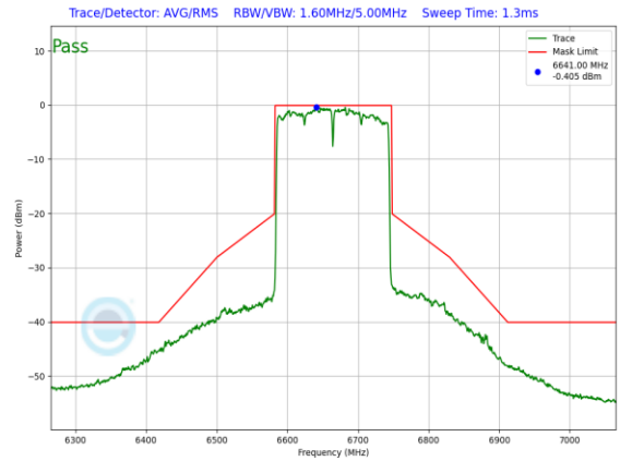
Plot 7-1144. SP In-Band Emission Plot SDM Diversity Antenna 4a (160MHz 802.11ax (UNII Band 7) – Ch. 143, MCS4)
