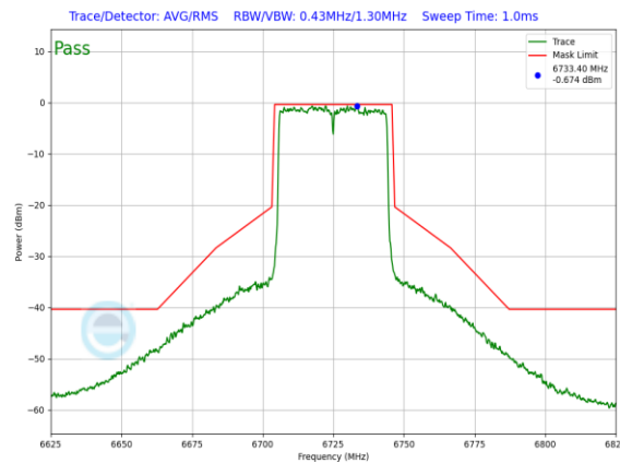
Plot 7-1142. SP In-Band Emission Plot SDM Diversity Antenna 4a (40MHz 802.11ax (UNII Band 7) – Ch. 155, MCS4)
