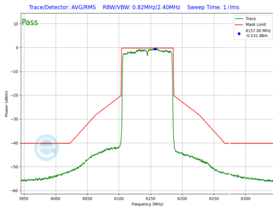
Plot 7-1131. SP In-Band Emission Plot SDM Diversity Antenna 4a (80MHz 802.11ax (UNII Band 5) – Ch. 39, MCS2)
