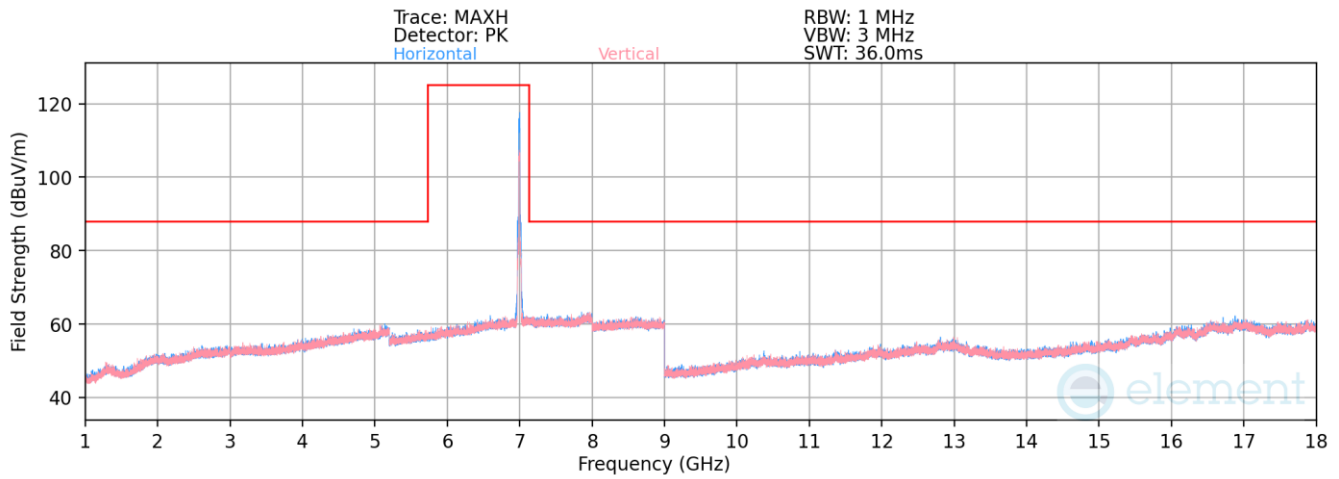
Plot 7-1199. Radiated Spurious Emissions above 1GHz Antenna WF5B (802.11ax – Ch. 209, MCS0)
