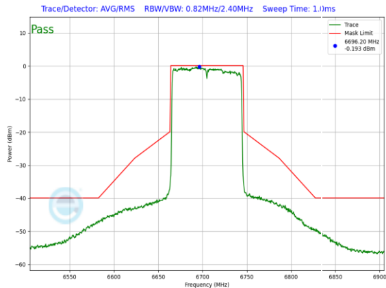
Plot 7-1135. SP In-Band Emission Plot SDM Diversity Antenna 4a (80MHz 802.11ax (UNII Band 7) – Ch. 151, MCS2)
