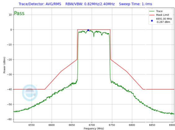
Plot 7-1151. SP In-Band Emission Plot SDM Diversity Antenna 4a (80MHz 802.11ax (UNII Band 7) – Ch. 151, MCS11)
