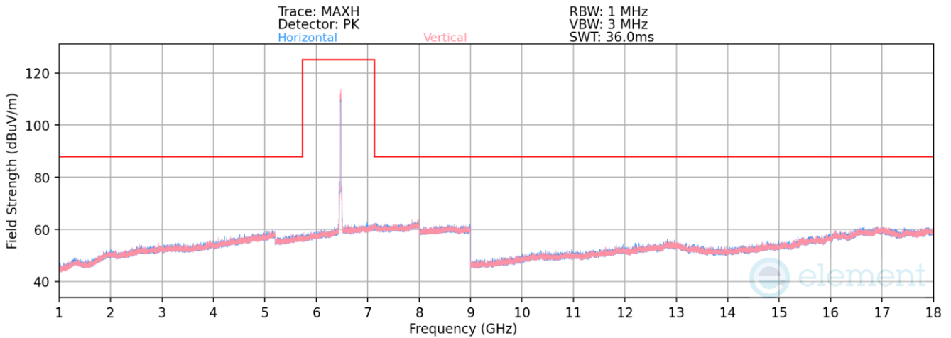
Plot 7-1205. Radiated Spurious Emissions above 1GHz Antenna 4a (802.11ax – Ch. 105, MCS0)
