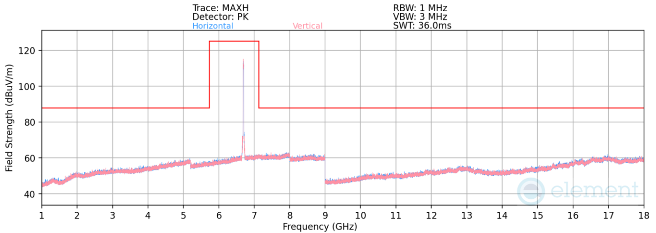
Plot 7-1208. Radiated Spurious Emissions above 1GHz Antenna 4a (802.11ax – Ch. 149, MCS0)
