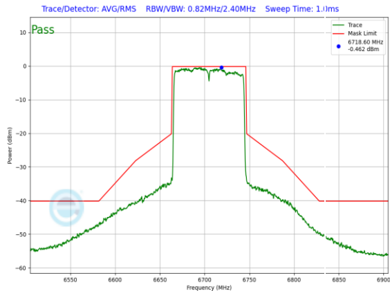
Plot 7-1143. SP In-Band Emission Plot SDM Diversity Antenna 4a (80MHz 802.11ax (UNII Band 7) – Ch. 151, MCS4)
