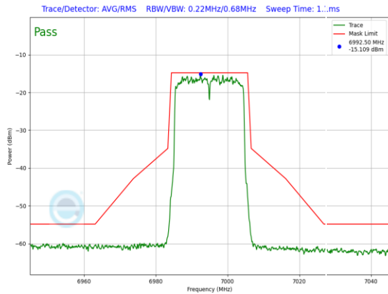
Plot 7-1125. LPI In-Band Emission Plot SDM Diversity Antenna 4a (20MHz 802.11ax (UNII Band 8) – Ch. 209, MCS11)
