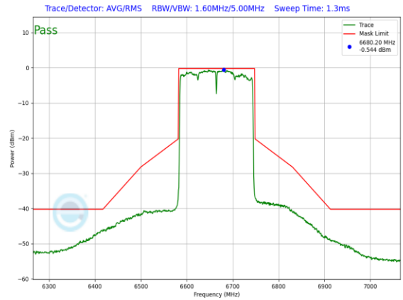
Plot 7-1136. SP In-Band Emission Plot SDM Diversity Antenna 4a (160MHz 802.11ax (UNII Band 7) – Ch. 143, MCS2)
