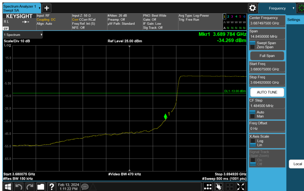
Plot 7-226. Channel Edge Plot (NR Band n48 - 10MHz QPSK - High Channel)
