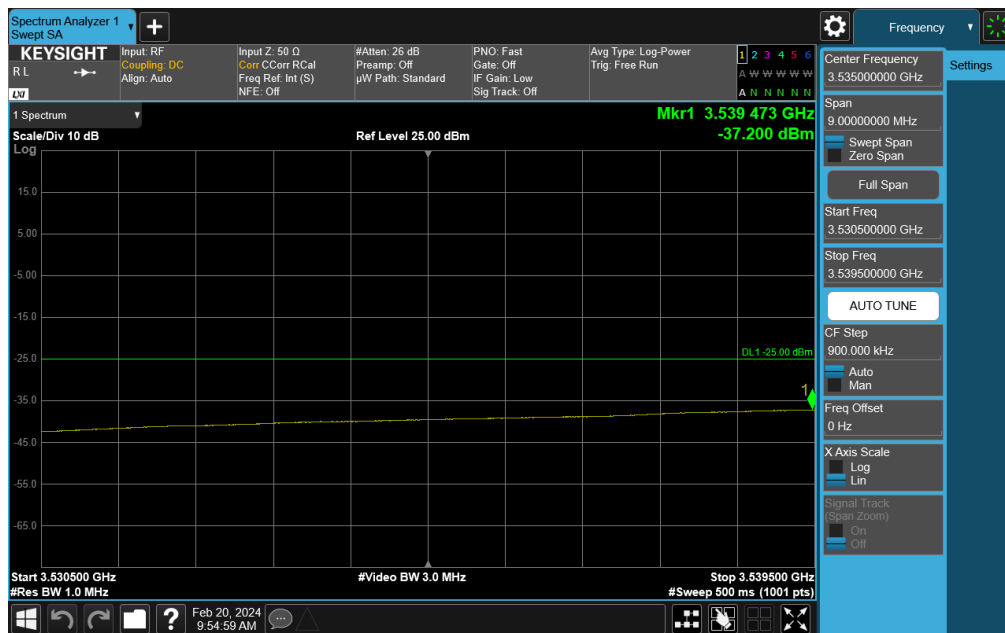
Plot 7-232. Channel Edge Plot (NR Band n48 - 15MHz QPSK - Low Channel)
