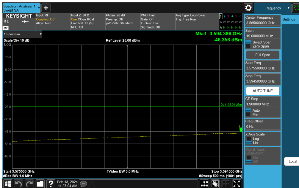
Plot 7-258. Channel Edge Plot (NR Band n48 - 20MHz QPSK - Mid Channel)
