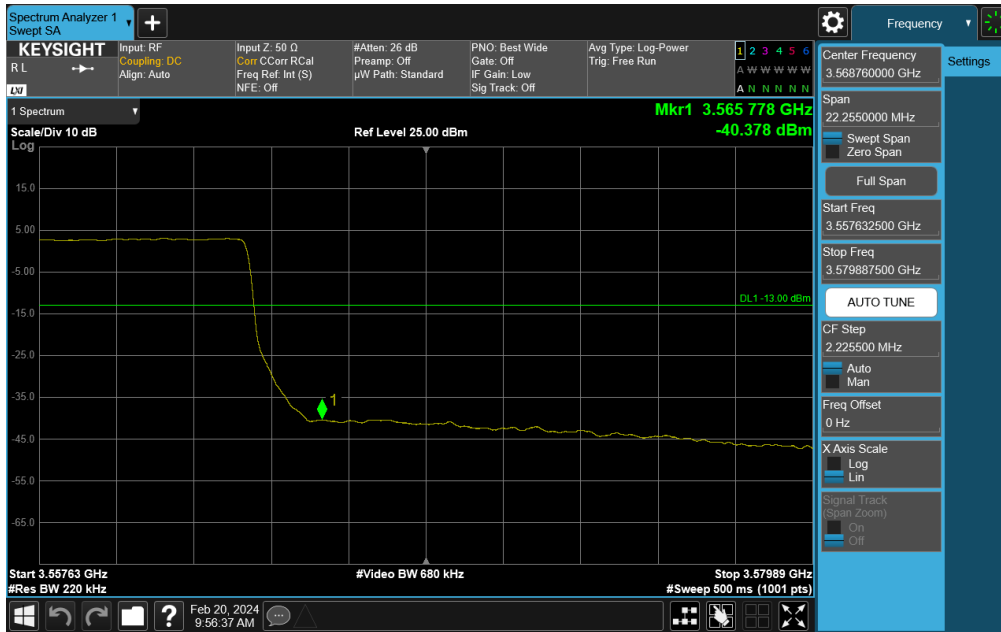
Plot 7-235. Channel Edge Plot (NR Band n48 - 15MHz QPSK - Low Channel)
