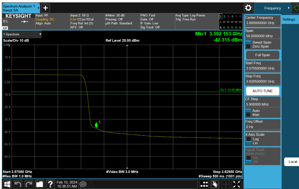
Plot 7-296. Channel Edge Plot (NR Band n48 - 40MHz QPSK - Low Channel)
