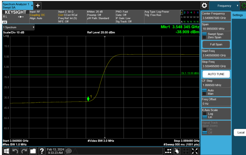
Plot 7-253. Channel Edge Plot (NR Band n48 - 20MHz QPSK - Low Channel)
