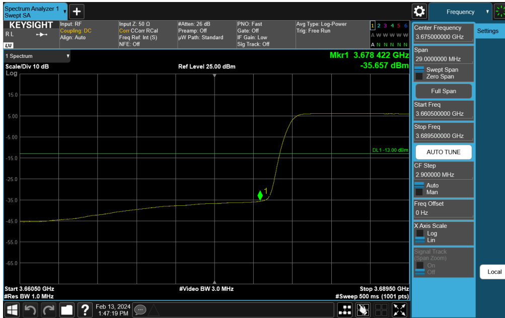
Plot 7-265. Channel Edge Plot (NR Band n48 - 20MHz QPSK - High Channel)
