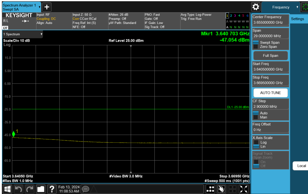
Plot 7-223. Channel Edge Plot (NR Band n48 - 10MHz QPSK - Mid Channel)
