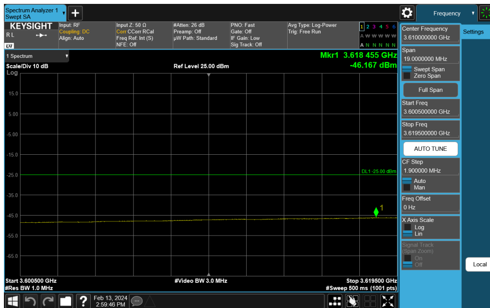
Plot 7-304. Channel Edge Plot (NR Band n48 - 40MHz QPSK - High Channel)
