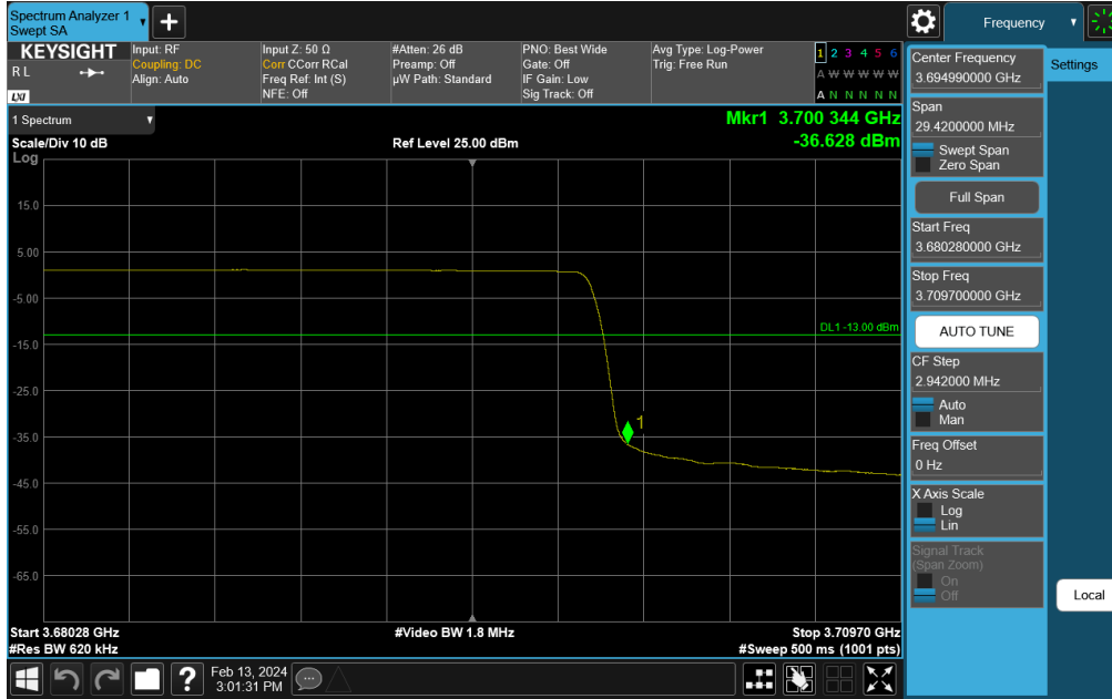
Plot 7-307. Channel Edge Plot (NR Band n48 - 40MHz QPSK - High Channel)
