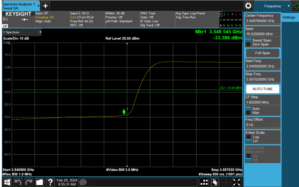
Plot 7-233. Channel Edge Plot (NR Band n48 - 15MHz QPSK - Low Channel)
