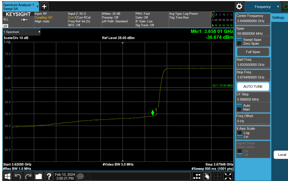
Plot 7-305. Channel Edge Plot (NR Band n48 - 40MHz QPSK - High Channel)
