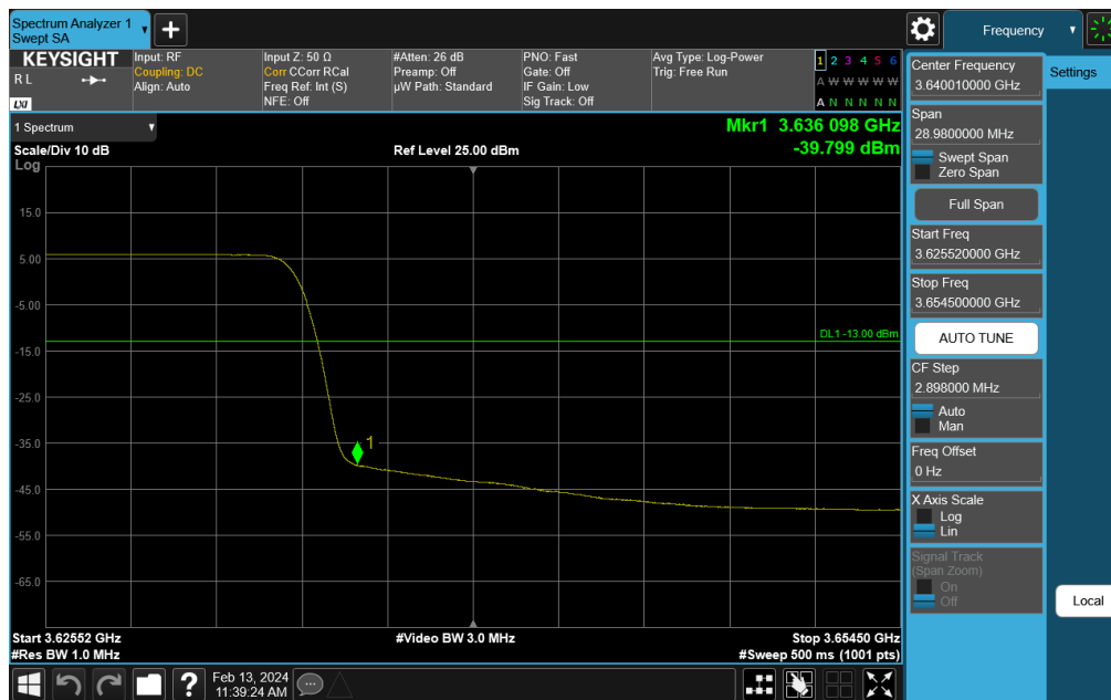
Plot 7-262. Channel Edge Plot (NR Band n48 - 20MHz QPSK - Mid Channel)
