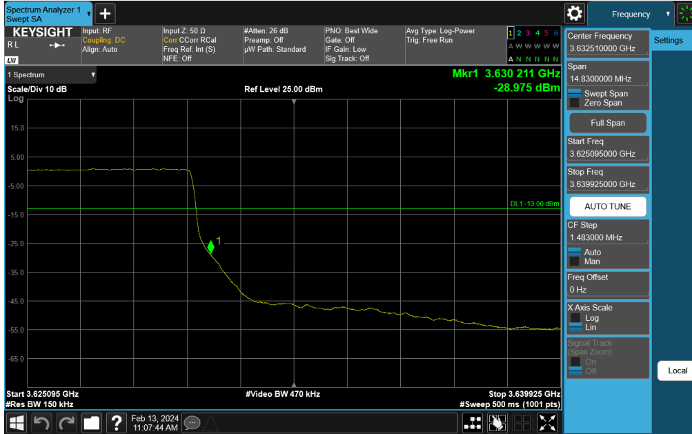
Plot 7-221. Channel Edge Plot (NR Band n48 - 10MHz QPSK - Mid Channel)
