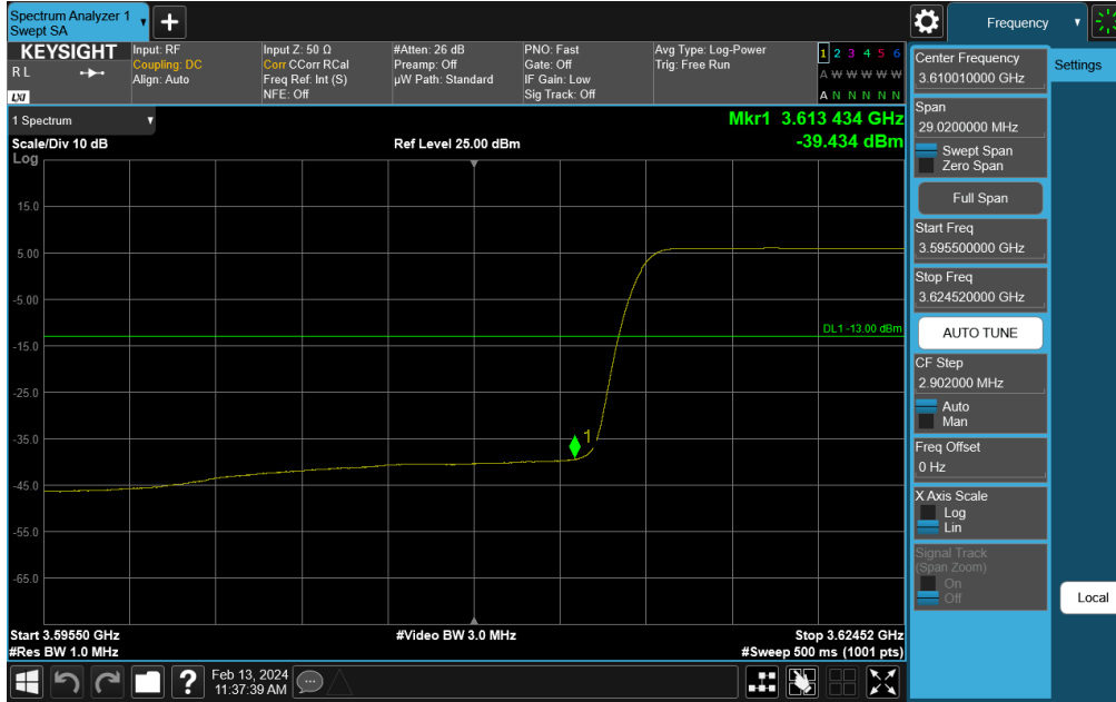
Plot 7-259. Channel Edge Plot (NR Band n48 - 20MHz QPSK - Mid Channel)
