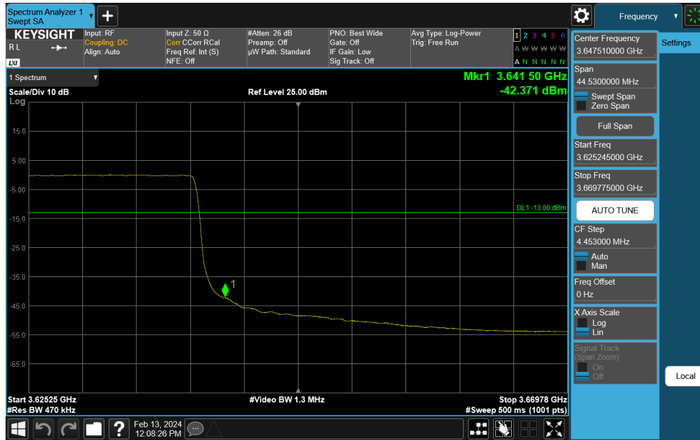
Plot 7-281. Channel Edge Plot (NR Band n48 - 30MHz QPSK - Mid Channel)
