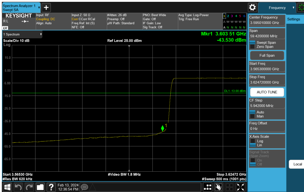
Plot 7-300. Channel Edge Plot (NR Band n48 - 40MHz QPSK - Mid Channel)
