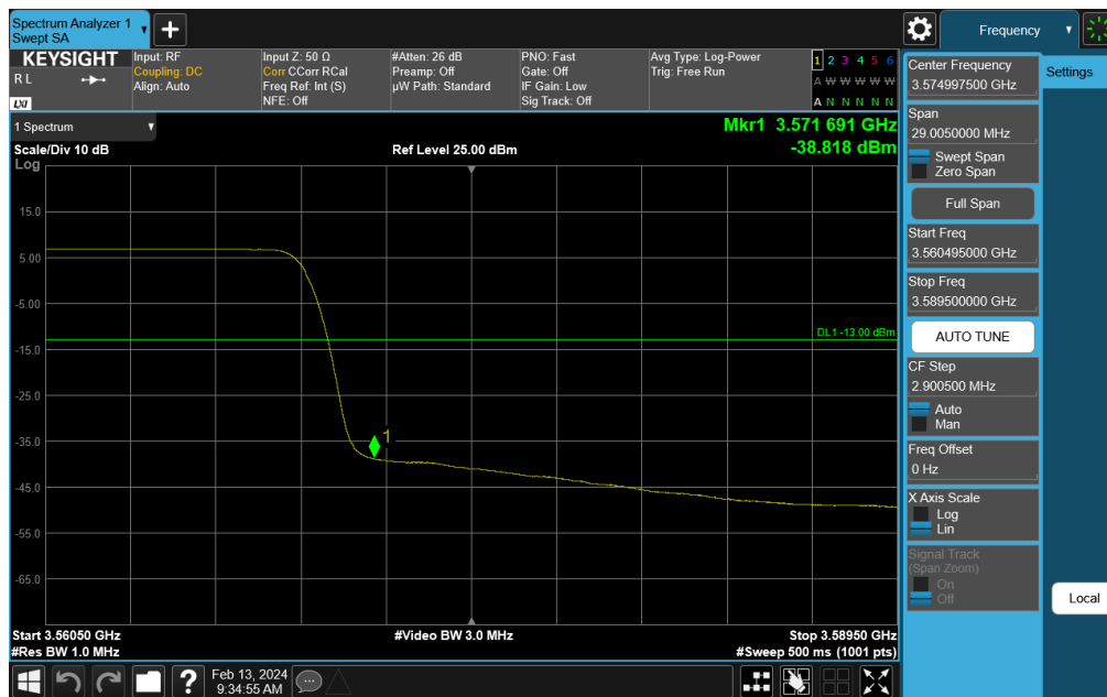
Plot 7-256. Channel Edge Plot (NR Band n48 - 20MHz QPSK - Low Channel)
