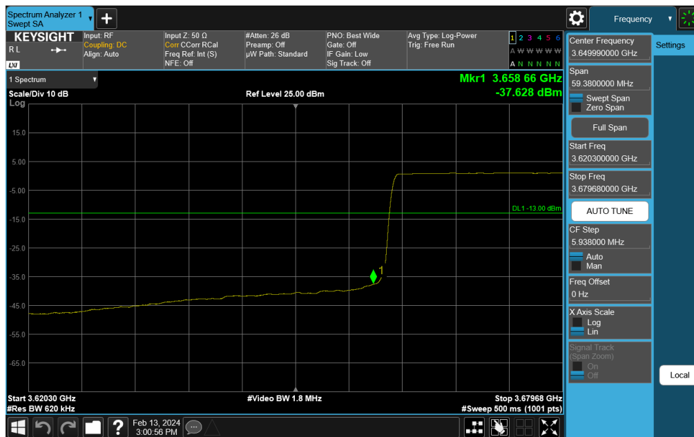
Plot 7-306. Channel Edge Plot (NR Band n48 - 40MHz QPSK - High Channel)
