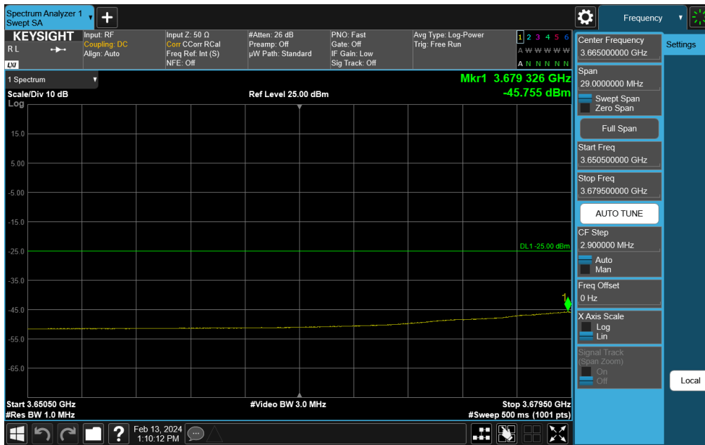
Plot 7-224. Channel Edge Plot (NR Band n48 - 10MHz QPSK - High Channel)
