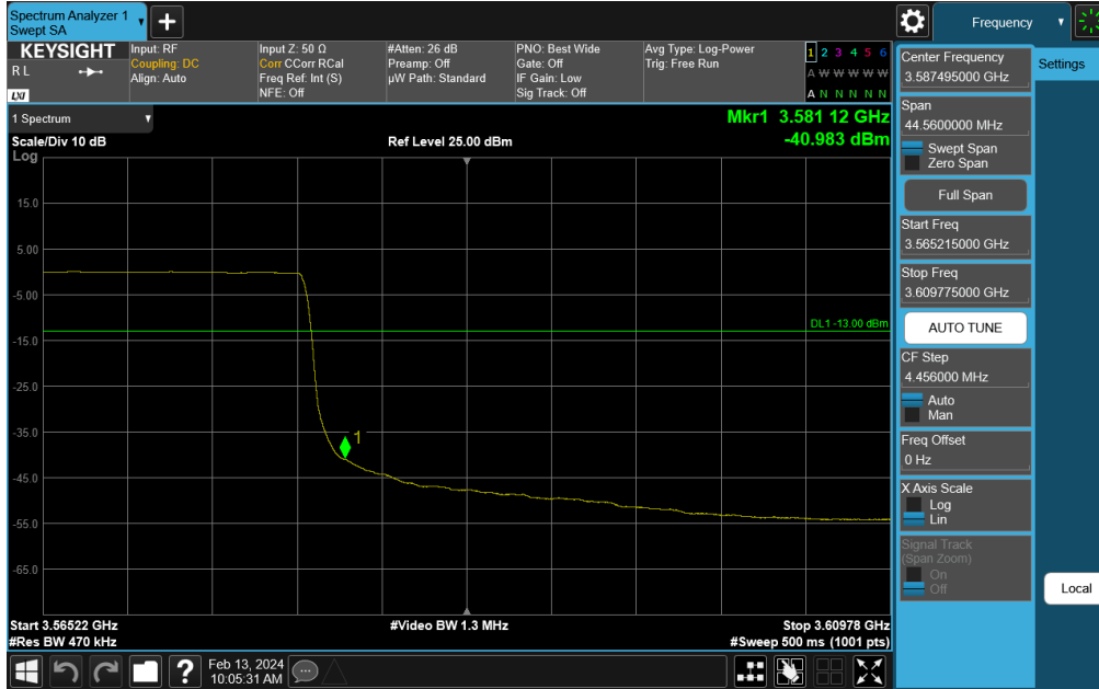
Plot 7-275. Channel Edge Plot (NR Band n48 - 30MHz QPSK - Low Channel)
