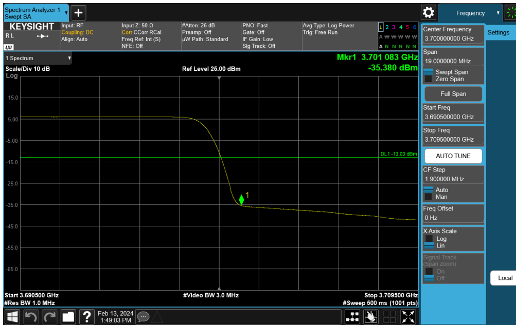
Plot 7-268. Channel Edge Plot (NR Band n48 - 20MHz QPSK - High Channel)
