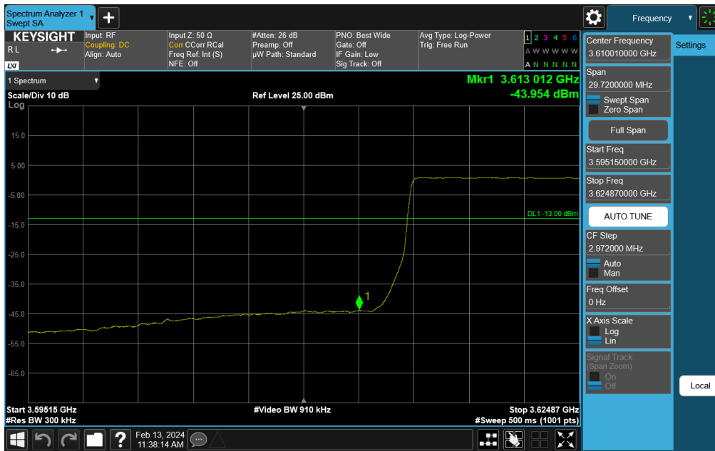
Plot 7-260. Channel Edge Plot (NR Band n48 - 20MHz QPSK - Mid Channel)
