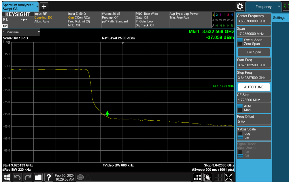
Plot 7-241. Channel Edge Plot (NR Band n48 - 15MHz QPSK - Mid Channel)
