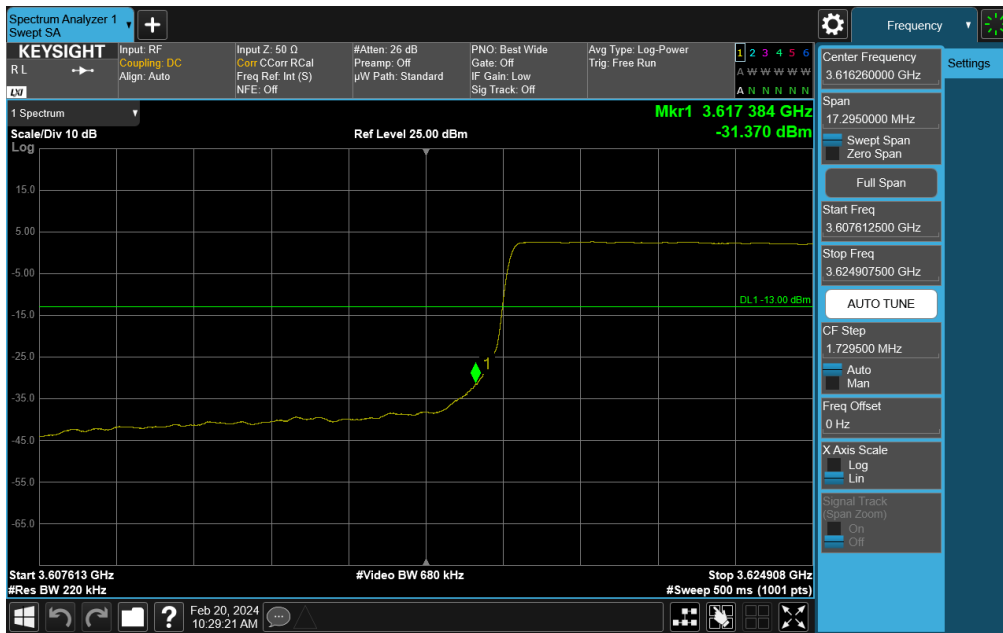
Plot 7-240. Channel Edge Plot (NR Band n48 - 15MHz QPSK - Mid Channel)
