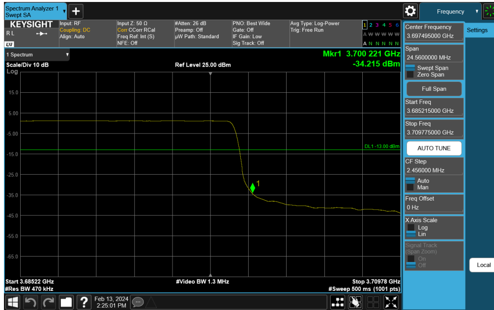
Plot 7-287. Channel Edge Plot (NR Band n48 - 30MHz QPSK - High Channel)
