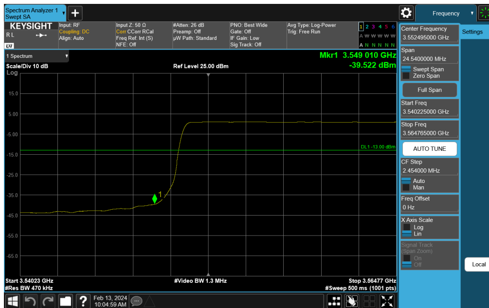
Plot 7-274. Channel Edge Plot (NR Band n48 - 30MHz QPSK - Low Channel)
