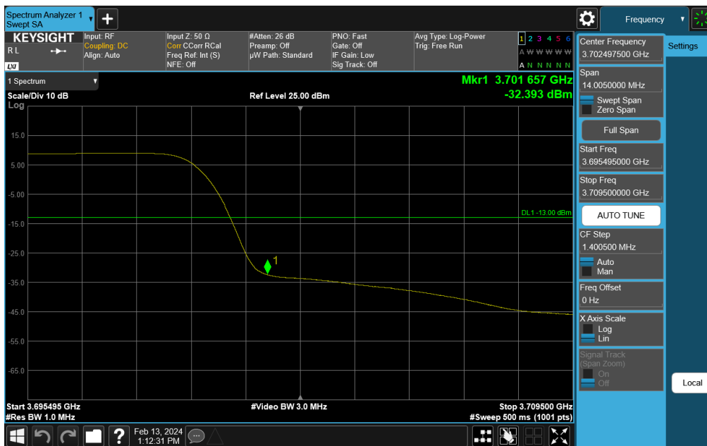
Plot 7-228. Channel Edge Plot (NR Band n48 - 10MHz QPSK - High Channel)
