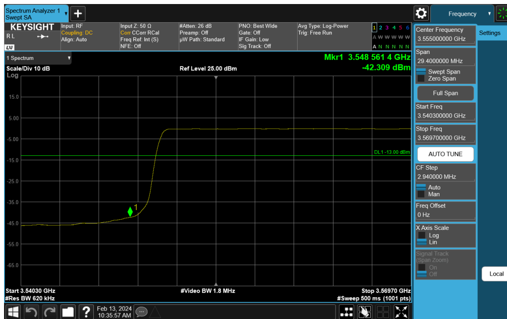
Plot 7-294. Channel Edge Plot (NR Band n48 - 40MHz QPSK - Low Channel)
