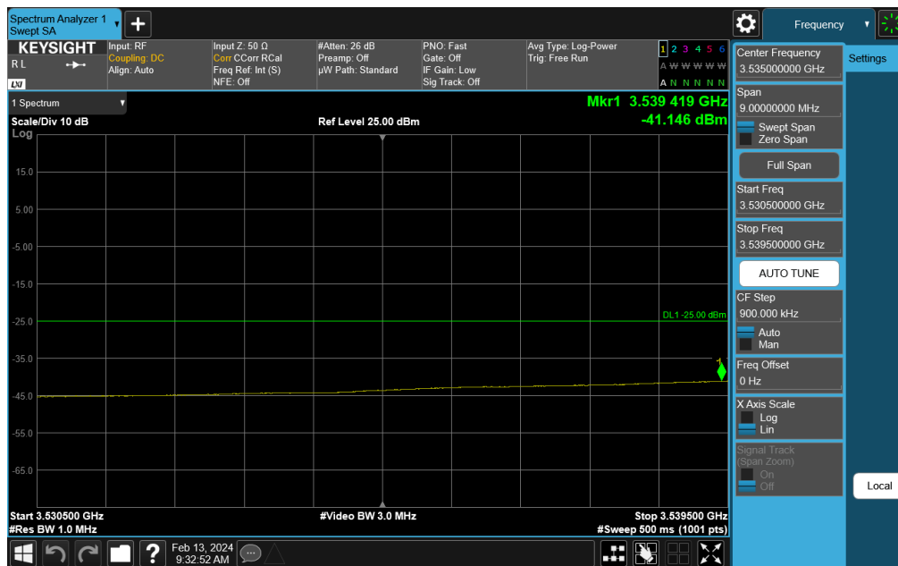
Plot 7-252. Channel Edge Plot (NR Band n48 - 20MHz QPSK - Low Channel)
