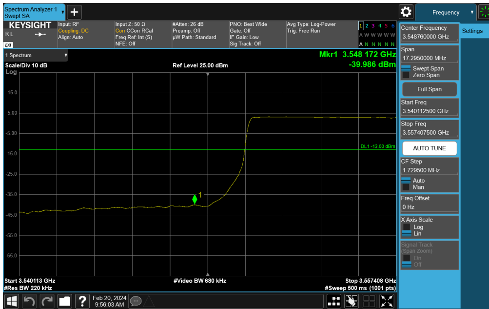
Plot 7-234. Channel Edge Plot (NR Band n48 - 15MHz QPSK - Low Channel)
