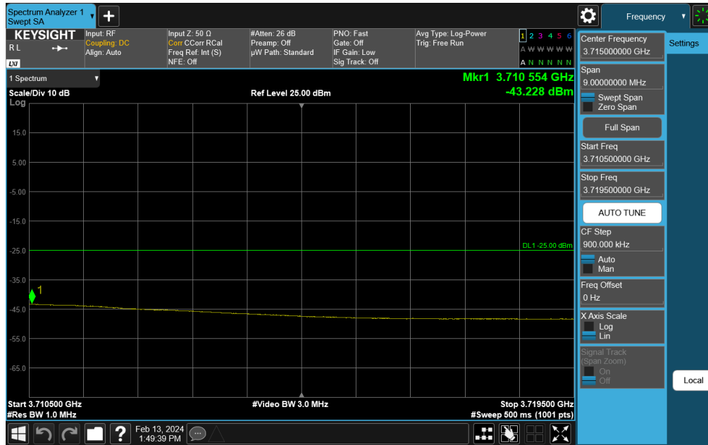
Plot 7-269. Channel Edge Plot (NR Band n48 - 20MHz QPSK - High Channel)
