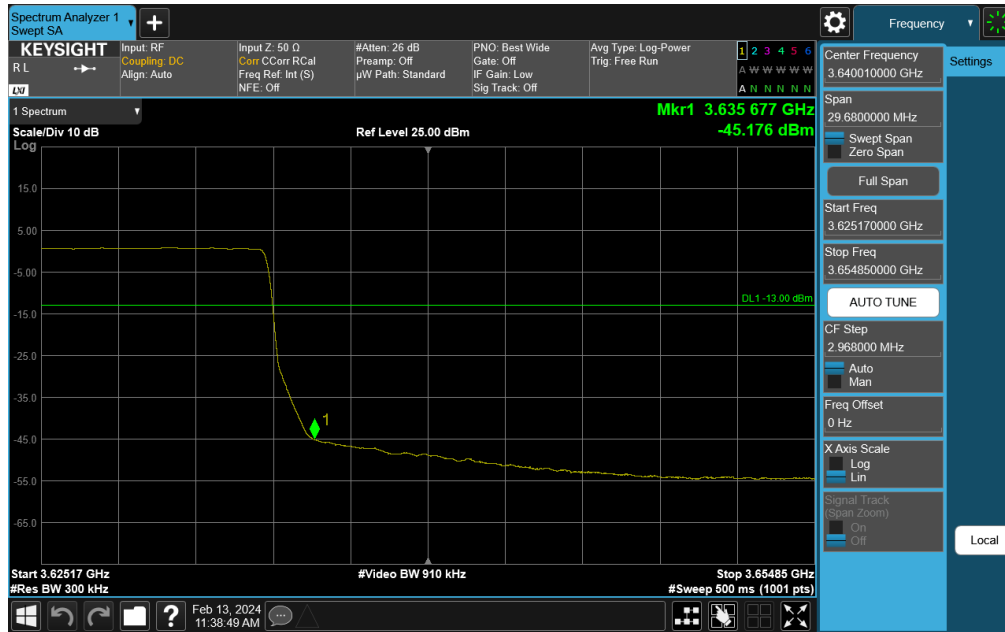
Plot 7-261. Channel Edge Plot (NR Band n48 - 20MHz QPSK - Mid Channel)
