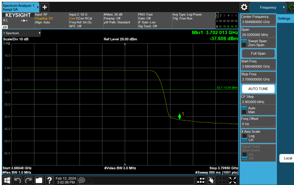
Plot 7-308. Channel Edge Plot (NR Band n48 - 40MHz QPSK - High Channel)
