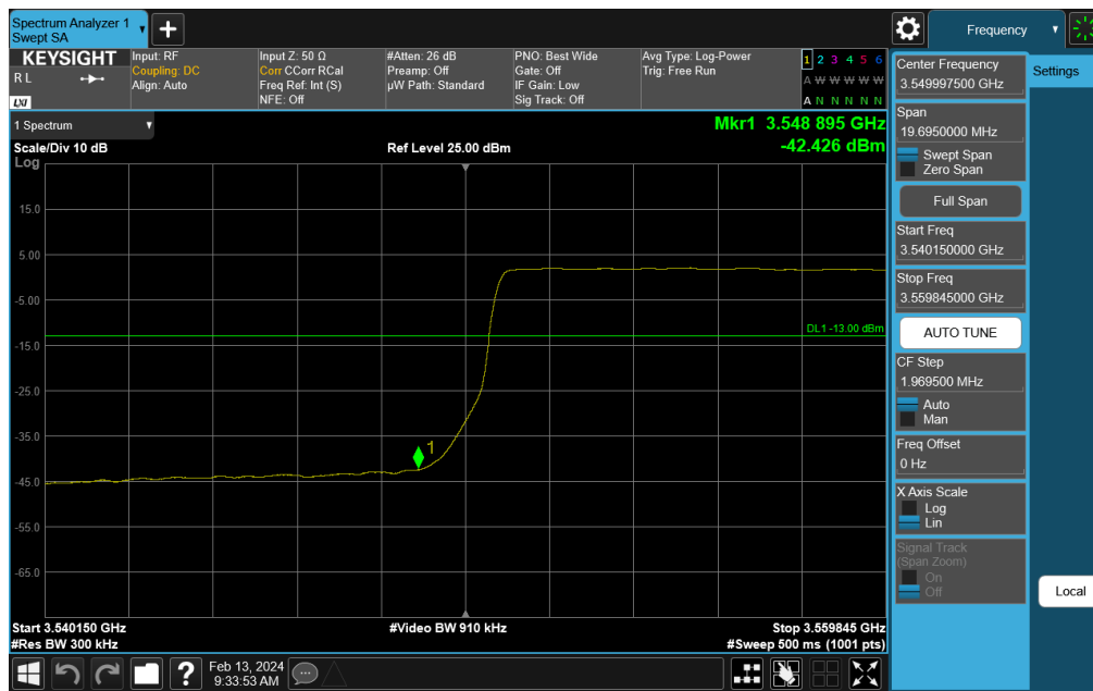
Plot 7-254. Channel Edge Plot (NR Band n48 - 20MHz QPSK - Low Channel)
