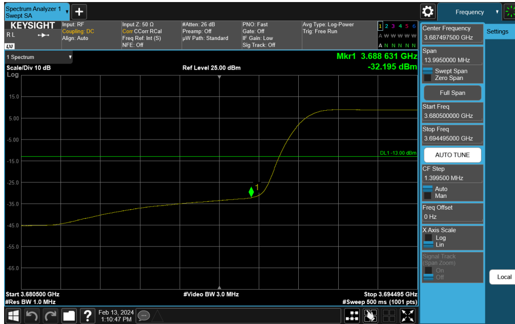
Plot 7-225. Channel Edge Plot (NR Band n48 - 10MHz QPSK - High Channel)
