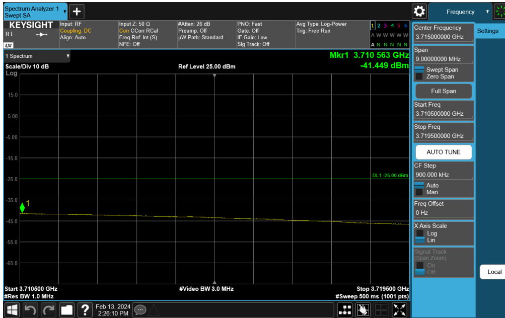
Plot 7-289. Channel Edge Plot (NR Band n48 - 30MHz QPSK - High Channel)
