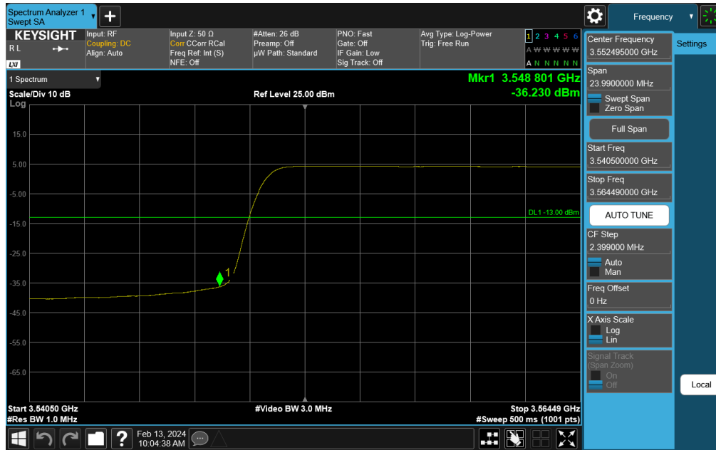
Plot 7-273. Channel Edge Plot (NR Band n48 - 30MHz QPSK - Low Channel)
