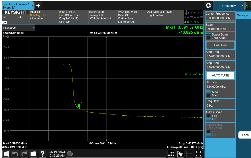
Plot 7-295. Channel Edge Plot (NR Band n48 - 40MHz QPSK - Low Channel)
