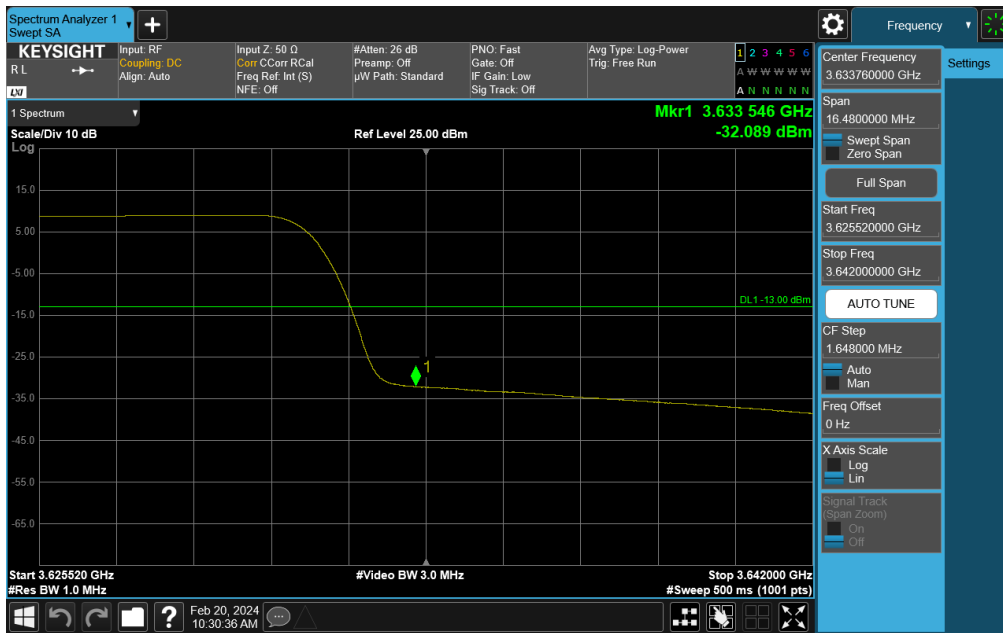
Plot 7-242. Channel Edge Plot (NR Band n48 - 15MHz QPSK - Mid Channel)
