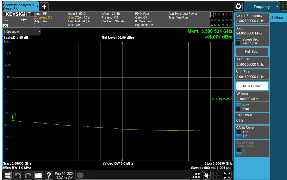
Plot 7-237. Channel Edge Plot (NR Band n48 - 15MHz QPSK - Low Channel)
