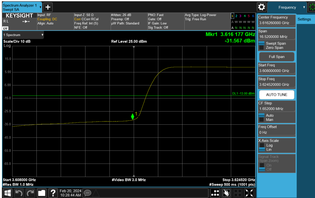
Plot 7-239. Channel Edge Plot (NR Band n48 - 15MHz QPSK - Mid Channel)
