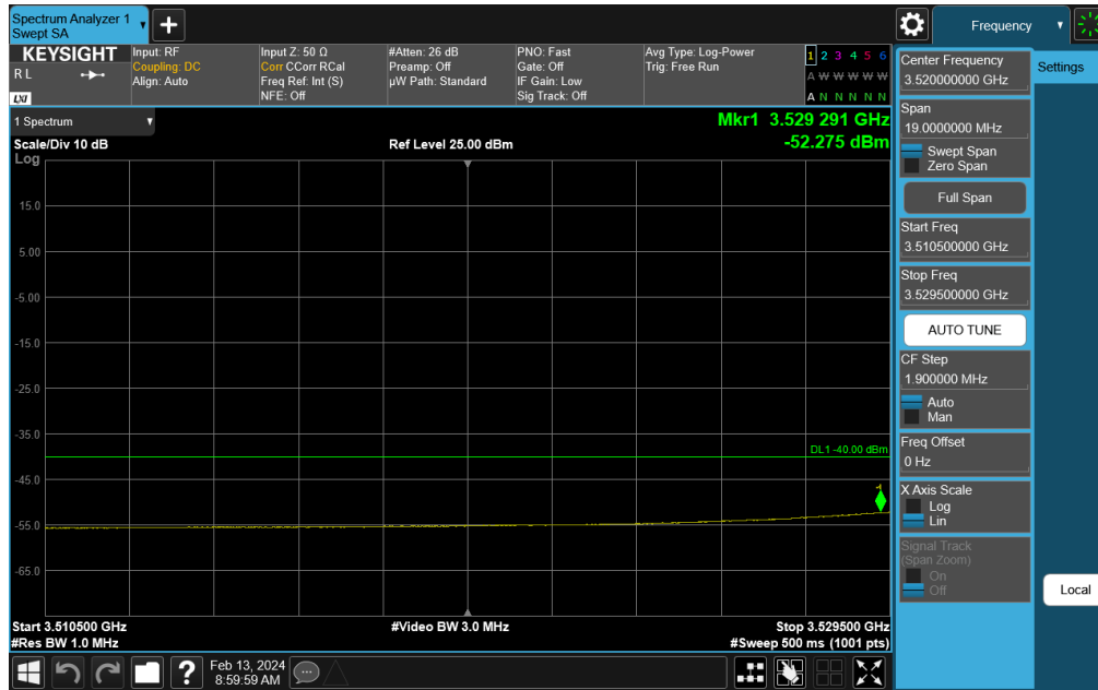
Plot 7-231. Channel Edge Plot (NR Band n48 - 10MHz QPSK - Low Channel)
