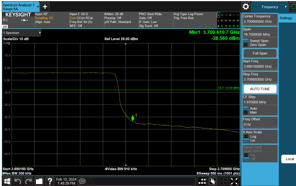
Plot 7-267. Channel Edge Plot (NR Band n48 - 20MHz QPSK - High Channel)
