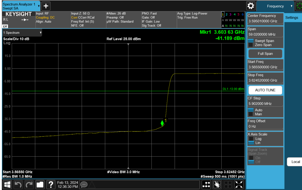
Plot 7-299. Channel Edge Plot (NR Band n48 - 40MHz QPSK - Mid Channel)
