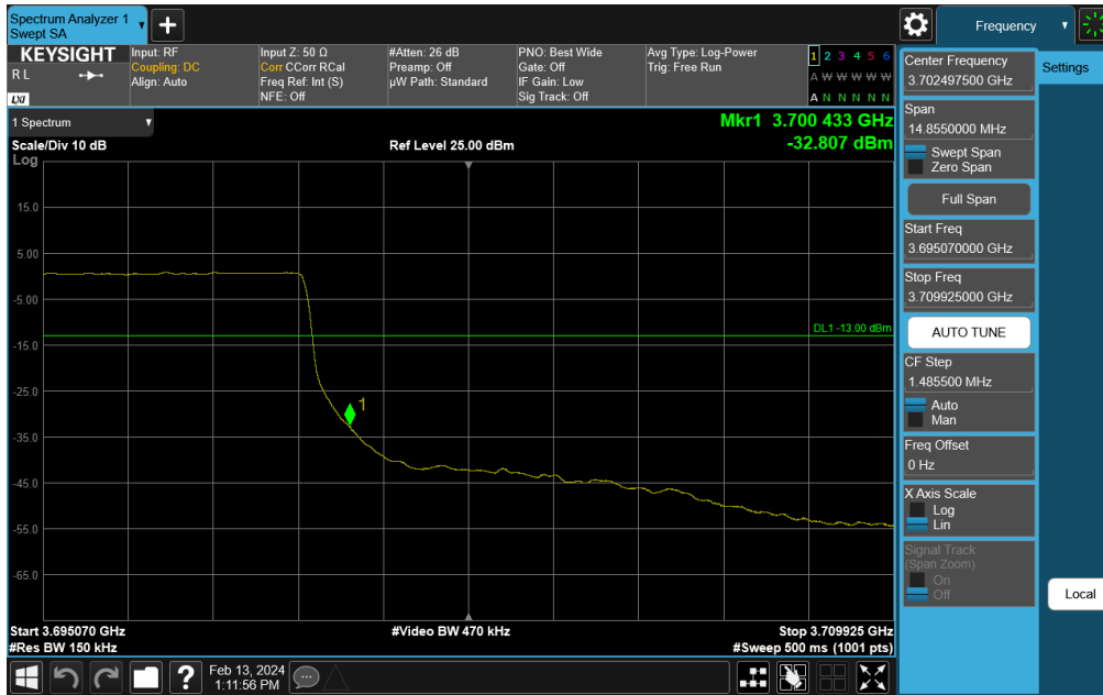
Plot 7-227. Channel Edge Plot (NR Band n48 - 10MHz QPSK - High Channel)
