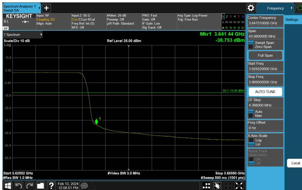
Plot 7-282. Channel Edge Plot (NR Band n48 - 30MHz QPSK - Mid Channel)
