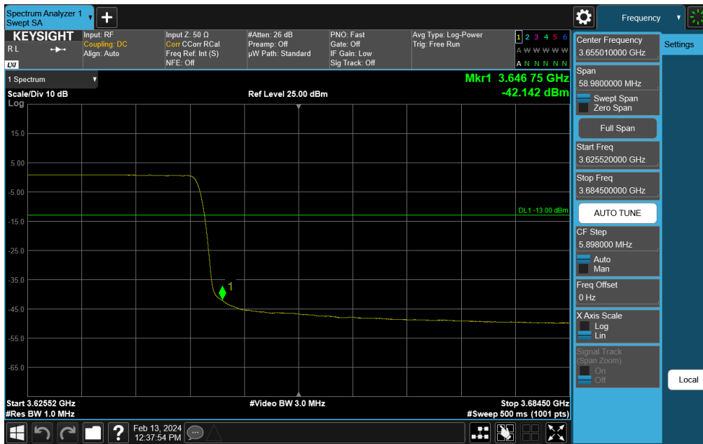
Plot 7-302. Channel Edge Plot (NR Band n48 - 40MHz QPSK - Mid Channel)
