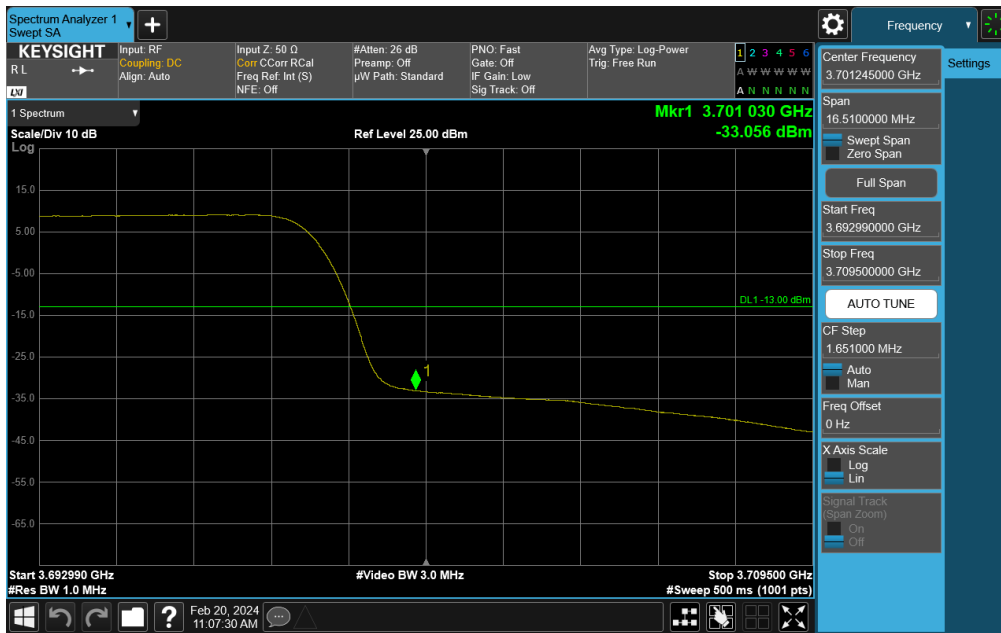
Plot 7-248. Channel Edge Plot (NR Band n48 - 15MHz QPSK - High Channel)
