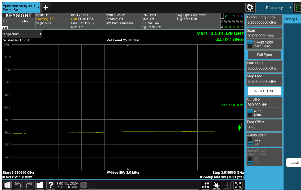
Plot 7-292. Channel Edge Plot (NR Band n48 - 40MHz QPSK - Low Channel)
