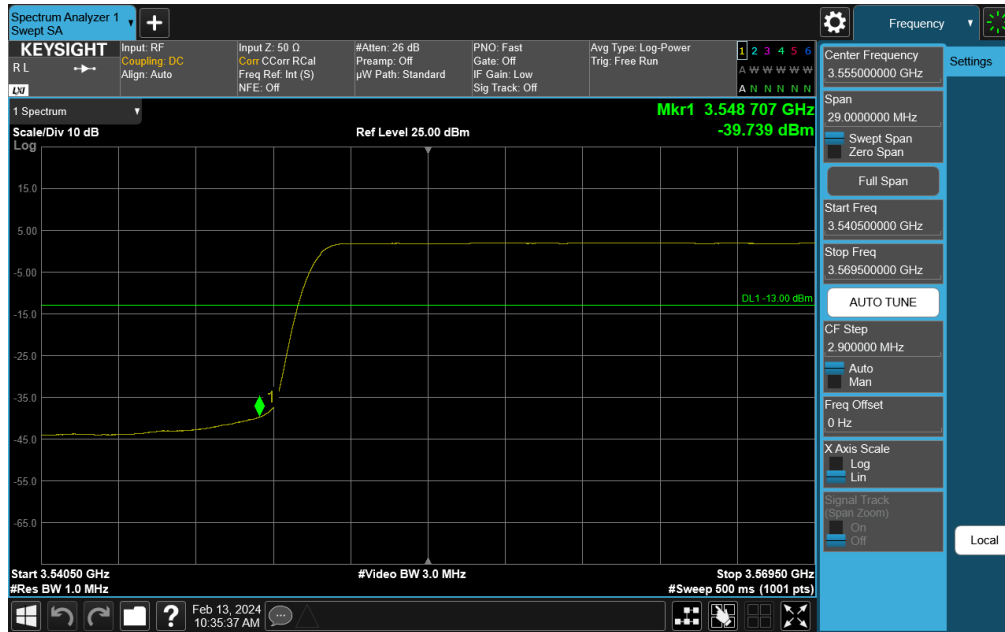
Plot 7-293. Channel Edge Plot (NR Band n48 - 40MHz QPSK - Low Channel)
