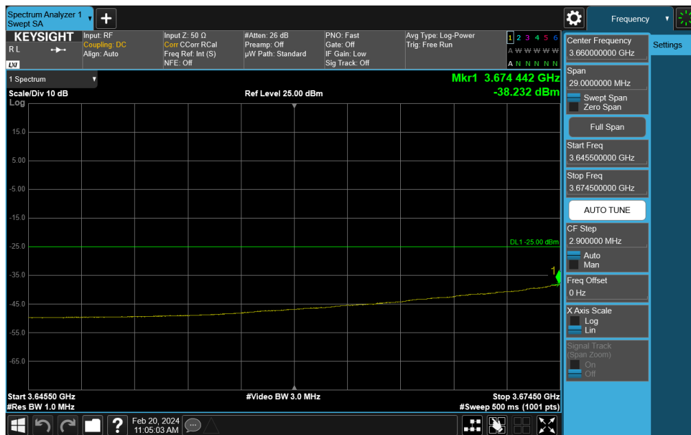
Plot 7-244. Channel Edge Plot (NR Band n48 - 15MHz QPSK - High Channel)
