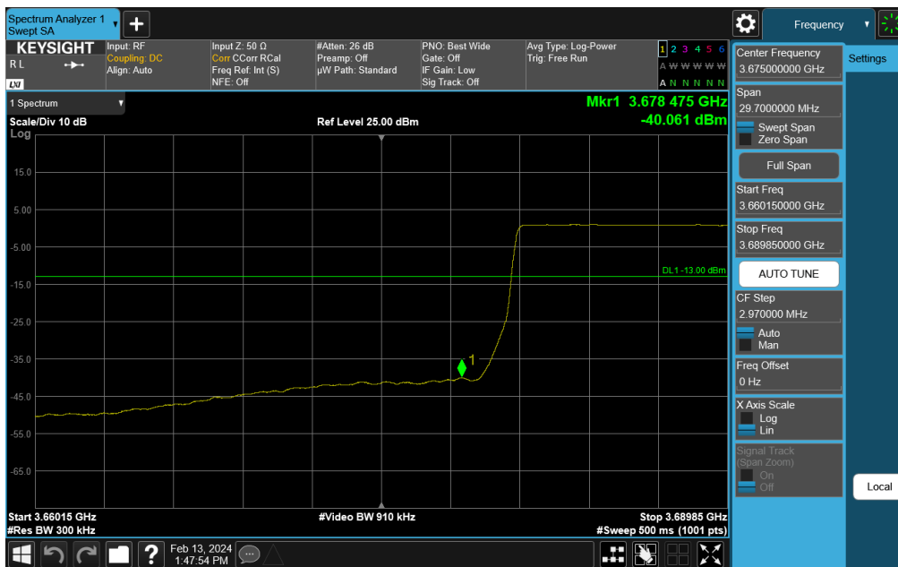
Plot 7-266. Channel Edge Plot (NR Band n48 - 20MHz QPSK - High Channel)
