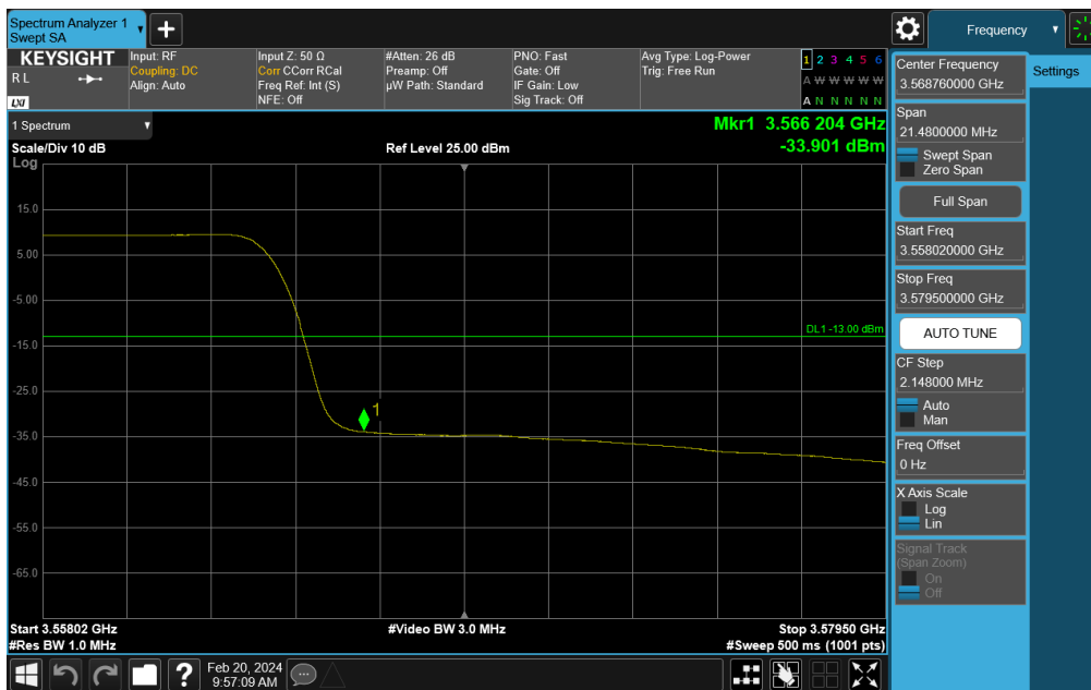
Plot 7-236. Channel Edge Plot (NR Band n48 - 15MHz QPSK - Low Channel)
