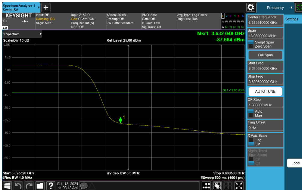
Plot 7-222. Channel Edge Plot (NR Band n48 - 10MHz QPSK - Mid Channel)
