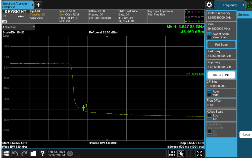
Plot 7-301. Channel Edge Plot (NR Band n48 - 40MHz QPSK - Mid Channel)
