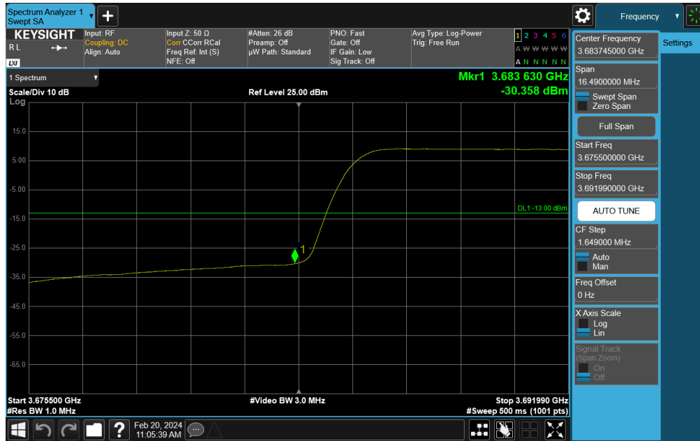
Plot 7-245. Channel Edge Plot (NR Band n48 - 15MHz QPSK - High Channel)
