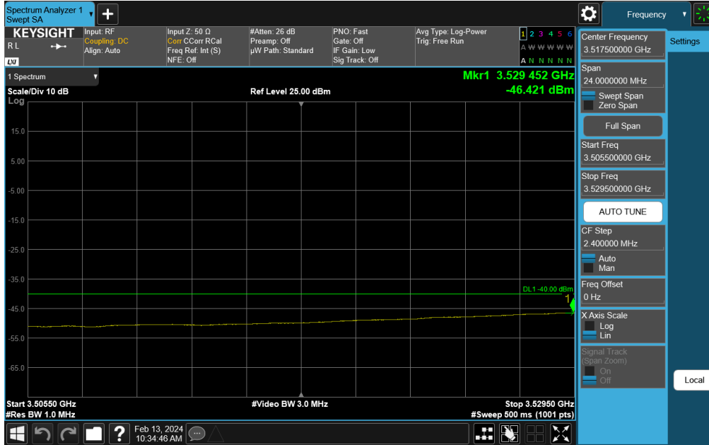
Plot 7-291. Channel Edge Plot (NR Band n48 - 40MHz QPSK - Low Channel)
