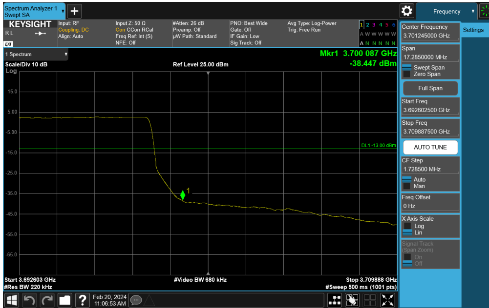
Plot 7-247. Channel Edge Plot (NR Band n48 - 15MHz QPSK - High Channel)
