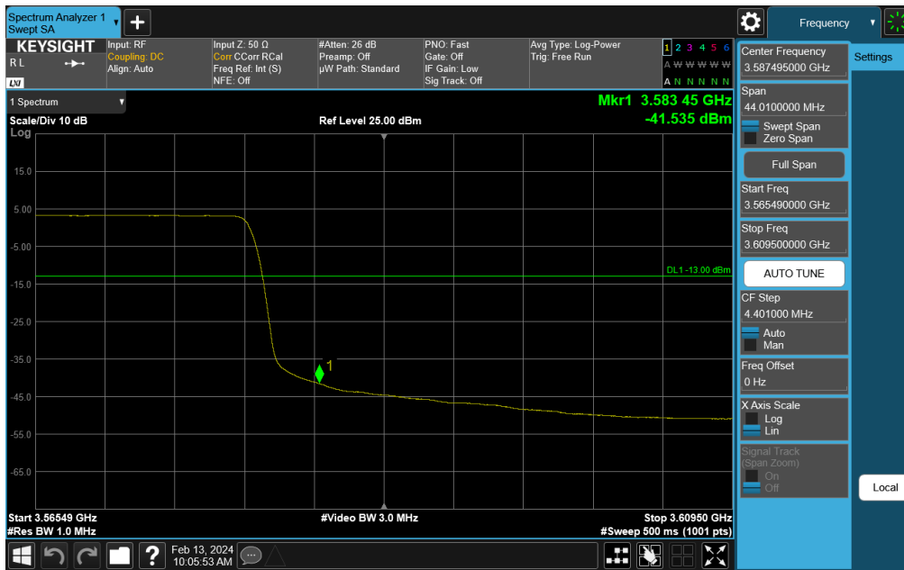
Plot 7-276. Channel Edge Plot (NR Band n48 - 30MHz QPSK - Low Channel)
