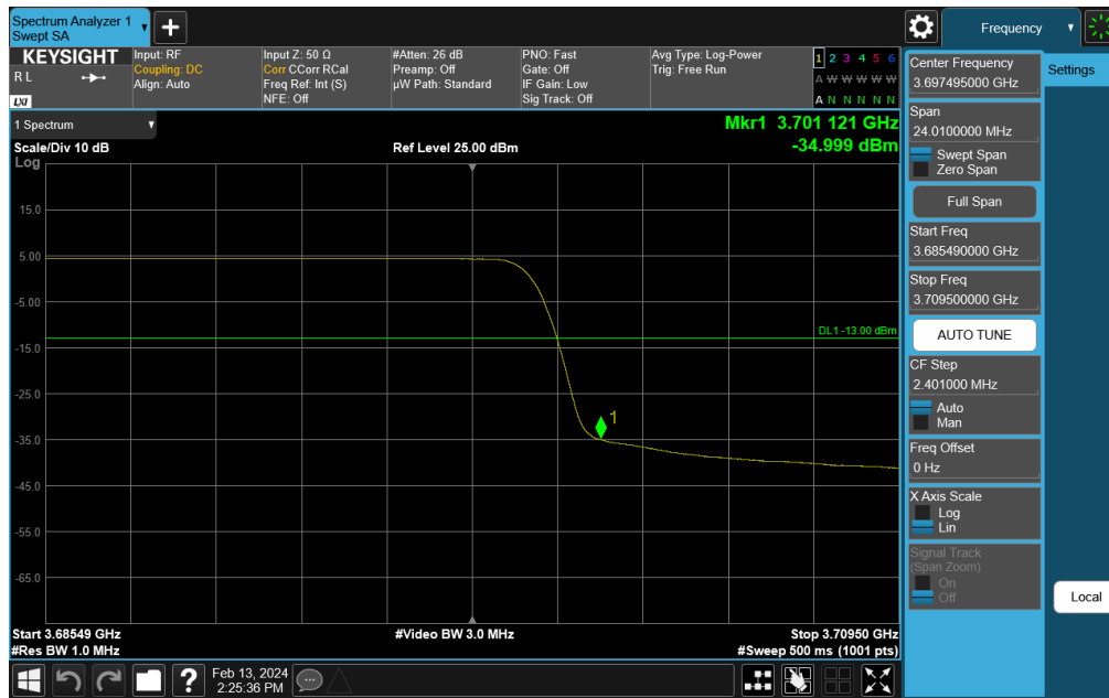
Plot 7-288. Channel Edge Plot (NR Band n48 - 30MHz QPSK - High Channel)
