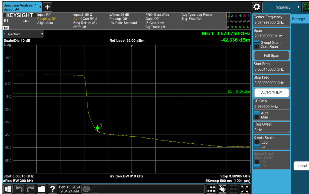
Plot 7-255. Channel Edge Plot (NR Band n48 - 20MHz QPSK - Low Channel)
