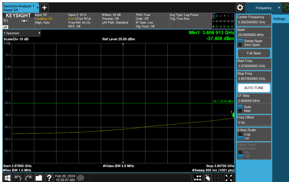
Plot 7-238. Channel Edge Plot (NR Band n48 - 15MHz QPSK - Mid Channel)
