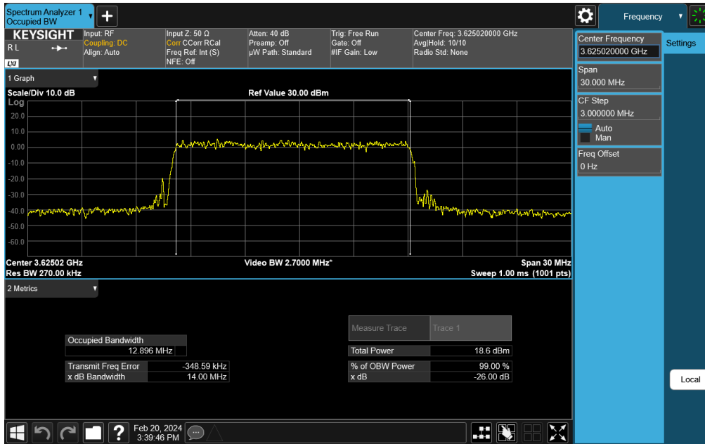
Plot 7-41. Occupied Bandwidth Plot (NR Band n48 - 15MHz 64-QAM - Full RB Configuration)
