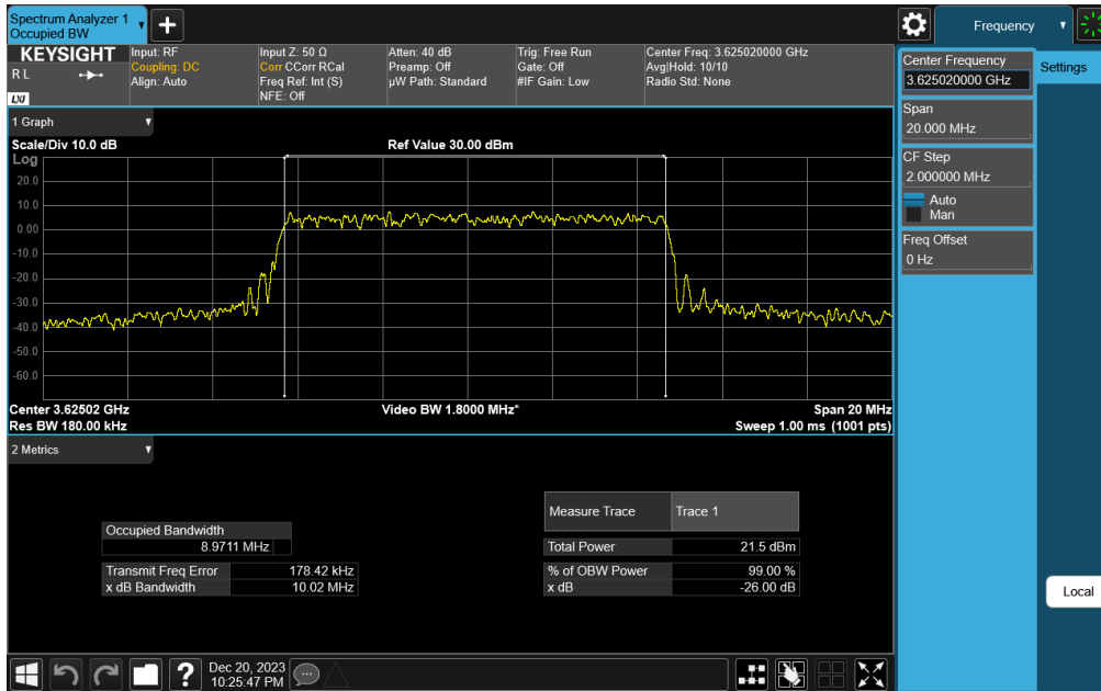
Plot 7-34. Occupied Bandwidth Plot (NR Band n48 - 10MHz QPSK - Full RB Configuration)
