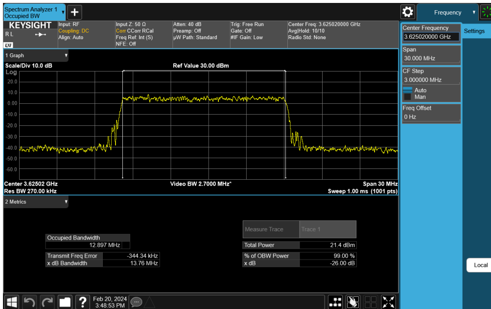
Plot 7-38. Occupied Bandwidth Plot (NR Band n48 - 15MHz \pi/2 BPSK - Full RB Configuration)
