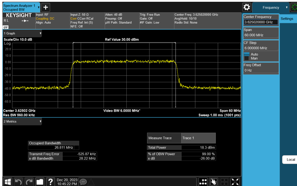
Plot 7-48. Occupied Bandwidth Plot (NR Band n48 - 30MHz \pi/2 BPSK - Full RB Configuration)
