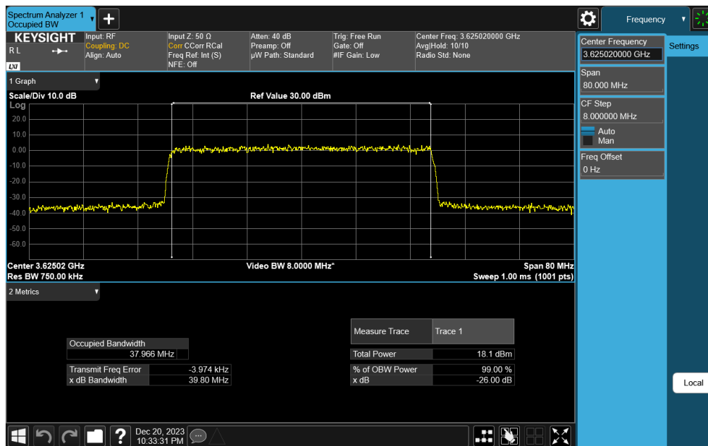
Plot 7-54. Occupied Bandwidth Plot (NR Band n48 - 40MHz QPSK - Full RB Configuration)
