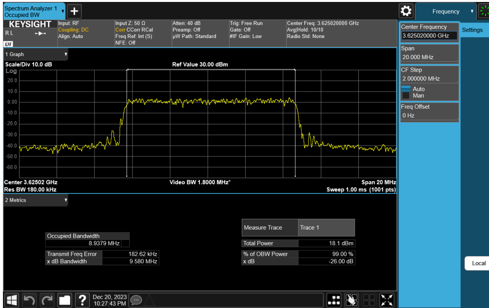
Plot 7-37. Occupied Bandwidth Plot (NR Band n48 - 10MHz 256-QAM - Full RB Configuration)
