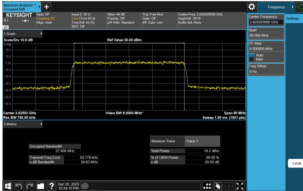
Plot 7-55. Occupied Bandwidth Plot (NR Band n48 - 40MHz 16-QAM - Full RB Configuration)
