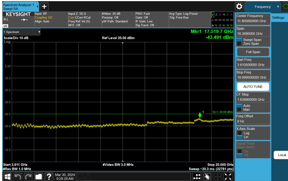
Plot 7-83. Conducted Spurious Plot (NR Band n48 - 40MHz QPSK - Low Channel)
