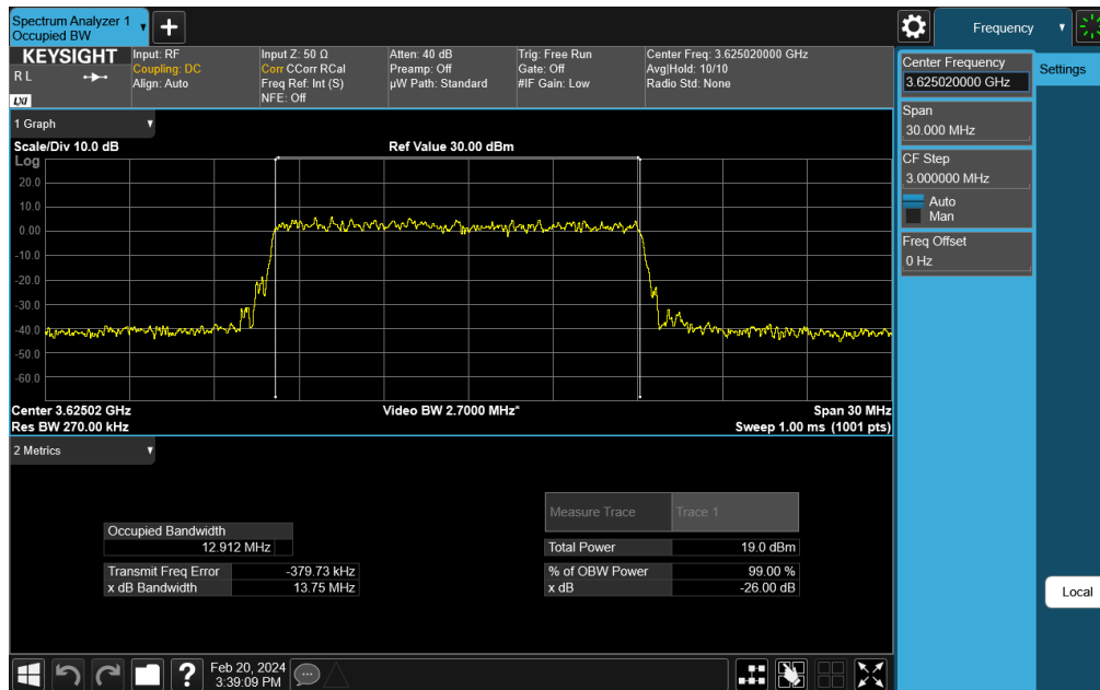
Plot 7-40. Occupied Bandwidth Plot (NR Band n48 - 15MHz 16-QAM - Full RB Configuration)
