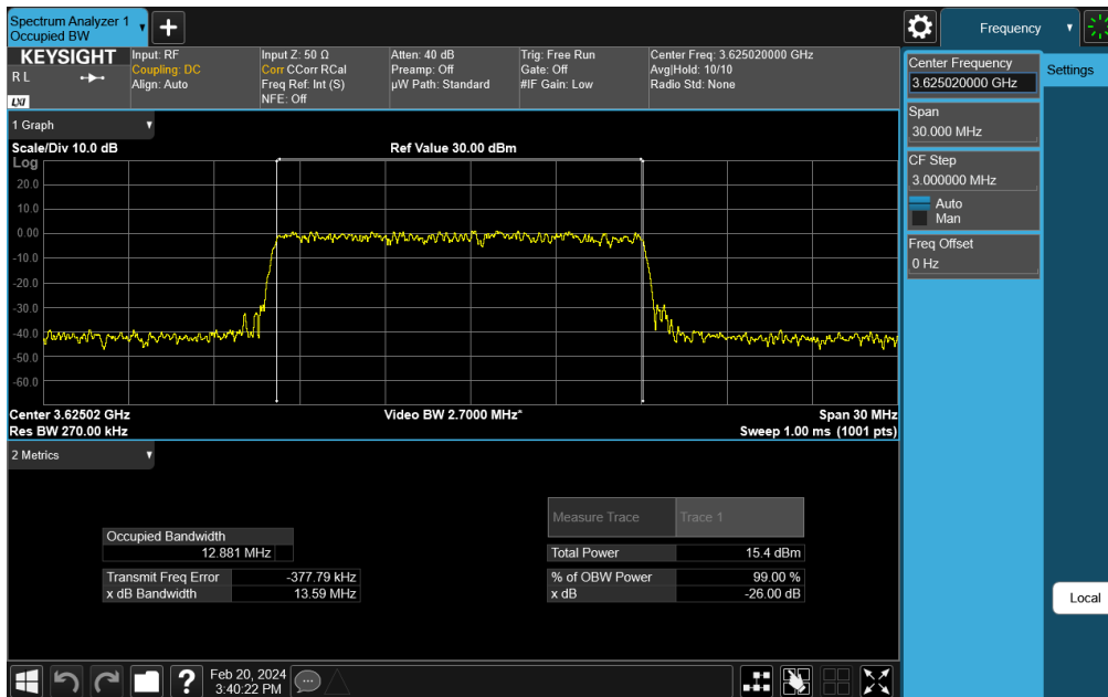
Plot 7-42. Occupied Bandwidth Plot (NR Band n48 - 15MHz 256-QAM - Full RB Configuration)
