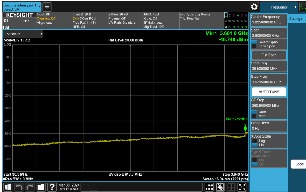
Plot 7-88. Conducted Spurious Plot (NR Band n48 - 40MHz QPSK - High Channel)
