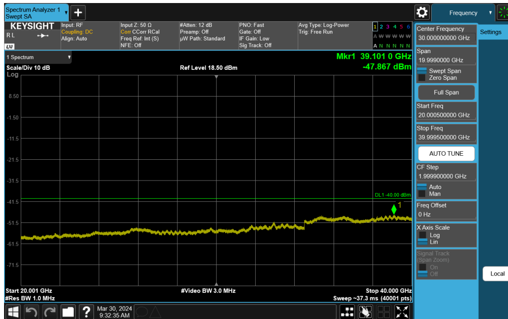
Plot 7-87. Conducted Spurious Plot (NR Band n48 - 40MHz QPSK - Mid Channel)
