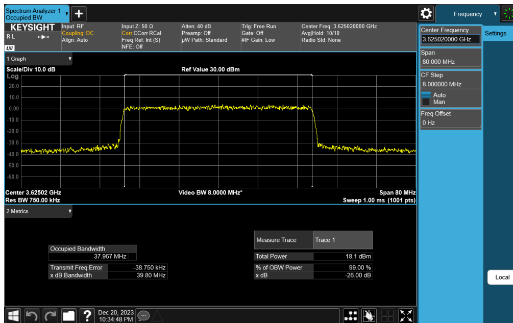
Plot 7-56. Occupied Bandwidth Plot (NR Band n48 - 40MHz 64-QAM - Full RB Configuration)
