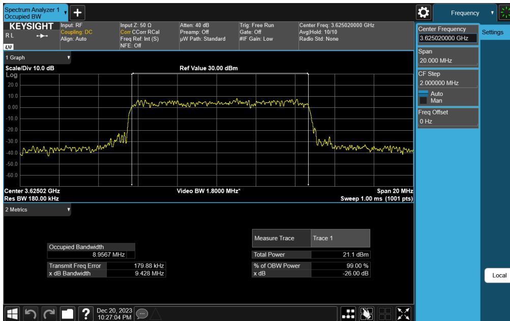
Plot 7-36. Occupied Bandwidth Plot (NR Band n48 - 10MHz 64-QAM - Full RB Configuration)
