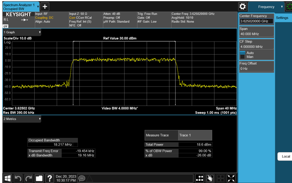
Plot 7-47. Occupied Bandwidth Plot (NR Band n48 - 20MHz 256-QAM - Full RB Configuration)
