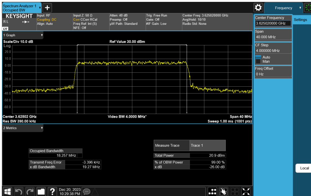
Plot 7-46. Occupied Bandwidth Plot (NR Band n48 - 20MHz 64-QAM - Full RB Configuration)
