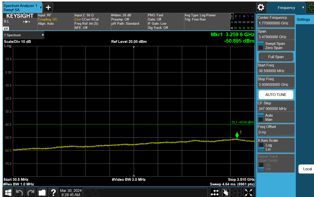
Plot 7-82. Conducted Spurious Plot (NR Band n48 - 40MHz QPSK - Low Channel)
