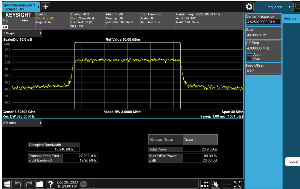
Plot 7-45. Occupied Bandwidth Plot (NR Band n48 - 20MHz 16-QAM - Full RB Configuration)
