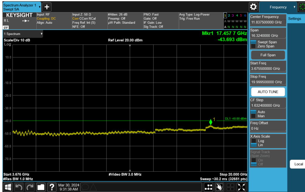
Plot 7-86. Conducted Spurious Plot (NR Band n48 - 40MHz QPSK - Mid Channel)
