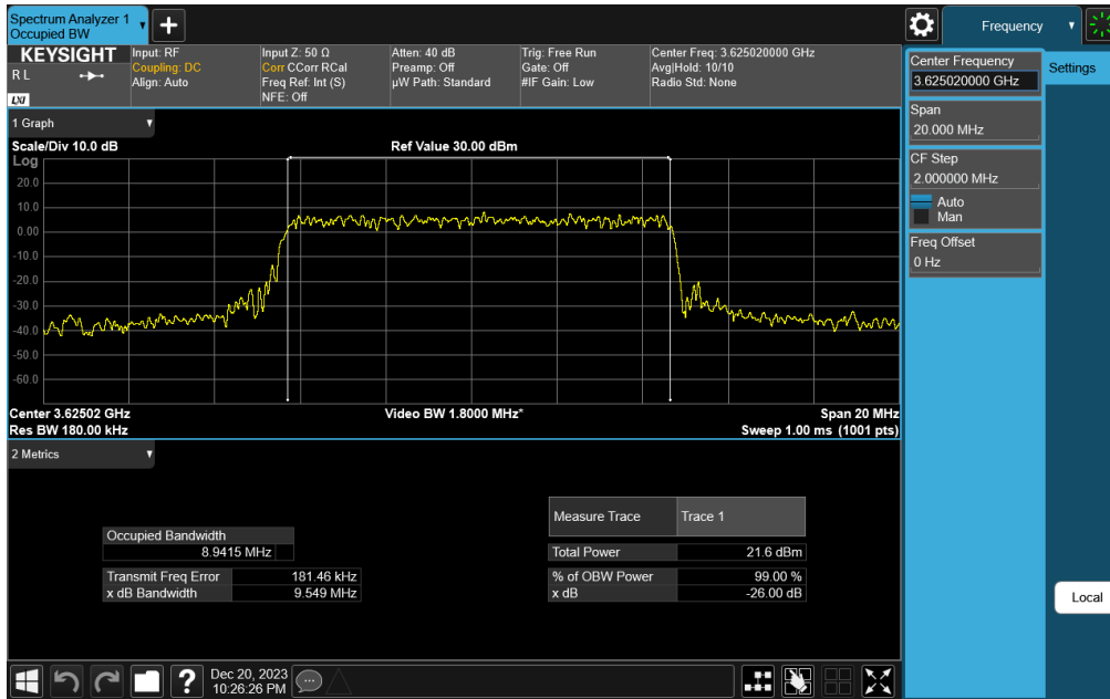
Plot 7-35. Occupied Bandwidth Plot (NR Band n48 - 10MHz 16-QAM - Full RB Configuration)
