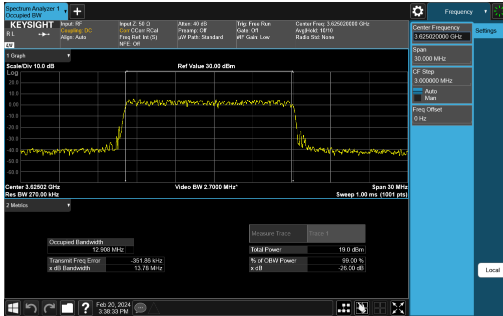
Plot 7-39. Occupied Bandwidth Plot (NR Band n48 - 15MHz QPSK - Full RB Configuration)
