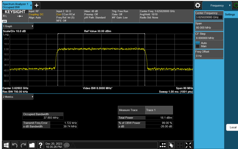
Plot 7-57. Occupied Bandwidth Plot (NR Band n48 - 40MHz 256-QAM - Full RB Configuration)
