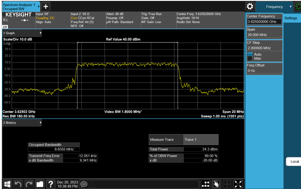
Plot 7-33. Occupied Bandwidth Plot (NR Band n48 - 10MHz \pi/2 BPSK - Full RB Configuration)
