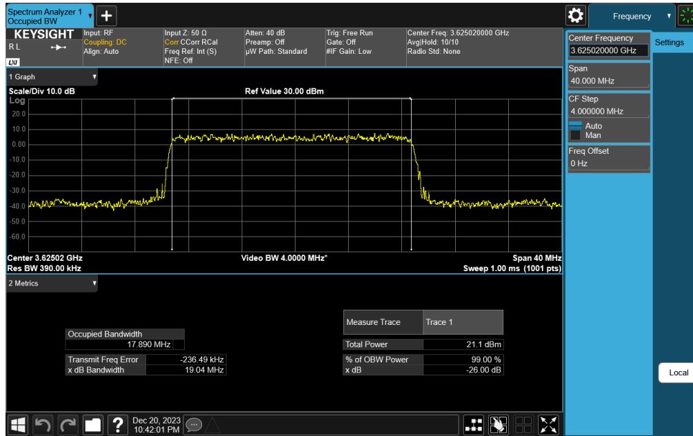
Plot 7-43. Occupied Bandwidth Plot (NR Band n48 - 20MHz \pi/2 BPSK - Full RB Configuration)
