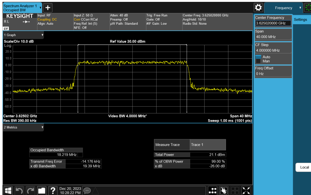
Plot 7-44. Occupied Bandwidth Plot (NR Band n48 - 20MHz QPSK - Full RB Configuration)
