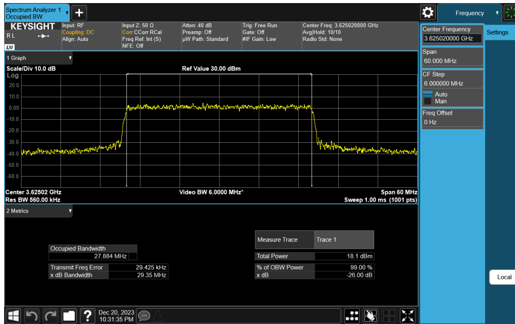
Plot 7-50. Occupied Bandwidth Plot (NR Band n48 - 30MHz 16-QAM - Full RB Configuration)
