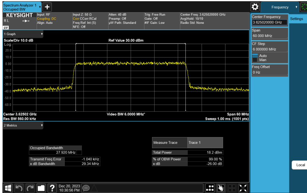
Plot 7-49. Occupied Bandwidth Plot (NR Band n48 - 30MHz QPSK - Full RB Configuration)
