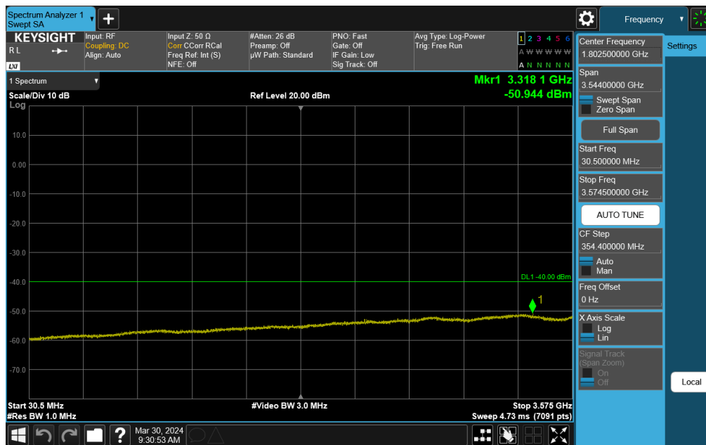
Plot 7-85. Conducted Spurious Plot (NR Band n48 - 40MHz QPSK - Mid Channel)
