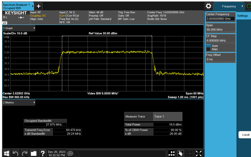
Plot 7-52. Occupied Bandwidth Plot (NR Band n48 - 30MHz 256-QAM - Full RB Configuration)
