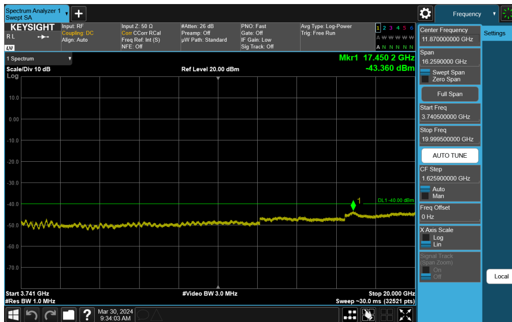
Plot 7-89. Conducted Spurious Plot (NR Band n48 - 40MHz QPSK - High Channel)
