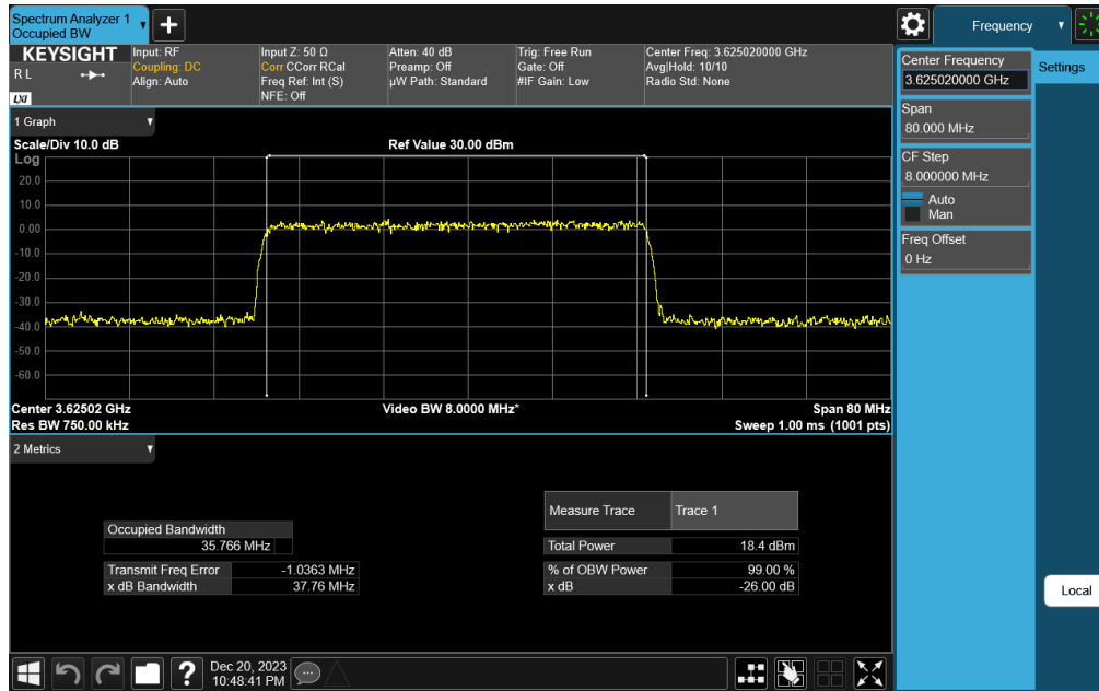
Plot 7-53. Occupied Bandwidth Plot (NR Band n48 - 40MHz \pi/2 BPSK - Full RB Configuration)
