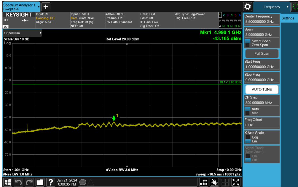
Plot 7-80. Conducted Spurious Plot (NR Band 14 - 5MHz DFT-s-OFDM QPSK - RB Size 1, RB Offset 0 - High Channel)
