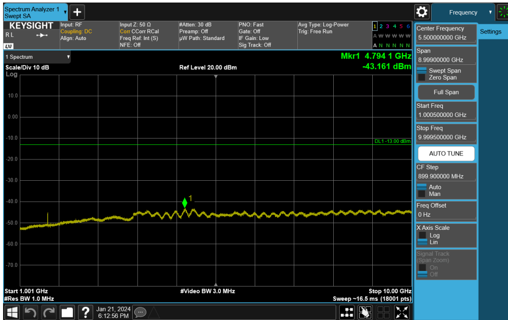
Plot 7-86. Conducted Spurious Plot (NR Band 26 - 10MHz DFT-s-OFDM QPSK - RB Size 1, RB Offset 0 - Mid Channel)
