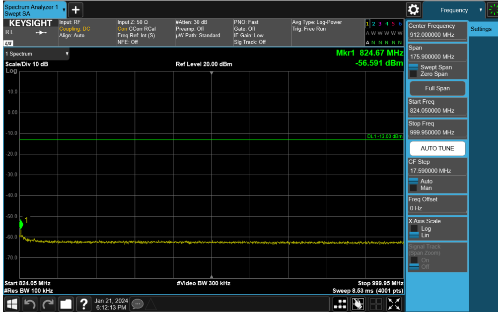
Plot 7-85. Conducted Spurious Plot (NR Band 26 - 10MHz DFT-s-OFDM QPSK - RB Size 1, RB Offset 0 - Mid Channel)
