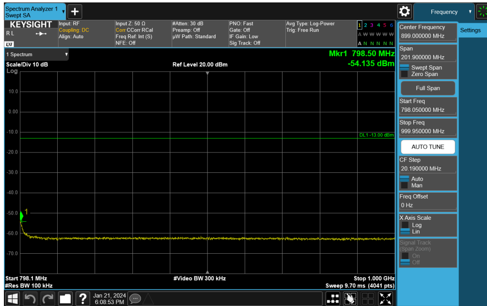
Plot 7-79. Conducted Spurious Plot (NR Band 14 - 5MHz DFT-s-OFDM QPSK - RB Size 1, RB Offset 0 - High Channel)
