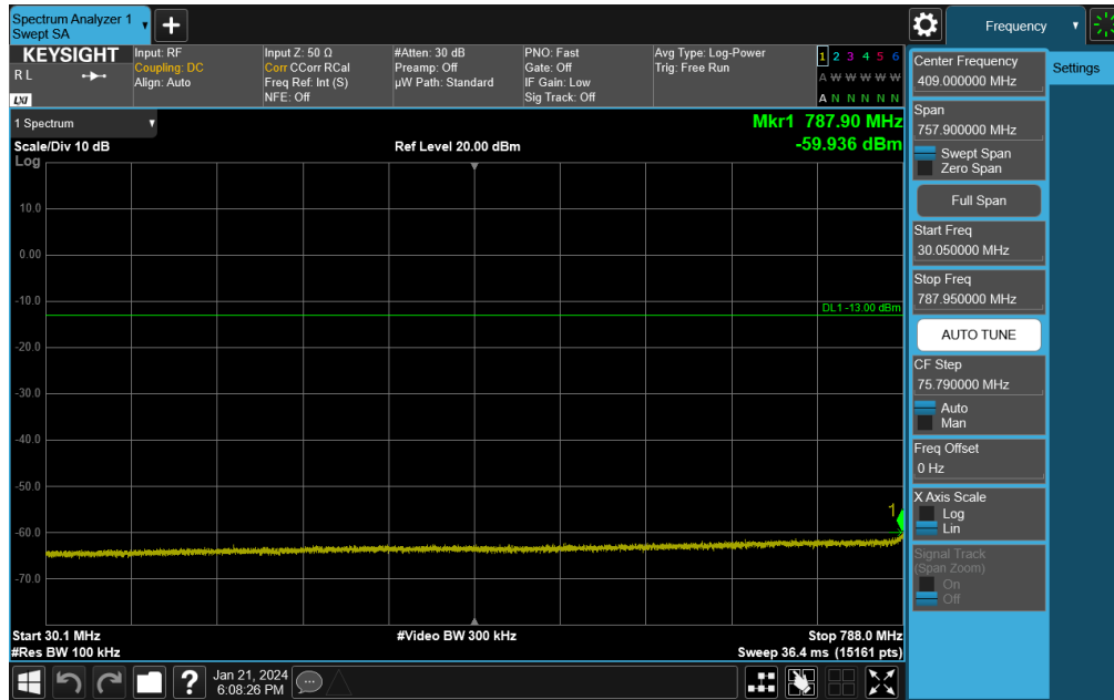
Plot 7-78. Conducted Spurious Plot (NR Band 14 - 5MHz DFT-s-OFDM QPSK - RB Size 1, RB Offset 0 - High Channel)
