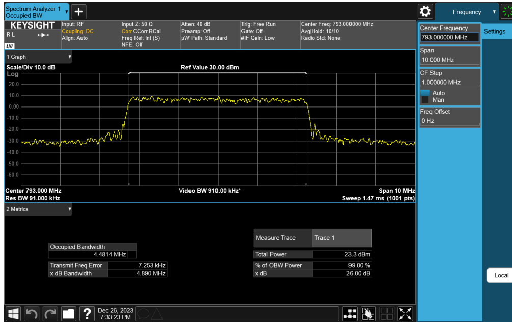
Plot 7-27. Occupied Bandwidth Plot (NR Band 14 - 5MHz CP-OFDM 16-QAM - Full RB)
