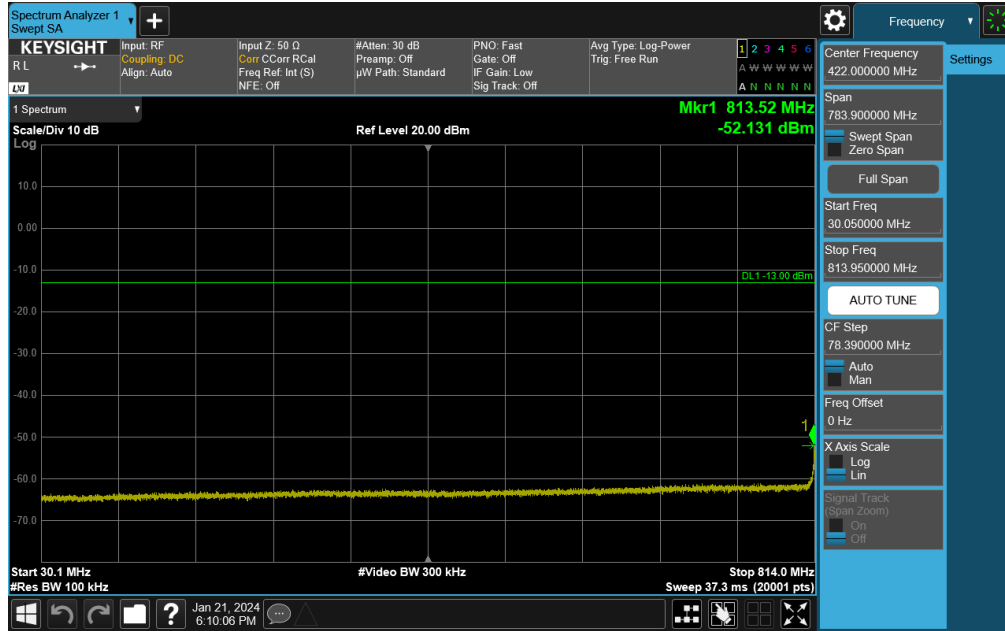
Plot 7-81. Conducted Spurious Plot (NR Band 26 - 5MHz DFT-s-OFDM QPSK - RB Size 1, RB Offset 0 - Low Channel)
