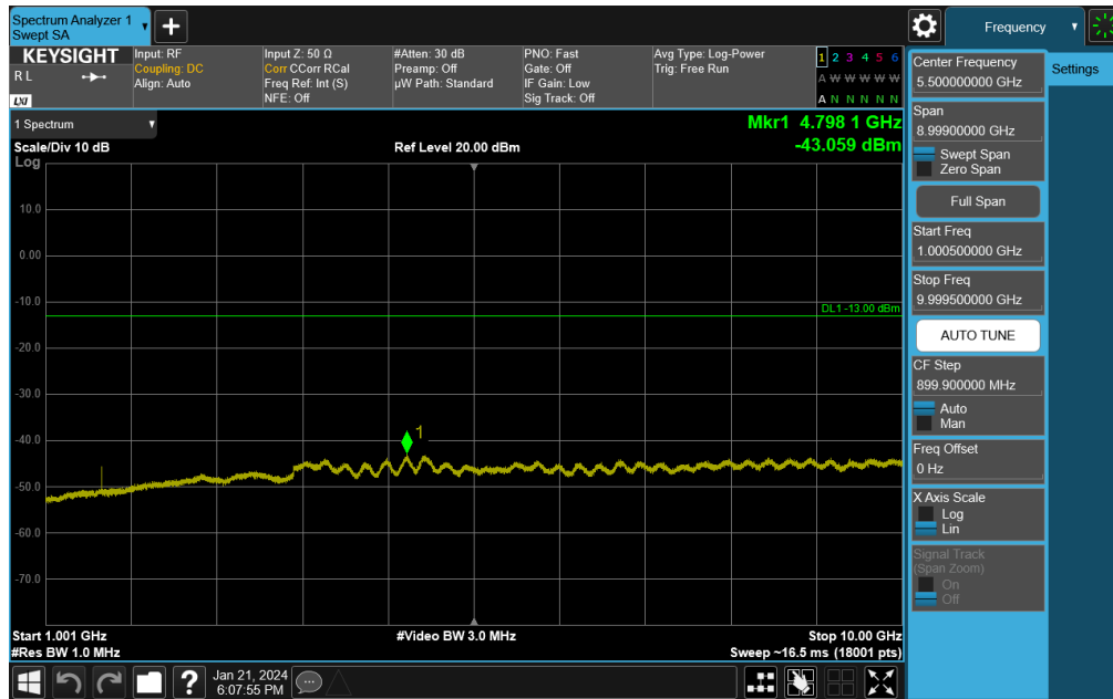
Plot 7-77. Conducted Spurious Plot (NR Band 14 - 10MHz DFT-s-OFDM QPSK - RB Size 1, RB Offset 0 - Mid Channel)
