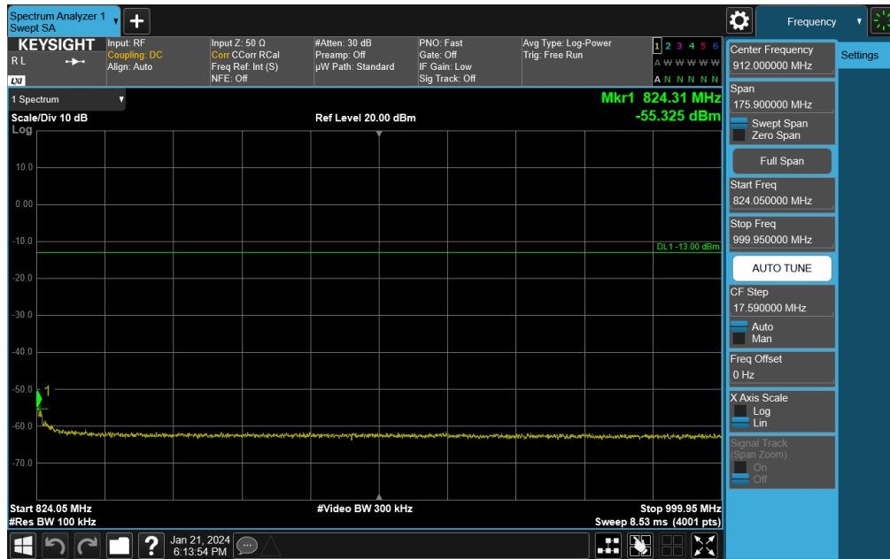
Plot 7-88. Conducted Spurious Plot (NR Band 26 - 5MHz DFT-s-OFDM QPSK - RB Size 1, RB Offset 0 - High Channel)
