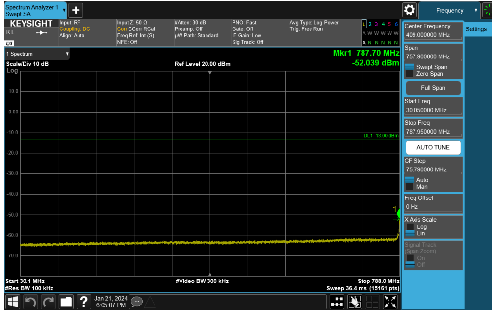
Plot 7-72. Conducted Spurious Plot (NR Band 14 - 5MHz DFT-s-OFDM QPSK - RB Size 1, RB Offset 0 - Low Channel)
