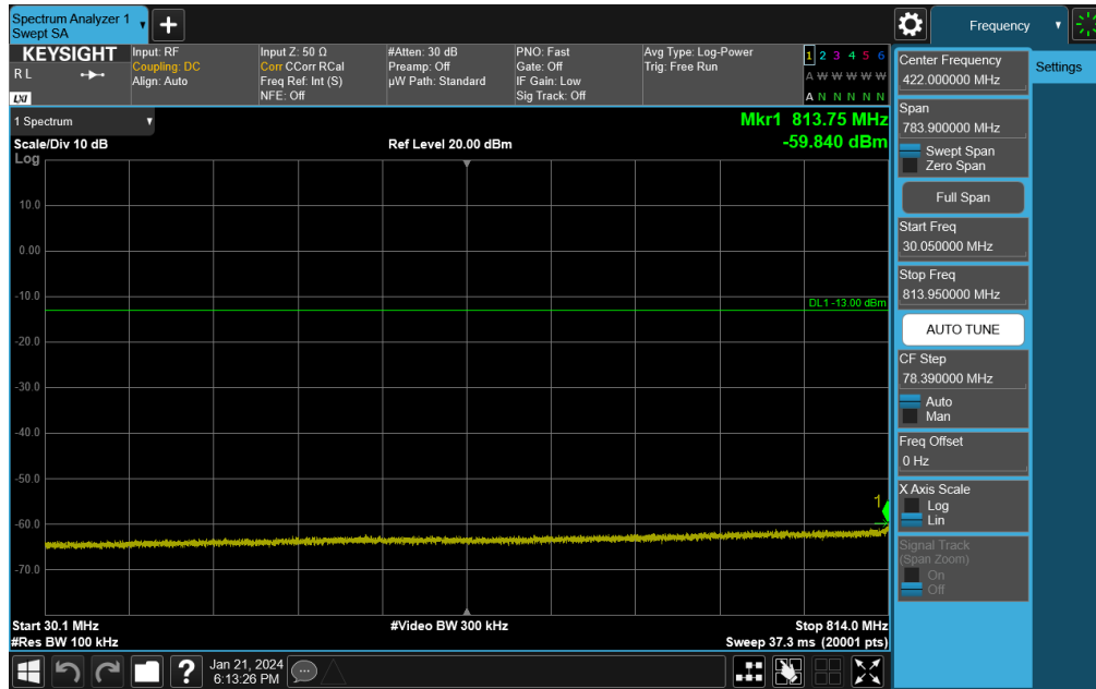
Plot 7-87. Conducted Spurious Plot (NR Band 26 - 5MHz DFT-s-OFDM QPSK - RB Size 1, RB Offset 0 - High Channel)
