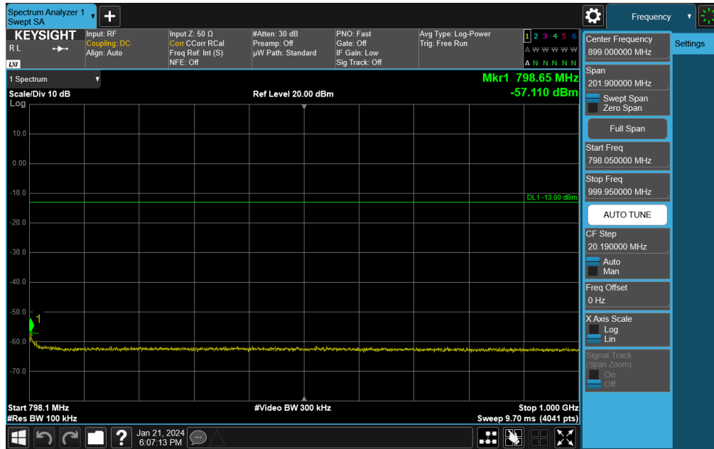
Plot 7-76. Conducted Spurious Plot (NR Band 14 - 10MHz DFT-s-OFDM QPSK - RB Size 1, RB Offset 0 - Mid Channel)
