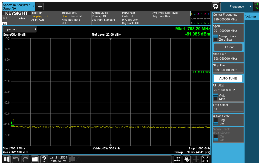
Plot 7-73. Conducted Spurious Plot (NR Band 14 - 5MHz DFT-s-OFDM QPSK - RB Size 1, RB Offset 0 - Low Channel)
