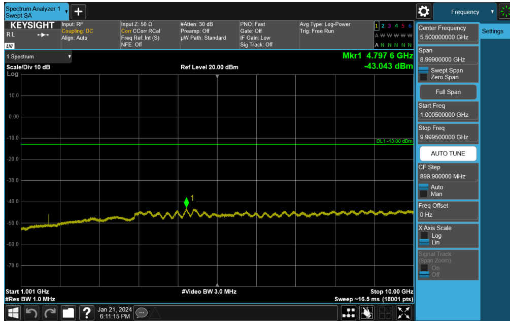
Plot 7-83. Conducted Spurious Plot (NR Band 26 - 5MHz DFT-s-OFDM QPSK - RB Size 1, RB Offset 0 - Low Channel)
