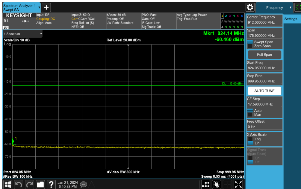
Plot 7-82. Conducted Spurious Plot (NR Band 26 - 5MHz DFT-s-OFDM QPSK - RB Size 1, RB Offset 0 - Low Channel)
