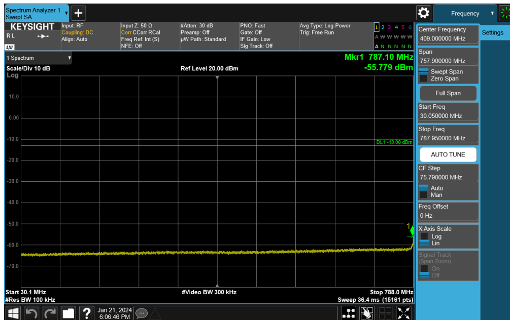
Plot 7-75. Conducted Spurious Plot (NR Band 14 - 10MHz DFT-s-OFDM QPSK - RB Size 1, RB Offset 0 - Mid Channel)
