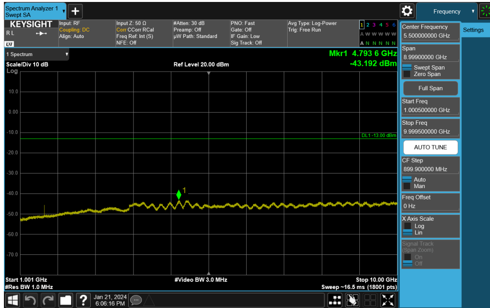
Plot 7-74. Conducted Spurious Plot (NR Band 14 - 5MHz DFT-s-OFDM QPSK - RB Size 1, RB Offset 0 - Low Channel)
