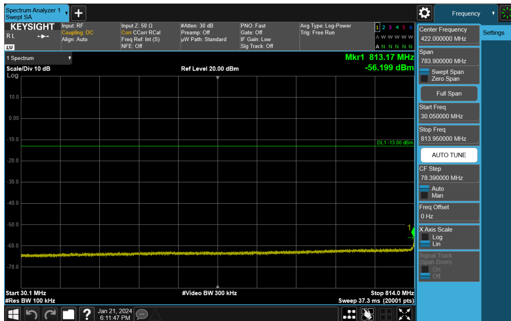
Plot 7-84. Conducted Spurious Plot (NR Band 26 - 10MHz DFT-s-OFDM QPSK - RB Size 1, RB Offset 0 - Mid Channel)
