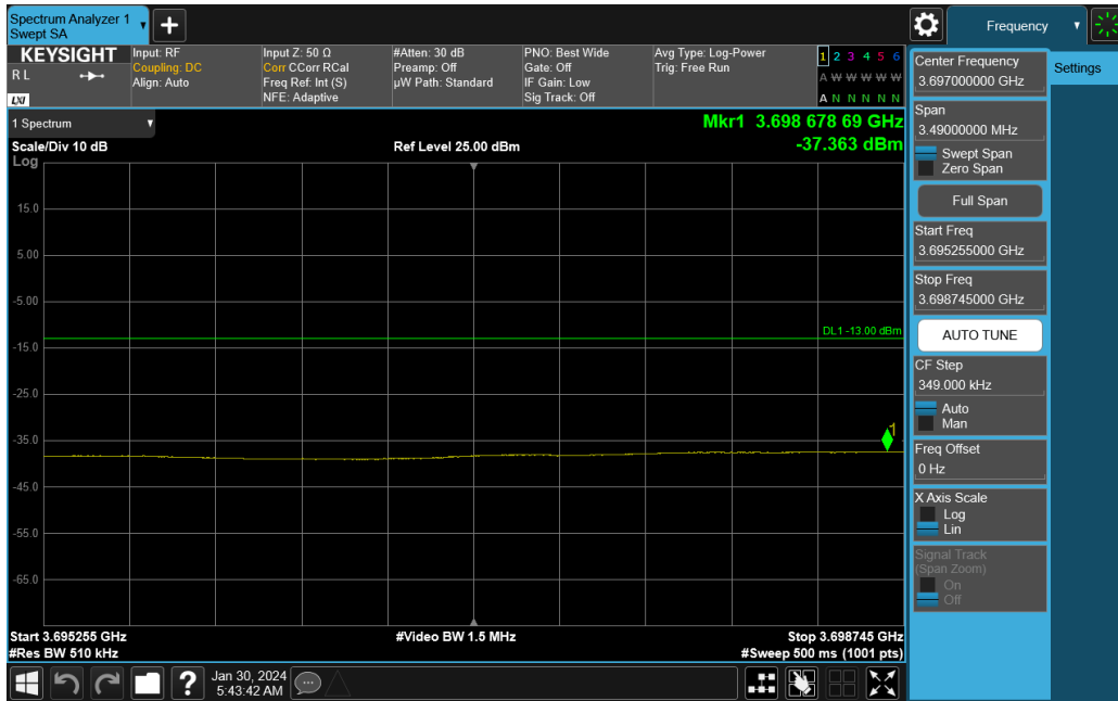
Plot 7-290. Lower ACP Plot (NR Band n77 C-Band - 90MHz DFT-s-OFDM QPSK – Full RB)
