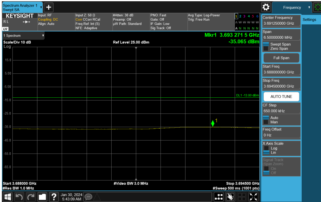
Plot 7-289. Lower ACP Plot (NR Band n77 C-Band - 90MHz DFT-s-OFDM QPSK – Full RB)
