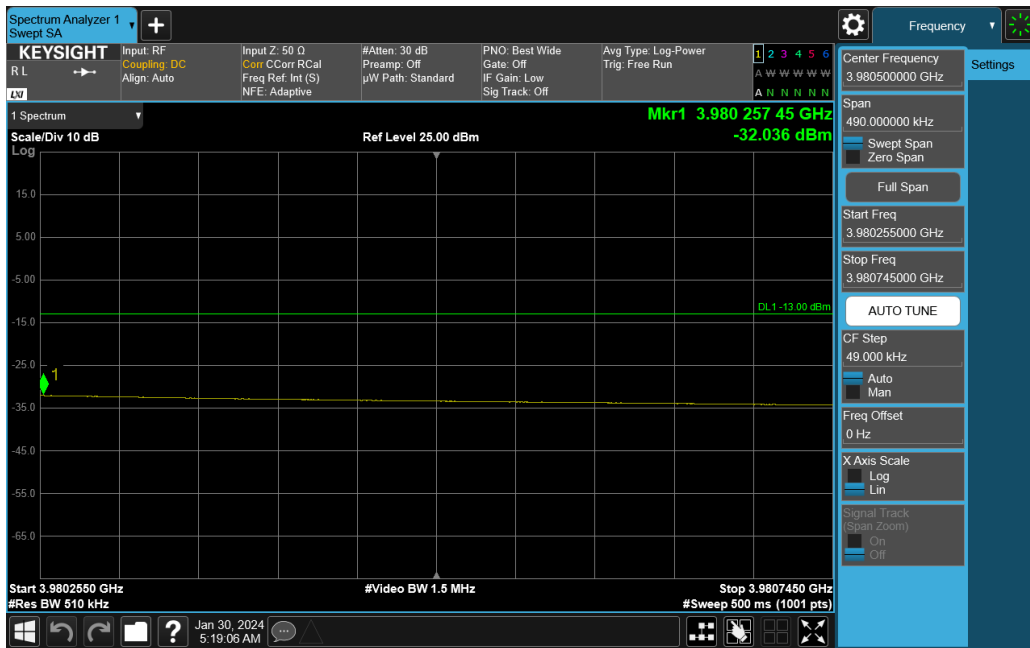
Plot 7-278. Upper ACP Plot (NR Band n77 C-Band - 70MHz DFT-s-OFDM QPSK – Full RB)
