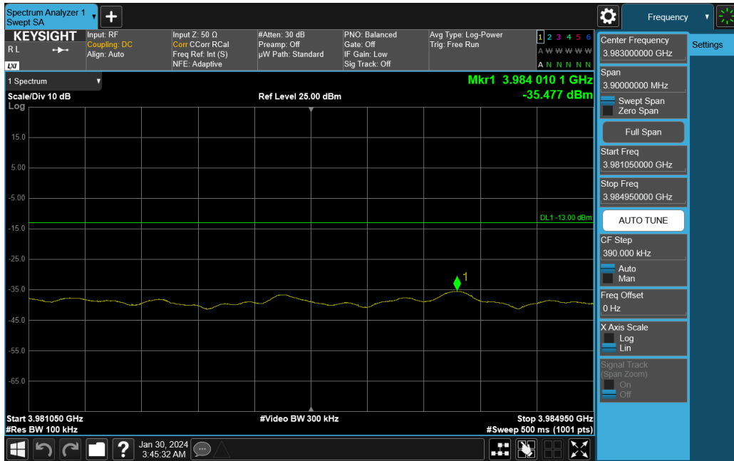
Plot 7-223. Upper ACP Plot (NR Band n77 C-Band - 10MHz DFT-s-OFDM QPSK – Full RB)
