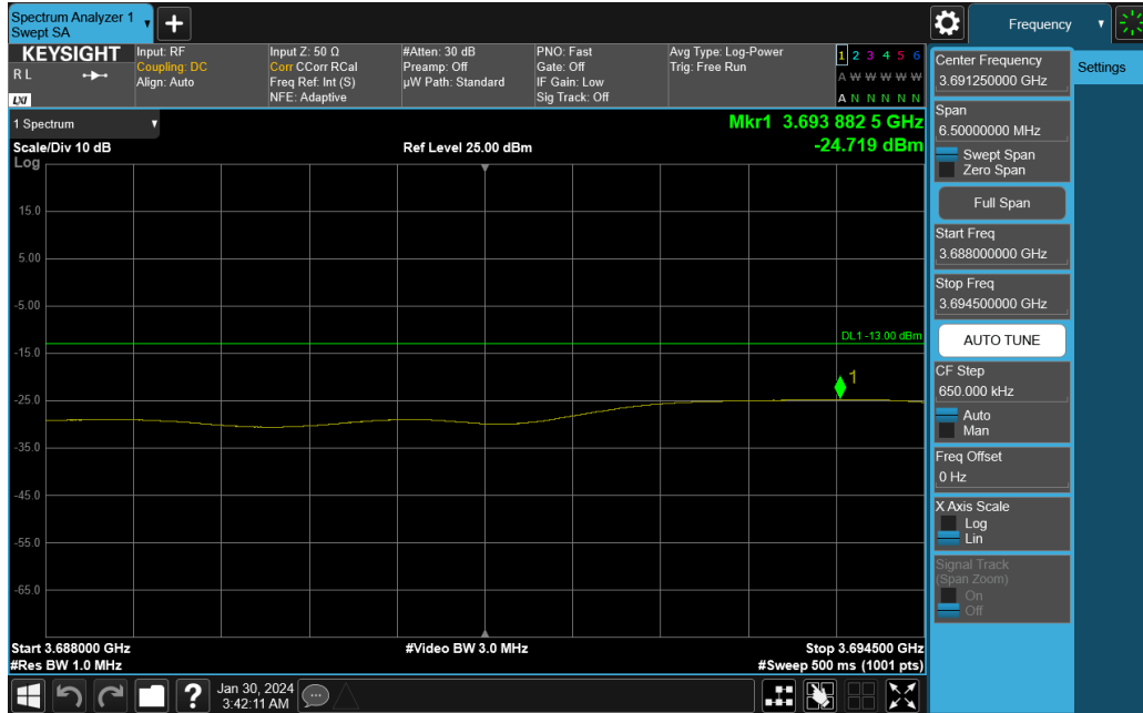
Plot 7-217. Lower ACP Plot (NR Band n77 C-Band - 10MHz DFT-s-OFDM QPSK – Full RB)
