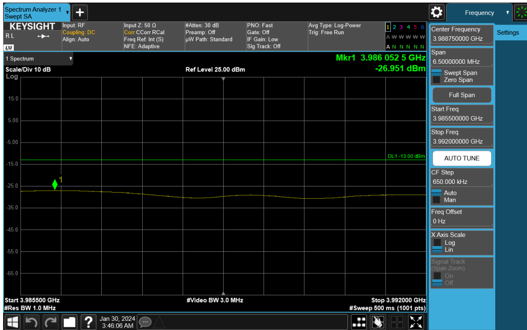
Plot 7-224. Upper ACP Plot (NR Band n77 C-Band - 10MHz DFT-s-OFDM QPSK – Full RB)
