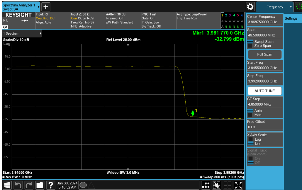
Plot 7-277. Upper ACP Plot (NR Band n77 C-Band - 70MHz DFT-s-OFDM QPSK – Full RB)
