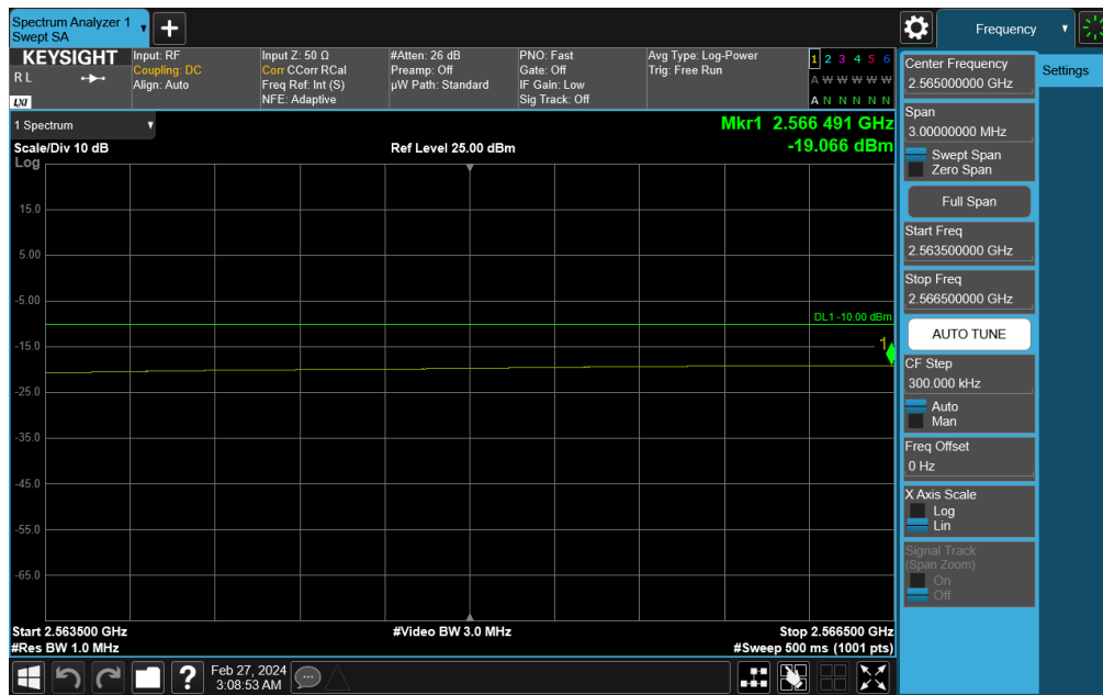
Plot 7-771. Middle Band Edge Plot (NR Band n41 - 50MHz DFT-s-OFDM QPSK – Full RB)
