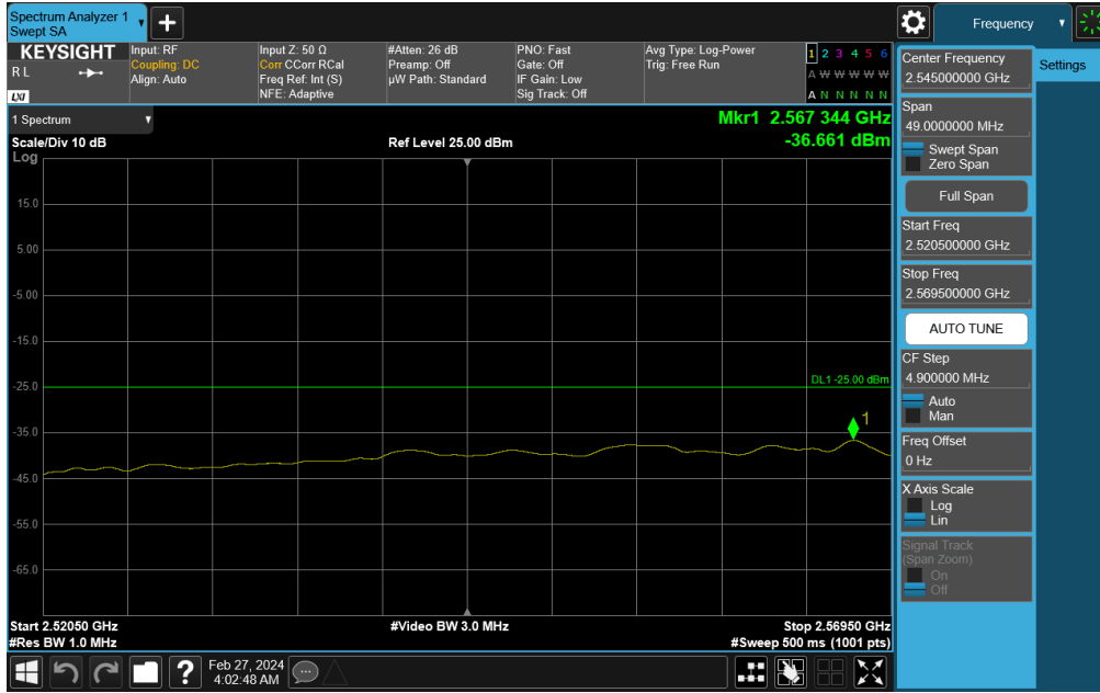
Plot 7-802. Upper Band Edge Plot (NR Band n41 - 60MHz DFT-s-OFDM QPSK – Full RB)
