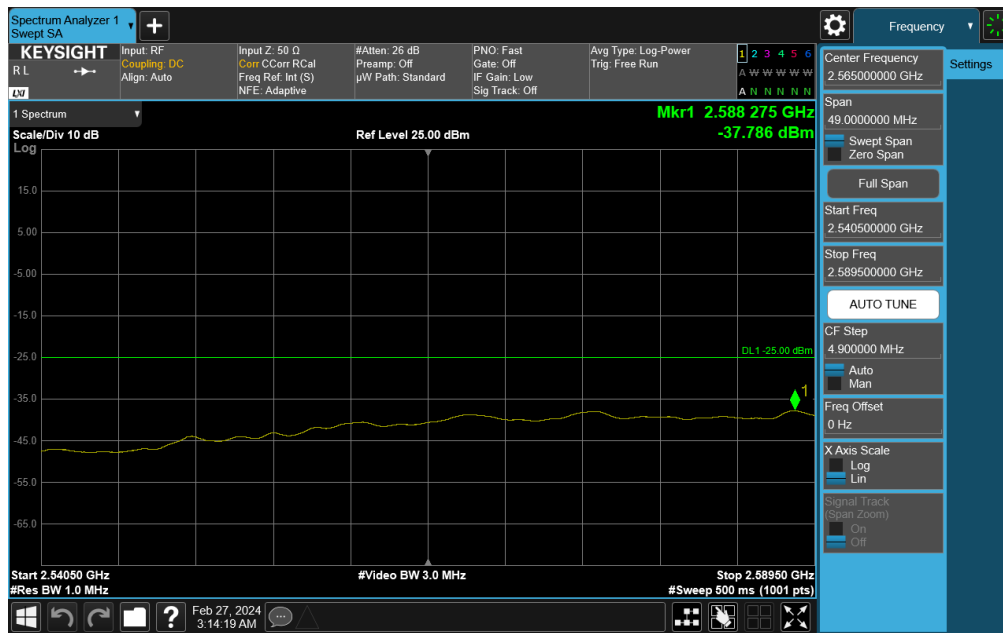
Plot 7-781. Upper Band Edge Plot (NR Band n41 - 50MHz DFT-s-OFDM QPSK – Full RB)
