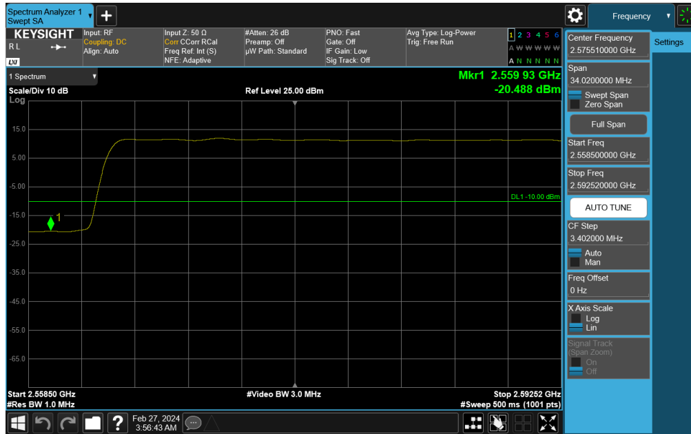
Plot 7-792. Middle Band Edge Plot (NR Band n41 - 60MHz DFT-s-OFDM QPSK – Full RB)
