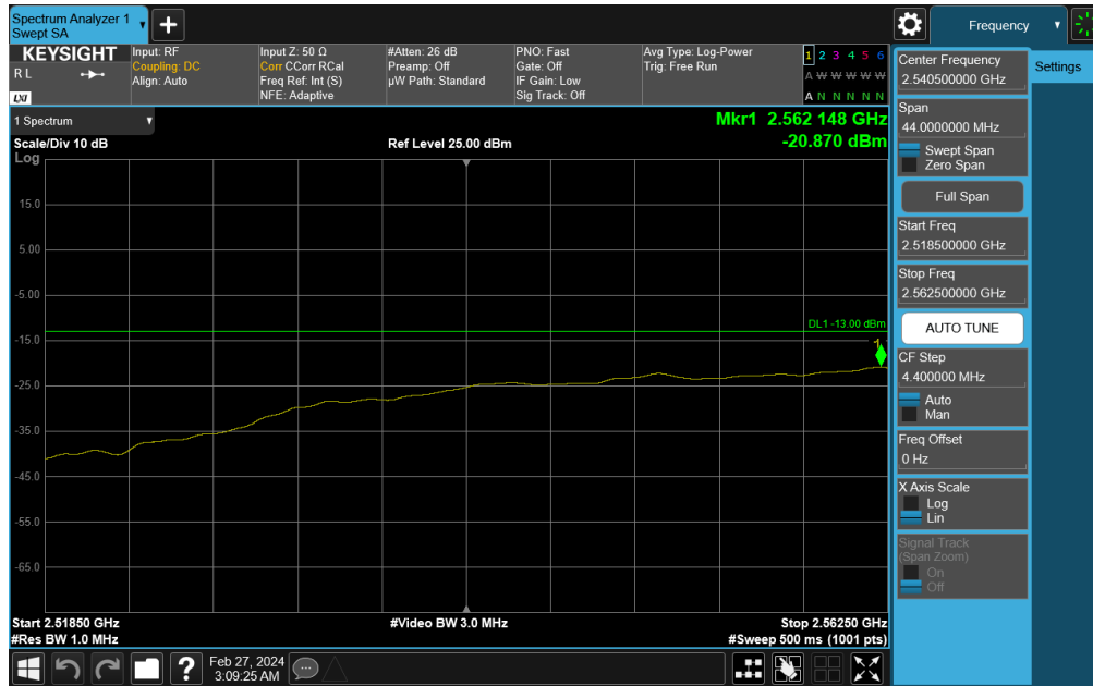
Plot 7-772. Middle Band Edge Plot (NR Band n41 - 50MHz DFT-s-OFDM QPSK – Full RB)
