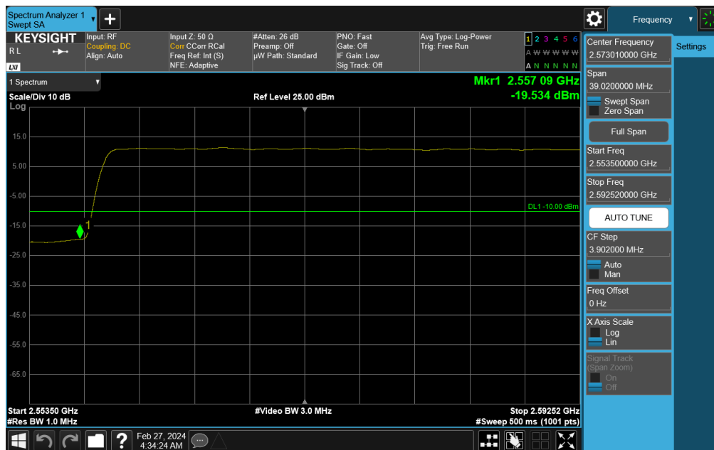
Plot 7-813. Middle Band Edge Plot (NR Band n41 - 70MHz DFT-s-OFDM QPSK – Full RB)
