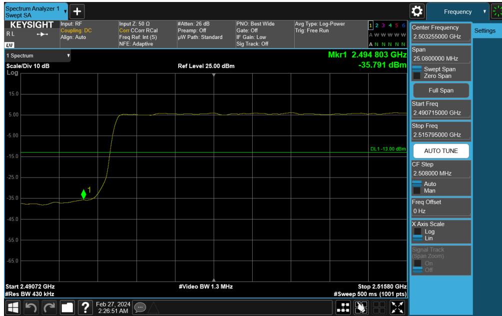
Plot 7-740. Lower Band Edge Plot (NR Band n41 - 40MHz DFT-s-OFDM QPSK – Full RB)
