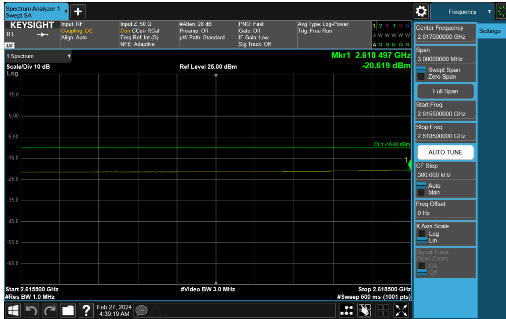
Plot 7-822. Upper Band Edge Plot (NR Band n41 - 70MHz DFT-s-OFDM QPSK – Full RB)
