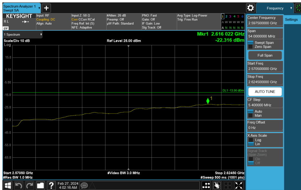
Plot 7-801. Upper Band Edge Plot (NR Band n41 - 60MHz DFT-s-OFDM QPSK – Full RB)
