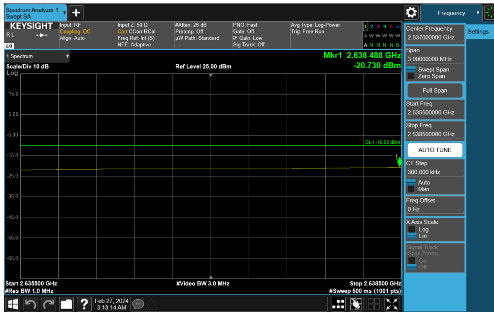
Plot 7-779. Upper Band Edge Plot (NR Band n41 - 50MHz DFT-s-OFDM QPSK – Full RB)
