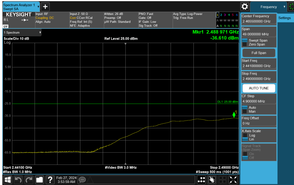
Plot 7-788. Lower Band Edge Plot (NR Band n41 - 60MHz DFT-s-OFDM QPSK – Full RB)
