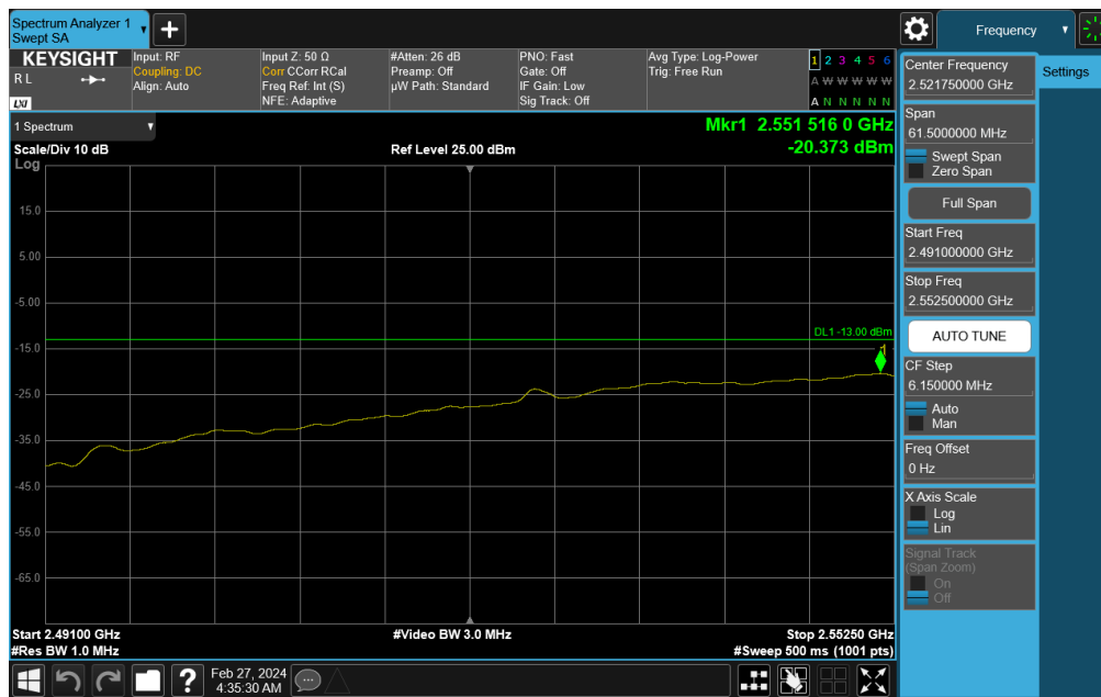
Plot 7-815. Middle Band Edge Plot (NR Band n41 - 70MHz DFT-s-OFDM QPSK – Full RB)
