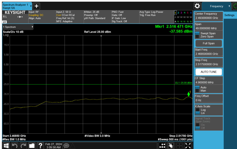
Plot 7-773. Middle Band Edge Plot (NR Band n41 - 50MHz DFT-s-OFDM QPSK – Full RB)
