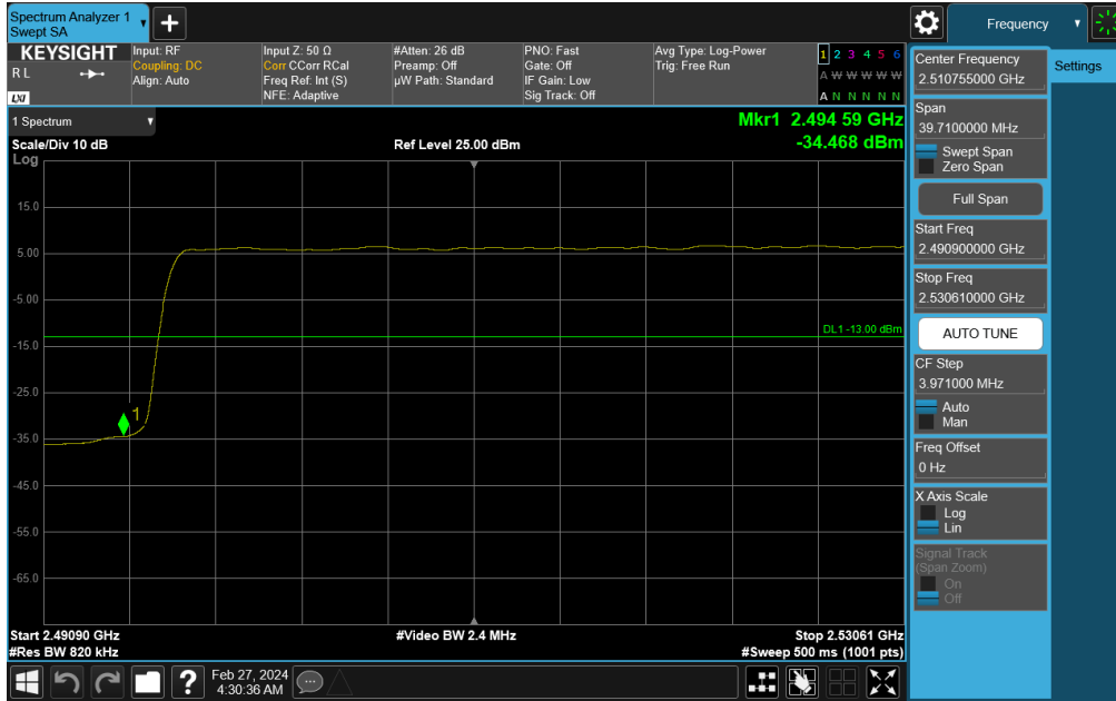
Plot 7-806. Lower Band Edge Plot (NR Band n41 - 70MHz DFT-s-OFDM QPSK – Full RB)
