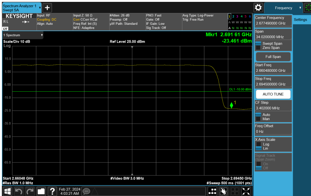
Plot 7-803. Upper Band Edge Plot (NR Band n41 - 60MHz DFT-s-OFDM QPSK – Full RB)
