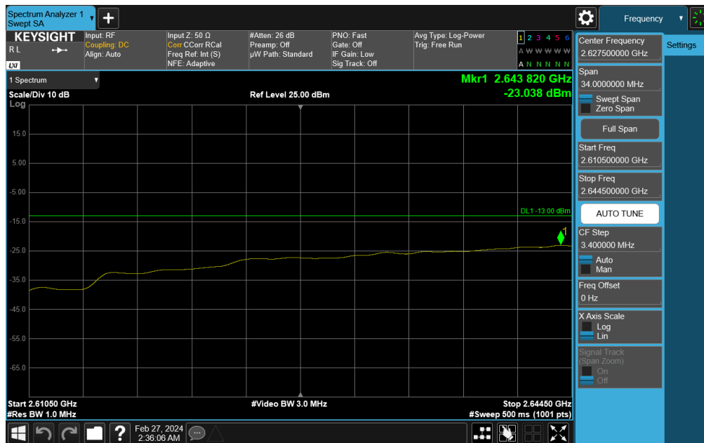
Plot 7-757. Upper Band Edge Plot (NR Band n41 - 40MHz DFT-s-OFDM QPSK – Full RB)
