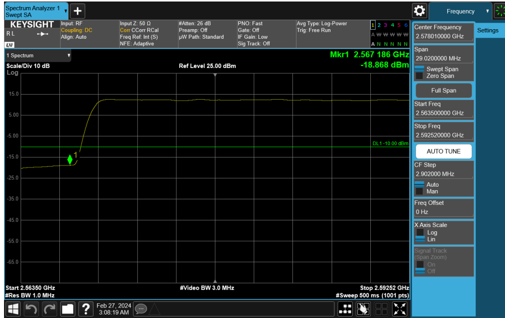
Plot 7-770. Middle Band Edge Plot (NR Band n41 - 50MHz DFT-s-OFDM QPSK – Full RB)
