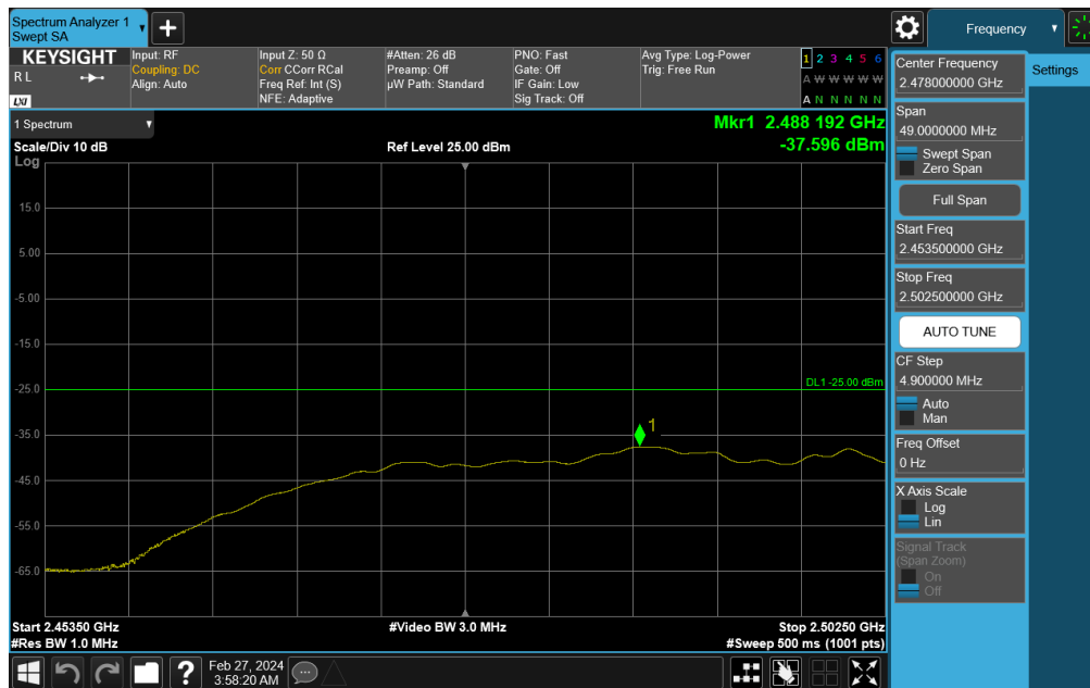
Plot 7-795. Middle Band Edge Plot (NR Band n41 - 60MHz DFT-s-OFDM QPSK – Full RB)
