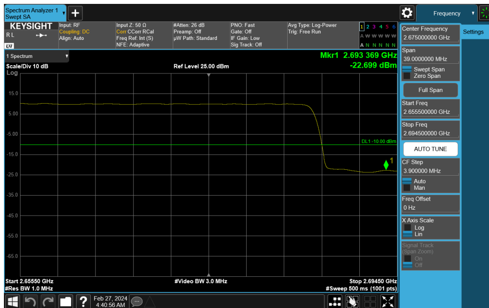
Plot 7-825. Upper Band Edge Plot (NR Band n41 - 70MHz DFT-s-OFDM QPSK – Full RB)
