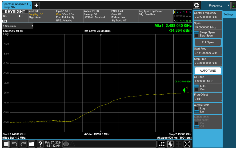
Plot 7-808. Lower Band Edge Plot (NR Band n41 - 70MHz DFT-s-OFDM QPSK – Full RB)
