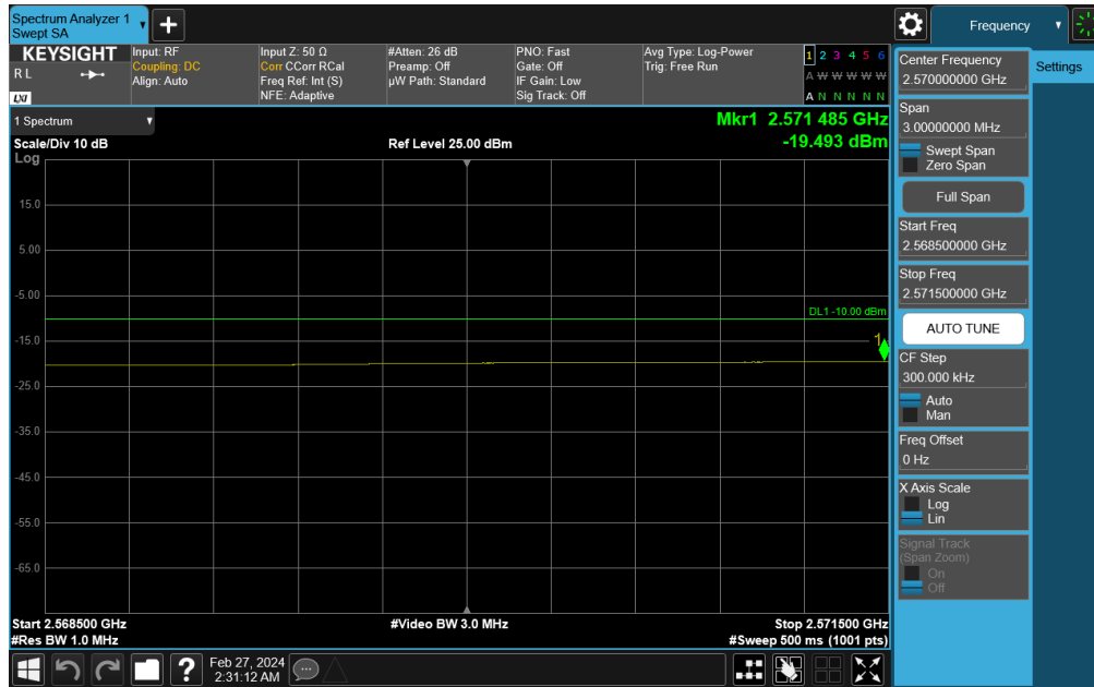
Plot 7-748. Middle Band Edge Plot (NR Band n41 - 40MHz DFT-s-OFDM QPSK – Full RB)
