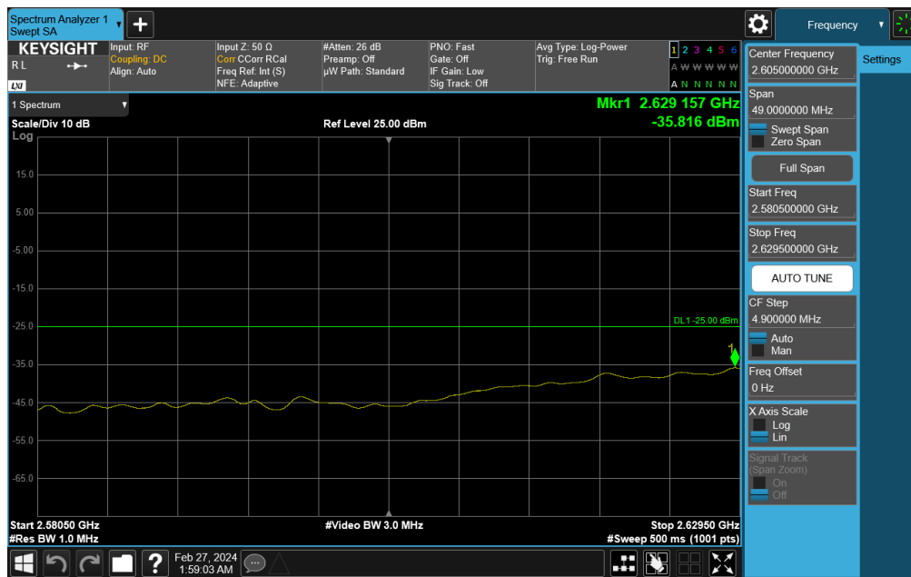
Plot 7-735. Upper Band Edge Plot (NR Band n41 - 30MHz DFT-s-OFDM QPSK – Full RB)
