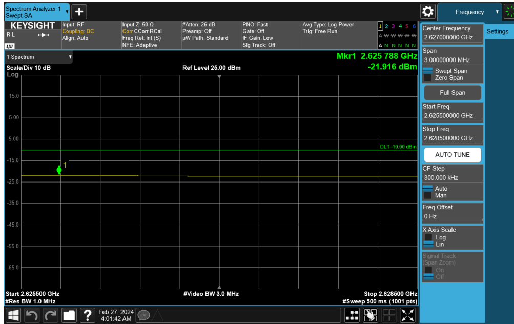
Plot 7-800. Upper Band Edge Plot (NR Band n41 - 60MHz DFT-s-OFDM QPSK – Full RB)
