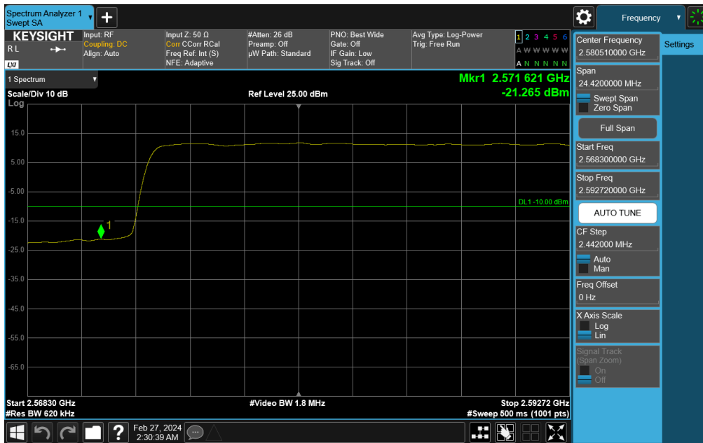
Plot 7-747. Middle Band Edge Plot (NR Band n41 - 40MHz DFT-s-OFDM QPSK – Full RB)
