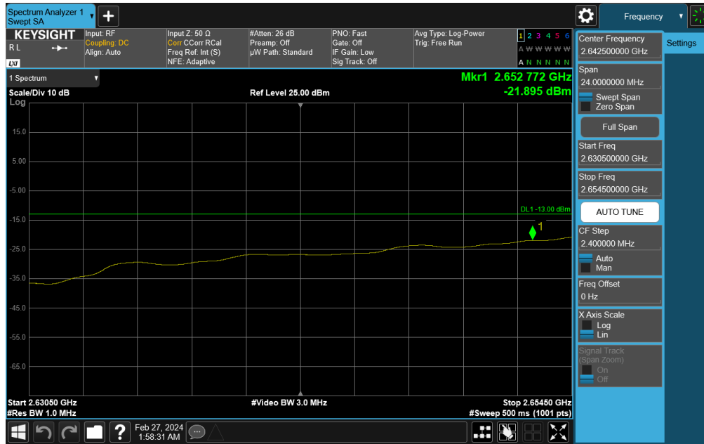
Plot 7-734. Upper Band Edge Plot (NR Band n41 - 30MHz DFT-s-OFDM QPSK – Full RB)
