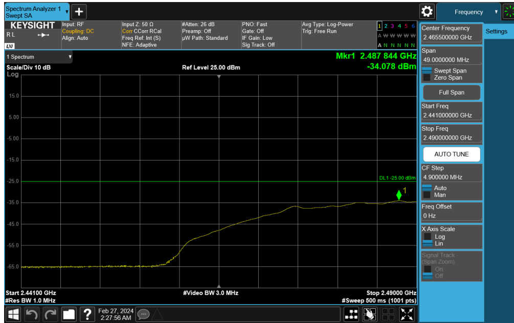
Plot 7-742. Lower Band Edge Plot (NR Band n41 - 40MHz DFT-s-OFDM QPSK – Full RB)
