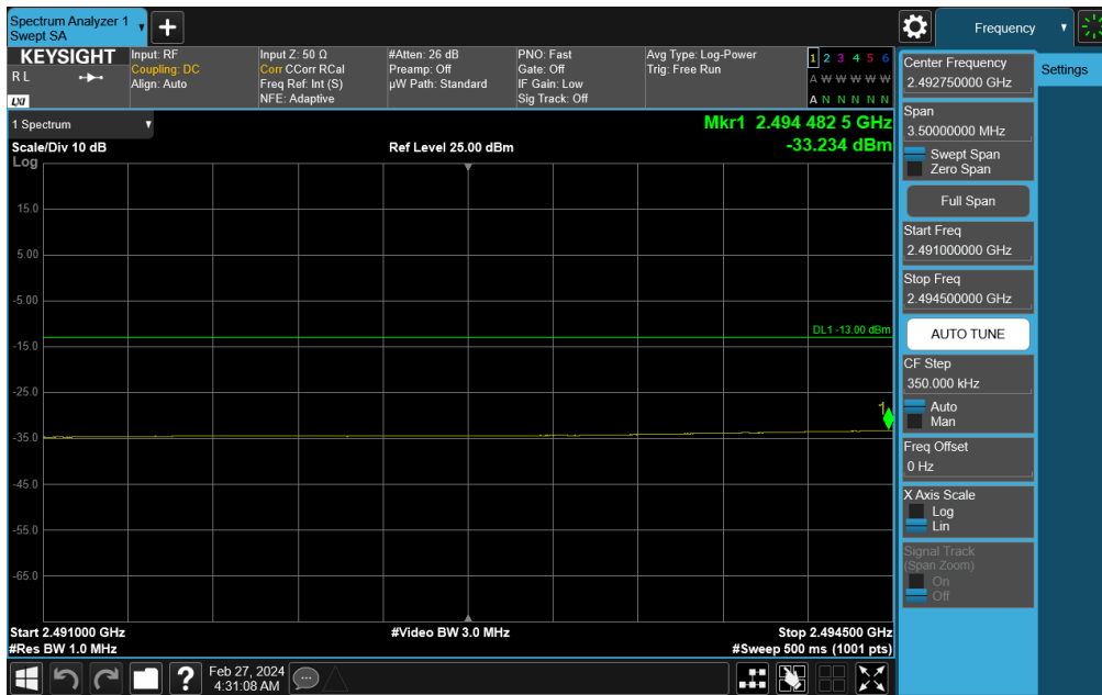
Plot 7-807. Lower Band Edge Plot (NR Band n41 - 70MHz DFT-s-OFDM QPSK – Full RB)
