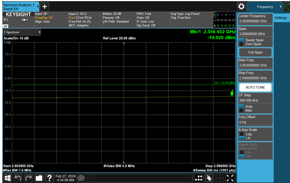
Plot 7-814. Middle Band Edge Plot (NR Band n41 - 70MHz DFT-s-OFDM QPSK – Full RB)
