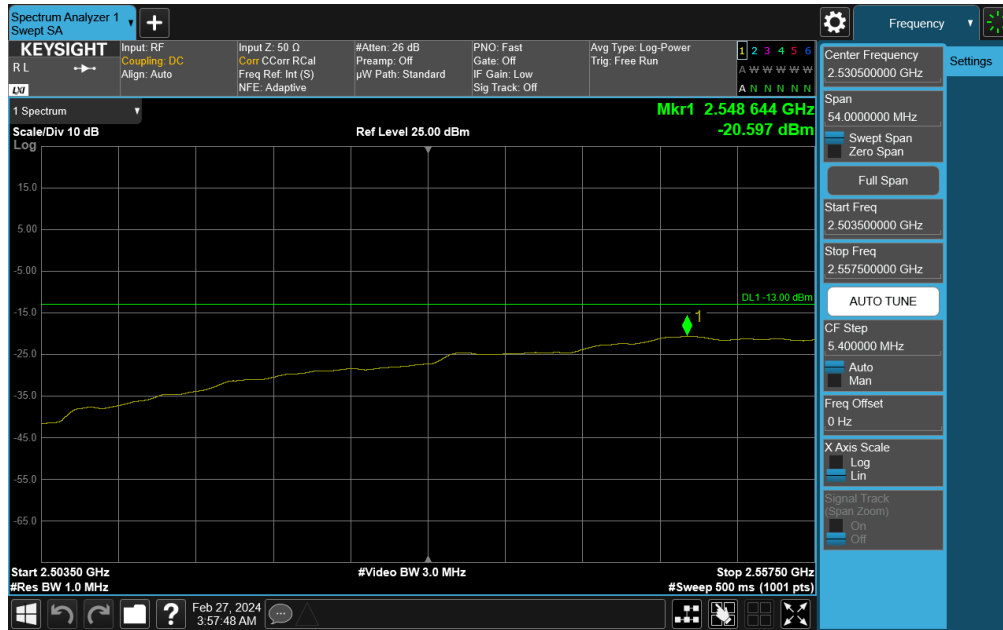
Plot 7-794. Middle Band Edge Plot (NR Band n41 - 60MHz DFT-s-OFDM QPSK – Full RB)
