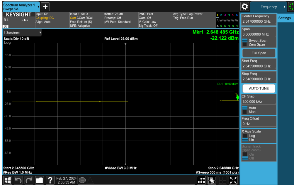
Plot 7-756. Upper Band Edge Plot (NR Band n41 - 40MHz DFT-s-OFDM QPSK – Full RB)
