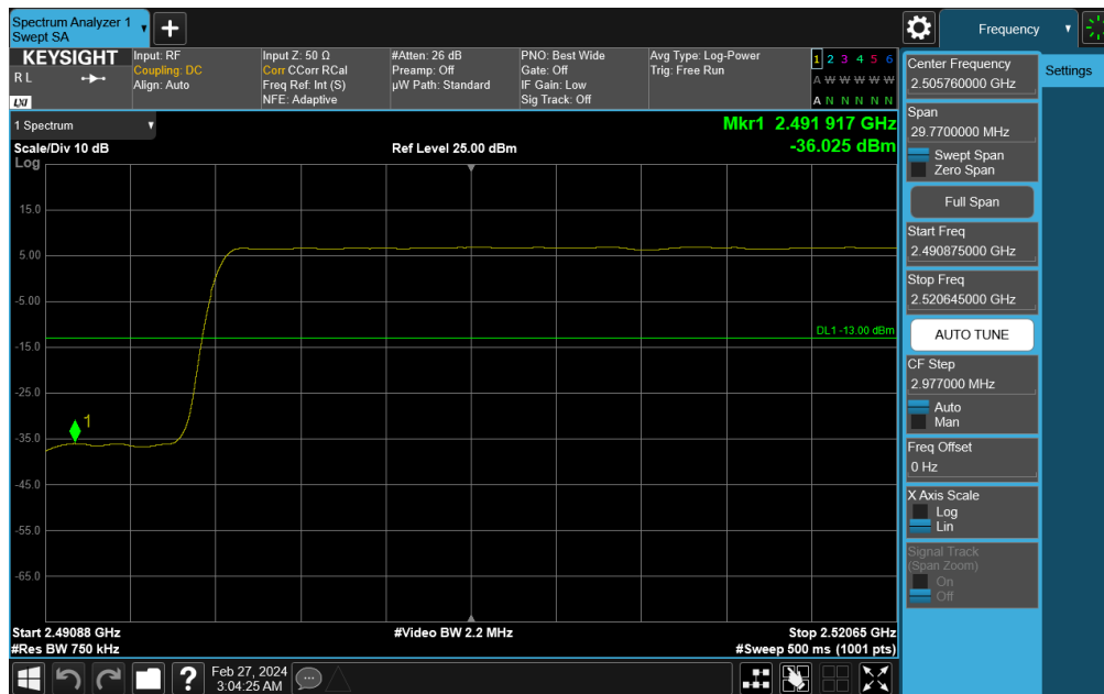
Plot 7-763. Lower Band Edge Plot (NR Band n41 - 50MHz DFT-s-OFDM QPSK – Full RB)
