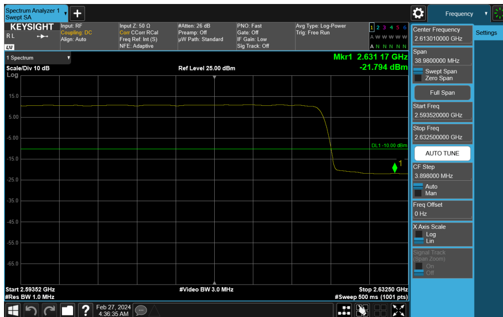
Plot 7-817. Middle Band Edge Plot (NR Band n41 - 70MHz DFT-s-OFDM QPSK – Full RB)
