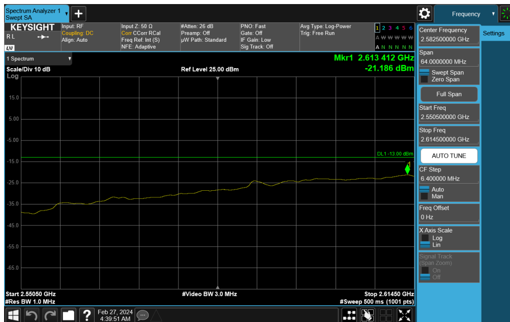
Plot 7-823. Upper Band Edge Plot (NR Band n41 - 70MHz DFT-s-OFDM QPSK – Full RB)
