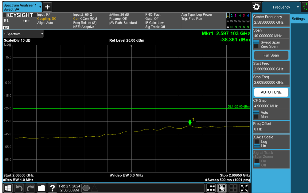
Plot 7-758. Upper Band Edge Plot (NR Band n41 - 40MHz DFT-s-OFDM QPSK – Full RB)
