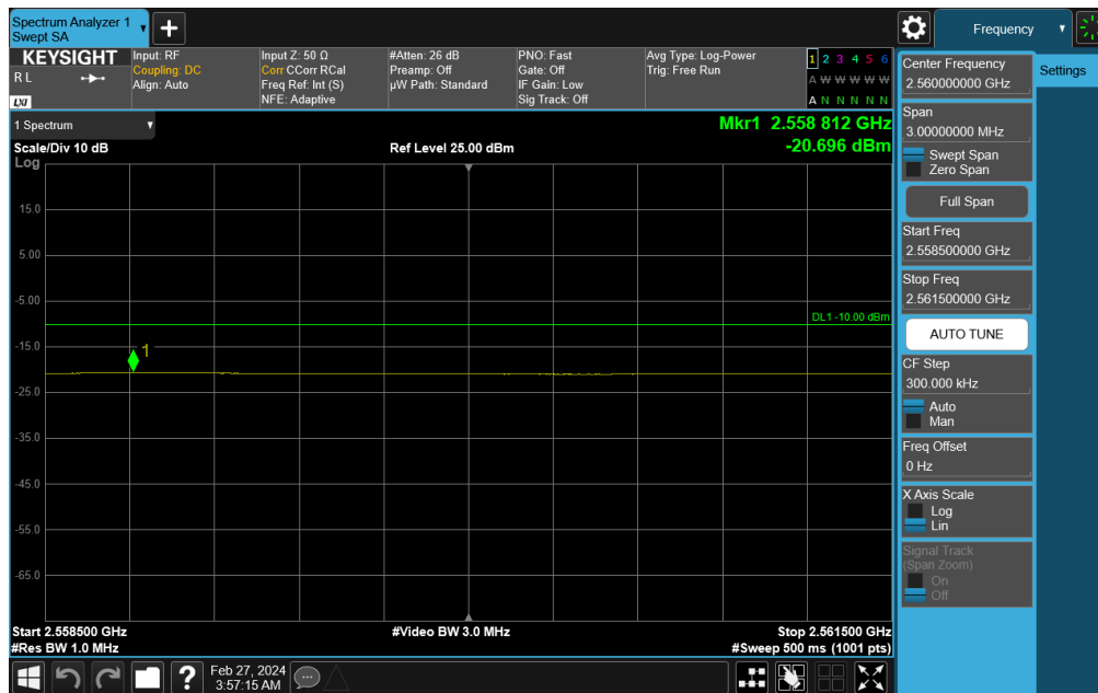
Plot 7-793. Middle Band Edge Plot (NR Band n41 - 60MHz DFT-s-OFDM QPSK – Full RB)
