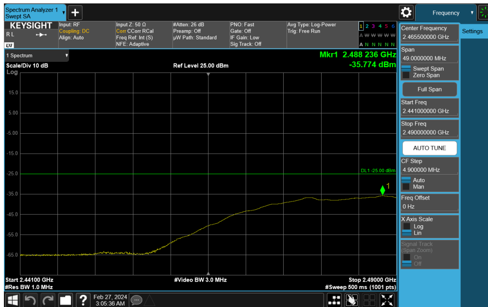
Plot 7-765. Lower Band Edge Plot (NR Band n41 - 50MHz DFT-s-OFDM QPSK – Full RB)
