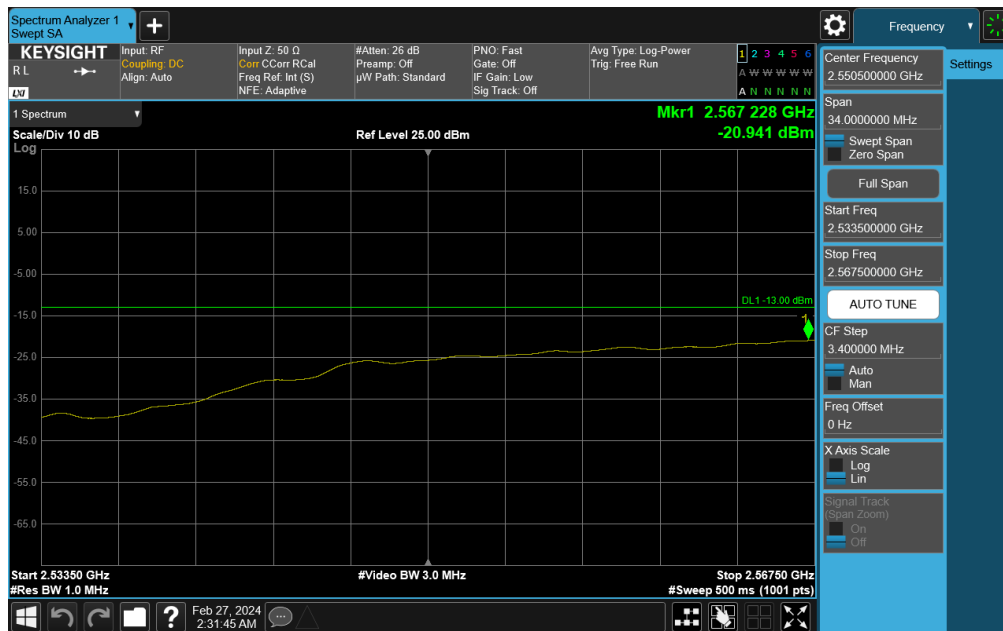
Plot 7-749. Middle Band Edge Plot (NR Band n41 - 40MHz DFT-s-OFDM QPSK – Full RB)
