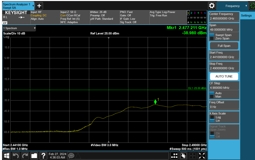
Plot 7-816. Middle Band Edge Plot (NR Band n41 - 70MHz DFT-s-OFDM QPSK – Full RB)
