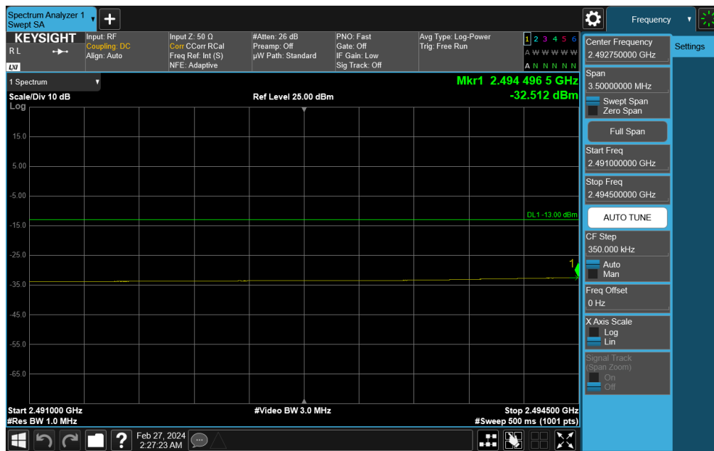
Plot 7-741. Lower Band Edge Plot (NR Band n41 - 40MHz DFT-s-OFDM QPSK – Full RB)
