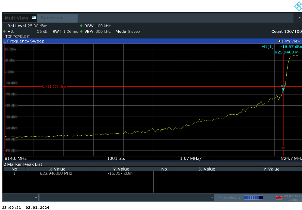
Plot 7-86. Lower BE Plot (LTE Band 5 – 1.4MHz QPSK – Full RB Configuration)
