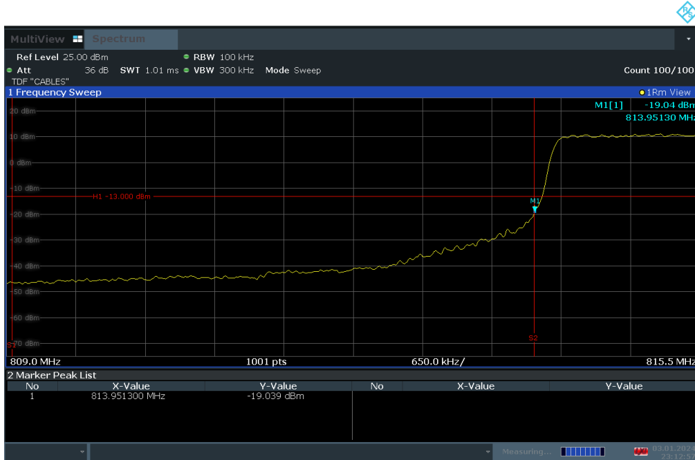
Plot 7-80. Lower BE Plot (LTE Band 26 - 3MHz QPSK – Full RB Configuration)
