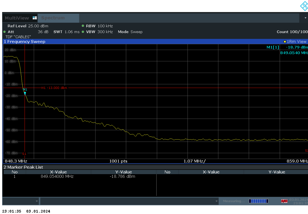
Plot 7-87. Upper BE Plot (LTE Band 5 – 1.4MHz QPSK – Full RB Configuration)
