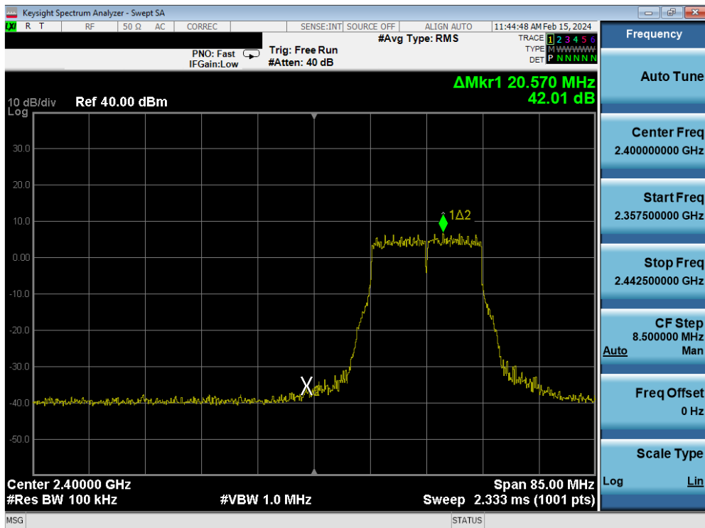
Plot 7-240. Band Edge Plot Antenna 4a (802.11g - Ch. 2) - 54Mbps
