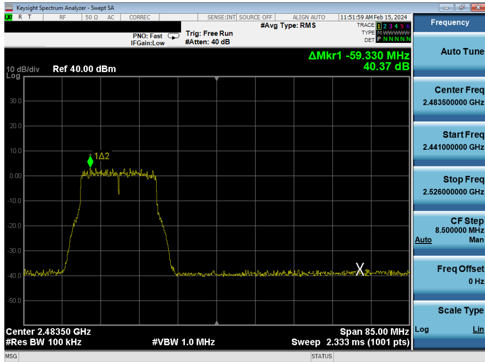
Plot 7-247. Band Edge Plot Antenna 4a (802.11g – Ch. 11) – 54Mbps
