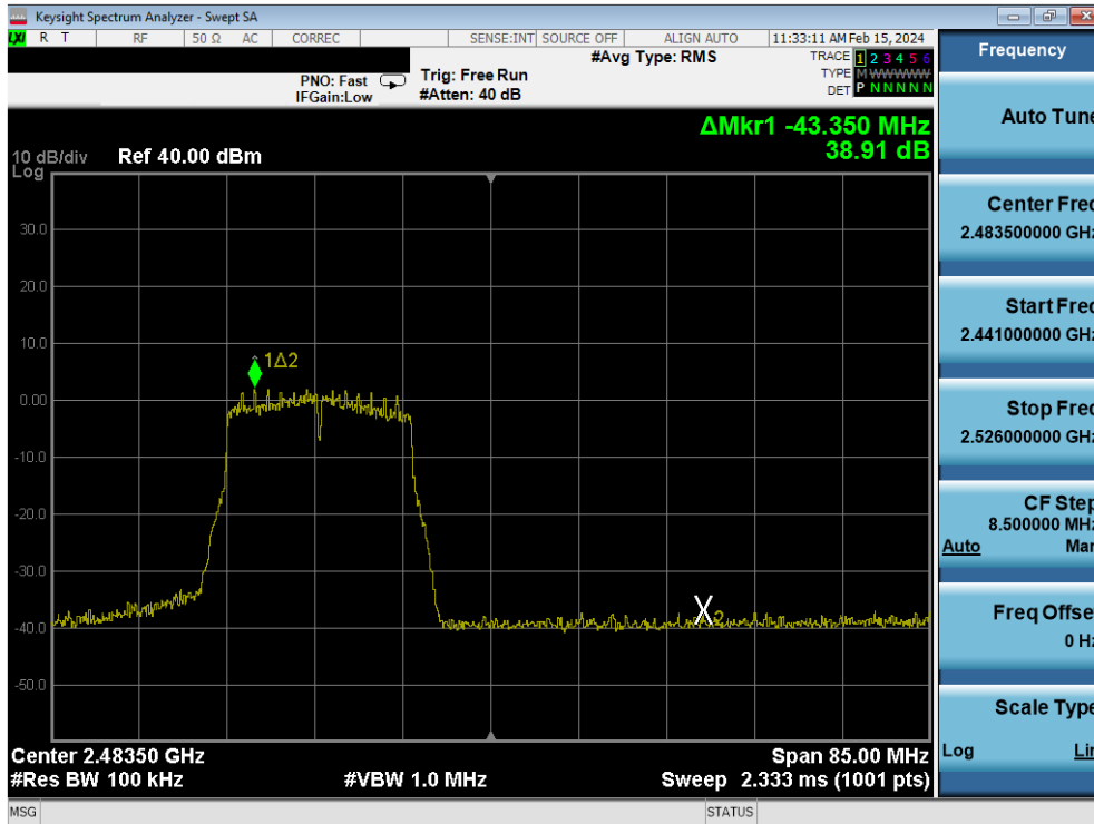
Plot 7-223. Band Edge Plot Antenna 4a (802.11n (2.4GHz) - Ch. 12) - MCS4
