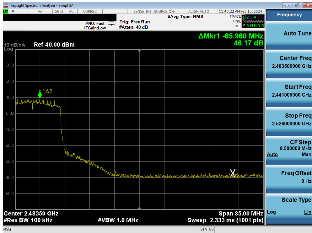
Plot 7-230. Band Edge Plot Antenna 4a (802.11ax (SU - 2.4GHz) – Ch. 8) – MCS4
