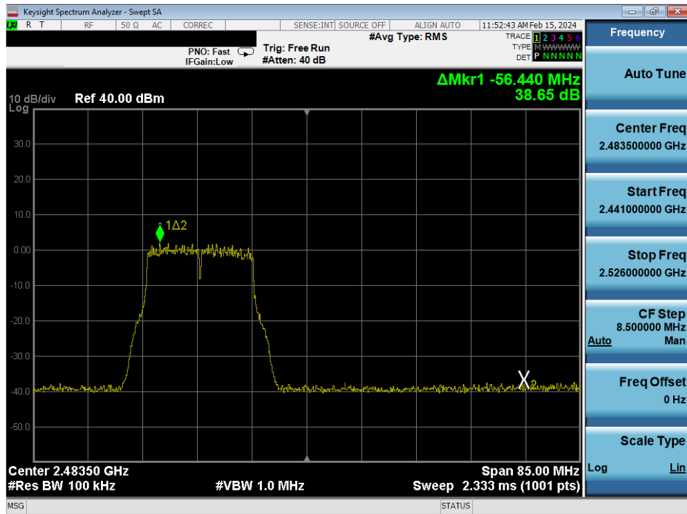
Plot 7-248. Band Edge Plot Antenna 4a (802.11g – Ch. 12) – 54Mbps
