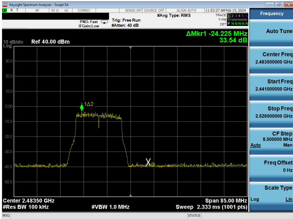
Plot 7-249. Band Edge Plot Antenna 4a (802.11g – Ch. 13) – 54Mbps
