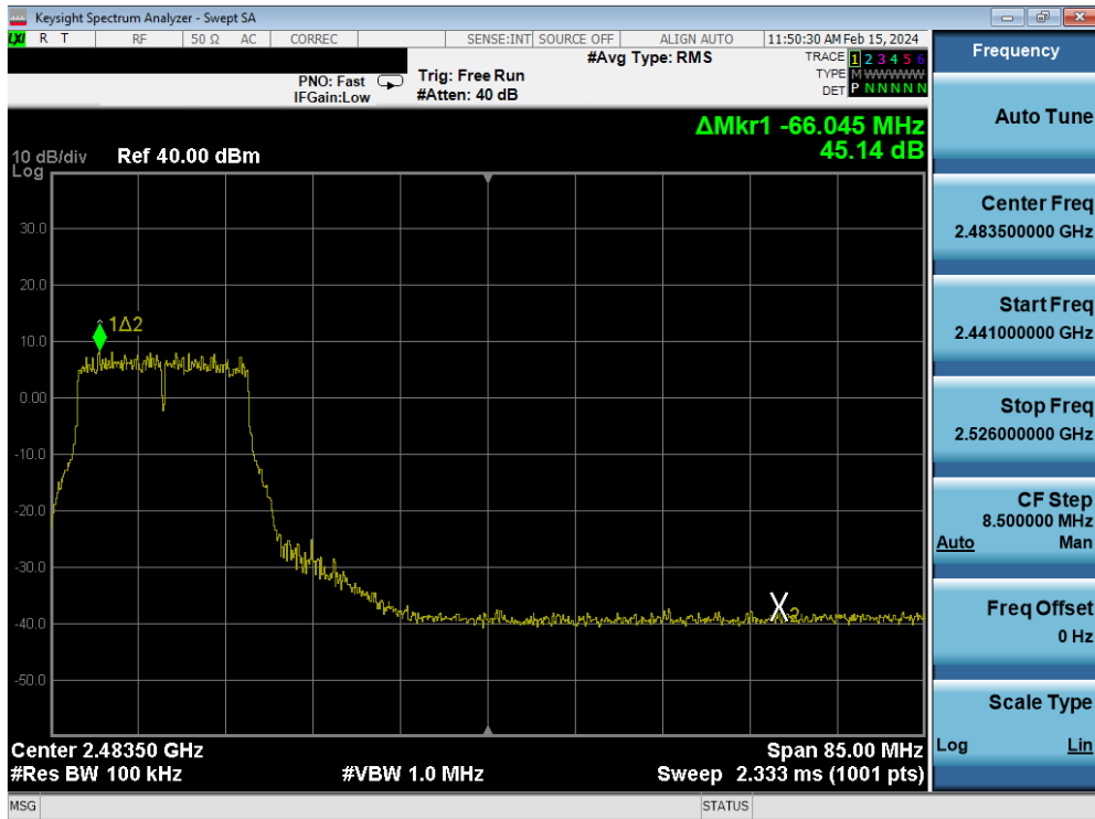
Plot 7-245. Band Edge Plot Antenna 4a (802.11g – Ch. 9) – 54Mbps
