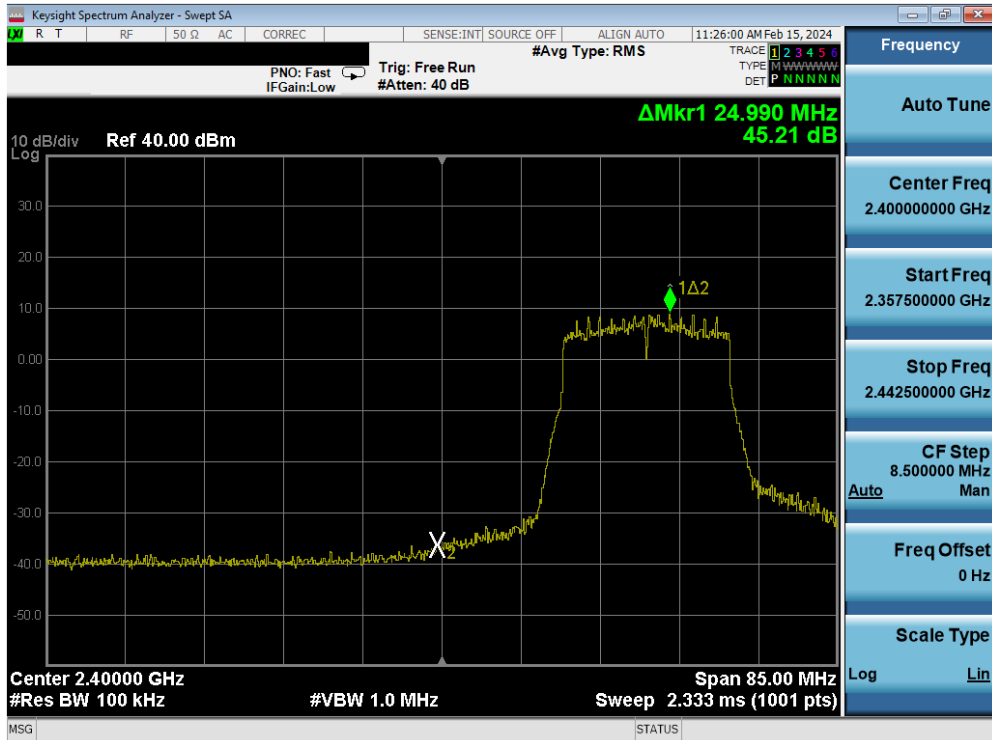
Plot 7-217. Band Edge Plot Antenna 4a (802.11n (2.4GHz) – Ch. 3) – MCS4
