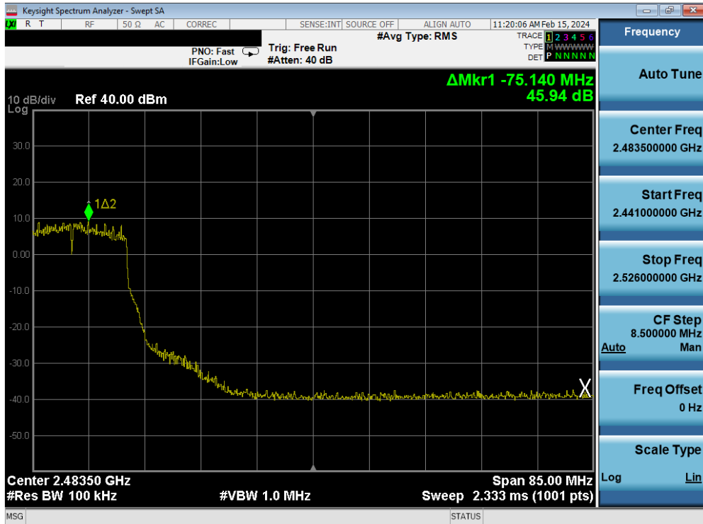
Plot 7-209. Band Edge Plot Antenna 4a (802.11g – Ch. 8) – 24Mbps
