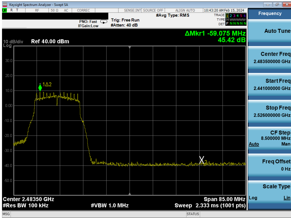
Plot 7-181. Band Edge Plot Antenna 4a (802.11g – Ch. 10) – 12Mbps
