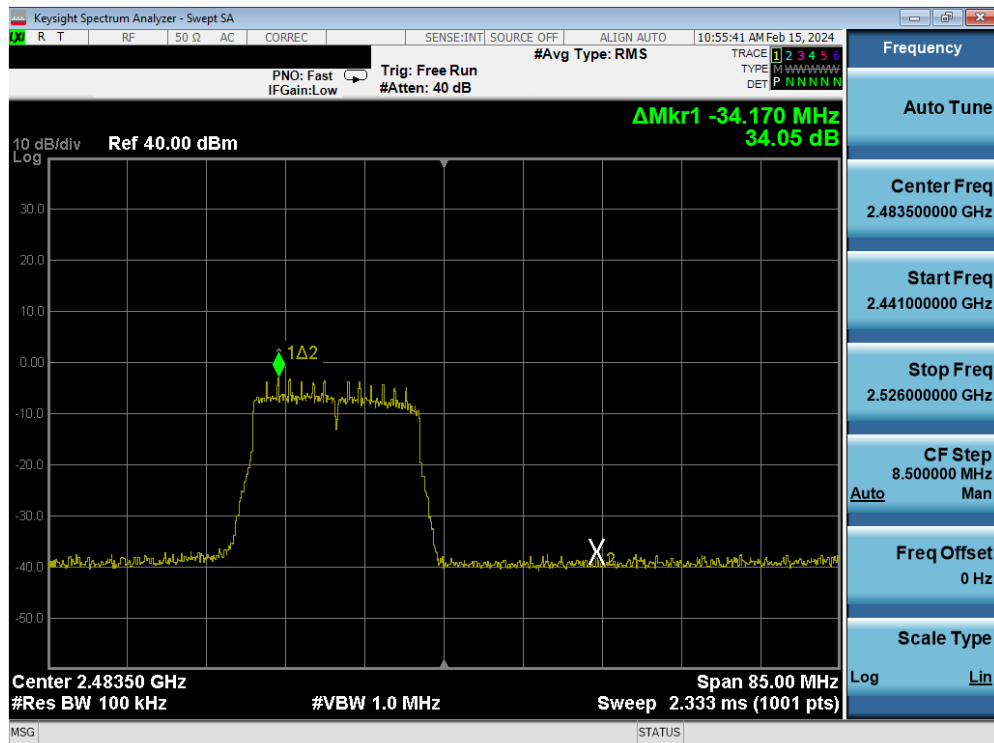
Plot 7-194. Band Edge Plot Antenna 4a (802.11n (2.4GHz) - Ch. 13) - MCS2
