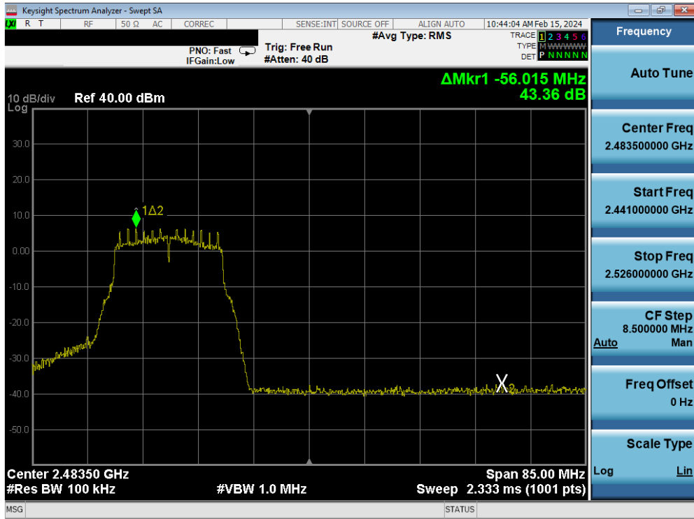
Plot 7-182. Band Edge Plot Antenna 4a (802.11g – Ch. 11) – 12Mbps
