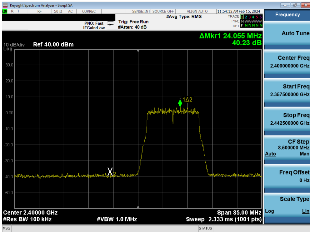
Plot 7-250. Band Edge Plot Antenna 4a (802.11n (2.4GHz) – Ch. 1) – MCS7
