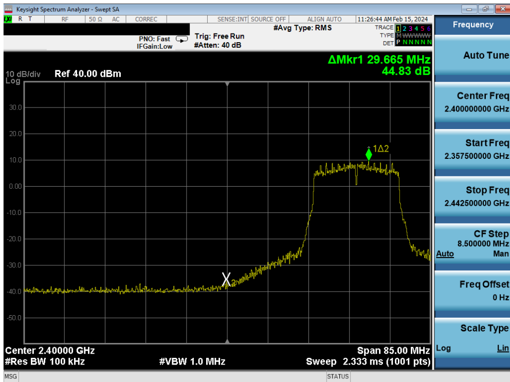
Plot 7-218. Band Edge Plot Antenna 4a (802.11n (2.4GHz) – Ch. 4) – MCS4
