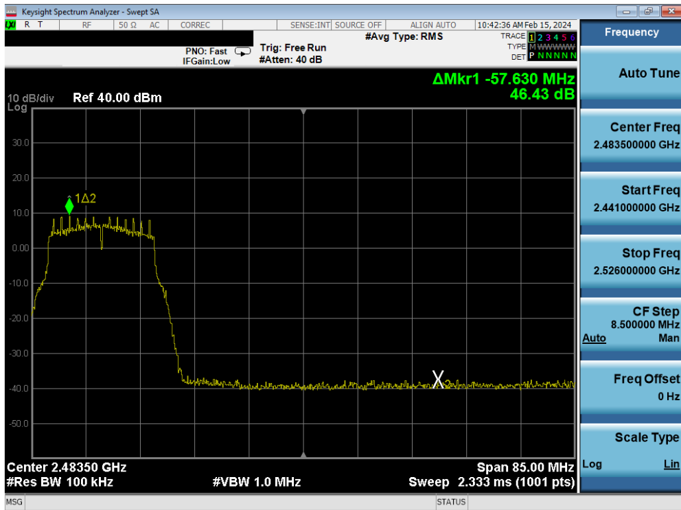
Plot 7-180. Band Edge Plot Antenna 4a (802.11g – Ch. 9) – 12Mbps
