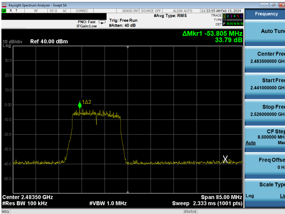
Plot 7-224. Band Edge Plot Antenna 4a (802.11n (2.4GHz) - Ch. 13) - MCS4
