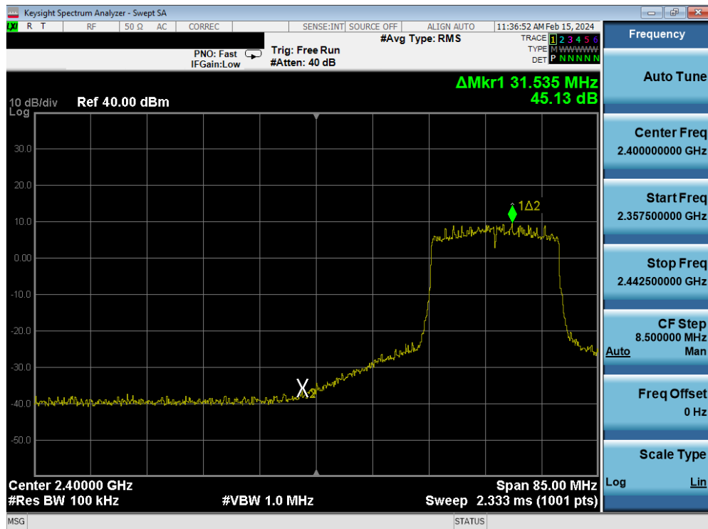
Plot 7-228. Band Edge Plot Antenna 4a (802.11ax (SU - 2.4GHz) – Ch. 4) – MCS4
