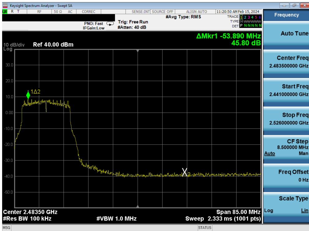
Plot 7-210. Band Edge Plot Antenna 4a (802.11g – Ch. 9) – 24Mbps
