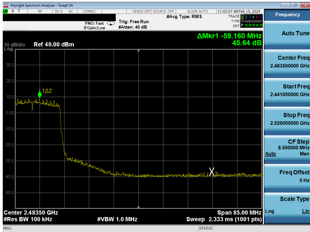
Plot 7-200. Band Edge Plot Antenna 4a (802.11ax (SU - 2.4GHz) – Ch. 8) – MCS2
