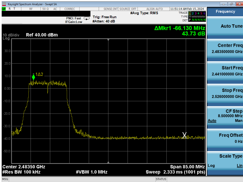
Plot 7-246. Band Edge Plot Antenna 4a (802.11g – Ch. 10) – 54Mbps
