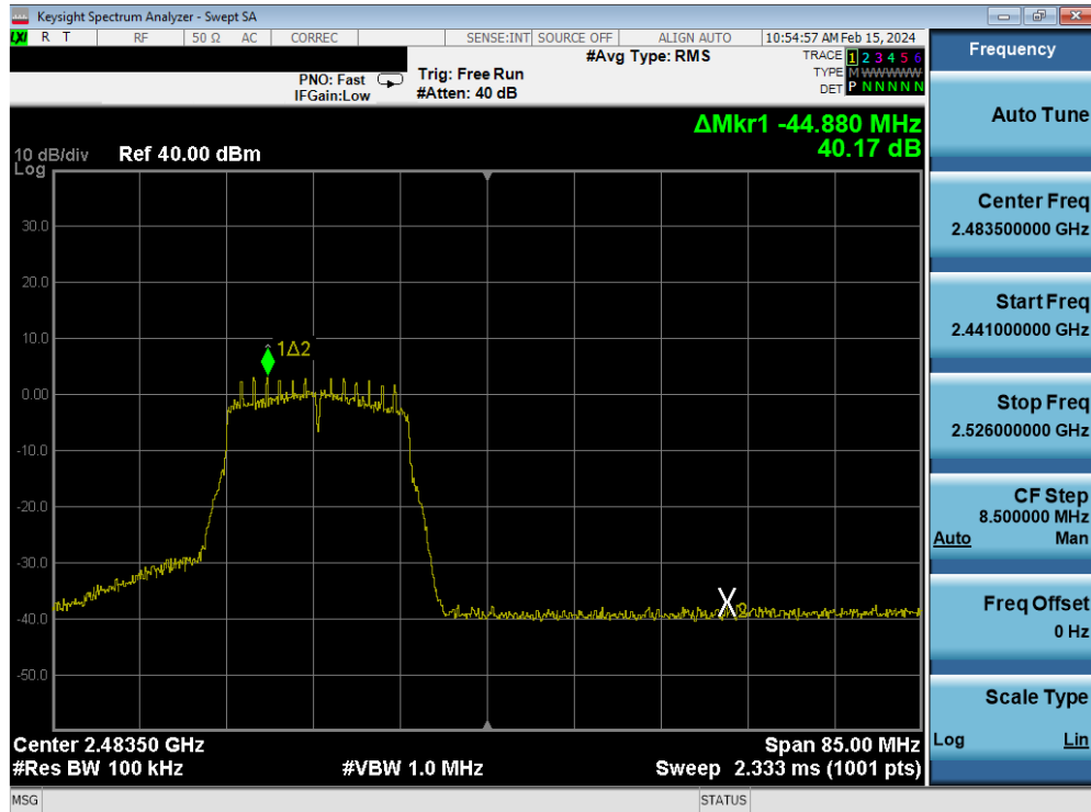
Plot 7-193. Band Edge Plot Antenna 4a (802.11n (2.4GHz) - Ch. 12) - MCS2
