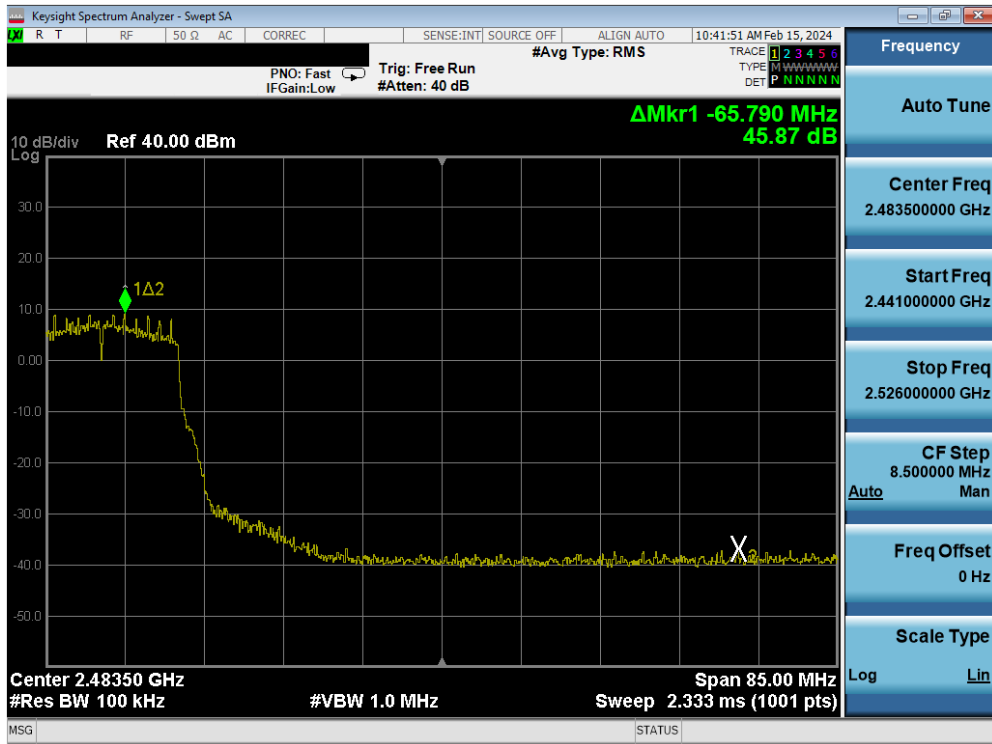
Plot 7-179. Band Edge Plot Antenna 4a (802.11g – Ch. 8) – 12Mbps
