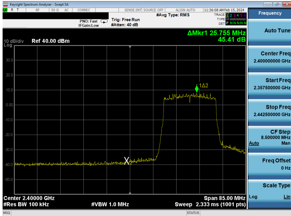
Plot 7-227. Band Edge Plot Antenna 4a (802.11ax (SU - 2.4GHz) – Ch. 3) – MCS4
