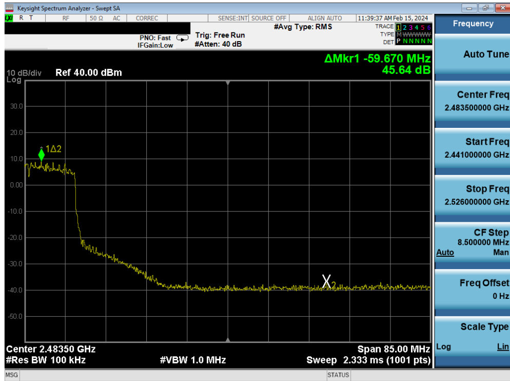
Plot 7-229. Band Edge Plot Antenna 4a (802.11ax (SU - 2.4GHz) – Ch. 7) – MCS4
