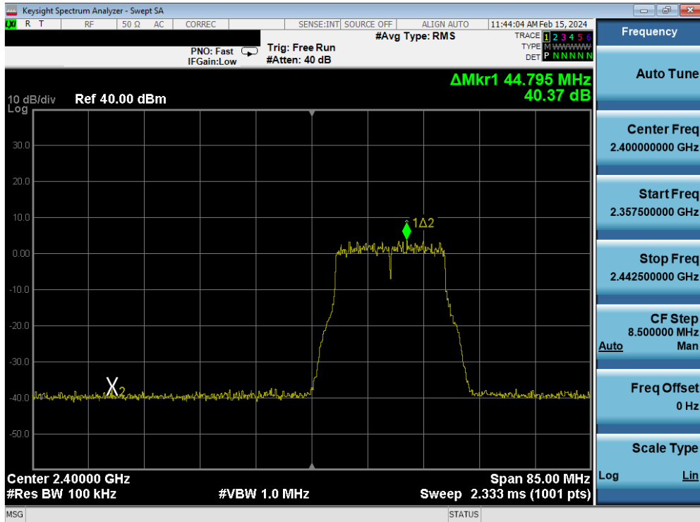
Plot 7-239. Band Edge Plot Antenna 4a (802.11g - Ch. 1) - 54Mbps
