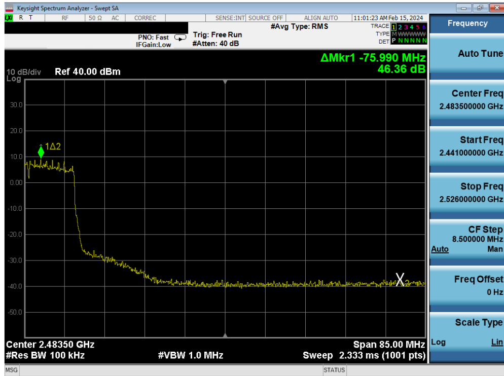
Plot 7-199. Band Edge Plot Antenna 4a (802.11ax (SU - 2.4GHz) – Ch. 7) – MCS2
