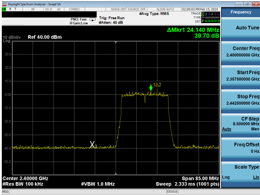
Plot 7-76. Band Edge Antenna 4a (802.11ax OFDMA – RU242 – Ch. 1)
