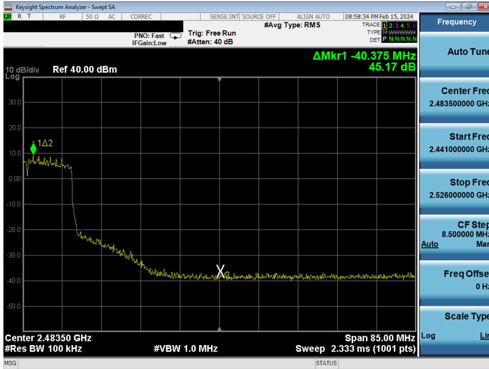
Plot 7-95. Band Edge Antenna 2a (802.11ax OFDMA – RU242 – Ch. 7)
