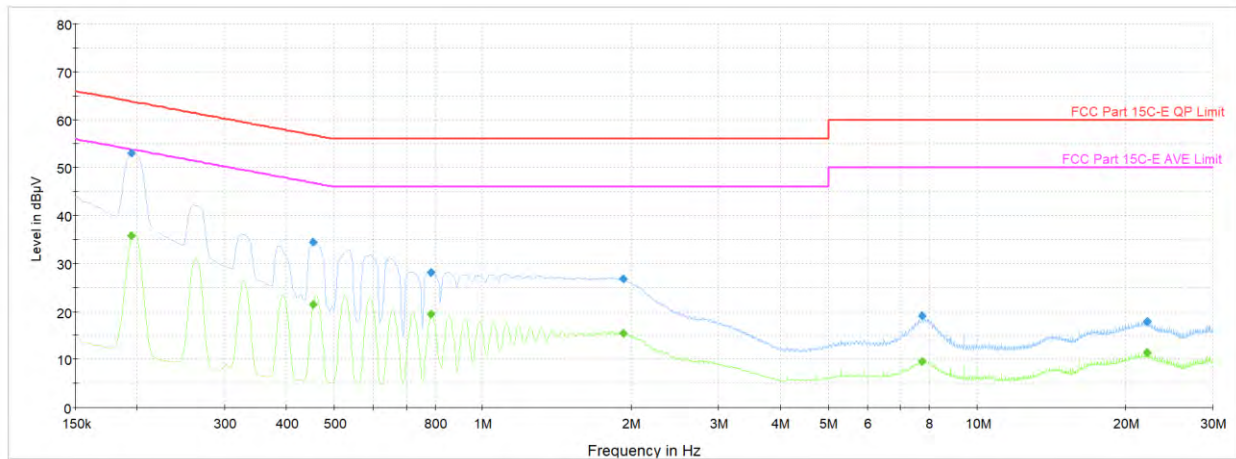
Plot 7-105. AC Line Conducted Plot with Bluetooth LE Tx BF (N, 1Mbps ePA – Ch.19, with AC/DC Adapter)
