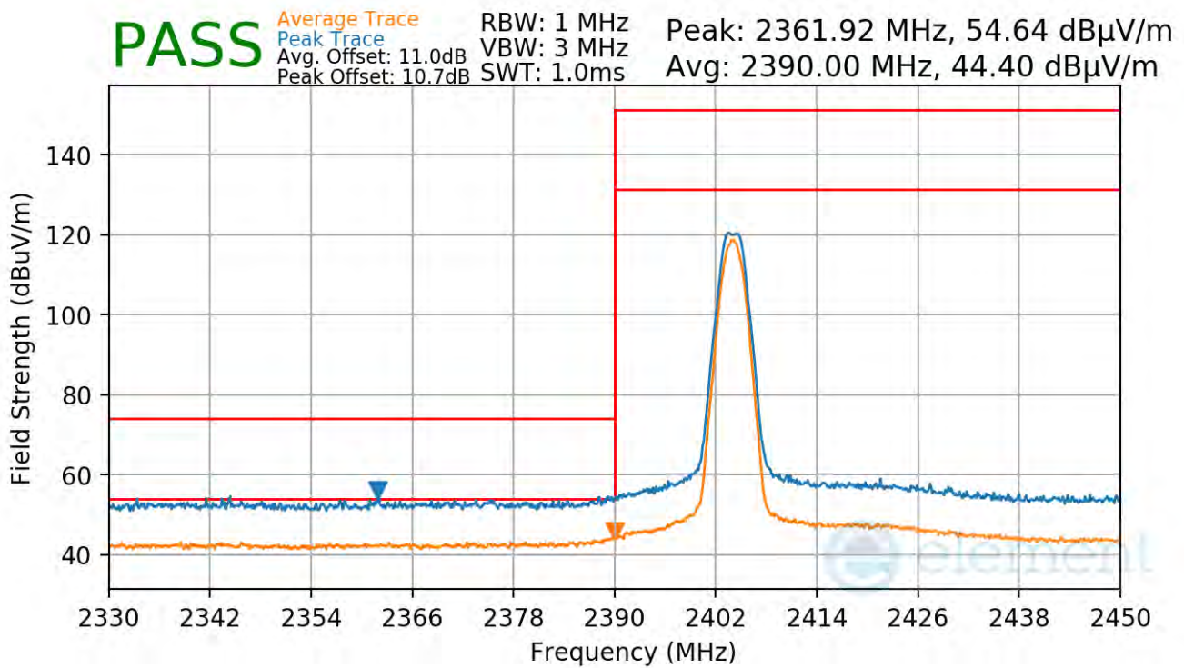
Plot 7-93. Radiated Restricted Lower Band Edge Measurement Antenna 4a (Average & Peak)
