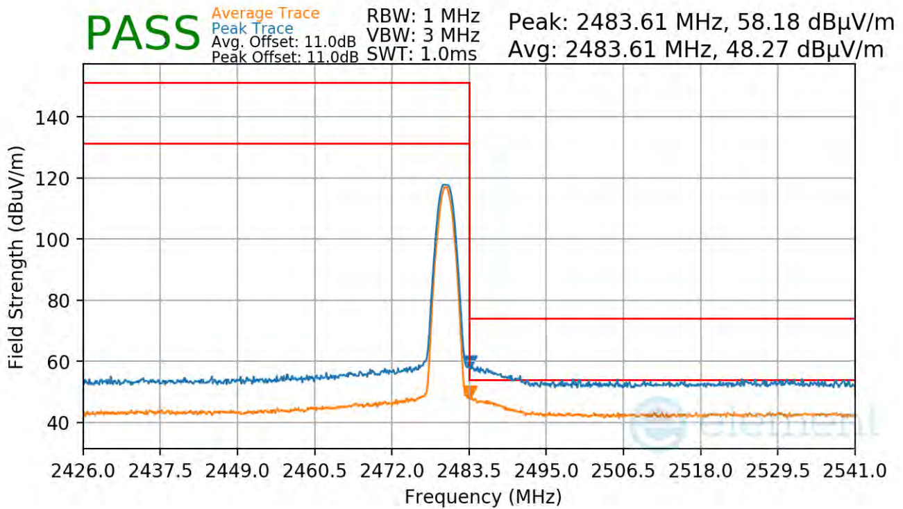
Plot 7-96. Radiated Restricted Upper Band Edge Measurement Antenna 2a (Average & Peak)
