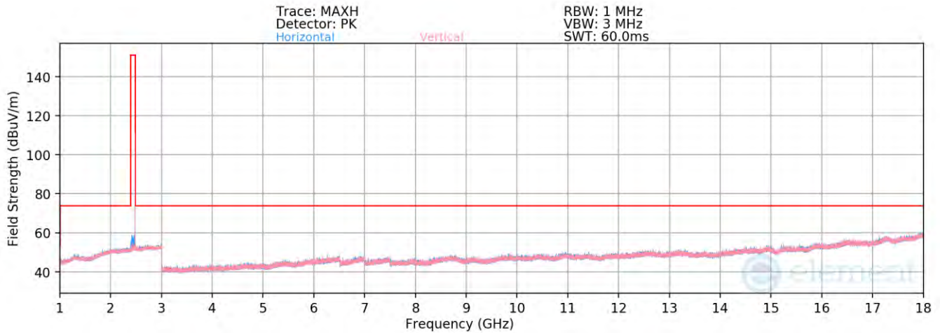
Plot 7-90. Radiated Spurious Emissions 1-18GHz TxBF (1Mbps ePA – Ch. 39)
