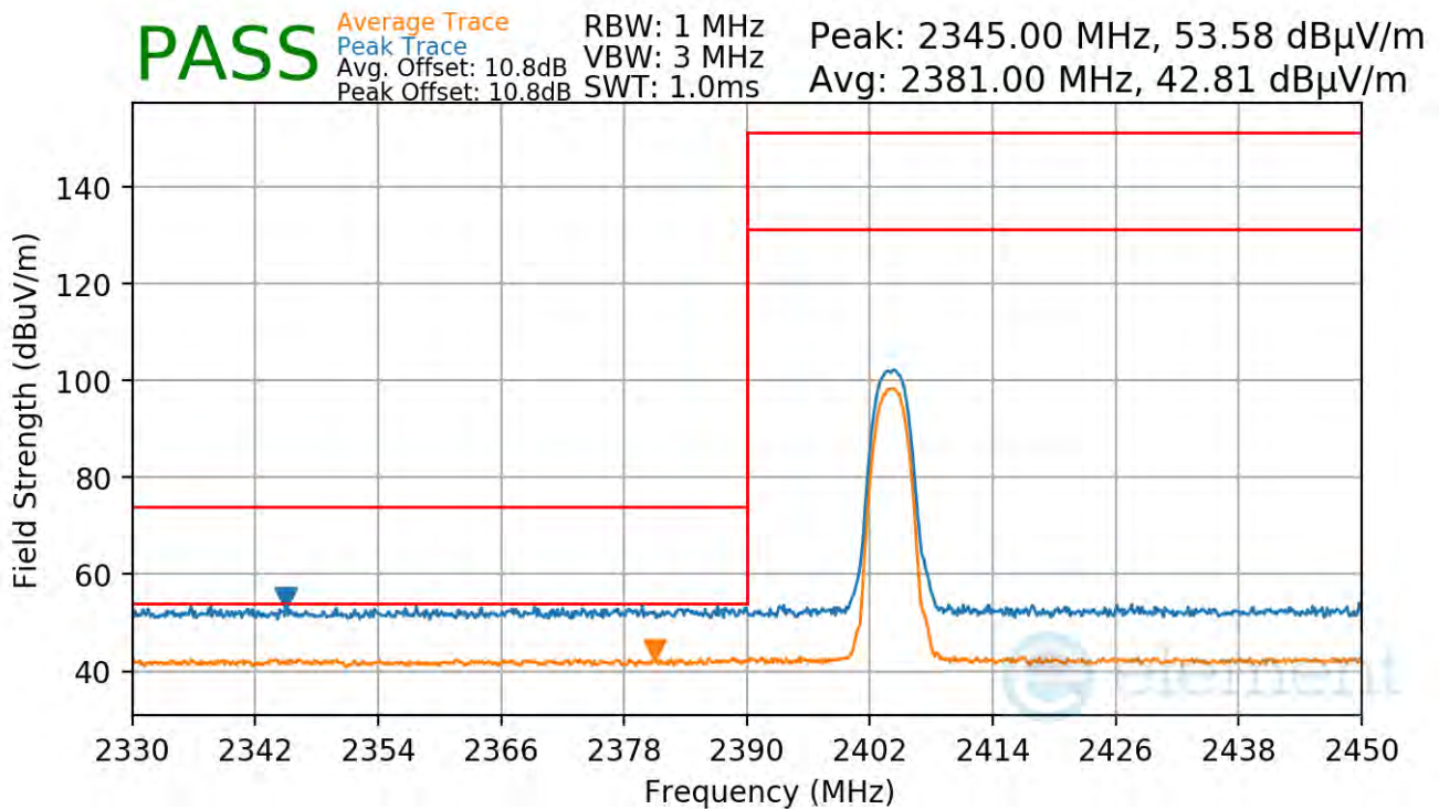
Plot 7-95. Radiated Restricted Lower Band Edge Measurement Antenna 2a
