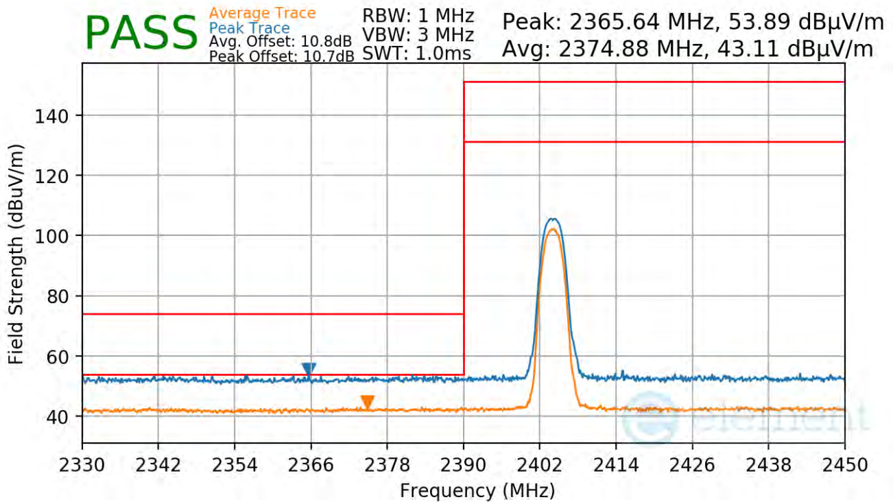
Plot 7-91. Radiated Restricted Lower Band Edge Measurement Antenna 4a
