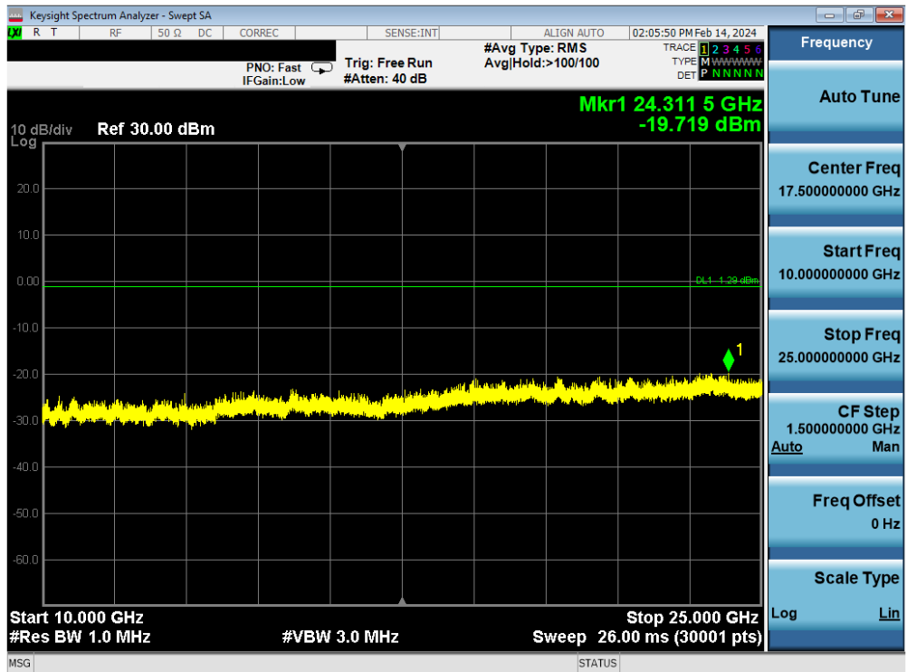
Plot 7-24. Conducted Spurious Antenna 4a (802.15.4, ePA – Ch. 11)
