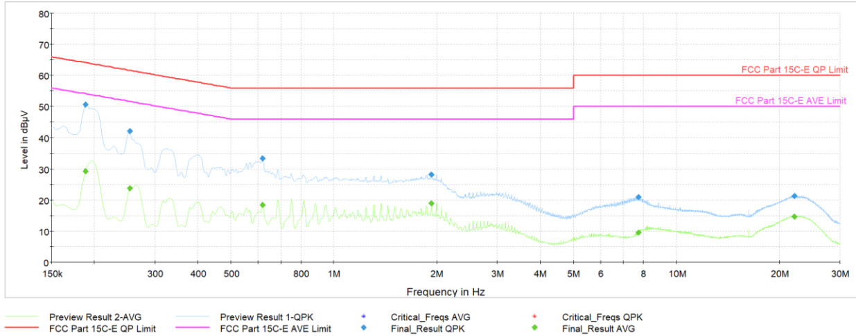
Plot 7-47. AC Line Conducted Emission with 802.15.4 Antenna 4a (L1, 250kbps, ePA - Ch25, with Laptop)
