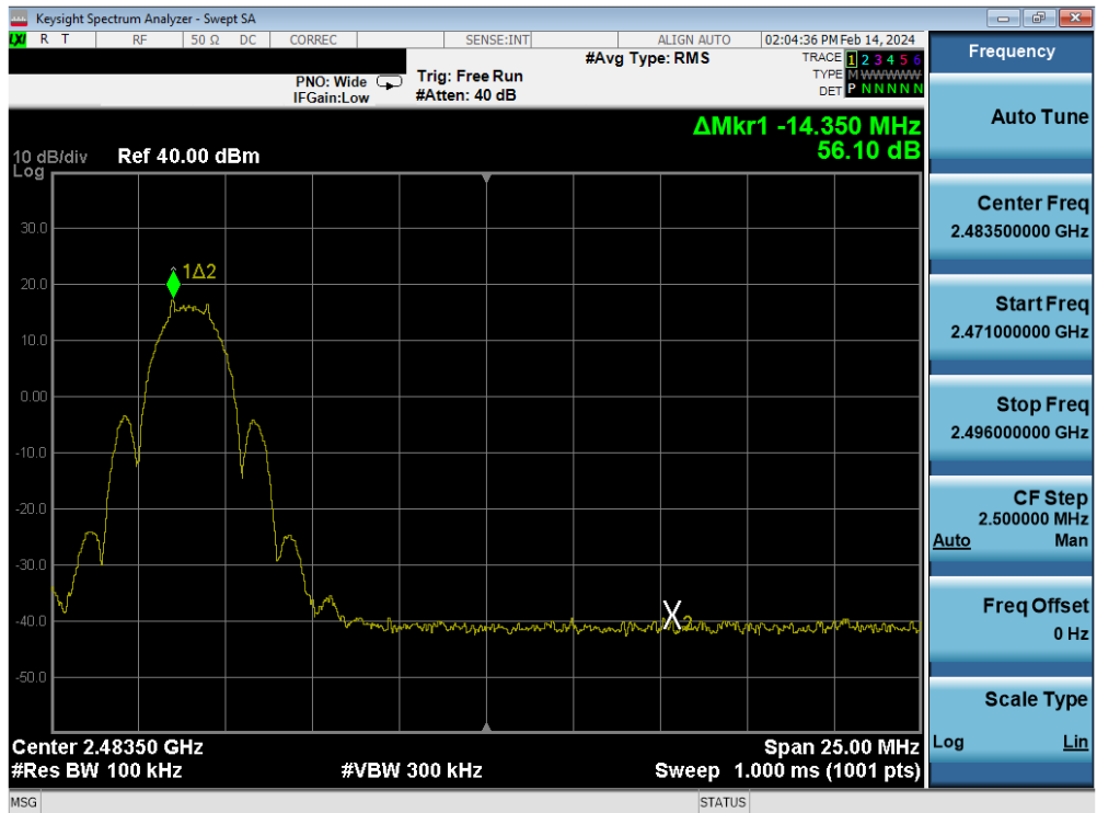
Plot 7-20. Band Edge Antenna 4a (802.15.4, ePA – Ch. 25)
