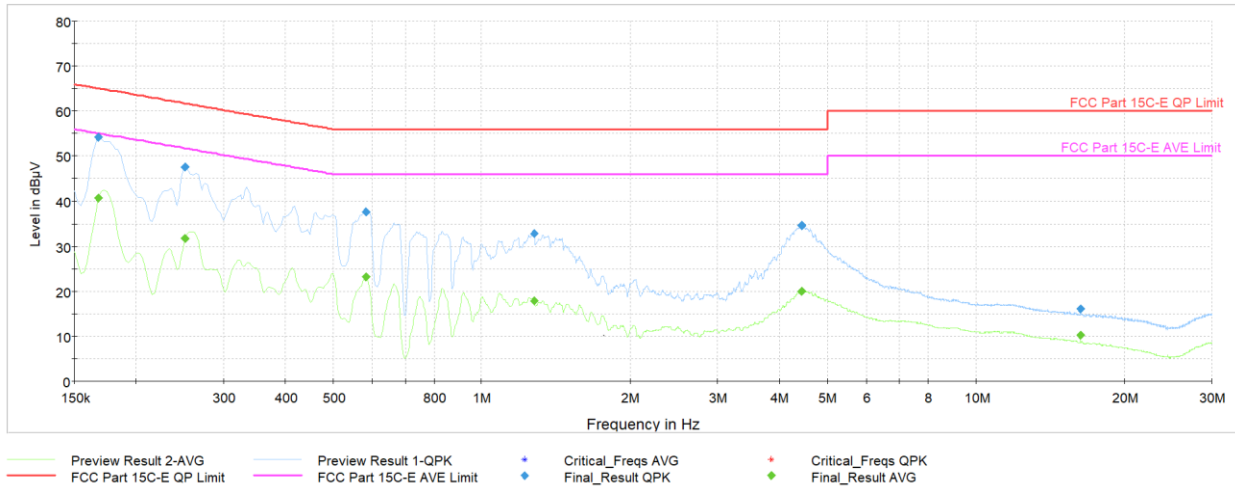
Plot 7-48. AC Line Conducted Emission with 802.15.4 Antenna 4a (N, 250kbps, ePA - Ch25, with Laptop)
