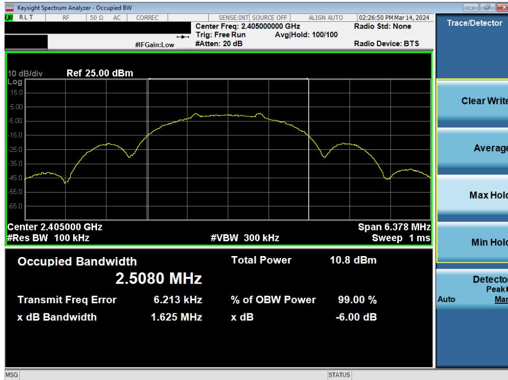
Plot 7-4. 6dB BW & 99% OBW Antenna 2a (802.15.4, Ch. 11)
