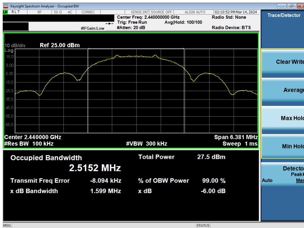
Plot 7-2. 6dB BW & 99% OBW Antenna 4a (802.15.4, Ch. 18)
