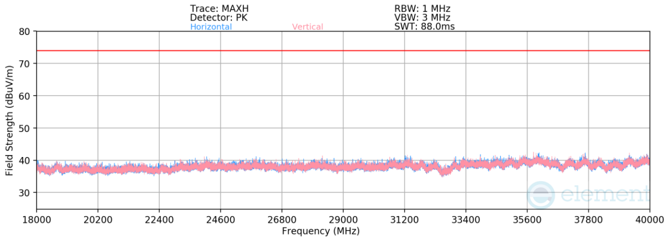
Plot 7-70. Radiated Spurious Emissions Above 18GHz - Simultaneous Transmission (Bluetooth + UNII)
