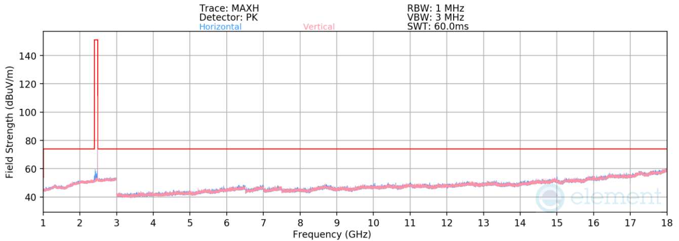
Plot 7-68. Radiated Spurious Emissions 1-18GHz, TxBF (BT GFSK ePA – Ch. 78)
