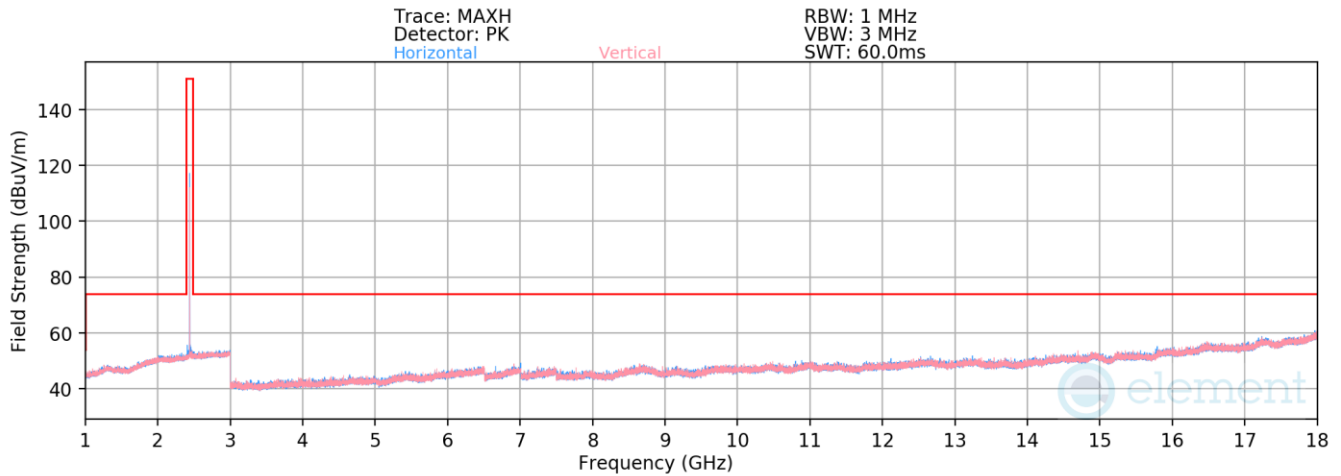
Plot 7-60. Radiated Spurious Emissions 1-18GHz, Antenna 4a (BT GFSK ePA – Ch. 39)
