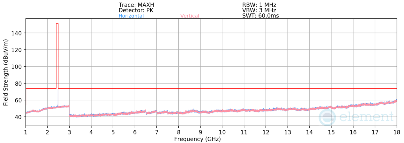
Plot 7-64. Radiated Spurious Emissions 1-18GHz, Antenna 2a (BT GFSK ePA – Ch. 78)
