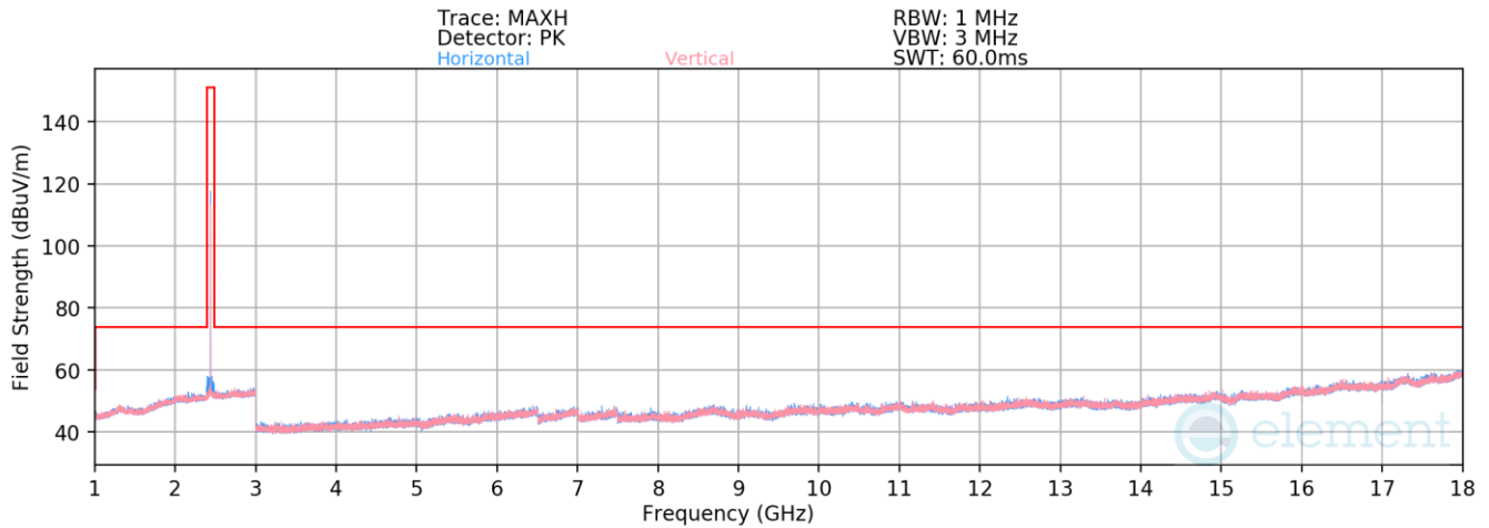
Plot 7-66. Radiated Spurious Emissions 1-18GHz, TxBF (BT GFSK ePA – Ch. 39)
