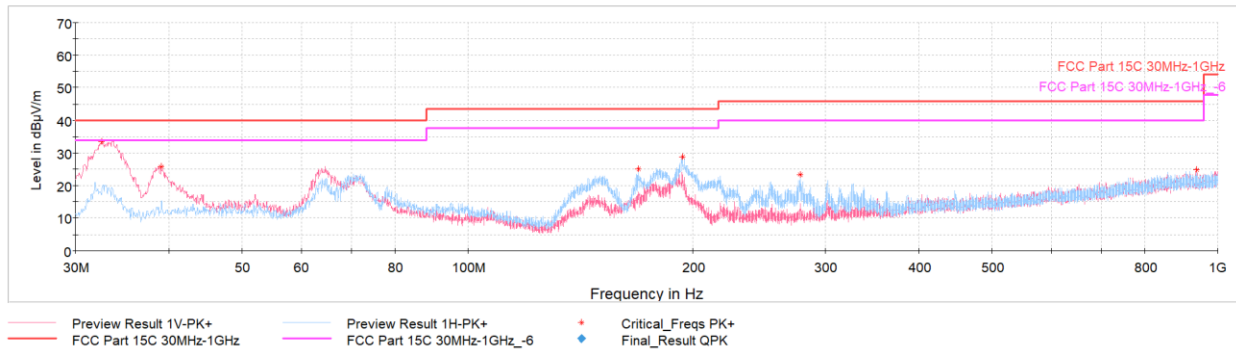
Plot 7-84. Worst Case Simultaneous Transmission Configuration
