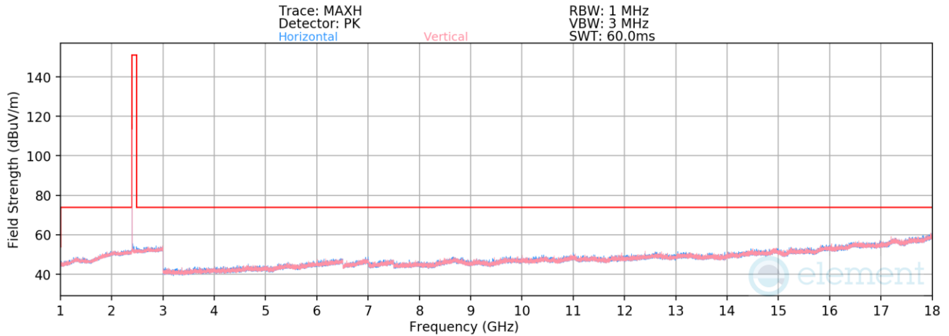
Plot 7-62. Radiated Spurious Emissions 1-18GHz, Antenna 2a (BT GFSK ePA – Ch. 0)
