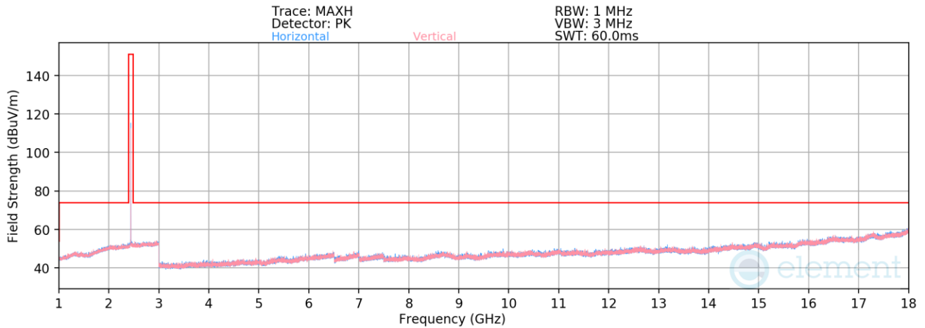
Plot 7-63. Radiated Spurious Emissions 1-18GHz, Antenna 2a (BT GFSK ePA – Ch. 39)
