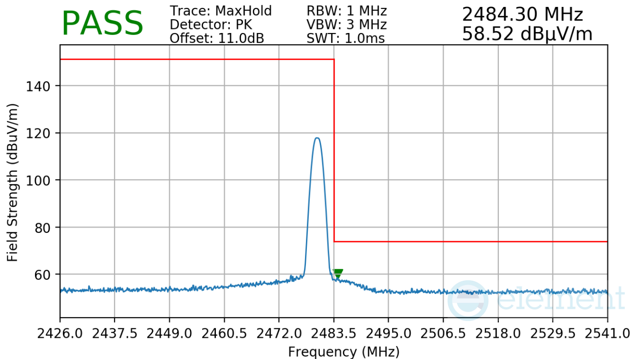
Plot 7-77. Radiated Restricted Upper Band Edge Measurement Antenna 2a
