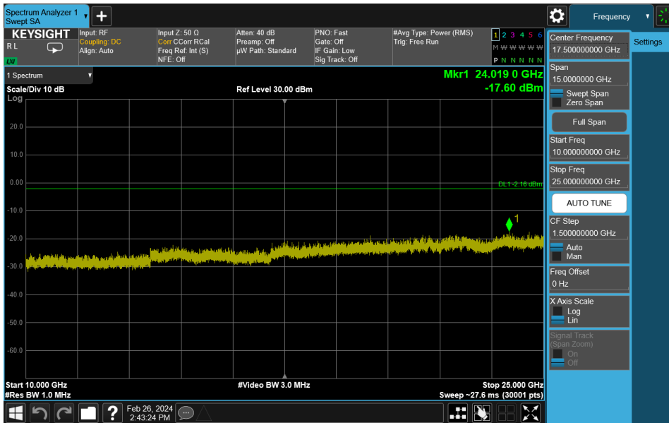
Plot 7-58. Conducted Simultaneous Tx Spurious Plot Antenna 2a (Bluetooth + UNII)
