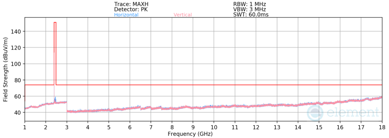
Plot 7-65. Radiated Spurious Emissions 1-18GHz, TxBF (BT GFSK ePA – Ch. 0)
