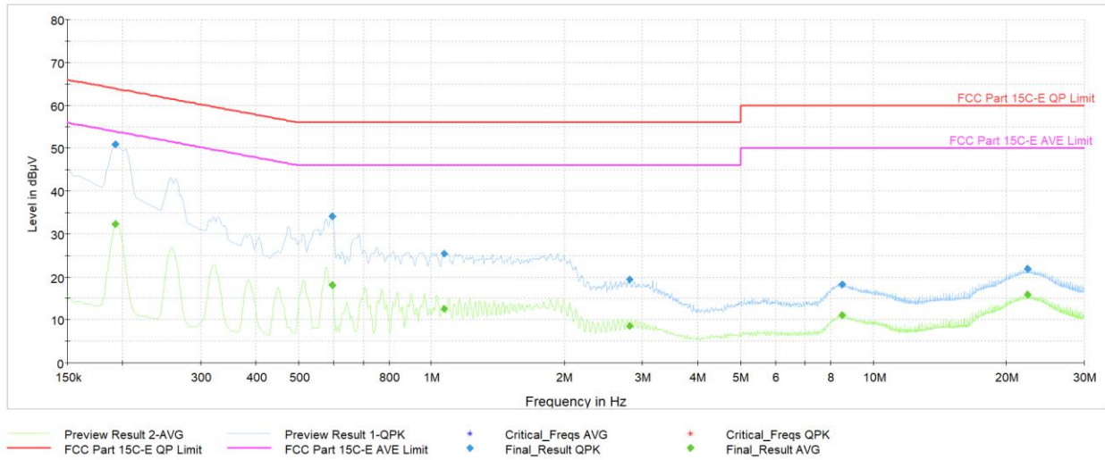
Plot 7-85. AC Line-Conducted Test Plot TxBF (L1, GFSK ePA – Ch.78, with Laptop)
