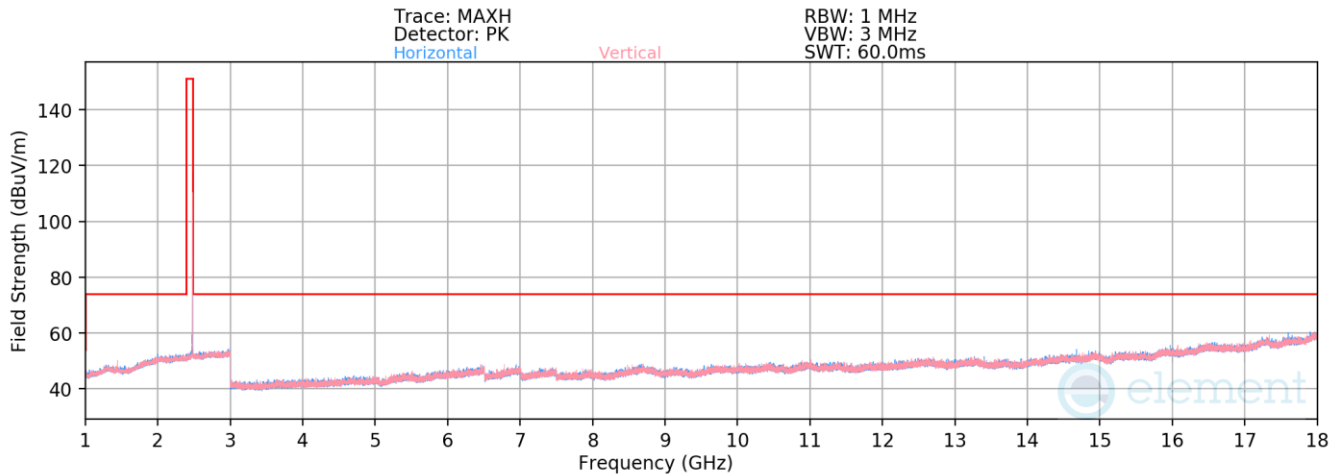
Plot 7-61. Radiated Spurious Emissions 1-18GHz, Antenna 4a (BT GFSK ePA – Ch. 78)
