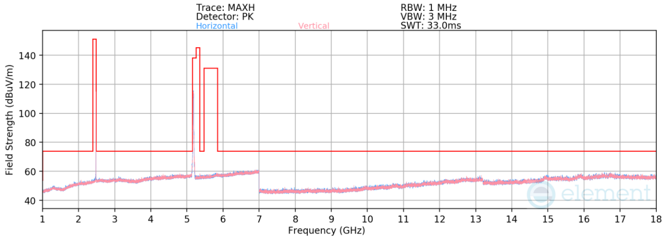
Plot 7-69. Radiated Spurious Emissions 1-18GHz - Simultaneous Transmission (Bluetooth + UNII)
