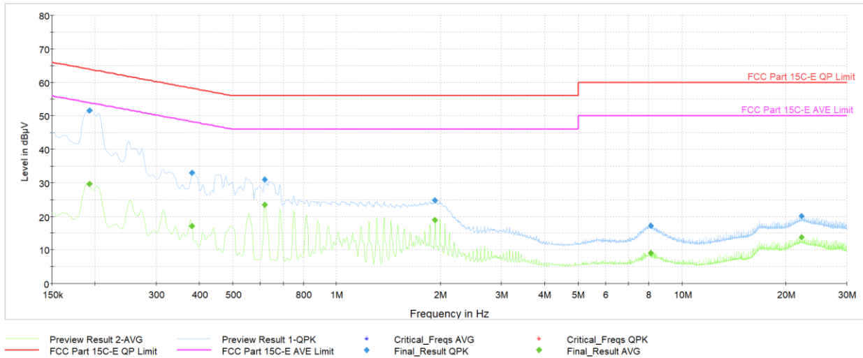
Plot 7-86. AC Line-Conducted Test Plot TxBF (N, GFSK ePA – Ch.78, with Laptop)
