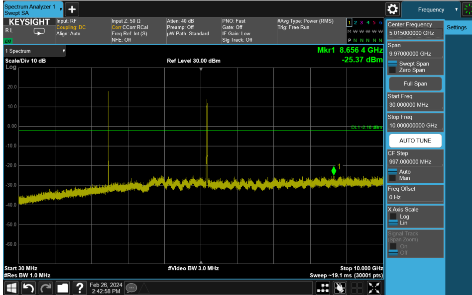
Plot 7-57. Conducted Simultaneous Tx Spurious Plot Antenna 2a (Bluetooth + UNII)
