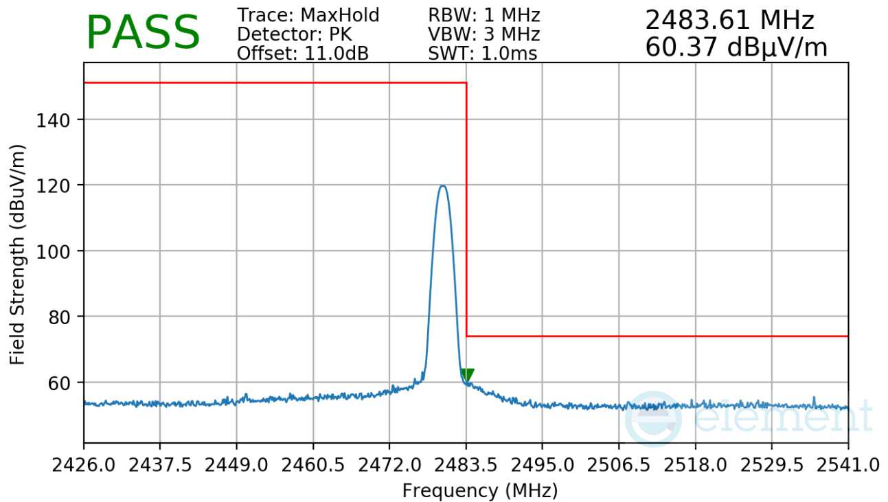
Plot 7-73. Radiated Restricted Upper Band Edge Measurement Antenna 4a
