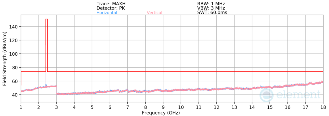
Plot 7-59. Radiated Spurious Emissions 1-18GHz, Antenna 4a (BT GFSK ePA – Ch. 0)
