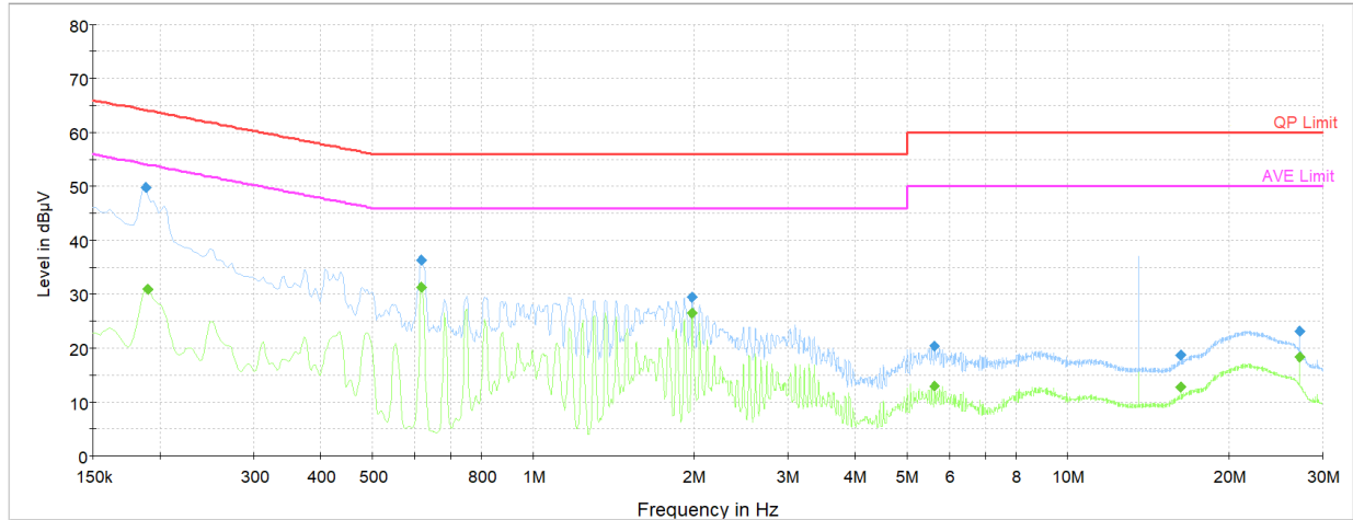
Plot 7-5. AC Line-Conducted Plot (N, Charging Rate 2.6C, with AC/DC Adapter)
