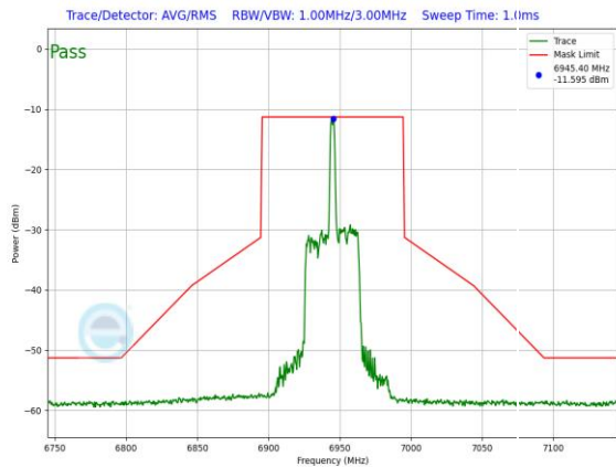
Plot 7-1524. LPI In-Band Emission Plot SDM Diversity Antenna WF7 (80MHz 802.11ax RU26 (UNII Band 8) – Ch. 199)
