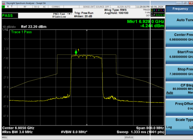
Plot 7-1535. LPI In-Band Emission Plot SDM Diversity Antenna WF5B (160MHz 802.11ax RU996x2 (UNII Band 8) – Ch. 207)
