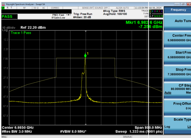
Plot 7-1531. LPI In-Band Emission Plot SDM Diversity Antenna WF5B (160MHz 802.11ax RU26 (UNII Band 8) – Ch. 207)
