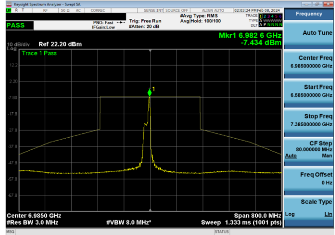
Plot 7-1532. LPI In-Band Emission Plot SDM Diversity Antenna WF7 (160MHz 802.11ax RU26 (UNII Band 8) – Ch. 207)
