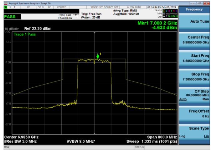
Plot 7-1536. LPI In-Band Emission Plot SDM Diversity Antenna WF7 (160MHz 802.11ax RU996x2 (UNII Band 8) – Ch. 207)
