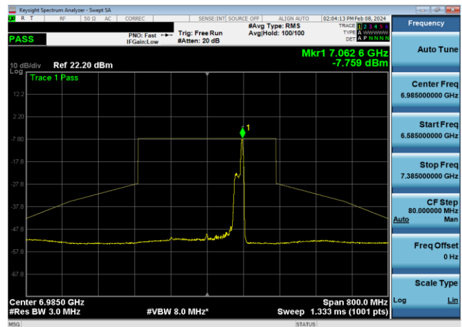
Plot 7-1534. LPI In-Band Emission Plot SDM Diversity Antenna WF7 (160MHz 802.11ax RU26 (UNII Band 8) – Ch. 207)
