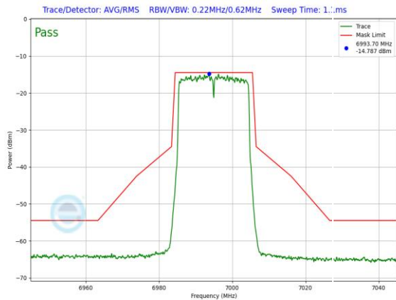
Plot 7-1512. LPI In-Band Emission Plot SDM Diversity Antenna WF7 (20MHz 802.11ax RU242 (UNII Band 8) – Ch. 209)
