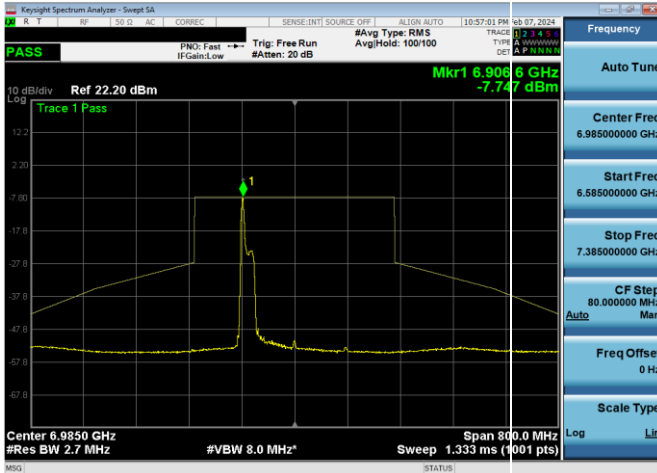
Plot 7-1402. LPI In-Band Emission Plot SDM Primary Antenna WF8 (160MHz 802.11ax RU26 (UNII Band 8) – Ch. 207)
