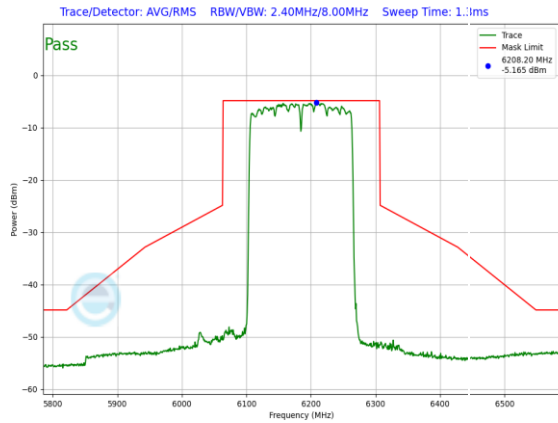
Plot 7-1439. LPI In-Band Emission Plot SDM Diversity Antenna WF5B (160MHz 802.11ax RU996x2 (UNII Band 5) – Ch. 47)
