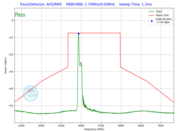
Plot 7-1497. LPI In-Band Emission Plot SDM Diversity Antenna WF5B (160MHz 802.11ax RU26 (UNII Band 7) – Ch. 143)
