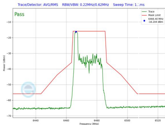
Plot 7-1441. LPI In-Band Emission Plot SDM Diversity Antenna WF5B (20MHz 802.11ax RU26 (UNII Band 6) – Ch. 105)
