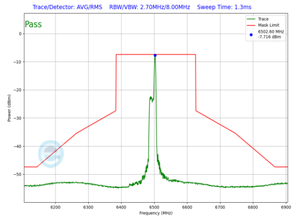
Plot 7-1467. LPI In-Band Emission Plot SDM Diversity Antenna WF5B (160MHz 802.11ax RU26 (UNII Band 6) – Ch. 111)
