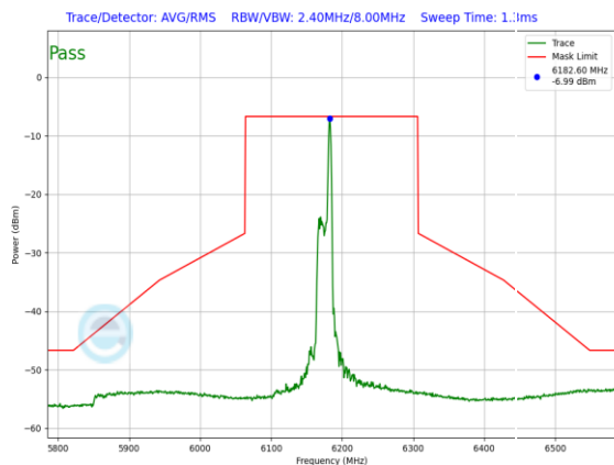
Plot 7-1435. LPI In-Band Emission Plot SDM Diversity Antenna WF5B (160MHz 802.11ax RU26 (UNII Band 5) – Ch. 47)
