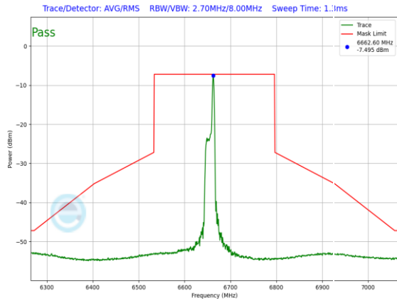
Plot 7-1499. LPI In-Band Emission Plot SDM Diversity Antenna WF5B (160MHz 802.11ax RU26 (UNII Band 7) – Ch. 143)
