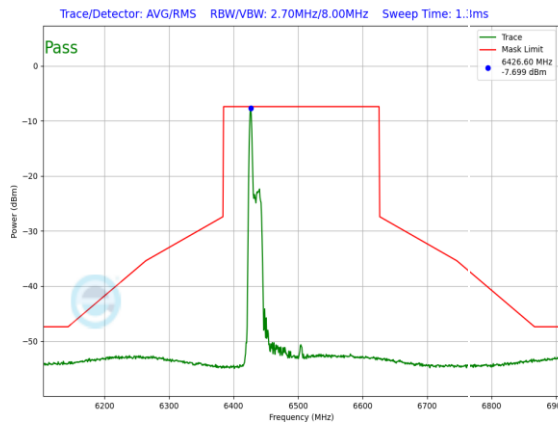
Plot 7-1465. LPI In-Band Emission Plot SDM Diversity Antenna WF5B (160MHz 802.11ax RU26 (UNII Band 6) – Ch. 111)
