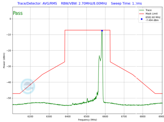
Plot 7-1469. LPI In-Band Emission Plot SDM Diversity Antenna WF5B (160MHz 802.11ax RU26 (UNII Band 6) – Ch. 111)
