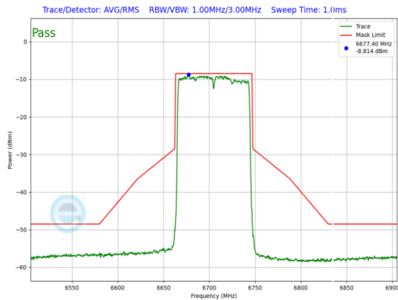
Plot 7-1495. LPI In-Band Emission Plot SDM Diversity Antenna WF5B (80MHz 802.11ax RU96 (UNII Band 7) – Ch. 151)
