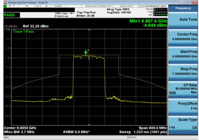
Plot 7-1408. LPI In-Band Emission Plot SDM Primary Antenna WF8 (160MHz 802.11ax RU996x2 (UNII Band 8) – Ch. 207)
