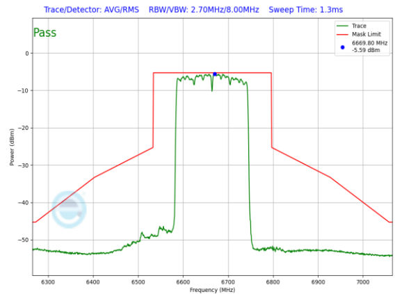
Plot 7-1503. LPI In-Band Emission Plot SDM Diversity Antenna WF5B (160MHz 802.11ax RU996x2 (UNII Band 7) – Ch. 143)
