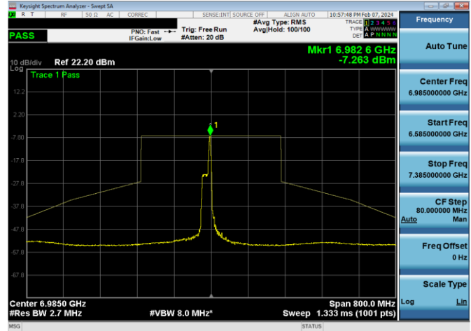
Plot 7-1404. LPI In-Band Emission Plot SDM Primary Antenna WF8 (160MHz 802.11ax RU26 (UNII Band 8) – Ch. 207)
