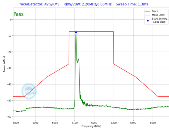
Plot 7-1434. LPI In-Band Emission Plot SDM Diversity Antenna WF7 (160MHz 802.11ax RU26 (UNII Band 5) – Ch. 47)
