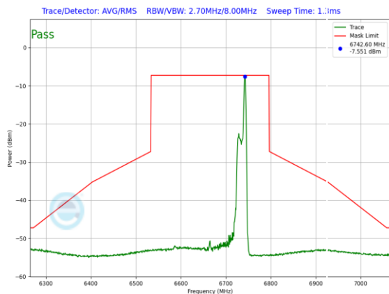
Plot 7-1501. LPI In-Band Emission Plot SDM Diversity Antenna WF5B (160MHz 802.11ax RU26 (UNII Band 7) – Ch. 143)
