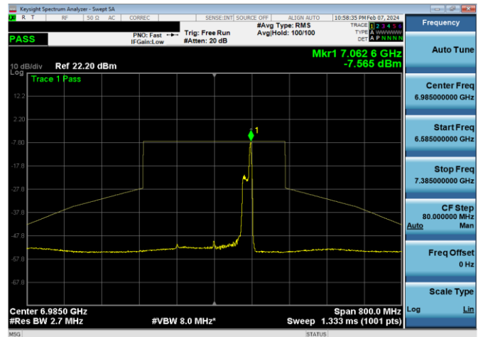
Plot 7-1406. LPI In-Band Emission Plot SDM Primary Antenna WF8 (160MHz 802.11ax RU26 (UNII Band 8) – Ch. 207)
