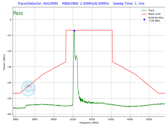
Plot 7-1433. LPI In-Band Emission Plot SDM Diversity Antenna WF5B (160MHz 802.11ax RU26 (UNII Band 5) – Ch. 47)
