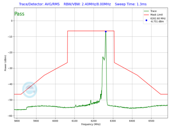
Plot 7-1437. LPI In-Band Emission Plot SDM Diversity Antenna WF5B (160MHz 802.11ax RU26 (UNII Band 5) – Ch. 47)
