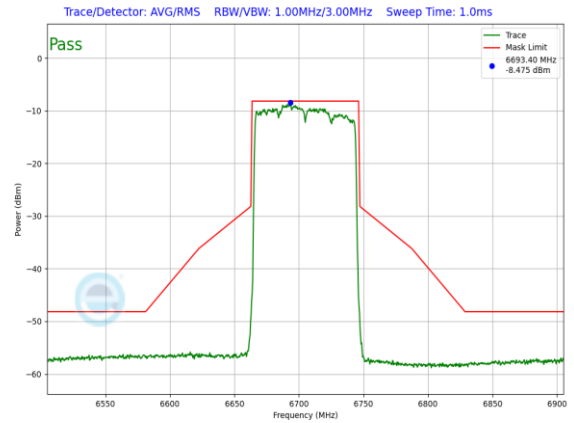
Plot 7-1496. LPI In-Band Emission Plot SDM Diversity Antenna WF7 (80MHz 802.11ax RU96 (UNII Band 7) – Ch. 151)
