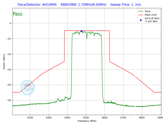
Plot 7-1471. LPI In-Band Emission Plot SDM Diversity Antenna WF5B (160MHz 802.11ax RU996x2 (UNII Band 6) – Ch. 111)
