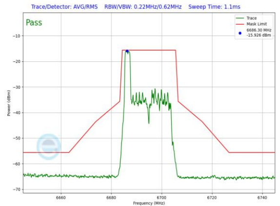
Plot 7-1473. LPI In-Band Emission Plot SDM Diversity Antenna WF5B (20MHz 802.11ax RU26 (UNII Band 7) – Ch. 149)
