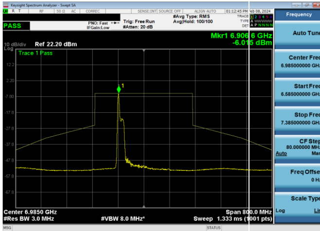
Plot 7-1277. LPI In-Band Emission Plot Antenna WF7 (160MHz 802.11ax RU26 (UNII Band 8) – Ch. 207)
