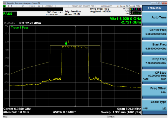
Plot 7-1280. LPI In-Band Emission Plot Antenna WF7 (160MHz 802.11ax RU996x2 (UNII Band 8) – Ch. 207)
