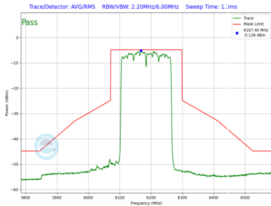
Plot 7-1312. LPI In-Band Emission Plot SDM Primary Antenna WF8 (160MHz 802.11ax RU996x2 (UNII Band 5) – Ch. 47)
