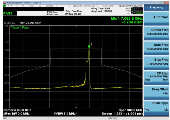
Plot 7-1279. LPI In-Band Emission Plot Antenna WF7 (160MHz 802.11ax RU26 (UNII Band 8) – Ch. 207)
