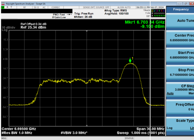
Plot 7-805. LPI Power Spectral Density Plot SDM Diversity Antenna WF8 (20MHz 802.11ax RU26 (UNII Band 7) – Ch. 149)
