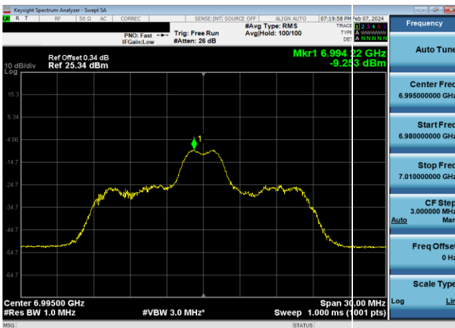
Plot 7-835. LPI Power Spectral Density Plot SDM Diversity Antenna WF8 (20MHz 802.11ax RU26 (UNII Band 8) – Ch. 209)
