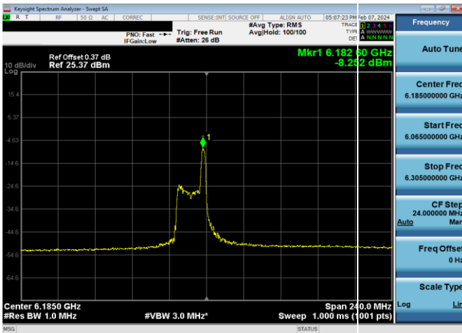
Plot 7-763. LPI Power Spectral Density Plot SDM Diversity Antenna WF8 (160MHz 802.11ax RU26 (UNII Band 5) – Ch. 47)
