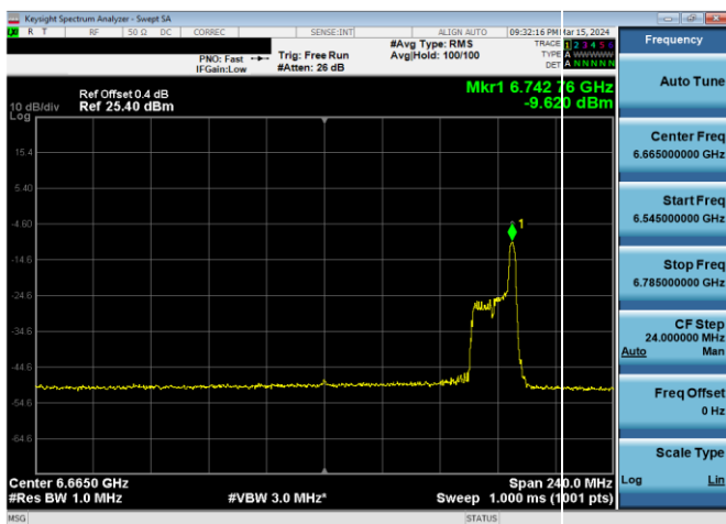
Plot 7-829. LPI Power Spectral Density Plot SDM Diversity Antenna WF8 (160MHz 802.11ax RU26 (UNII Band 7) – Ch. 143)
