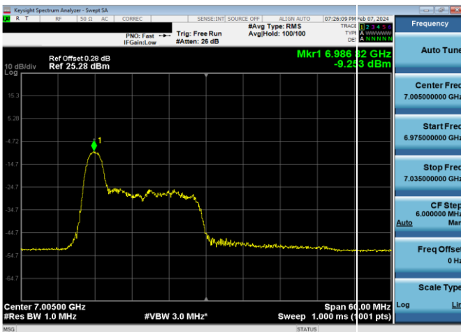
Plot 7-841. LPI Power Spectral Density Plot SDM Diversity Antenna WF8 (40MHz 802.11ax RU26 (UNII Band 8) – Ch. 211)
