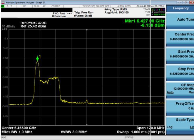
Plot 7-785. LPI Power Spectral Density Plot SDM Diversity Antenna WF8 (80MHz 802.11ax RU26 (UNII Band 6) – Ch. 103)
