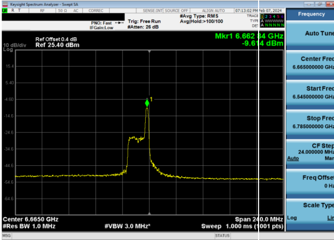
Plot 7-827. LPI Power Spectral Density Plot SDM Diversity Antenna WF8 (160MHz 802.11ax RU26 (UNII Band 7) – Ch. 143)
