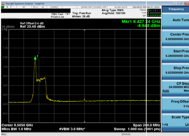
Plot 7-793. LPI Power Spectral Density Plot SDM Diversity Antenna WF8 (160MHz 802.11ax RU26 (UNII Band 6) – Ch. 111)
