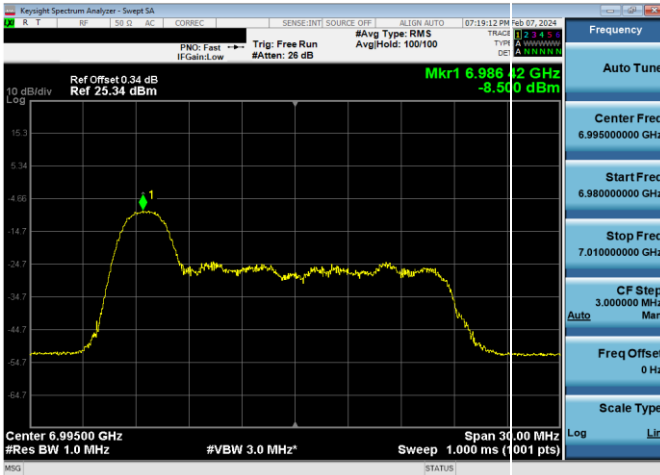
Plot 7-833. LPI Power Spectral Density Plot SDM Diversity Antenna WF8 (20MHz 802.11ax RU26 (UNII Band 8) – Ch. 209)
