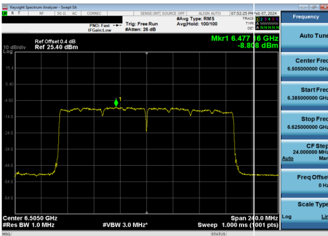
Plot 7-799. LPI Power Spectral Density Plot SDM Diversity Antenna WF8 (160MHz 802.11ax RU996x2 (UNII Band 6) – Ch. 111)
