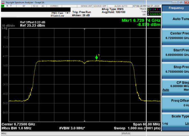
Plot 7-815. LPI Power Spectral Density Plot SDM Diversity Antenna WF8 (40MHz 802.11ax RU484 (UNII Band 7) – Ch. 155)
