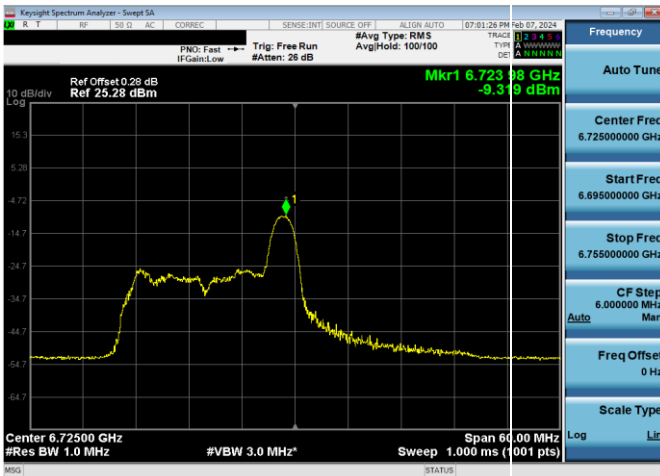
Plot 7-811. LPI Power Spectral Density Plot SDM Diversity Antenna WF8 (40MHz 802.11ax RU26 (UNII Band 7) – Ch. 155)
