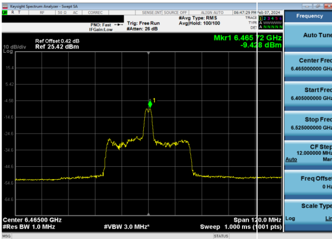
Plot 7-787. LPI Power Spectral Density Plot SDM Diversity Antenna WF8 (80MHz 802.11ax RU26 (UNII Band 6) – Ch. 103)
