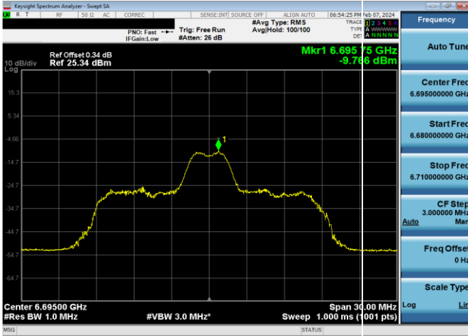
Plot 7-803. LPI Power Spectral Density Plot SDM Diversity Antenna WF8 (20MHz 802.11ax RU26 (UNII Band 7) – Ch. 149)
