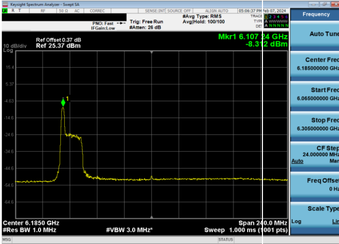
Plot 7-761. LPI Power Spectral Density Plot SDM Diversity Antenna WF8 (160MHz 802.11ax RU26 (UNII Band 5) – Ch. 47)
