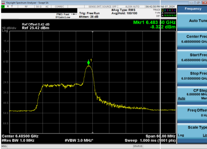
Plot 7-779. LPI Power Spectral Density Plot SDM Diversity Antenna WF8 (40MHz 802.11ax RU26 (UNII Band 6) – Ch. 107)
