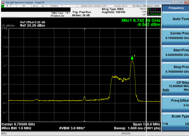
Plot 7-821. LPI Power Spectral Density Plot SDM Diversity Antenna WF8 (80MHz 802.11ax RU26 (UNII Band 7) – Ch. 151)
