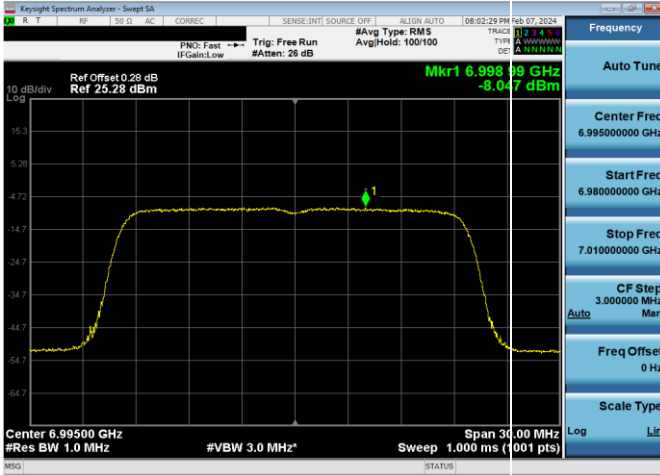
Plot 7-839. LPI Power Spectral Density Plot SDM Diversity Antenna WF8 (20MHz 802.11ax RU242 (UNII Band 8) – Ch. 209)
