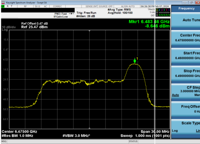
Plot 7-773. LPI Power Spectral Density Plot SDM Diversity Antenna WF8 (20MHz 802.11ax RU26 (UNII Band 6) – Ch. 105)
