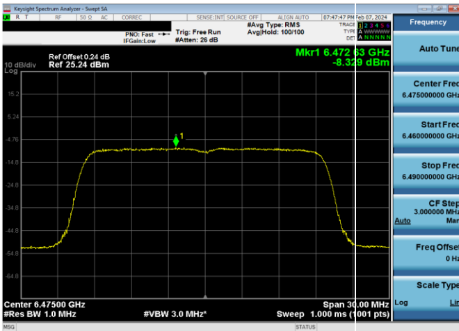
Plot 7-775. LPI Power Spectral Density Plot SDM Diversity Antenna WF8 (20MHz 802.11ax RU242 (UNII Band 6) – Ch. 105)
