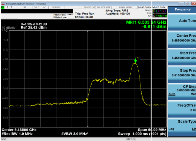
Plot 7-781. LPI Power Spectral Density Plot SDM Diversity Antenna WF8 (40MHz 802.11ax RU26 (UNII Band 6) – Ch. 107)
