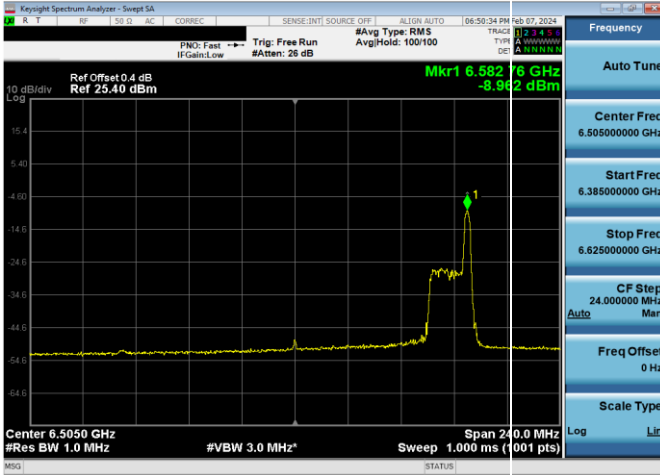
Plot 7-797. LPI Power Spectral Density Plot SDM Diversity Antenna WF8 (160MHz 802.11ax RU26 (UNII Band 6) – Ch. 111)
