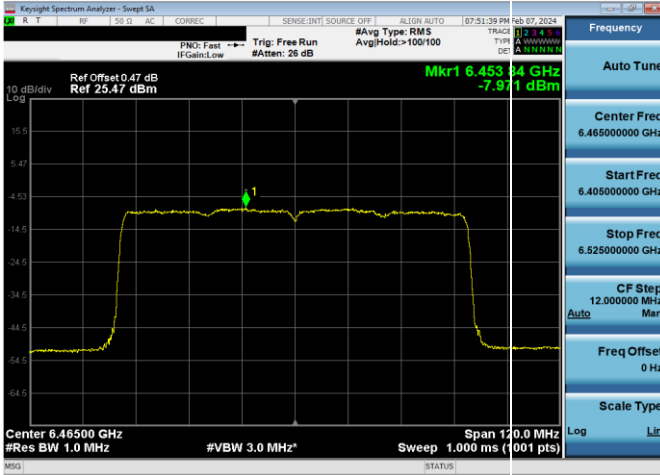
Plot 7-791. LPI Power Spectral Density Plot SDM Diversity Antenna WF8 (80MHz 802.11ax RU996 (UNII Band 6) – Ch. 103)
