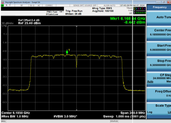
Plot 7-767. LPI Power Spectral Density Plot SDM Diversity Antenna WF8 (160MHz 802.11ax RU996x2 (UNII Band 5) – Ch. 47)
