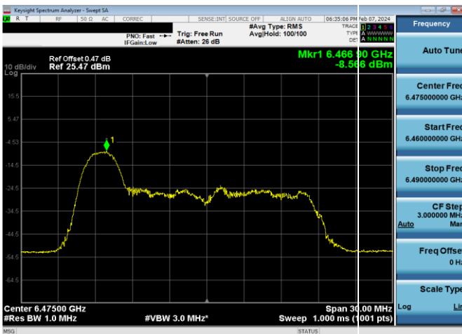
Plot 7-769. LPI Power Spectral Density Plot SDM Diversity Antenna WF8 (20MHz 802.11ax RU26 (UNII Band 6) – Ch. 105)
