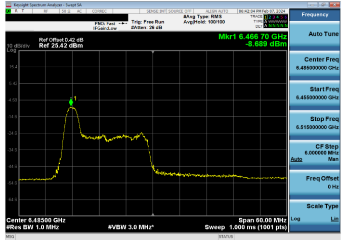
Plot 7-777. LPI Power Spectral Density Plot SDM Diversity Antenna WF8 (40MHz 802.11ax RU26 (UNII Band 6) – Ch. 107)
