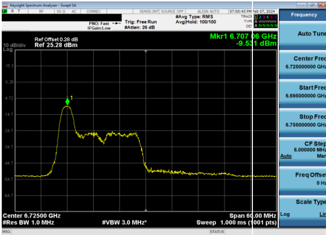
Plot 7-809. LPI Power Spectral Density Plot SDM Diversity Antenna WF8 (40MHz 802.11ax RU26 (UNII Band 7) – Ch. 155)
