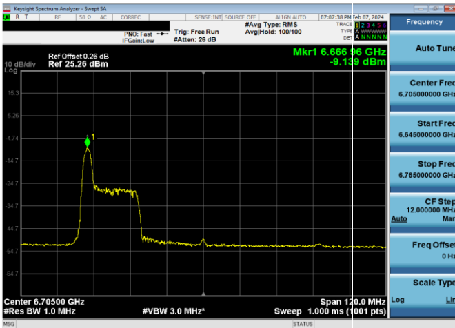
Plot 7-817. LPI Power Spectral Density Plot SDM Diversity Antenna WF8 (80MHz 802.11ax RU26 (UNII Band 7) – Ch. 151)
