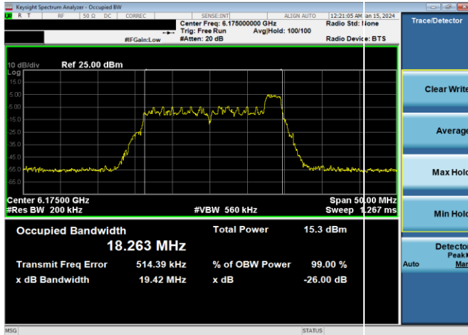
Plot 7-67. 26dB & 99% Bandwidth Plot Antenna WF8 (20MHz 802.11ax RU26 (UNII Band 5) – Ch. 45)
