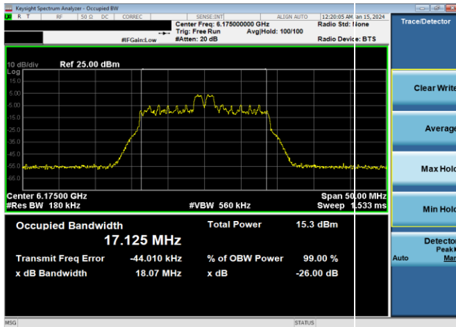
Plot 7-66. 26dB & 99% Bandwidth Plot Antenna WF8 (20MHz 802.11ax RU26 (UNII Band 5) – Ch. 45)
