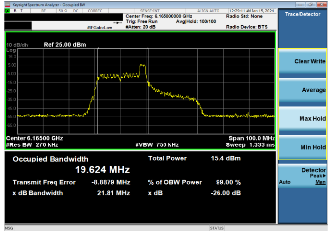
Plot 7-70. 26dB & 99% Bandwidth Plot Antenna WF8 (40MHz 802.11ax RU26 (UNII Band 5) – Ch. 43)
