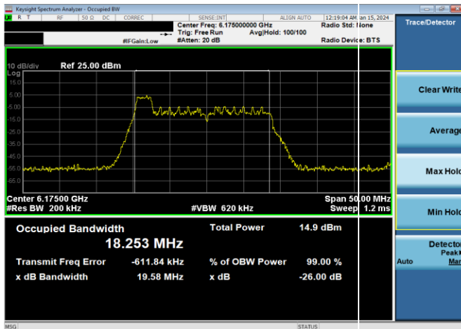
Plot 7-65. 26dB & 99% Bandwidth Plot Antenna WF8 (20MHz 802.11ax RU26 (UNII Band 5) – Ch. 45)
