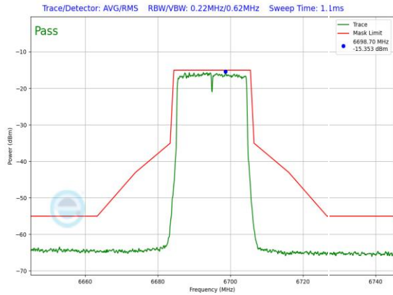
Plot 7-978. LPI In-Band Emission Plot SDM Primary Antenna WF8 (20MHz 802.11ax (UNII Band 7) – Ch. 149, MCS2)
