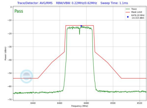
Plot 7-1002. LPI In-Band Emission Plot SDM Primary Antenna WF8 (20MHz 802.11ax (UNII Band 6) – Ch. 105, MCS4)
