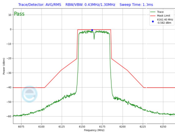
Plot 7-953. SP In-Band Emission Plot Antenna WF7 (40MHz 802.11ax (UNII Band 5) – Ch. 43, MCS11)
