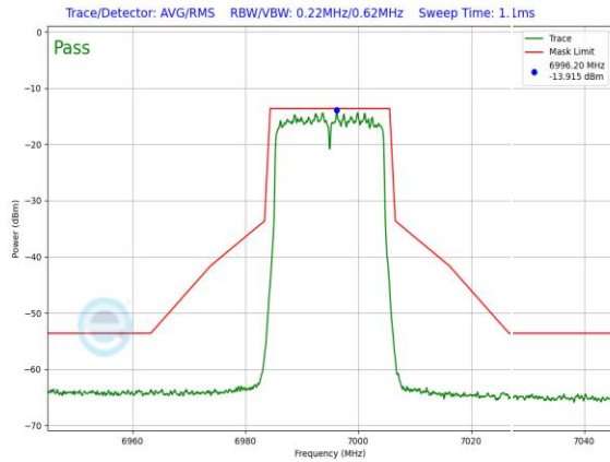
Plot 7-1049. LPI In-Band Emission Plot SDM Primary Antenna WF5B (20MHz 802.11ax (UNII Band 8) – Ch. 209, MCS11)
