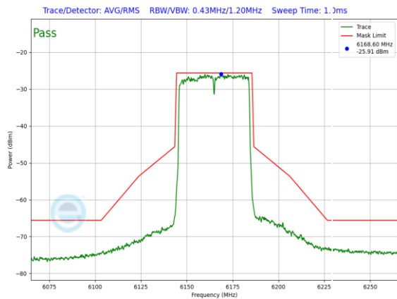
Plot 7-1075. SP In-Band Emission Plot CDD Primary Antenna WF5B (40MHz 802.11ax (UNII Band 5) – Ch. 43, MCS4)
