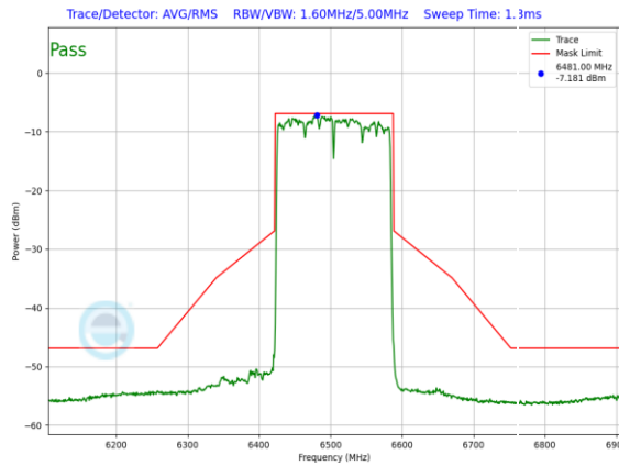
Plot 7-1039. LPI In-Band Emission Plot SDM Primary Antenna WF5B (160MHz 802.11ax (UNII Band 6) – Ch. 111, MCS11)
