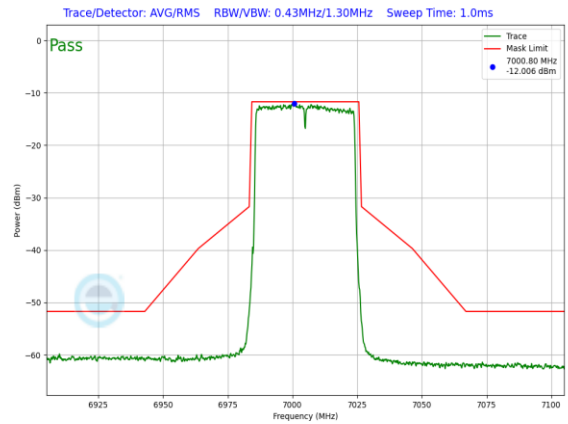
Plot 7-988. LPI In-Band Emission Plot SDM Primary Antenna WF8 (40MHz 802.11ax (UNII Band 8) – Ch. 211, MCS2)
