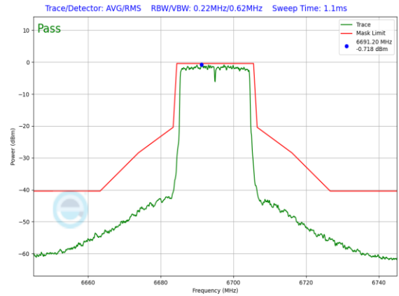
Plot 7-1066. SP In-Band Emission Plot CDD Primary Antenna WF8 (20MHz 802.11ax (UNII Band 7) – Ch. 149, MCS2)
