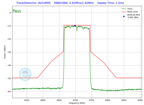
Plot 7-1046. LPI In-Band Emission Plot SDM Primary Antenna WF8 (80MHz 802.11ax (UNII Band 7) – Ch. 151, MCS11)
