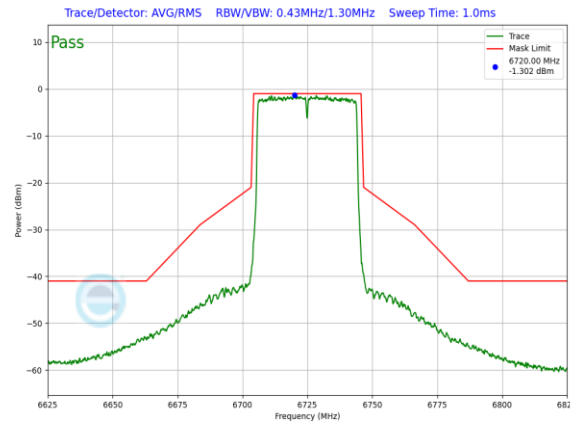
Plot 7-1068. SP In-Band Emission Plot CDD Primary Antenna WF8 (40MHz 802.11ax (UNII Band 7) – Ch. 155, MCS2)
