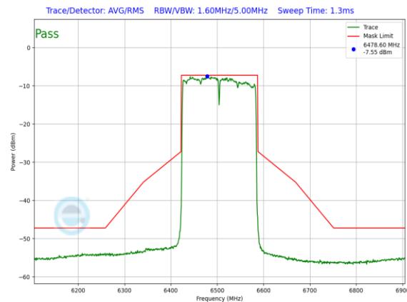
Plot 7-976. LPI In-Band Emission Plot SDM Primary Antenna WF8 (160MHz 802.11ax (UNII Band 6) – Ch. 111, MCS2)
