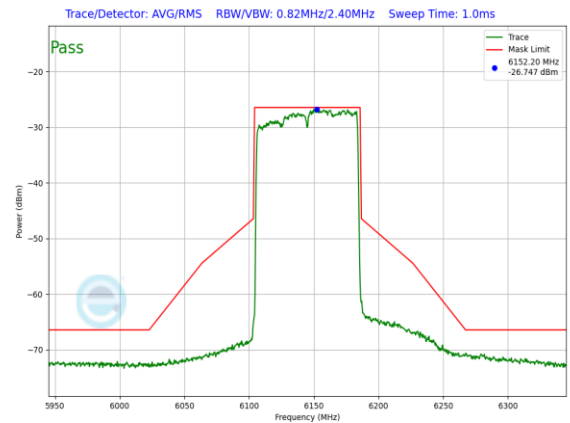
Plot 7-1077. SP In-Band Emission Plot CDD Primary Antenna WF5B (80MHz 802.11ax (UNII Band 5) – Ch. 39, MCS4)
