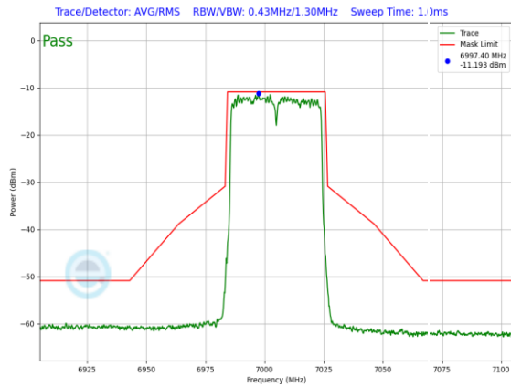
Plot 7-1051. LPI In-Band Emission Plot SDM Primary Antenna WF5B (40MHz 802.11ax (UNII Band 8) – Ch. 211, MCS11)
