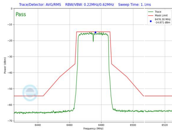
Plot 7-1001. LPI In-Band Emission Plot SDM Primary Antenna WF5B (20MHz 802.11ax (UNII Band 6) – Ch. 105, MCS4)
