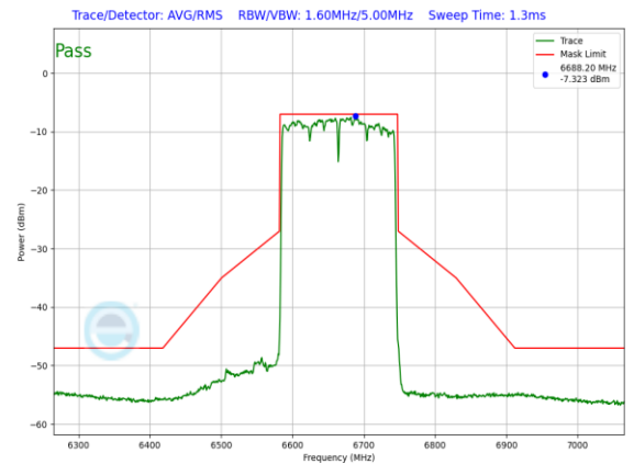
Plot 7-1047. LPI In-Band Emission Plot SDM Primary Antenna WF5B (160MHz 802.11ax (UNII Band 7) – Ch. 143, MCS11)
