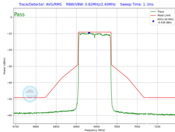
Plot 7-990. LPI In-Band Emission Plot SDM Primary Antenna WF8 (80MHz 802.11ax (UNII Band 8) – Ch. 199, MCS2)
