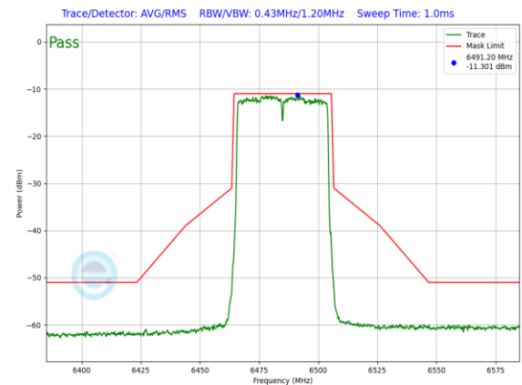
Plot 7-1004. LPI In-Band Emission Plot SDM Primary Antenna WF8 (40MHz 802.11ax (UNII Band 6) – Ch. 107, MCS4)
