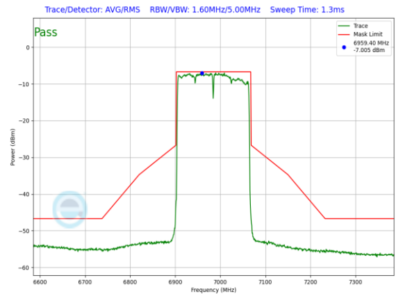
Plot 7-992. LPI In-Band Emission Plot SDM Primary Antenna WF8 (160MHz 802.11ax (UNII Band 8) – Ch. 207, MCS2)
