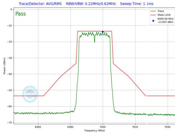
Plot 7-1050. LPI In-Band Emission Plot SDM Primary Antenna WF8 (20MHz 802.11ax (UNII Band 8) – Ch. 209, MCS11)
