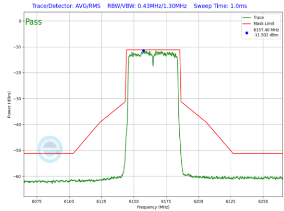
Plot 7-1028. LPI In-Band Emission Plot SDM Primary Antenna WF8 (40MHz 802.11ax (UNII Band 5) – Ch. 43, MCS11)
