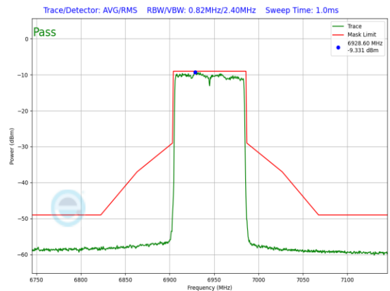
Plot 7-1022. LPI In-Band Emission Plot SDM Primary Antenna WF8 (80MHz 802.11ax (UNII Band 8) – Ch. 199, MCS4)
