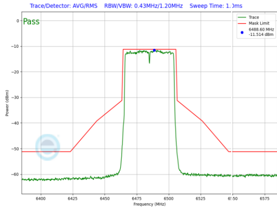
Plot 7-972. LPI In-Band Emission Plot SDM Primary Antenna WF8 (40MHz 802.11ax (UNII Band 6) – Ch. 107, MCS2)
