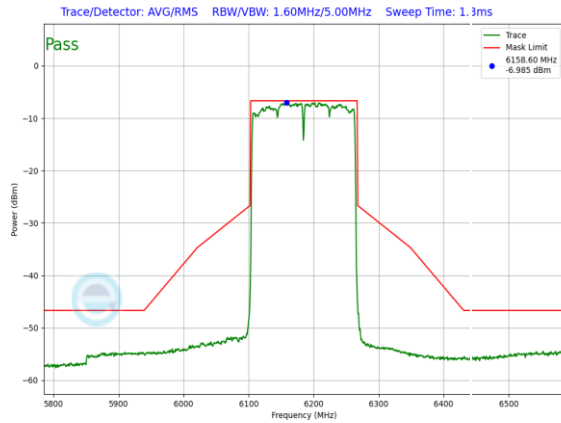
Plot 7-999. LPI In-Band Emission Plot SDM Primary Antenna WF5B (160MHz 802.11ax (UNII Band 5) – Ch. 47, MCS4)
