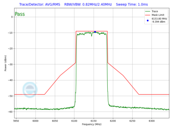
Plot 7-998. LPI In-Band Emission Plot SDM Primary Antenna WF8 (80MHz 802.11ax (UNII Band 5) – Ch. 39, MCS4)
