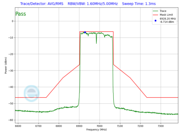
Plot 7-991. LPI In-Band Emission Plot SDM Primary Antenna WF5B (160MHz 802.11ax (UNII Band 8) – Ch. 207, MCS2)
