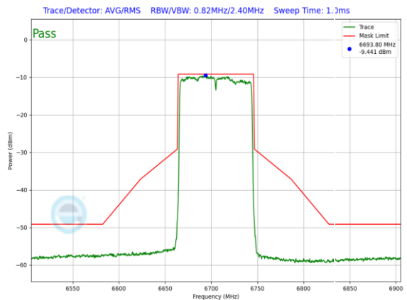
Plot 7-1013. LPI In-Band Emission Plot SDM Primary Antenna WF5B (80MHz 802.11ax (UNII Band 7) – Ch. 151, MCS4)
