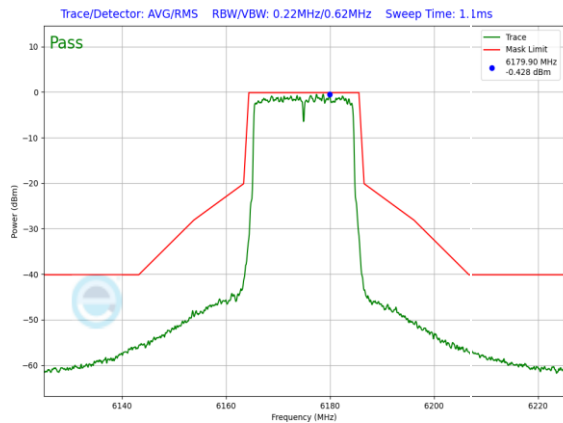
Plot 7-1074. SP In-Band Emission Plot CDD Primary Antenna WF8 (20MHz 802.11ax (UNII Band 5) – Ch. 45, MCS4)
