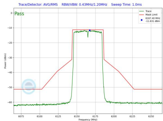
Plot 7-964. LPI In-Band Emission Plot SDM Primary Antenna WF8 (40MHz 802.11ax (UNII Band 5) – Ch. 43, MCS2)
