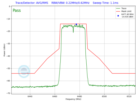
Plot 7-1034. LPI In-Band Emission Plot SDM Primary Antenna WF8 (20MHz 802.11ax (UNII Band 6) – Ch. 105, MCS11)
