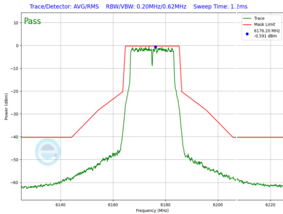
Plot 7-951. SP In-Band Emission Plot Antenna WF7 (20MHz 802.11a (UNII Band 5) – Ch. 45, 54Mbps)
