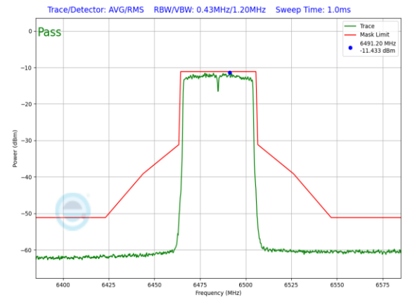
Plot 7-1003. LPI In-Band Emission Plot SDM Primary Antenna WF5B (40MHz 802.11ax (UNII Band 6) – Ch. 107, MCS4)
