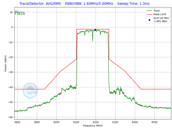
Plot 7-955. SP In-Band Emission Plot Antenna WF7 (160MHz 802.11ax (UNII Band 5) – Ch. 47, MCS11)
