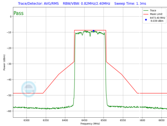
Plot 7-1037. LPI In-Band Emission Plot SDM Primary Antenna WF5B (80MHz 802.11ax (UNII Band 6) – Ch. 103, MCS11)
