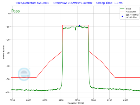
Plot 7-965. LPI In-Band Emission Plot SDM Primary Antenna WF5B (80MHz 802.11ax (UNII Band 5) – Ch. 39, MCS2)
