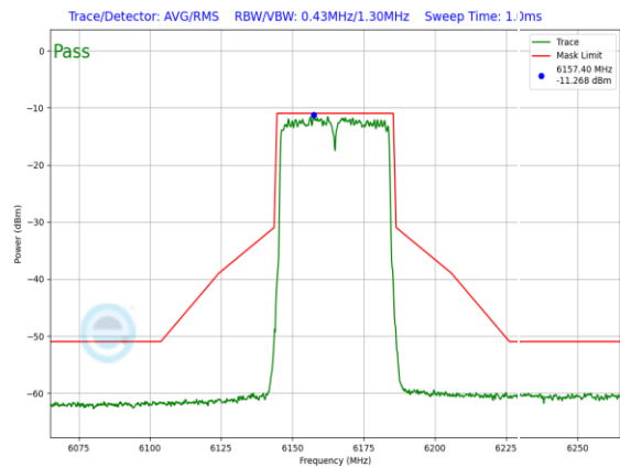
Plot 7-1027. LPI In-Band Emission Plot SDM Primary Antenna WF5B (40MHz 802.11ax (UNII Band 5) – Ch. 43, MCS11)
