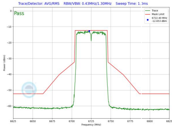
Plot 7-1043. LPI In-Band Emission Plot SDM Primary Antenna WF5B (40MHz 802.11ax (UNII Band 7) – Ch. 155, MCS11)
