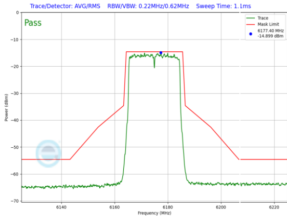
Plot 7-994. LPI In-Band Emission Plot SDM Primary Antenna WF8 (20MHz 802.11ax (UNII Band 5) – Ch. 45, MCS4)
