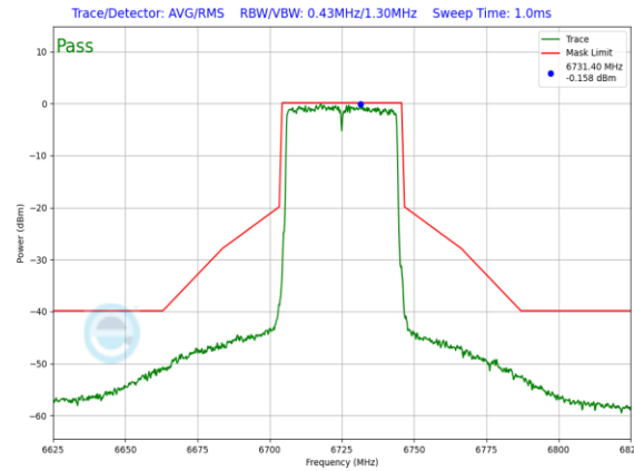
Plot 7-1067. SP In-Band Emission Plot CDD Primary Antenna WF5B (40MHz 802.11ax (UNII Band 7) – Ch. 155, MCS2)
