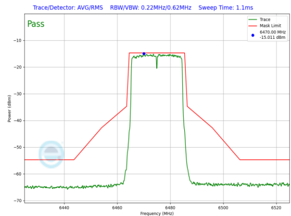
Plot 7-970. LPI In-Band Emission Plot SDM Primary Antenna WF8 (20MHz 802.11ax (UNII Band 6) – Ch. 105, MCS2)
