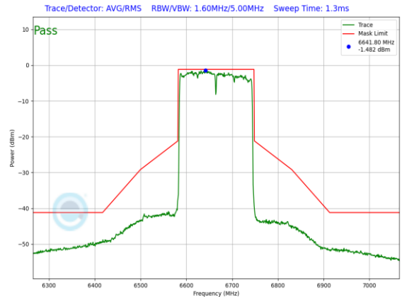
Plot 7-1071. SP In-Band Emission Plot CDD Primary Antenna WF5B (160MHz 802.11ax (UNII Band 7) – Ch. 143, MCS2)
