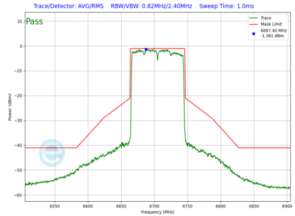
Plot 7-959. SP In-Band Emission Plot Antenna WF7 (80MHz) 802.11ax (UNII Band 7) – Ch. 151, MCS11)
