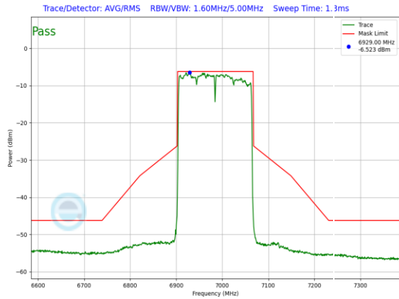
Plot 7-1023. LPI In-Band Emission Plot SDM Primary Antenna WF5B (160MHz 802.11ax (UNII Band 8) – Ch. 207, MCS4)
