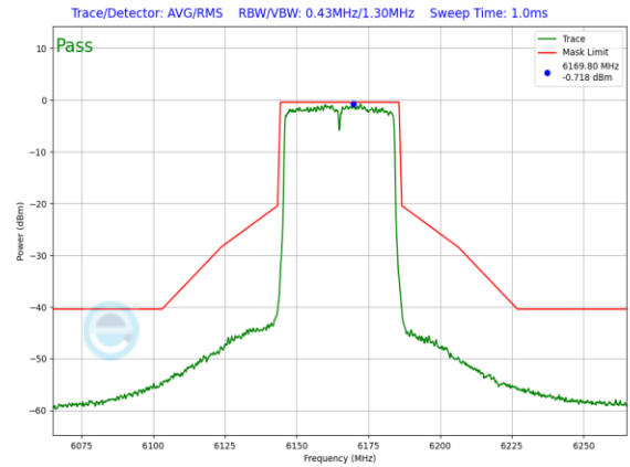
Plot 7-1076. SP In-Band Emission Plot CDD Primary Antenna WF8 (40MHz 802.11ax (UNII Band 5) – Ch. 43, MCS4)
