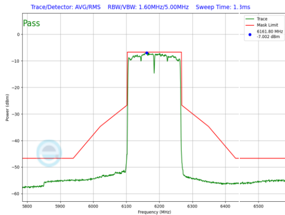
Plot 7-1000. LPI In-Band Emission Plot SDM Primary Antenna WF8 (160MHz 802.11ax (UNII Band 5) – Ch. 47, MCS4)
