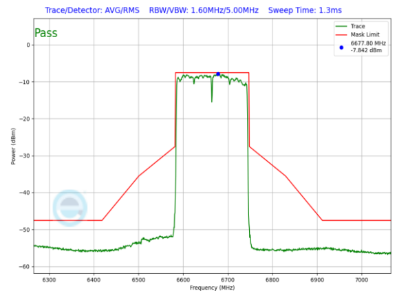
Plot 7-1016. LPI In-Band Emission Plot SDM Primary Antenna WF8 (160MHz 802.11ax (UNII Band 7) – Ch. 143, MCS4)
