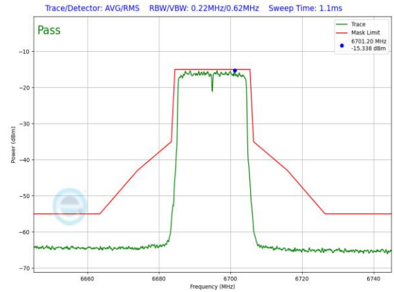
Plot 7-1009. LPI In-Band Emission Plot SDM Primary Antenna WF5B (20MHz 802.11ax (UNII Band 7) – Ch. 149, MCS4)
