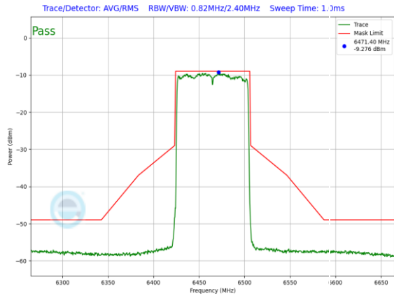
Plot 7-1006. LPI In-Band Emission Plot SDM Primary Antenna WF8 (80MHz 802.11ax (UNII Band 6) – Ch. 103, MCS4)
