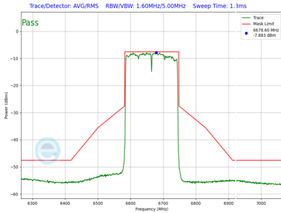
Plot 7-984. LPI In-Band Emission Plot SDM Primary Antenna WF8 (160MHz 802.11ax (UNII Band 7) – Ch. 143, MCS2)
