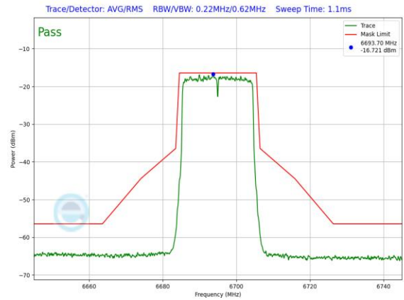
Plot 7-1010. LPI In-Band Emission Plot SDM Primary Antenna WF8 (20MHz 802.11ax (UNII Band 7) – Ch. 149, MCS4)
