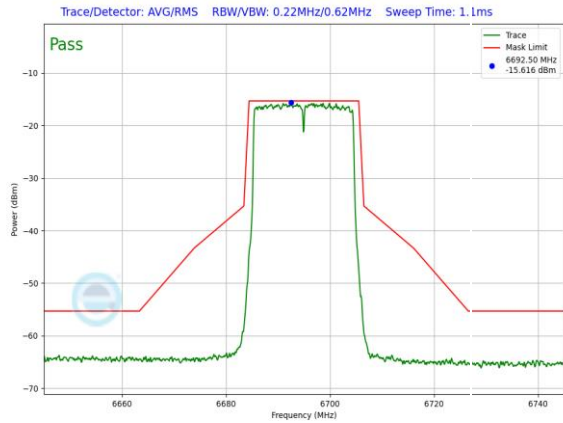
Plot 7-977. LPI In-Band Emission Plot SDM Primary Antenna WF5B (20MHz 802.11ax (UNII Band 7) – Ch. 149, MCS2)
