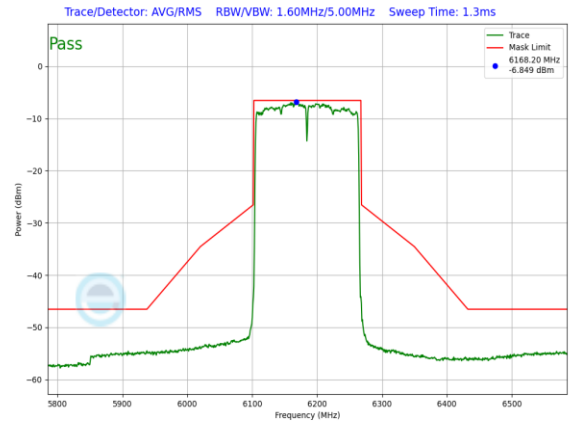
Plot 7-968. LPI In-Band Emission Plot SDM Primary Antenna WF8 (160MHz 802.11ax (UNII Band 5) – Ch. 47, MCS2)
