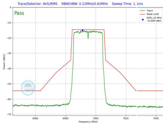
Plot 7-985. LPI In-Band Emission Plot SDM Primary Antenna WF5B (20MHz 802.11ax (UNII Band 8) – Ch. 209, MCS2)
