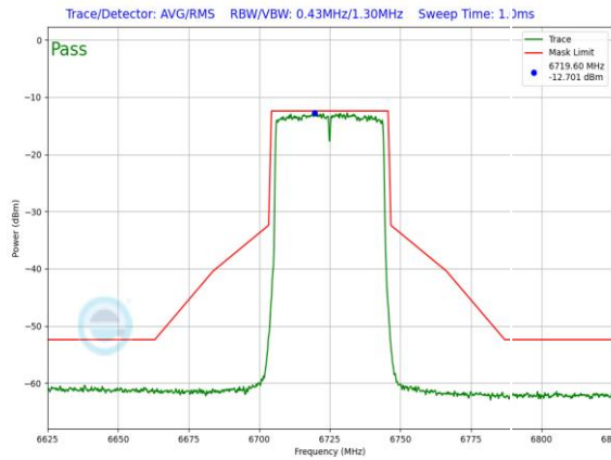
Plot 7-979. LPI In-Band Emission Plot SDM Primary Antenna WF5B (40MHz 802.11ax (UNII Band 7) – Ch. 155, MCS2)
