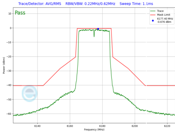
Plot 7-1058. SP In-Band Emission Plot CDD Primary Antenna WF8 (20MHz 802.11ax (UNII Band 5) – Ch. 45, MCS2)
