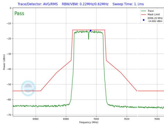
Plot 7-1018. LPI In-Band Emission Plot SDM Primary Antenna WF8 (20MHz 802.11ax (UNII Band 8) – Ch. 209, MCS4)
