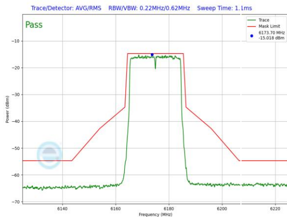
Plot 7-962. LPI In-Band Emission Plot SDM Primary Antenna WF8 (20MHz 802.11ax (UNII Band 5) – Ch. 45, MCS2)
