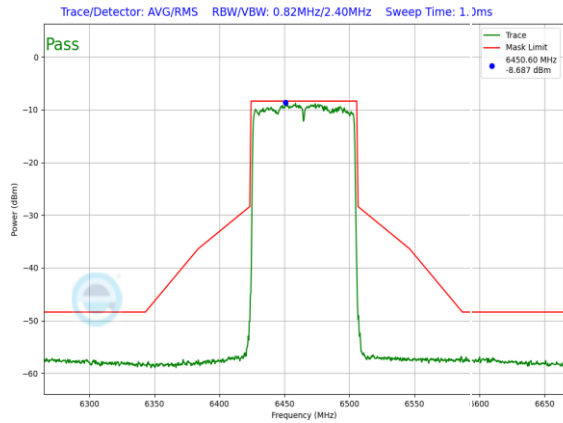
Plot 7-1005. LPI In-Band Emission Plot SDM Primary Antenna WF5B (80MHz 802.11ax (UNII Band 6) – Ch. 103, MCS4)
