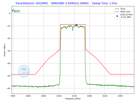
Plot 7-1029. LPI In-Band Emission Plot SDM Primary Antenna WF5B (80MHz 802.11ax (UNII Band 5) – Ch. 39, MCS11)
