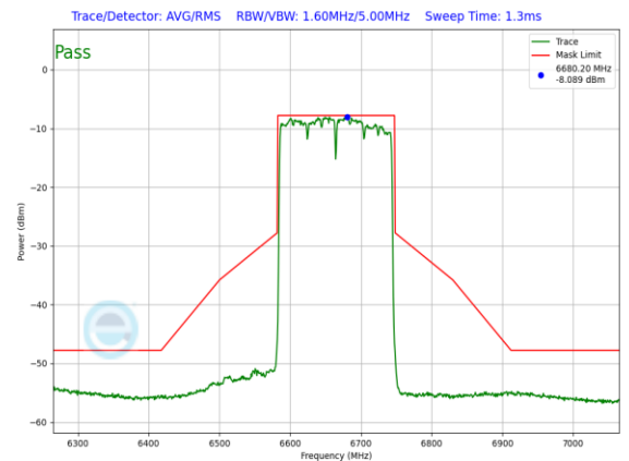
Plot 7-1048. LPI In-Band Emission Plot SDM Primary Antenna WF8 (160MHz 802.11ax (UNII Band 7) – Ch. 143, MCS11)
