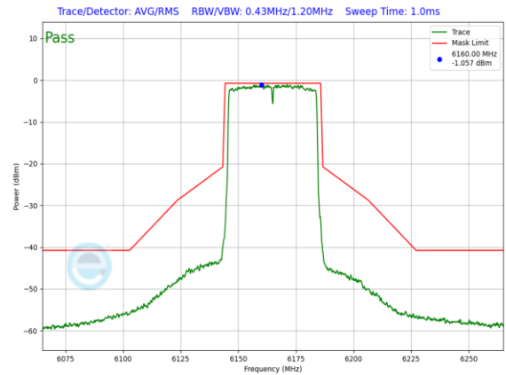
Plot 7-1060. SP In-Band Emission Plot CDD Primary Antenna WF8 (40MHz 802.11ax (UNII Band 5) – Ch. 43, MCS2)
