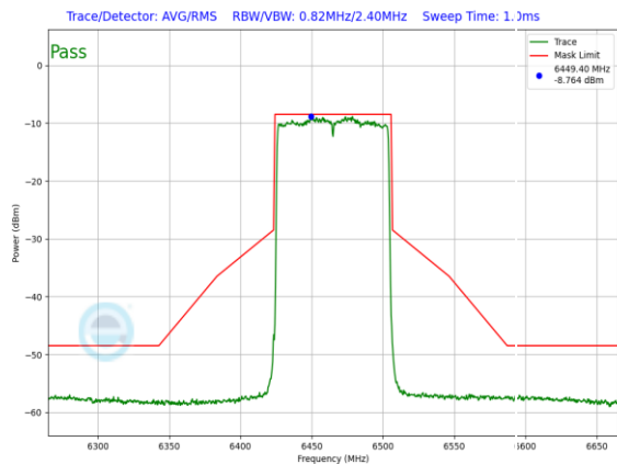
Plot 7-973. LPI In-Band Emission Plot SDM Primary Antenna WF5B (80MHz 802.11ax (UNII Band 6) – Ch. 103, MCS2)
