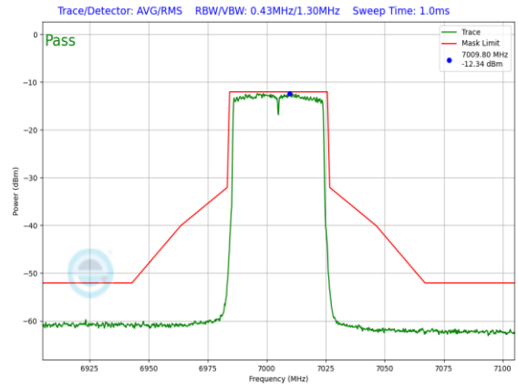
Plot 7-987. LPI In-Band Emission Plot SDM Primary Antenna WF5B (40MHz 802.11ax (UNII Band 8) – Ch. 211, MCS2)
