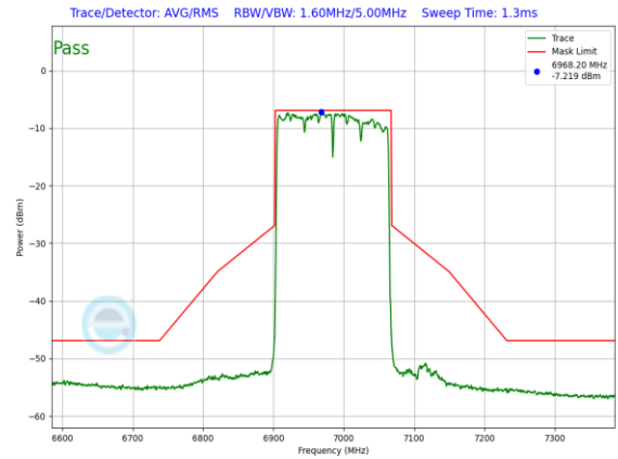
Plot 7-1056. LPI In-Band Emission Plot SDM Primary Antenna WF8 (160MHz 802.11ax (UNII Band 8) – Ch. 207, MCS11)
