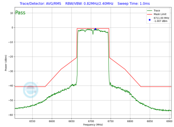
Plot 7-949. SP In-Band Emission Plot Antenna WF7 (80MHz 802.11ax (UNII Band 7) – Ch. 151, MCS4)
