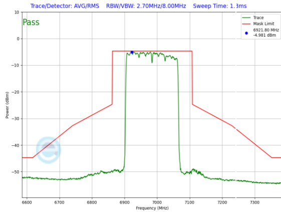
Plot 7-1055. LPI In-Band Emission Plot SDM Primary Antenna WF5B (160MHz 802.11ax (UNII Band 8) – Ch. 207, MCS11)
