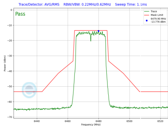
Plot 7-1033. LPI In-Band Emission Plot SDM Primary Antenna WF5B (20MHz 802.11ax (UNII Band 6) – Ch. 105, MCS11)
