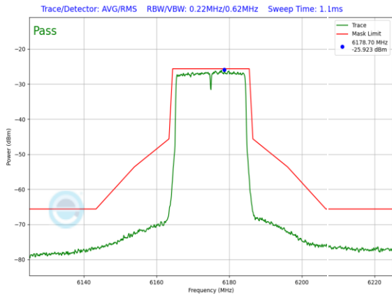
Plot 7-1057. SP In-Band Emission Plot CDD Primary Antenna WF5B (20MHz 802.11ax (UNII Band 5) – Ch. 45, MCS2)
