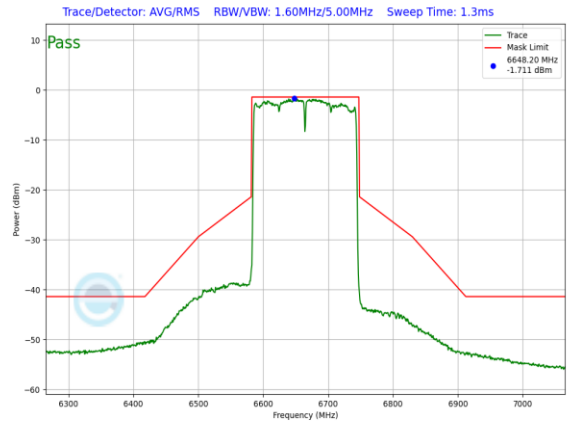
Plot 7-1072. SP In-Band Emission Plot CDD Primary Antenna WF8 (160MHz 802.11ax (UNII Band 7) – Ch. 143, MCS2)
