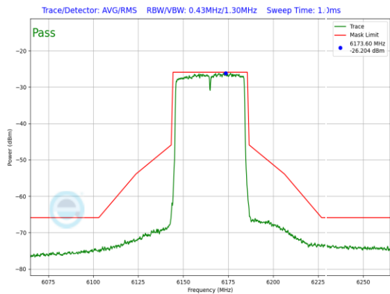
Plot 7-1059. SP In-Band Emission Plot CDD Primary Antenna WF5B (40MHz 802.11ax (UNII Band 5) – Ch. 43, MCS2)
