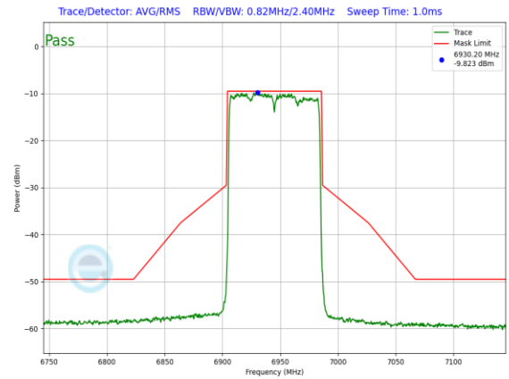
Plot 7-1054. LPI In-Band Emission Plot SDM Primary Antenna WF8 (80MHz 802.11ax (UNII Band 8) – Ch. 199, MCS11)
