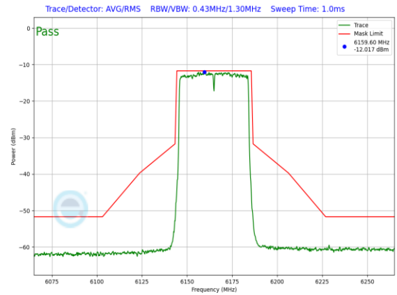
Plot 7-963. LPI In-Band Emission Plot SDM Primary Antenna WF5B (40MHz 802.11ax (UNII Band 5) – Ch. 43, MCS2)
