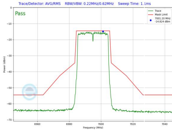
Plot 7-1017. LPI In-Band Emission Plot SDM Primary Antenna WF5B (20MHz 802.11ax (UNII Band 8) – Ch. 209, MCS4)
