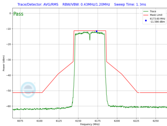
Plot 7-995. LPI In-Band Emission Plot SDM Primary Antenna WF5B (40MHz 802.11ax (UNII Band 5) – Ch. 43, MCS4)
