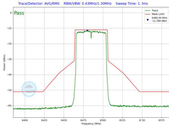
Plot 7-971. LPI In-Band Emission Plot SDM Primary Antenna WF5B (40MHz 802.11ax (UNII Band 6) – Ch. 107, MCS2)
