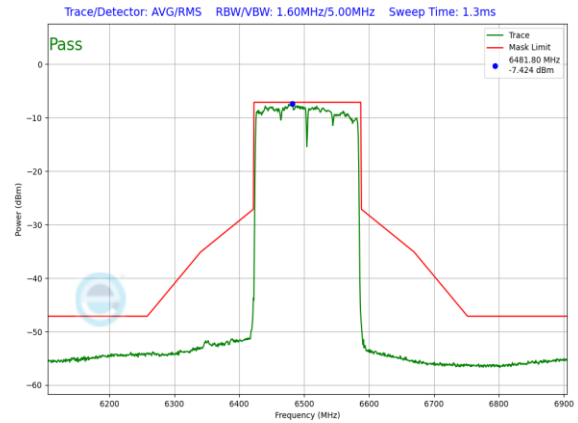
Plot 7-1008. LPI In-Band Emission Plot SDM Primary Antenna WF8 (160MHz 802.11ax (UNII Band 6) – Ch. 111, MCS4)
