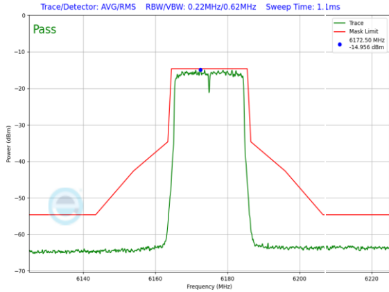
Plot 7-993. LPI In-Band Emission Plot SDM Primary Antenna WF5B (20MHz 802.11ax (UNII Band 5) – Ch. 45, MCS4)
