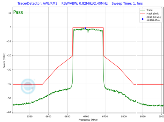
Plot 7-1069. SP In-Band Emission Plot CDD Primary Antenna WF5B (80MHz 802.11ax (UNII Band 7) – Ch. 151, MCS2)
