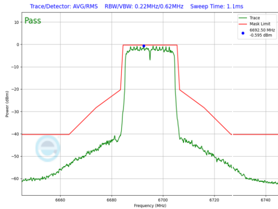
Plot 7-957. SP In-Band Emission Plot Antenna WF7 (20MHz) 802.11ax (UNII Band 7) – Ch. 149, MCS11)
