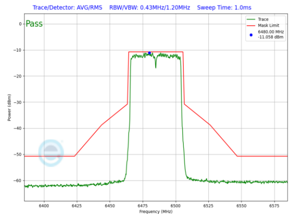
Plot 7-1036. LPI In-Band Emission Plot SDM Primary Antenna WF8 (40MHz 802.11ax (UNII Band 6) – Ch. 107, MCS11)
