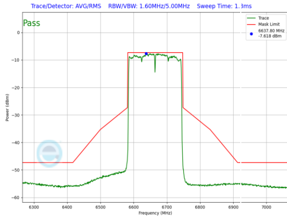
Plot 7-983. LPI In-Band Emission Plot SDM Primary Antenna WF5B (160MHz 802.11ax (UNII Band 7) – Ch. 143, MCS2)
