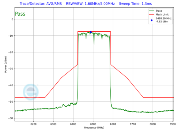
Plot 7-1040. LPI In-Band Emission Plot SDM Primary Antenna WF8 (160MHz 802.11ax (UNII Band 6) – Ch. 111, MCS11)
