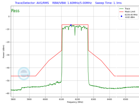
Plot 7-1032. LPI In-Band Emission Plot SDM Primary Antenna WF8 (160MHz 802.11ax (UNII Band 5) – Ch. 47, MCS11)
