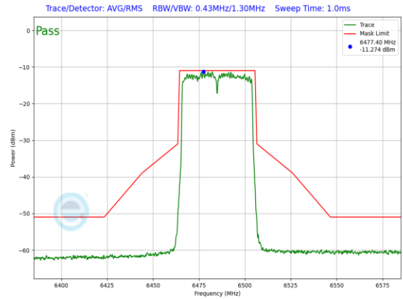
Plot 7-1035. LPI In-Band Emission Plot SDM Primary Antenna WF5B (40MHz 802.11ax (UNII Band 6) – Ch. 107, MCS11)
