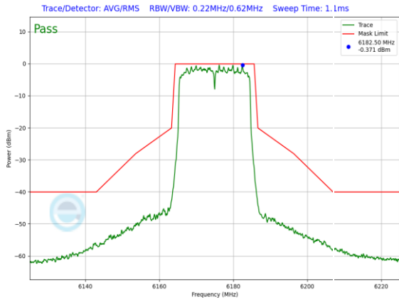
Plot 7-952. SP In-Band Emission Plot Antenna WF7 (20MHz 802.11ax (UNII Band 5) – Ch. 45, MCS11)
