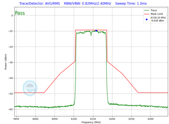
Plot 7-997. LPI In-Band Emission Plot SDM Primary Antenna WF5B (80MHz 802.11ax (UNII Band 5) – Ch. 39, MCS4)
