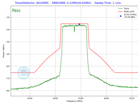
Plot 7-1073. SP In-Band Emission Plot CDD Primary Antenna WF5B (20MHz 802.11ax (UNII Band 5) – Ch. 45, MCS4)
