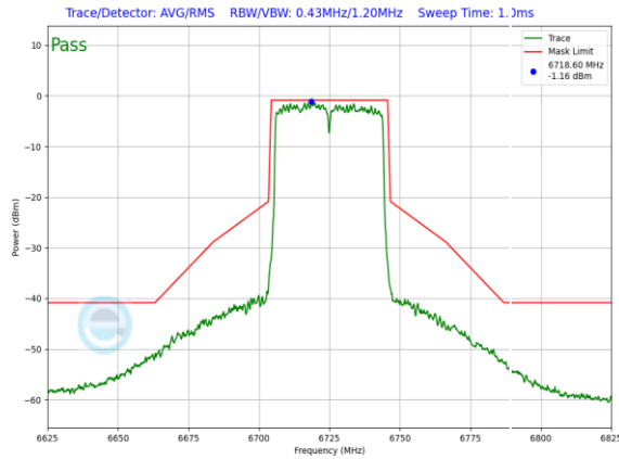
Plot 7-958. SP In-Band Emission Plot Antenna WF7 (40MHz) 802.11ax (UNII Band 7) – Ch. 155, MCS11)
