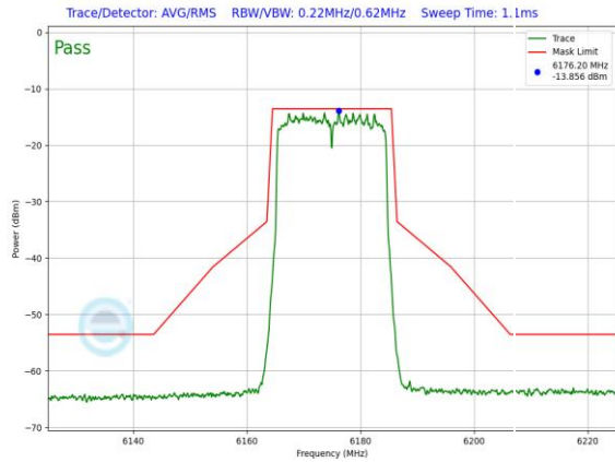
Plot 7-1025. LPI In-Band Emission Plot SDM Primary Antenna WF5B (20MHz 802.11ax (UNII Band 5) – Ch. 45, MCS11)
