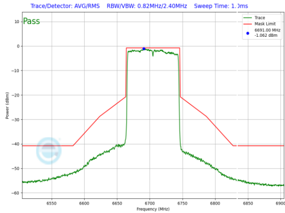
Plot 7-1070. SP In-Band Emission Plot CDD Primary Antenna WF8 (80MHz 802.11ax (UNII Band 7) – Ch. 151, MCS2)
