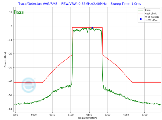
Plot 7-954. SP In-Band Emission Plot Antenna WF7 (80MHz 802.11ax (UNII Band 5) – Ch. 39, MCS11)
