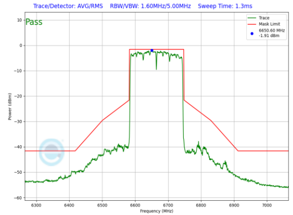
Plot 7-960. SP In-Band Emission Plot Antenna WF7 (160MHz) 802.11ax (UNII Band 7) – Ch. 143, MCS11)
