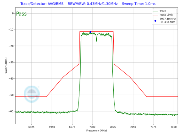
Plot 7-1052. LPI In-Band Emission Plot SDM Primary Antenna WF8 (40MHz 802.11ax (UNII Band 8) – Ch. 211, MCS11)
