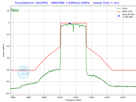
Plot 7-1064. SP In-Band Emission Plot CDD Primary Antenna WF8 (160MHz 802.11ax (UNII Band 5) – Ch. 47, MCS2)
