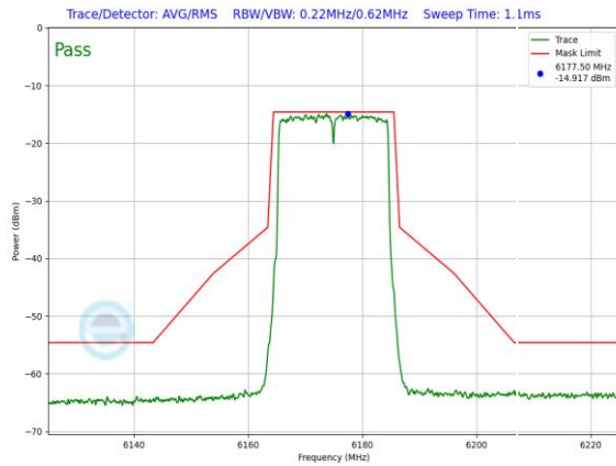
Plot 7-961. LPI In-Band Emission Plot SDM Primary Antenna WF5B (20MHz 802.11ax (UNII Band 5) – Ch. 45, MCS2)
