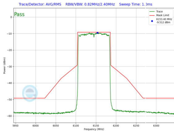
Plot 7-966. LPI In-Band Emission Plot SDM Primary Antenna WF8 (80MHz 802.11ax (UNII Band 5) – Ch. 39, MCS2)
