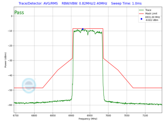
Plot 7-1053. LPI In-Band Emission Plot SDM Primary Antenna WF5B (80MHz 802.11ax (UNII Band 8) – Ch. 199, MCS11)
