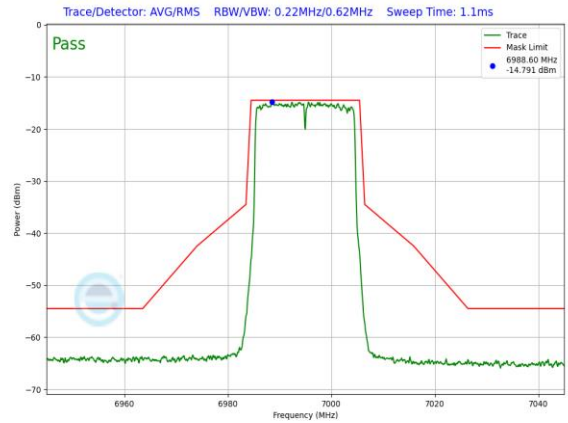
Plot 7-986. LPI In-Band Emission Plot SDM Primary Antenna WF8 (20MHz 802.11ax (UNII Band 8) – Ch. 209, MCS2)
