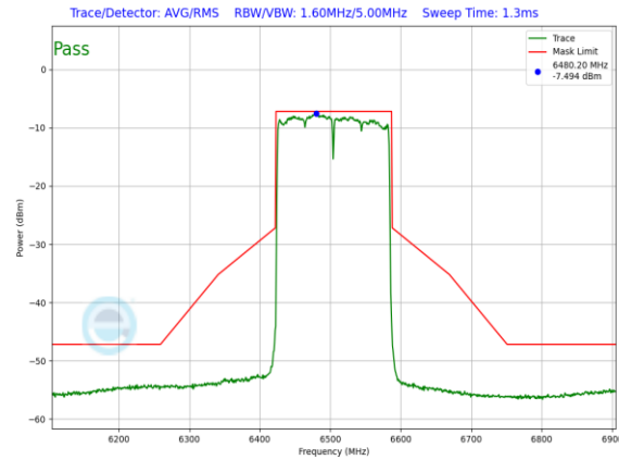
Plot 7-975. LPI In-Band Emission Plot SDM Primary Antenna WF5B (160MHz 802.11ax (UNII Band 6) – Ch. 111, MCS2)
