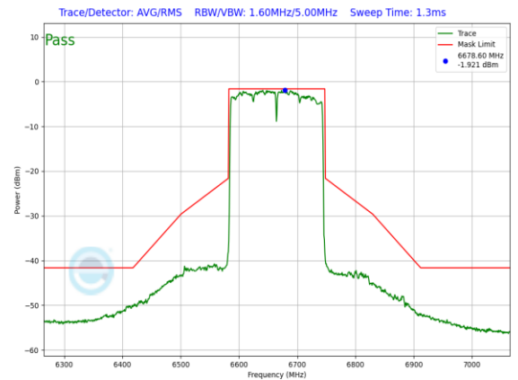
Plot 7-950. SP In-Band Emission Plot Antenna WF7 (160MHz 802.11ax (UNII Band 7) – Ch. 143, MCS4)
