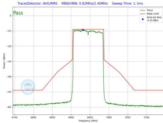
Plot 7-989. LPI In-Band Emission Plot SDM Primary Antenna WF5B (80MHz 802.11ax (UNII Band 8) – Ch. 199, MCS2)
