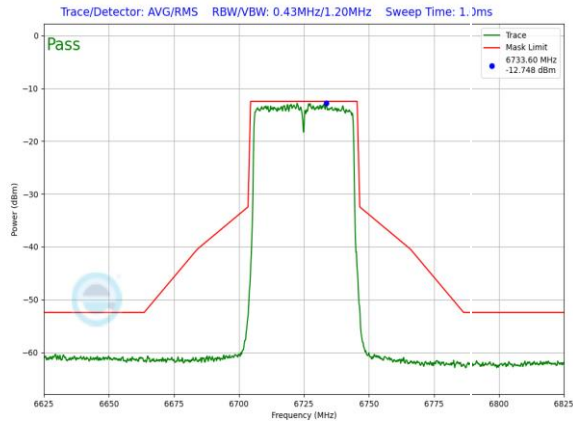
Plot 7-1011. LPI In-Band Emission Plot SDM Primary Antenna WF5B (40MHz 802.11ax (UNII Band 7) – Ch. 155, MCS4)
