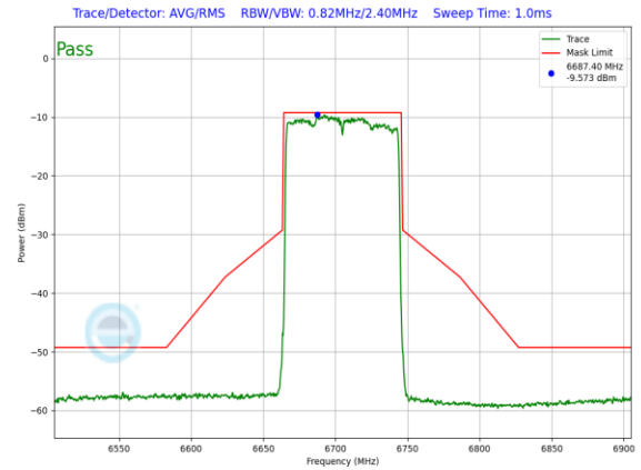
Plot 7-1014. LPI In-Band Emission Plot SDM Primary Antenna WF8 (80MHz 802.11ax (UNII Band 7) – Ch. 151, MCS4)
