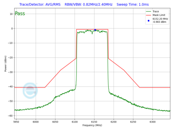
Plot 7-1078. SP In-Band Emission Plot CDD Primary Antenna WF8 (80MHz 802.11ax (UNII Band 5) – Ch. 39, MCS4)
