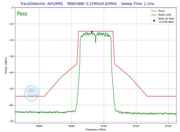
Plot 7-1041. LPI In-Band Emission Plot SDM Primary Antenna WF5B (20MHz 802.11ax (UNII Band 7) – Ch. 149, MCS11)
