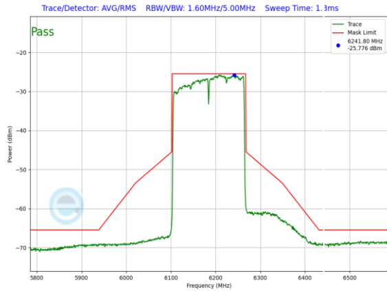
Plot 7-1063. SP In-Band Emission Plot CDD Primary Antenna WF5B (160MHz 802.11ax (UNII Band 5) – Ch. 47, MCS2)
