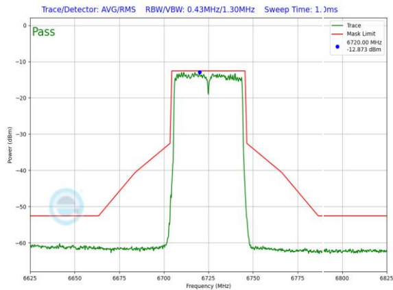
Plot 7-1044. LPI In-Band Emission Plot SDM Primary Antenna WF8 (40MHz 802.11ax (UNII Band 7) – Ch. 155, MCS11)
