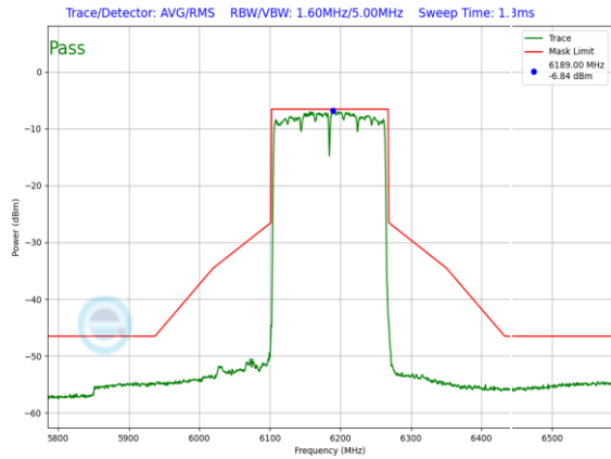
Plot 7-1031. LPI In-Band Emission Plot SDM Primary Antenna WF5B (160MHz 802.11ax (UNII Band 5) – Ch. 47, MCS11)
