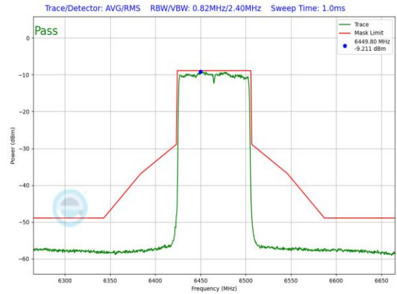
Plot 7-974. LPI In-Band Emission Plot SDM Primary Antenna WF8 (80MHz 802.11ax (UNII Band 6) – Ch. 103, MCS2)
