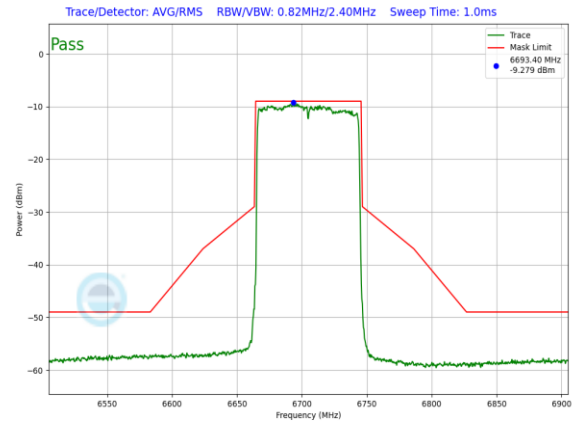
Plot 7-981. LPI In-Band Emission Plot SDM Primary Antenna WF5B (80MHz 802.11ax (UNII Band 7) – Ch. 151, MCS2)
