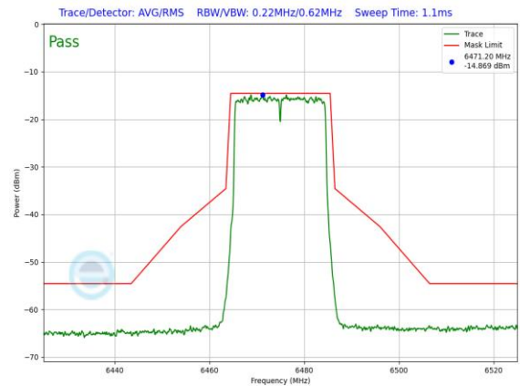
Plot 7-969. LPI In-Band Emission Plot SDM Primary Antenna WF5B (20MHz 802.11ax (UNII Band 6) – Ch. 105, MCS2)
