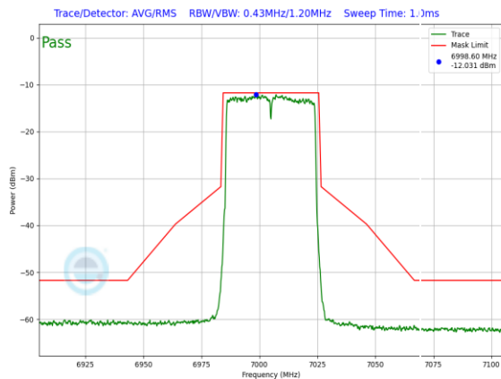
Plot 7-1019. LPI In-Band Emission Plot SDM Primary Antenna WF5B (40MHz 802.11ax (UNII Band 8) – Ch. 211, MCS4)
