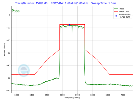
Plot 7-1015. LPI In-Band Emission Plot SDM Primary Antenna WF5B (160MHz 802.11ax (UNII Band 7) – Ch. 143, MCS4)
