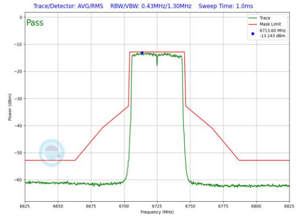
Plot 7-980. LPI In-Band Emission Plot SDM Primary Antenna WF8 (40MHz 802.11ax (UNII Band 7) – Ch. 155, MCS2)
