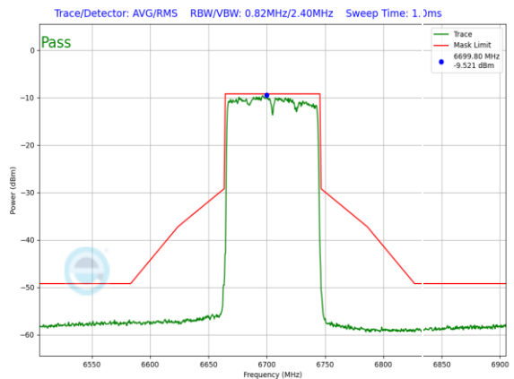
Plot 7-1045. LPI In-Band Emission Plot SDM Primary Antenna WF5B (80MHz 802.11ax (UNII Band 7) – Ch. 151, MCS11)
