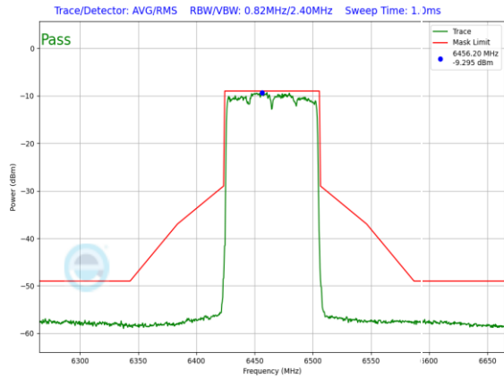
Plot 7-1038. LPI In-Band Emission Plot SDM Primary Antenna WF8 (80MHz 802.11ax (UNII Band 6) – Ch. 103, MCS11)
