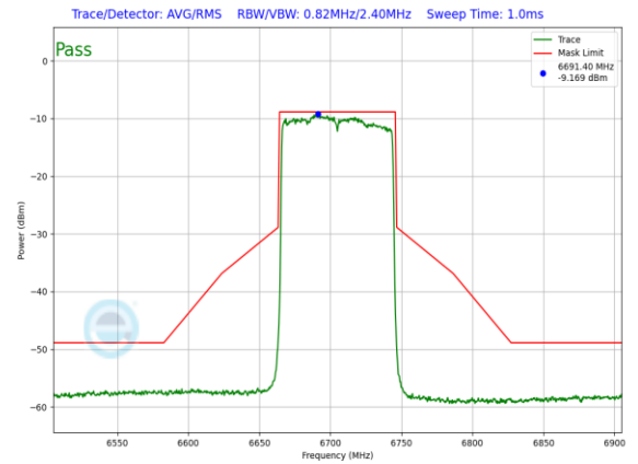
Plot 7-982. LPI In-Band Emission Plot SDM Primary Antenna WF8 (80MHz 802.11ax (UNII Band 7) – Ch. 151, MCS2)
