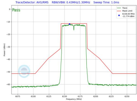
Plot 7-996. LPI In-Band Emission Plot SDM Primary Antenna WF8 (40MHz 802.11ax (UNII Band 5) – Ch. 43, MCS4)
