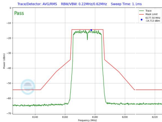
Plot 7-1026. LPI In-Band Emission Plot SDM Primary Antenna WF8 (20MHz 802.11ax (UNII Band 5) – Ch. 45, MCS11)
