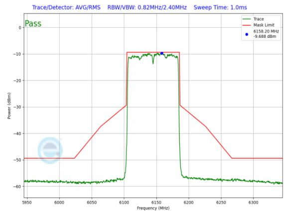
Plot 7-1030. LPI In-Band Emission Plot SDM Primary Antenna WF8 (80MHz 802.11ax (UNII Band 5) – Ch. 39, MCS11)
