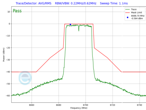
Plot 7-1065. SP In-Band Emission Plot CDD Primary Antenna WF5B (20MHz 802.11ax (UNII Band 7) – Ch. 149, MCS2)
