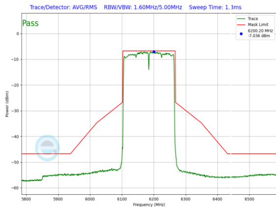
Plot 7-967. LPI In-Band Emission Plot SDM Primary Antenna WF5B (160MHz 802.11ax (UNII Band 5) – Ch. 47, MCS2)
