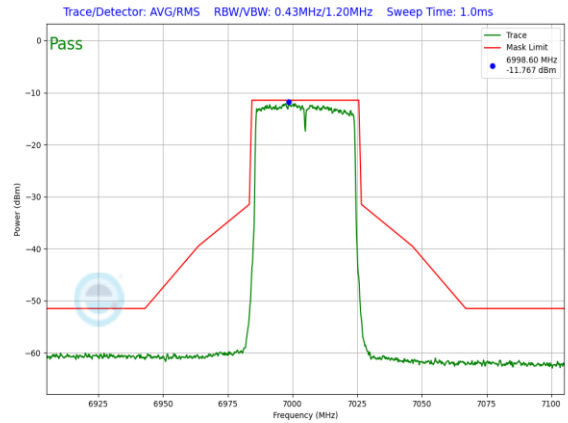
Plot 7-1020. LPI In-Band Emission Plot SDM Primary Antenna WF8 (40MHz 802.11ax (UNII Band 8) – Ch. 211, MCS4)
