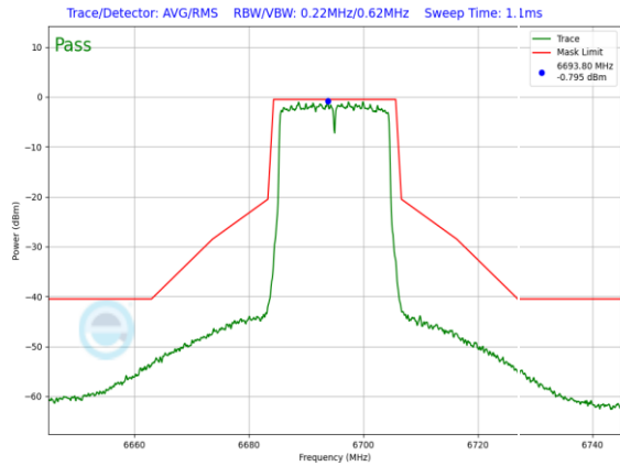
Plot 7-947. SP In-Band Emission Plot Antenna WF7 (20MHz 802.11ax (UNII Band 7) – Ch. 149, MCS4)
