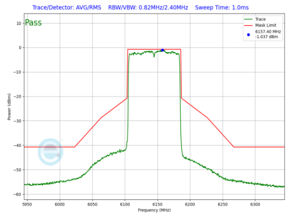
Plot 7-1062. SP In-Band Emission Plot CDD Primary Antenna WF8 (80MHz 802.11ax (UNII Band 5) – Ch. 39, MCS2)
