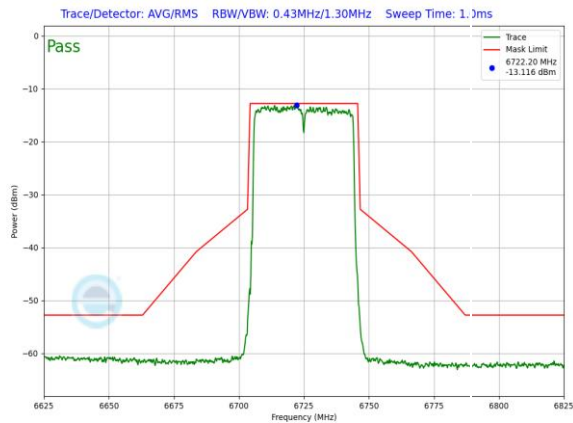
Plot 7-1012. LPI In-Band Emission Plot SDM Primary Antenna WF8 (40MHz 802.11ax (UNII Band 7) – Ch. 155, MCS4)
