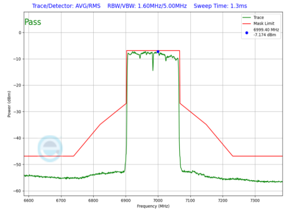
Plot 7-1024. LPI In-Band Emission Plot SDM Primary Antenna WF8 (160MHz 802.11ax (UNII Band 8) – Ch. 207, MCS4)
