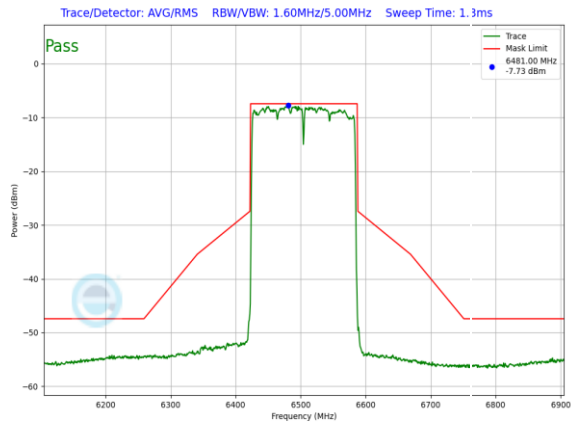
Plot 7-1007. LPI In-Band Emission Plot SDM Primary Antenna WF5B (160MHz 802.11ax (UNII Band 6) – Ch. 111, MCS4)
