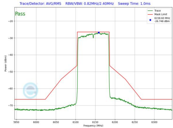
Plot 7-1061. SP In-Band Emission Plot CDD Primary Antenna WF5B (80MHz 802.11ax (UNII Band 5) – Ch. 39, MCS2)
