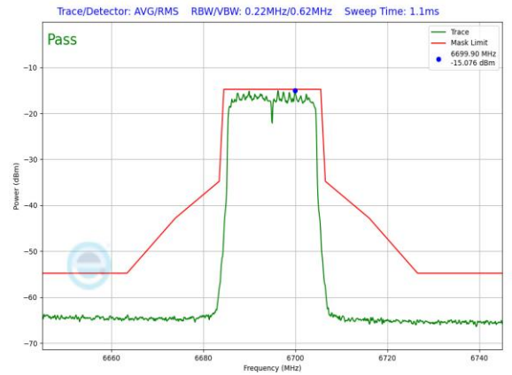
Plot 7-1042. LPI In-Band Emission Plot SDM Primary Antenna WF8 (20MHz 802.11ax (UNII Band 7) – Ch. 149, MCS11)
