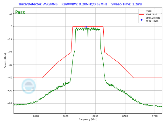
Plot 7-956. SP In-Band Emission Plot Antenna WF7 (20MHz 802.11a (UNII Band 7) – Ch. 149, 54Mbps)
