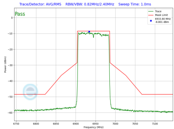
Plot 7-1021. LPI In-Band Emission Plot SDM Primary Antenna WF5B (80MHz 802.11ax (UNII Band 8) – Ch. 199, MCS4)
