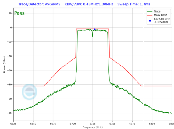
Plot 7-948. SP In-Band Emission Plot Antenna WF7 (40MHz 802.11ax (UNII Band 7) – Ch. 155, MCS4)
