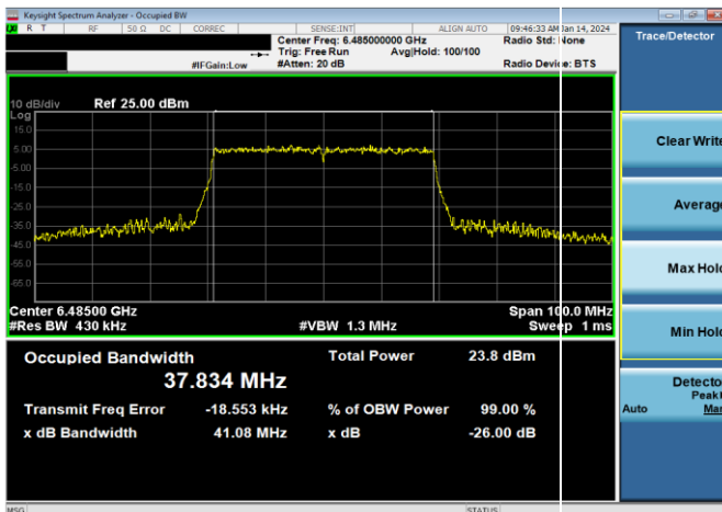
Plot 7-48. 26dB & 99% Bandwidth Plot Antenna WF5B (40MHz 802.11ax (UNII Band 6) – Ch. 107, MCS11)
