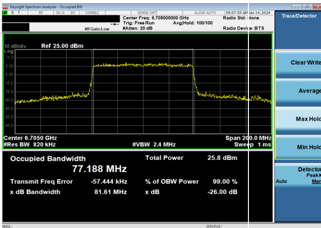
Plot 7-34. 26dB & 99% Bandwidth Plot Antenna WF5B (80MHz 802.11ax (UNII Band 7) – Ch. 151, MCS4)
