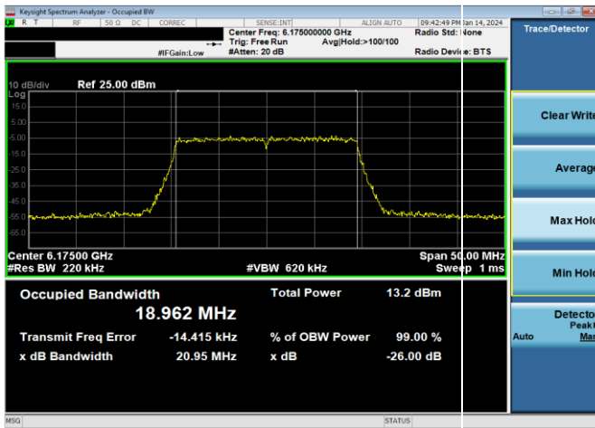
Plot 7-62. 26dB & 99% Bandwidth Plot Antenna WF8 (20MHz 802.11ax (UNII Band 5) – Ch. 45, MCS2)
