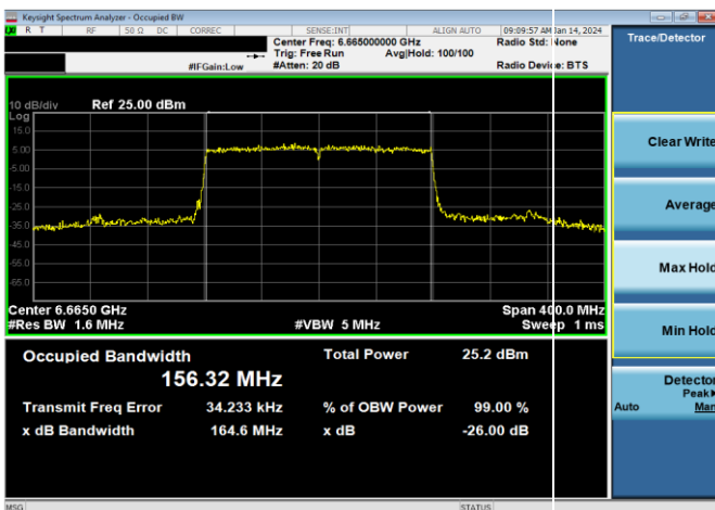
Plot 7-35. 26dB & 99% Bandwidth Plot Antenna WF5B (160MHz 802.11ax (UNII Band 7) – Ch. 143, MCS4)
