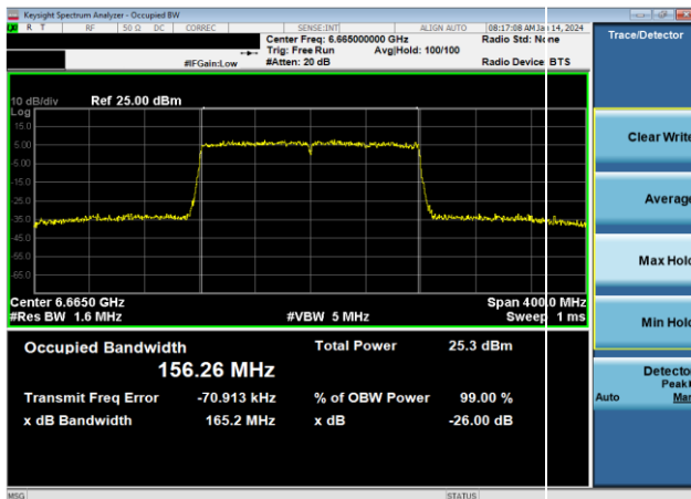
Plot 7-15. 26dB & 99% Bandwidth Plot Antenna WF5B (160MHz 802.11ax (UNII Band 7) – Ch. 143, MCS2)
