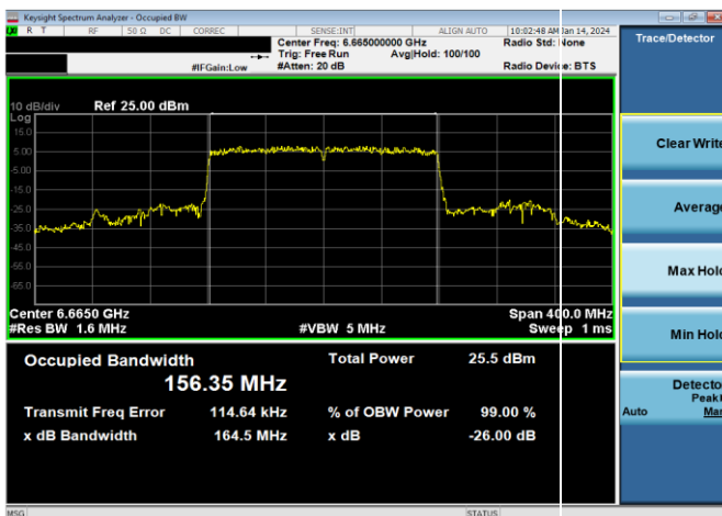
Plot 7-55. 26dB & 99% Bandwidth Plot Antenna WF5B (160MHz 802.11ax (UNII Band 7) – Ch. 143, MCS11)
