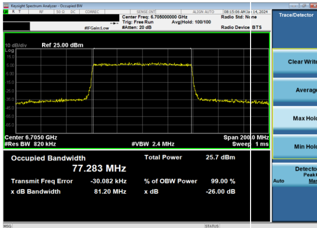
Plot 7-14. 26dB & 99% Bandwidth Plot Antenna WF5B (80MHz 802.11ax (UNII Band 7) – Ch. 151, MCS2)
