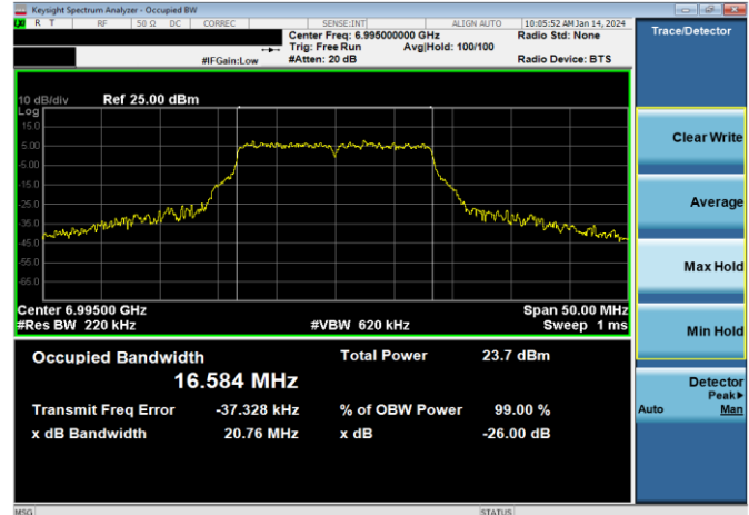
Plot 7-56. 26dB & 99% Bandwidth Plot Antenna WF5B (20MHz 802.11a (UNII Band 8) – Ch. 209, 54Mbps)
