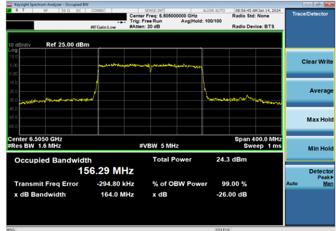
Plot 7-30. 26dB & 99% Bandwidth Plot Antenna WF5B (160MHz 802.11ax (UNII Band 6) – Ch. 111, MCS4)
