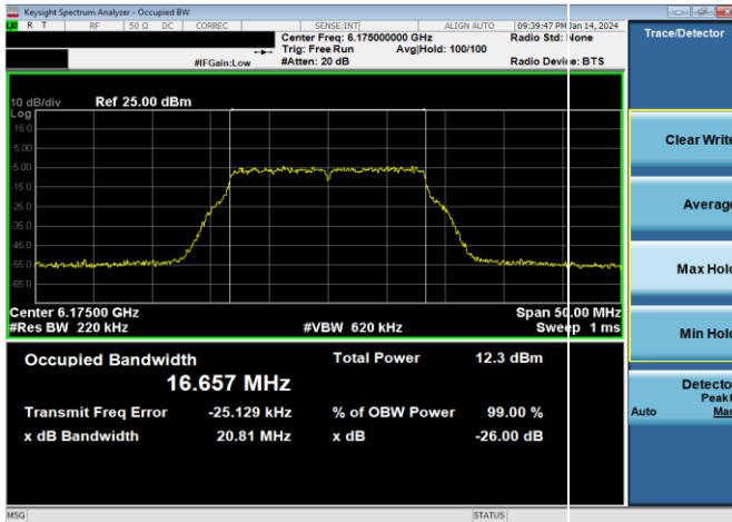
Plot 7-61. 26dB & 99% Bandwidth Plot Antenna WF8 (20MHz 802.11a (UNII Band 5) – Ch. 45, 12Mbps)
