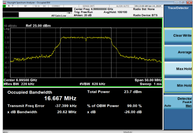
Plot 7-36. 26dB & 99% Bandwidth Plot Antenna WF5B (20MHz 802.11a (UNII Band 8) – Ch. 209, 24Mbps)
