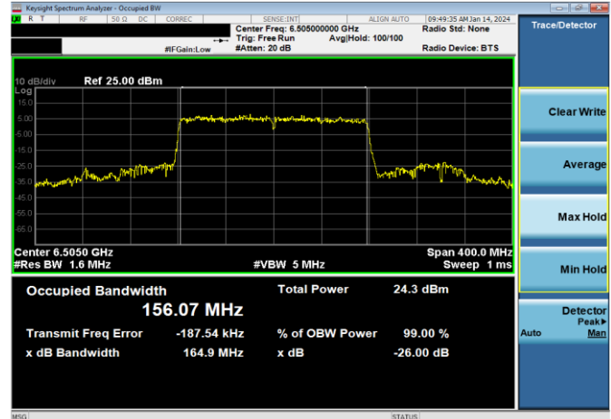
Plot 7-50. 26dB & 99% Bandwidth Plot Antenna WF5B (160MHz 802.11ax (UNII Band 6) – Ch. 111, MCS11)
