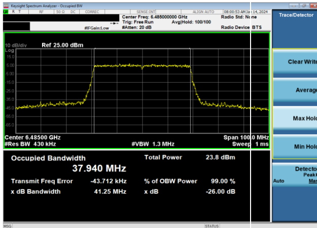
Plot 7-8. 26dB & 99% Bandwidth Plot Antenna WF5B (40MHz 802.11ax (UNII Band 6) – Ch. 107, MCS2)
