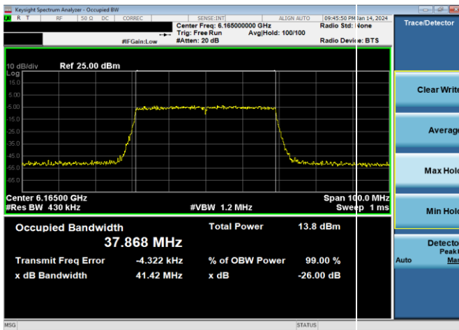
Plot 7-63. 26dB & 99% Bandwidth Plot Antenna WF8 (40MHz 802.11ax (UNII Band 5) – Ch. 43, MCS2)
