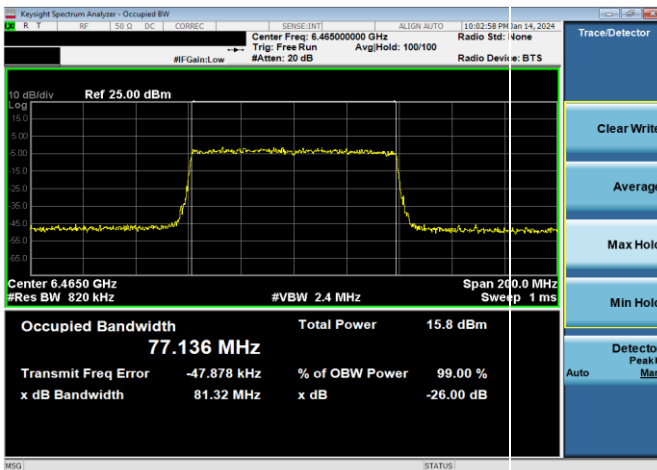
Plot 7-69. 26dB & 99% Bandwidth Plot Antenna WF8 (80MHz 802.11ax (UNII Band 6) – Ch. 103, MCS2)
