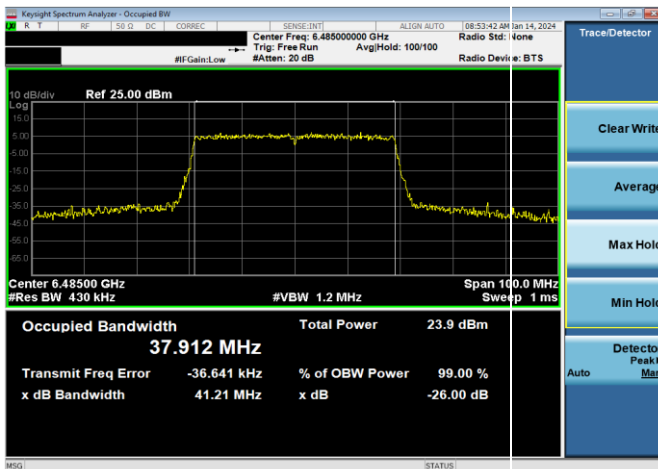
Plot 7-28. 26dB & 99% Bandwidth Plot Antenna WF5B (40MHz 802.11ax (UNII Band 6) – Ch. 107, MCS4)
