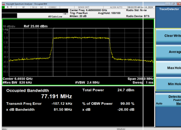
Plot 7-9. 26dB & 99% Bandwidth Plot Antenna WF5B (80MHz 802.11ax (UNII Band 6) – Ch. 103, MCS2)
