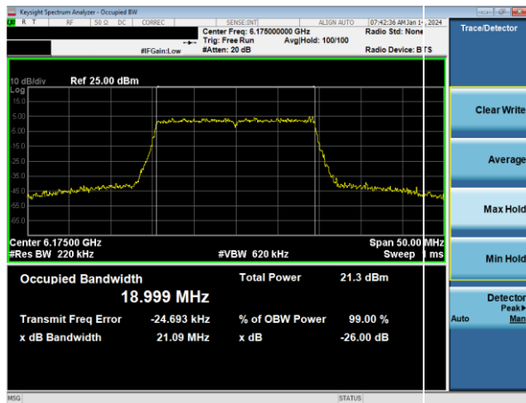
Plot 7-2. 26dB & 99% Bandwidth Plot Antenna WF5B (20MHz 802.11ax (UNII Band 5) – Ch. 45, MCS2)
