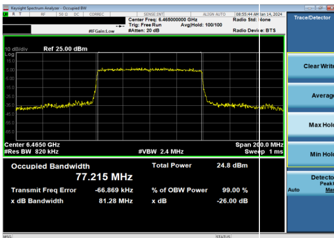
Plot 7-29. 26dB & 99% Bandwidth Plot Antenna WF5B (80MHz 802.11ax (UNII Band 6) – Ch. 103, MCS4)
