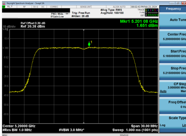
Plot 7-643. ISED PSD SDM Diversity Antenna WF7 (20MHz BW 11ax- RU242 – Ch.40)
