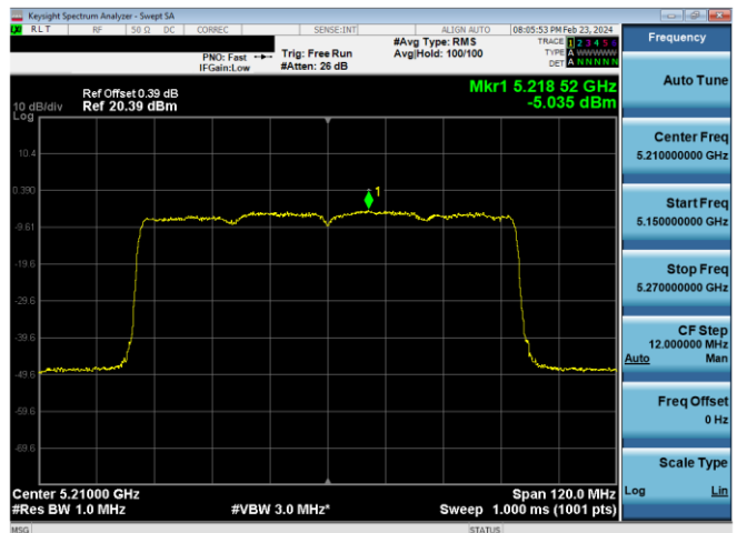
Plot 7-659. ISED PSD SDM Diversity Antenna WF7 (80MHz BW 11ax - RU996 - Ch.42)
