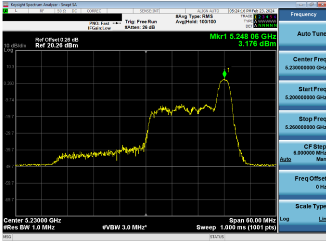
Plot 7-648. ISED PSD SDM Diversity Antenna WF5B (40MHz BW 11ax Index 17 - RU26 - Ch.46)
