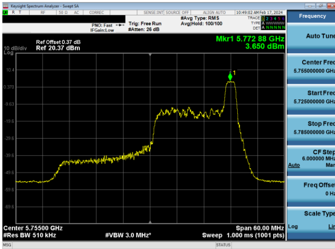
Plot 7-624. PSD CDD Diversity Antenna WF5B (40MHz BW 11ax Index 17 – RU26 – Ch.151)
