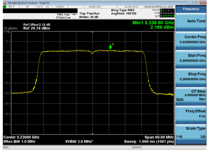
Plot 7-651. ISED PSD SDM Diversity Antenna WF7 (40MHz BW 11ax - RU484 - Ch.46)
