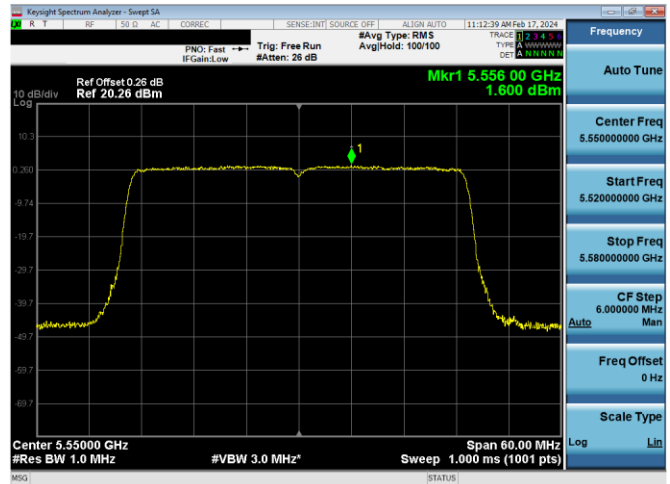
Plot 7-594. PSD CDD Diversity Antenna WF5B (40MHz BW 11ax - RU484 - Ch.110)
