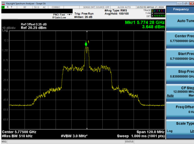
Plot 7-630. PSD CDD Diversity Antenna WF5B (80MHz BW 11ax Index 18 – RU26 – Ch.155)
