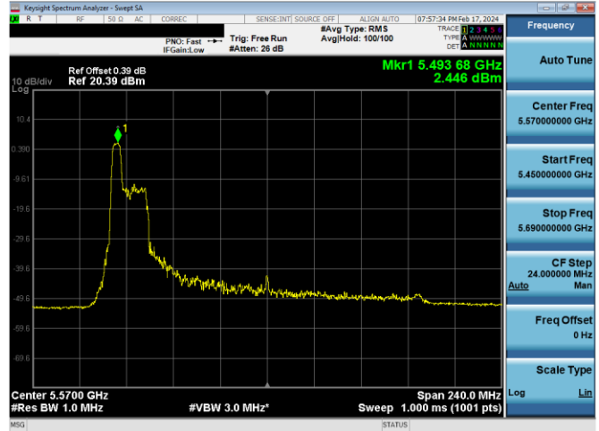
Plot 7-605. PSD CDD Diversity Antenna WF7 (160MHz BW 11ax Index 37 - RU52 - Ch.114 (L))
