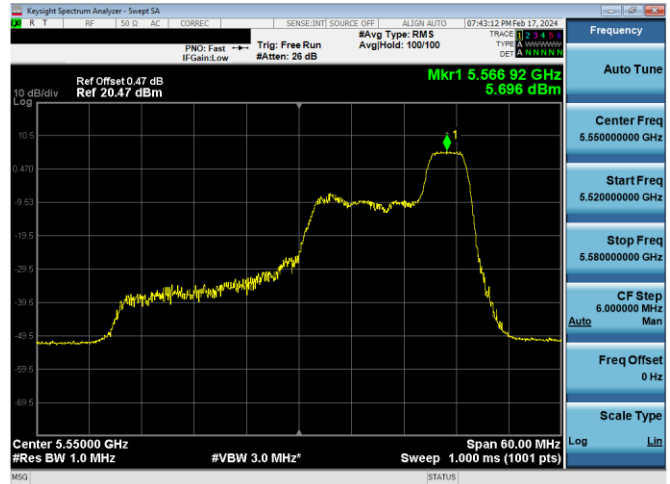
Plot 7-593. PSD CDD Diversity Antenna WF7 (40MHz BW 11ax Index 44 - RU52 - Ch.110)
