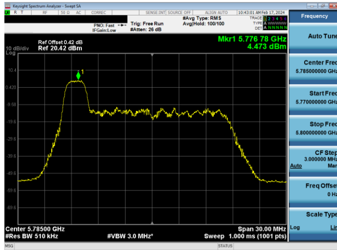
Plot 7-612. PSD CDD Diversity Antenna WF5B (20MHz BW 11ax Index 0 - RU26 - Ch.157)
