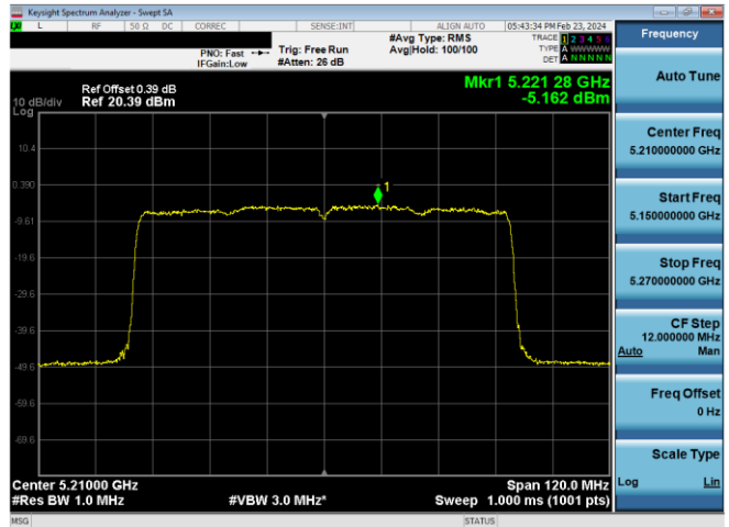
Plot 7-658. ISED PSD SDM Diversity Antenna WF5B (80MHz BW 11ax - RU996 - Ch.42)
