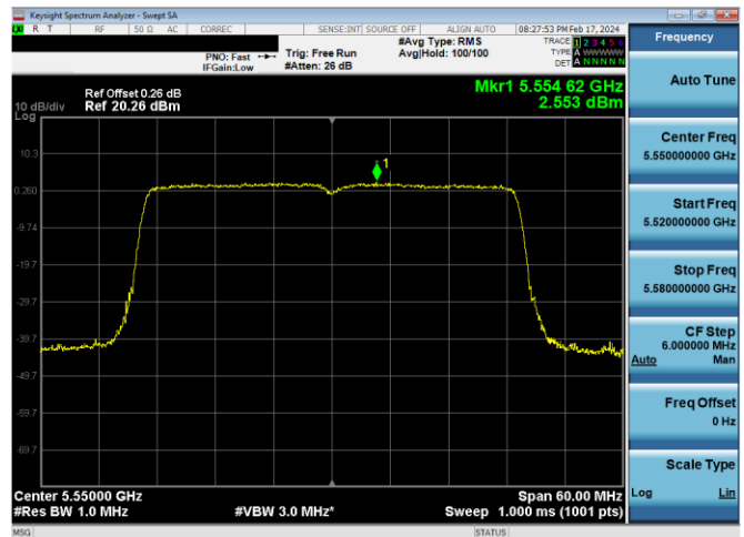
Plot 7-595. PSD CDD Diversity Antenna WF7 (40MHz BW 11ax - RU484 - Ch.110)
