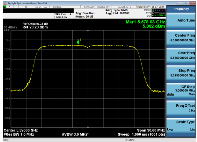
Plot 7-587. PSD CDD Diversity Antenna WF7 (20MHz BW 11ax– RU242 – Ch.116)
