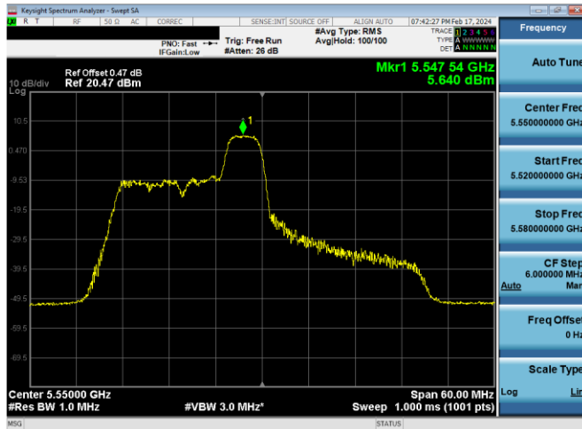
Plot 7-591. PSD CDD Diversity Antenna WF7 (40MHz BW 11ax Index 40 - RU52 - Ch.110)
