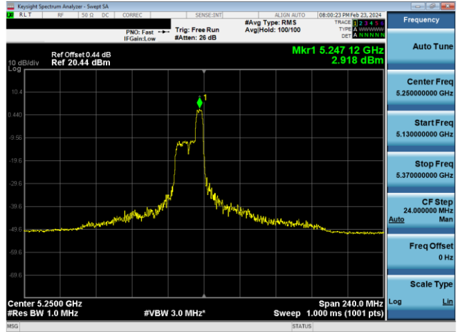
Plot 7-663. ISED PSD SDM Diversity Antenna WF7 (160MHz BW 11ax Index 52 – RU52 – Ch.50(L))
