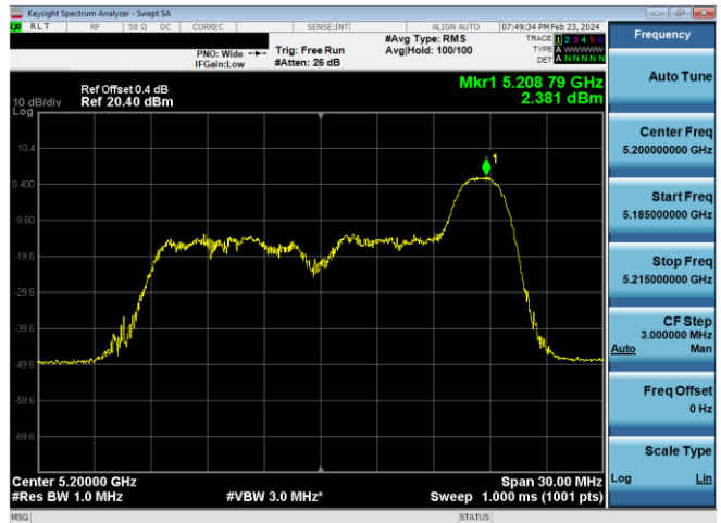
Plot 7-641. ISED PSD SDM Diversity Antenna WF7 (20MHz BW 11ax Index 8 – RU26 – Ch.40)
