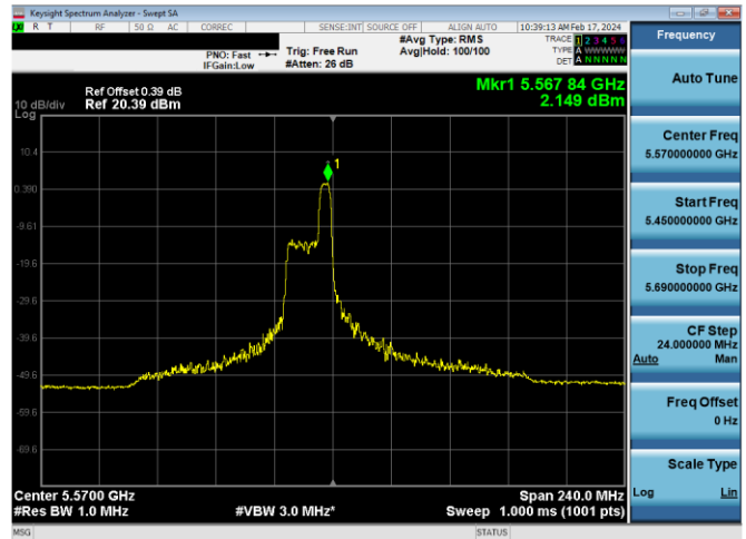
Plot 7-606. PSD CDD Diversity Antenna WF5B (160MHz BW 11ax Index 52 - RU52 - Ch.114 (L))
