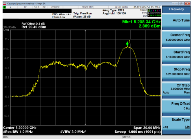
Plot 7-640. ISED PSD SDM Diversity Antenna WF5B (20MHz BW 11ax Index 8 – RU26 – Ch.40)
