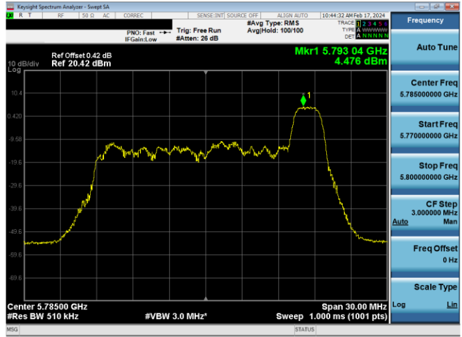
Plot 7-616. PSD CDD Diversity Antenna WF5B (20MHz BW 11ax Index 8 - RU26 - Ch.157)
