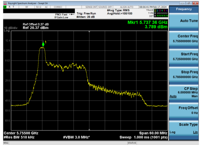
Plot 7-621. PSD CDD Diversity Antenna WF7 (40MHz BW 11ax Index 0 - RU26 - Ch.151)
