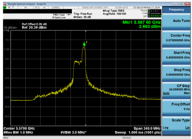
Plot 7-607. PSD CDD Diversity Antenna WF7 (160MHz BW 11ax Index 52 - RU52 - Ch.114 (L))
