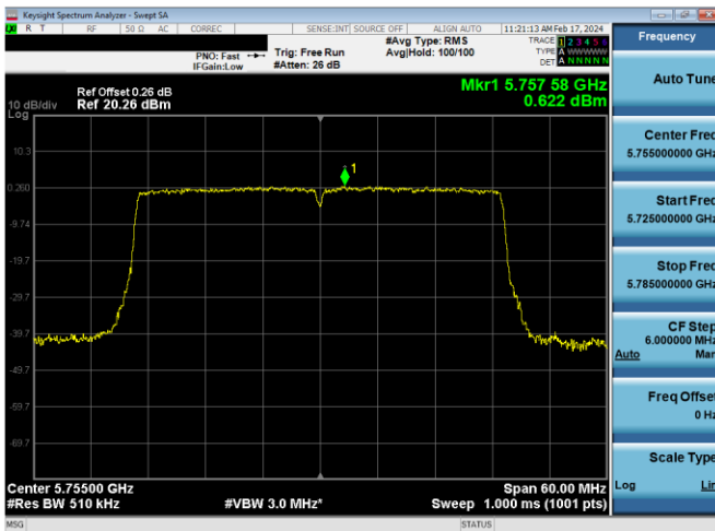
Plot 7-626. PSD CDD Diversity Antenna WF5B (40MHz BW 11ax – RU484 – Ch.151)
