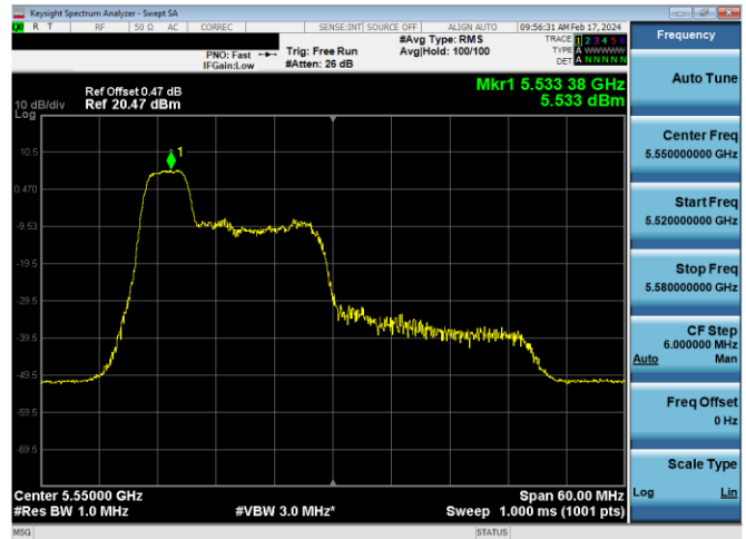
Plot 7-588. PSD CDD Diversity Antenna WF5B (40MHz BW 11ax Index 37 – RU52 – Ch.110)
