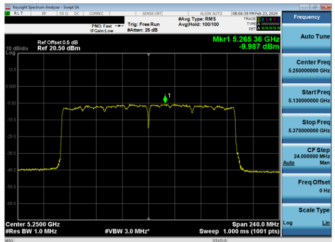
Plot 7-665. ISED PSD SDM Diversity Antenna WF7 (160MHz BW 11ax – RU996x2 – Ch.50)
