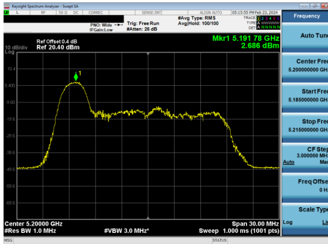
Plot 7-636. ISED PSD SDM Diversity Antenna WF5B (20MHz BW 11ax Index 0 – RU26 – Ch.40)
