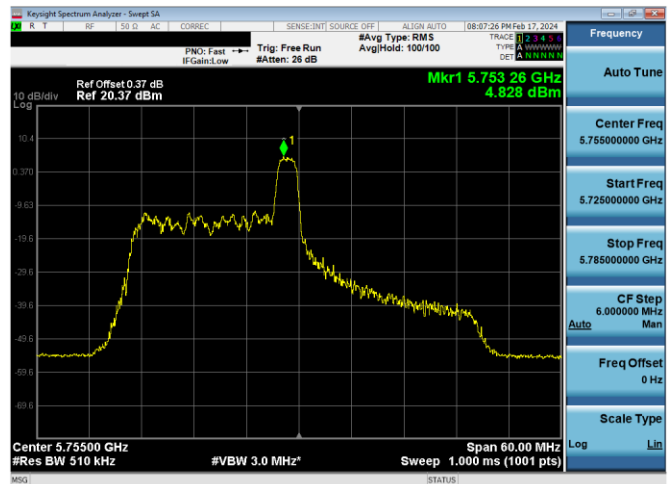
Plot 7-623. PSD CDD Diversity Antenna WF7 (40MHz BW 11ax Index 8 - RU26 - Ch.151)
