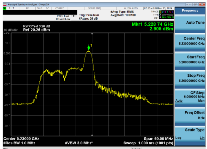
Plot 7-647. ISED PSD SDM Diversity Antenna WF7 (40MHz BW 11ax Index 8 – RU26 – Ch.46)
