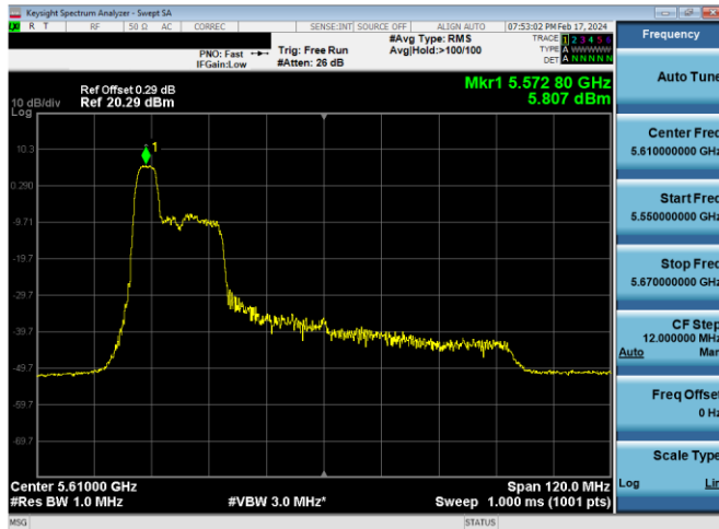
Plot 7-597. PSD CDD Diversity Antenna WF7 (80MHz BW 11ax Index 37 – RU52 – Ch.122)
