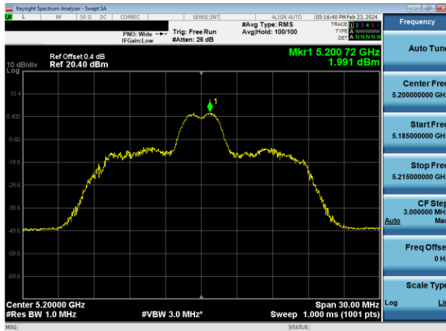
Plot 7-638. ISED PSD SDM Diversity Antenna WF5B (20MHz BW 11ax Index 4 – RU26 – Ch.40)
