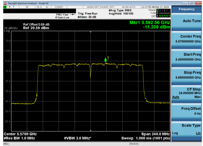
Plot 7-610. PSD CDD Diversity Antenna WF5B (160MHz BW 11ax – RU996x2 – Ch.114)
