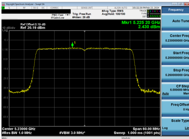
Plot 7-650. ISED PSD SDM Diversity Antenna WF5B (40MHz BW 11ax - RU484 - Ch.46)
