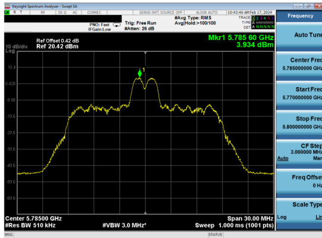
Plot 7-614. PSD CDD Diversity Antenna WF5B (20MHz BW 11ax Index 4 - RU26 - Ch.157)
