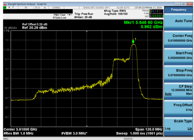
Plot 7-601. PSD CDD Diversity Antenna WF7 (80MHz BW 11ax Index 52 – RU52 – Ch.122)
