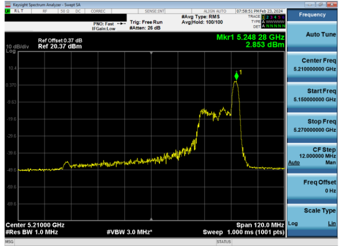
Plot 7-657. ISED PSD SDM Diversity Antenna WF7 (80MHz BW 11ax Index 36 - RU26 - Ch.42)
