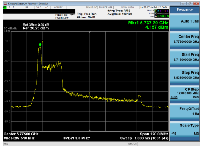
Plot 7-628. PSD CDD Diversity Antenna WF5B (80MHz BW 11ax Index 0 – RU26 – Ch.155)
