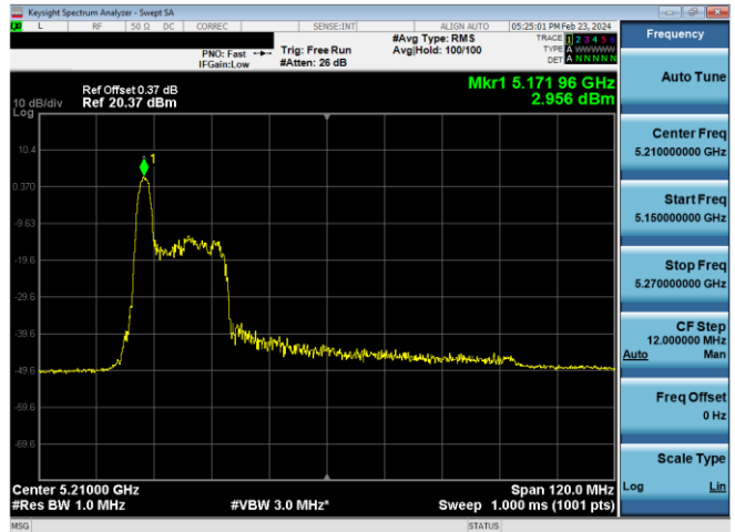
Plot 7-652. ISED PSD SDM Diversity Antenna WF5B (80MHz BW 11ax Index 0 - RU26 - Ch.42)
