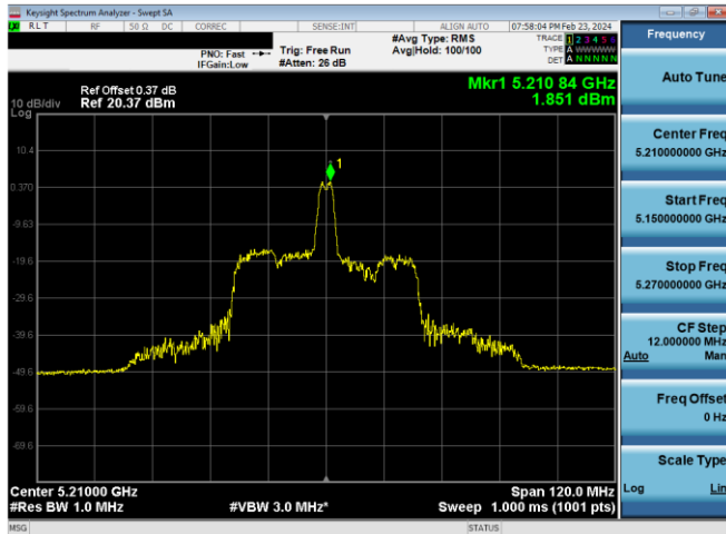
Plot 7-655. ISED PSD SDM Diversity Antenna WF7 (80MHz BW 11ax Index 18 - RU26 - Ch.42)
