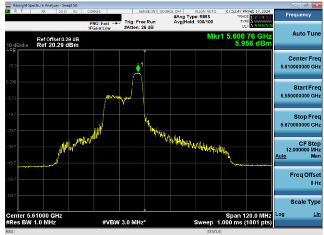
Plot 7-599. PSD CDD Diversity Antenna WF7 (80MHz BW 11ax Index 44 – RU52 – Ch.122)
