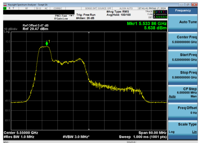
Plot 7-589. PSD CDD Diversity Antenna WF7 (40MHz BW 11ax Index 37 – RU52 – Ch.110)
