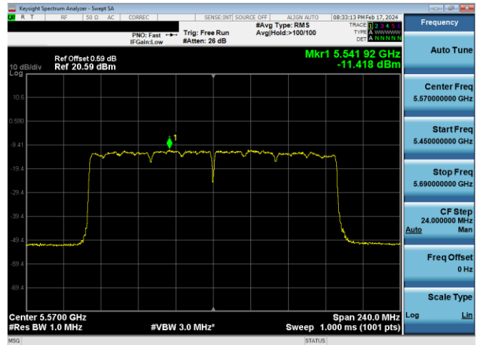
Plot 7-611. PSD CDD Diversity Antenna WF7 (160MHz BW 11ax – RU996x2 – Ch.114)
