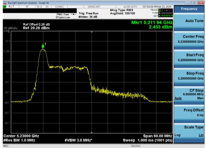
Plot 7-645. ISED PSD SDM Diversity Antenna WF7 (40MHz BW 11ax Index 0 – RU26 – Ch.46)
