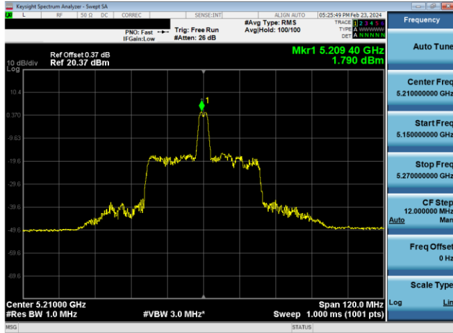
Plot 7-654. ISED PSD SDM Diversity Antenna WF5B (80MHz BW 11ax Index 18 - RU26 - Ch.42)
