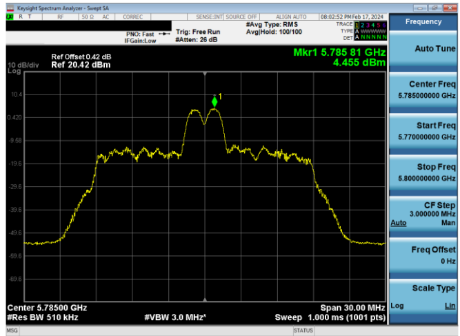
Plot 7-615. PSD CDD Diversity Antenna WF7 (20MHz BW 11ax Index 4 - RU26 - Ch.157)
