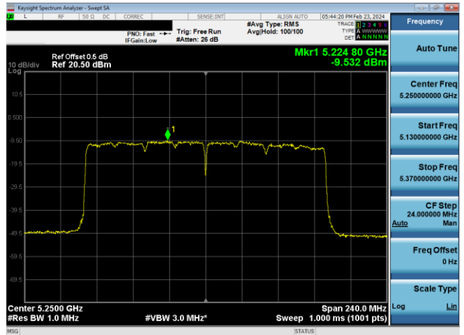
Plot 7-664. ISED PSD SDM Diversity Antenna WF5B (160MHz BW 11ax – RU996x2 – Ch.50)
