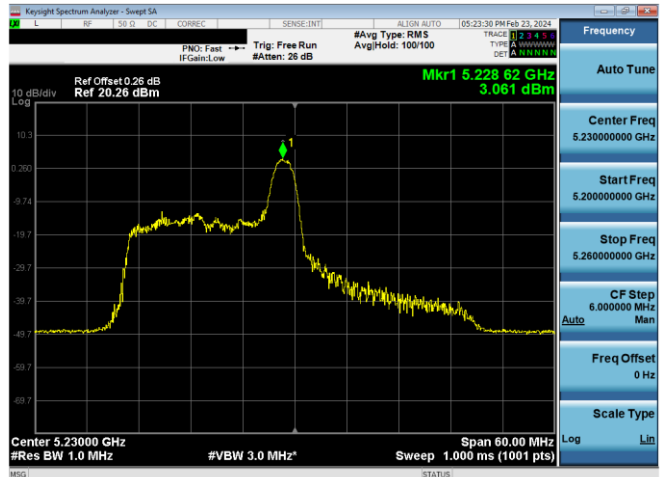
Plot 7-646. ISED PSD SDM Diversity Antenna WF5B (40MHz BW 11ax Index 8 – RU26 – Ch.46)
