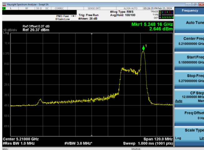
Plot 7-656. ISED PSD SDM Diversity Antenna WF5B (80MHz BW 11ax Index 36 - RU26 - Ch.42)
