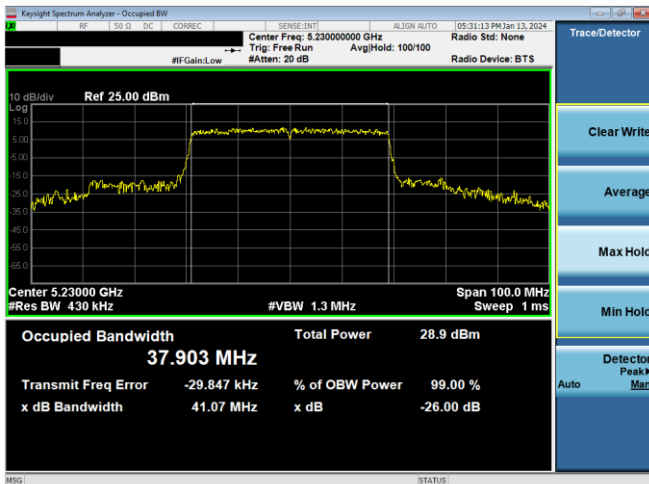
Plot 7-52. 26dB BW & 99% OBW Antenna WF8 (40MHz BW 11ax – RU484 – Ch.46)
