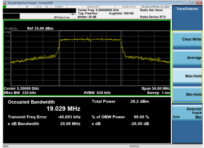
Plot 7-46. 26dB BW & 99% OBW Antenna WF8 (20MHz BW 11ax– RU242 – Ch.40)
