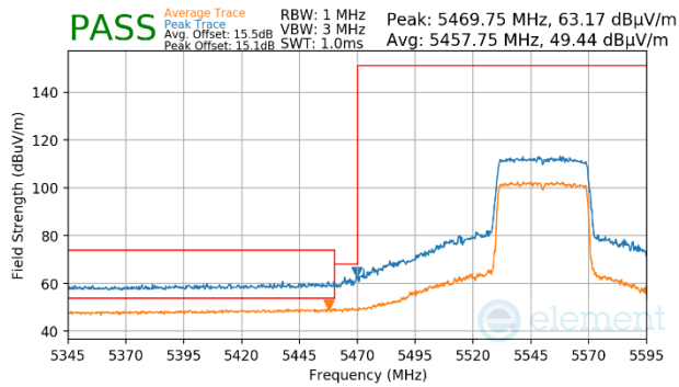
Plot 7-1742. CDD Primary (Peak & Average, Ch.110, 802.11ax(SU), MCS4)
