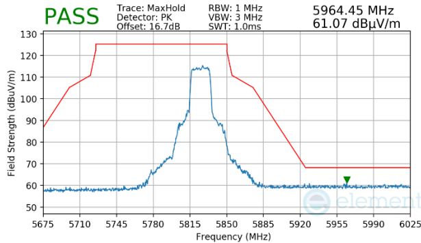
Plot 7-1663. CDD Primary (Peak, Ch.165, 802.11n, MCS15)
