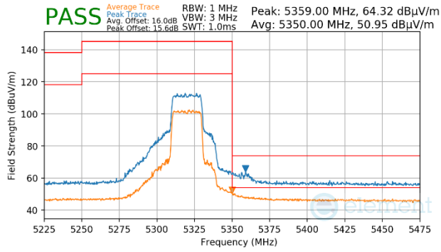
Plot 7-1674. CDD Primary (Peak & Average, Ch.64, 802.11ax(SU), MCS4)
