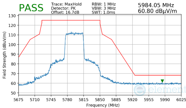
Plot 7-1756. CDD Primary (Peak, Ch.159, 802.11ax(SU), MCS2)
