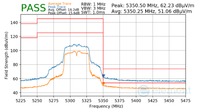
Plot 7-1704. CDD Primary (Peak & Average, Ch.62, 802.11n, MCS12)
