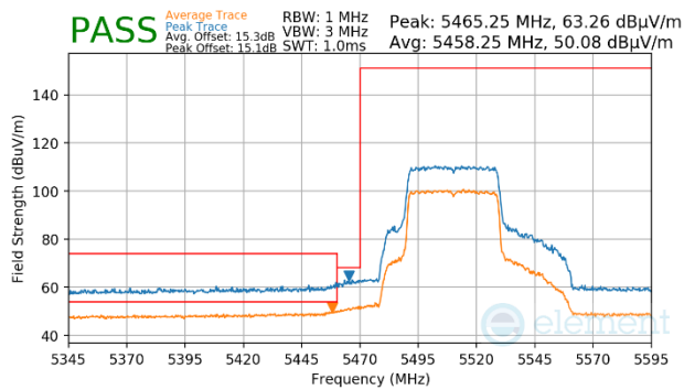
Plot 7-1738. CDD Primary (Peak & Average, Ch.102, 802.11ax(SU), MCS2)
