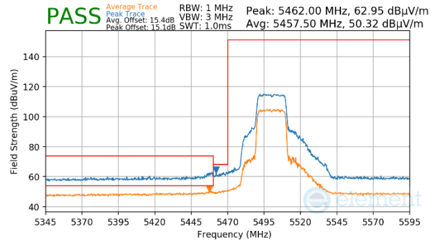
Plot 7-1677. CDD Primary (Peak & Average, Ch.100, 802.11ax(SU), MCS4)
