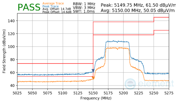
Plot 7-1726. CDD Primary (Peak & Average, Ch.38, 802.11ax(SU), MCS2)
