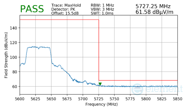
Plot 7-1716. (FCC Only) CDD Primary (Peak, Ch.126, 802.11n, MCS15)
