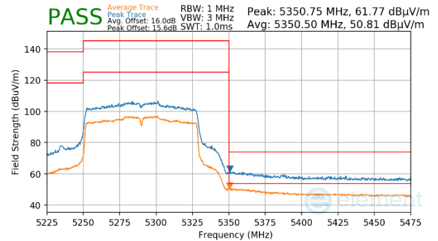
Plot 7-1762. CDD Primary (Peak & Average, Ch.58, 802.11ac, MCS2)
