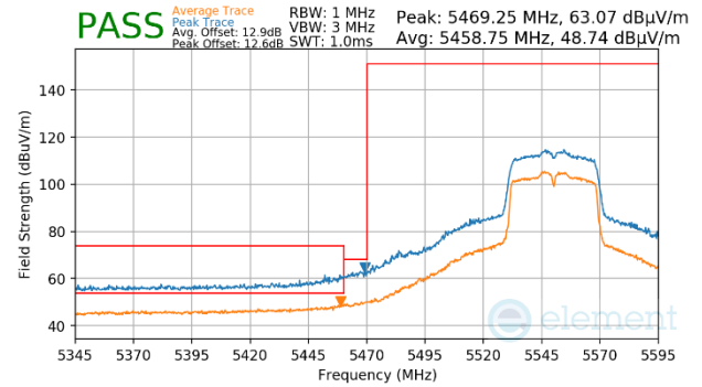
Plot 7-1709. CDD Primary (Peak & Average, Ch.110, 802.11n, MCS10)
