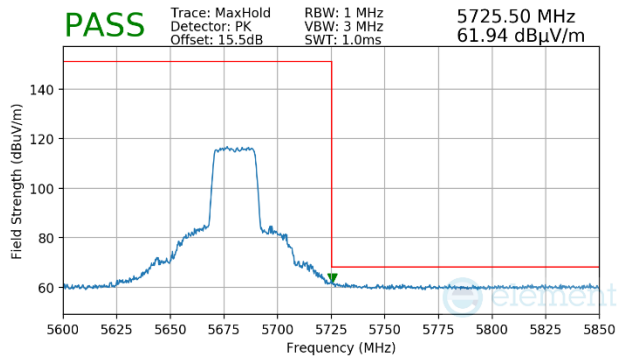
Plot 7-1682. CDD Primary (Peak, Ch.136, 802.11ax(SU), MCS2)
