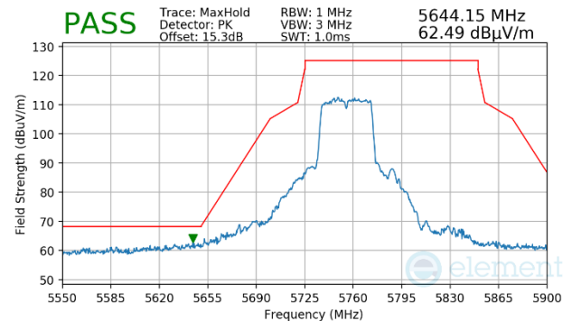
Plot 7-1722. CDD Primary (Peak, Ch.151, 802.11n, MCS15)
