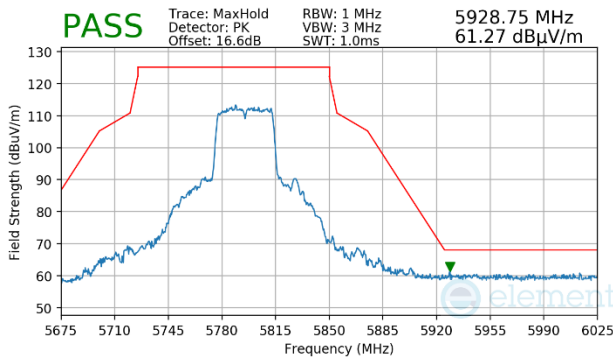
Plot 7-1725. CDD Primary (Peak, Ch.159, 802.11n, MCS15)
