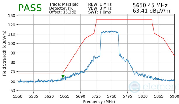
Plot 7-1755. CDD Primary (Peak, Ch.151, 802.11ax(SU), MCS11)
