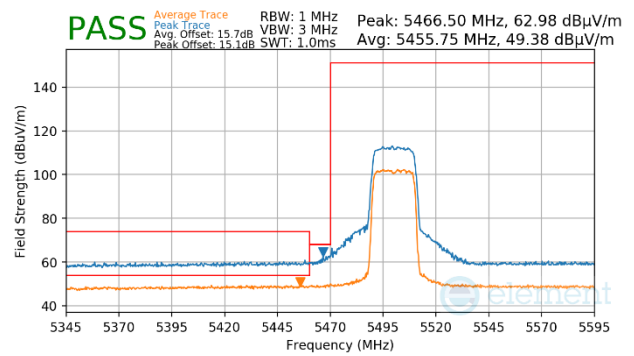
Plot 7-1678. CDD Primary (Peak & Average, Ch.100, 802.11ax(SU), MCS11)
