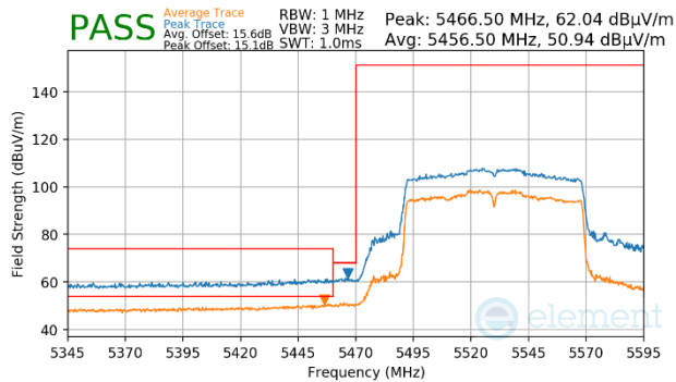
Plot 7-1766. CDD Primary (Peak & Average, Ch.106, 802.11ac, MCS4)
