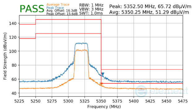
Plot 7-1675. CDD Primary (Peak & Average, Ch.64, 802.11ax(SU), MCS11)
