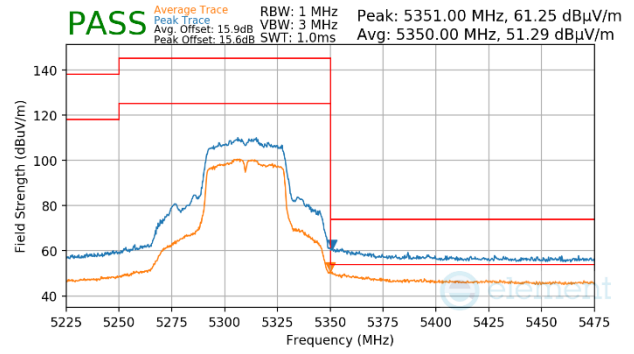
Plot 7-1703. CDD Primary (Peak & Average, Ch.62, 802.11n, MCS10)
