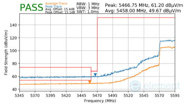
Plot 7-1745. (FCC Only) CDD Primary (Peak & Average, Ch.118, 802.11ax(SU), MCS4)
