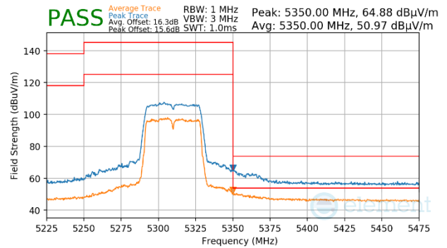
Plot 7-1705. CDD Primary (Peak & Average, Ch.62, 802.11n, MCS15)
