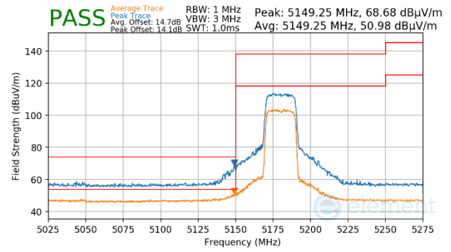
Plot 7-1666. CDD Primary (Peak & Average, Ch.36, 802.11ax(SU), MCS11)
