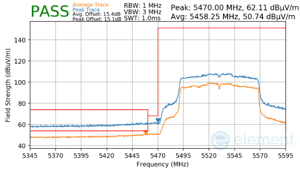
Plot 7-1765. CDD Primary (Peak & Average, Ch.106, 802.11ac, MCS2)
