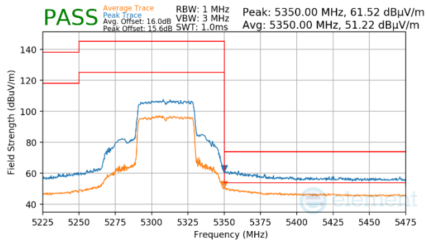
Plot 7-1736. CDD Primary (Peak & Average, Ch.62, 802.11ax(SU), MCS4)
