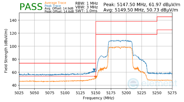
Plot 7-1727. CDD Primary (Peak & Average, Ch.38, 802.11ax(SU), MCS4)
