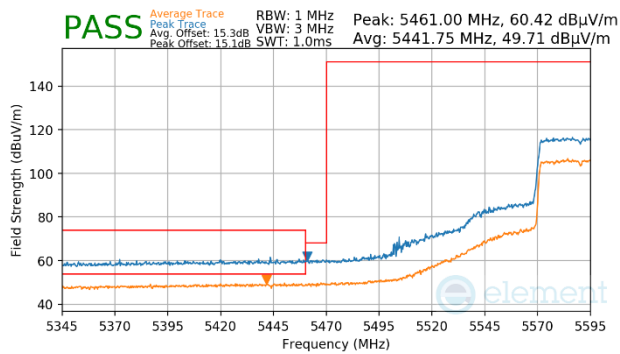
Plot 7-1744. (FCC Only) CDD Primary (Peak & Average, Ch.118, 802.11ax(SU), MCS2)
