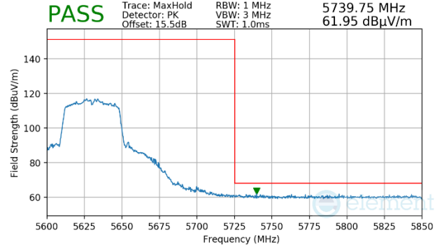
Plot 7-1715. (FCC Only) CDD Primary (Peak, Ch.126, 802.11n, MCS12)
