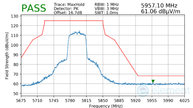
Plot 7-1723. CDD Primary (Peak, Ch.159, 802.11n, MCS10)
