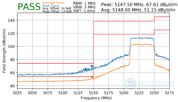
Plot 7-1730. CDD Primary (Peak & Average, Ch.46, 802.11ax(SU), MCS4)
