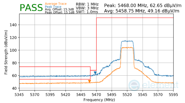
Plot 7-1679. CDD Primary (Peak & Average, Ch.104, 802.11ax(SU), MCS2)
