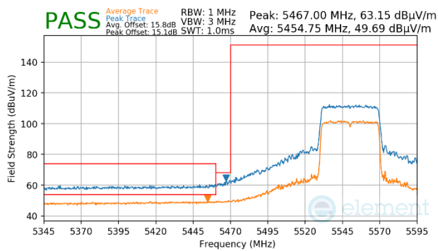
Plot 7-1743. CDD Primary (Peak & Average, Ch.110, 802.11ax(SU), MCS11)
