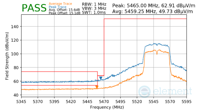
Plot 7-1710. CDD Primary (Peak & Average, Ch.110, 802.11n, MCS12)
