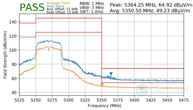
Plot 7-1700. CDD Primary (Peak & Average, Ch.54, 802.11n, MCS10)
