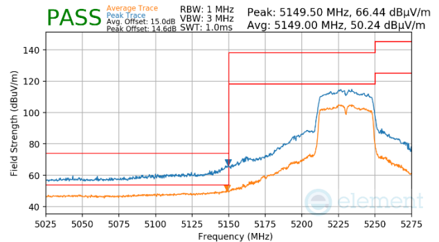
Plot 7-1698. CDD Primary (Peak & Average, Ch.46, 802.11n, MCS12)
