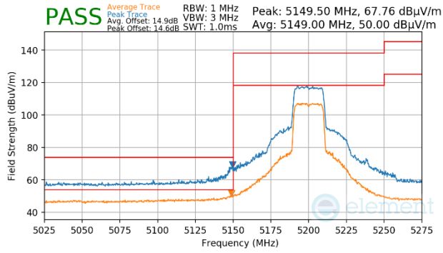
Plot 7-1668. CDD Primary (Peak & Average, Ch.40, 802.11ax(SU), MCS4)
