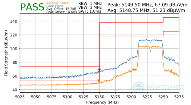
Plot 7-1699. CDD Primary (Peak & Average, Ch.46, 802.11n, MCS15)
