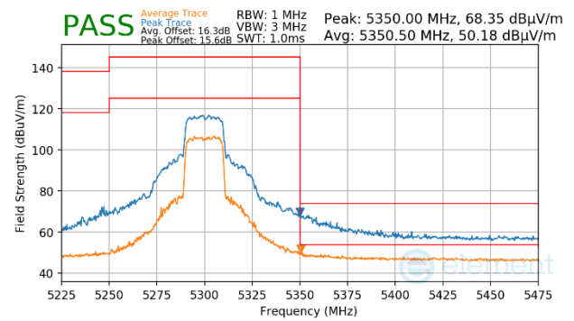
Plot 7-1672. CDD Primary (Peak & Average, Ch.60, 802.11ax(SU), MCS11)
