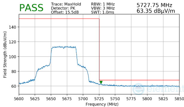
Plot 7-1750. CDD Primary (Peak, Ch.134, 802.11ax(SU), MCS2)
