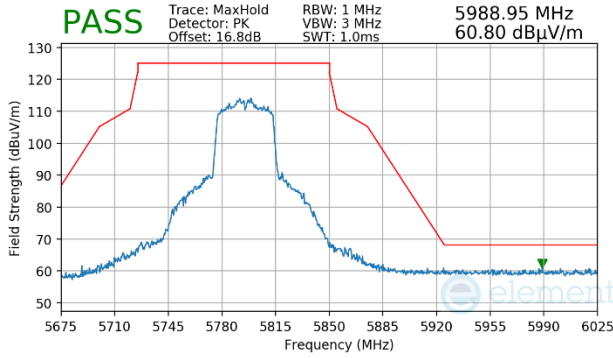
Plot 7-1724. CDD Primary (Peak, Ch.159, 802.11n, MCS12)
