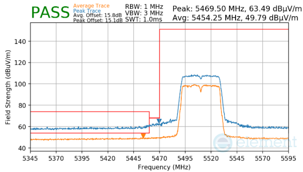
Plot 7-1708. CDD Primary (Peak & Average, Ch.102, 802.11n, MCS15)
