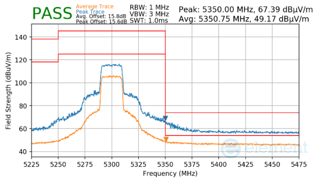
Plot 7-1670. CDD Primary (Peak & Average, Ch.60, 802.11ax(SU), MCS2)
