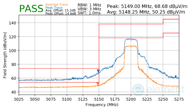
Plot 7-1669. CDD Primary (Peak & Average, Ch.40, 802.11ax(SU), MCS11)
