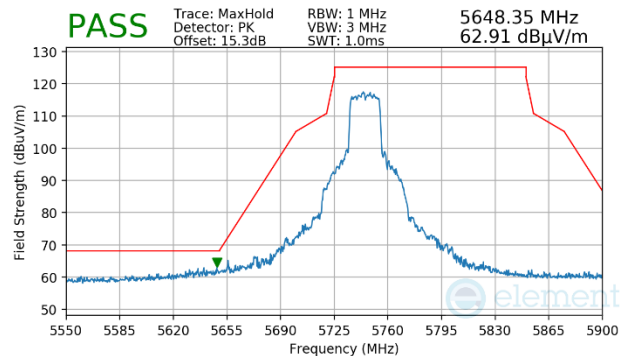
Plot 7-1690. CDD Primary (Peak, Ch.149, 802.11ax(SU), MCS11)
