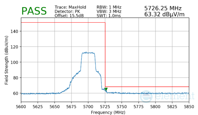
Plot 7-1685. CDD Primary (Peak, Ch.140, 802.11ax(SU), MCS2)
