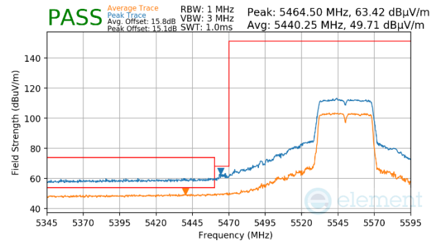
Plot 7-1711. CDD Primary (Peak & Average, Ch.110, 802.11n, MCS15)
