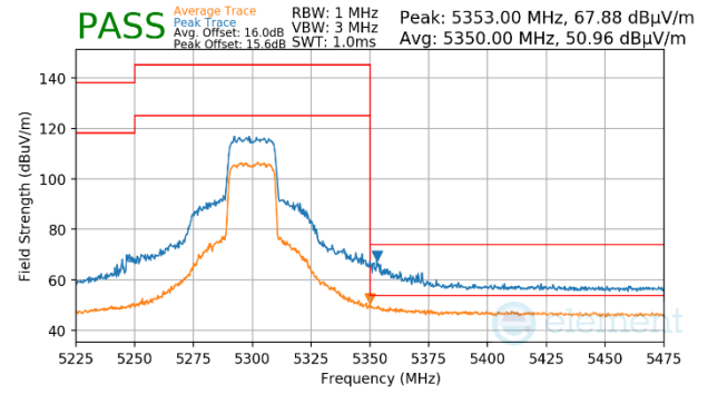
Plot 7-1671. CDD Primary (Peak & Average, Ch.60, 802.11ax(SU), MCS4)
