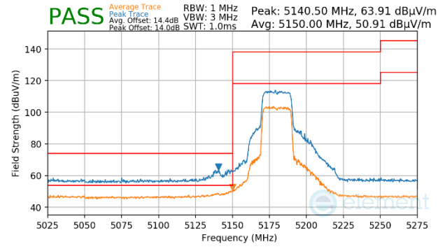
Plot 7-1665. CDD Primary (Peak & Average, Ch.36, 802.11ax(SU), MCS4)
