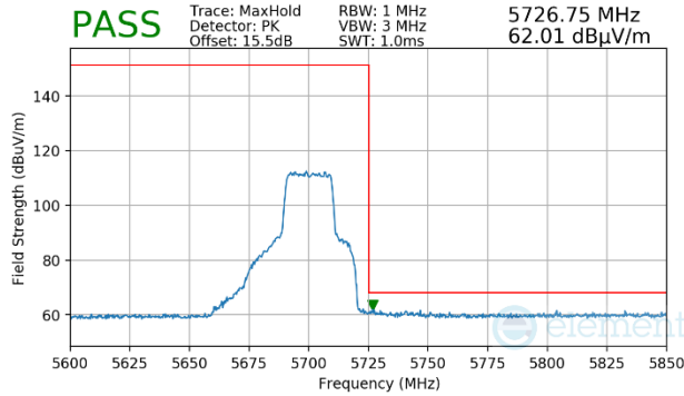
Plot 7-1686. CDD Primary (Peak, Ch.140, 802.11ax(SU), MCS4)
