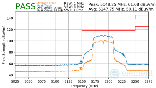
Plot 7-1695. CDD Primary (Peak & Average, Ch.38, 802.11n, MCS12)
