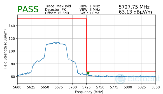
Plot 7-1717. CDD Primary (Peak, Ch.134, 802.11n, MCS10)
