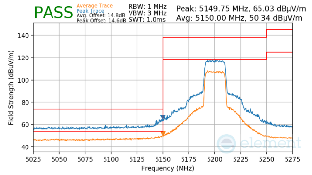
Plot 7-1667. CDD Primary (Peak & Average, Ch.40, 802.11ax(SU), MCS2)
