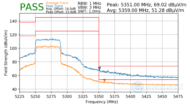
Plot 7-1733. CDD Primary (Peak & Average, Ch.54, 802.11ax(SU), MCS4)
