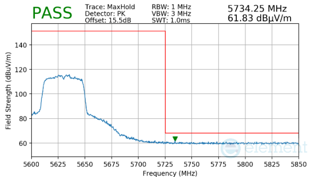
Plot 7-1714. (FCC Only) CDD Primary (Peak, Ch.126, 802.11n, MCS10)
