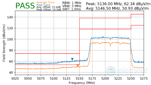
Plot 7-1761. CDD Primary (Peak & Average, Ch.42, 802.11ac, MCS9)
