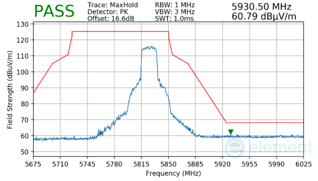
Plot 7-1693. CDD Primary (Peak, Ch.165, 802.11ax(SU), MCS11)
