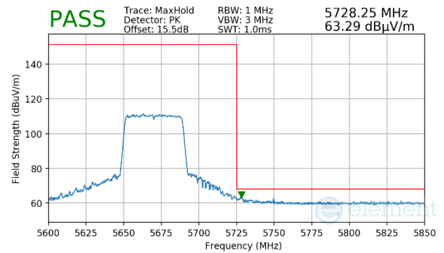
Plot 7-1752. CDD Primary (Peak, Ch.134, 802.11ax(SU), MCS11)
