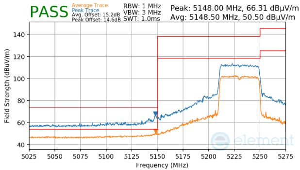
Plot 7-1731. CDD Primary (Peak & Average, Ch.46, 802.11ax(SU), MCS11)
