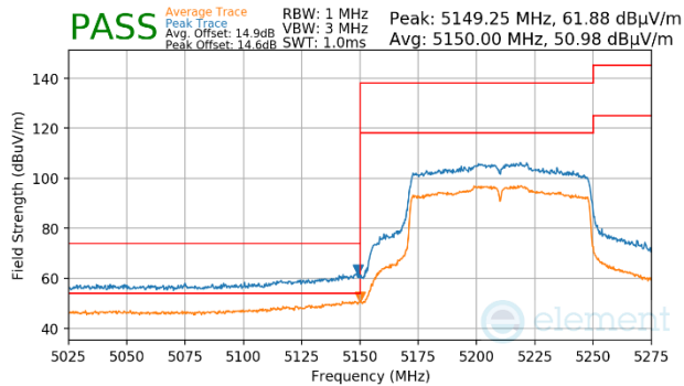
Plot 7-1759. CDD Primary (Peak & Average, Ch.42, 802.11ac, MCS2)
