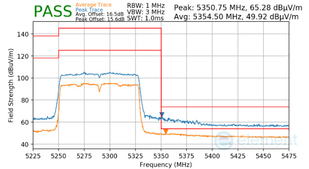
Plot 7-1764. CDD Primary (Peak & Average, Ch.58, 802.11ac, MCS9)
