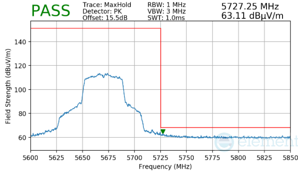
Plot 7-1718. CDD Primary (Peak, Ch.134, 802.11n, MCS12)
