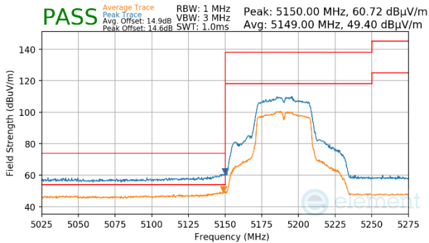
Plot 7-1694. CDD Primary (Peak & Average, Ch.38, 802.11n, MCS10)
