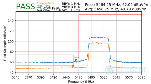
Plot 7-1740. CDD Primary (Peak & Average, Ch.102, 802.11ax(SU), MCS11)
