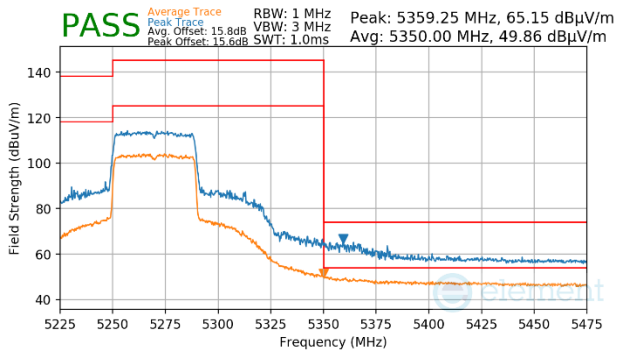
Plot 7-1732. CDD Primary (Peak & Average, Ch.54, 802.11ax(SU), MCS2)
