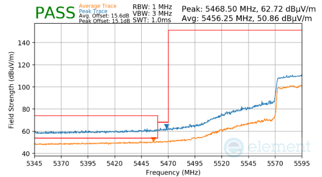
Plot 7-1769. (FCC Only) CDD Primary (Peak & Average, Ch.122, 802.11ac, MCS4)
