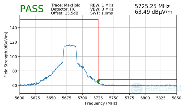
Plot 7-1684. CDD Primary (Peak, Ch.136, 802.11ax(SU), MCS11)
