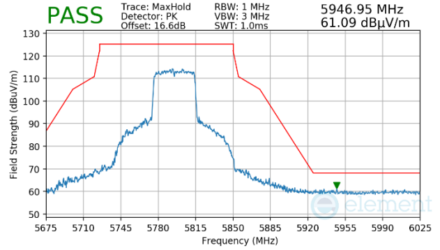
Plot 7-1757. CDD Primary (Peak, Ch.159, 802.11ax(SU), MCS4)
