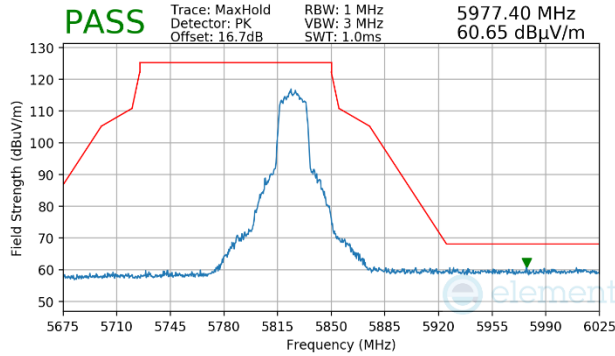
Plot 7-1662. CDD Primary (Peak, Ch.165, 802.11n, MCS12)
