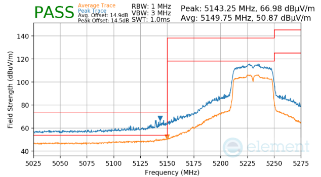
Plot 7-1697. CDD Primary (Peak & Average, Ch.46, 802.11n, MCS10)
