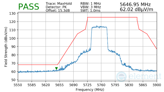
Plot 7-1753. CDD Primary (Peak, Ch.151, 802.11ax(SU), MCS2)
