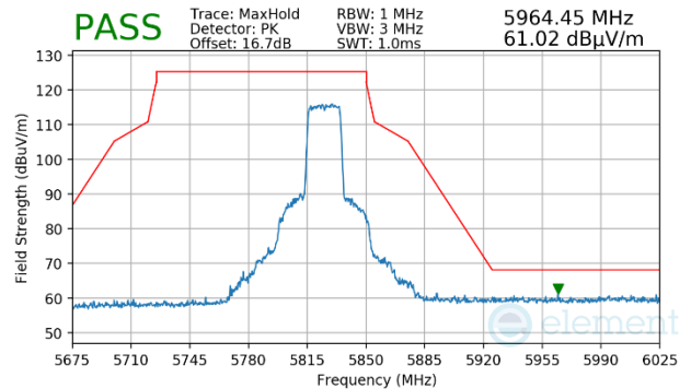
Plot 7-1691. CDD Primary (Peak, Ch.165, 802.11ax(SU), MCS2)
