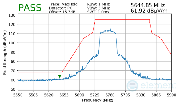
Plot 7-1720. CDD Primary (Peak, Ch.151, 802.11n, MCS10)
