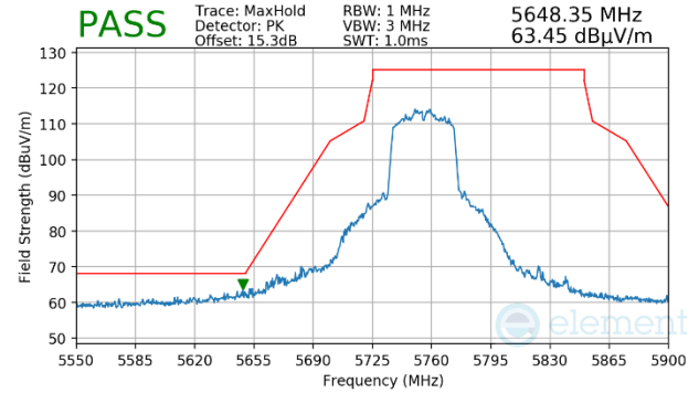
Plot 7-1721. CDD Primary (Peak, Ch.151, 802.11n, MCS12)
