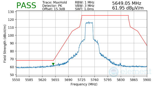
Plot 7-1689. CDD Primary (Peak, Ch.149, 802.11ax(SU), MCS4)
