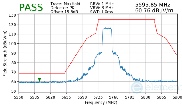
Plot 7-1688. CDD Primary (Peak, Ch.149, 802.11ax(SU), MCS2)
