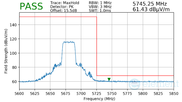
Plot 7-1683. CDD Primary (Peak, Ch.136, 802.11ax(SU), MCS4)
