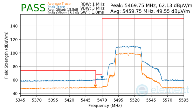
Plot 7-1739. CDD Primary (Peak & Average, Ch.102, 802.11ax(SU), MCS4)
