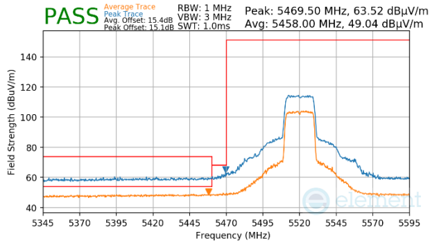
Plot 7-1680. CDD Primary (Peak & Average, Ch.104, 802.11ax(SU), MCS4)
