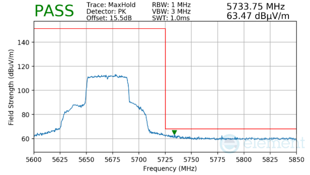
Plot 7-1751. CDD Primary (Peak, Ch.134, 802.11ax(SU), MCS4)
