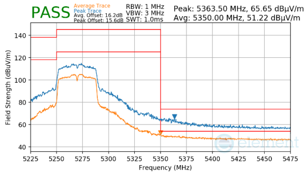
Plot 7-1701. CDD Primary (Peak & Average, Ch.54, 802.11n, MCS12)
