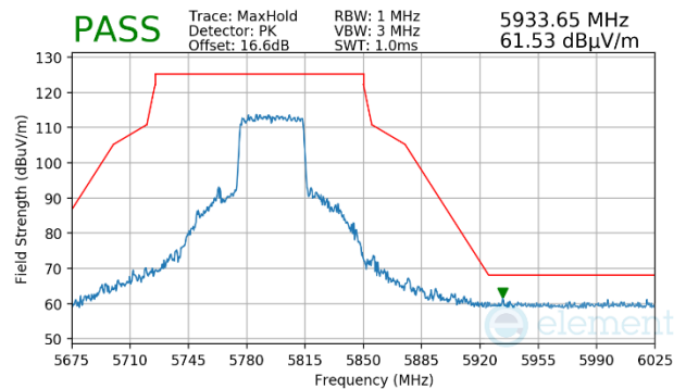
Plot 7-1758. CDD Primary (Peak, Ch.159, 802.11ax(SU), MCS11)
