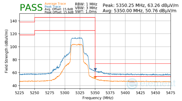
Plot 7-1673. CDD Primary (Peak & Average, Ch.64, 802.11ax(SU), MCS2)
