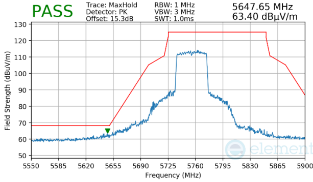
Plot 7-1754. CDD Primary (Peak, Ch.151, 802.11ax(SU), MCS4)
