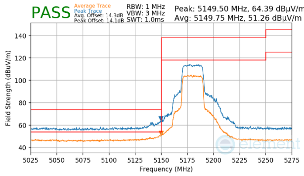
Plot 7-1664. CDD Primary (Peak & Average, Ch.36, 802.11ax(SU), MCS2)
