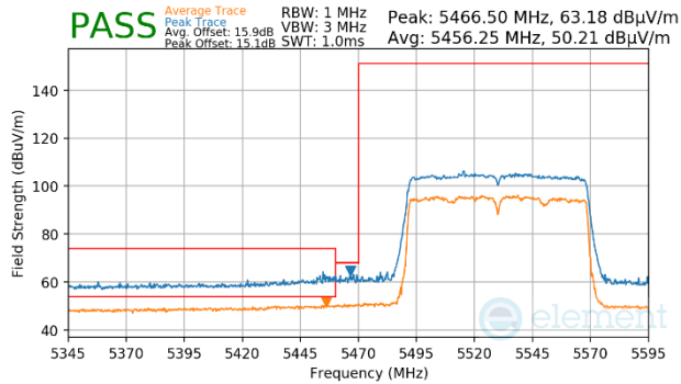
Plot 7-1767. CDD Primary (Peak & Average, Ch.106, 802.11ac, MCS11)
