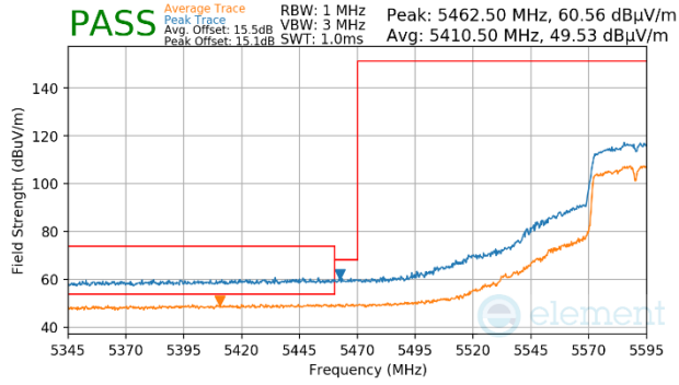
Plot 7-1712. (FCC Only) CDD Primary (Peak & Average, Ch.118, 802.11n, MCS12)
