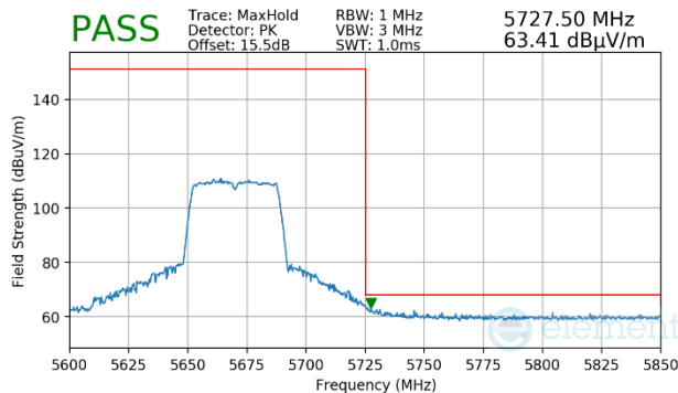
Plot 7-1719. CDD Primary (Peak, Ch.134, 802.11n, MCS15)
