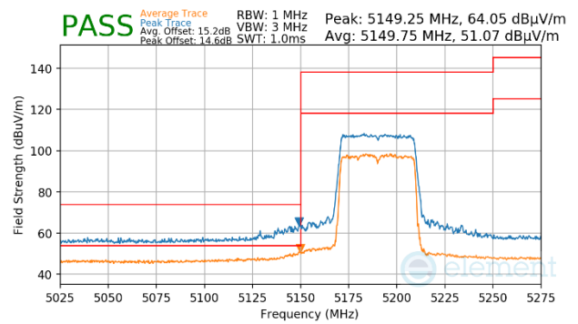
Plot 7-1728. CDD Primary (Peak & Average, Ch.38, 802.11ax(SU), MCS11)
