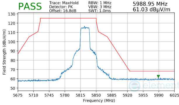
Plot 7-1692. CDD Primary (Peak, Ch.165, 802.11ax(SU), MCS4)
