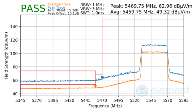
Plot 7-1741. CDD Primary (Peak & Average, Ch.110, 802.11ax(SU), MCS2)
