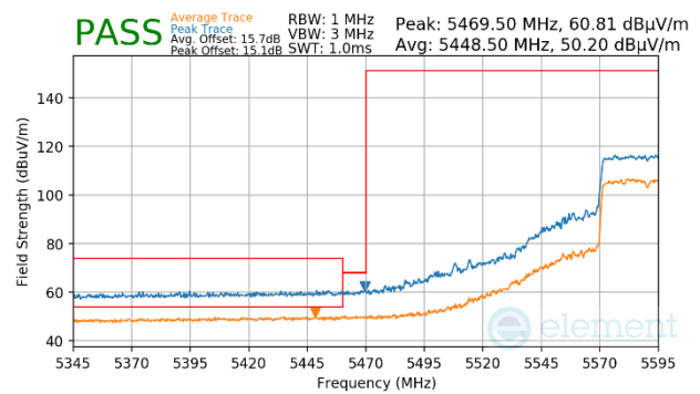
Plot 7-1746. (FCC Only) CDD Primary (Peak & Average, Ch.118, 802.11ax(SU), MCS11)
