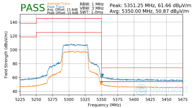
Plot 7-1735. CDD Primary (Peak & Average, Ch.62, 802.11ax(SU), MCS2)
