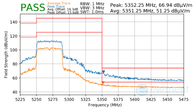
Plot 7-1734. CDD Primary (Peak & Average, Ch.54, 802.11ax(SU), MCS11)
