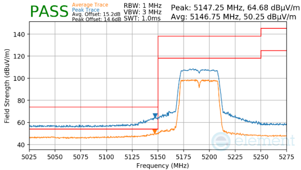
Plot 7-1696. CDD Primary (Peak & Average, Ch.38, 802.11n, MCS15)
