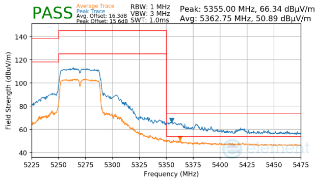
Plot 7-1702. CDD Primary (Peak & Average, Ch.54, 802.11n, MCS15)
