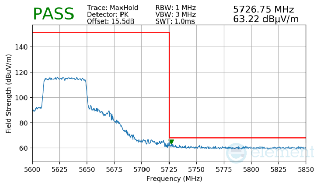
Plot 7-1749. (FCC Only) CDD Primary (Peak, Ch.126, 802.11ax(SU), MCS11)
