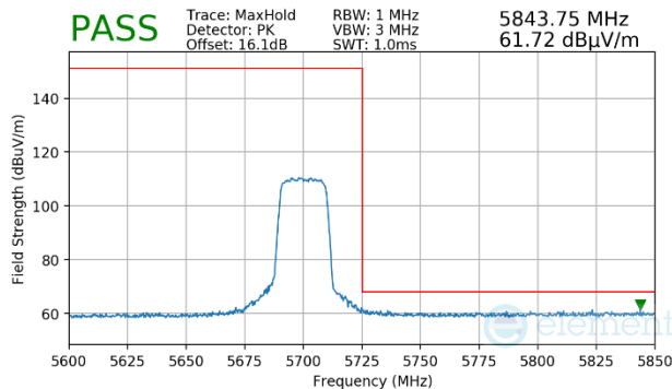
Plot 7-1687. CDD Primary (Peak, Ch.140, 802.11ax(SU), MCS11)
