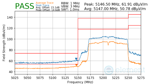
Plot 7-1760. CDD Primary (Peak & Average, Ch.42, 802.11ac, MCS4)
