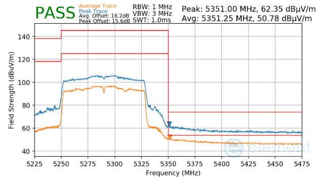
Plot 7-1763. CDD Primary (Peak & Average, Ch.58, 802.11ac, MCS4)
