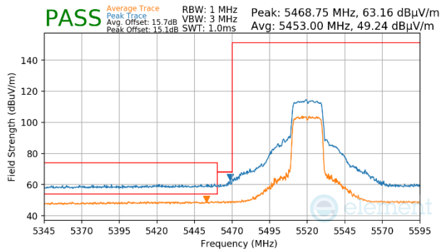
Plot 7-1681. CDD Primary (Peak & Average, Ch.104, 802.11ax(SU), MCS11)
