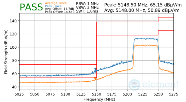
Plot 7-1729. CDD Primary (Peak & Average, Ch.46, 802.11ax(SU), MCS2)
