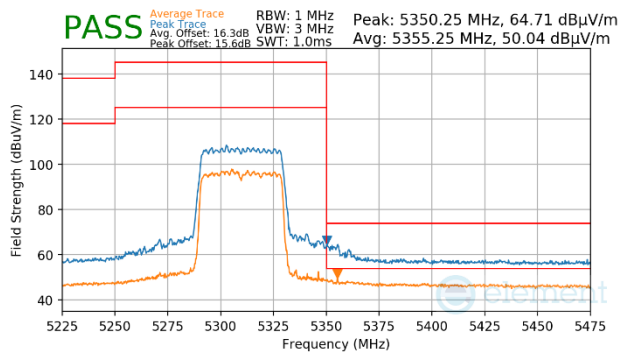
Plot 7-1737. CDD Primary (Peak & Average, Ch.62, 802.11ax(SU), MCS11)
