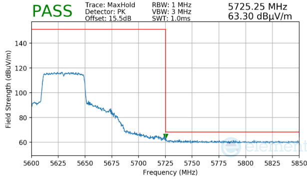
Plot 7-1748. (FCC Only) CDD Primary (Peak, Ch.126, 802.11ax(SU), MCS4)
