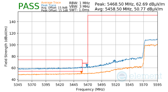
Plot 7-1770. (FCC Only) CDD Primary (Peak & Average, Ch.122, 802.11ac, MCS9)
