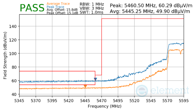
Plot 7-1713. (FCC Only) CDD Primary (Peak & Average, Ch.118, 802.11n, MCS15)
