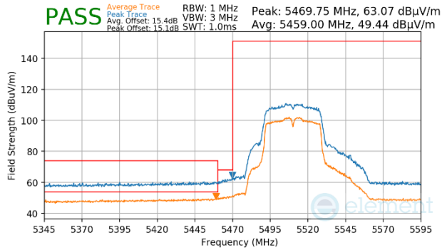
Plot 7-1706. CDD Primary (Peak & Average, Ch.102, 802.11n, MCS10)
