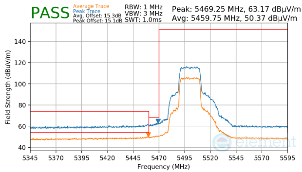
Plot 7-1676. CDD Primary (Peak & Average, Ch.100, 802.11ax(SU), MCS2)
