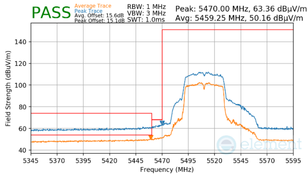
Plot 7-1707. CDD Primary (Peak & Average, Ch.102, 802.11n, MCS12)
