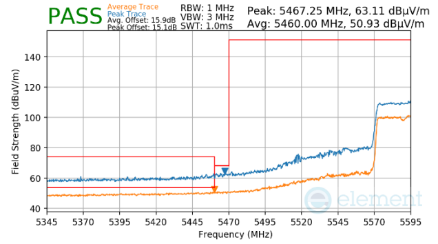
Plot 7-1768. (FCC Only) CDD Primary (Peak & Average, Ch.122, 802.11ac, MCS2)
