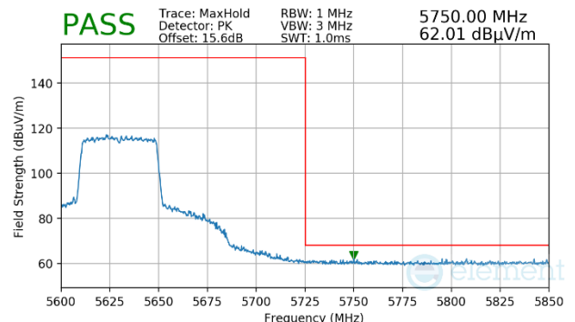
Plot 7-1747. (FCC Only) CDD Primary (Peak, Ch.126, 802.11ax(SU), MCS2)
