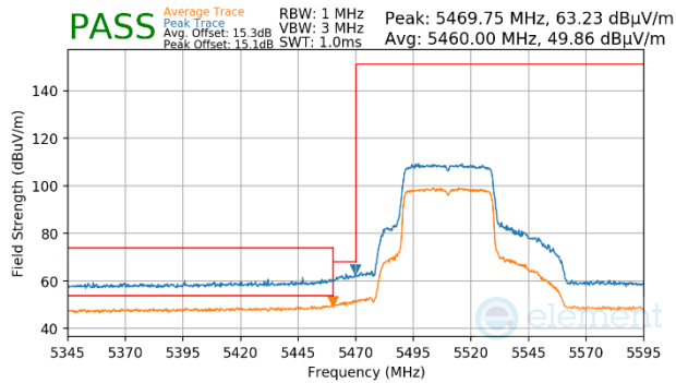
Plot 7-1551. Antenna WF7 (Peak & Average, Ch.102, 802.11ax(SU), MCS2)
