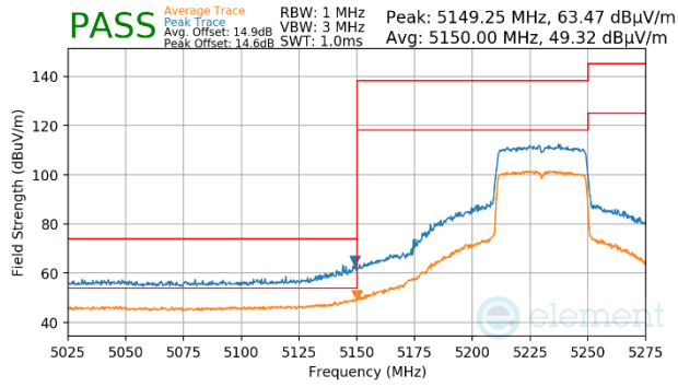
Plot 7-1543. Antenna WF7 (Peak & Average, Ch.46, 802.11ax(SU), MCS4)
