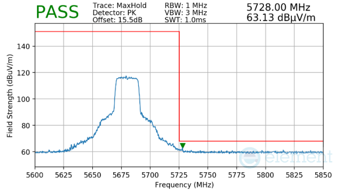
Plot 7-1497. Antenna WF7 (Peak, Ch.136, 802.11ax(SU), MCS11)
