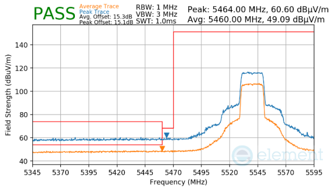
Plot 7-1490. Antenna WF7 (Peak & Average, Ch.108, 802.11ax(SU), MCS2)
