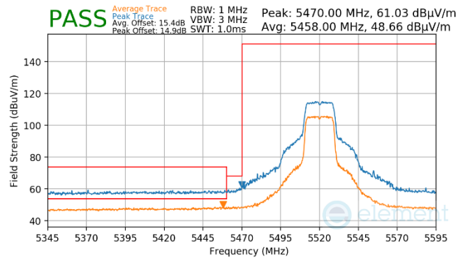
Plot 7-1457. Antenna WF7 (Peak & Average, Ch.104, 802.11n, MCS7)
