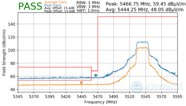
Plot 7-1458. Antenna WF7 (Peak & Average, Ch.108, 802.11n, MCS7)
