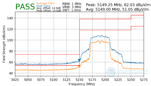
Plot 7-1508. Antenna WF7 (Peak & Average, Ch.38, 802.11n, MCS4)
