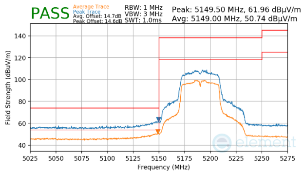
Plot 7-1507. Antenna WF7 (Peak & Average, Ch.38, 802.11n, MCS2)
