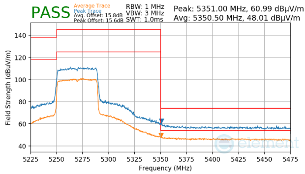
Plot 7-1545. Antenna WF7 (Peak & Average, Ch.54, 802.11ax(SU), MCS2)
