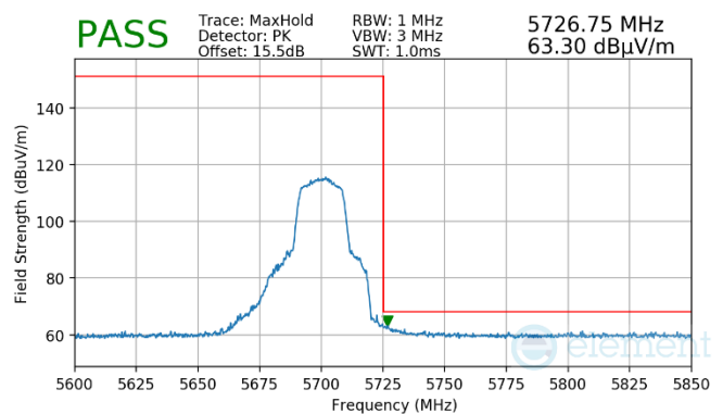
Plot 7-1463. Antenna WF7 (Peak, Ch.140, 802.11n, MCS2)
