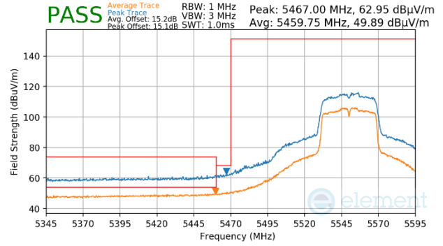
Plot 7-1522. Antenna WF7 (Peak & Average, Ch.110, 802.11n, MCS2)
