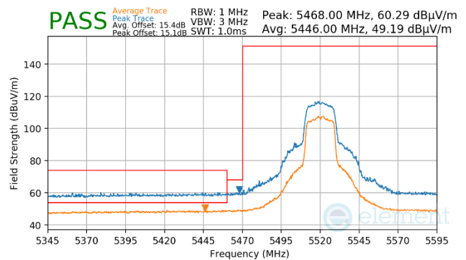
Plot 7-1456. Antenna WF7 (Peak & Average, Ch.104, 802.11n, MCS4)
