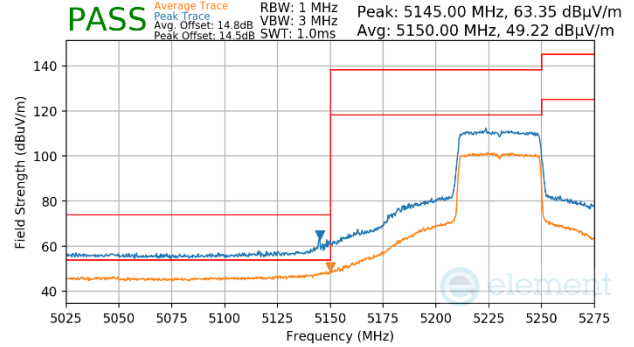
Plot 7-1542. Antenna WF7 (Peak & Average, Ch.46, 802.11ax(SU), MCS2)
