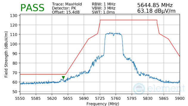
Plot 7-1535. Antenna WF7 (Peak, Ch.151, 802.11n, MCS7)
