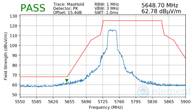
Plot 7-1468. Antenna WF7 (Peak, Ch.149, 802.11n, MCS7)
