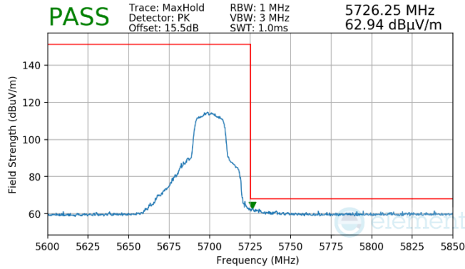
Plot 7-1464. Antenna WF7 (Peak, Ch.140, 802.11n, MCS4)
