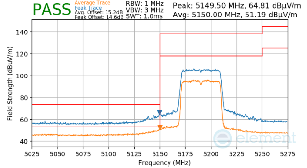
Plot 7-1541. Antenna WF7 (Peak & Average, Ch.38, 802.11ax(SU), MCS11)
