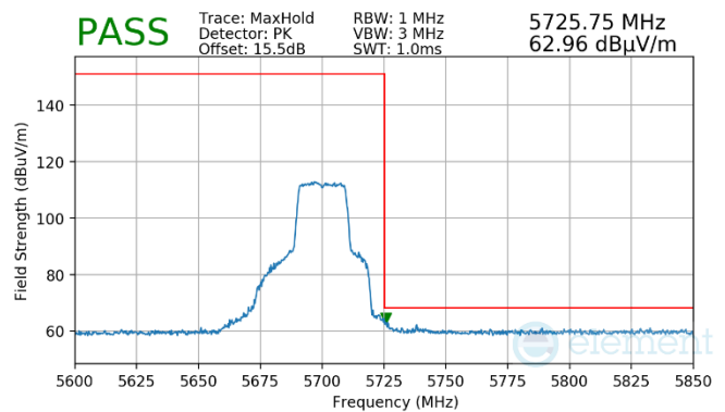
Plot 7-1498. Antenna WF7 (Peak, Ch.140, 802.11ax(SU), MCS2)
