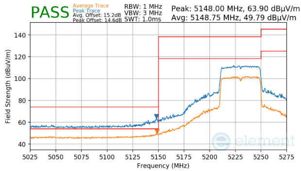
Plot 7-1544. Antenna WF7 (Peak & Average, Ch.46, 802.11ax(SU), MCS11)
