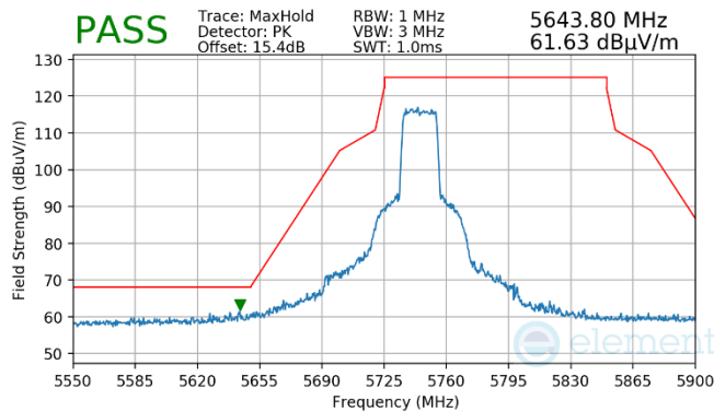
Plot 7-1502. Antenna WF7 (Peak, Ch.149, 802.11ax(SU), MCS4)
