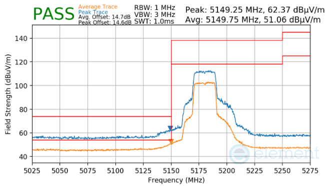
Plot 7-1472. Antenna WF7 (Peak & Average, Ch.36, 802.11ax(SU), MCS2)
