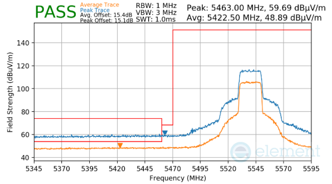
Plot 7-1491. Antenna WF7 (Peak & Average, Ch.108, 802.11ax(SU), MCS4)
