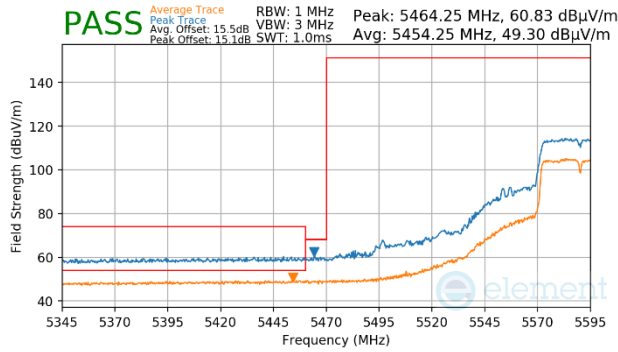
Plot 7-1526. (FCC Only) Antenna WF7 (Peak & Average, Ch.118, 802.11n, MCS7)
