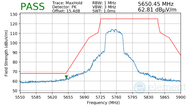
Plot 7-1534. Antenna WF7 (Peak, Ch.151, 802.11n, MCS4)
