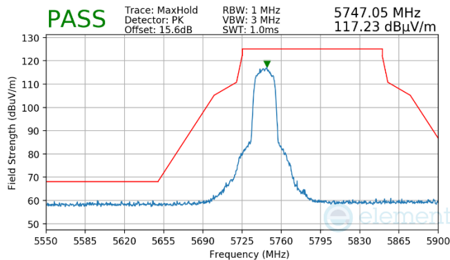
Plot 7-1466. Antenna WF7 (Peak, Ch.149, 802.11n, MCS2)
