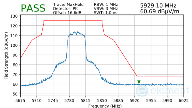
Plot 7-1536. Antenna WF7 (Peak, Ch.159, 802.11n, MCS2)
