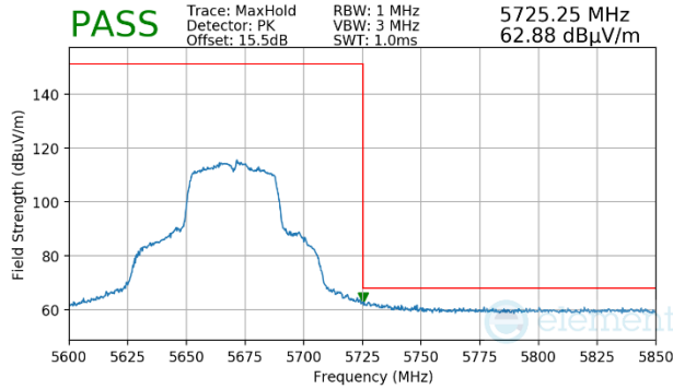
Plot 7-1531. Antenna WF7 (Peak, Ch.134, 802.11n, MCS4)
