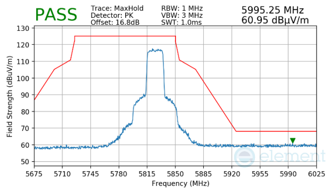
Plot 7-1504. Antenna WF7 (Peak, Ch.165, 802.11ax(SU), MCS2)
