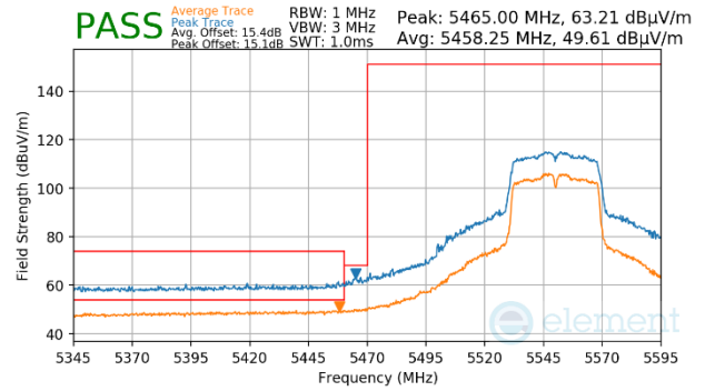
Plot 7-1523. Antenna WF7 (Peak & Average, Ch.110, 802.11n, MCS4)
