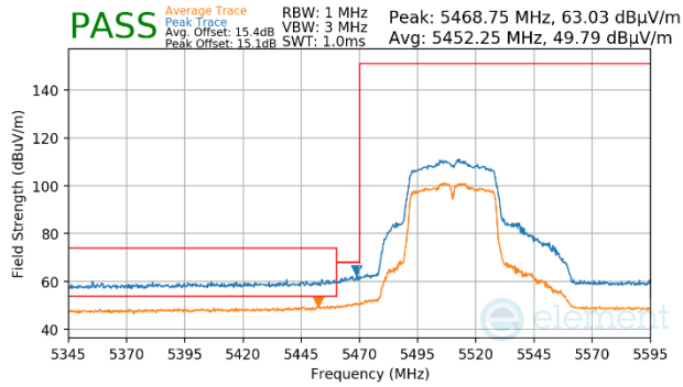
Plot 7-1520. Antenna WF7 (Peak & Average, Ch.102, 802.11n, MCS4)
