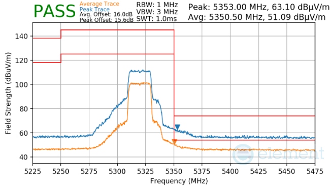
Plot 7-1482. Antenna WF7 (Peak & Average, Ch.64, 802.11ax(SU), MCS4)
