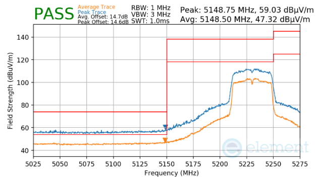
Plot 7-1510. Antenna WF7 (Peak & Average, Ch.46, 802.11n, MCS2)
