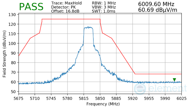
Plot 7-1506. Antenna WF7 (Peak, Ch.165, 802.11ax(SU), MCS11)
