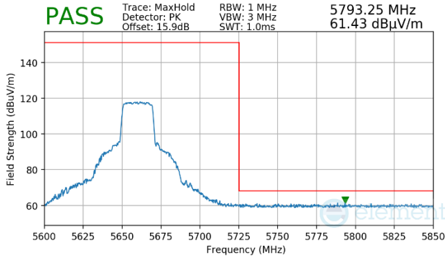
Plot 7-1494. Antenna WF7 (Peak, Ch.132, 802.11ax(SU), MCS11)
