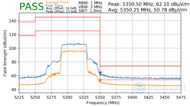
Plot 7-1549. Antenna WF7 (Peak & Average, Ch.62, 802.11ax(SU), MCS4)
