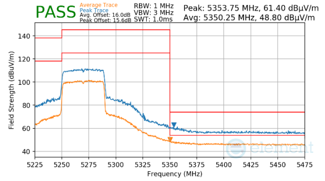
Plot 7-1546. Antenna WF7 (Peak & Average, Ch.54, 802.11ax(SU), MCS4)
