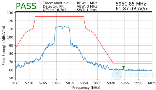
Plot 7-1538. Antenna WF7 (Peak, Ch.159, 802.11n, MCS4)
