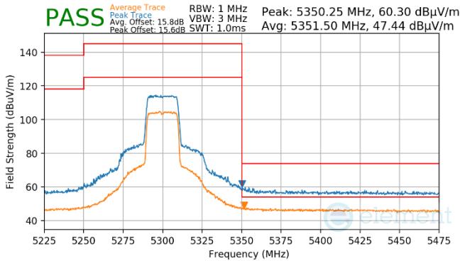
Plot 7-1478. Antenna WF7 (Peak & Average, Ch.60, 802.11ax(SU), MCS2)
