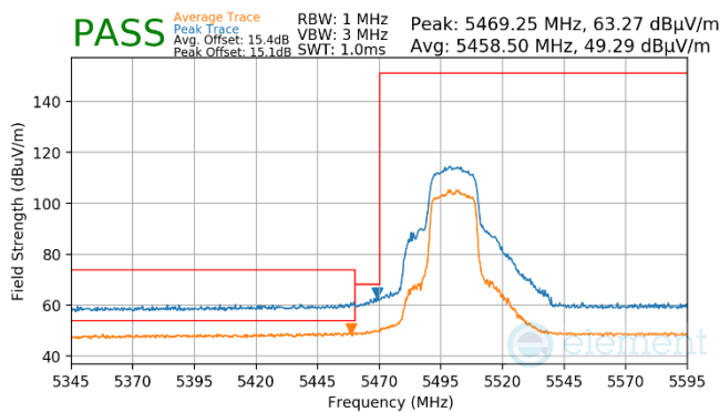
Plot 7-1453. Antenna WF7 (Peak & Average, Ch.100, 802.11n, MCS4)
