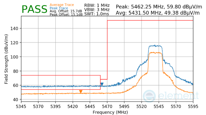
Plot 7-1492. Antenna WF7 (Peak & Average, Ch.108, 802.11ax(SU), MCS11)
