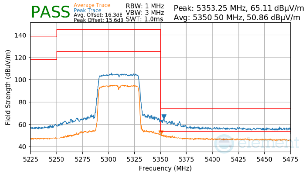
Plot 7-1550. Antenna WF7 (Peak & Average, Ch.62, 802.11ax(SU), MCS11)
