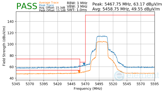
Plot 7-1484. Antenna WF7 (Peak & Average, Ch.100, 802.11ax(SU), MCS2)
