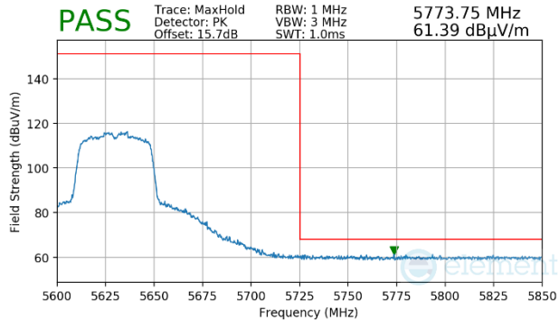
Plot 7-1527. (FCC Only) Antenna WF7 (Peak, Ch.126, 802.11n, MCS2)
