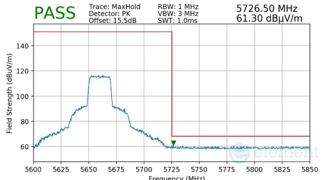
Plot 7-1493. Antenna WF7 (Peak, Ch.132, 802.11ax(SU), MCS4)
