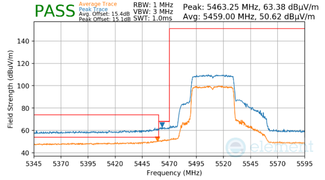
Plot 7-1552. Antenna WF7 (Peak & Average, Ch.102, 802.11ax(SU), MCS4)
