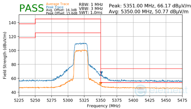
Plot 7-1483. Antenna WF7 (Peak & Average, Ch.64, 802.11ax(SU), MCS11)
