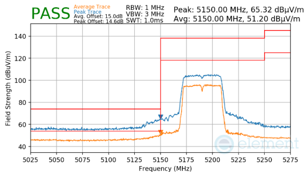
Plot 7-1509. Antenna WF7 (Peak & Average, Ch.38, 802.11n, MCS7)
