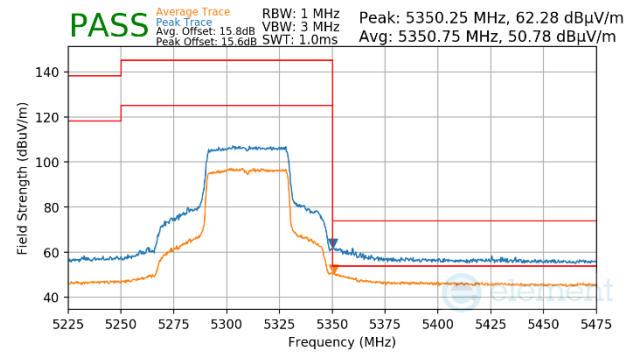
Plot 7-1548. Antenna WF7 (Peak & Average, Ch.62, 802.11ax(SU), MCS2)
