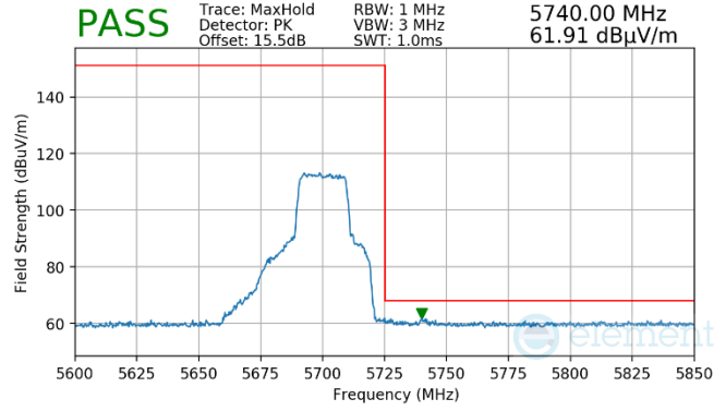
Plot 7-1499. Antenna WF7 (Peak, Ch.140, 802.11ax(SU), MCS4)
