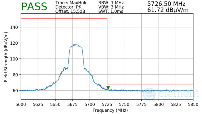
Plot 7-1461. Antenna WF7 (Peak, Ch.136, 802.11n, MCS4)
