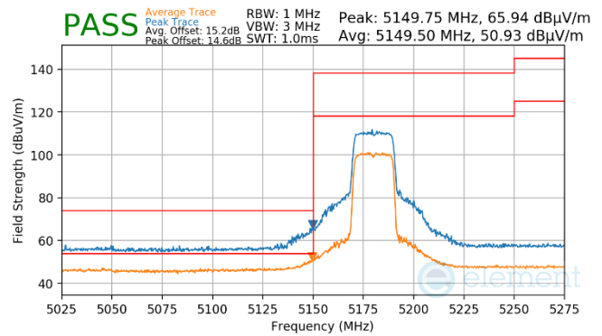
Plot 7-1474. Antenna WF7 (Peak & Average, Ch.36, 802.11ax(SU), MCS11)
