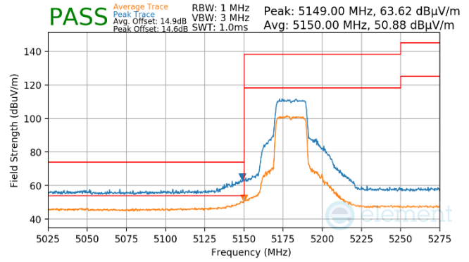
Plot 7-1473. Antenna WF7 (Peak & Average, Ch.36, 802.11ax(SU), MCS4)
