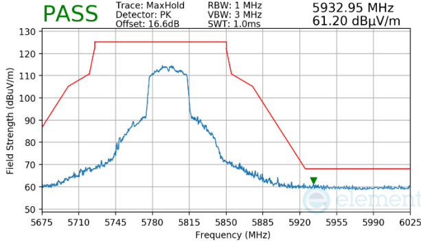
Plot 7-1537. Antenna WF7 (Peak, Ch.159, 802.11n, MCS4)
