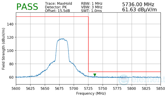
Plot 7-1460. Antenna WF7 (Peak, Ch.136, 802.11n, MCS2)
