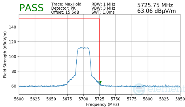
Plot 7-1465. Antenna WF7 (Peak, Ch.140, 802.11n, MCS7)
