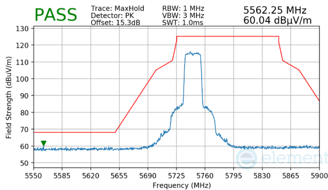
Plot 7-1501. Antenna WF7 (Peak, Ch.149, 802.11ax(SU), MCS2)
