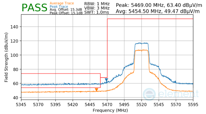
Plot 7-1487. Antenna WF7 (Peak & Average, Ch.104, 802.11ax(SU), MCS2)
