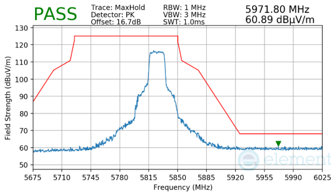
Plot 7-1471. Antenna WF7 (Peak, Ch.165, 802.11n, MCS7)
