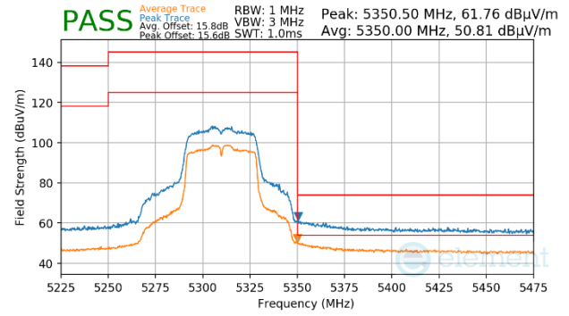
Plot 7-1516. Antenna WF7 (Peak & Average, Ch.62, 802.11n, MCS2)
