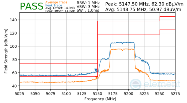
Plot 7-1540. Antenna WF7 (Peak & Average, Ch.38, 802.11ax(SU), MCS4)
