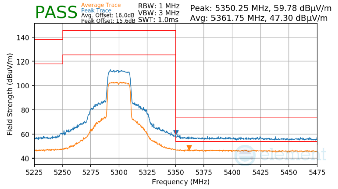
Plot 7-1479. Antenna WF7 (Peak & Average, Ch.60, 802.11ax(SU), MCS4)
