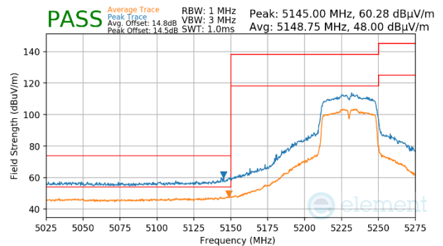
Plot 7-1511. Antenna WF7 (Peak & Average, Ch.46, 802.11n, MCS4)
