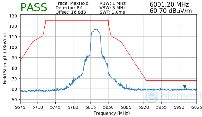
Plot 7-1470. Antenna WF7 (Peak, Ch.165, 802.11n, MCS4)
