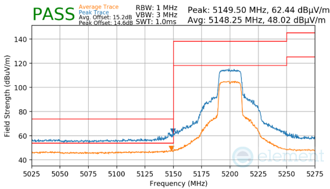
Plot 7-1477. Antenna WF7 (Peak & Average, Ch.40, 802.11ax(SU), MCS11)
