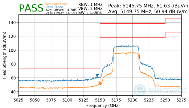
Plot 7-1539. Antenna WF7 (Peak & Average, Ch.38, 802.11ax(SU), MCS2)
