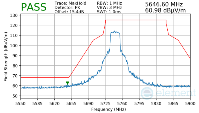
Plot 7-1503. Antenna WF7 (Peak, Ch.149, 802.11ax(SU), MCS11)
