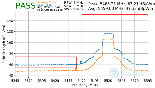
Plot 7-1488. Antenna WF7 (Peak & Average, Ch.104, 802.11ax(SU), MCS4)
