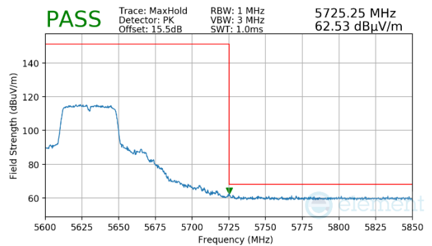
Plot 7-1529. (FCC Only) Antenna WF7 (Peak, Ch.126, 802.11n, MCS7)
