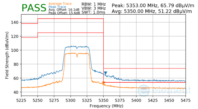
Plot 7-1518. Antenna WF7 (Peak & Average, Ch.62, 802.11n, MCS7)
