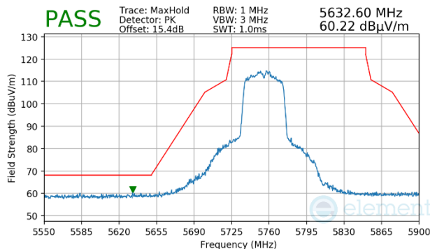
Plot 7-1533. Antenna WF7 (Peak, Ch.151, 802.11n, MCS2)
