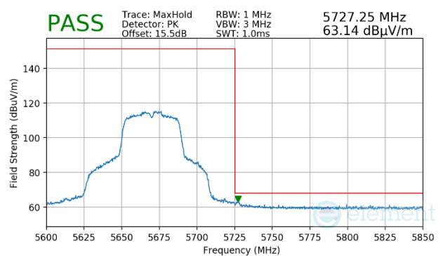
Plot 7-1530. Antenna WF7 (Peak, Ch.134, 802.11n, MCS2)
