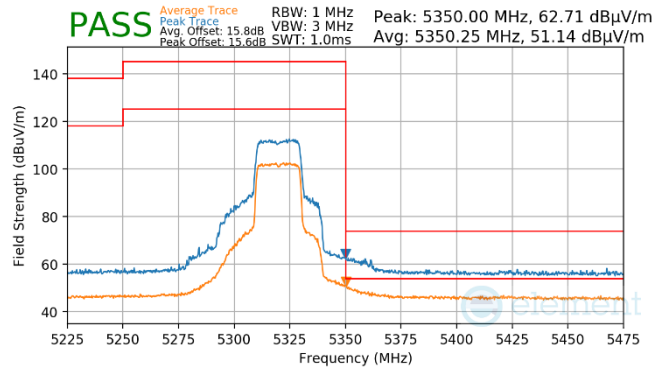
Plot 7-1481. Antenna WF7 (Peak & Average, Ch.64, 802.11ax(SU), MCS2)
