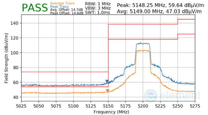
Plot 7-1475. Antenna WF7 (Peak & Average, Ch.40, 802.11ax(SU), MCS2)
