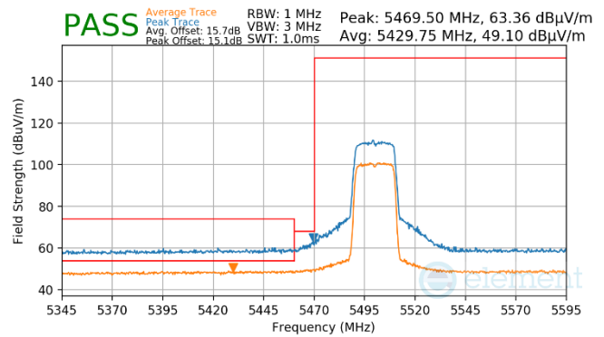
Plot 7-1486. Antenna WF7 (Peak & Average, Ch.100, 802.11ax(SU), MCS11)
