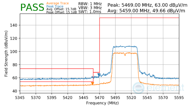
Plot 7-1553. Antenna WF7 (Peak & Average, Ch.102, 802.11ax(SU), MCS11)
