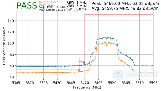
Plot 7-1519. Antenna WF7 (Peak & Average, Ch.102, 802.11n, MCS2)
