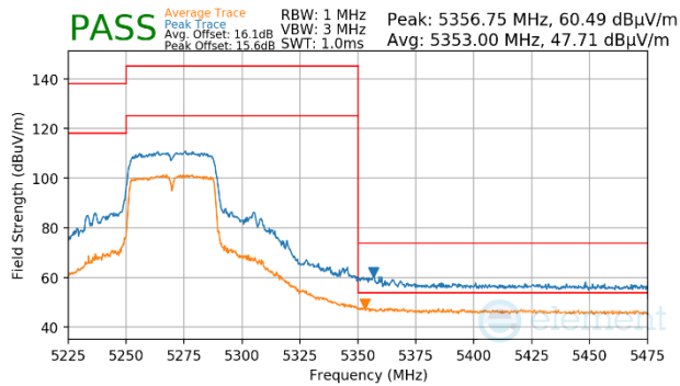
Plot 7-1515. Antenna WF7 (Peak & Average, Ch.54, 802.11n, MCS7)
