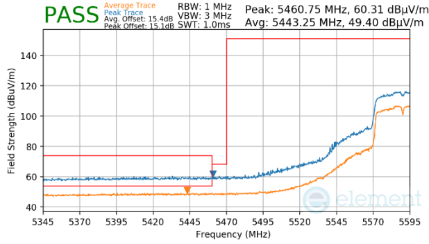
Plot 7-1525. (FCC Only) Antenna WF7 (Peak & Average, Ch.118, 802.11n, MCS4)
