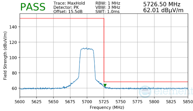
Plot 7-1500. Antenna WF7 (Peak, Ch.140, 802.11ax(SU), MCS11)
