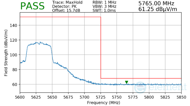
Plot 7-1528. (FCC Only) Antenna WF7 (Peak, Ch.126, 802.11n, MCS4)
