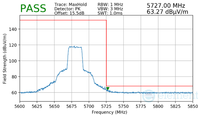
Plot 7-1496. Antenna WF7 (Peak, Ch.136, 802.11ax(SU), MCS4)
