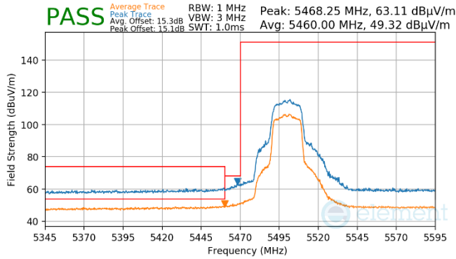
Plot 7-1452. Antenna WF7 (Peak & Average, Ch.100, 802.11n, MCS2)
