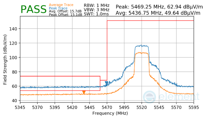
Plot 7-1489. Antenna WF7 (Peak & Average, Ch.104, 802.11ax(SU), MCS11)
