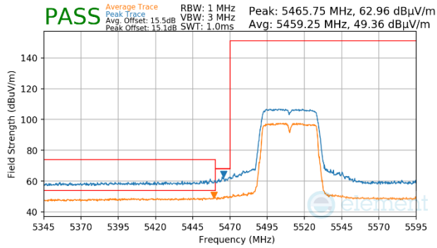
Plot 7-1521. Antenna WF7 (Peak & Average, Ch.102, 802.11n, MCS7)
