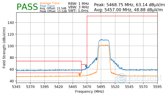
Plot 7-1454. Antenna WF7 (Peak & Average, Ch.100, 802.11n, MCS7)
