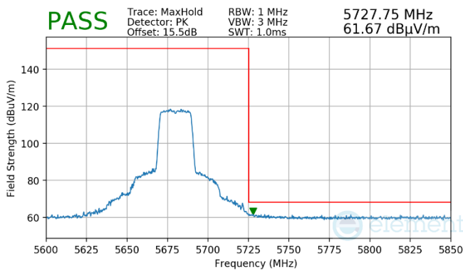
Plot 7-1495. Antenna WF7 (Peak, Ch.136, 802.11ax(SU), MCS2)
