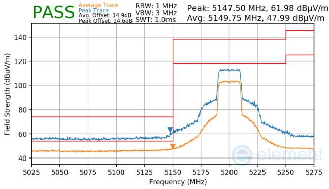
Plot 7-1476. Antenna WF7 (Peak & Average, Ch.40, 802.11ax(SU), MCS4)
