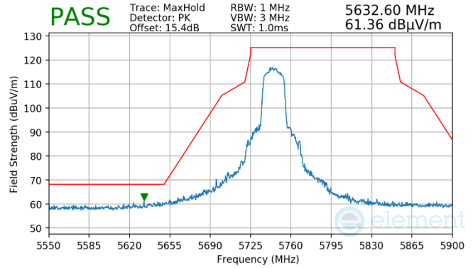
Plot 7-1467. Antenna WF7 (Peak, Ch.149, 802.11n, MCS4)
