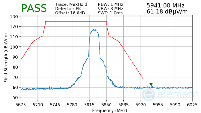
Plot 7-1469. Antenna WF7 (Peak, Ch.165, 802.11n, MCS2)
