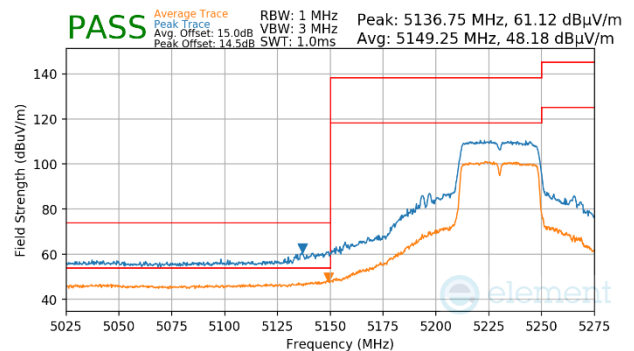
Plot 7-1512. Antenna WF7 (Peak & Average, Ch.46, 802.11n, MCS7)
