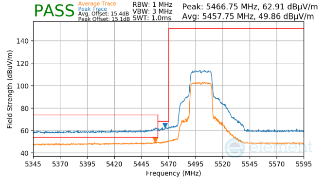
Plot 7-1485. Antenna WF7 (Peak & Average, Ch.100, 802.11ax(SU), MCS4)
