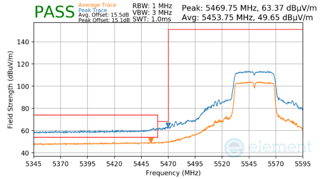
Plot 7-1524. Antenna WF7 (Peak & Average, Ch.110, 802.11n, MCS7)
