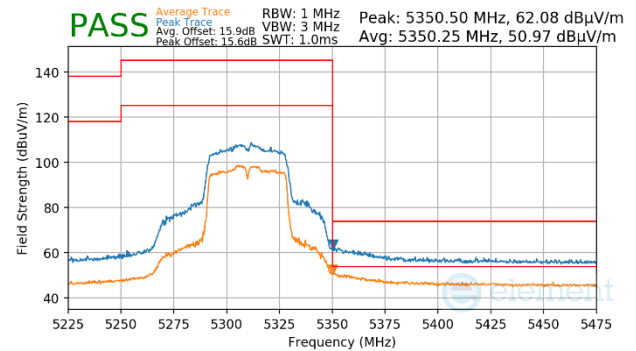
Plot 7-1517. Antenna WF7 (Peak & Average, Ch.62, 802.11n, MCS4)
