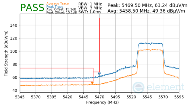
Plot 7-1554. Antenna WF7 (Peak & Average, Ch.110, 802.11ax(SU), MCS2)
