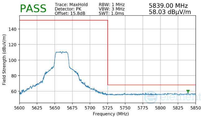
Plot 7-1459. Antenna WF7 (Peak, Ch.132, 802.11n, MCS7)
