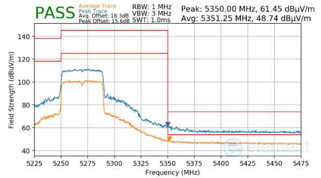
Plot 7-1547. Antenna WF7 (Peak & Average, Ch.54, 802.11ax(SU), MCS11)
