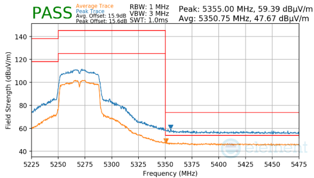
Plot 7-1514. Antenna WF7 (Peak & Average, Ch.54, 802.11n, MCS4)
