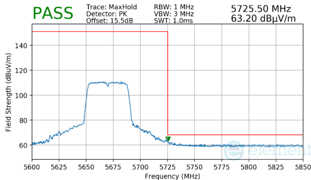
Plot 7-1532. Antenna WF7 (Peak, Ch.134, 802.11n, MCS7)
