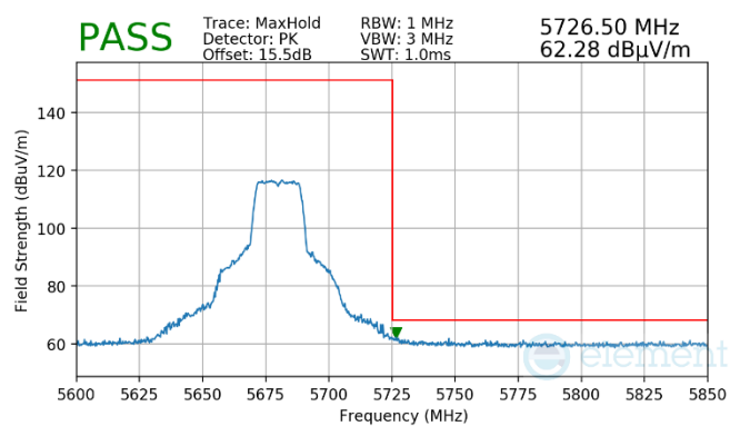
Plot 7-1462. Antenna WF7 (Peak, Ch.136, 802.11n, MCS7)
