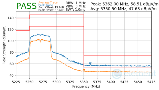
Plot 7-1513. Antenna WF7 (Peak & Average, Ch.54, 802.11n, MCS2)
