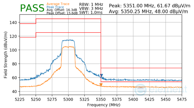
Plot 7-1480. Antenna WF7 (Peak & Average, Ch.60, 802.11ax(SU), MCS11)
