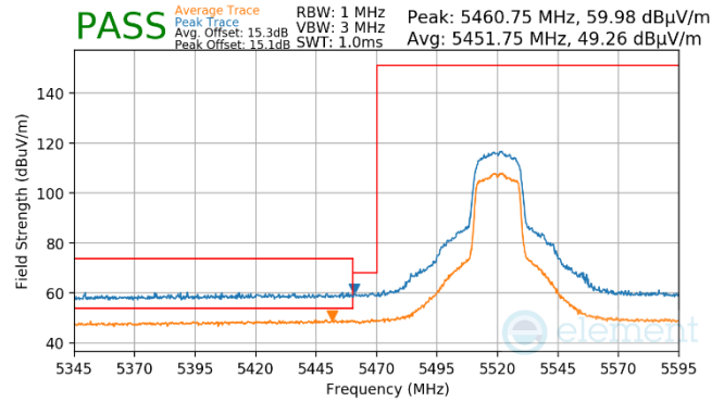
Plot 7-1455. Antenna WF7 (Peak & Average, Ch.104, 802.11n, MCS2)
