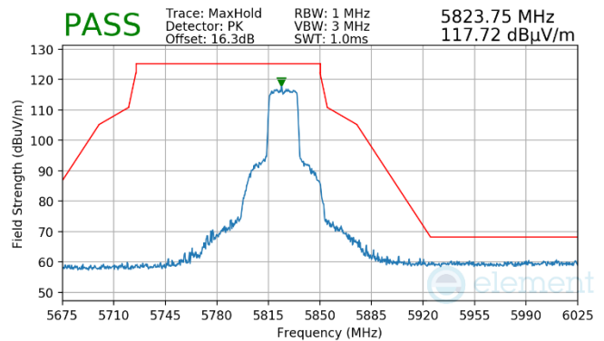
Plot 7-1505. Antenna WF7 (Peak, Ch.165, 802.11ax(SU), MCS4)
