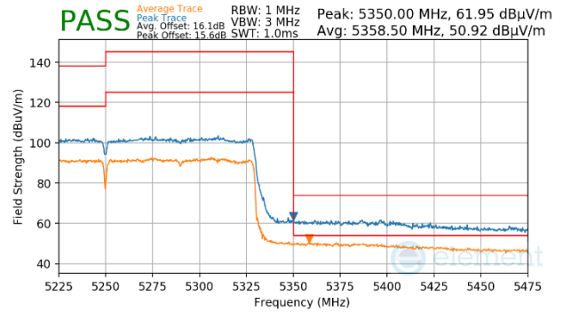
Plot 7-1234. Antenna WF5b (Peak & Average, Ch.50, 802.11ax(SU), MCS4)
