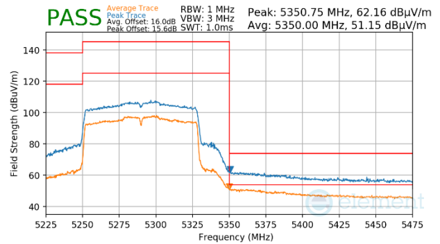
Plot 7-1180. Antenna WF5b (Peak & Average, Ch.58, 802.11ac, MCS4)
