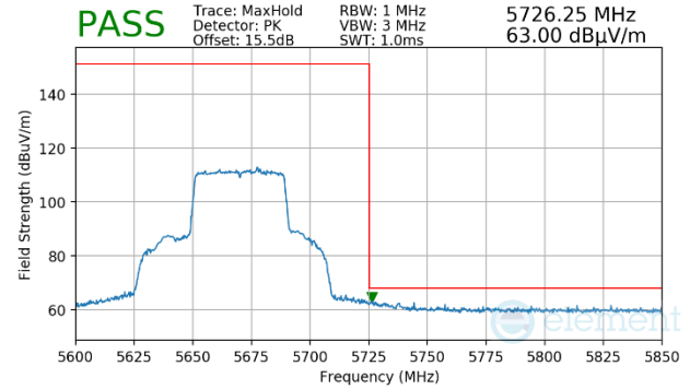
Plot 7-1168. Antenna WF5b (Peak, Ch.134, 802.11ax(SU), MCS4)
