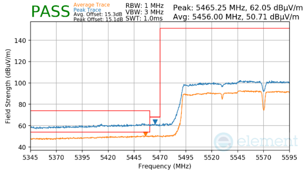
Plot 7-1224. (FCC Only) Antenna WF5b (Peak & Average, Ch.114, 802.11ac, MCS2)
