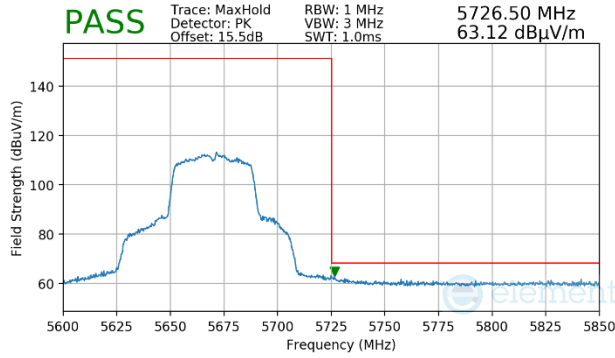
Plot 7-1135. Antenna WF5b (Peak, Ch.134, 802.11n, MCS4)
