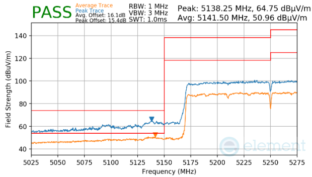
Plot 7-1232. Antenna WF5b (Peak & Average, Ch.50, 802.11ax(SU), MCS11)
