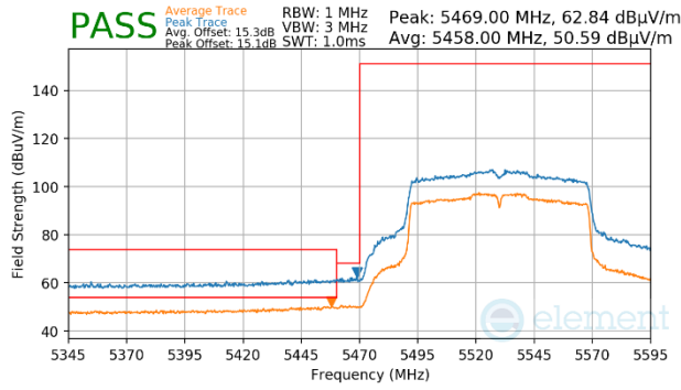
Plot 7-1182. Antenna WF5b (Peak & Average, Ch.106, 802.11ac, MCS2)
