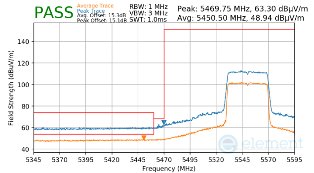
Plot 7-1158. Antenna WF5b (Peak & Average, Ch.110, 802.11ax(SU), MCS2)
