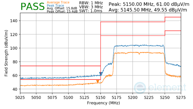
Plot 7-1198. Antenna WF5b (Peak & Average, Ch.42, 802.11ax(SU), MCS4)
