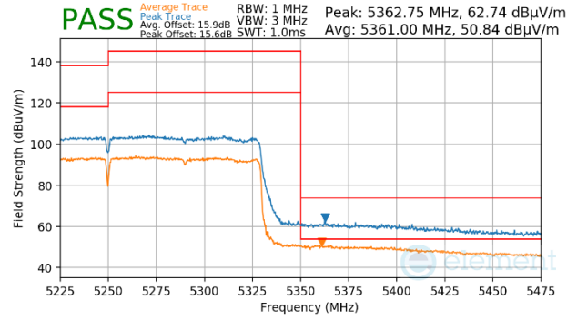
Plot 7-1233. Antenna WF5b (Peak & Average, Ch.50, 802.11ax(SU), MCS2)
