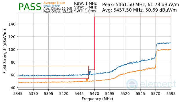
Plot 7-1207. (FCC Only) Antenna WF5b (Peak & Average, Ch122, 802.11ax(SU), MCS4)
