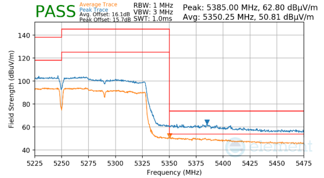
Plot 7-1222. Antenna WF5b (Peak & Average, Ch.50, 802.11ac, MCS4)
