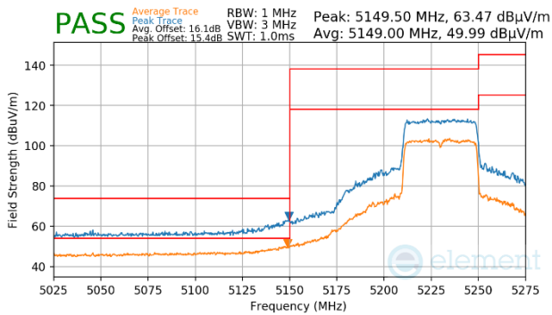
Plot 7-1148. Antenna WF5b (Peak & Average, Ch.46, 802.11ax(SU), MCS11)
