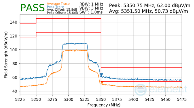
Plot 7-1152. Antenna WF5b (Peak & Average, Ch.62, 802.11ax(SU), MCS2)
