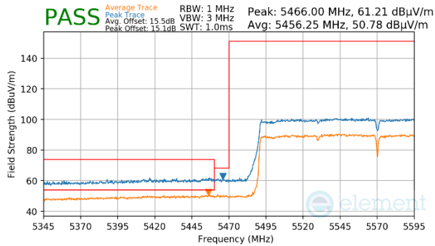
Plot 7-1237. (FCC Only) Antenna WF5b (Peak & Average, Ch.114, 802.11ax(SU), MCS4)
