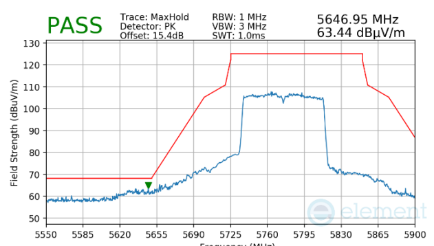
Plot 7-1193. Antenna WF5b (Peak, Ch.155, 802.11ac, MCS9)
