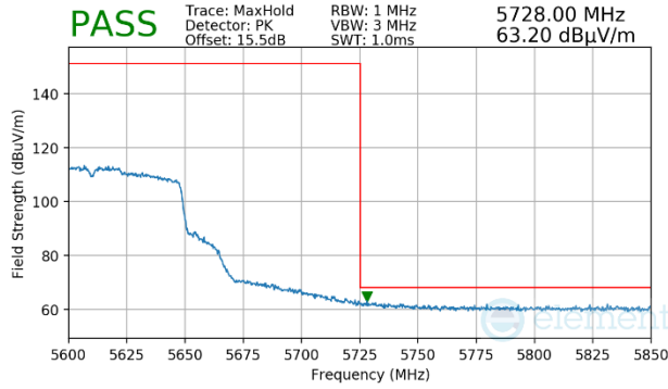
Plot 7-1188. (FCC Only) Antenna WF5b (Peak, Ch.122, 802.11ac, MCS2)
