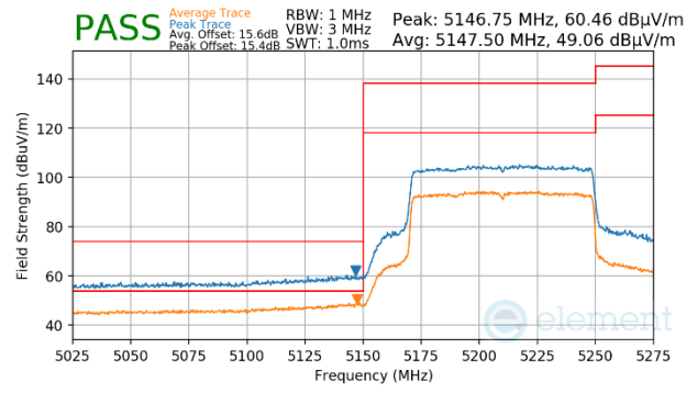
Plot 7-1197. Antenna WF5b (Peak & Average, Ch.42, 802.11ax(SU), MCS2)
