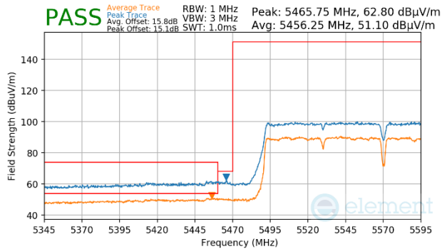
Plot 7-1226. (FCC Only) Antenna WF5b (Peak & Average, Ch.114, 802.11ac, MCS9)
