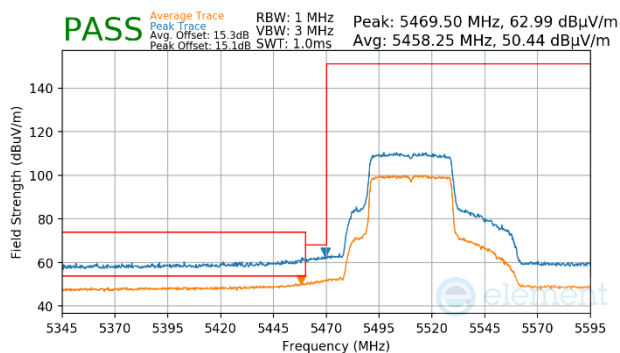
Plot 7-1155. Antenna WF5b (Peak & Average, Ch.102, 802.11ax(SU), MCS2)
