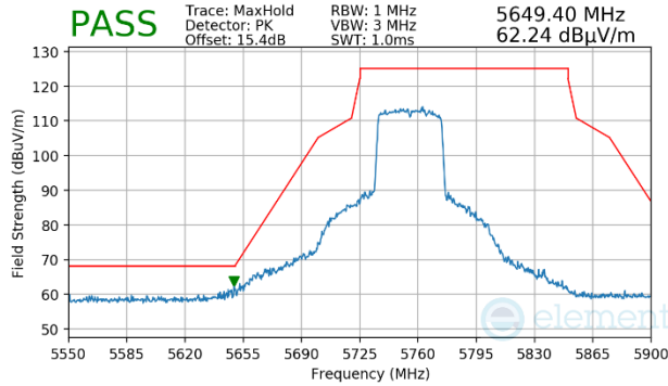
Plot 7-1171. Antenna WF5b (Peak, Ch.151, 802.11ax(SU), MCS4)
