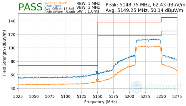
Plot 7-1147. Antenna WF5b (Peak & Average, Ch.46, 802.11ax(SU), MCS4)
