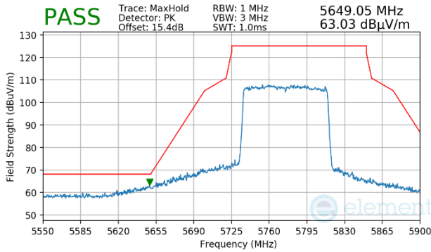
Plot 7-1213. Antenna WF5b (Peak, Ch155, 802.11ax(SU), MCS4)
