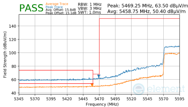
Plot 7-1208. (FCC Only) Antenna WF5b (Peak & Average, Ch122, 802.11ax(SU), MCS11)
