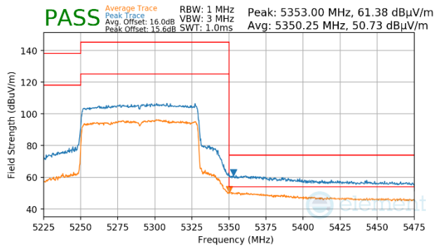
Plot 7-1201. Antenna WF5b (Peak & Average, Ch58, 802.11ax(SU), MCS4)
