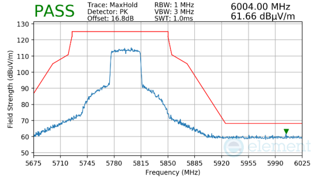
Plot 7-1174. Antenna WF5b (Peak, Ch.159, 802.11ax(SU), MCS4)
