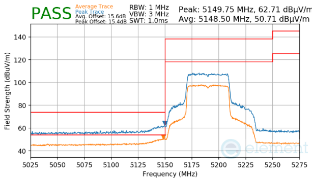
Plot 7-1143. Antenna WF5b (Peak & Average, Ch.38, 802.11ax(SU), MCS2)
