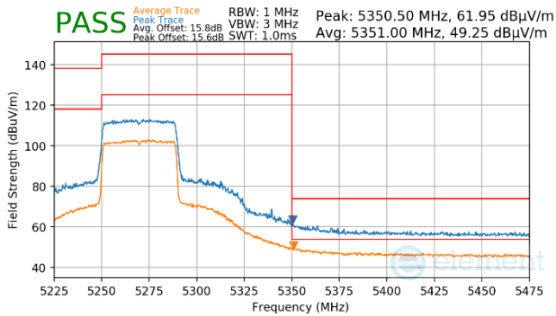
Plot 7-1149. Antenna WF5b (Peak & Average, Ch.54, 802.11ax(SU), MCS2)
