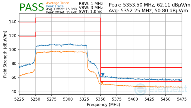
Plot 7-1200. Antenna WF5b (Peak & Average, Ch58, 802.11ax(SU), MCS2)
