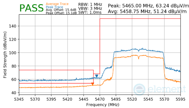
Plot 7-1183. Antenna WF5b (Peak & Average, Ch.106, 802.11ac, MCS4)
