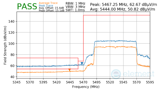
Plot 7-1204. Antenna WF5b (Peak & Average, Ch106, 802.11ax(SU), MCS4)
