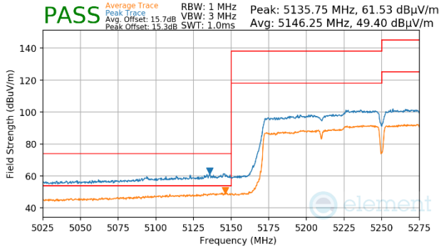
Plot 7-1218. Antenna WF5b (Peak & Average, Ch.50, 802.11ac, MCS2)
