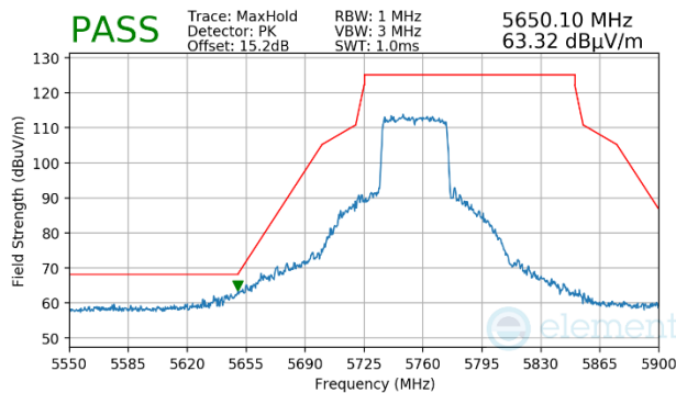
Plot 7-1172. Antenna WF5b (Peak, Ch.151, 802.11ax(SU), MCS11)
