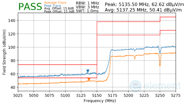
Plot 7-1219. Antenna WF5b (Peak & Average, Ch.50, 802.11ac, MCS4)
