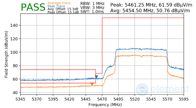
Plot 7-1203. Antenna WF5b (Peak & Average, Ch106, 802.11ax(SU), MCS2)
