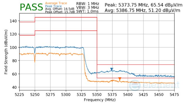
Plot 7-1235. Antenna WF5b (Peak & Average, Ch.50, 802.11ax(SU), MCS11)
