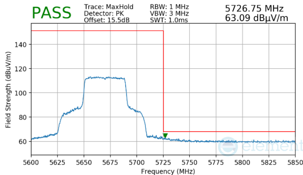
Plot 7-1167. Antenna WF5b (Peak, Ch.134, 802.11ax(SU), MCS2)
