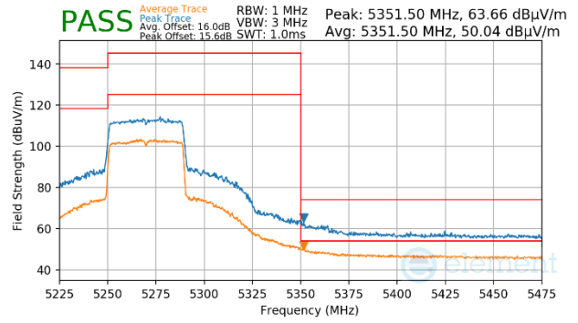
Plot 7-1150. Antenna WF5b (Peak & Average, Ch.54, 802.11ax(SU), MCS4)
