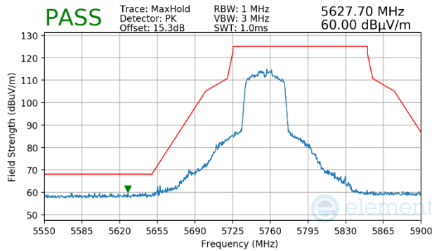
Plot 7-1137. Antenna WF5b (Peak, Ch.151, 802.11n, MCS2)
