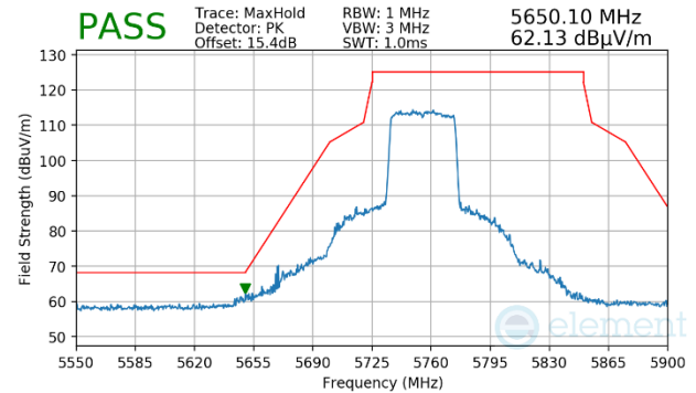
Plot 7-1170. Antenna WF5b (Peak, Ch.151, 802.11ax(SU), MCS2)
