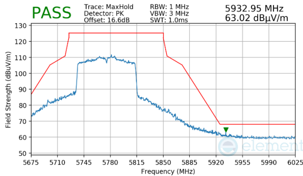
Plot 7-1195. Antenna WF5b (Peak, Ch.155, 802.11ac, MCS4)
