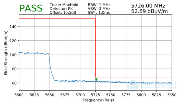
Plot 7-1240. (FCC Only) Antenna WF5b (Peak, Ch.114, 802.11ax(SU), MCS4)
