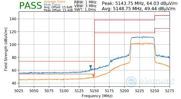
Plot 7-1146. Antenna WF5b (Peak & Average, Ch.46, 802.11ax(SU), MCS2)
