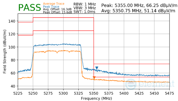
Plot 7-1202. Antenna WF5b (Peak & Average, Ch58, 802.11ax(SU), MCS11)
