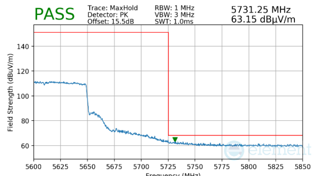
Plot 7-1210. (FCC Only) Antenna WF5b (Peak, Ch122, 802.11ax(SU), MCS4)
