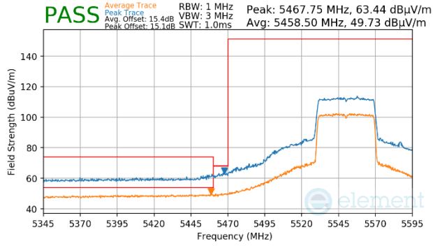
Plot 7-1159. Antenna WF5b (Peak & Average, Ch.110, 802.11ax(SU), MCS4)
