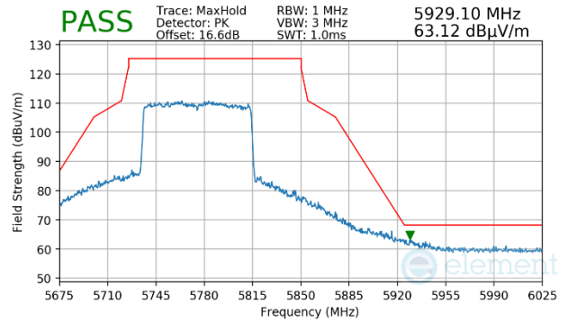
Plot 7-1216. Antenna WF5b (Peak, Ch155, 802.11ax(SU), MCS4)
