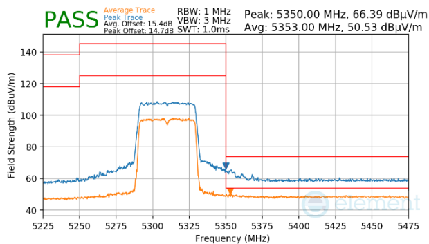
Plot 7-1154. Antenna WF5b (Peak & Average, Ch.62, 802.11ax(SU), MCS11)
