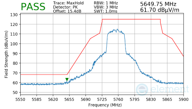
Plot 7-1138. Antenna WF5b (Peak, Ch.151, 802.11n, MCS4)
