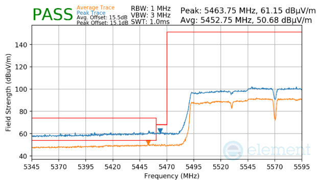
Plot 7-1225. (FCC Only) Antenna WF5b (Peak & Average, Ch.114, 802.11ac, MCS4)
