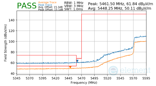
Plot 7-1185. (FCC Only) Antenna WF5b (Peak & Average, Ch.122, 802.11ac, MCS2)
