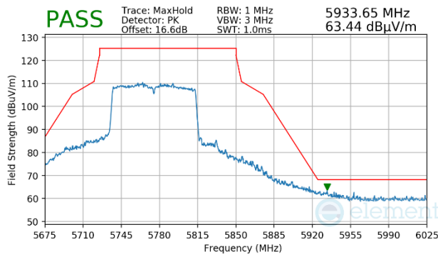
Plot 7-1196. Antenna WF5b (Peak, Ch.155, 802.11ac, MCS9)
