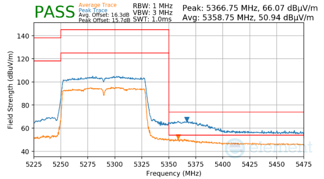
Plot 7-1181. Antenna WF5b (Peak & Average, Ch.58, 802.11ac, MCS9)
