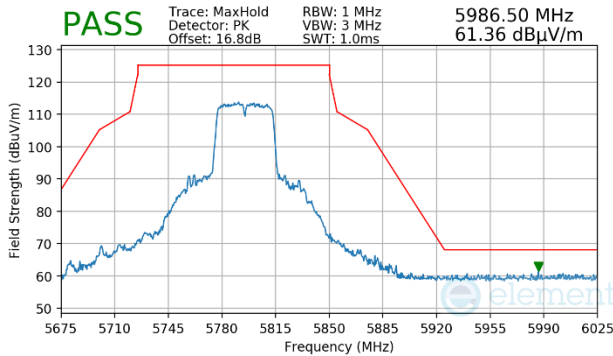
Plot 7-1142. Antenna WF5b (Peak, Ch.159, 802.11n, MCS4)
