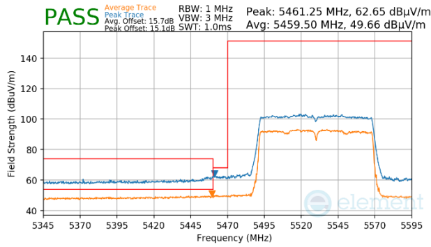
Plot 7-1184. Antenna WF5b (Peak & Average, Ch.106, 802.11ac, MCS9)
