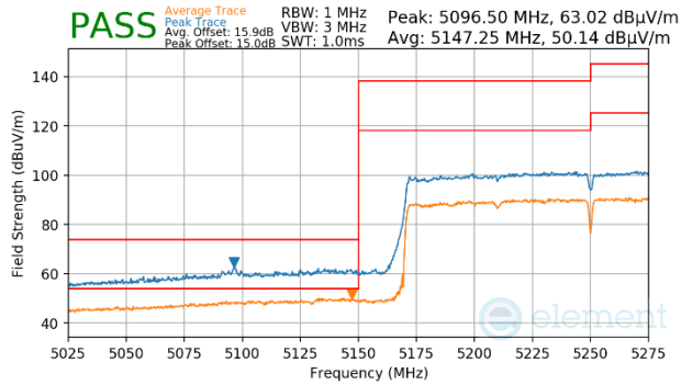
Plot 7-1231. Antenna WF5b (Peak & Average, Ch.50, 802.11ax(SU), MCS4)
