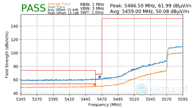
Plot 7-1186. (FCC Only) Antenna WF5b (Peak & Average, Ch.122, 802.11ac, MCS4)
