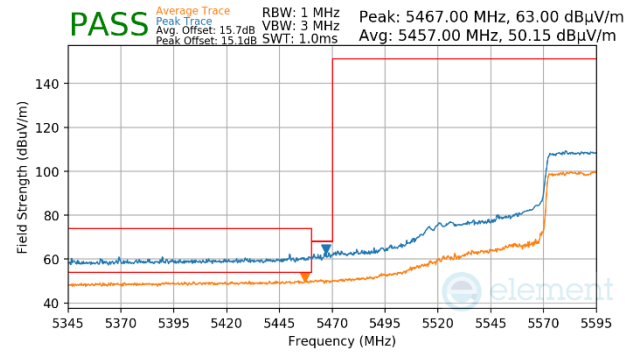
Plot 7-1187. (FCC Only) Antenna WF5b (Peak & Average, Ch.122, 802.11ac, MCS9)
