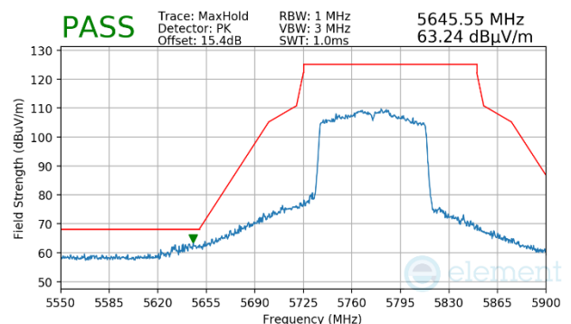
Plot 7-1192. Antenna WF5b (Peak, Ch.155, 802.11ac, MCS4)
