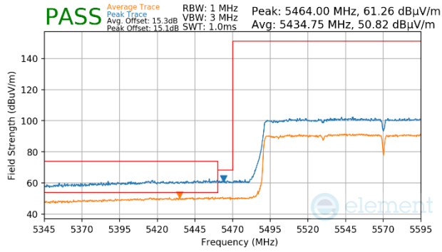
Plot 7-1236. (FCC Only) Antenna WF5b (Peak & Average, Ch.114, 802.11ax(SU), MCS2)
