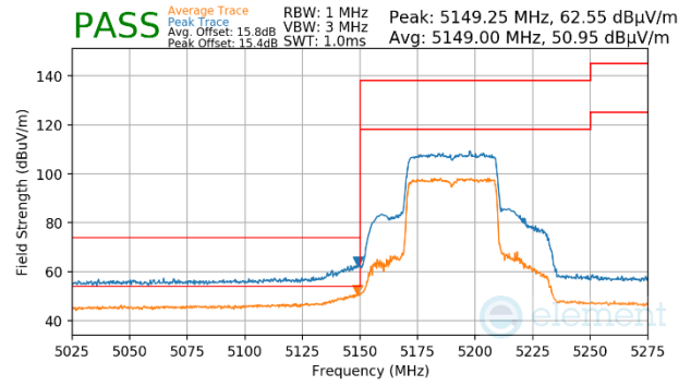
Plot 7-1144. Antenna WF5b (Peak & Average, Ch.38, 802.11ax(SU), MCS4)
