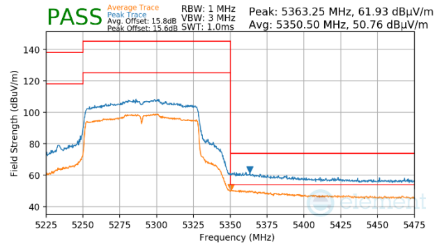
Plot 7-1179. Antenna WF5b (Peak & Average, Ch.58, 802.11ac, MCS2)
