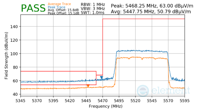
Plot 7-1205. Antenna WF5b (Peak & Average, Ch106, 802.11ax(SU), MCS11)
