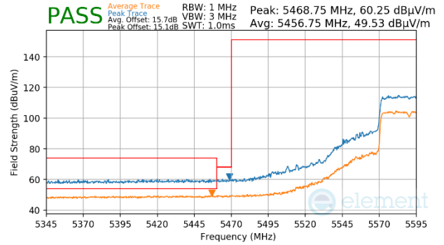
Plot 7-1163. (FCC Only) Antenna WF5b (Peak & Average, Ch.118, 802.11ax(SU), MCS11)
