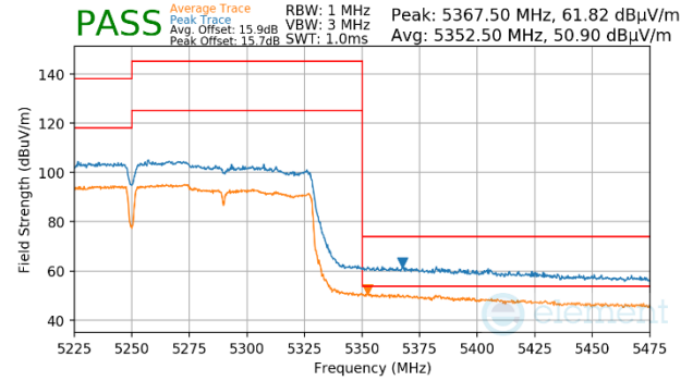
Plot 7-1221. Antenna WF5b (Peak & Average, Ch.50, 802.11ac, MCS2)
