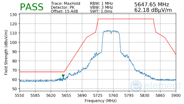
Plot 7-1139. Antenna WF5b (Peak, Ch.151, 802.11n, MCS7)
