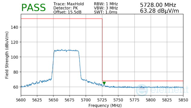
Plot 7-1169. Antenna WF5b (Peak, Ch.134, 802.11ax(SU), MCS11)
