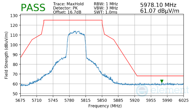
Plot 7-1140. Antenna WF5b (Peak, Ch.159, 802.11n, MCS2)
