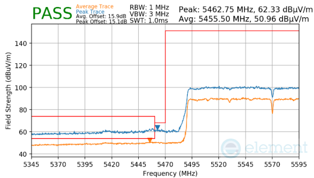
Plot 7-1238. (FCC Only) Antenna WF5b (Peak & Average, Ch.114, 802.11ax(SU), MCS11)
