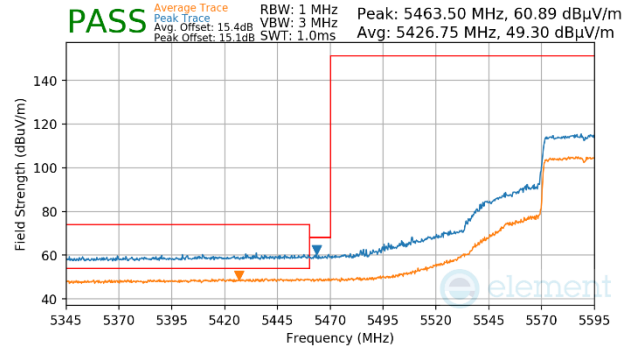
Plot 7-1162. (FCC Only) Antenna WF5b (Peak & Average, Ch.118, 802.11ax(SU), MCS4)
