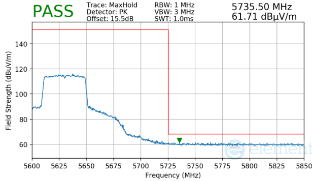
Plot 7-1165. (FCC Only) Antenna WF5b (Peak, Ch.126, 802.11ax(SU), MCS4)
