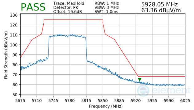
Plot 7-1217. Antenna WF5b (Peak, Ch155, 802.11ax(SU), MCS11)
