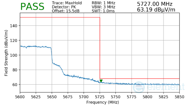
Plot 7-1209. (FCC Only) Antenna WF5b (Peak, Ch122, 802.11ax(SU), MCS2)
