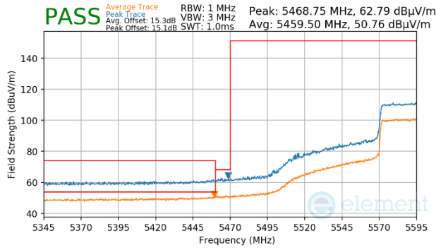
Plot 7-1206. (FCC Only) Antenna WF5b (Peak & Average, Ch122, 802.11ax(SU), MCS2)
