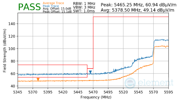
Plot 7-1161. (FCC Only) Antenna WF5b (Peak & Average, Ch.118, 802.11ax(SU), MCS2)
