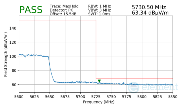
Plot 7-1229. (FCC Only) Antenna WF5b (Peak, Ch.114, 802.11ac, MCS9)
