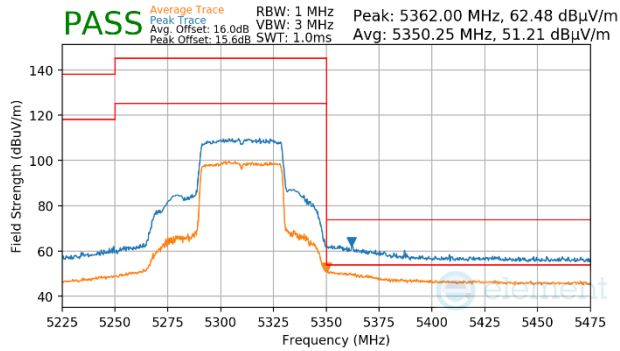
Plot 7-1153. Antenna WF5b (Peak & Average, Ch.62, 802.11ax(SU), MCS4)
