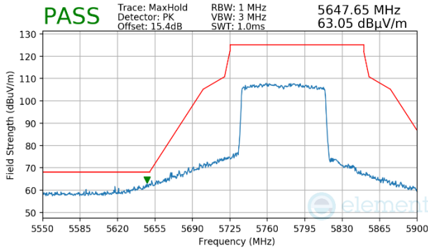
Plot 7-1214. Antenna WF5b (Peak, Ch155, 802.11ax(SU), MCS11)
