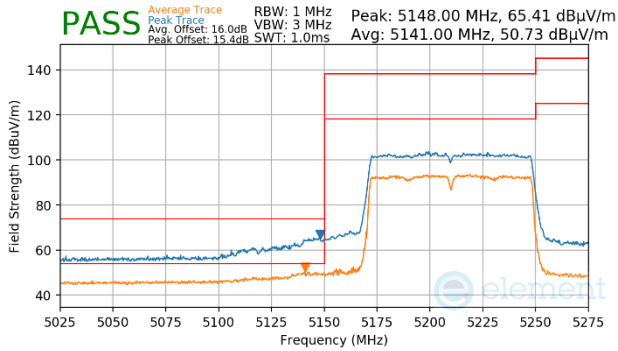
Plot 7-1178. Antenna WF5b (Peak & Average, Ch.42, 802.11ac, MCS9)
