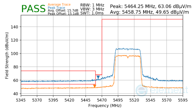
Plot 7-1157. Antenna WF5b (Peak & Average, Ch.102, 802.11ax(SU), MCS11)
