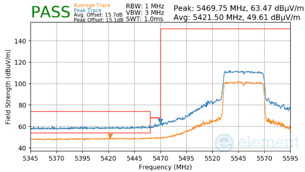
Plot 7-1160. Antenna WF5b (Peak & Average, Ch.110, 802.11ax(SU), MCS11)
