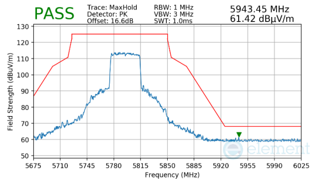
Plot 7-1175. Antenna WF5b (Peak, Ch.159, 802.11ax(SU), MCS7)
