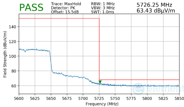
Plot 7-1190. (FCC Only) Antenna WF5b (Peak, Ch.122, 802.11ac, MCS9)
