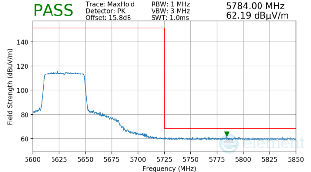
Plot 7-1164. (FCC Only) Antenna WF5b (Peak, Ch.126, 802.11ax(SU), MCS2)
