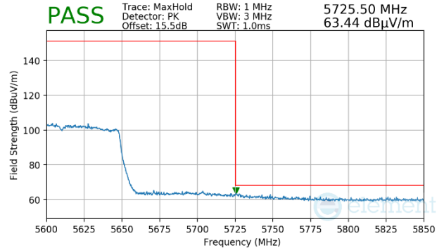
Plot 7-1227. (FCC Only) Antenna WF5b (Peak, Ch.114, 802.11ac, MCS2)
