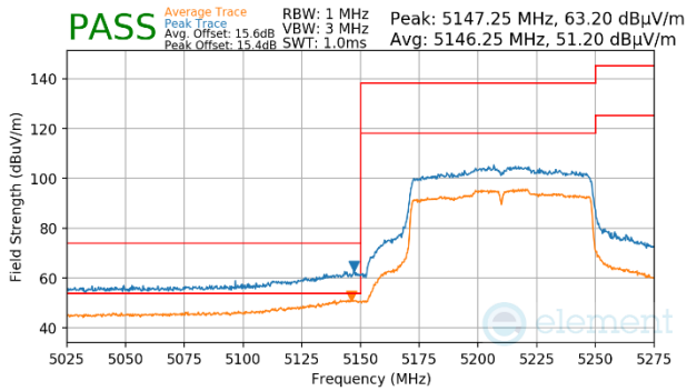
Plot 7-1176. Antenna WF5b (Peak & Average, Ch.42, 802.11ac, MCS2)
