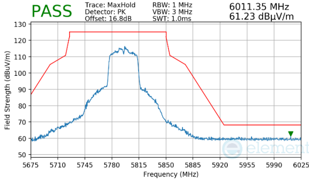
Plot 7-1141. Antenna WF5b (Peak, Ch.159, 802.11n, MCS4)
