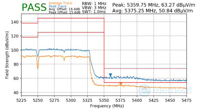
Plot 7-1223. Antenna WF5b (Peak & Average, Ch.50, 802.11ac, MCS9)
