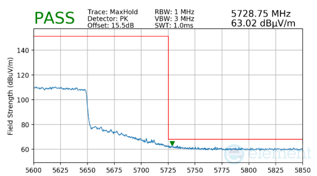
Plot 7-1211. (FCC Only) Antenna WF5b (Peak, Ch122, 802.11ax(SU), MCS11)
