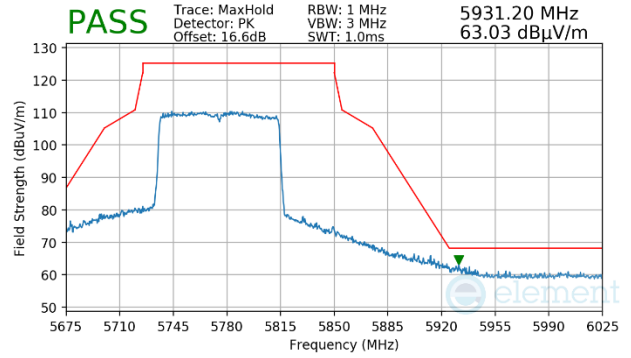
Plot 7-1215. Antenna WF5b (Peak, Ch155, 802.11ax(SU), MCS2)
