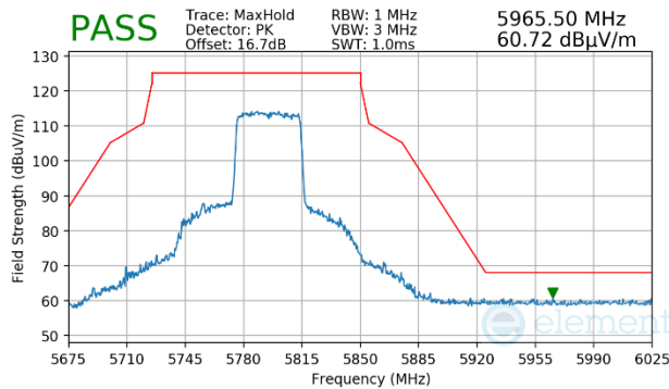
Plot 7-1173. Antenna WF5b (Peak, Ch.159, 802.11ax(SU), MCS2)
