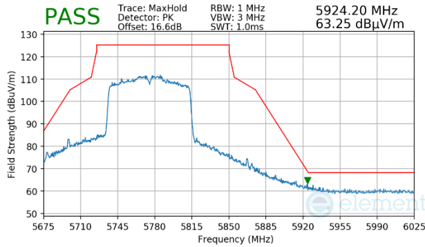
Plot 7-1194. Antenna WF5b (Peak, Ch.155, 802.11ac, MCS2)
