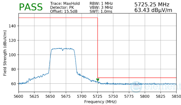
Plot 7-1136. Antenna WF5b (Peak, Ch.134, 802.11n, MCS7)
