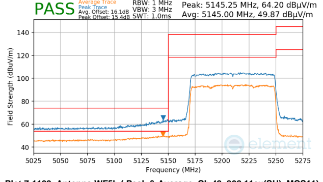
Plot 7-1199. Antenna WF5b (Peak & Average, Ch.42, 802.11ax(SU), MCS11)
