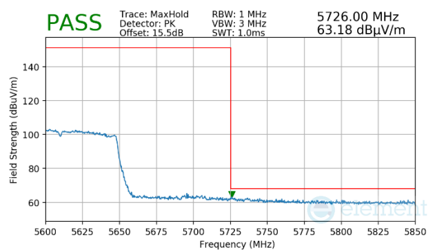
Plot 7-1228. (FCC Only) Antenna WF5b (Peak, Ch.114, 802.11ac, MCS4)
