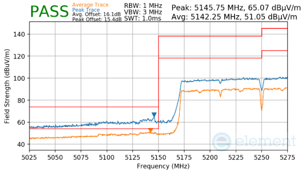
Plot 7-1220. Antenna WF5b (Peak & Average, Ch.50, 802.11ac, MCS9)
