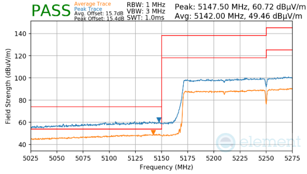
Plot 7-1230. Antenna WF5b (Peak & Average, Ch.50, 802.11ax(SU), MCS2)
