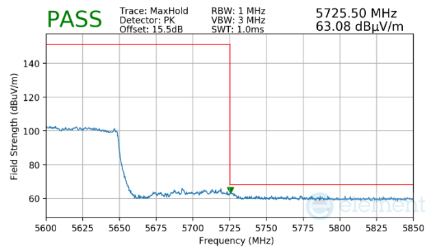
Plot 7-1241. (FCC Only) Antenna WF5b (Peak, Ch.114, 802.11ax(SU), MCS11)
