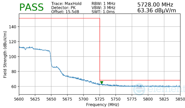
Plot 7-1189. (FCC Only) Antenna WF5b (Peak, Ch.122, 802.11ac, MCS4)
