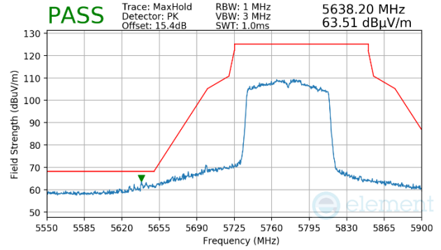
Plot 7-1191. Antenna WF5b (Peak, Ch.155, 802.11ac, MCS2)
