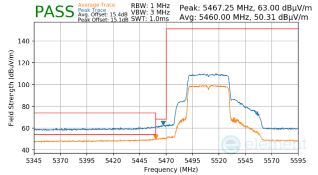
Plot 7-1156. Antenna WF5b (Peak & Average, Ch.102, 802.11ax(SU), MCS4)
