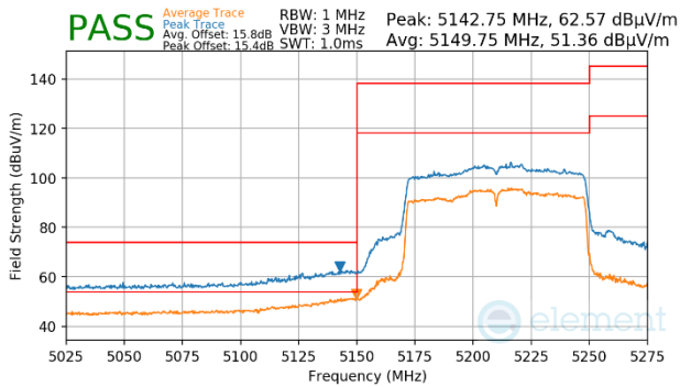
Plot 7-1177. Antenna WF5b (Peak & Average, Ch.42, 802.11ac, MCS4)
