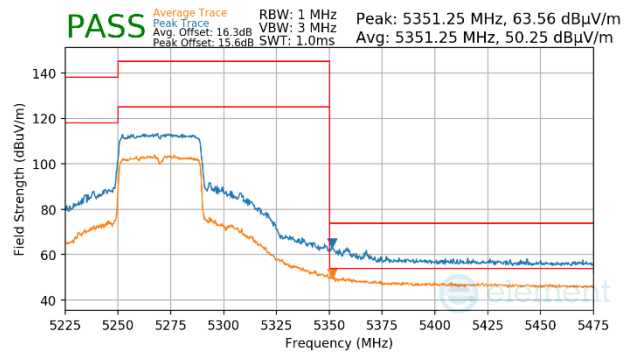
Plot 7-1151. Antenna WF5b (Peak & Average, Ch.54, 802.11ax(SU), MCS11)
