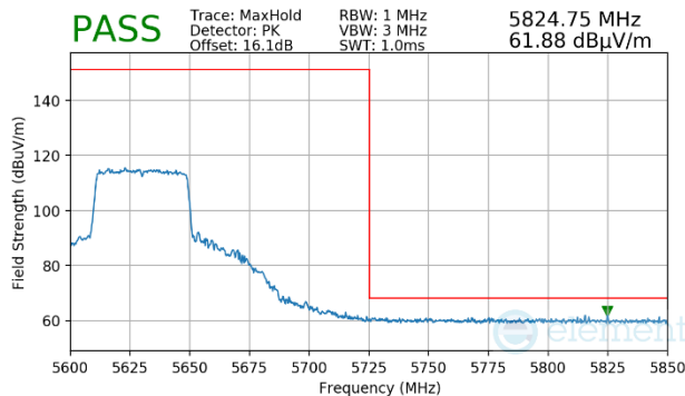
Plot 7-1166. (FCC Only) Antenna WF5b (Peak, Ch.126, 802.11ax(SU), MCS11)
