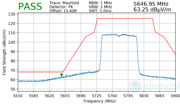
Plot 7-1212. Antenna WF5b (Peak, Ch155, 802.11ax(SU), MCS2)
