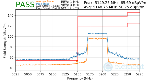
Plot 7-1145. Antenna WF5b (Peak & Average, Ch.38, 802.11ax(SU), MCS11)
