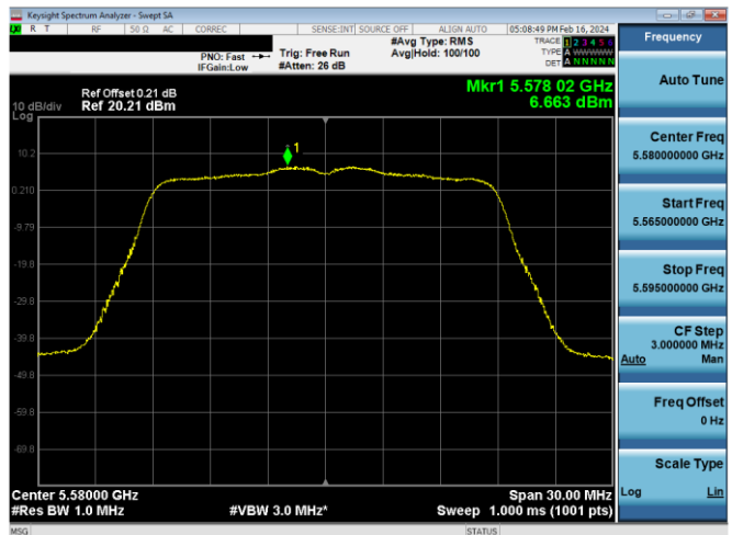
Plot 7-604. PSD CDD Antenna WF5b (20MHz BW 802.11n – Ch. 116, MCS10)
