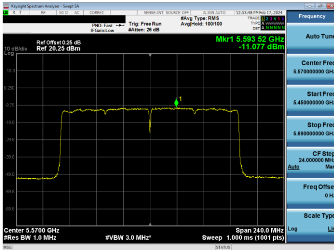
Plot 7-663. PSD CDD Antenna WF8 (160MHz BW 802.11ax(SU) – Ch. 114, MCS4)
