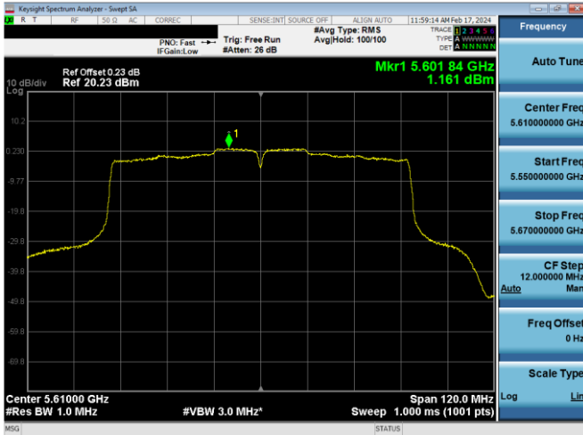
Plot 7-613. PSD CDD Antenna WF8 (80MHz BW 802.11ac – Ch. 122, MCS2)
