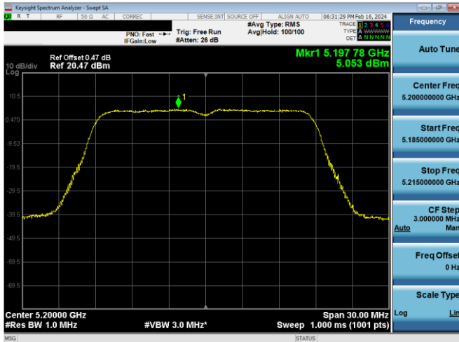
Plot 7-664. PSD CDD Antenna WF5b (20MHz BW 802.11n – Ch. 40, MCS15)
