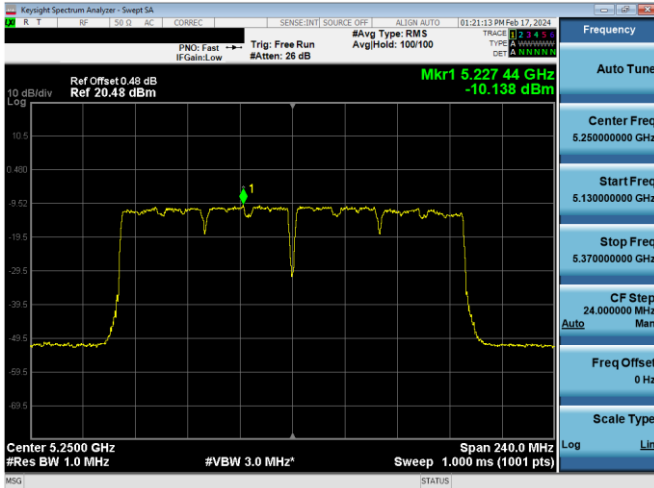
Plot 7-677. PSD CDD Antenna WF8 (160MHz BW 802.11ac – Ch. 50, MCS9)
