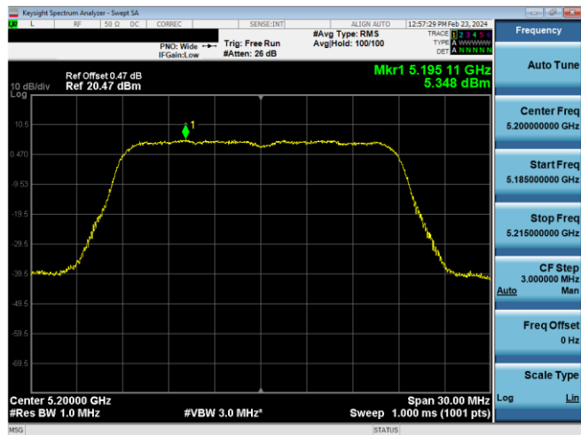
Plot 7-665. PSD CDD Antenna WF8 (20MHz BW 802.11n – Ch. 40, MCS15)
