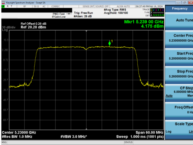
Plot 7-670. PSD CDD Antenna WF5b (40MHz BW 802.11ax(SU) – Ch. 46, MCS11)
