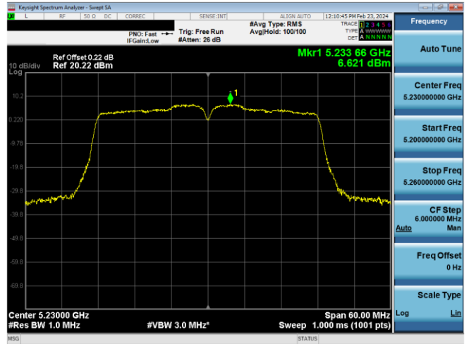
Plot 7-625. PSD CDD Antenna WF8 (40MHz BW 802.11n – Ch. 46, MCS12)
