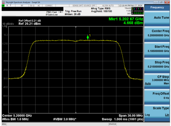
Plot 7-623. PSD CDD Antenna WF8 (20MHz BW 802.11ax(SU) – Ch. 40, MCS4)
