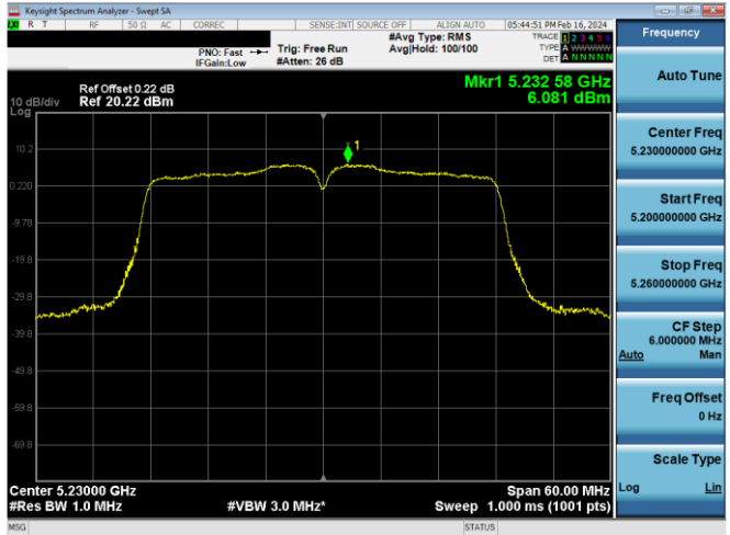
Plot 7-624. PSD CDD Antenna WF5b (40MHz BW 802.11n – Ch. 46, MCS12)
