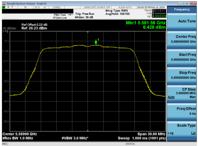
Plot 7-648. PSD CDD Antenna WF5b (20MHz BW 802.11n – Ch. 116, MCS12)
