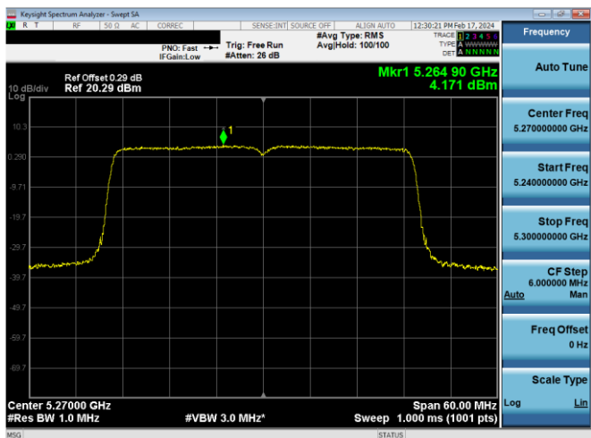
Plot 7-643. PSD CDD Antenna WF8 (40MHz BW 802.11ax(SU) – Ch. 54, MCS4)
