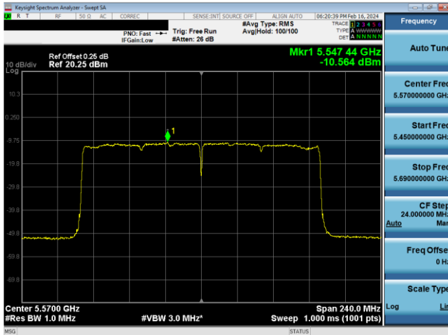
Plot 7-662. PSD CDD Antenna WF5b (160MHz BW 802.11ax(SU) – Ch. 114, MCS4)
