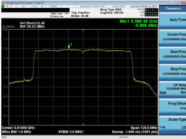
Plot 7-658. PSD CDD Antenna WF5b (80MHz BW 802.11ax(SU) – Ch. 122, MCS4)
