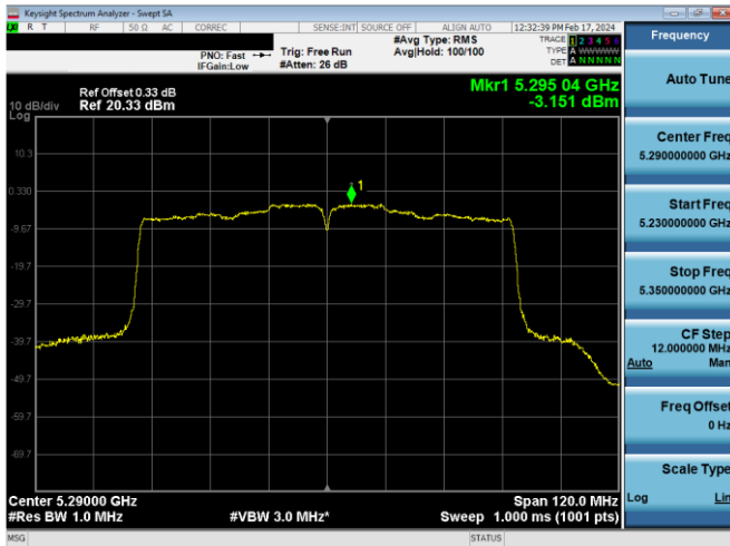
Plot 7-645. PSD CDD Antenna WF8 (80MHz BW 802.11ac – Ch. 58, MCS4)
