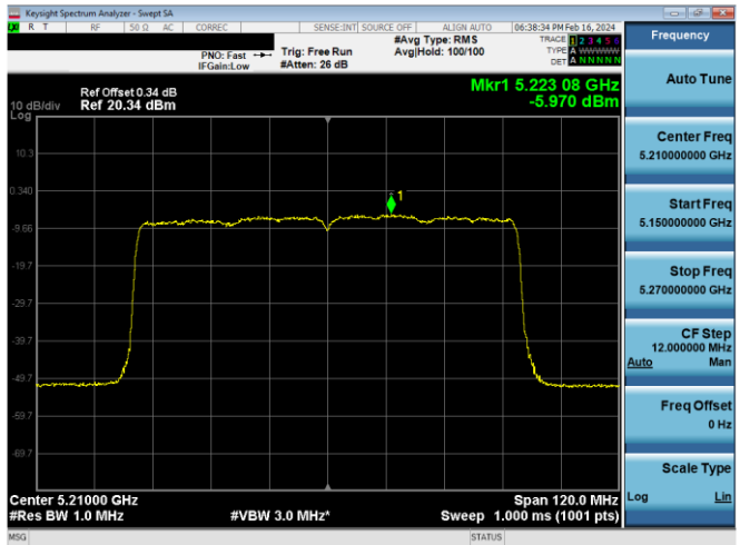
Plot 7-674. PSD CDD Antenna WF5b (80MHz BW 802.11ax(SU) – Ch. 42, MCS11)
