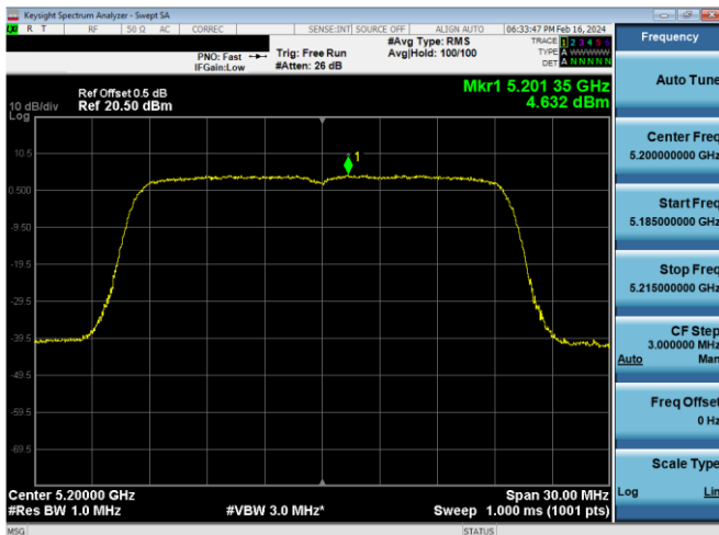
Plot 7-666. PSD CDD Antenna WF5b (20MHz BW 802.11ax(SU) – Ch. 40, MCS11)
