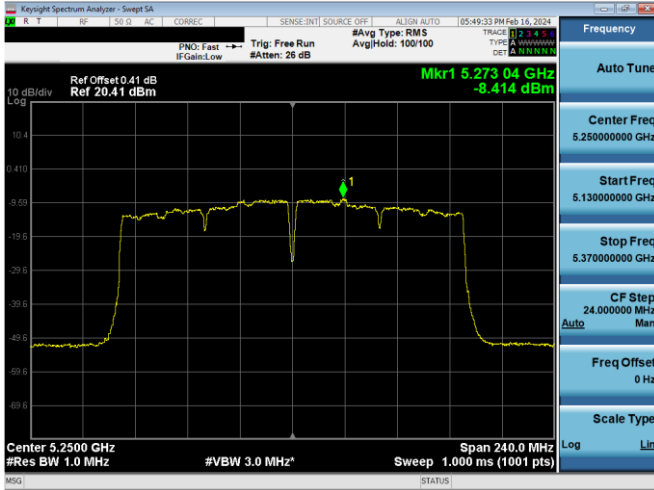
Plot 7-632. PSD CDD Antenna WF5b (160MHz BW 802.11ac – Ch. 50, MCS4)
