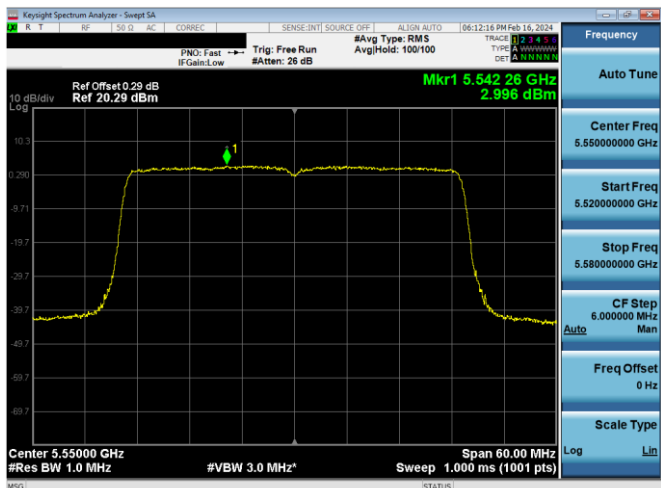
Plot 7-654. PSD CDD Antenna WF5b (40MHz BW 802.11ax(SU) – Ch. 110, MCS4)
