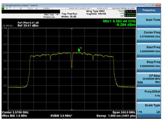
Plot 7-660. PSD CDD Antenna WF5b (160MHz BW 802.11ac – Ch. 114, MCS4)
