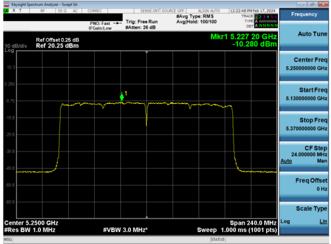
Plot 7-635. PSD CDD Antenna WF8 (160MHz BW 802.11ax(SU) – Ch. 50, MCS4)
