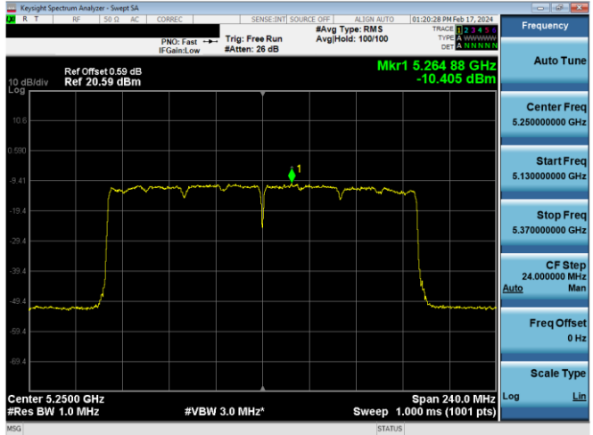
Plot 7-679. PSD CDD Antenna WF8 (160MHz BW 802.11ax(SU) – Ch. 50, MCS11)
