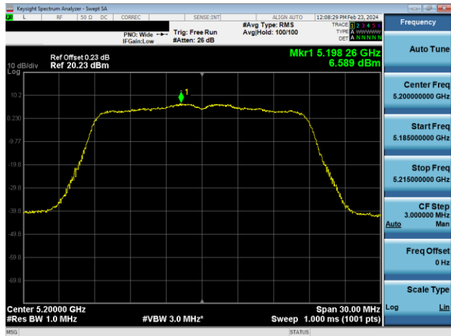
Plot 7-621. PSD CDD Antenna WF8 (20MHz BW 802.11n – Ch. 40, MCS12)
