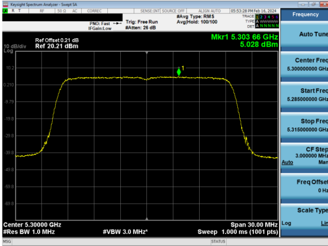
Plot 7-638. PSD CDD Antenna WF5b (20MHz BW 802.11ax(SU) – Ch. 60, MCS4)
