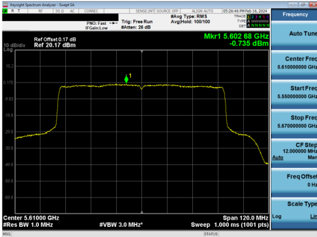
Plot 7-614. PSD CDD Antenna WF5b (80MHz BW 802.11ax(SU) – Ch. 122, MCS2)
