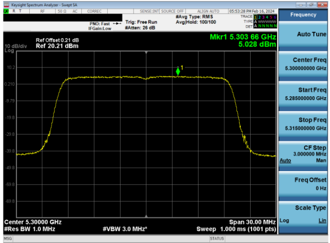
Plot 7-636. PSD CDD Antenna WF5b (20MHz BW 802.11n – Ch. 60, MCS12)
