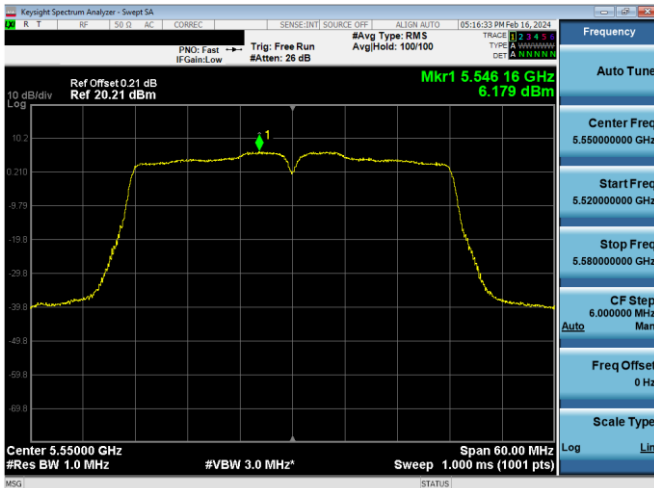
Plot 7-608. PSD CDD Antenna WF5b (40MHz BW 802.11n – Ch. 110, MCS10)
