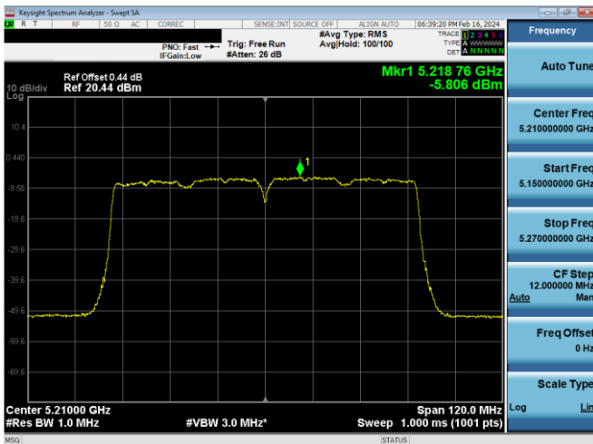
Plot 7-672. PSD CDD Antenna WF5b (80MHz BW 802.11ac – Ch. 42, MCS9)
