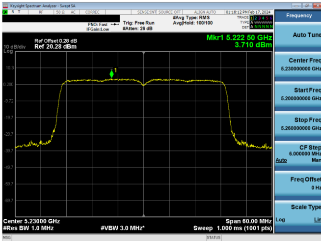
Plot 7-671. PSD CDD Antenna WF8 (40MHz BW 802.11ax(SU) – Ch. 46, MCS11)
