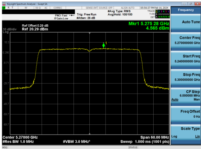
Plot 7-642. PSD CDD Antenna WF5b (40MHz BW 802.11ax(SU) – Ch. 54, MCS4)
