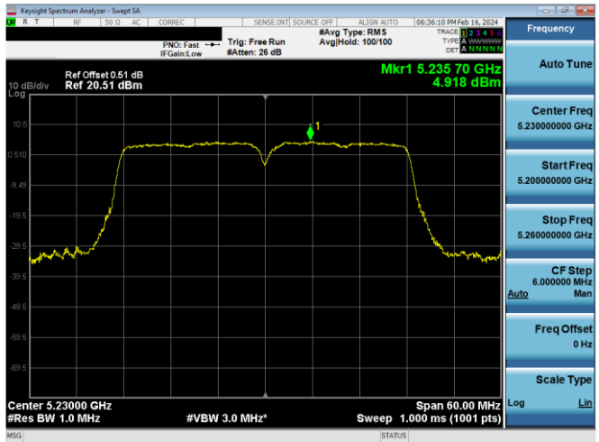
Plot 7-668. PSD CDD Antenna WF5b (40MHz BW 802.11n – Ch. 46, MCS15)
