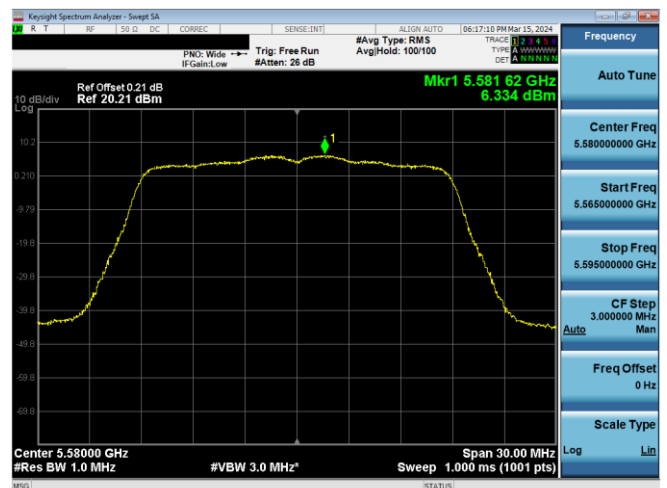
Plot 7-605. PSD CDD Antenna WF8 (20MHz BW 802.11n – Ch. 116, MCS10)
