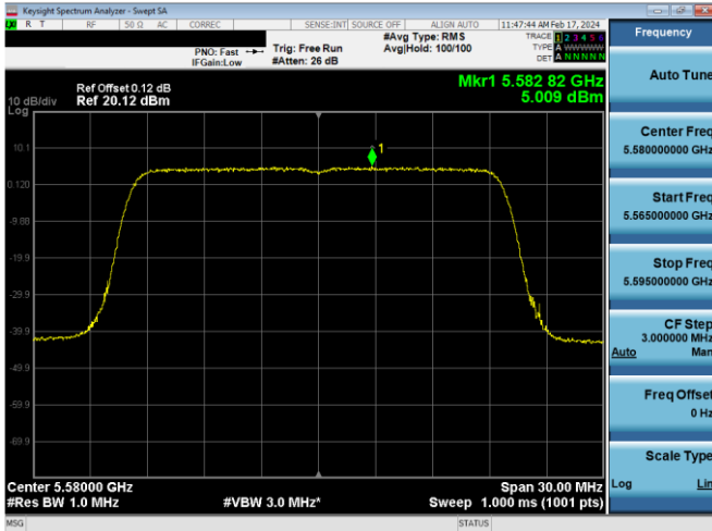
Plot 7-607. PSD CDD Antenna WF8 (20MHz BW 802.11ax(SU) – Ch. 116, MCS2)
