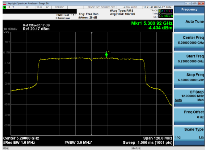
Plot 7-603. PSD CDD Antenna WF8 (80MHz BW 802.11ax(SU) – Ch. 58, MCS2)
