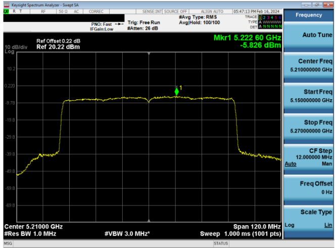
Plot 7-630. PSD CDD Antenna WF5b (80MHz BW 802.11ax(SU) - Ch. 42, MCS4)
