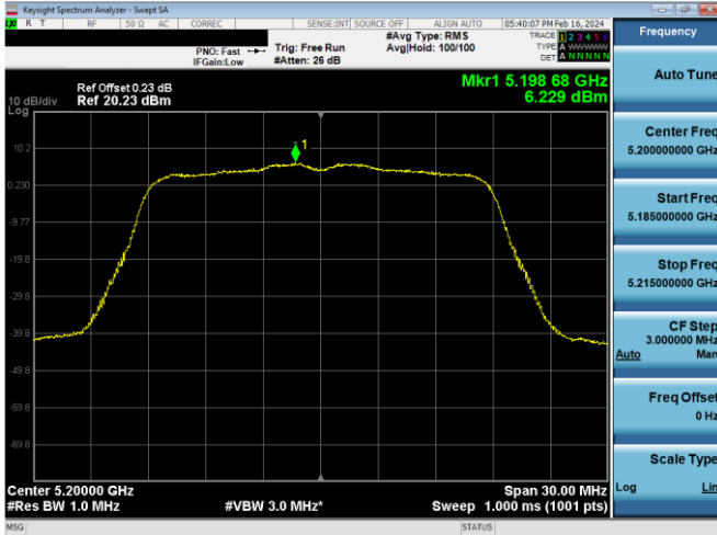
Plot 7-620. PSD CDD Antenna WF5b (20MHz BW 802.11n – Ch. 40, MCS12)
