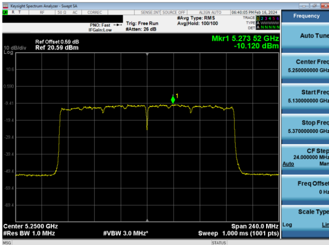
Plot 7-678. PSD CDD Antenna WF5b (160MHz BW 802.11ax(SU) – Ch. 50, MCS11)
