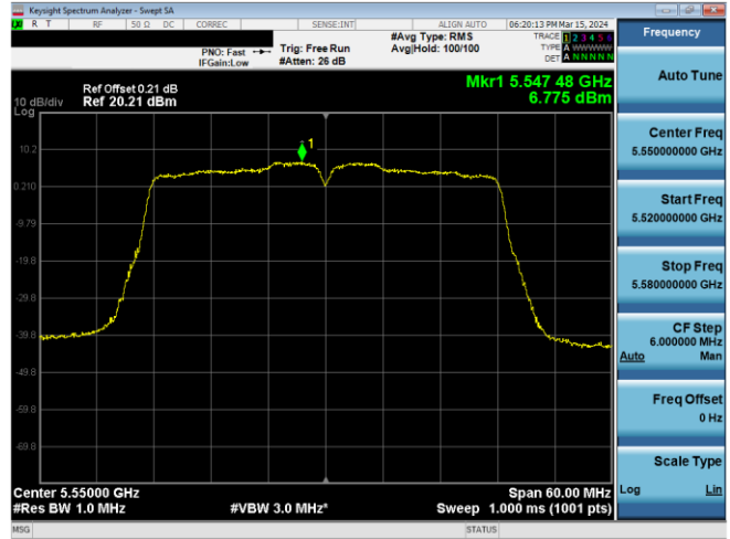
Plot 7-609. PSD CDD Antenna WF8 (40MHz BW 802.11n – Ch. 110, MCS10)
