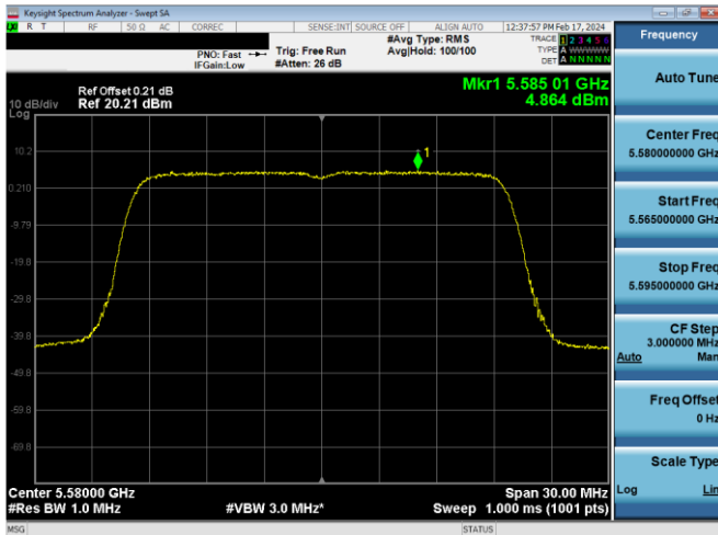
Plot 7-651. PSD CDD Antenna WF8 (20MHz BW 802.11ax(SU) – Ch. 116, MCS4)
