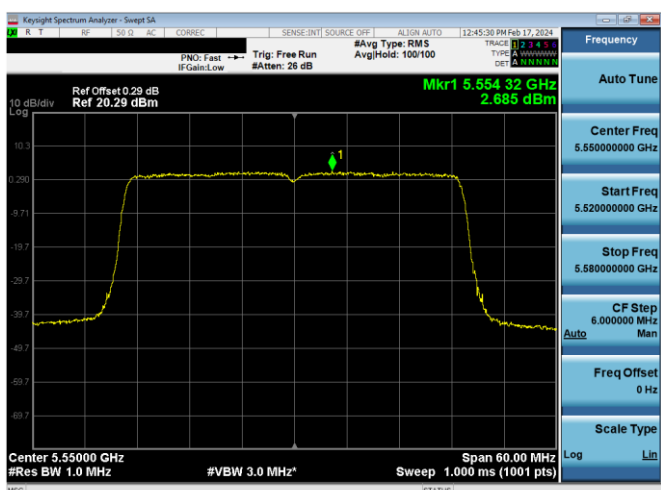
Plot 7-655. PSD CDD Antenna WF8 (40MHz BW 802.11ax(SU) – Ch. 110, MCS4)
