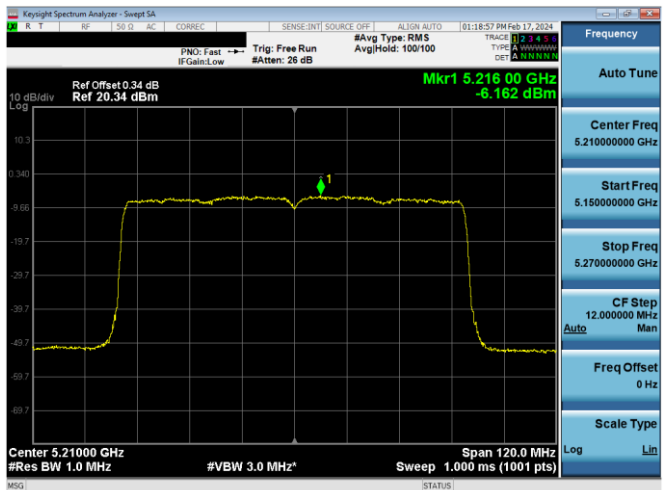
Plot 7-675. PSD CDD Antenna WF8 (80MHz BW 802.11ax(SU) – Ch. 42, MCS11)
