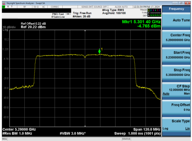
Plot 7-647. PSD CDD Antenna WF8 (80MHz BW 802.11ax(SU) – Ch. 58, MCS4)
