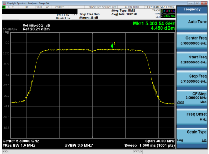
Plot 7-637. PSD CDD Antenna WF8 (20MHz BW 802.11n – Ch. 60, MCS12)
