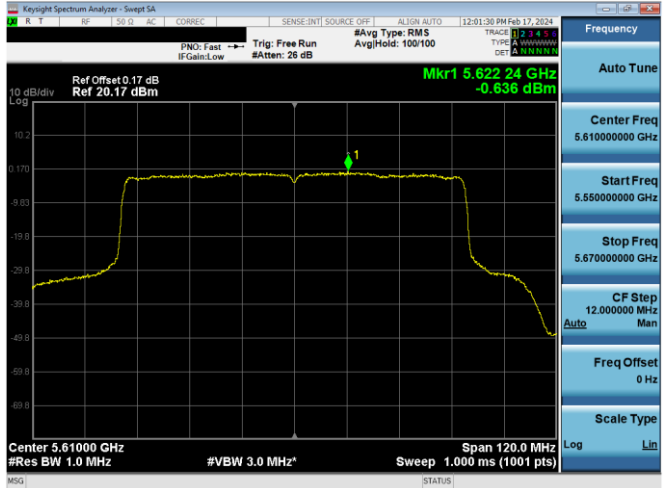
Plot 7-615. PSD CDD Antenna WF8 (80MHz BW 802.11ax(SU) – Ch. 122, MCS2)
