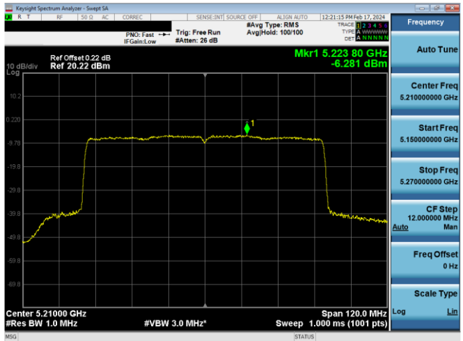
Plot 7-631. PSD CDD Antenna WF8 (80MHz BW 802.11ax(SU) - Ch. 42, MCS4)
