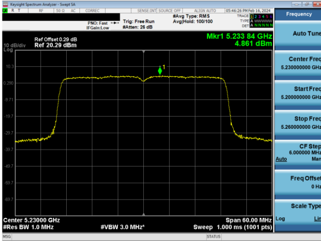
Plot 7-626. PSD CDD Antenna WF5b (40MHz BW 802.11ax(SU) - Ch. 46, MCS4)
