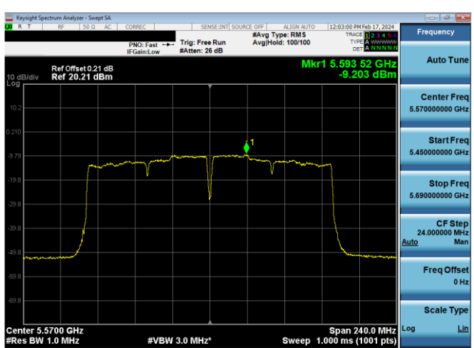
Plot 7-617. PSD CDD Antenna WF8 (160MHz BW 802.11ac – Ch. 114, MCS2)
