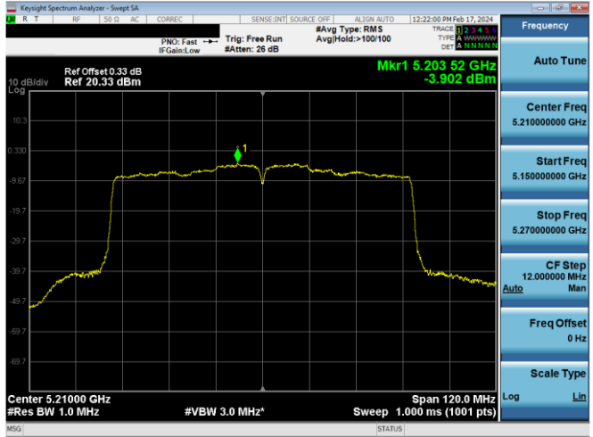
Plot 7-629. PSD CDD Antenna WF8 (80MHz BW 802.11ac - Ch. 42, MCS4)
