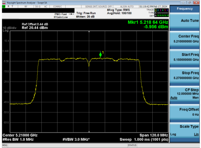
Plot 7-673. PSD CDD Antenna WF8 (80MHz BW 802.11ac – Ch. 42, MCS9)
