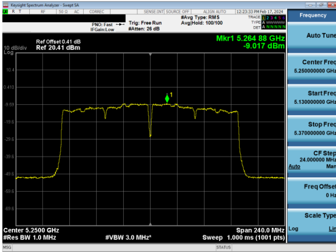
Plot 7-633. PSD CDD Antenna WF8 (160MHz BW 802.11ac – Ch. 50, MCS4)
