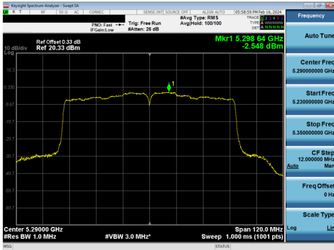
Plot 7-644. PSD CDD Antenna WF5b (80MHz BW 802.11ac – Ch. 58, MCS4)
