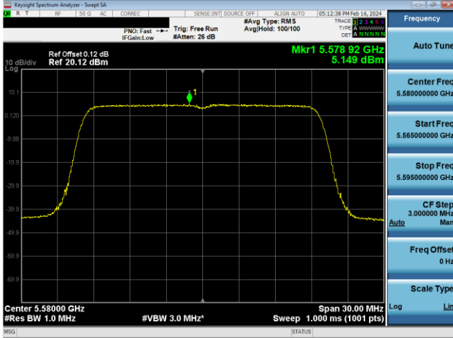
Plot 7-606. PSD CDD Antenna WF5b (20MHz BW 802.11ax(SU) – Ch. 116, MCS2)
