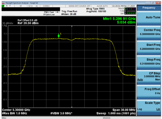
Plot 7-681. PSD CDD Antenna WF8 (20MHz BW 802.11n – Ch. 60, MCS15)
