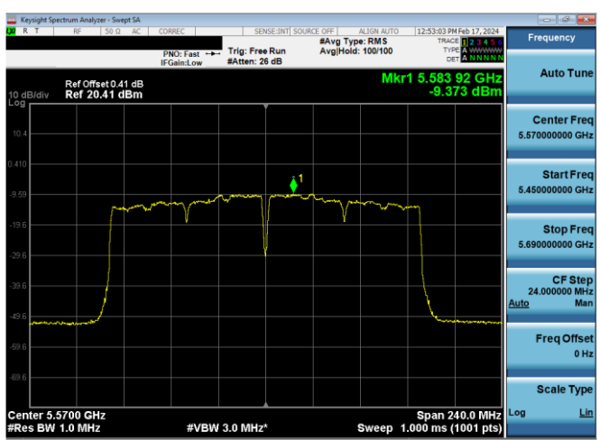
Plot 7-661. PSD CDD Antenna WF8 (160MHz BW 802.11ac – Ch. 114, MCS4)
