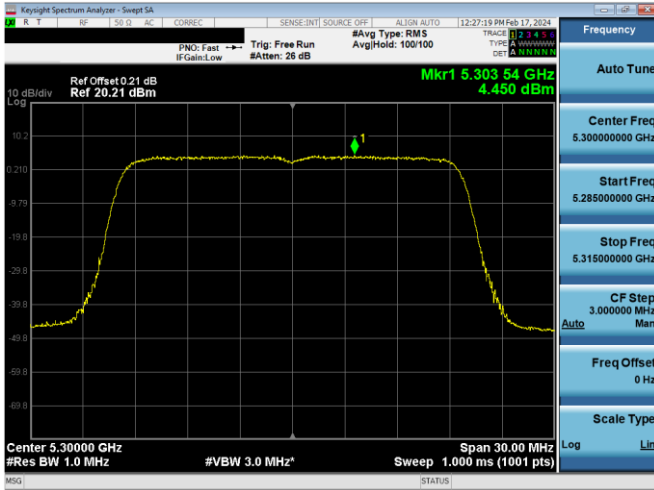
Plot 7-639. PSD CDD Antenna WF8 (20MHz BW 802.11ax(SU) – Ch. 60, MCS4)
