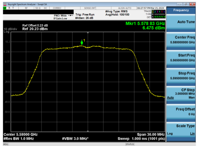
Plot 7-649. PSD CDD Antenna WF8 (20MHz BW 802.11n – Ch. 116, MCS12)
