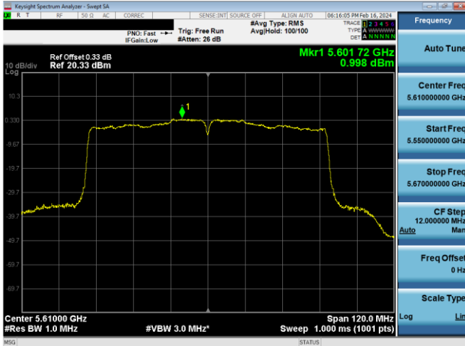
Plot 7-656. PSD CDD Antenna WF5b (80MHz BW 802.11ac – Ch. 122, MCS4)
