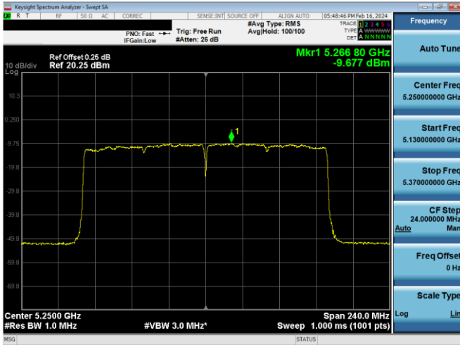
Plot 7-634. PSD CDD Antenna WF5b (160MHz BW 802.11ax(SU) – Ch. 50, MCS4)
