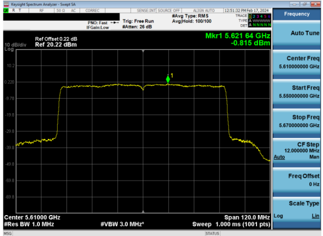
Plot 7-659. PSD CDD Antenna WF8 (80MHz BW 802.11ax(SU) – Ch. 122, MCS4)
