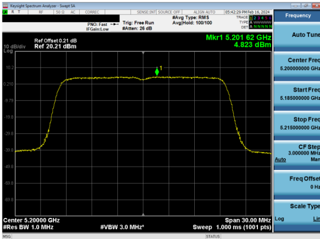
Plot 7-622. PSD CDD Antenna WF5b (20MHz BW 802.11ax(SU) – Ch. 40, MCS4)
