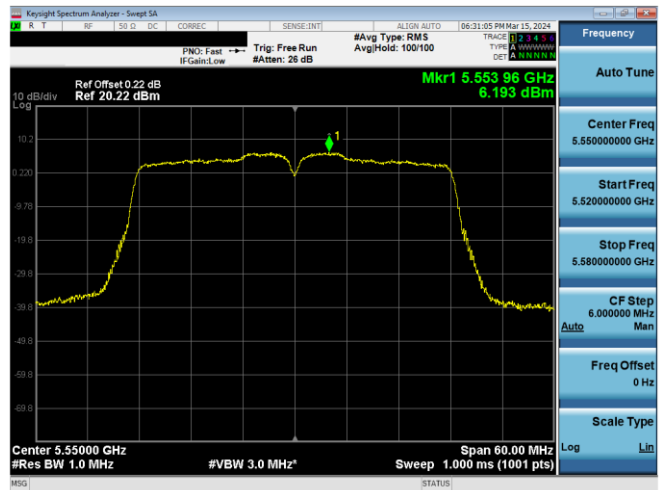
Plot 7-653. PSD CDD Antenna WF8 (40MHz BW 802.11n – Ch. 110, MCS12)
