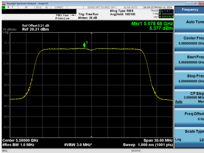
Plot 7-650. PSD CDD Antenna WF5b (20MHz BW 802.11ax(SU) – Ch. 116, MCS4)
