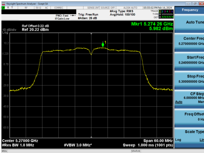
Plot 7-640. PSD CDD Antenna WF5b (40MHz BW 802.11n – Ch. 54, MCS12)
