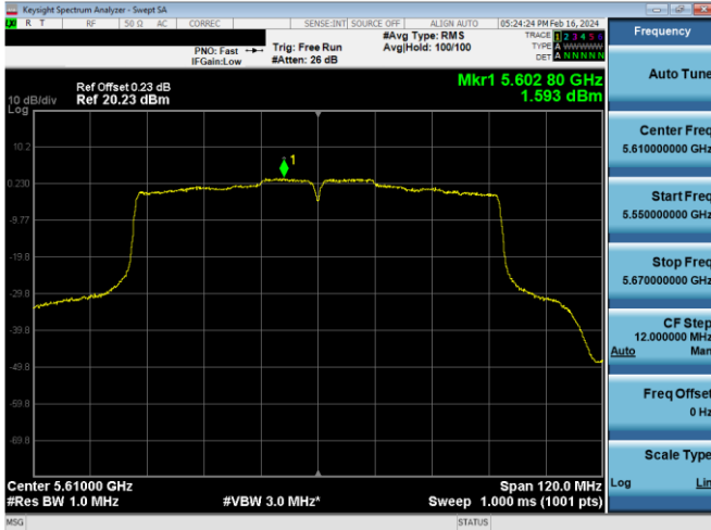
Plot 7-612. PSD CDD Antenna WF5b (80MHz BW 802.11ac – Ch. 122, MCS2)
