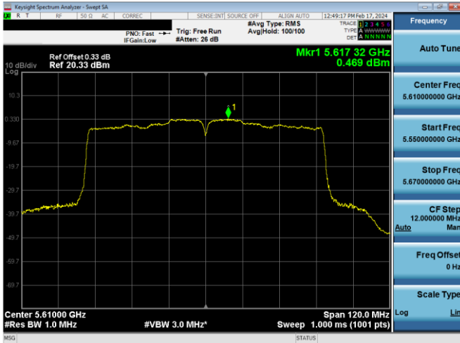
Plot 7-657. PSD CDD Antenna WF8 (80MHz BW 802.11ac – Ch. 122, MCS4)
