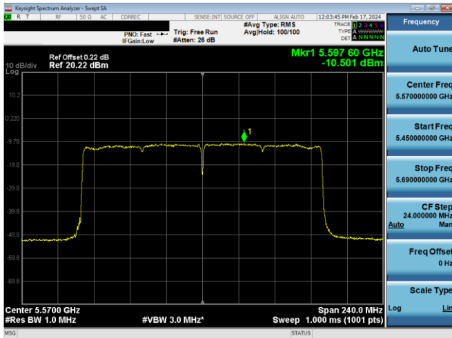
Plot 7-619. PSD CDD Antenna WF8 (160MHz BW 802.11ax(SU) – Ch. 114, MCS2)
