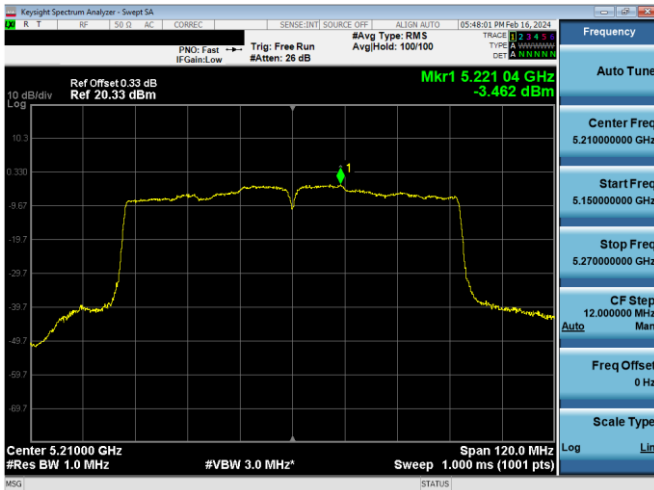
Plot 7-628. PSD CDD Antenna WF5b (80MHz BW 802.11ac - Ch. 42, MCS4)
