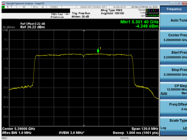
Plot 7-646. PSD CDD Antenna WF5b (80MHz BW 802.11ax(SU) – Ch. 58, MCS4)
