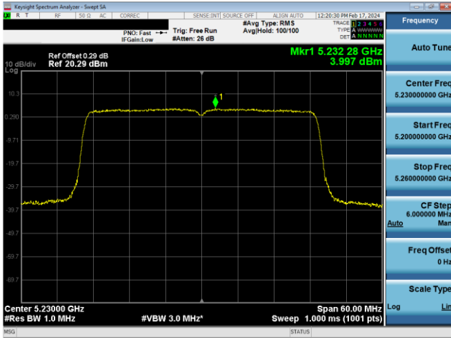
Plot 7-627. PSD CDD Antenna WF8 (40MHz BW 802.11ax(SU) - Ch. 46, MCS4)
