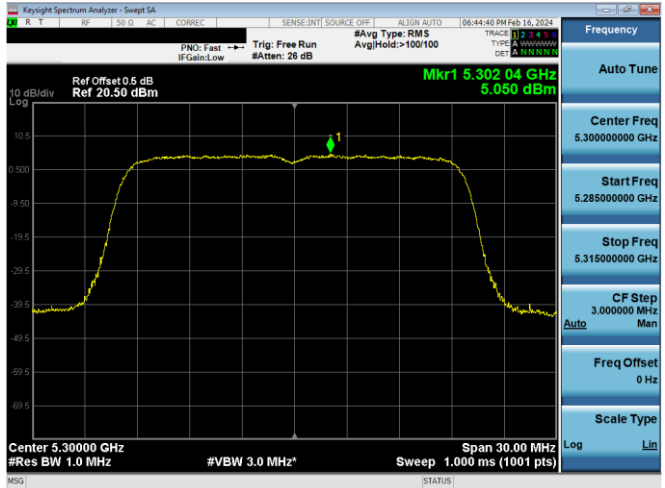
Plot 7-680. PSD CDD Antenna WF5b (20MHz BW 802.11n – Ch. 60, MCS15)
