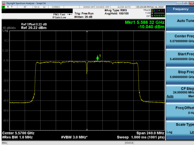
Plot 7-618. PSD CDD Antenna WF5b (160MHz BW 802.11ax(SU) – Ch. 114, MCS2)
