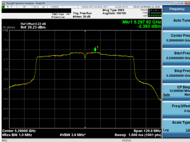
Plot 7-600. PSD CDD Antenna WF5b (80MHz BW 802.11ac – Ch. 58, MCS2)
