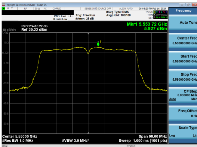
Plot 7-652. PSD CDD Antenna WF5b (40MHz BW 802.11n – Ch. 110, MCS12)
