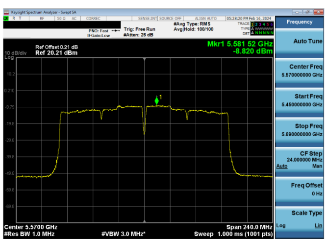
Plot 7-616. PSD CDD Antenna WF5b (160MHz BW 802.11ac – Ch. 114, MCS2)
