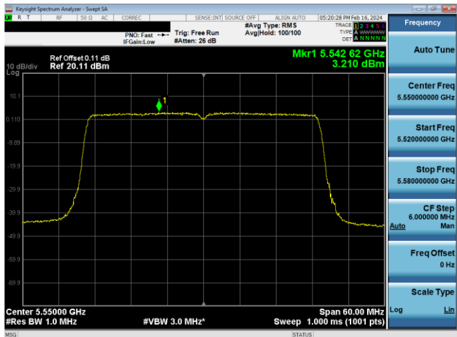
Plot 7-610. PSD CDD Antenna WF5b (40MHz BW 802.11ax(SU) – Ch. 110, MCS2)
