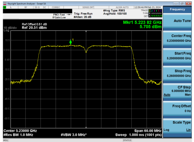
Plot 7-669. PSD CDD Antenna WF8 (40MHz BW 802.11n – Ch. 46, MCS15)
