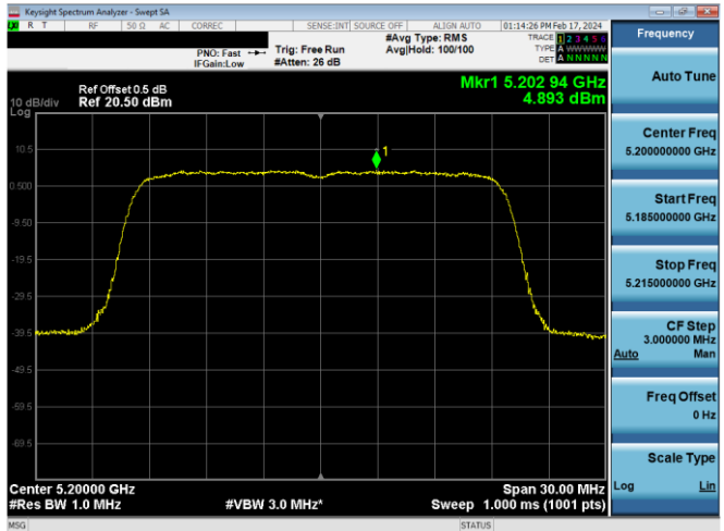
Plot 7-667. PSD CDD Antenna WF8 (20MHz BW 802.11ax(SU) – Ch. 40, MCS11)
