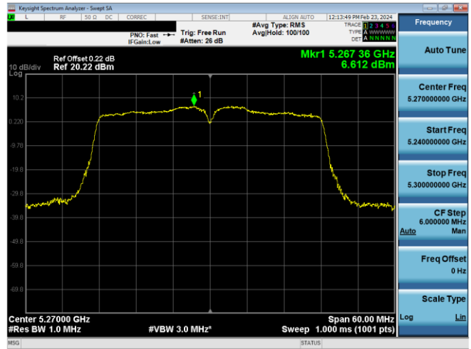
Plot 7-641. PSD CDD Antenna WF8 (40MHz BW 802.11n – Ch. 54, MCS12)
