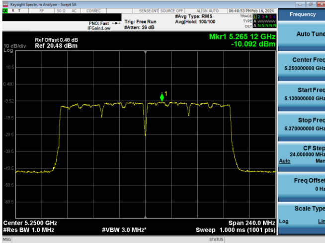
Plot 7-676. PSD CDD Antenna WF5b (160MHz BW 802.11ac – Ch. 50, MCS9)
