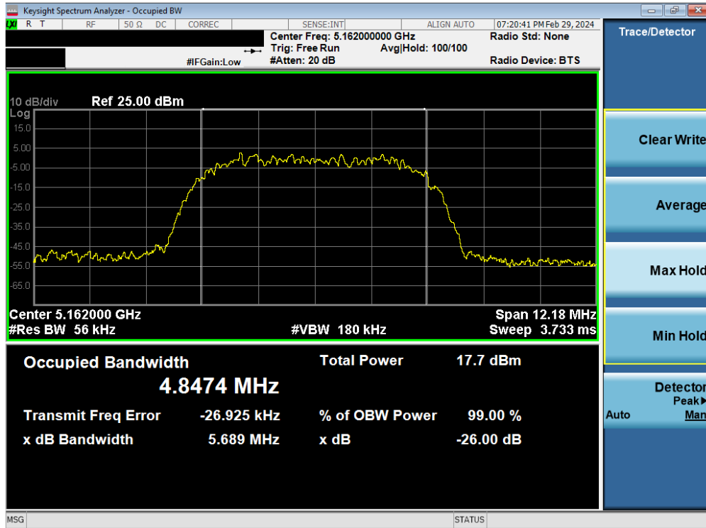
Plot 7-16. 26dB BW & 99% OBW Antenna WF7 (HDR8, ePA- 5162MHz)
