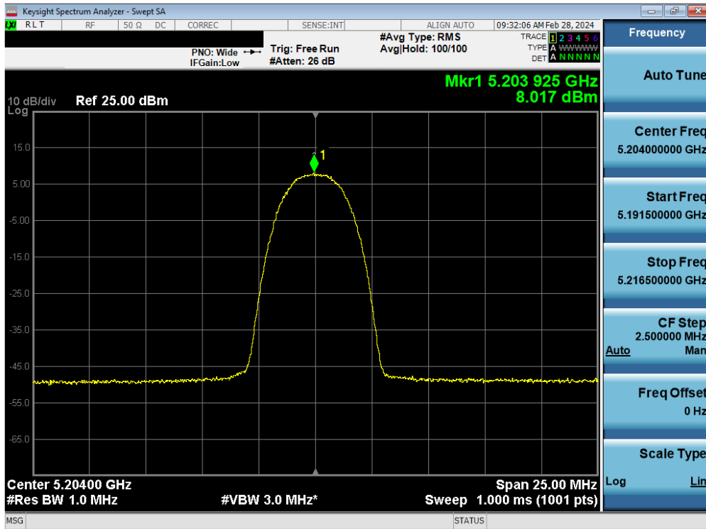
Plot 7-68. FCC PSD Antenna WF8 (HDR4, ePA – 5204MHz)
