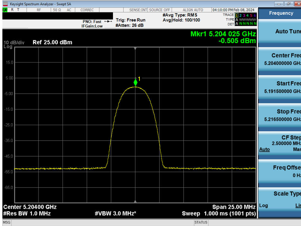
Plot 7-71. FCC/ISED PSD Antenna WF8 (HDR4, iPA – 5204MHz)
