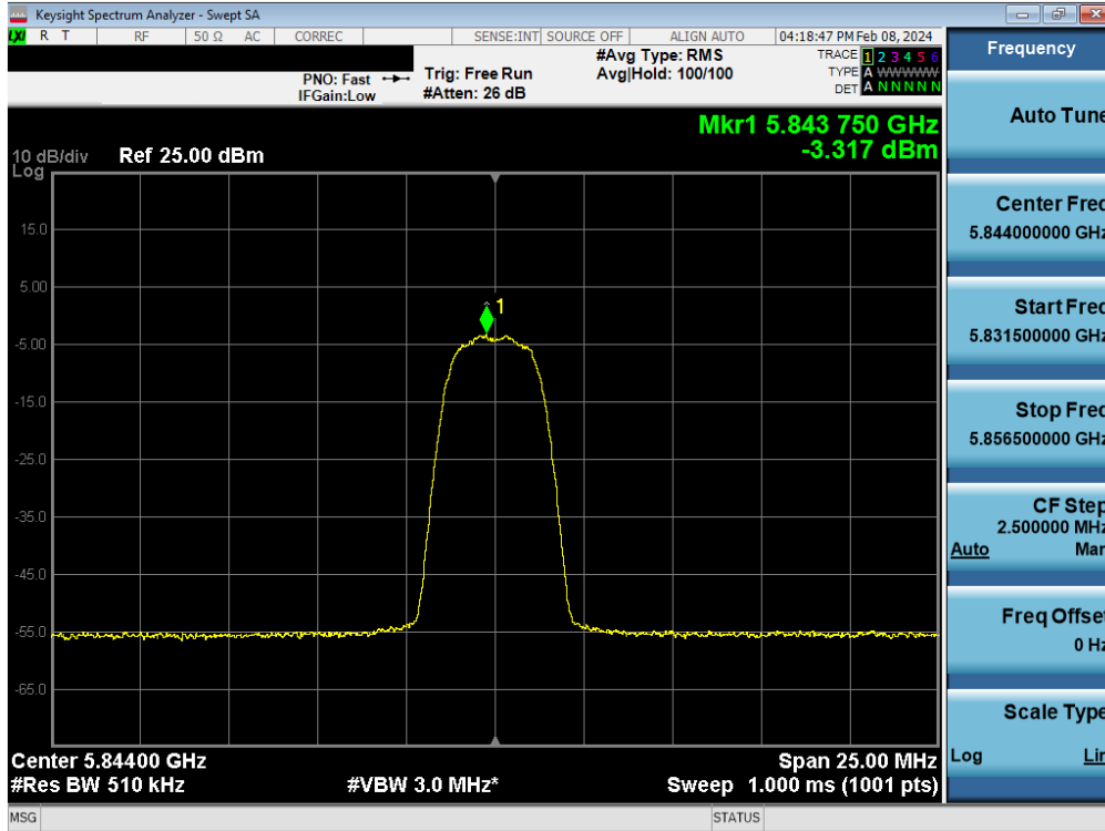
Plot 7-87. PSD Antenna WF8 (HDR4, iPA 5844MHz)
