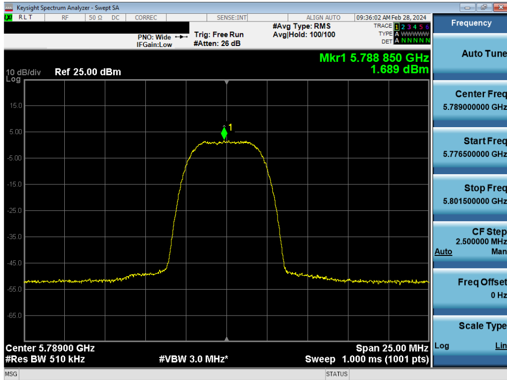
Plot 7-89. PSD Antenna WF8 (HDR8, ePA 5789MHz)
