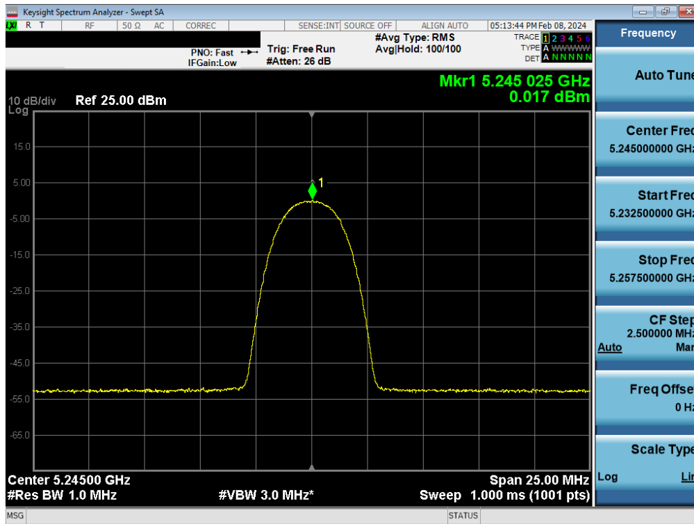
Plot 7-99. PSD Antenna WF7 (HDR4, iPA– 5245MHz)
