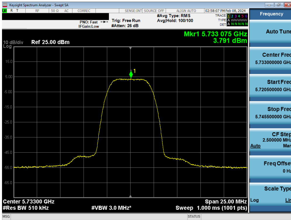
Plot 7-61. PSD Antenna WF5B (HDR8, ePA 5733MHz)
