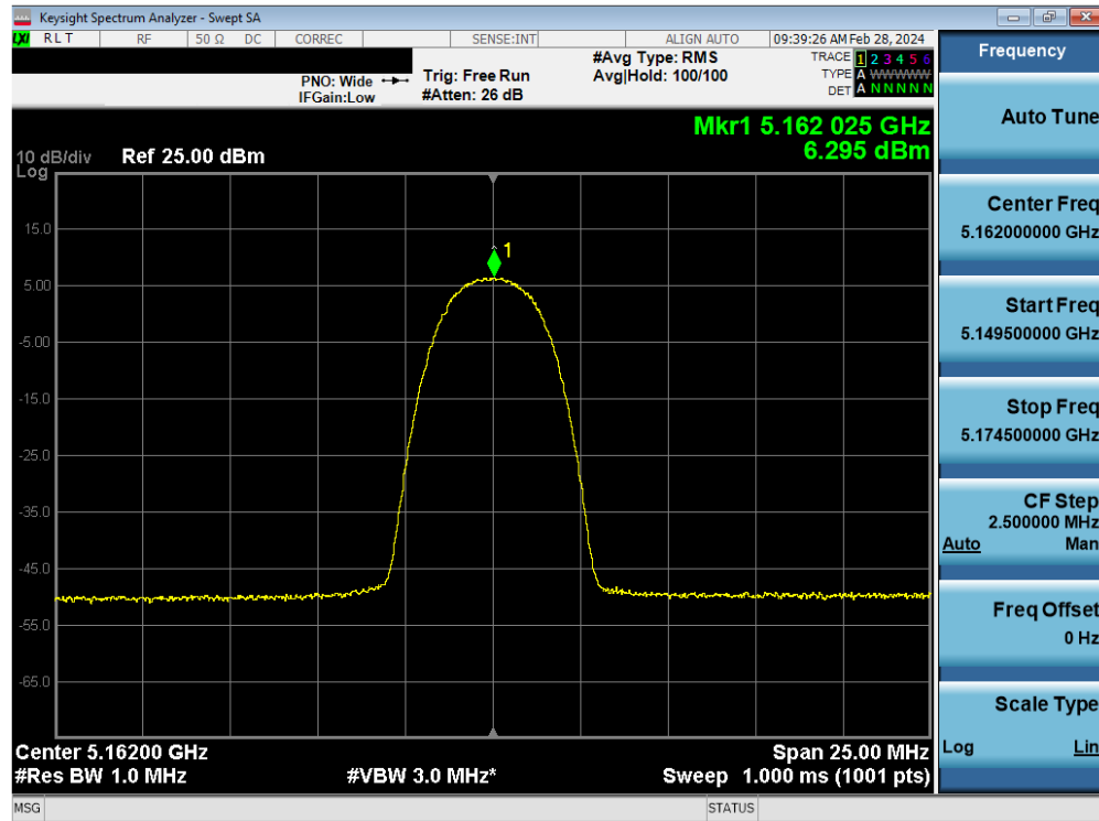
Plot 7-119. FCC PSD TxBF Antenna WF8 (HDR4, ePA – 5162MHz)
