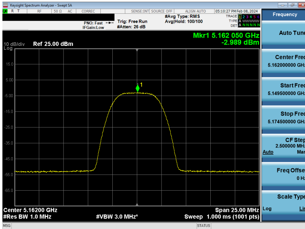
Plot 7-103. PSD Antenna WF7 (HDR8, iPA - 5162MHz)
