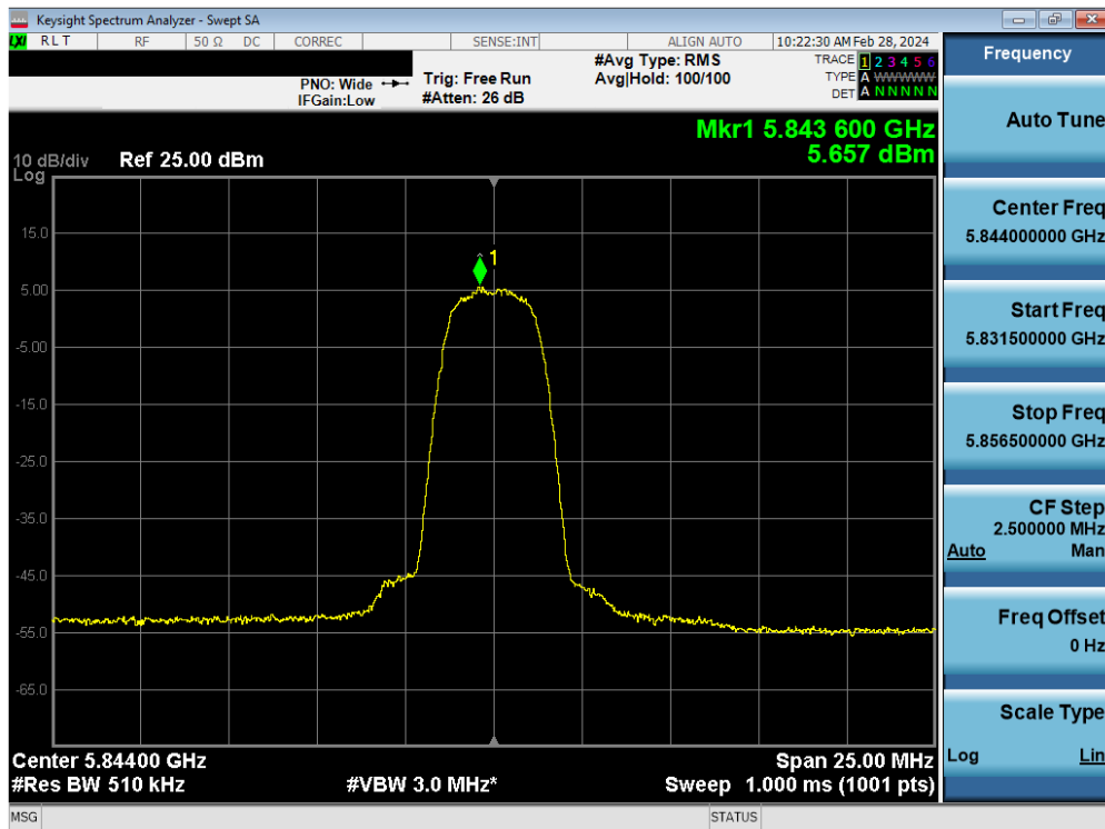
Plot 7-108. PSD Antenna WF7 (HDR4, ePA 5844MHz)
