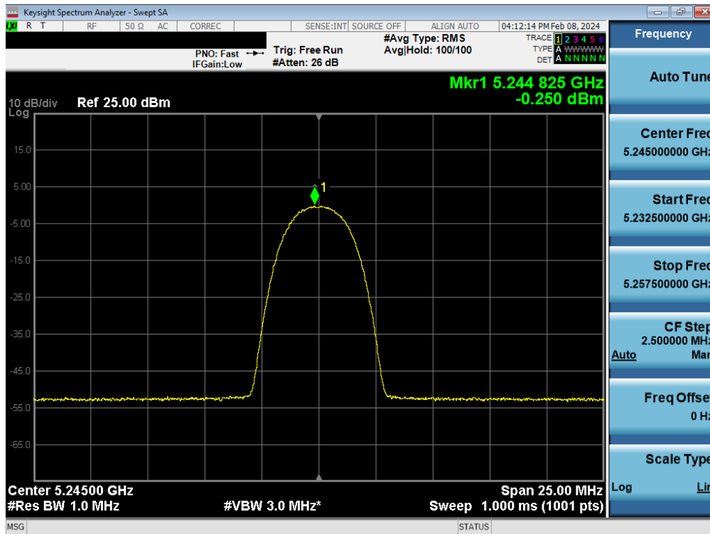
Plot 7-72. FCC/ISED PSD Antenna WF8 (HDR4, iPA– 5245MHz)
