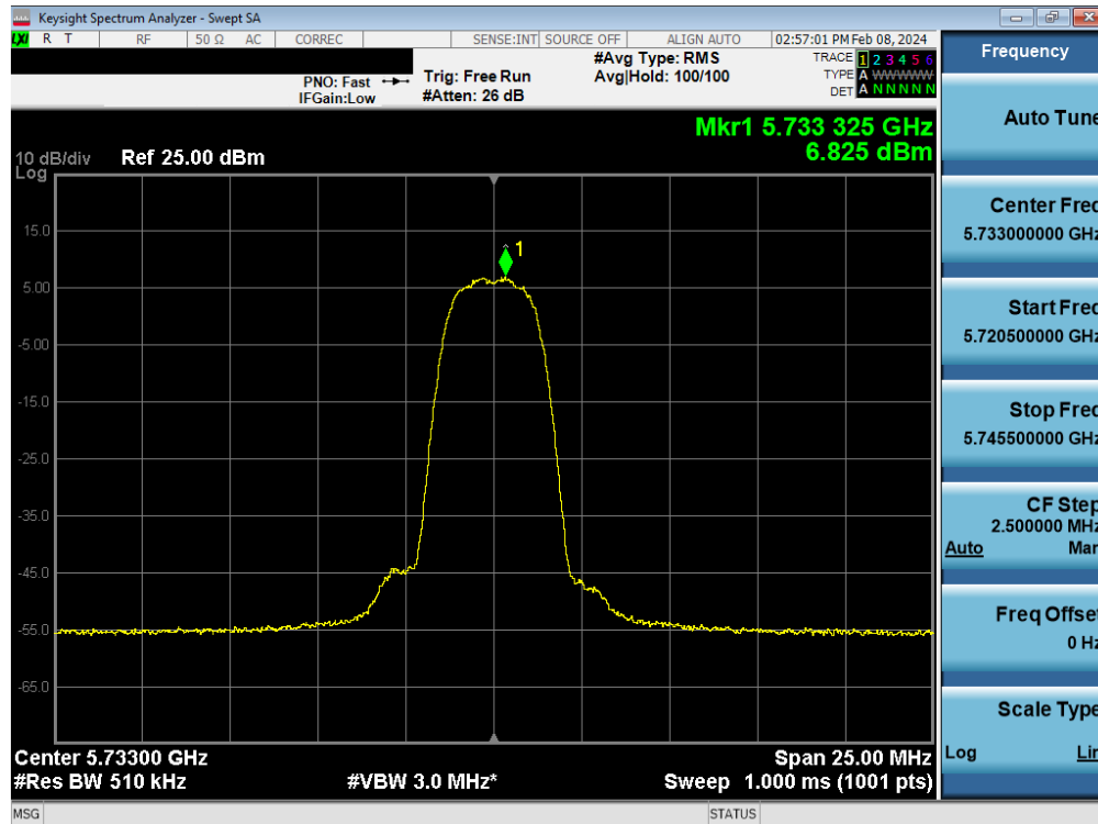
Plot 7-55. PSD Antenna WF5B (HDR4, ePA 5733MHz)
