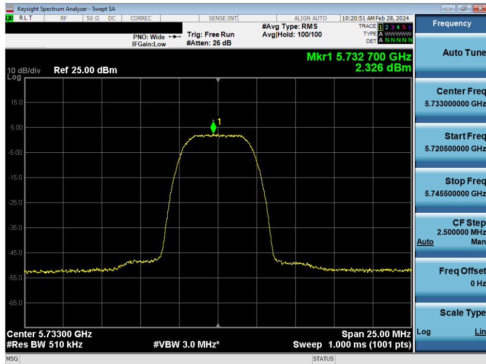
Plot 7-112. PSD Antenna WF7 (HDR8, ePA 5733MHz)
