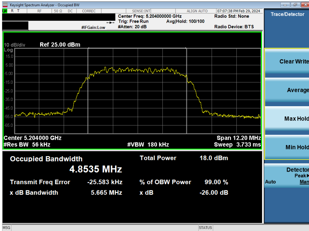
Plot 7-11. 26dB BW & 99% OBW Antenna WF8 (HDR8, ePA- 5204MHz)
