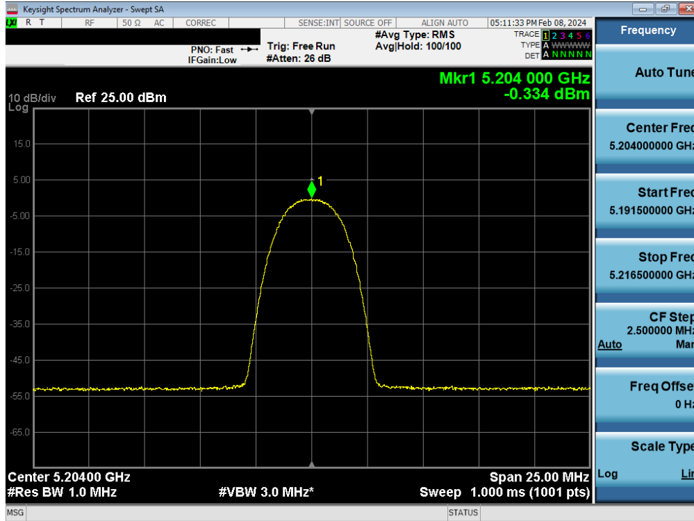
Plot 7-98. PSD Antenna WF7 (HDR4, iPA – 5204MHz)
