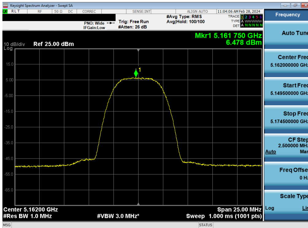
Plot 7-52. ISED PSD Antenna WF5B (HDR8, ePA – 5162MHz)
