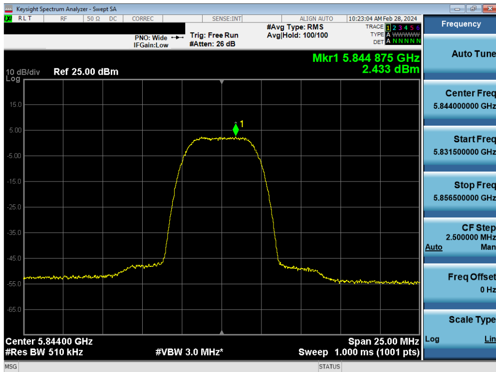
Plot 7-114. PSD Antenna WF7 (HDR8, ePA 5844MHz)
