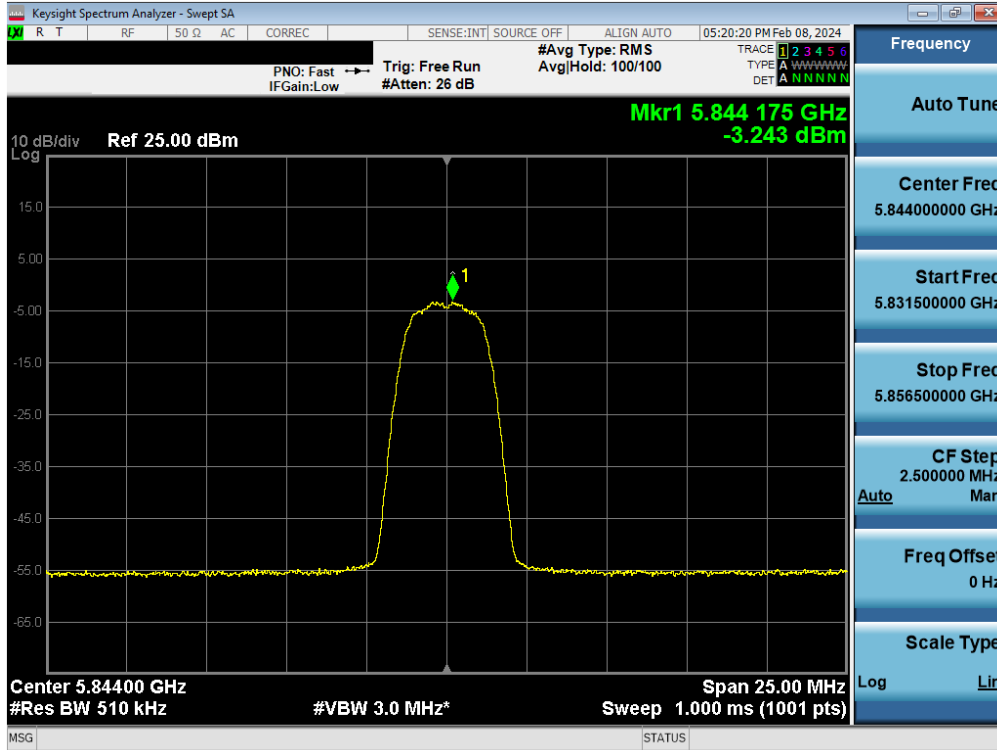
Plot 7-111. PSD Antenna WF7 (HDR4, iPA 5844MHz)
