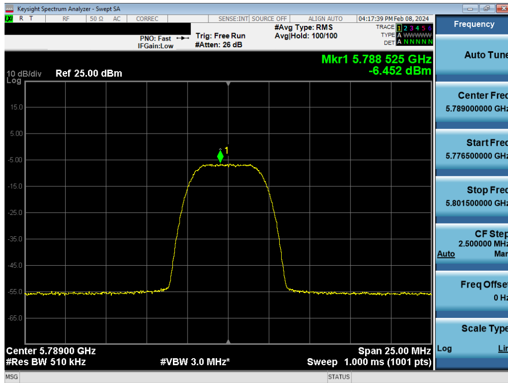
Plot 7-92. PSD Antenna WF8 (HDR8, iPA 5789MHz)
