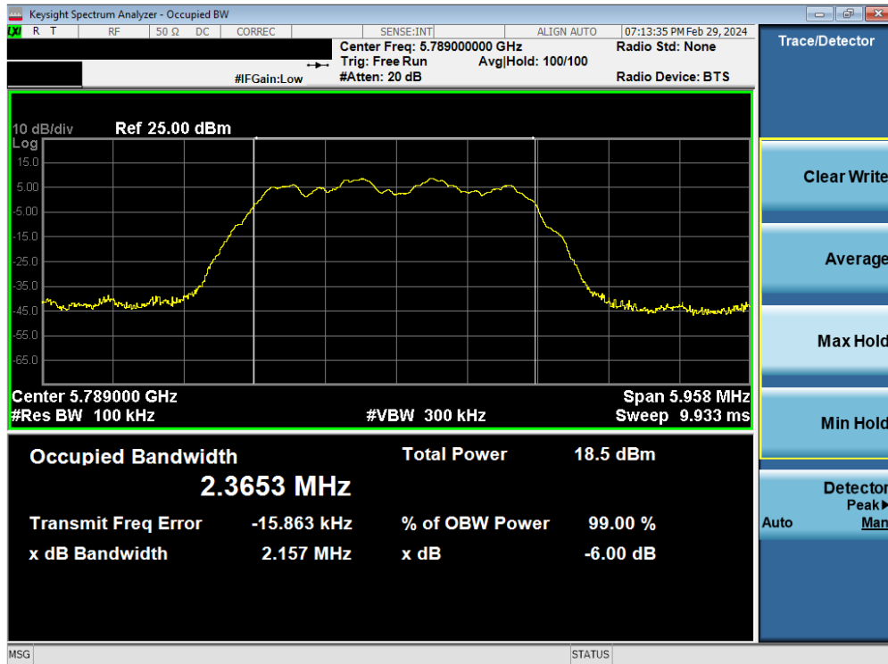
Plot 7-26. 6dB BW & 99% OBW Antenna WF8 (HDR4, ePA, 5789MHz)
