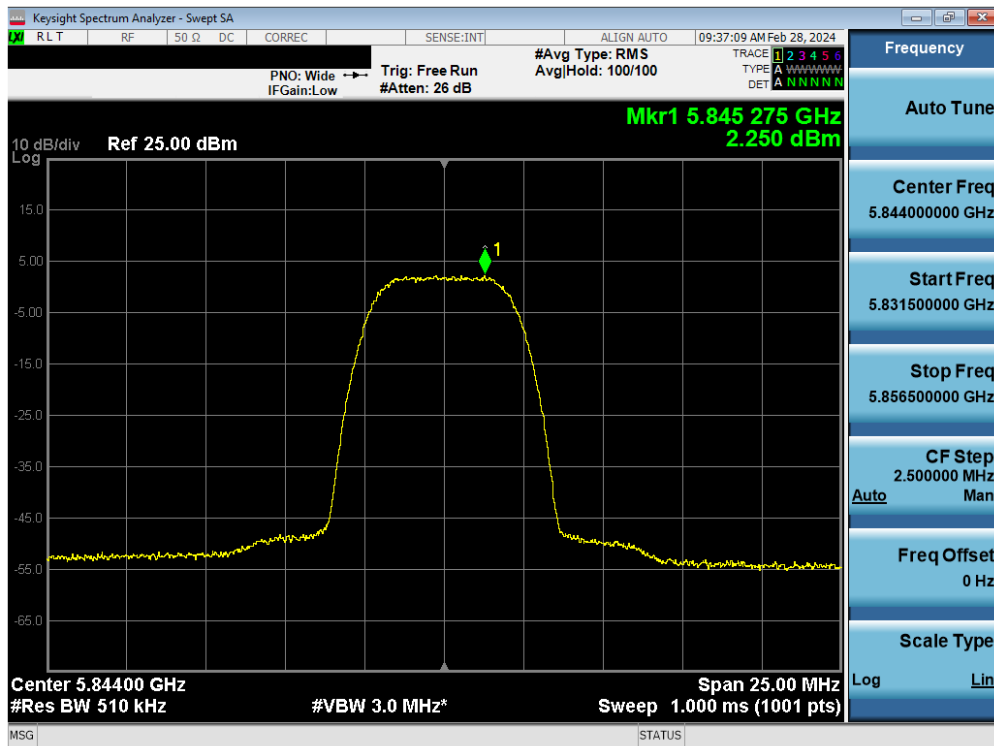
Plot 7-90. PSD Antenna WF8 (HDR8, ePA 5844MHz)
