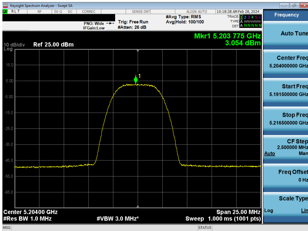
Plot 7-101. PSD Antenna WF7 (HDR8, ePA – 5204MHz)
