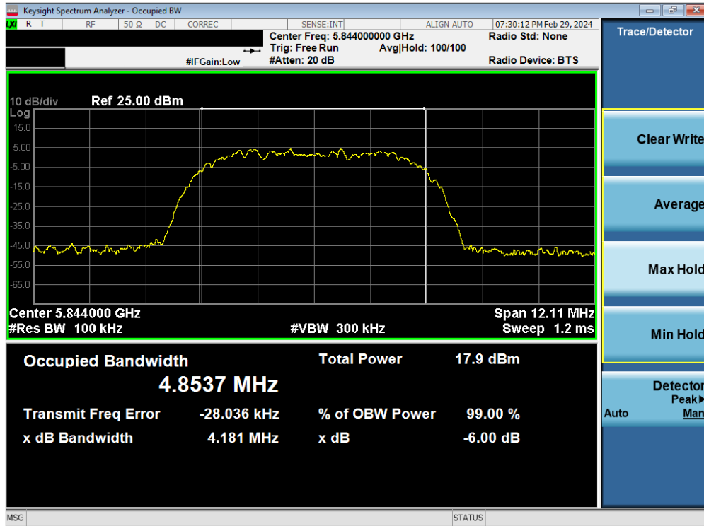
Plot 7-36. 6dB BW & 99% OBW Antenna WF7 (HDR8, ePA, 5844MHz)
