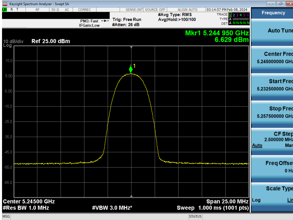
Plot 7-122. FCC PSD TxBF Antenna WF5B (HDR4, ePA- 5245MHz)
