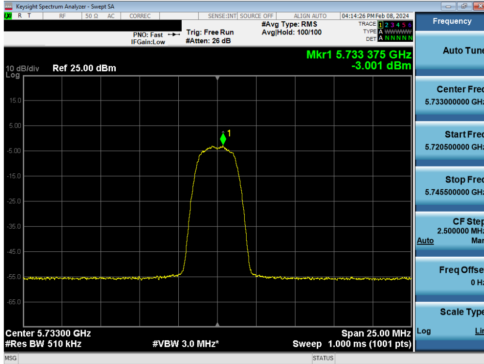
Plot 7-85. PSD Antenna WF8 (HDR4, iPA 5733MHz)
