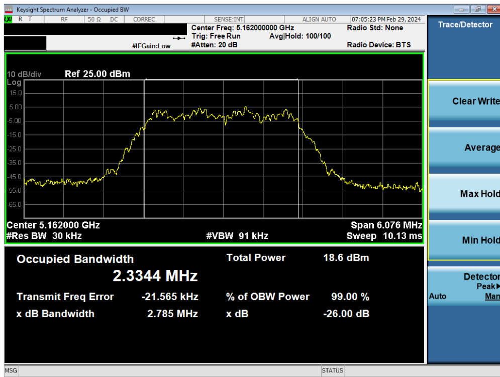
Plot 7-7. 26dB BW & 99% OBW Antenna WF8 (HDR4, ePA– 5162MHz)
