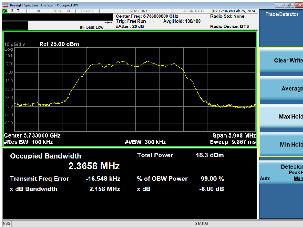
Plot 7-25. 6dB BW & 99% OBW Antenna WF8 (HDR4, ePA, 5733MHz)
