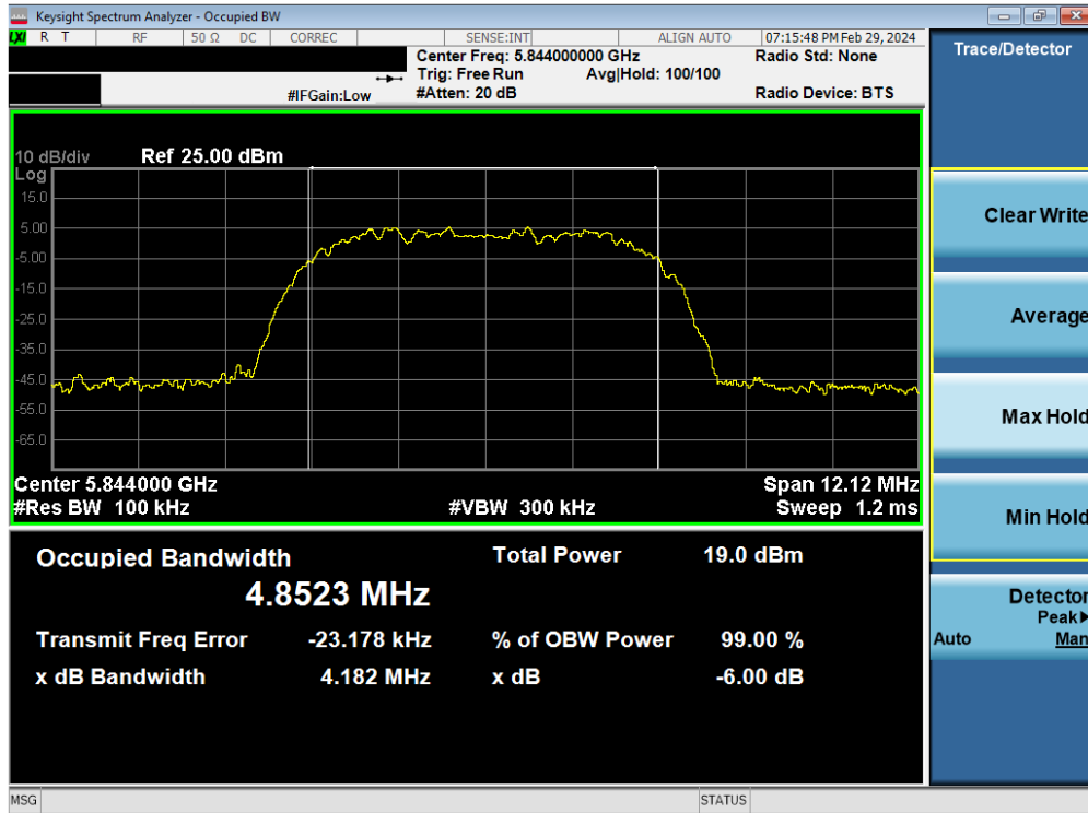
Plot 7-30. 6dB BW & 99% OBW Antenna WF8 (HDR8, ePA, 5844MHz)
