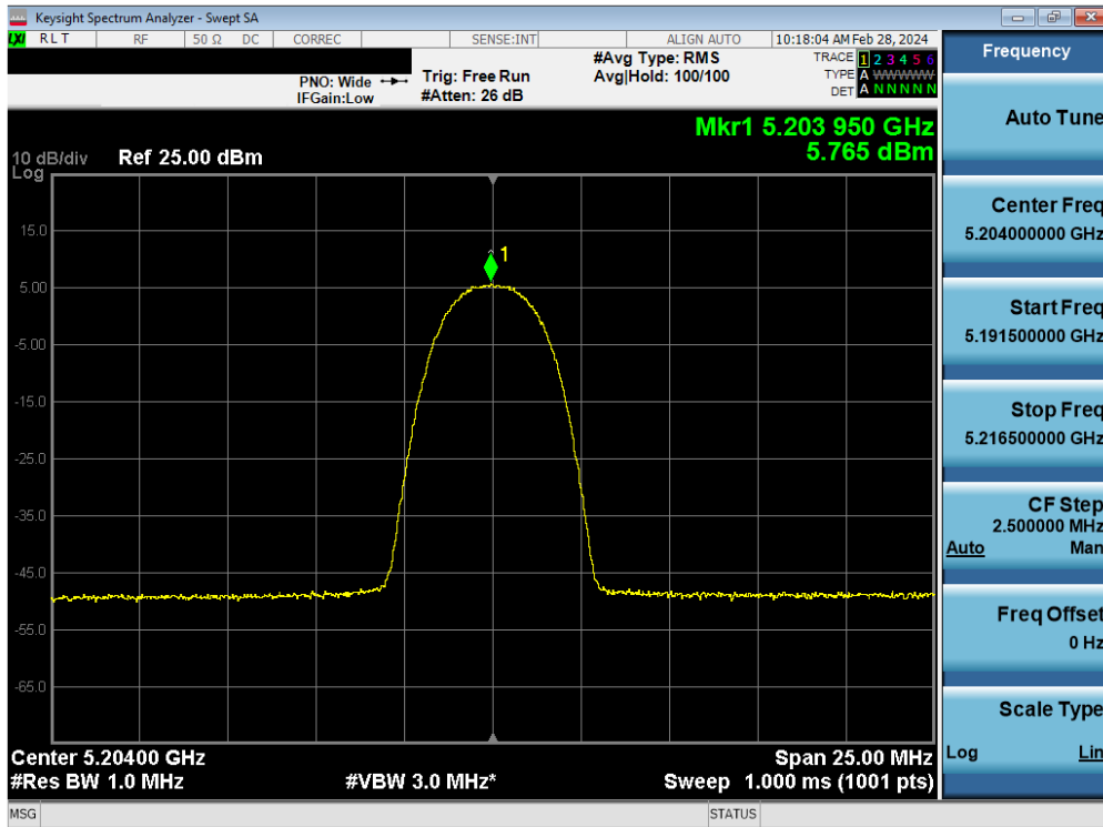
Plot 7-95. PSD Antenna WF7 (HDR4, ePA – 5204MHz)
