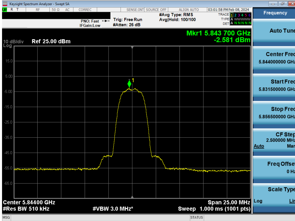
Plot 7-60. PSD Antenna WF5B (HDR4, iPA 5844MHz)
