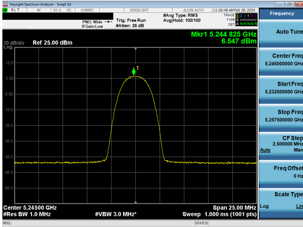
Plot 7-81. ISED PSD Antenna WF8 (HDR4, ePA- 5245MHz)
