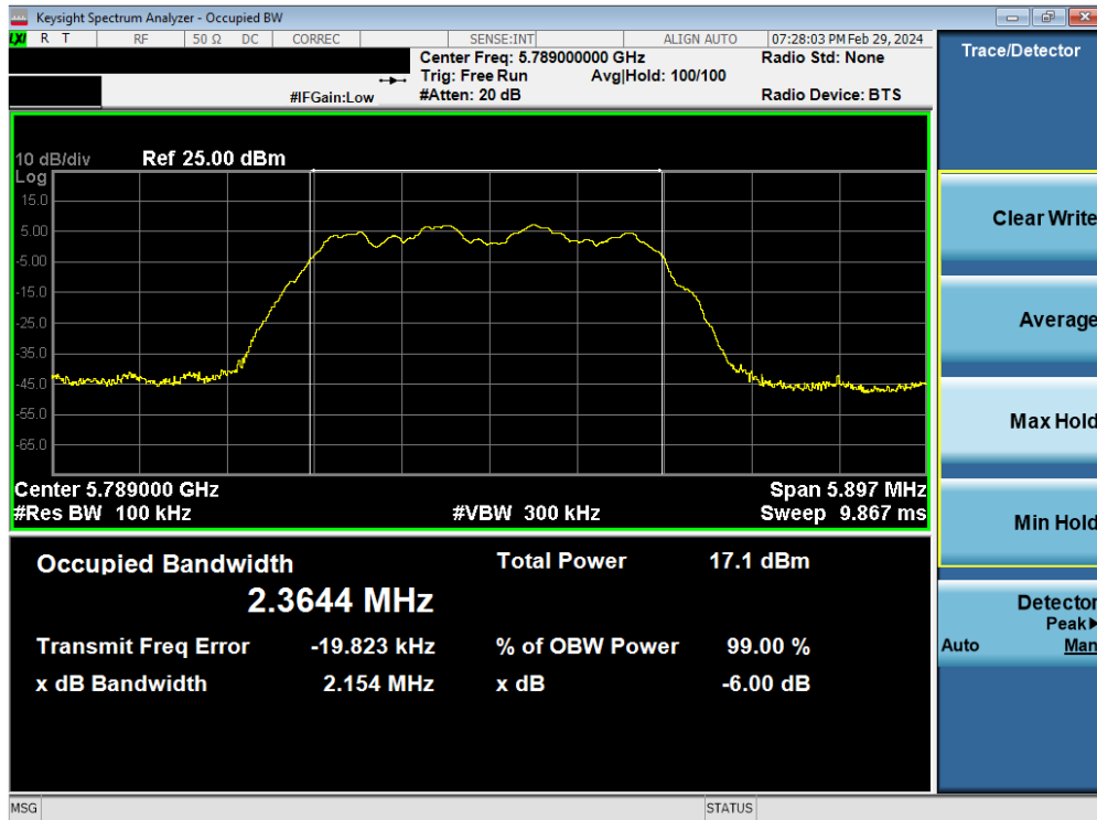
Plot 7-32. 6dB BW & 99% OBW Antenna WF7 (HDR4, ePA, 5789MHz)
