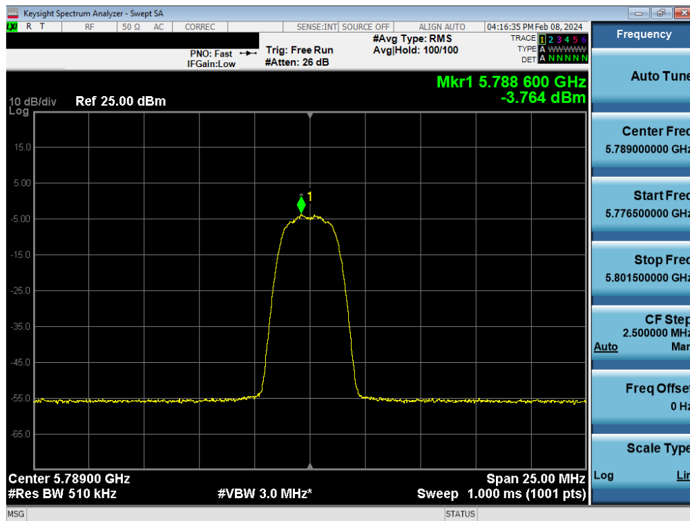
Plot 7-86. PSD Antenna WF8 (HDR4, iPA 5789MHz)
