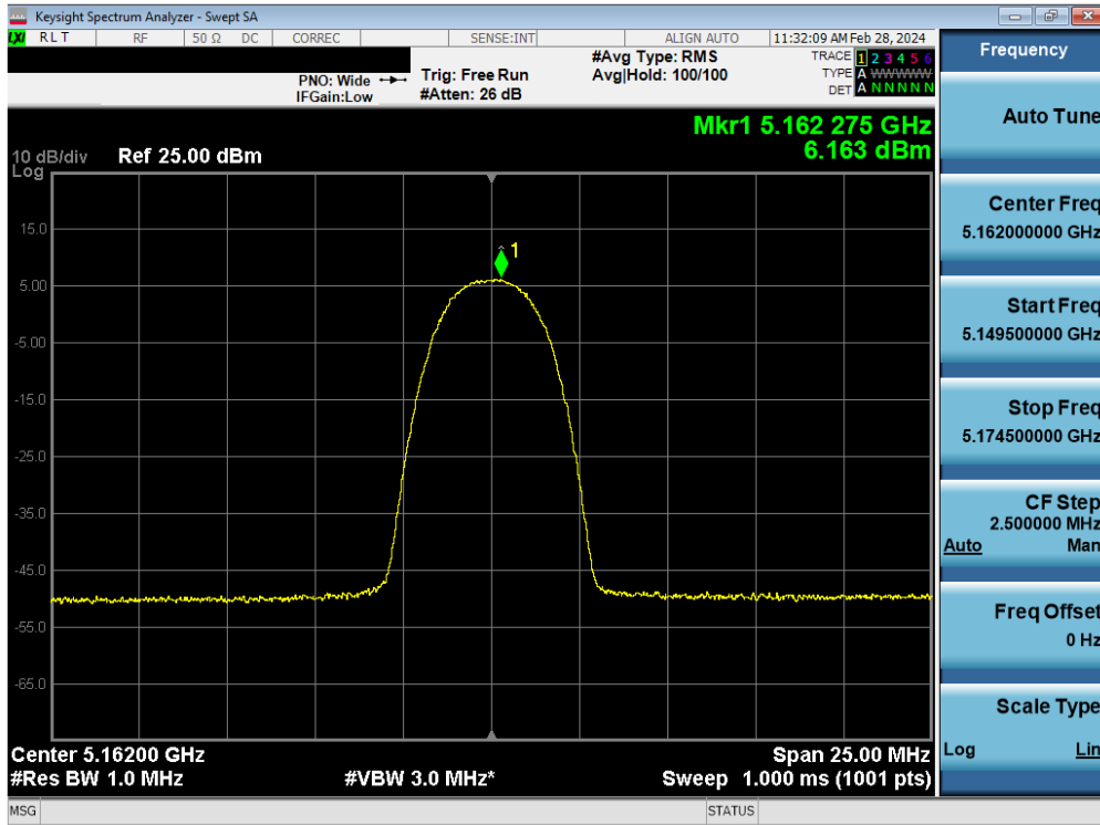
Plot 7-79. ISED PSD Antenna WF8 (HDR4, ePA – 5162MHz)
