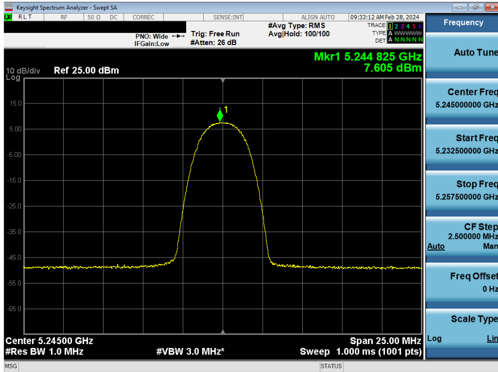
Plot 7-69. FCC PSD Antenna WF8 (HDR4, ePA- 5245MHz)
