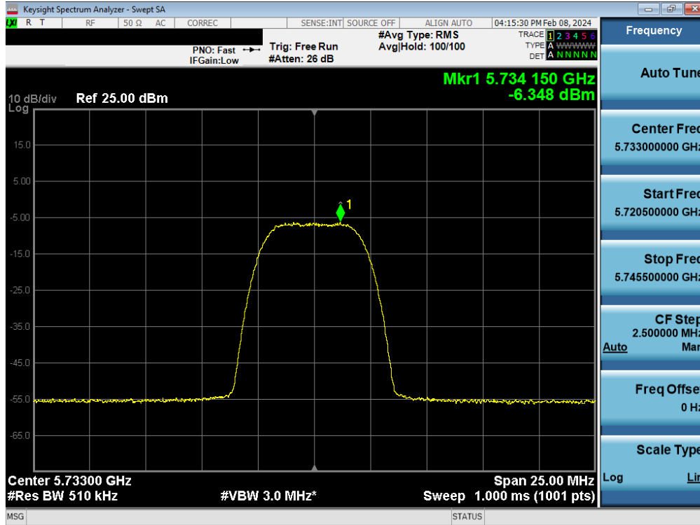
Plot 7-91. PSD Antenna WF8 (HDR8, iPA 5733MHz)
