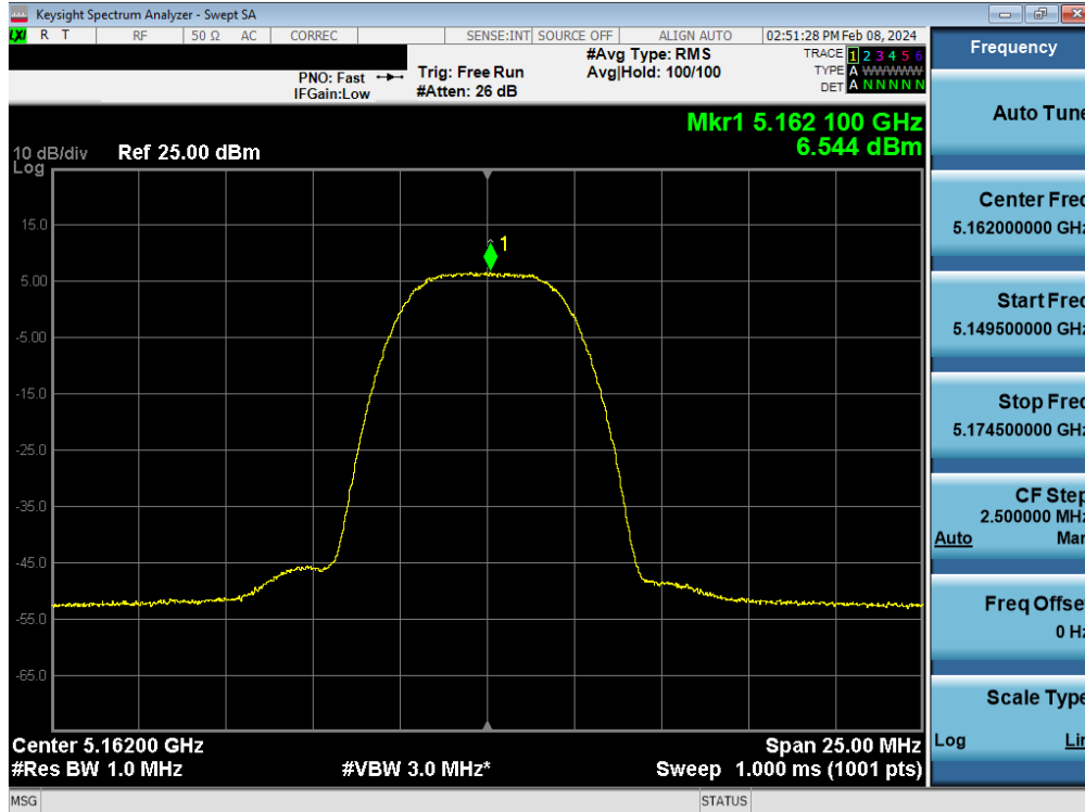
Plot 7-43. FCC PSD Antenna WF5B (HDR8, ePA - 5162MHz)
