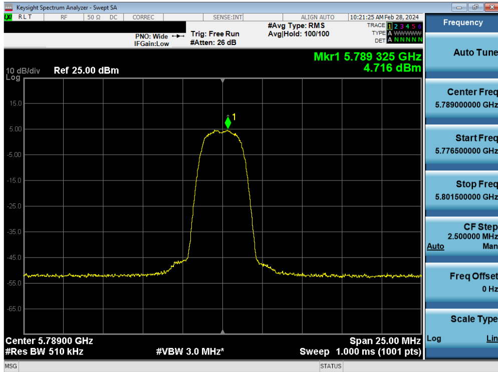
Plot 7-107. PSD Antenna WF7 (HDR4, ePA 5789MHz)
