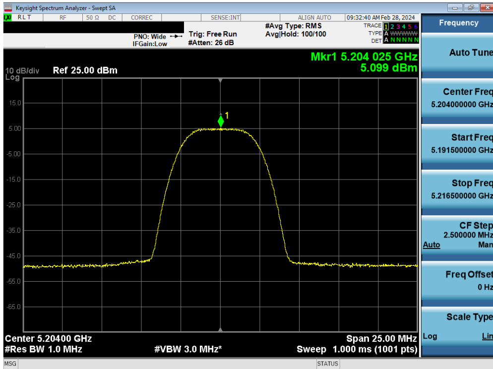
Plot 7-74. FCC/ISED PSD Antenna WF8 (HDR8, ePA – 5204MHz)
