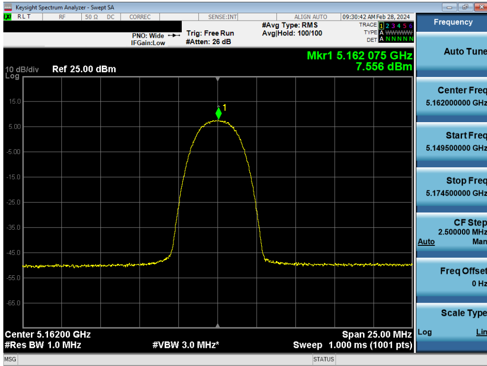
Plot 7-67. FCC PSD Antenna WF8 (HDR4, ePA – 5162MHz)
