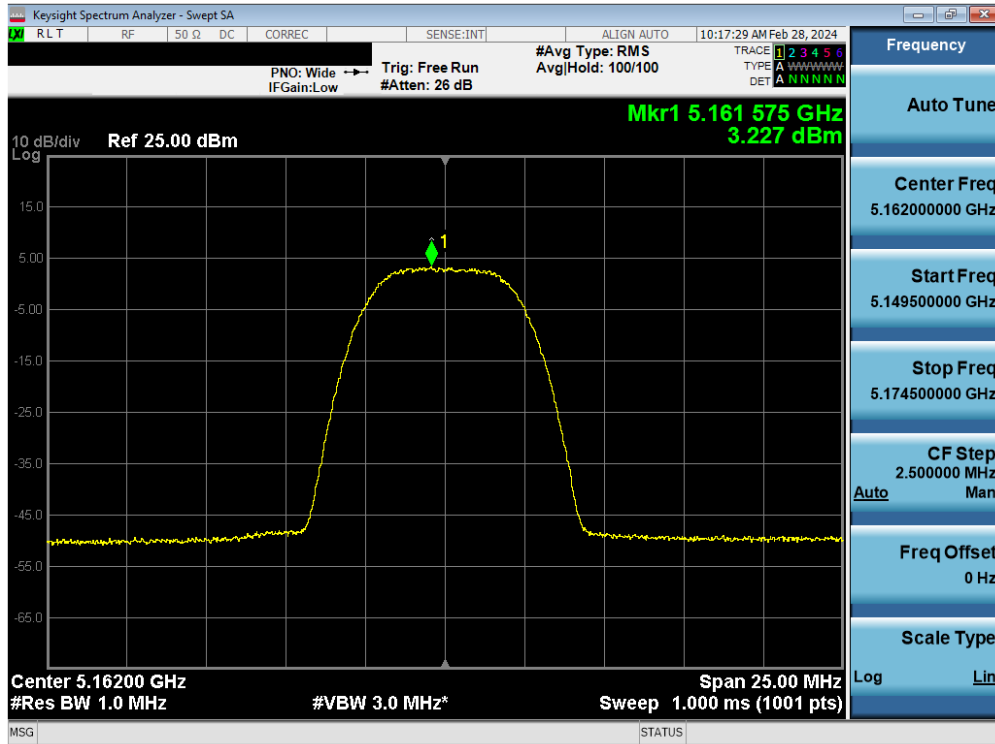
Plot 7-100. PSD Antenna WF7 (HDR8, ePA – 5162MHz)
