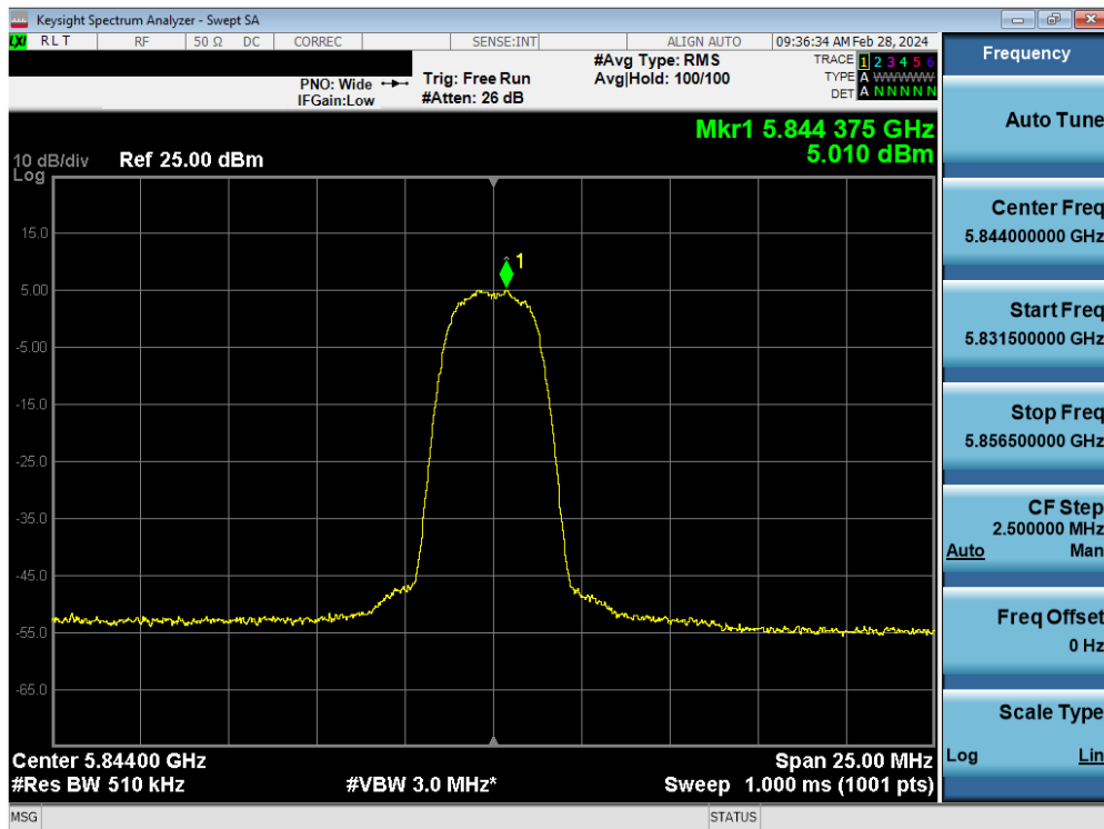
Plot 7-84. PSD Antenna WF8 (HDR4, ePA 5844MHz)
