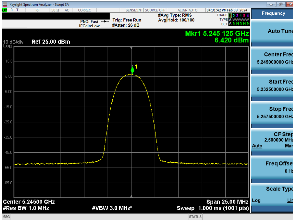
Plot 7-123. FCC PSD TxBF Antenna WF8 (HDR4, ePA- 5245MHz)
