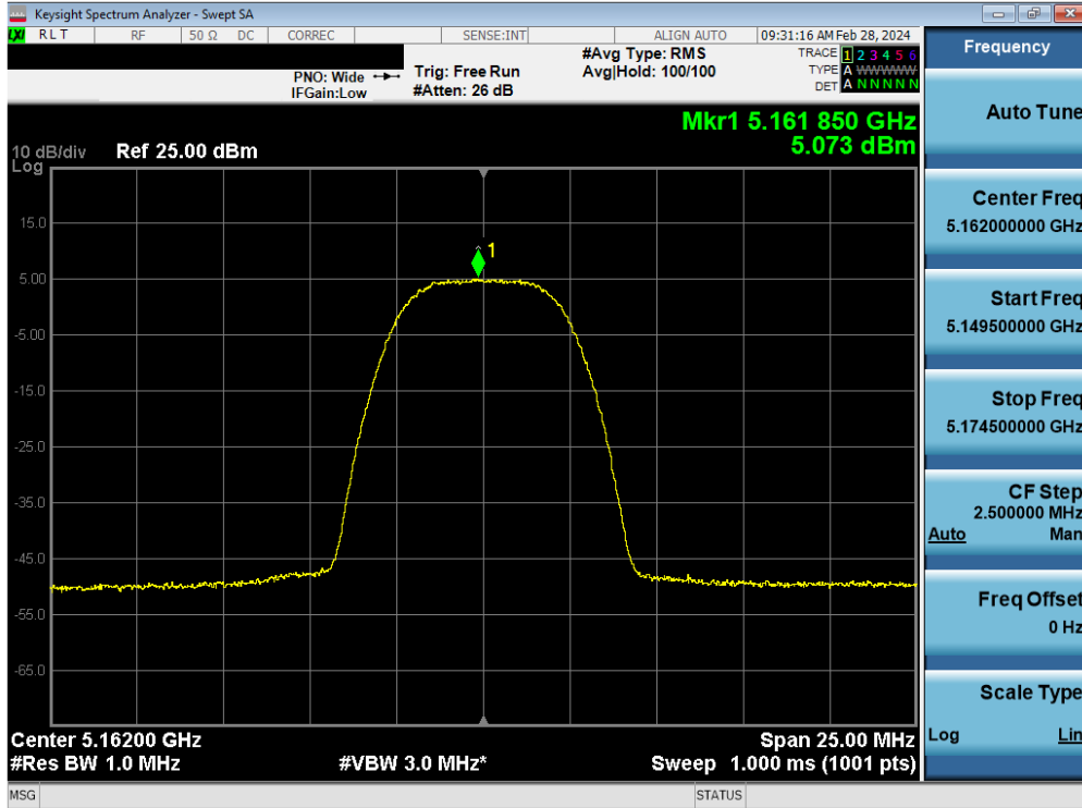
Plot 7-73. FCC/ISED PSD Antenna WF8 (HDR8, ePA – 5162MHz)
