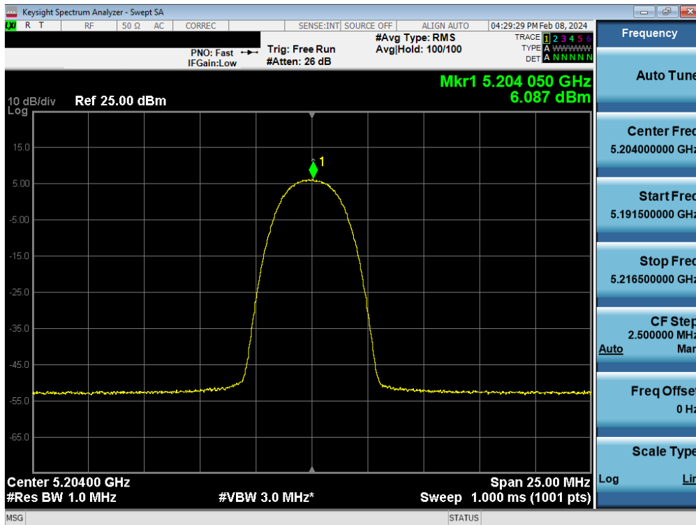
Plot 7-121. FCC PSD TxBF Antenna WF8 (HDR4, ePA – 5204MHz)
