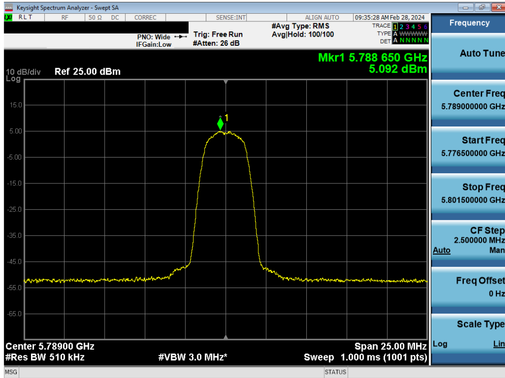
Plot 7-83. PSD Antenna WF8 (HDR4, ePA 5789MHz)
