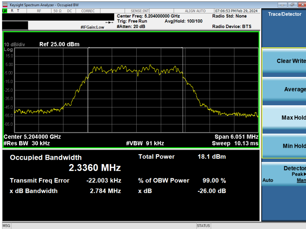
Plot 7-8. 26dB BW & 99% OBW Antenna WF8 (HDR4, ePA- 5204MHz)
