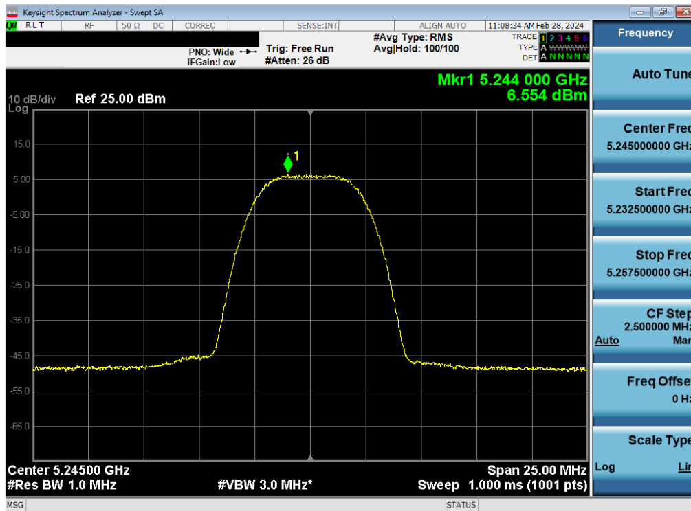
Plot 7-54. ISED PSD Antenna WF5B (HDR8, ePA– 5245MHz)
