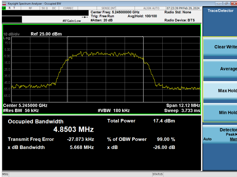
Plot 7-18. 26dB BW & 99% OBW Antenna WF7 (HDR8, ePA- 5245MHz)
