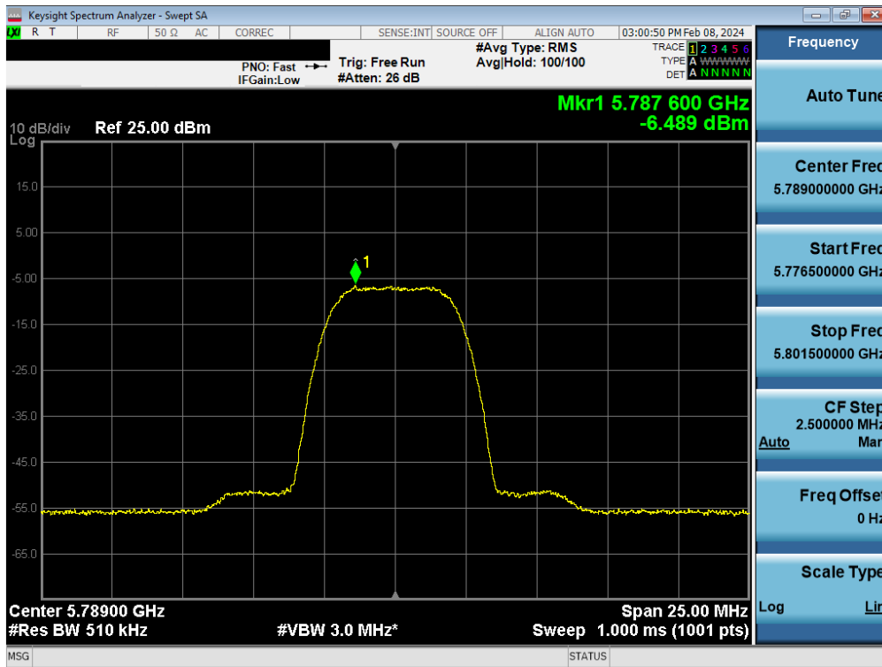
Plot 7-65. PSD Antenna WF5B (HDR8, iPA 5789MHz)
