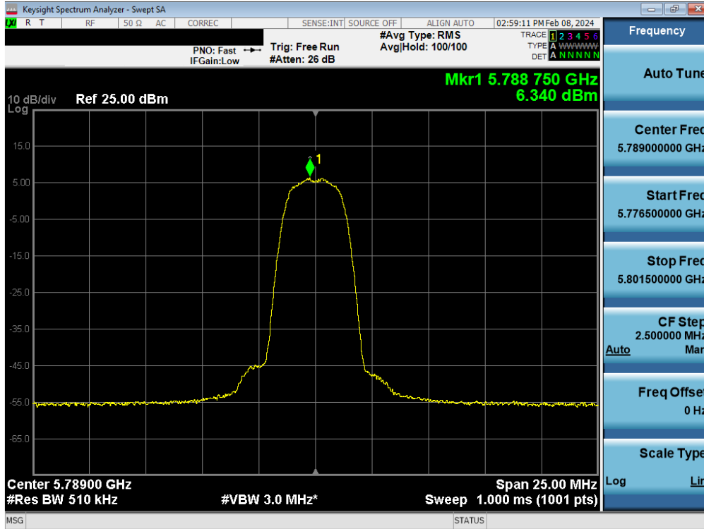
Plot 7-56. PSD Antenna WF5B (HDR4, ePA 5789MHz)
