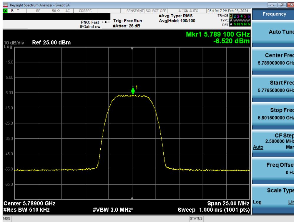
Plot 7-116. PSD Antenna WF7 (HDR8, iPA 5789MHz)
