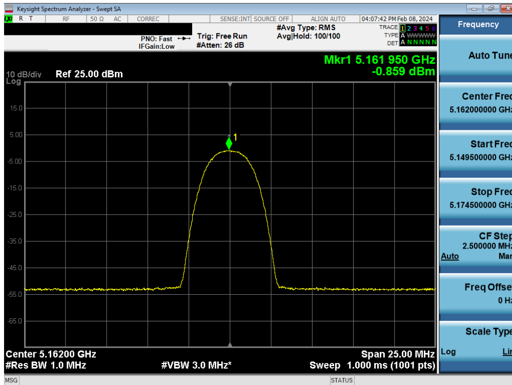
Plot 7-70. FCC/ISED PSD Antenna WF8 (HDR4, iPA - 5162MHz)
