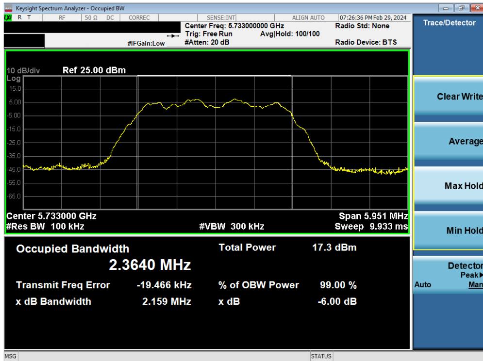
Plot 7-31. 6dB BW & 99% OBW Antenna WF7 (HDR4, ePA, 5733MHz)
