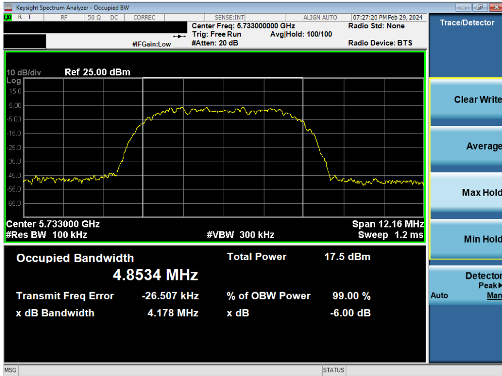
Plot 7-34. 6dB BW & 99% OBW Antenna WF7 (HDR8, ePA, 5733MHz)
