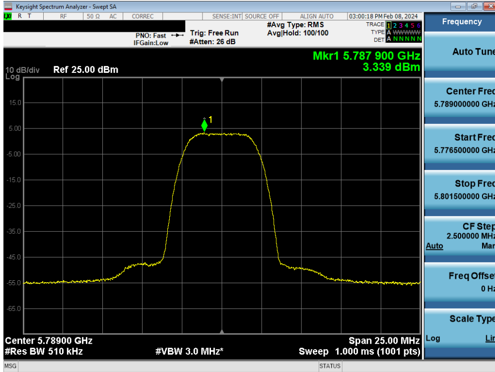
Plot 7-62. PSD Antenna WF5B (HDR8, ePA 5789MHz)
