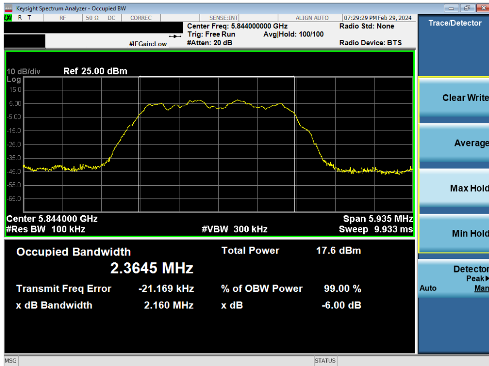
Plot 7-33. 6dB BW & 99% OBW Antenna WF7 (HDR4, ePA, 5844MHz)
