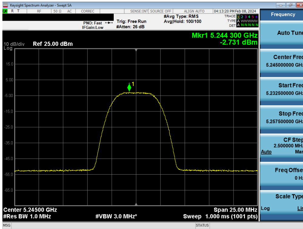
Plot 7-78. FCC/ISED PSD Antenna WF8 (HDR8, iPA– 5245MHz)
