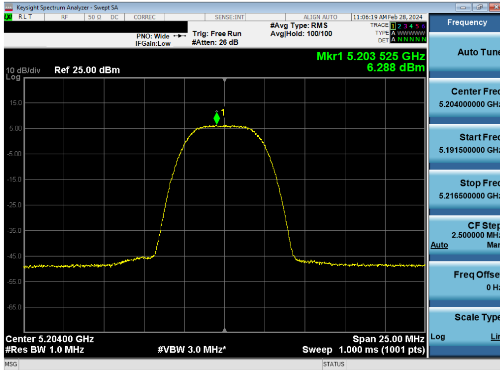
Plot 7-53. ISED PSD Antenna WF5B (HDR8, ePA – 5204MHz)
