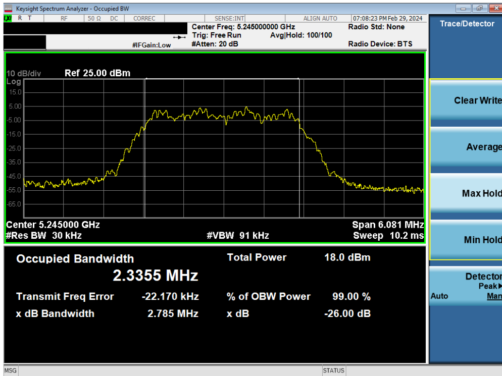
Plot 7-9. 26dB BW & 99% OBW Antenna WF8 (HDR4, ePA- 5245MHz)
