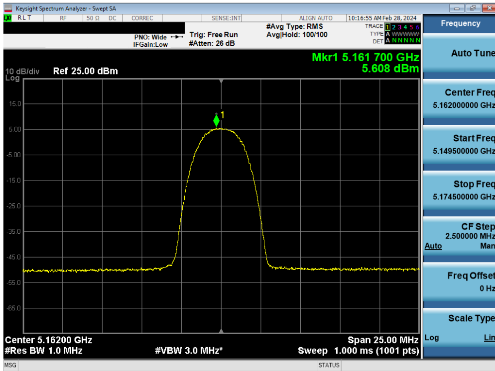
Plot 7-94. PSD Antenna WF7 (HDR4, ePA – 5162MHz)
