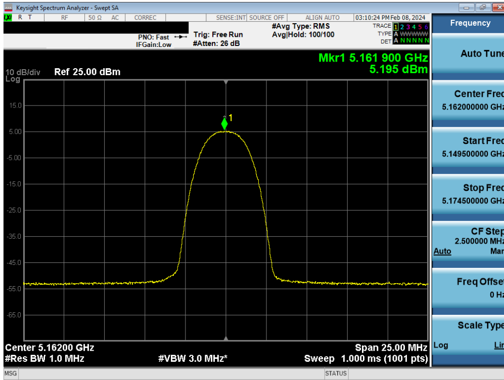
Plot 7-118. FCC PSD TxBF Antenna WF5B (HDR4, ePA – 5162MHz)
