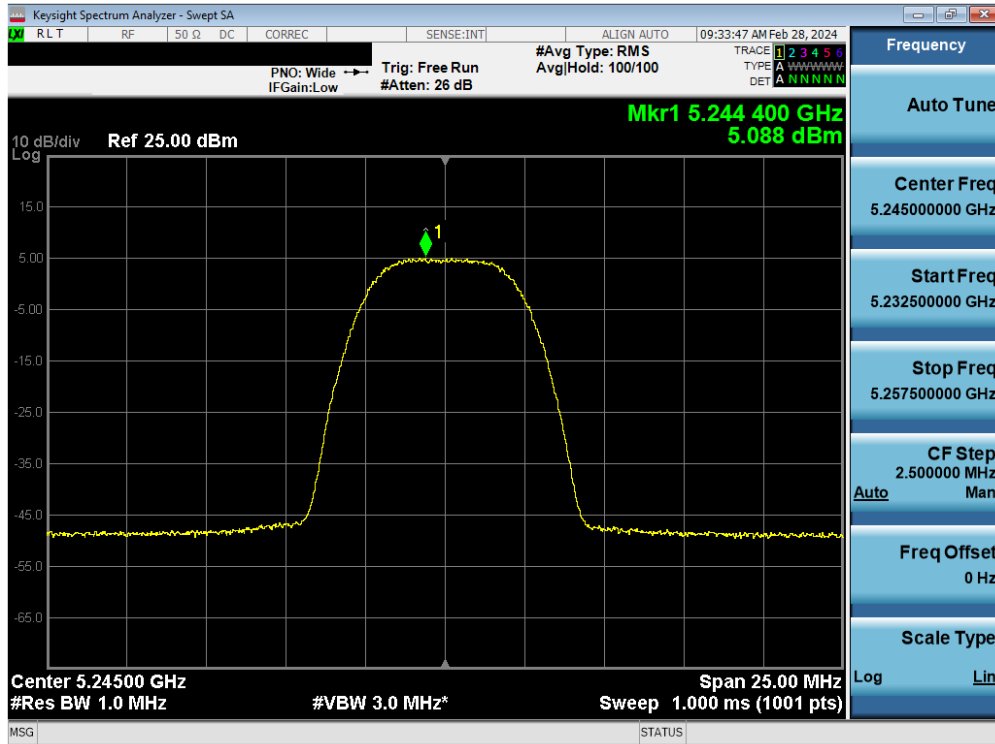
Plot 7-75. FCC/ISED PSD Antenna WF8 (HDR8, ePA– 5245MHz)
