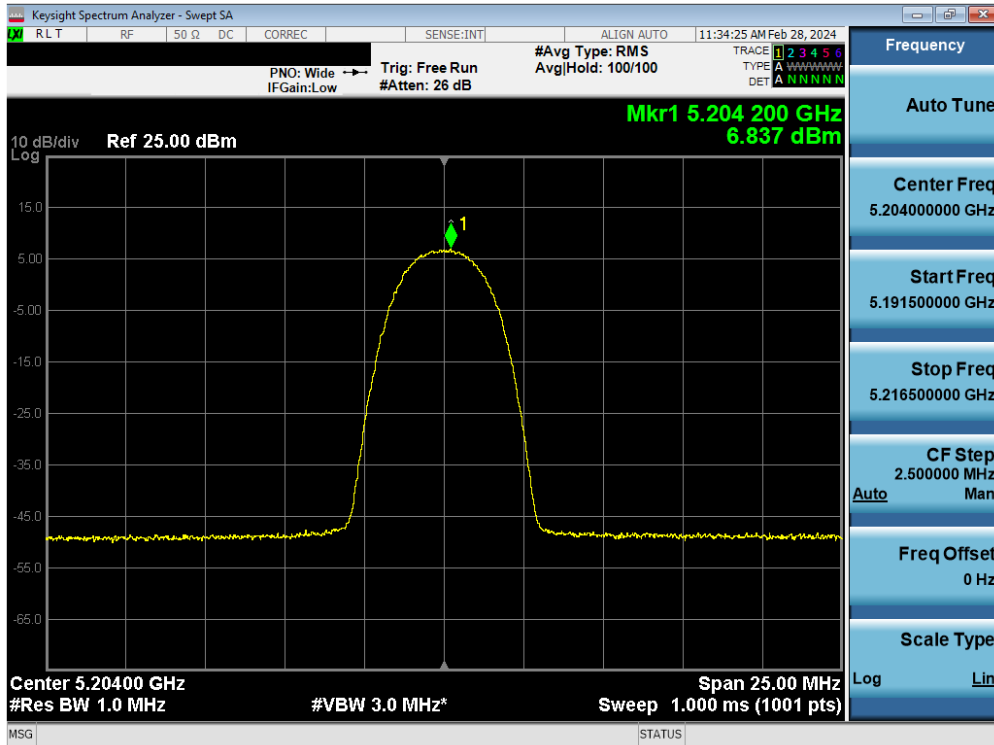
Plot 7-80. ISED PSD Antenna WF8 (HDR4, ePA – 5204MHz)
