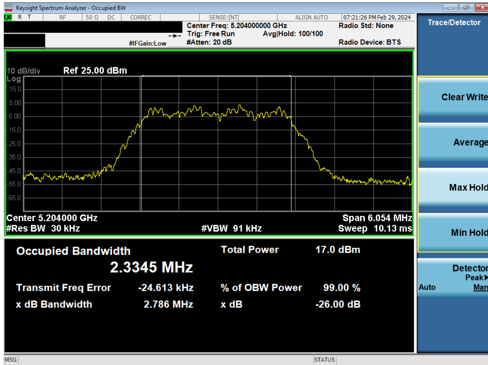
Plot 7-14. 26dB BW & 99% OBW Antenna WF7 (HDR4, ePA- 5204MHz)
