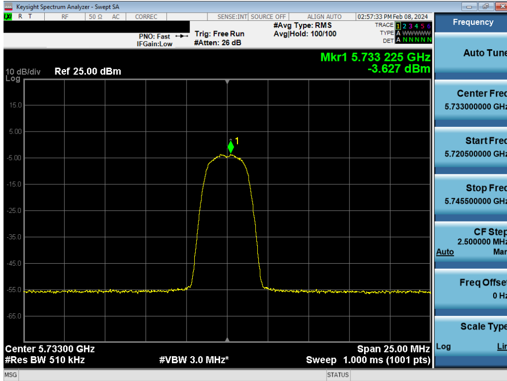
Plot 7-58. PSD Antenna WF5B (HDR4, iPA 5733MHz)
