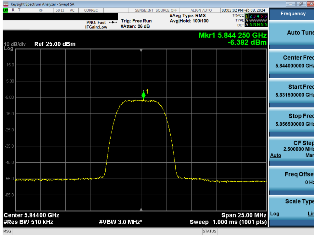
Plot 7-66. PSD Antenna WF5B (HDR8, iPA 5844MHz)
