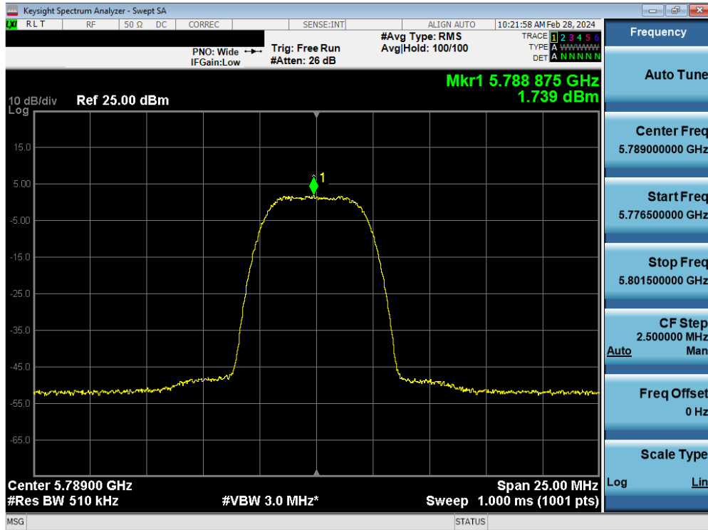
Plot 7-113. PSD Antenna WF7 (HDR8, ePA 5789MHz)
