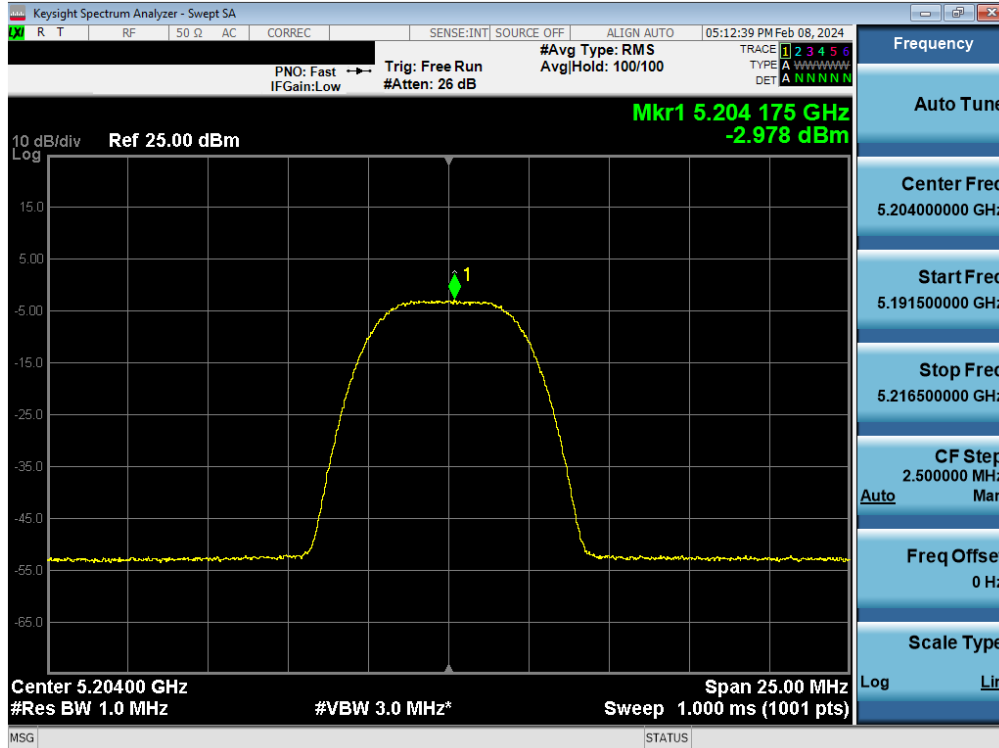
Plot 7-104. PSD Antenna WF7 (HDR8, iPA – 5204MHz)
