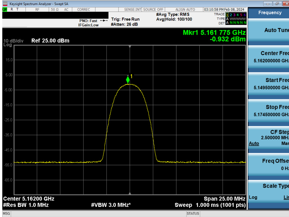
Plot 7-124. FCC/ISED PSD TxBF Antenna WF5B (HDR4, iPA - 5162MHz)
