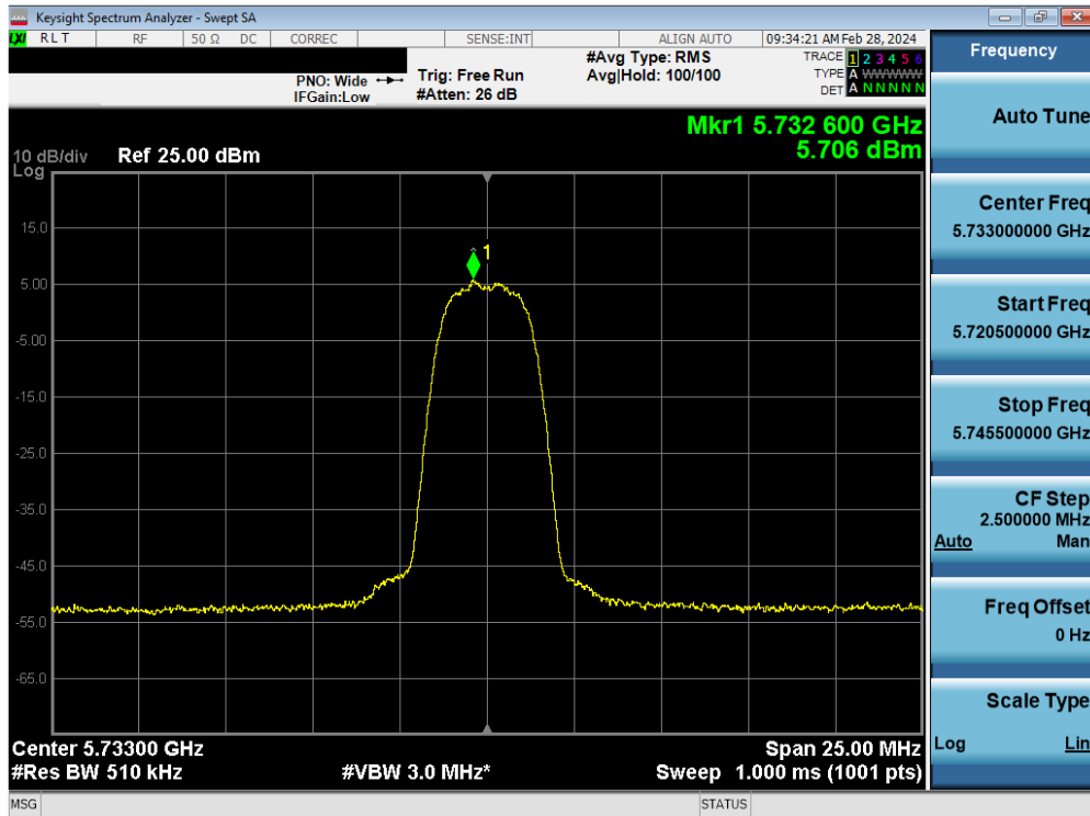
Plot 7-82. PSD Antenna WF8 (HDR4, ePA 5733MHz)
