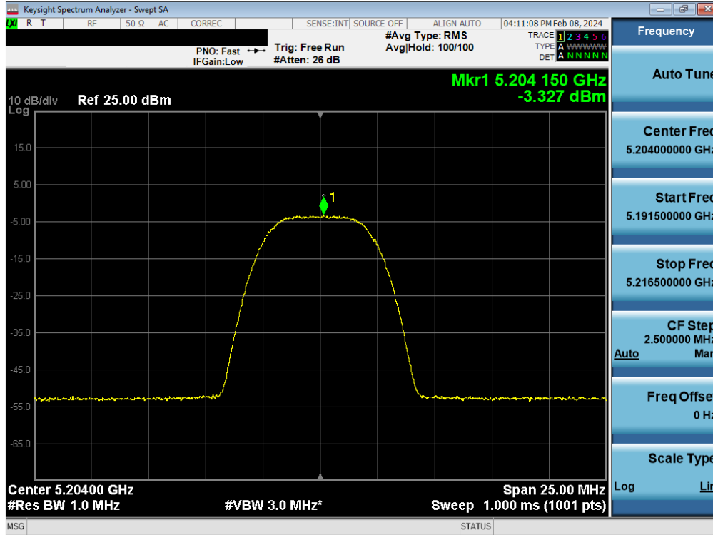
Plot 7-77. FCC/ISED PSD Antenna WF8 (HDR8, iPA – 5204MHz)
