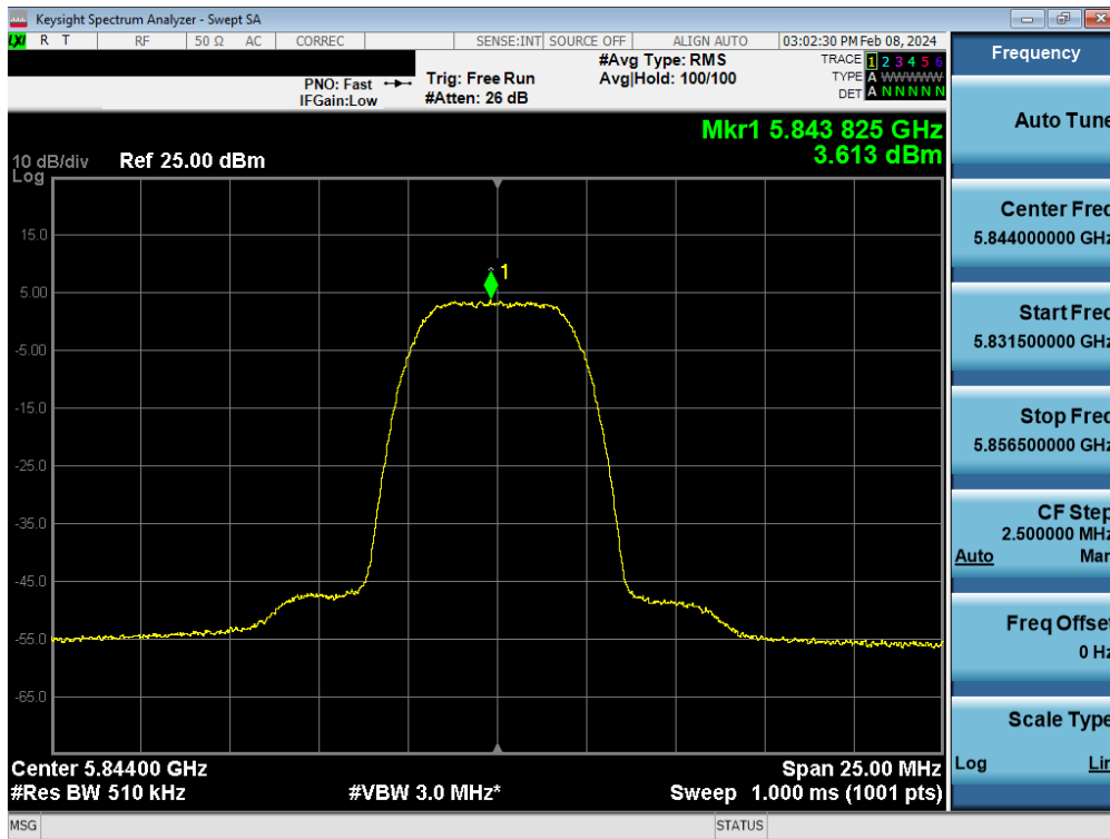
Plot 7-63. PSD Antenna WF5B (HDR8, ePA 5844MHz)
