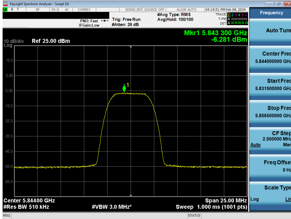
Plot 7-93. PSD Antenna WF8 (HDR8, iPA 5844MHz)
