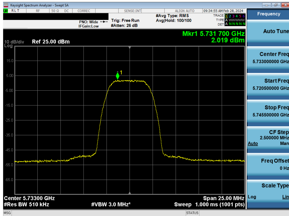
Plot 7-88. PSD Antenna WF8 (HDR8, ePA 5733MHz)
