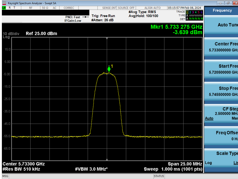
Plot 7-109. PSD Antenna WF7 (HDR4, iPA 5733MHz)
