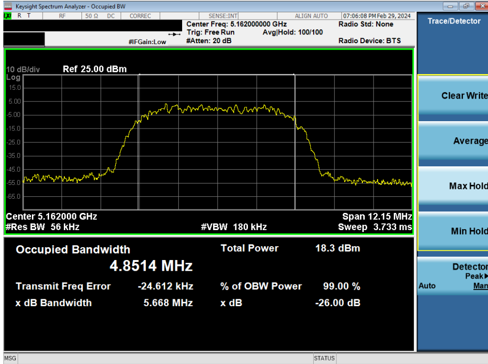
Plot 7-10. 26dB BW & 99% OBW Antenna WF8 (HDR8, ePA- 5162MHz)
