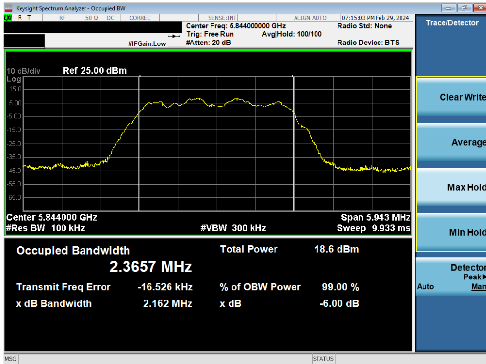
Plot 7-27. 6dB BW & 99% OBW Antenna WF8 (HDR4, ePA, 5844MHz)
