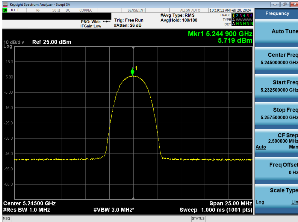
Plot 7-96. PSD Antenna WF7 (HDR4, ePA– 5245MHz)
