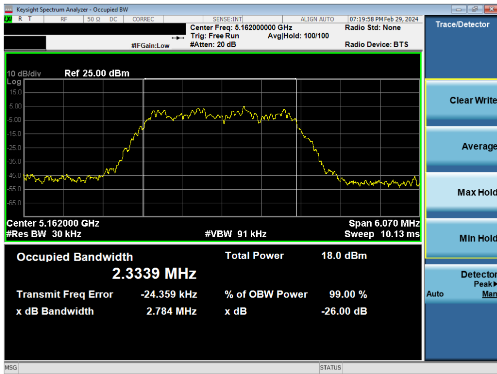
Plot 7-13. 26dB BW & 99% OBW Antenna WF7 (HDR4, ePA– 5162MHz)
