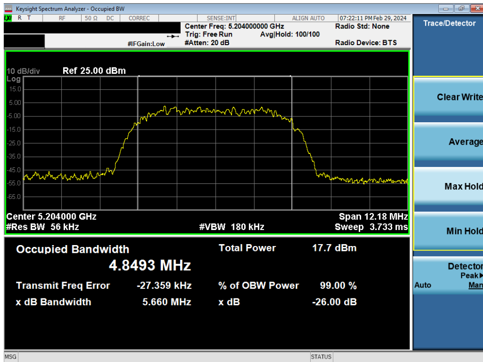
Plot 7-17. 26dB BW & 99% OBW Antenna WF7 (HDR8, ePA- 5204MHz)
