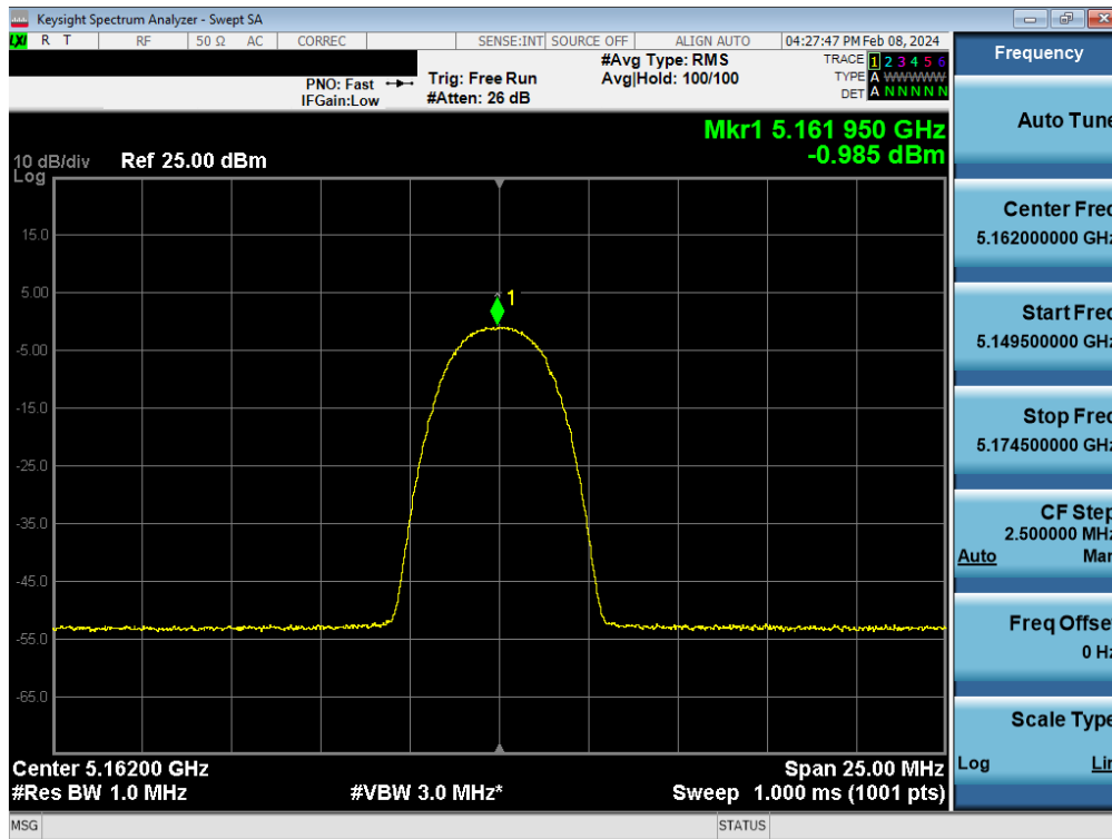
Plot 7-125. FCC/ISED PSD TxBF Antenna WF8 (HDR4, iPA - 5162MHz)
