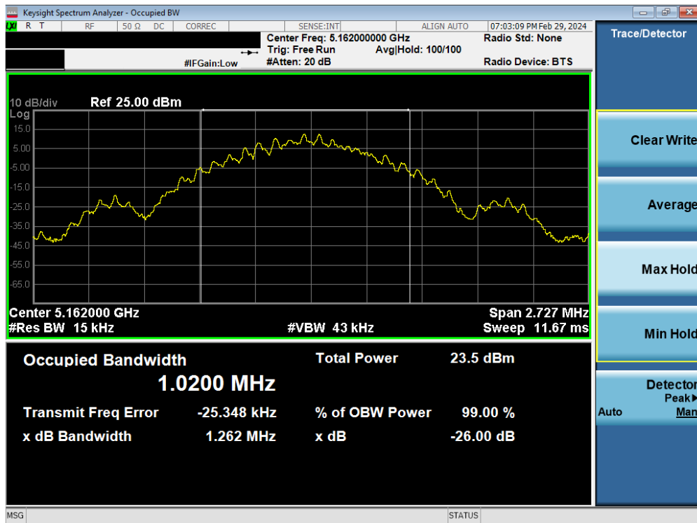
Plot 7-4. 26dB BW & 99% OBW Antenna WF8 (BDR GFSK, ePA– 5162MHz)
