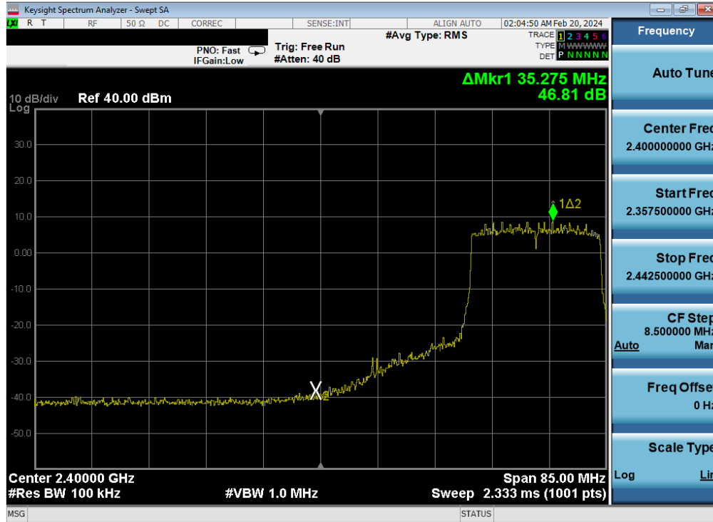
Plot 7-354. Band Edge Plot Antenna WF8 (802.11ax (SU - 2.4GHz) – Ch. 5) – MCS9
