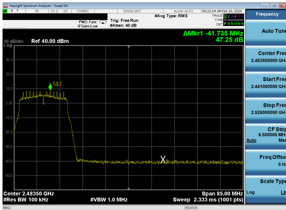
Plot 7-372. Band Edge Plot Antenna WF7 (802.11n (2.4GHz) – Ch. 9) – MCS2
