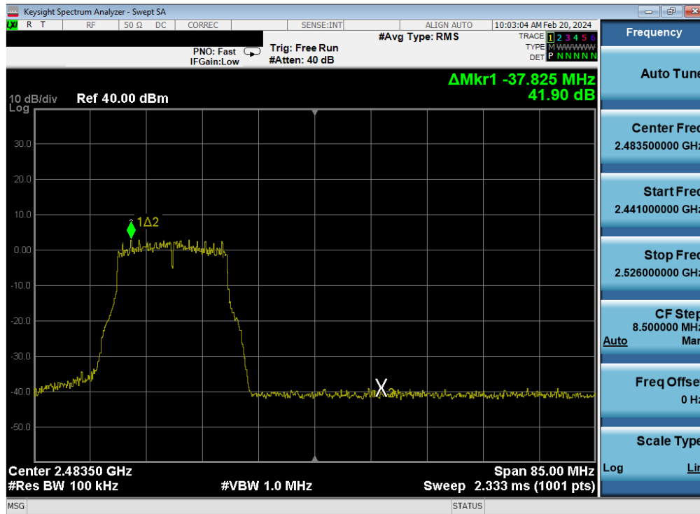
Plot 7-396. Band Edge Plot Antenna WF7 (802.11g – Ch. 11) – 24Mbps
