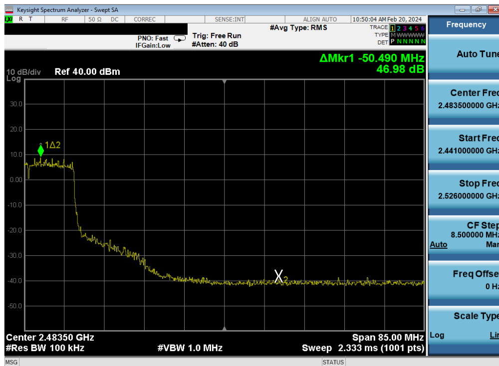
Plot 7-454. Band Edge Plot Antenna WF7 (802.11ax (SU - 2.4GHz) – Ch. 7) – MCS9
