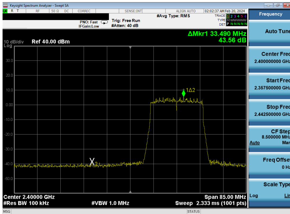
Plot 7-351. Band Edge Plot Antenna WF8 (802.11ax (SU - 2.4GHz) – Ch. 2) – MCS9
