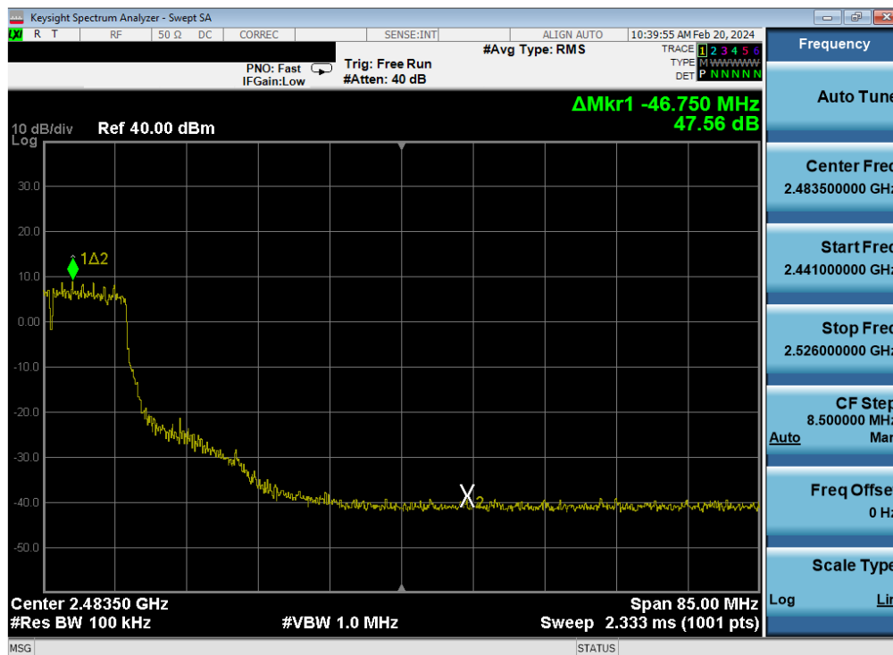
Plot 7-442. Band Edge Plot Antenna WF7 (802.11n (2.4GHz) – Ch. 7) – MCS7
