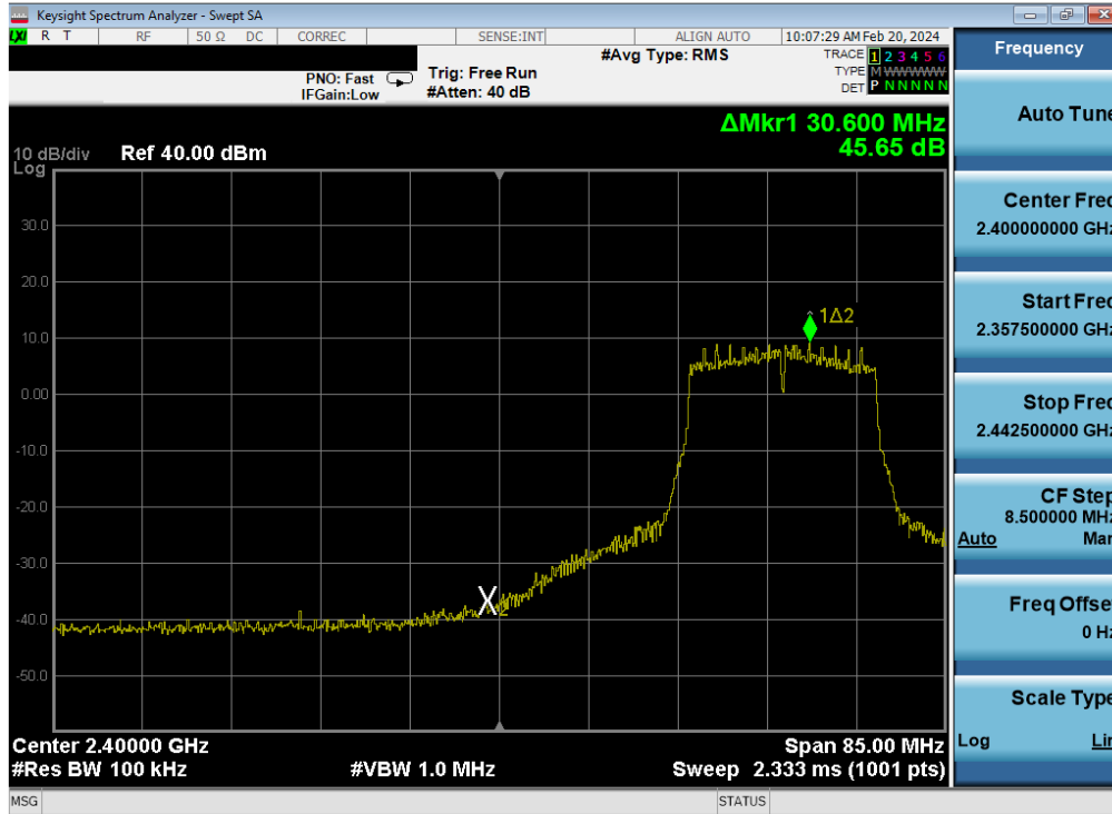
Plot 7-402. Band Edge Plot Antenna WF7 (802.11n (2.4GHz) – Ch. 4) – MCS4
