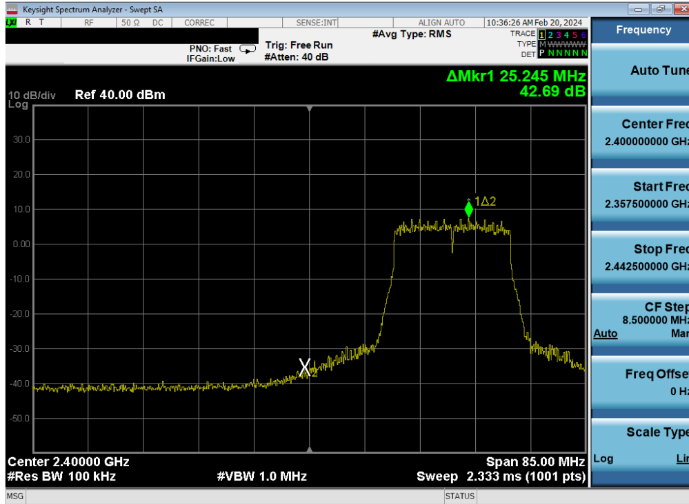
Plot 7-439. Band Edge Plot Antenna WF7 (802.11n (2.4GHz) – Ch. 3) – MCS7
