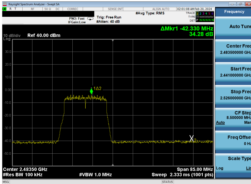
Plot 7-349. Band Edge Plot Antenna WF8 (802.11n (2.4GHz) – Ch. 13) – MCS7
