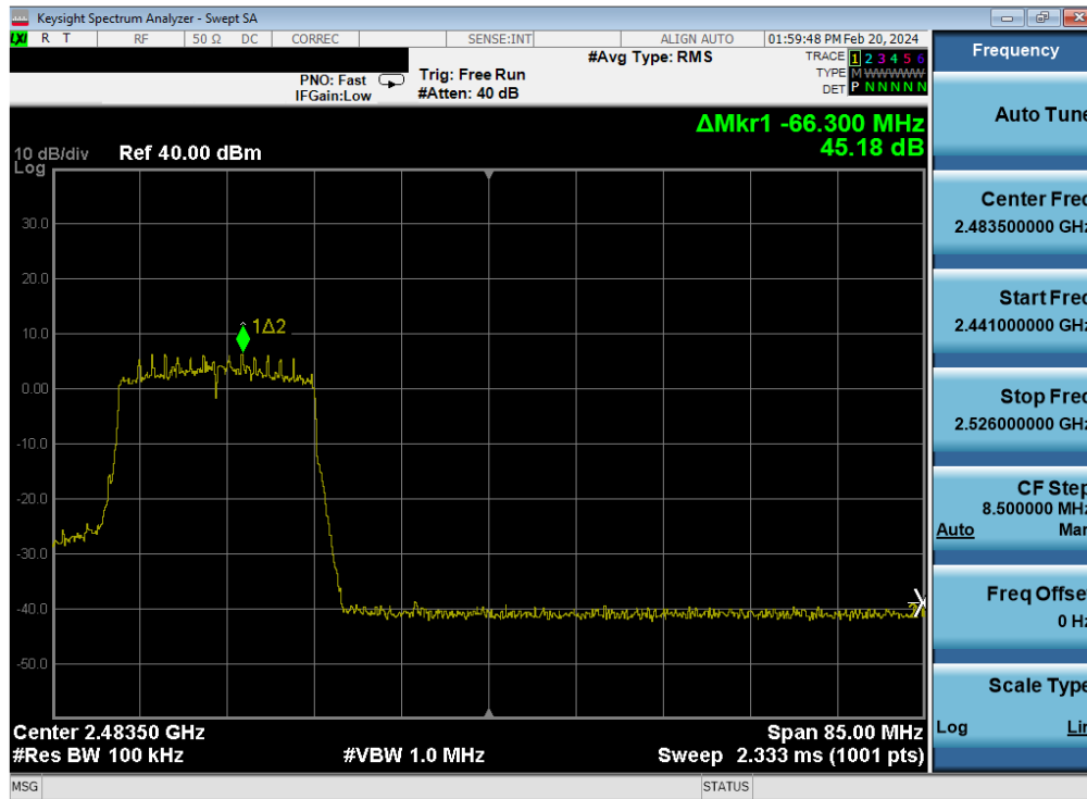
Plot 7-484. Band Edge Plot Antenna WF9 (802.11ax (SU - 2.4GHz) – Ch. 10) – MCS2
