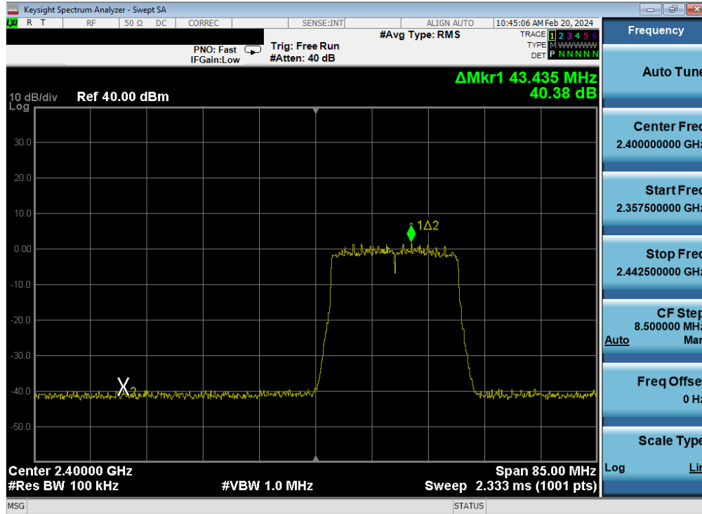
Plot 7-449. Band Edge Plot Antenna WF7 (802.11ax (SU - 2.4GHz) – Ch. 1) – MCS9
