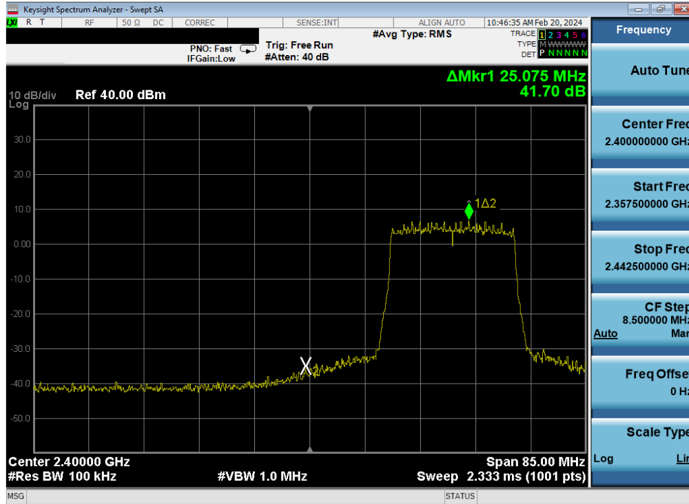
Plot 7-451. Band Edge Plot Antenna WF7 (802.11ax (SU - 2.4GHz) – Ch. 3) – MCS9
