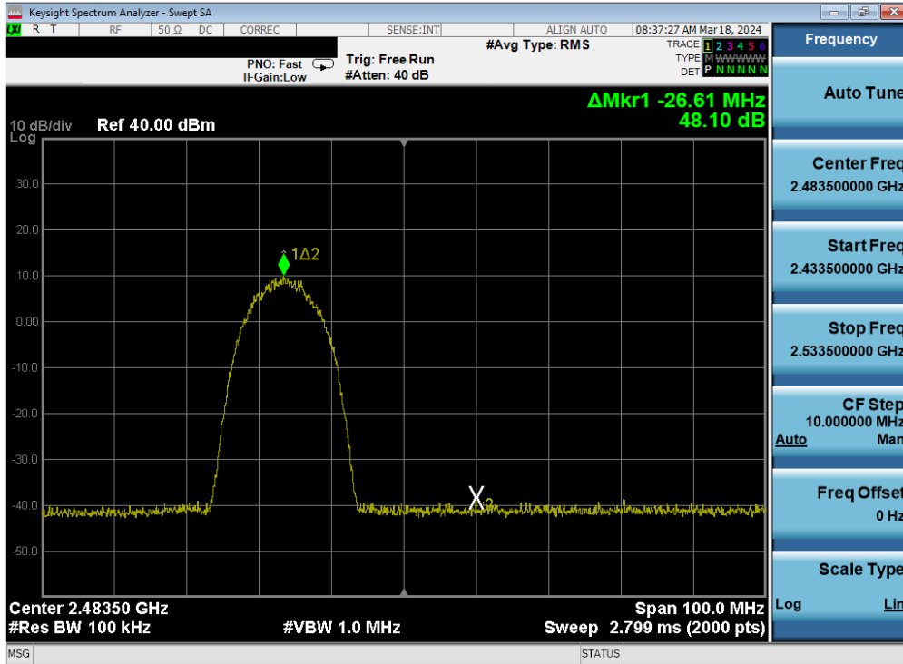
Plot 7-423. Band Edge Plot Antenna WF7 (802.11b – Ch. 12) – 11Mbps
