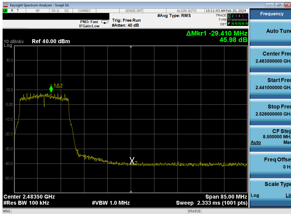
Plot 7-405. Band Edge Plot Antenna WF7 (802.11n (2.4GHz) – Ch. 9) – MCS4
