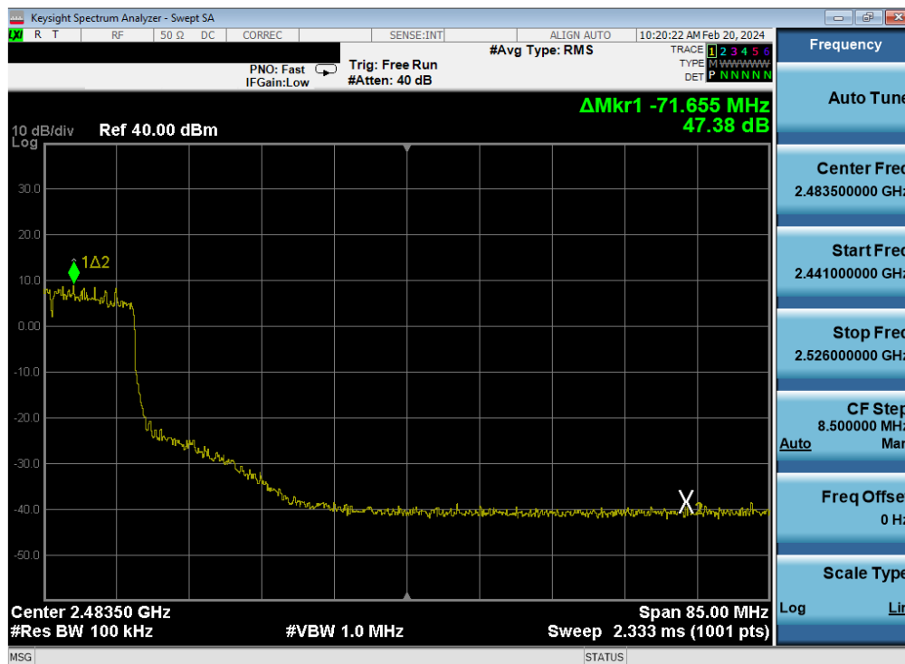
Plot 7-415. Band Edge Plot Antenna WF7 (802.11ax (SU - 2.4GHz) – Ch. 7) – MCS4
