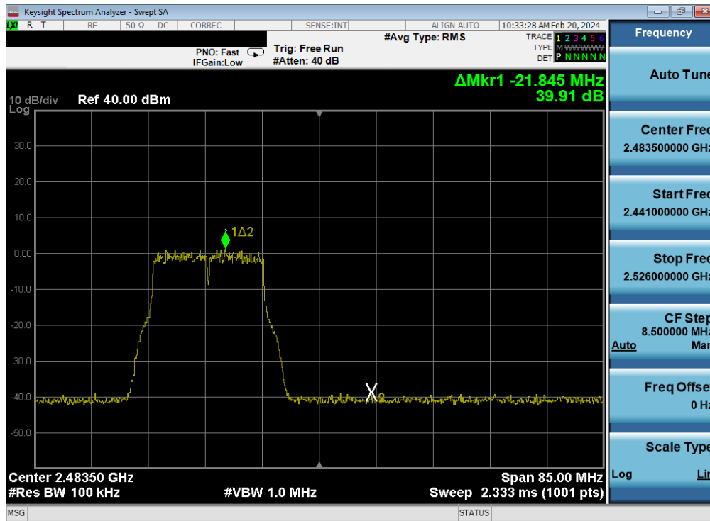
Plot 7-435. Band Edge Plot Antenna WF7 (802.11g – Ch. 12) – 54Mbps
