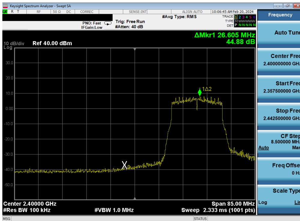
Plot 7-401. Band Edge Plot Antenna WF7 (802.11n (2.4GHz) – Ch. 3) – MCS4
