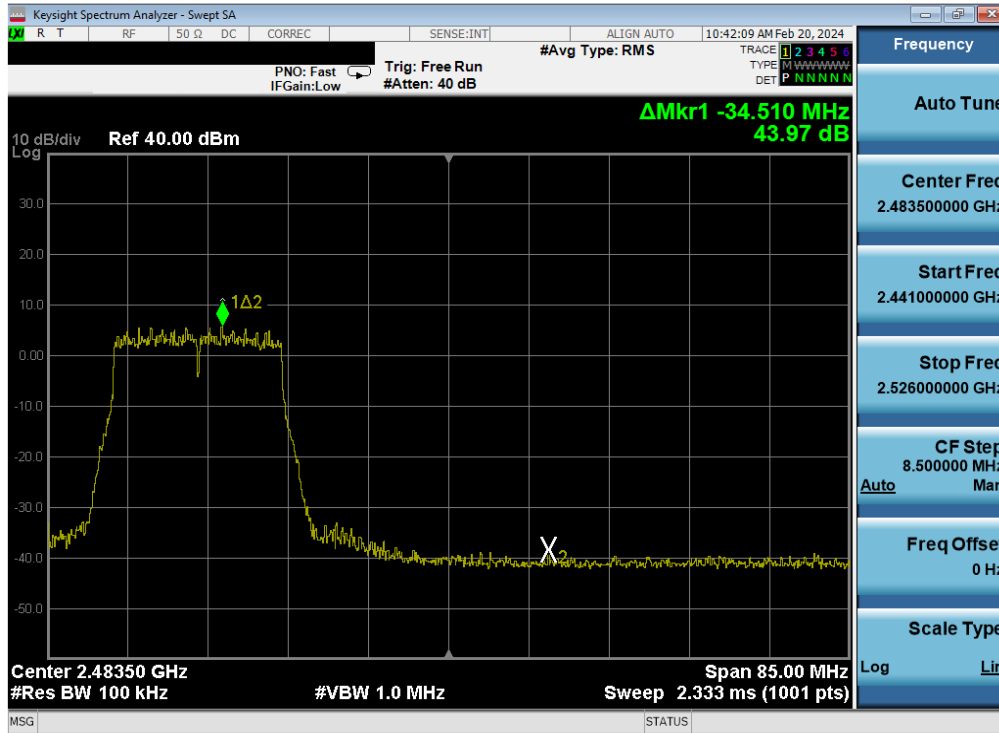
Plot 7-445. Band Edge Plot Antenna WF7 (802.11n (2.4GHz) – Ch. 10) – MCS7
