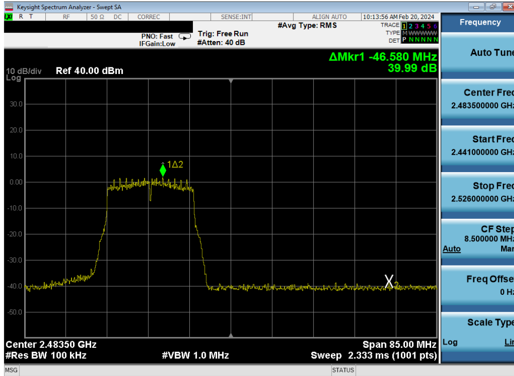
Plot 7-408. Band Edge Plot Antenna WF7 (802.11n (2.4GHz) – Ch. 12) – MCS4
