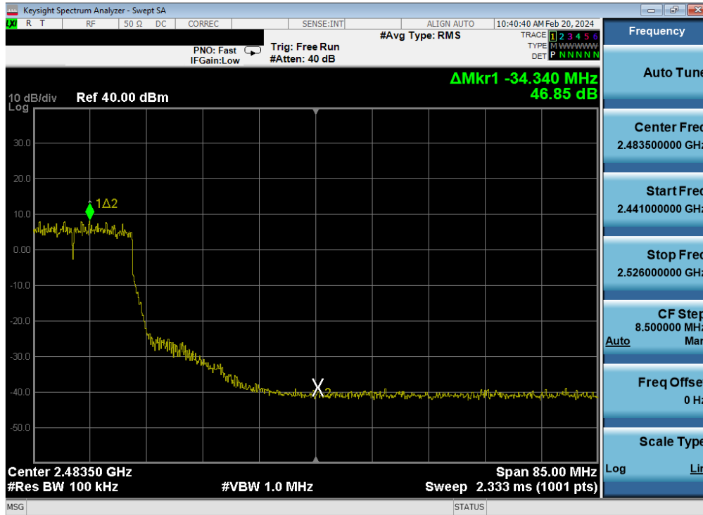
Plot 7-443. Band Edge Plot Antenna WF7 (802.11n (2.4GHz) – Ch. 8) – MCS7
