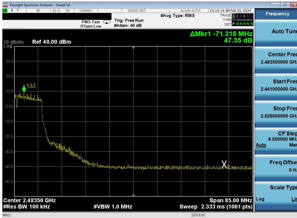
Plot 7-403. Band Edge Plot Antenna WF7 (802.11n (2.4GHz) – Ch. 7) – MCS4
