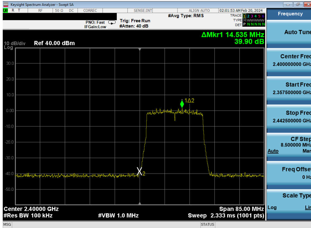
Plot 7-350. Band Edge Plot Antenna WF8 (802.11ax (SU - 2.4GHz) – Ch. 1) – MCS9
