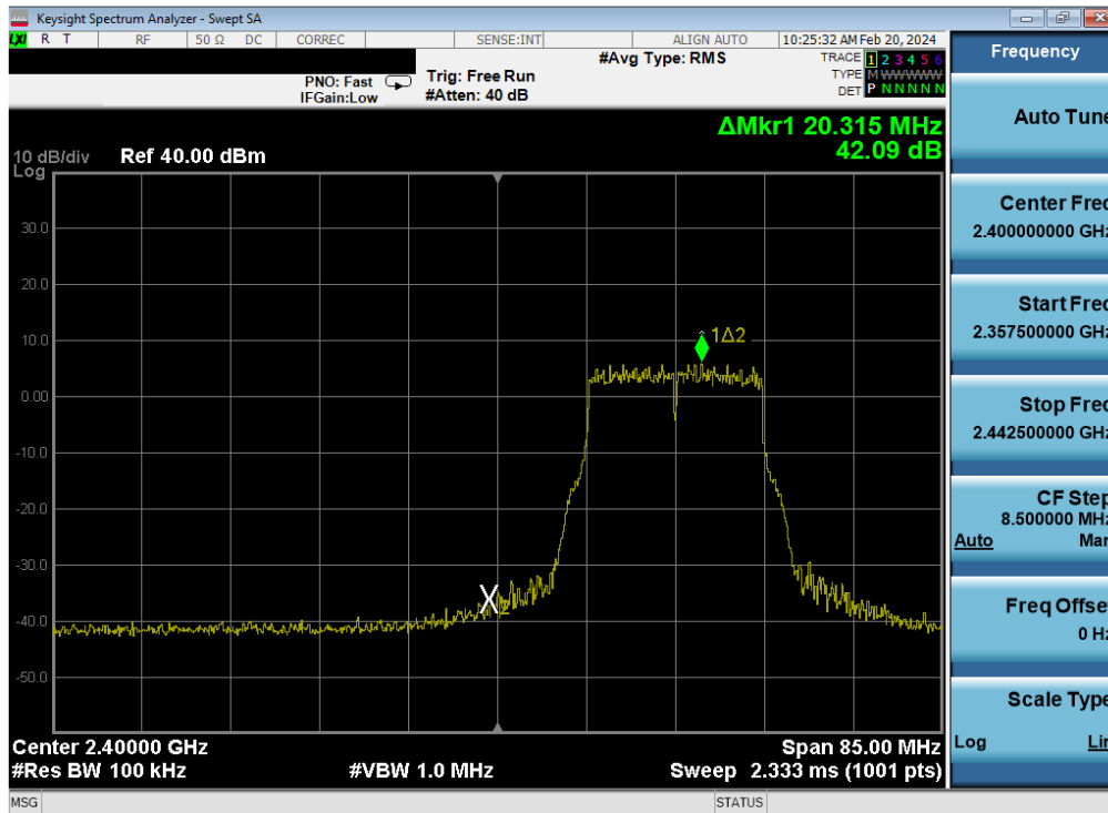
Plot 7-426. Band Edge Plot Antenna WF7 (802.11g – Ch. 2) – 54Mbps
