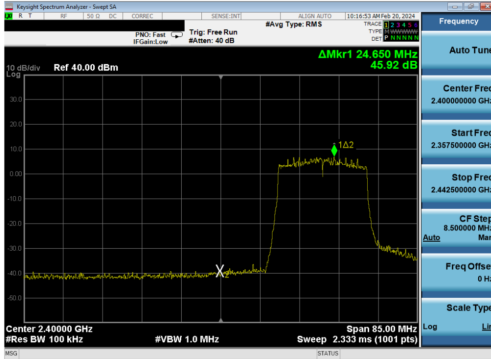
Plot 7-412. Band Edge Plot Antenna WF7 (802.11ax (SU - 2.4GHz) – Ch. 3) – MCS4
