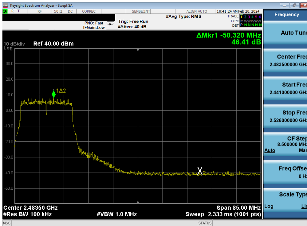
Plot 7-444. Band Edge Plot Antenna WF7 (802.11n (2.4GHz) – Ch. 9) – MCS7
