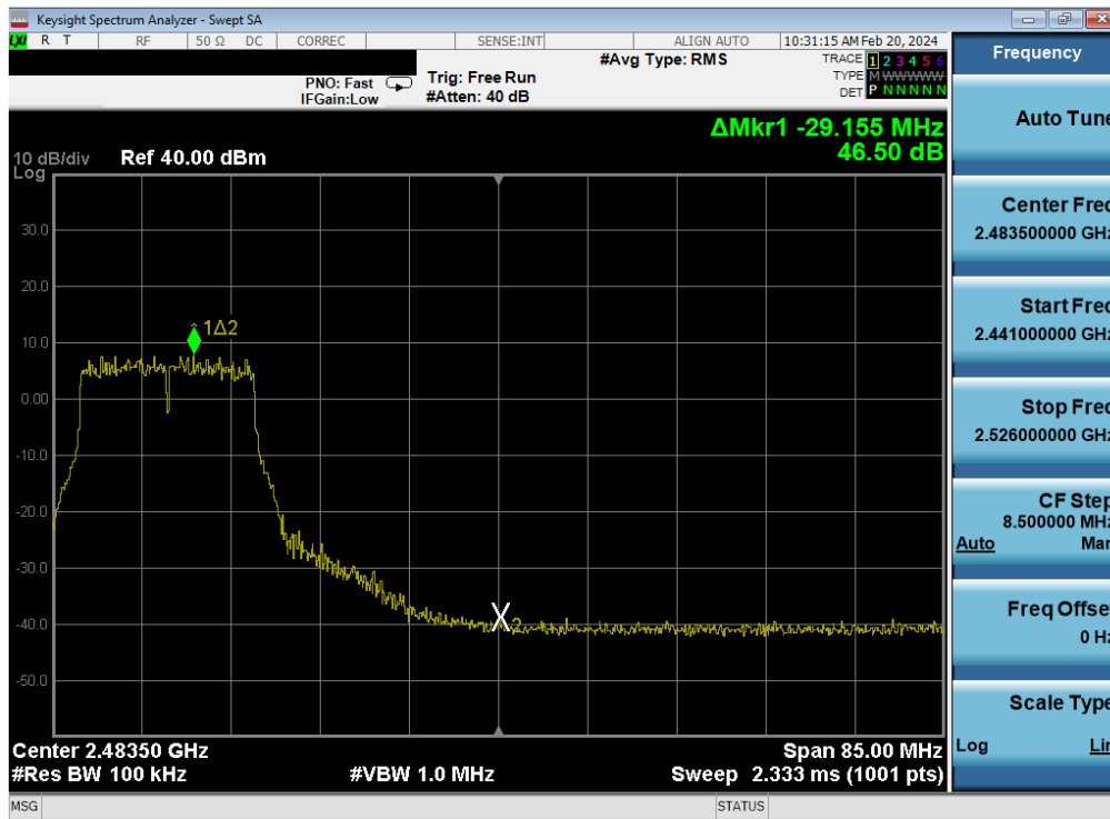
Plot 7-432. Band Edge Plot Antenna WF7 (802.11g – Ch. 9) – 54Mbps
