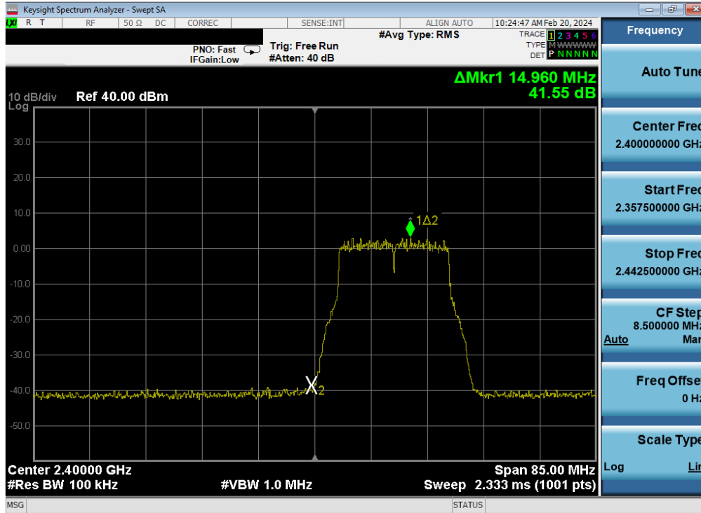
Plot 7-425. Band Edge Plot Antenna WF7 (802.11g – Ch. 1) – 54Mbps
