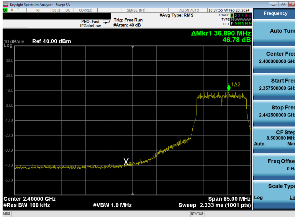
Plot 7-441. Band Edge Plot Antenna WF7 (802.11n (2.4GHz) – Ch. 5) – MCS7
