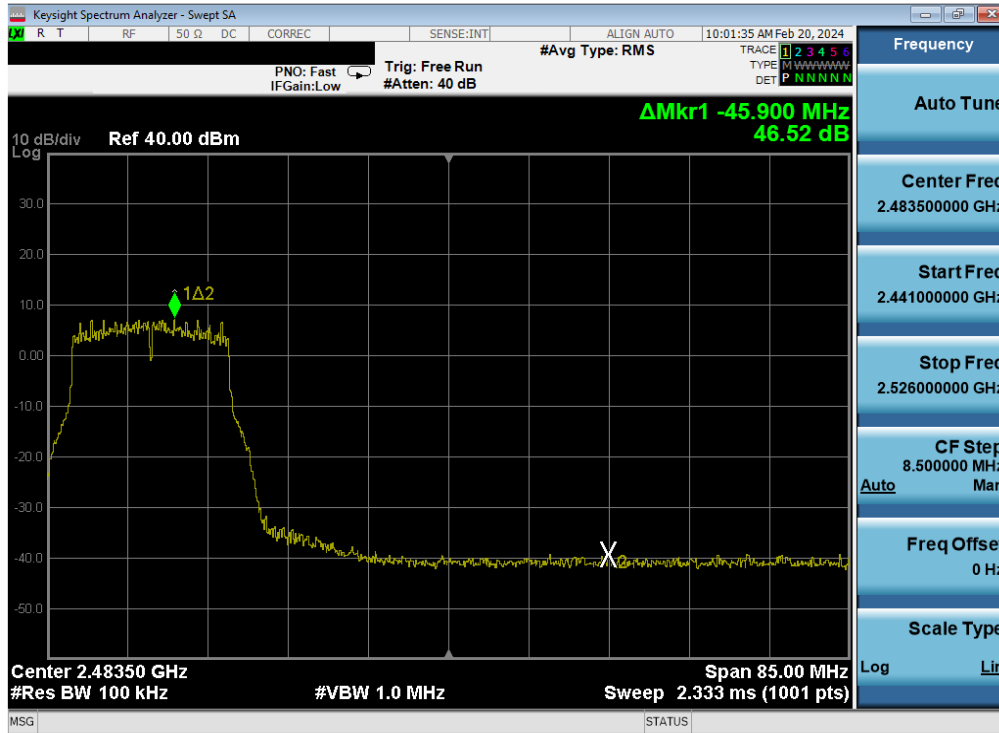
Plot 7-394. Band Edge Plot Antenna WF7 (802.11g – Ch. 9) – 24Mbps
