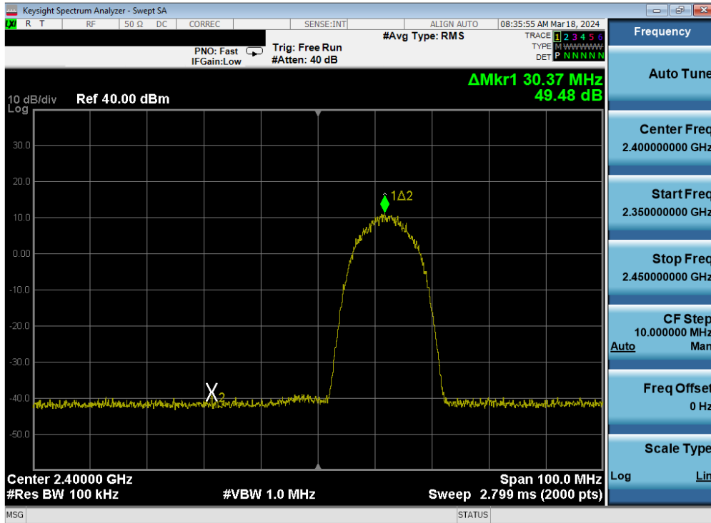
Plot 7-421. Band Edge Plot Antenna WF7 (802.11b – Ch. 1) – 11Mbps
