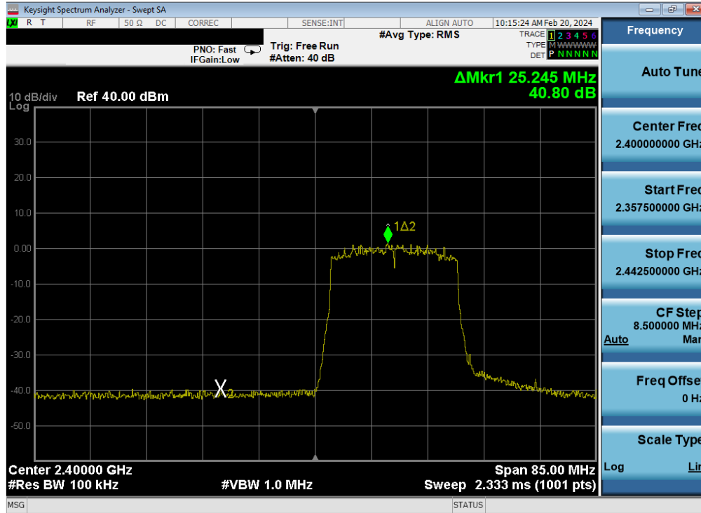
Plot 7-410. Band Edge Plot Antenna WF7 (802.11ax (SU - 2.4GHz) – Ch. 1) – MCS4
