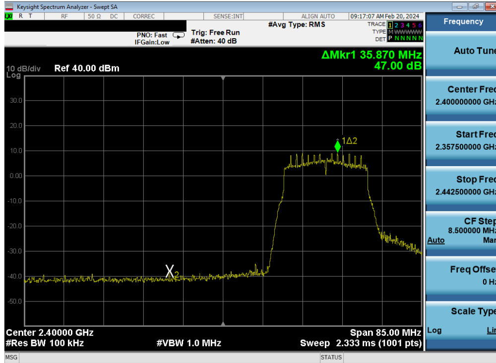
Plot 7-371. Band Edge Plot Antenna WF7 (802.11n (2.4GHz) – Ch. 3) – MCS2
