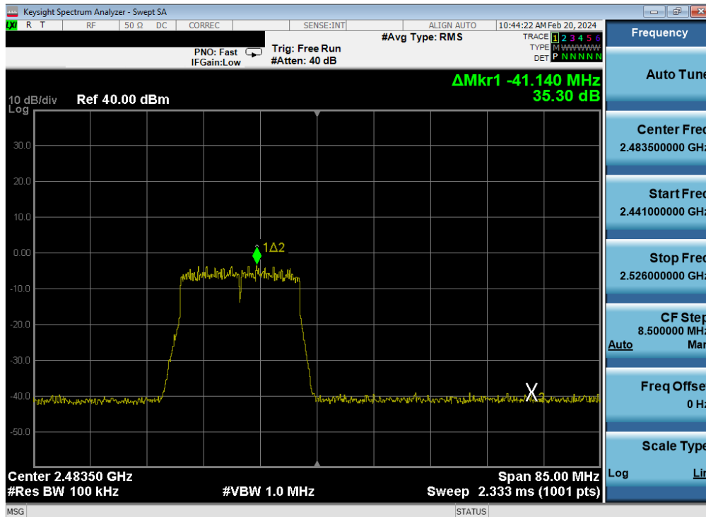
Plot 7-448. Band Edge Plot Antenna WF7 (802.11n (2.4GHz) – Ch. 13) – MCS7
