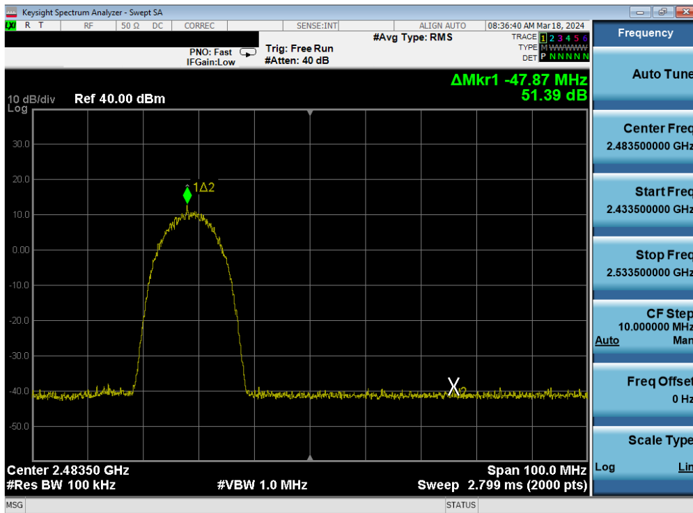
Plot 7-422. Band Edge Plot Antenna WF7 (802.11b – Ch. 11) – 11Mbps
