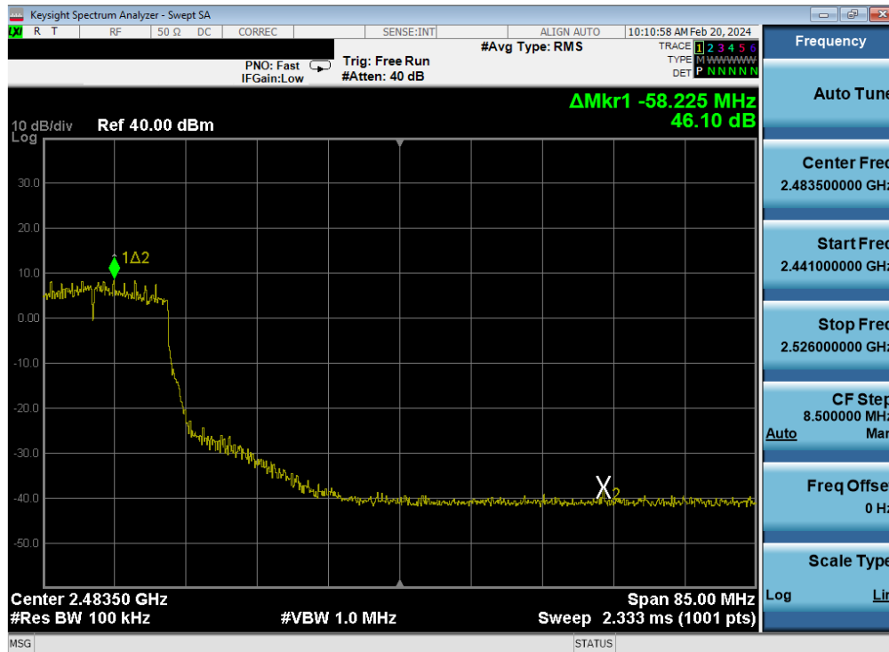
Plot 7-404. Band Edge Plot Antenna WF7 (802.11n (2.4GHz) – Ch. 8) – MCS4
