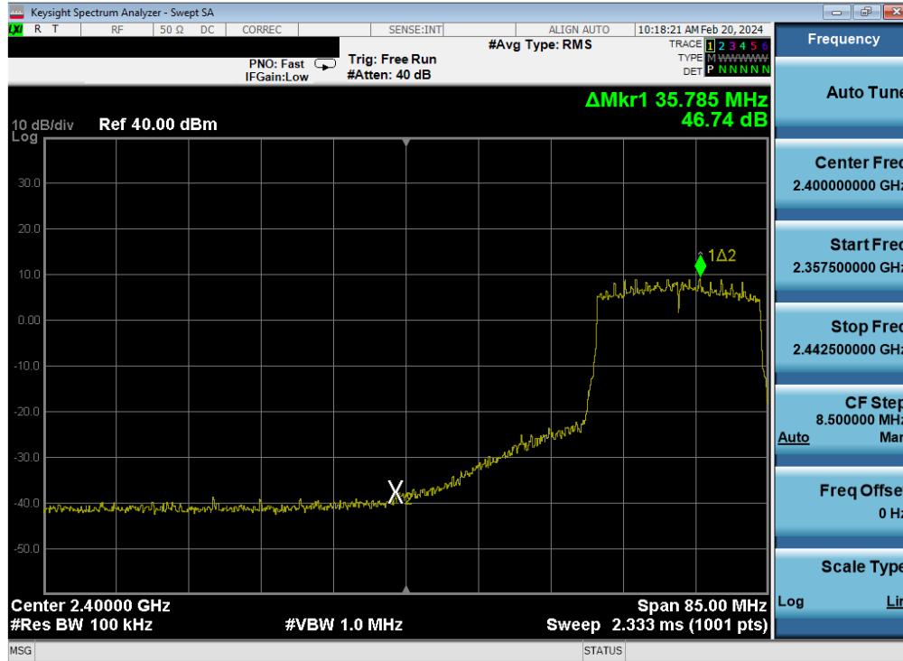
Plot 7-414. Band Edge Plot Antenna WF7 (802.11ax (SU - 2.4GHz) – Ch. 5) – MCS4
