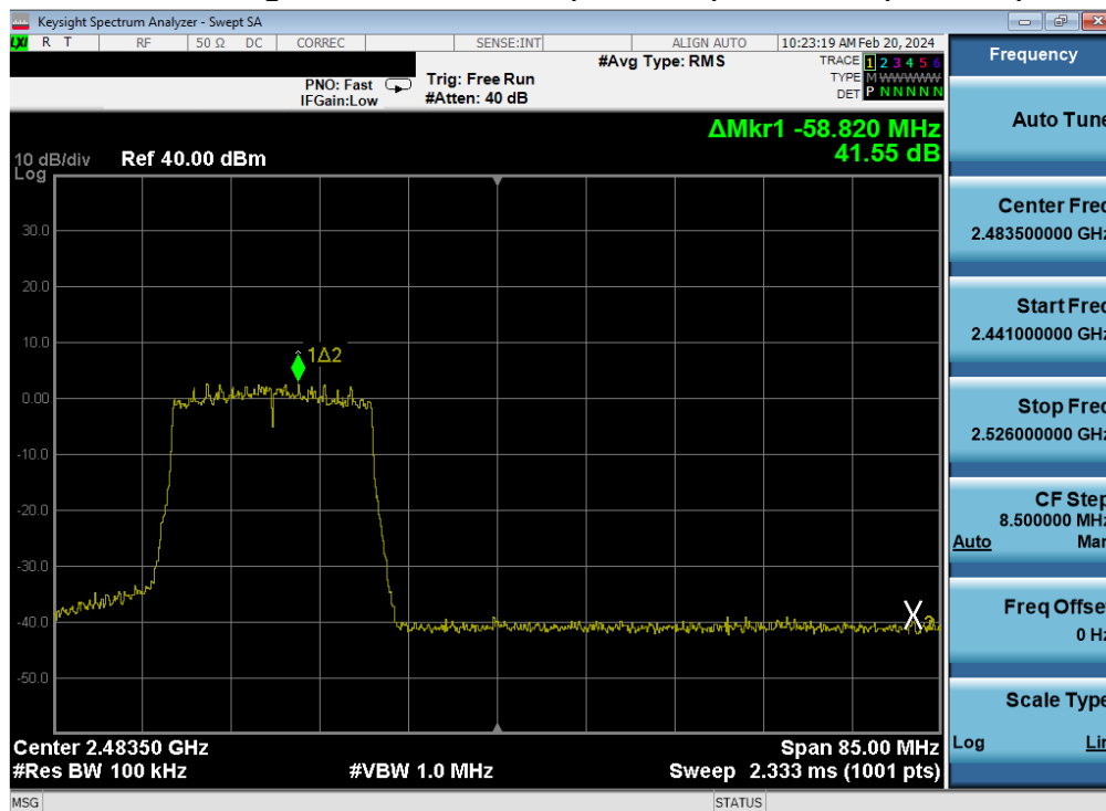
Plot 7-419. Band Edge Plot Antenna WF7 (802.11ax (SU - 2.4GHz) – Ch. 11) – MCS4
