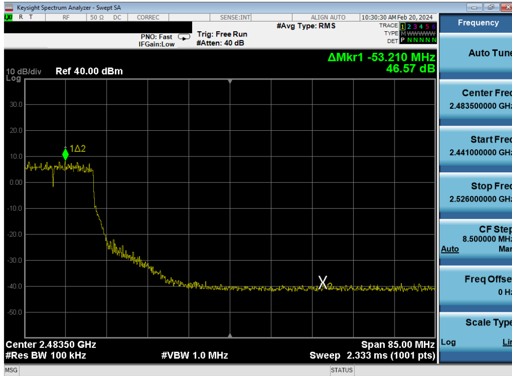
Plot 7-431. Band Edge Plot Antenna WF7 (802.11g – Ch. 8) – 54Mbps
