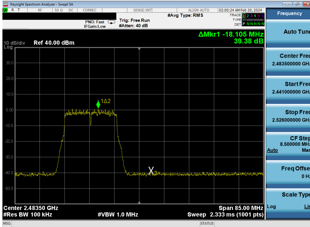
Plot 7-348. Band Edge Plot Antenna WF8 (802.11n (2.4GHz) – Ch. 12) – MCS7
