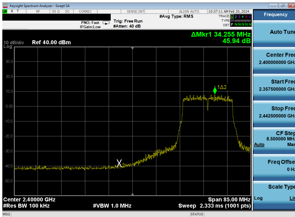
Plot 7-440. Band Edge Plot Antenna WF7 (802.11n (2.4GHz) – Ch. 4) – MCS7
