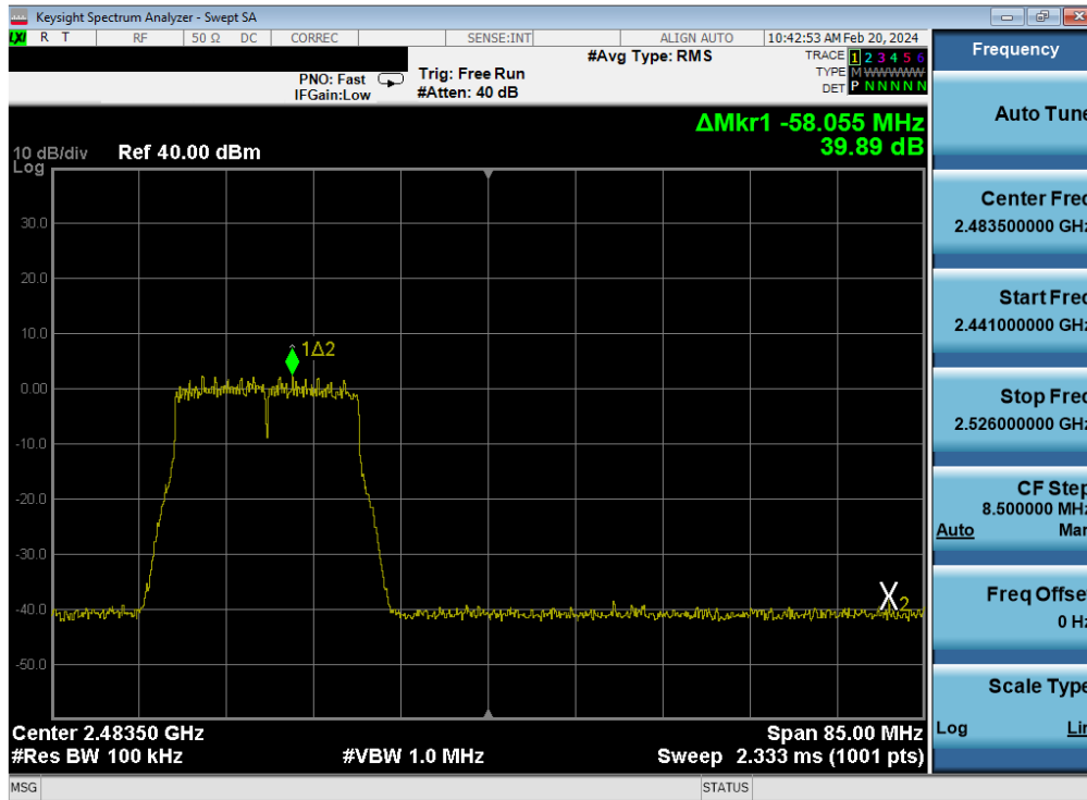
Plot 7-446. Band Edge Plot Antenna WF7 (802.11n (2.4GHz) – Ch. 11) – MCS7
