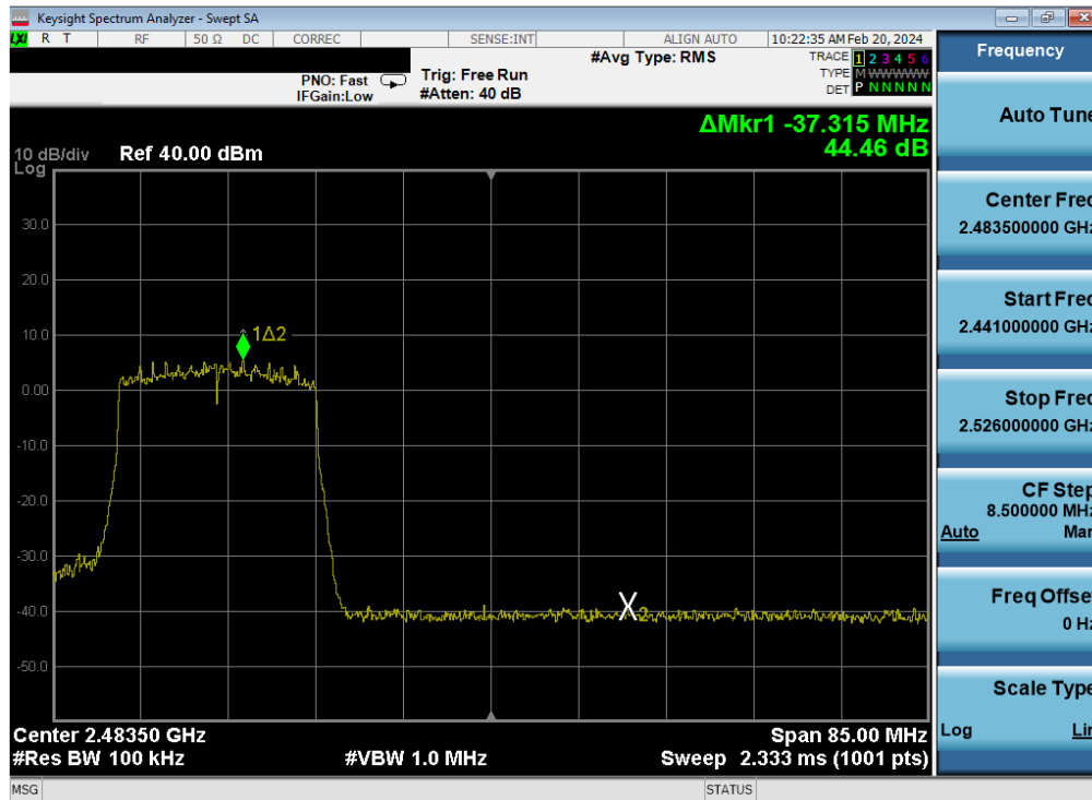
Plot 7-418. Band Edge Plot Antenna WF7 (802.11ax (SU - 2.4GHz) – Ch. 10) – MCS4
