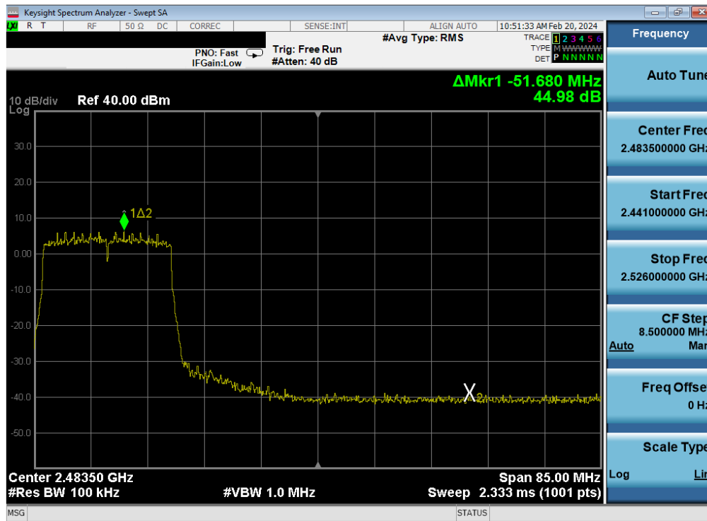
Plot 7-456. Band Edge Plot Antenna WF7 (802.11ax (SU - 2.4GHz) – Ch. 9) – MCS9
