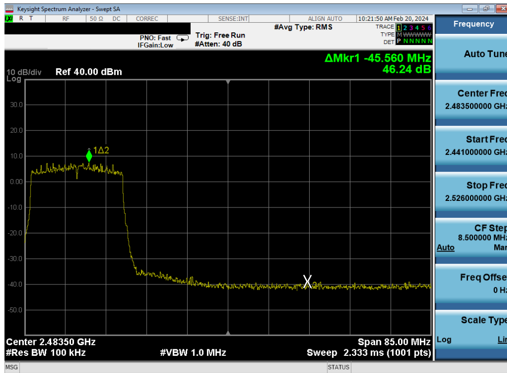
Plot 7-417. Band Edge Plot Antenna WF7 (802.11ax (SU - 2.4GHz) – Ch. 9) – MCS4
