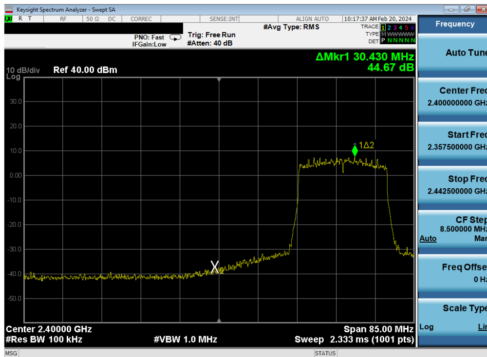
Plot 7-413. Band Edge Plot Antenna WF7 (802.11ax (SU - 2.4GHz) – Ch. 4) – MCS4
