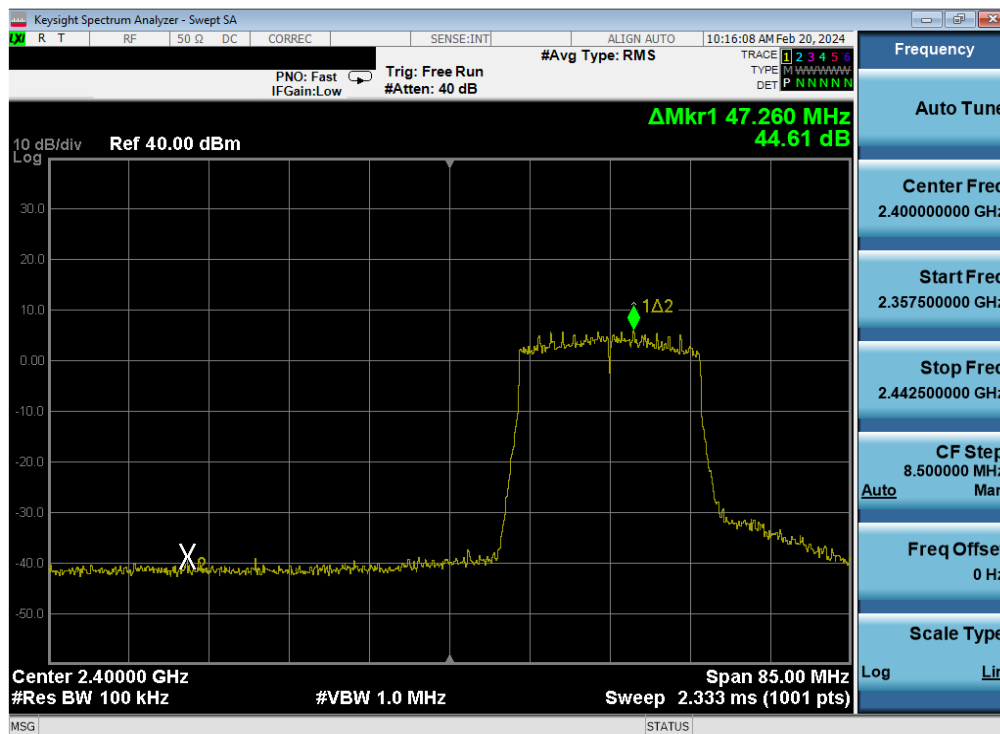
Plot 7-411. Band Edge Plot Antenna WF7 (802.11ax (SU - 2.4GHz) – Ch. 2) – MCS4
