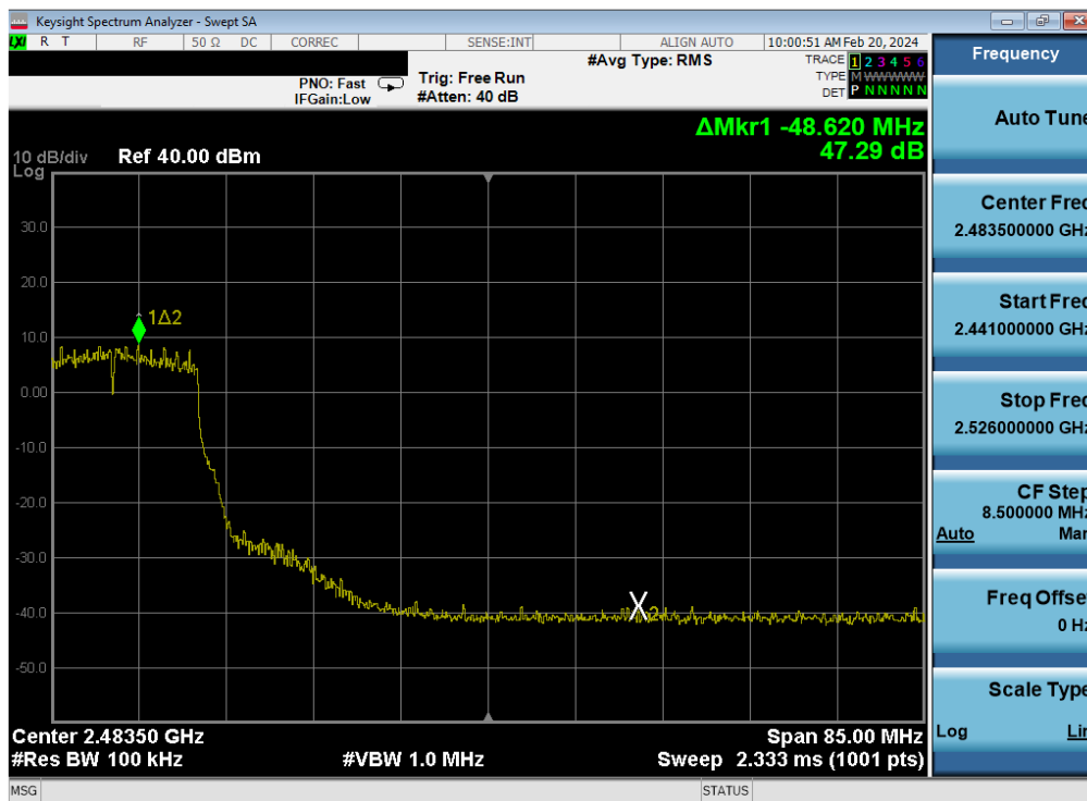
Plot 7-393. Band Edge Plot Antenna WF7 (802.11g – Ch. 8) – 24Mbps
