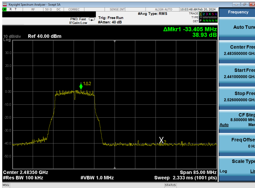
Plot 7-397. Band Edge Plot Antenna WF7 (802.11g – Ch. 12) – 24Mbps
