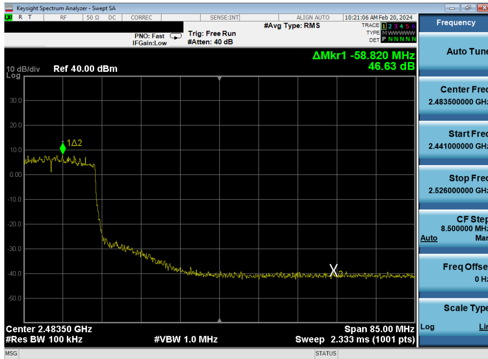
Plot 7-416. Band Edge Plot Antenna WF7 (802.11ax (SU - 2.4GHz) – Ch. 8) – MCS4
