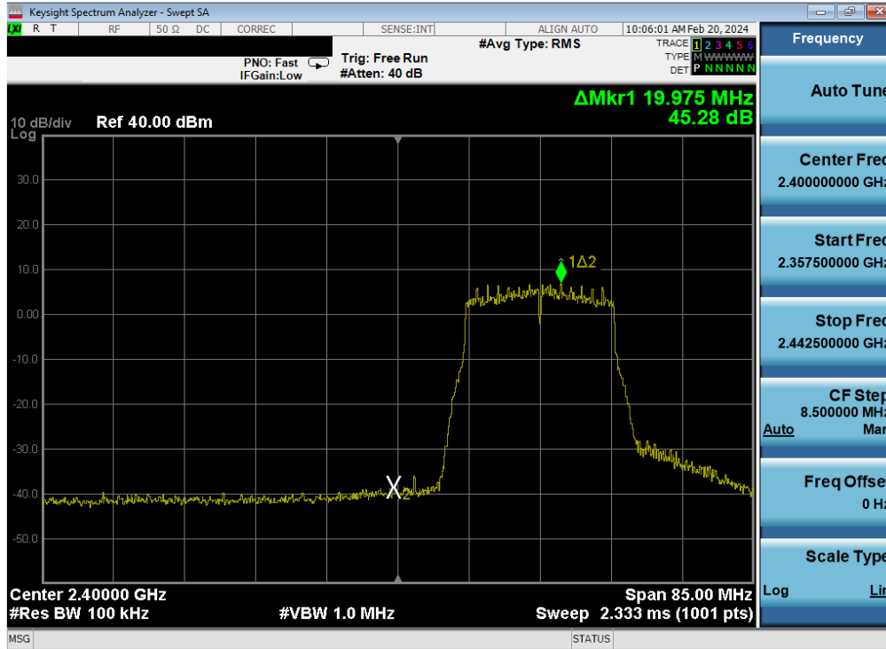
Plot 7-400. Band Edge Plot Antenna WF7 (802.11n (2.4GHz) – Ch. 2) – MCS4
