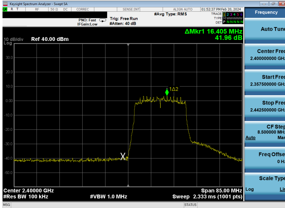
Plot 7-476. Band Edge Plot Antenna WF9 (802.11ax (SU - 2.4GHz) – Ch. 1) – MCS2
