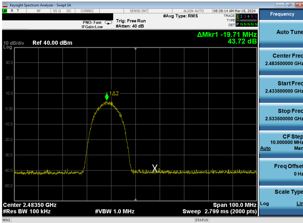
Plot 7-424. Band Edge Plot Antenna WF7 (802.11b – Ch. 13) – 11Mbps
