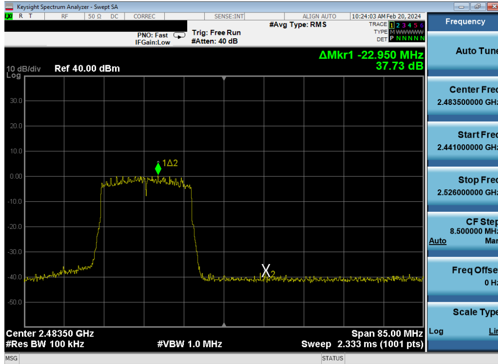
Plot 7-420. Band Edge Plot Antenna WF7 (802.11ax (SU - 2.4GHz) – Ch. 12) – MCS4
