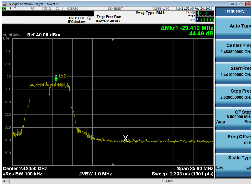
Plot 7-433. Band Edge Plot Antenna WF7 (802.11g – Ch. 10) – 54Mbps
