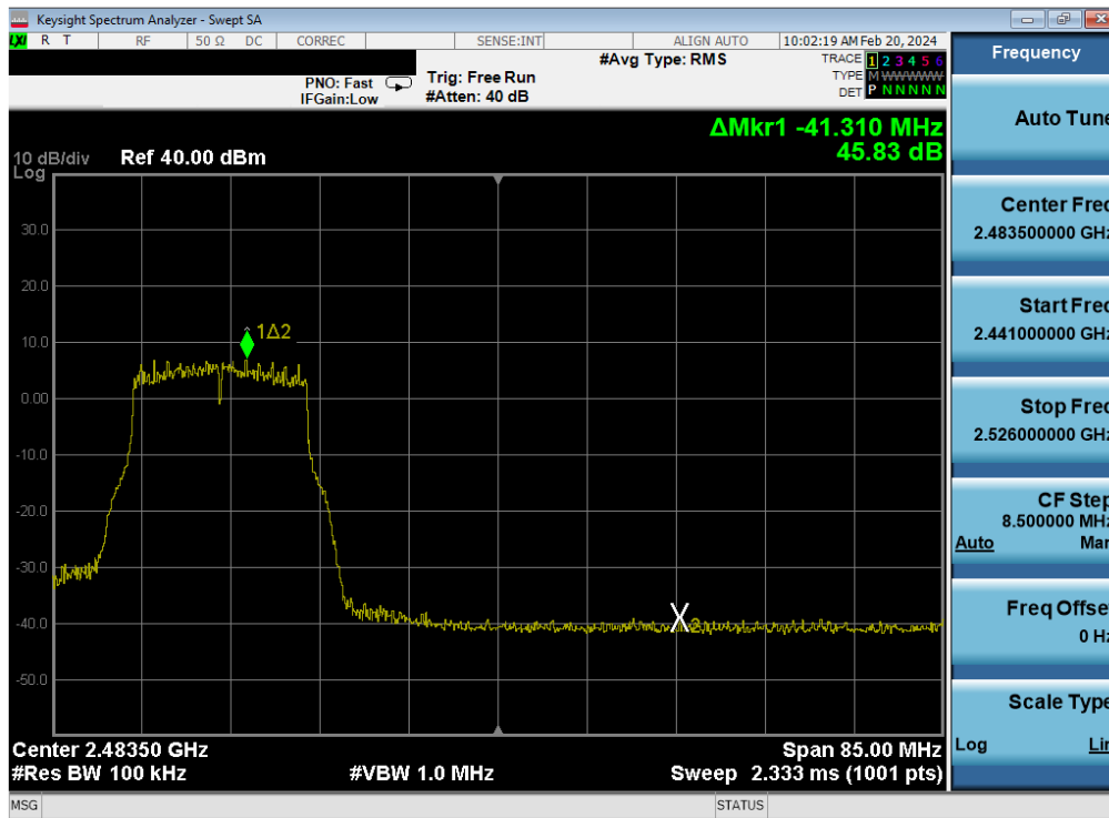
Plot 7-395. Band Edge Plot Antenna WF7 (802.11g – Ch. 10) – 24Mbps
