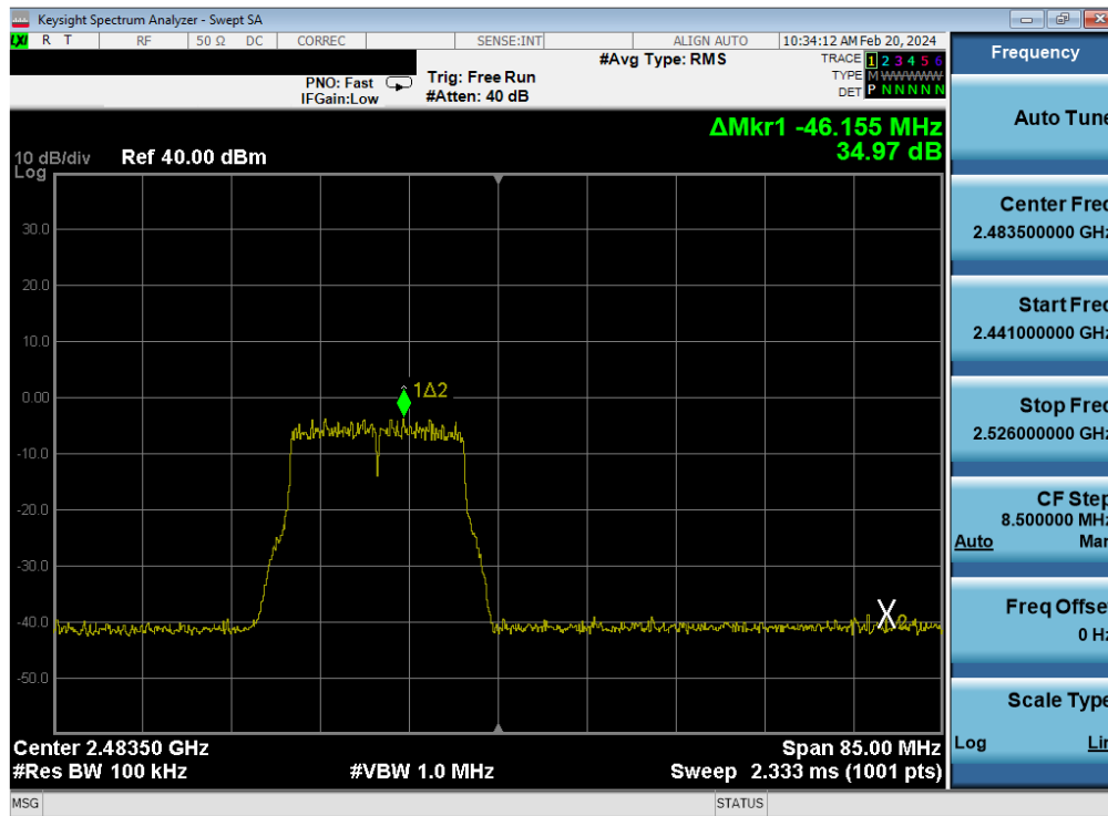
Plot 7-436. Band Edge Plot Antenna WF7 (802.11g – Ch. 13) – 54Mbps
