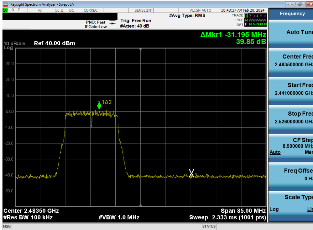
Plot 7-447. Band Edge Plot Antenna WF7 (802.11n (2.4GHz) – Ch. 12) – MCS7
