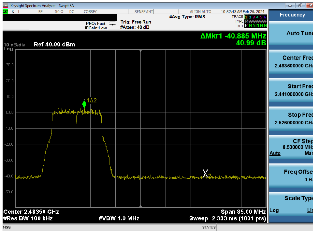
Plot 7-434. Band Edge Plot Antenna WF7 (802.11g – Ch. 11) – 54Mbps
