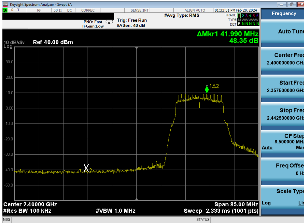
Plot 7-462. Band Edge Plot Antenna WF9 (802.11g – Ch. 3) – 12Mbps
