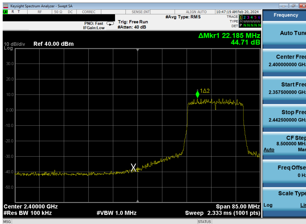
Plot 7-452. Band Edge Plot Antenna WF7 (802.11ax (SU - 2.4GHz) – Ch. 4) – MCS9
