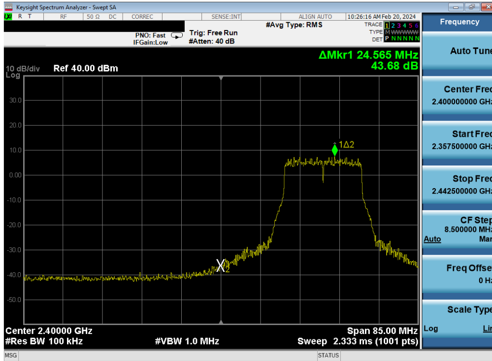
Plot 7-427. Band Edge Plot Antenna WF7 (802.11g – Ch. 3) – 54Mbps
