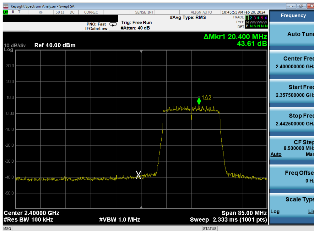
Plot 7-450. Band Edge Plot Antenna WF7 (802.11ax (SU - 2.4GHz) – Ch. 2) – MCS9
