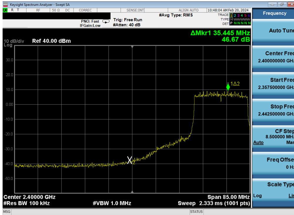
Plot 7-453. Band Edge Plot Antenna WF7 (802.11ax (SU - 2.4GHz) – Ch. 5) – MCS9
