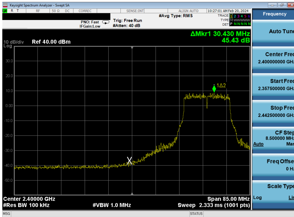
Plot 7-428. Band Edge Plot Antenna WF7 (802.11g – Ch. 4) – 54Mbps
