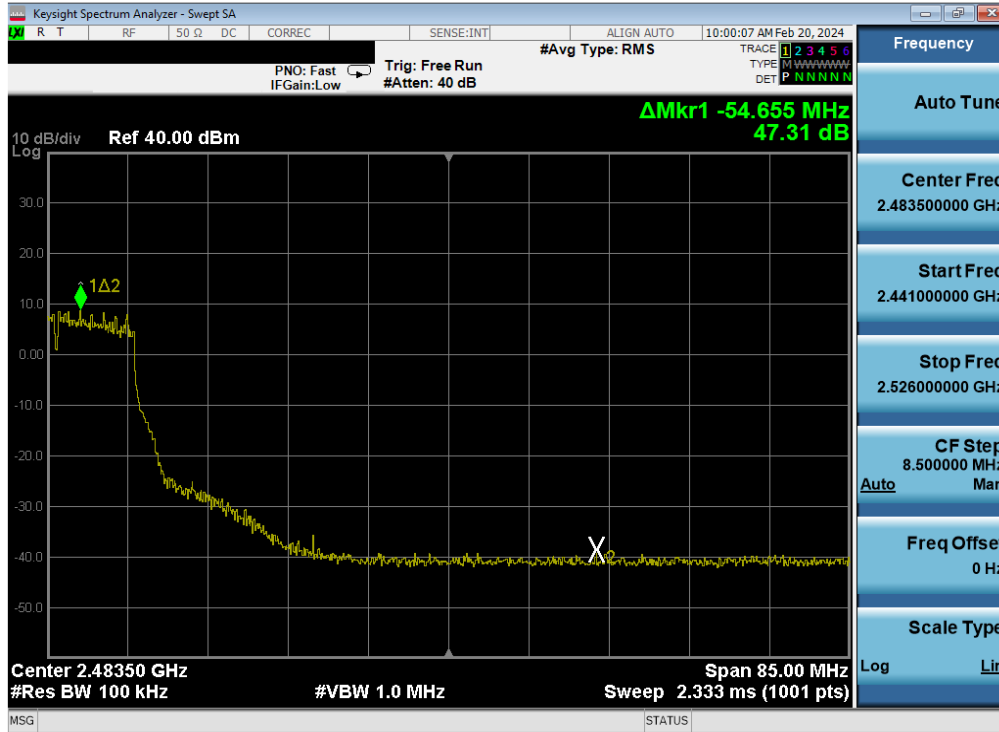
Plot 7-392. Band Edge Plot Antenna WF7 (802.11g – Ch. 7) – 24Mbps
