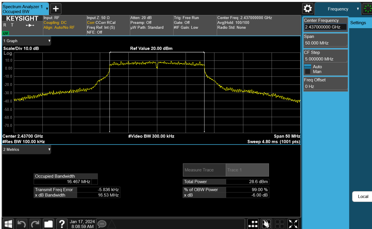
Plot 7-71. 6 dB BW and 99% OBW Plot Antenna WF9 (802.11g – Ch. 6) – 24Mbps
