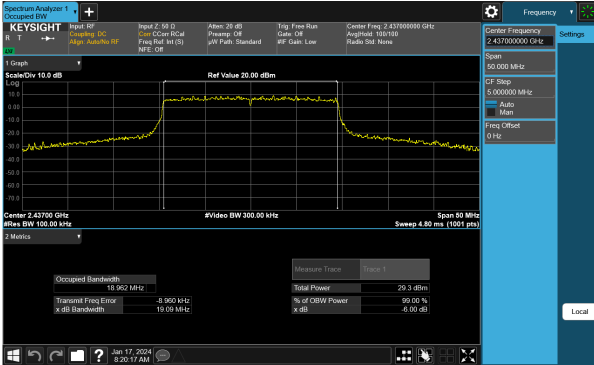
Plot 7-89. 6 dB BW and 99% OBW Plot Antenna WF9 (802.11ax (SU - 2.4GHz) – Ch. 6) – MCS9
