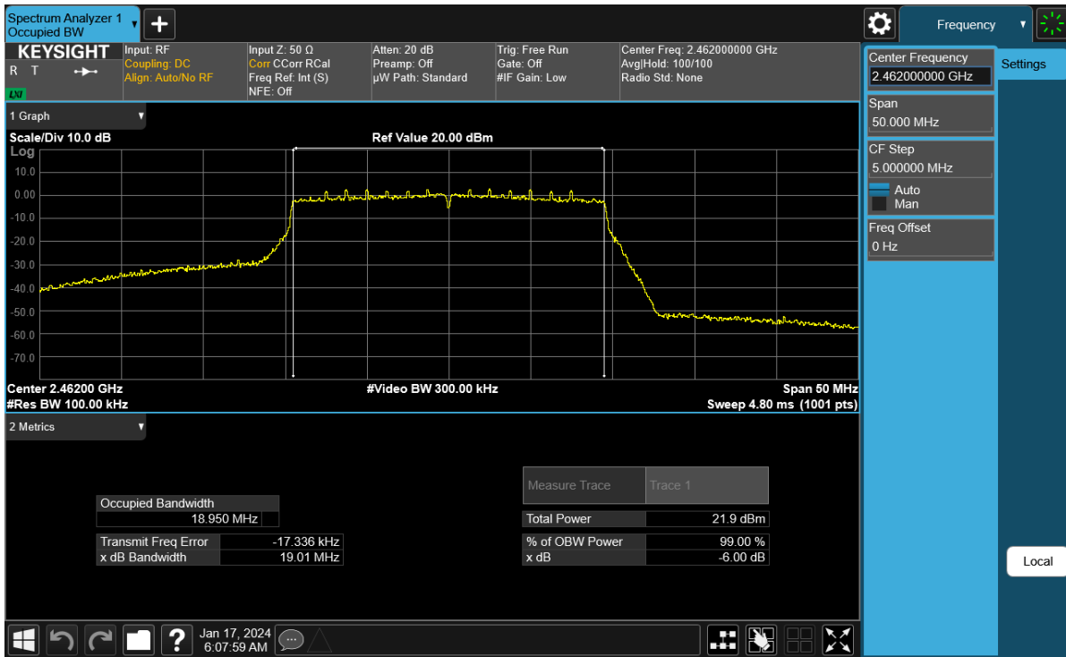
Plot 7-9. 6 dB BW and 99% OBW Plot Antenna WF8 (802.11ax (SU - 2.4GHz) – Ch. 11) – MCS2
