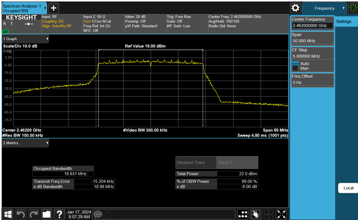
Plot 7-69. 6 dB BW and 99% OBW Plot Antenna WF9 (802.11ax (SU - 2.4GHz) – Ch. 11) – MCS2
