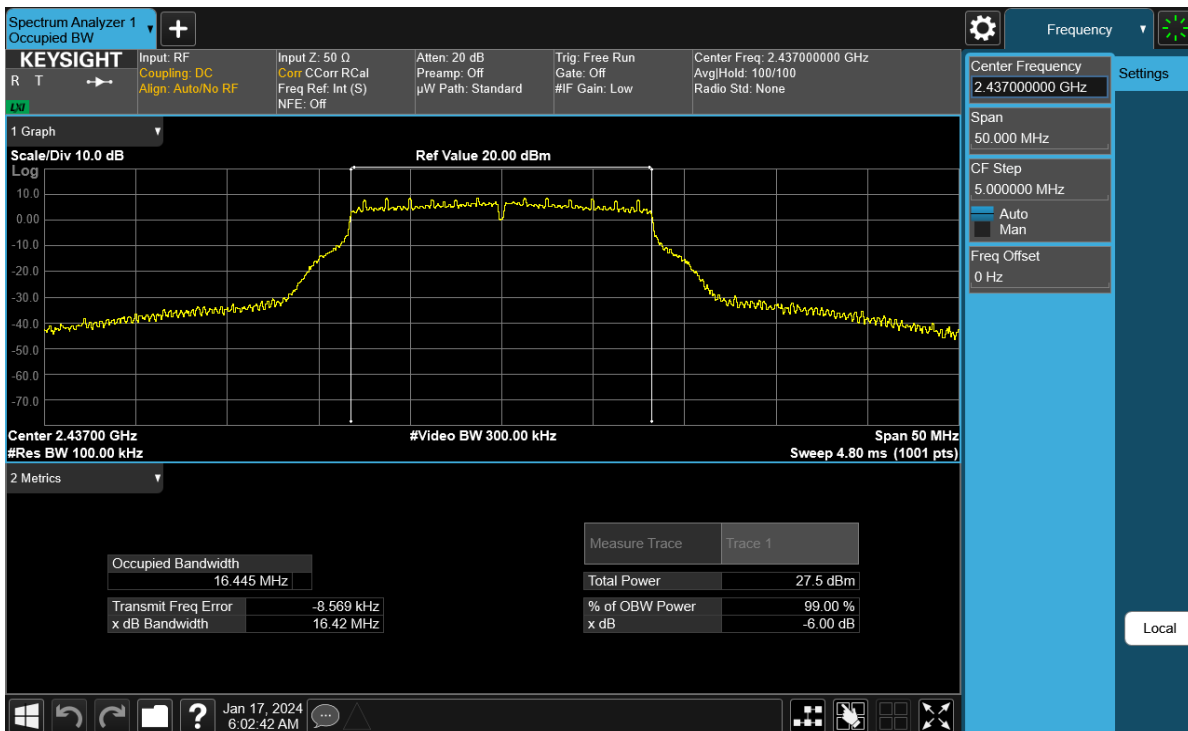
Plot 7-2. 6 dB BW and 99% OBW Plot Antenna WF8 (802.11g – Ch. 6) – 12Mbps
