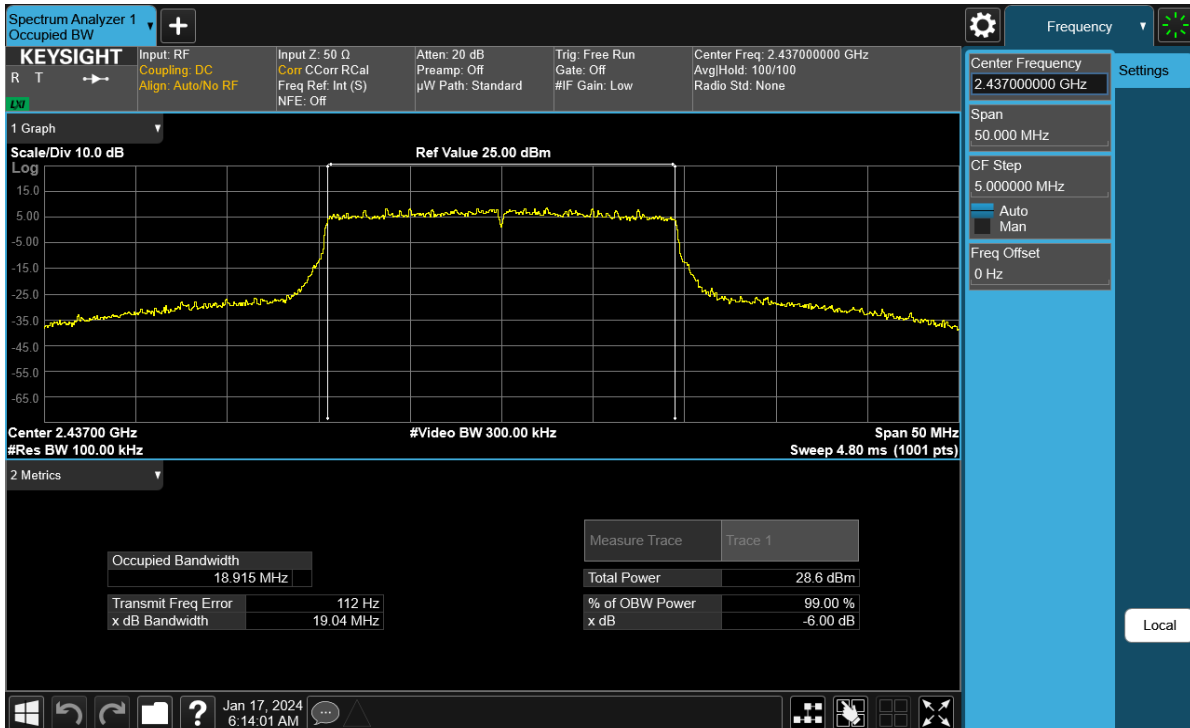
Plot 7-17. 6 dB BW and 99% OBW Plot Antenna WF8 (802.11ax (SU - 2.4GHz) - Ch. 6) - MCS4
