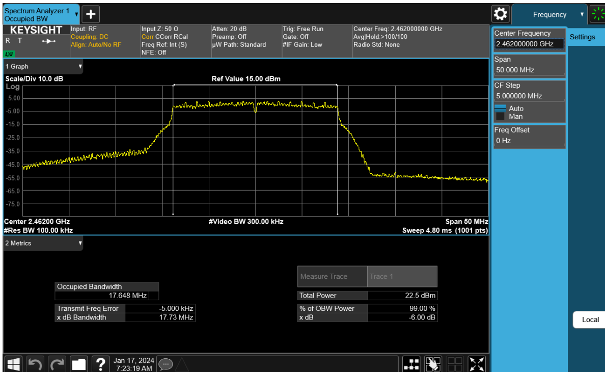
Plot 7-45. 6 dB BW and 99% OBW Plot Antenna WF7 (802.11n (2.4GHz) – Ch. 11) – MCS4
