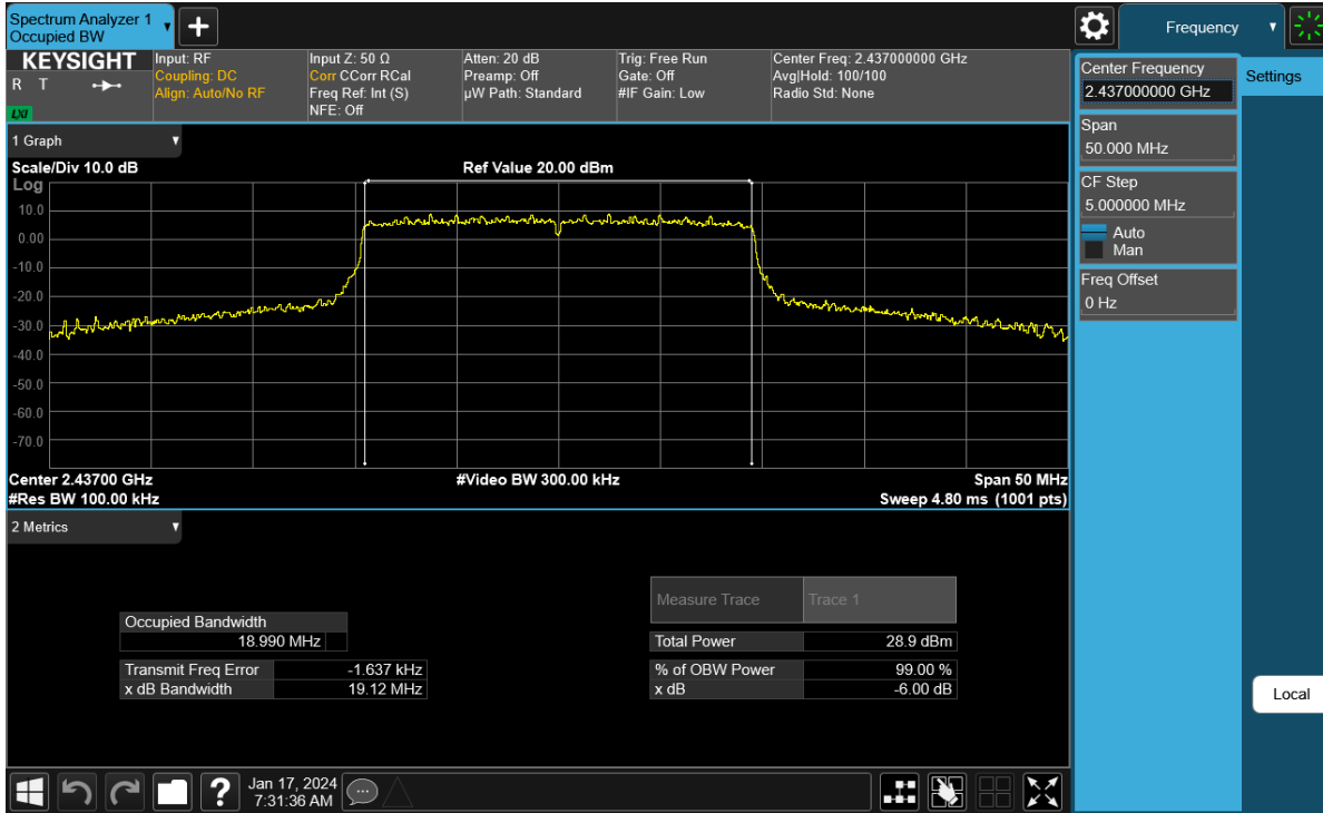
Plot 7-59. 6 dB BW and 99% OBW Plot Antenna WF7 (802.11ax (SU - 2.4GHz) – Ch. 6) – MCS9
