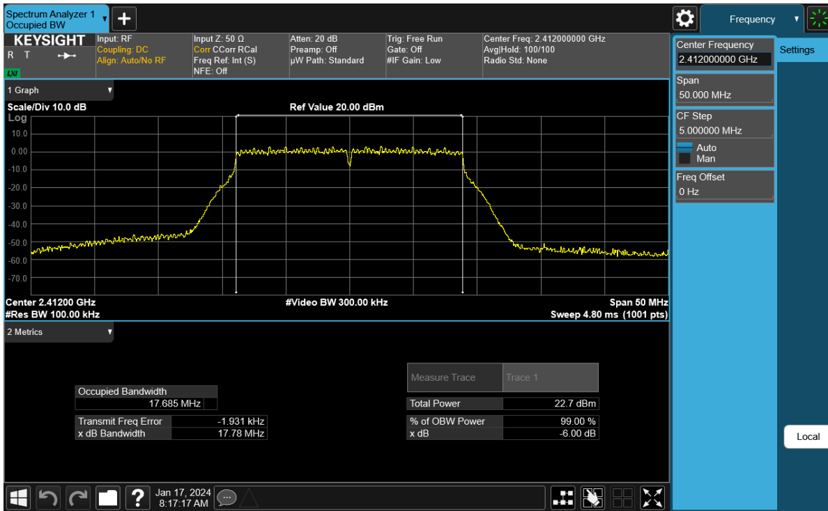
Plot 7-85. 6 dB BW and 99% OBW Plot Antenna WF9 (802.11n (2.4GHz) – Ch. 1) – MCS7
