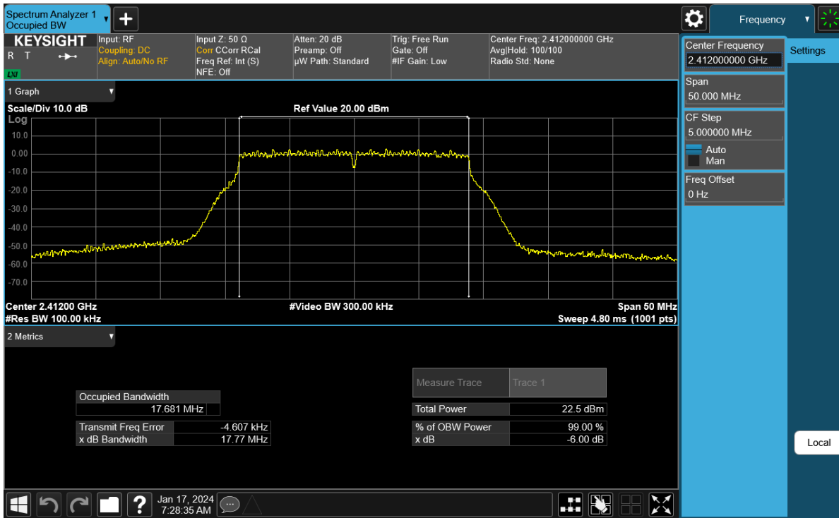
Plot 7-55. 6 dB BW and 99% OBW Plot Antenna WF7 (802.11n (2.4GHz) – Ch. 1) – MCS7
