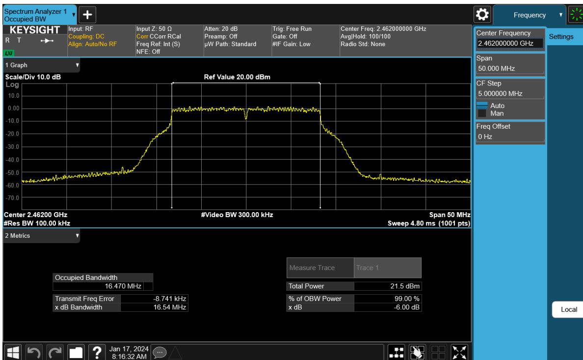
Plot 7-84. 6 dB BW and 99% OBW Plot Antenna WF9 (802.11g – Ch. 11) – 54Mbps
