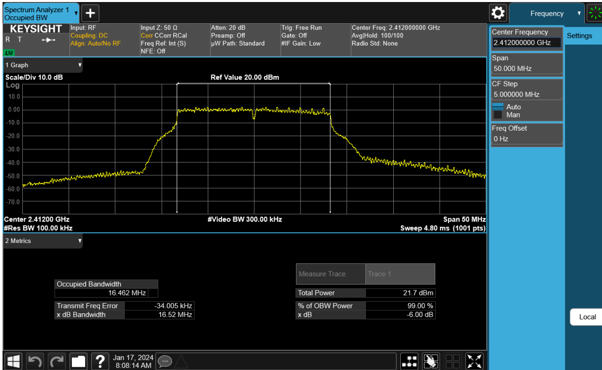
Plot 7-70. 6 dB BW and 99% OBW Plot Antenna WF9 (802.11g – Ch. 1) – 24Mbps
