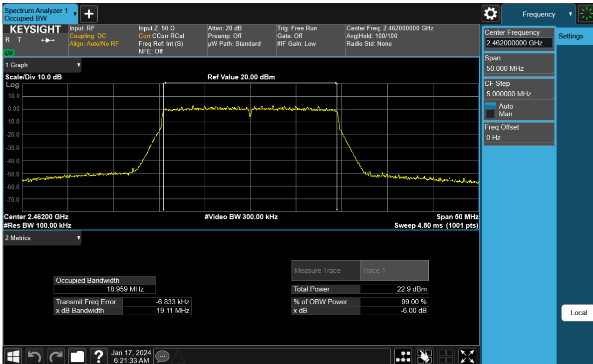
Plot 7-30. 6 dB BW and 99% OBW Plot Antenna WF8 (802.11ax (SU - 2.4GHz) – Ch. 11) – MCS9
