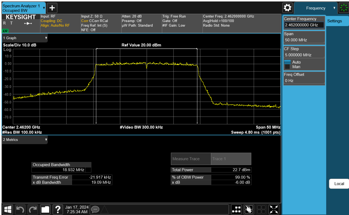
Plot 7-48. 6 dB BW and 99% OBW Plot Antenna WF7 (802.11ax (SU - 2.4GHz) – Ch. 11) – MCS4
