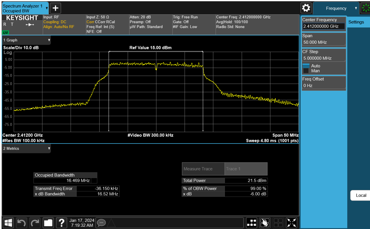
Plot 7-40. 6 dB BW and 99% OBW Plot Antenna WF7 (802.11g – Ch. 1) – 24Mbps
