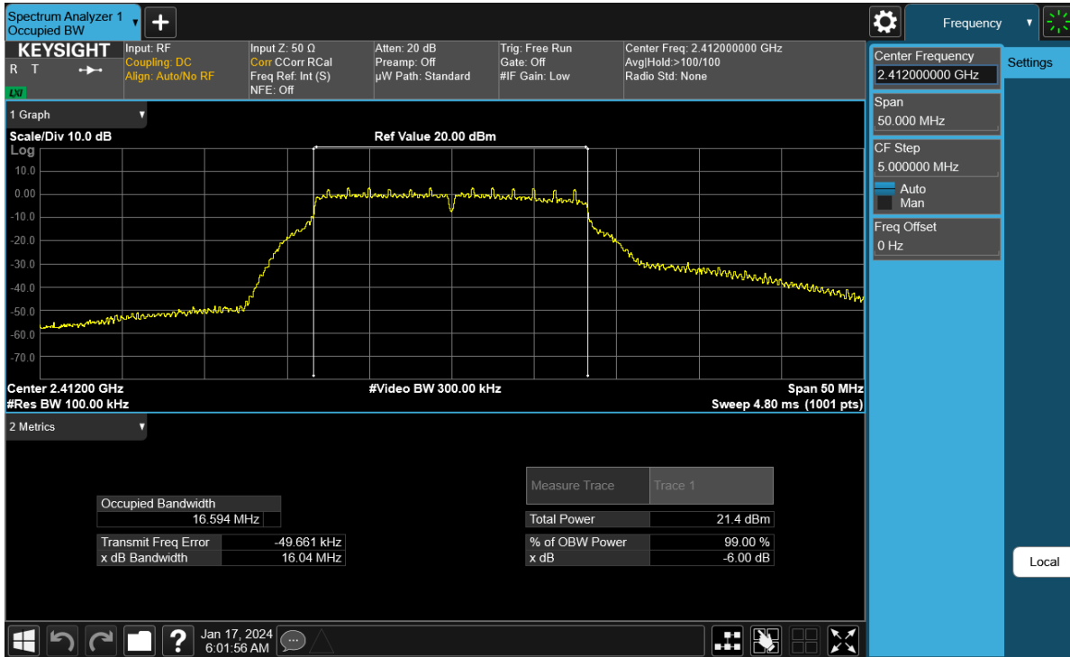
Plot 7-1. 6 dB BW and 99% OBW Plot Antenna WF8 (802.11g – Ch. 1) – 12Mbps
