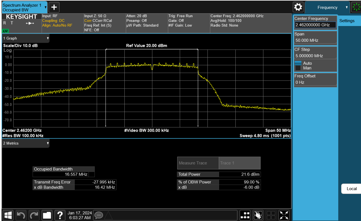
Plot 7-3. 6 dB BW and 99% OBW Plot Antenna WF8 (802.11g – Ch. 11) – 12Mbps
