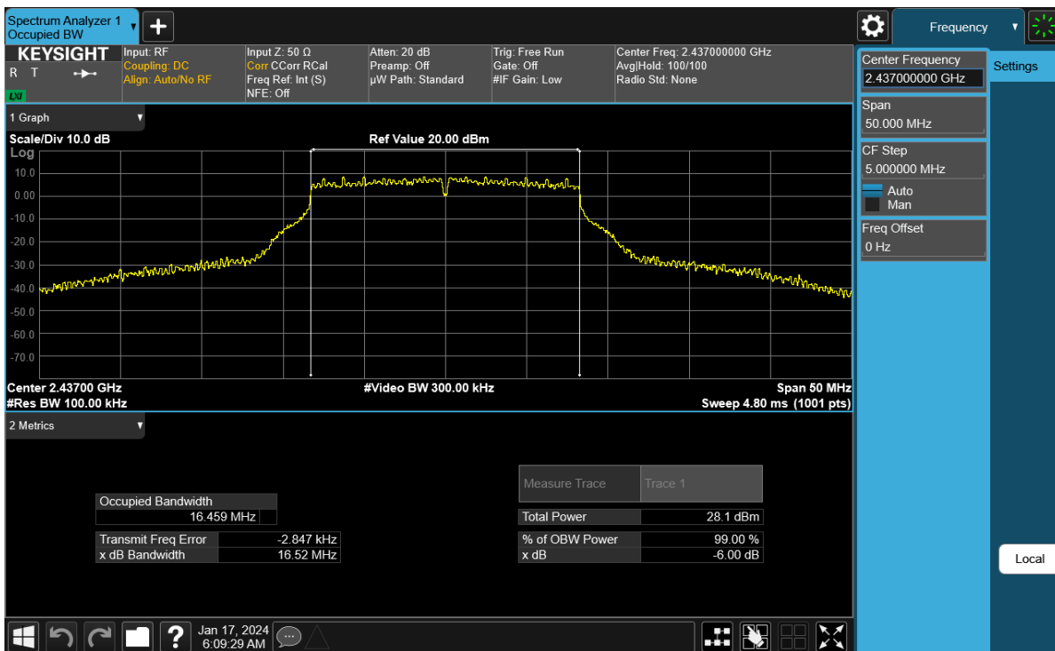
Plot 7-11. 6 dB BW and 99% OBW Plot Antenna WF8 (802.11g – Ch. 6) – 24Mbps
