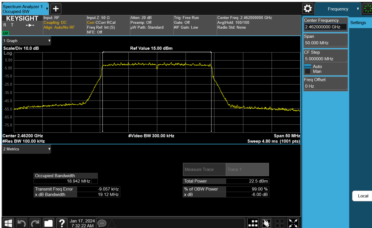
Plot 7-60. 6 dB BW and 99% OBW Plot Antenna WF7 (802.11ax (SU - 2.4GHz) – Ch. 11) – MCS9
