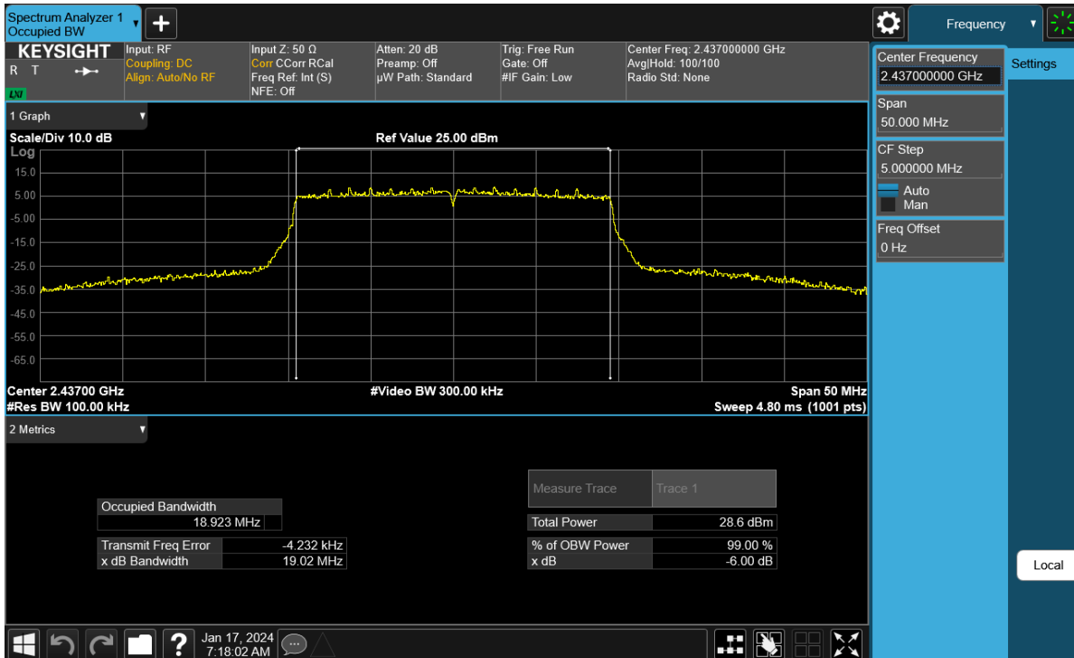
Plot 7-38. 6 dB BW and 99% OBW Plot Antenna WF7 (802.11ax (SU - 2.4GHz) – Ch. 6) – MCS2
