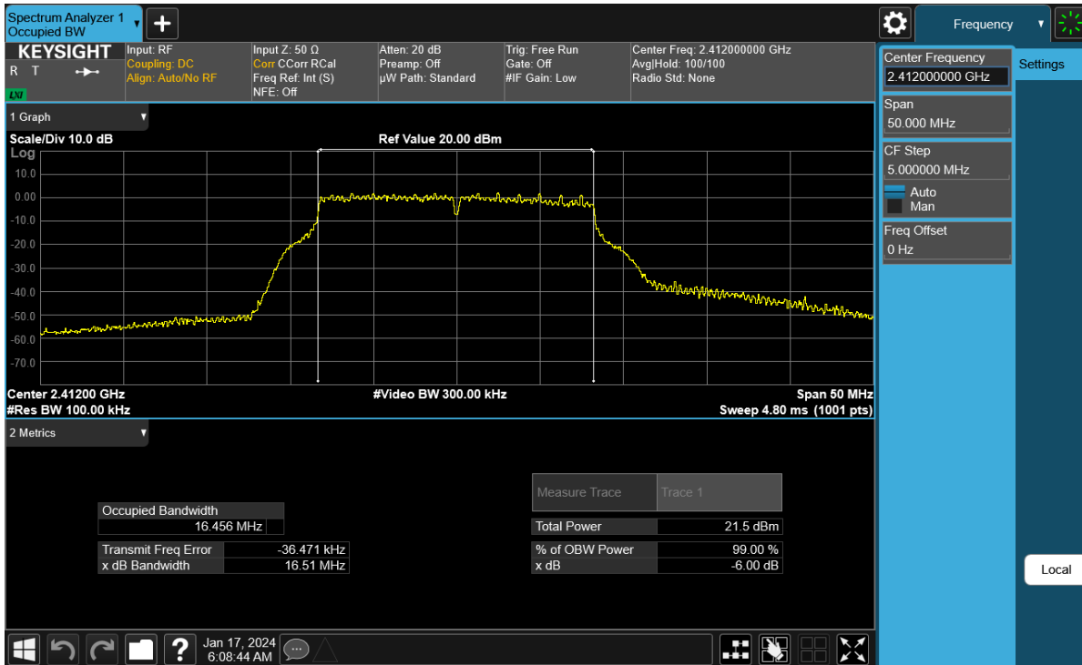
Plot 7-10. 6 dB BW and 99% OBW Plot Antenna WF8 (802.11g – Ch. 1) – 24Mbps
