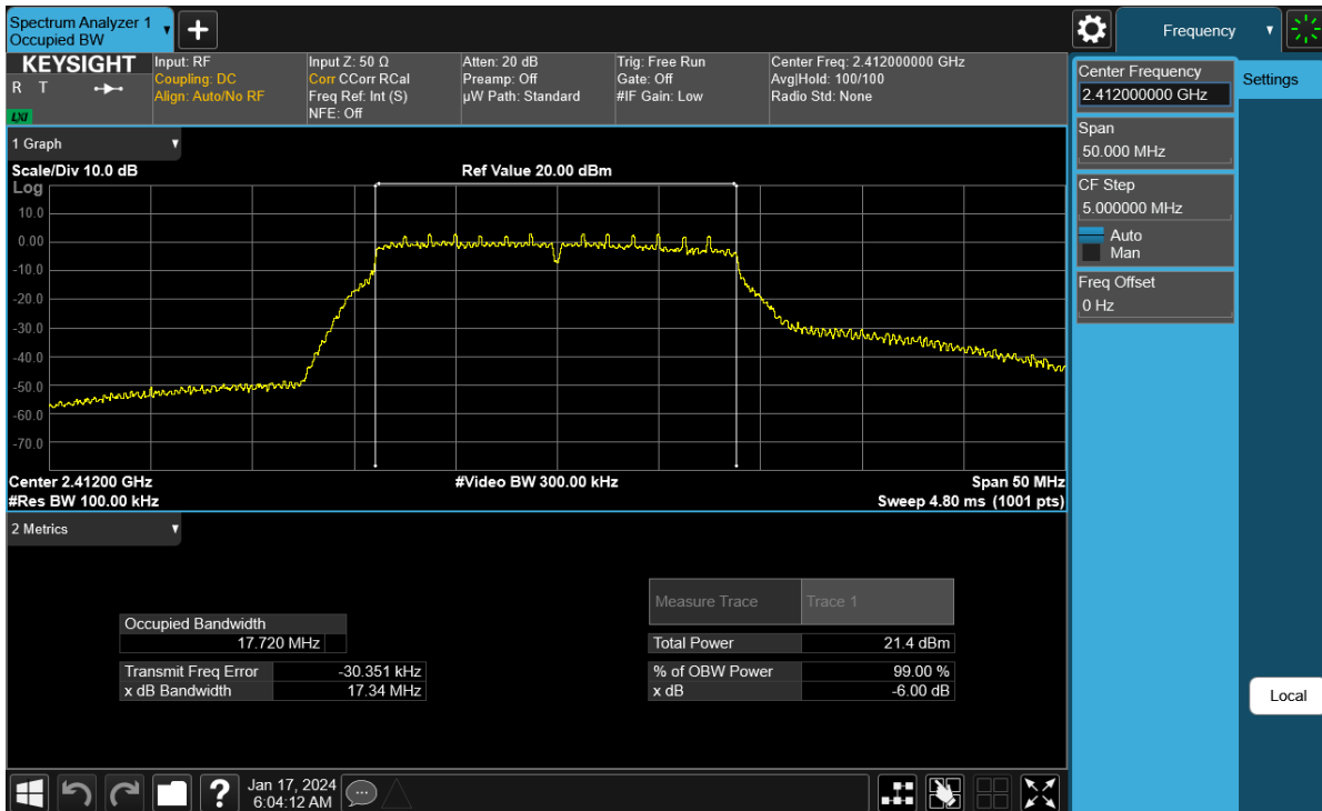
Plot 7-4. 6 dB BW and 99% OBW Plot Antenna WF8 (802.11n (2.4GHz) – Ch. 1) – MCS2
