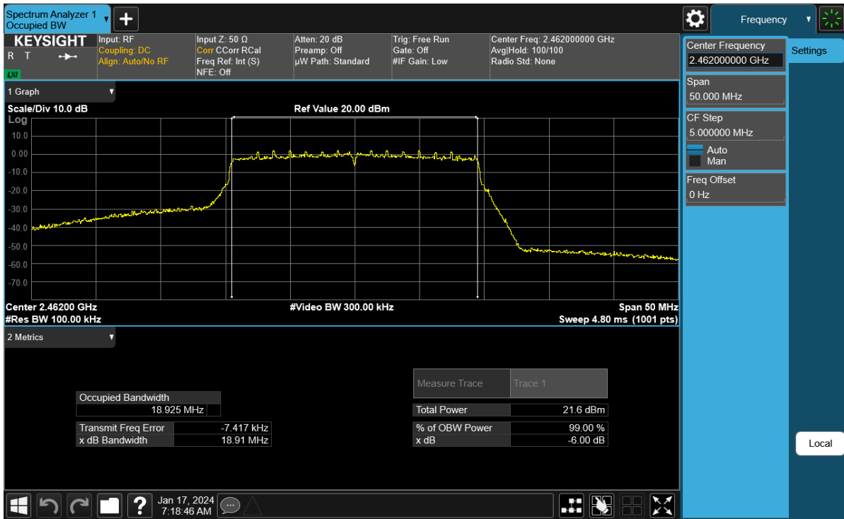
Plot 7-39. 6 dB BW and 99% OBW Plot Antenna WF7 (802.11ax (SU - 2.4GHz) – Ch. 11) – MCS2
