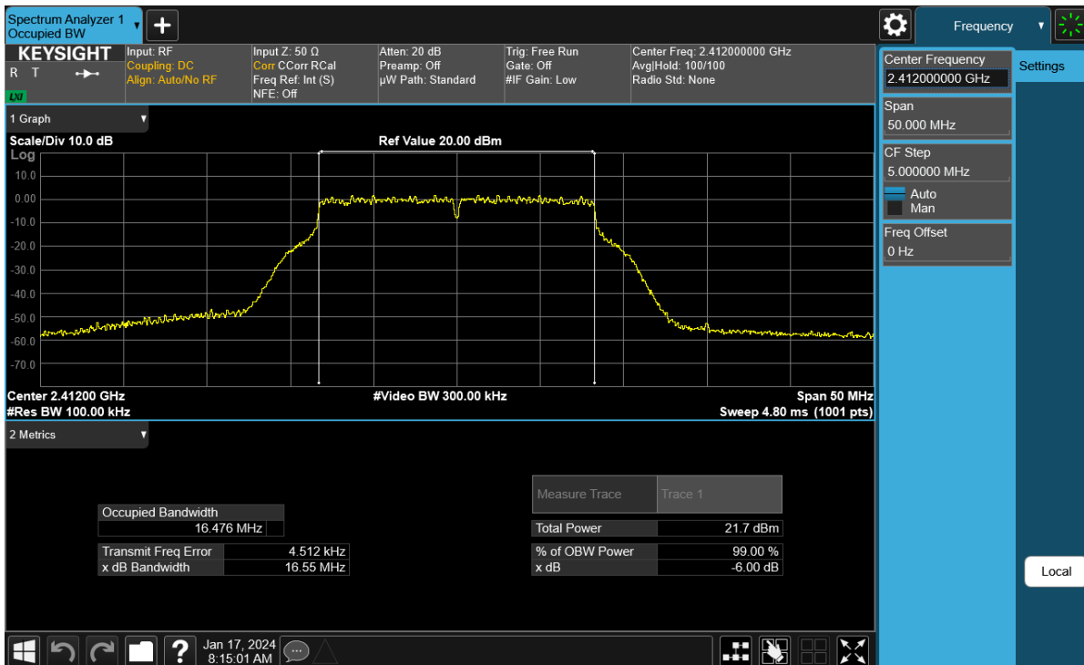
Plot 7-82. 6 dB BW and 99% OBW Plot Antenna WF9 (802.11g – Ch. 1) – 54Mbps
