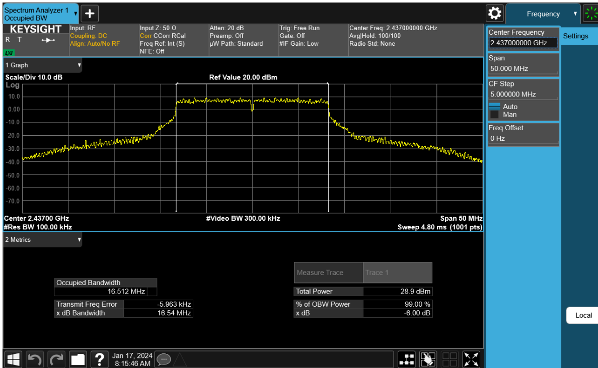
Plot 7-83. 6 dB BW and 99% OBW Plot Antenna WF9 (802.11g – Ch. 6) – 54Mbps
