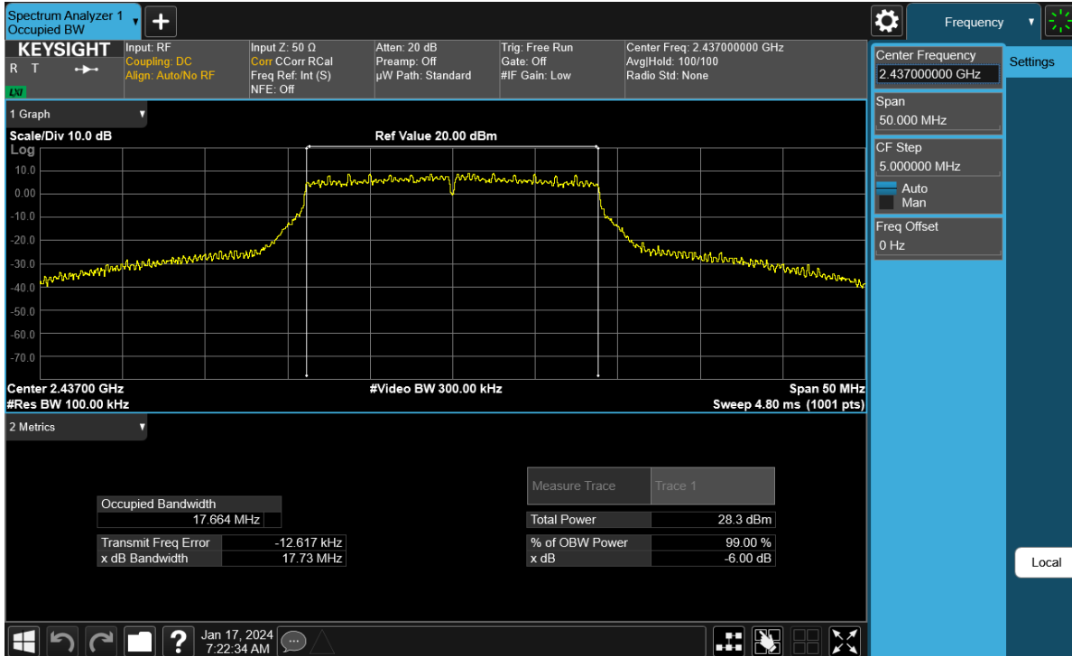
Plot 7-44. 6 dB BW and 99% OBW Plot Antenna WF7 (802.11n (2.4GHz) – Ch. 6) – MCS4
