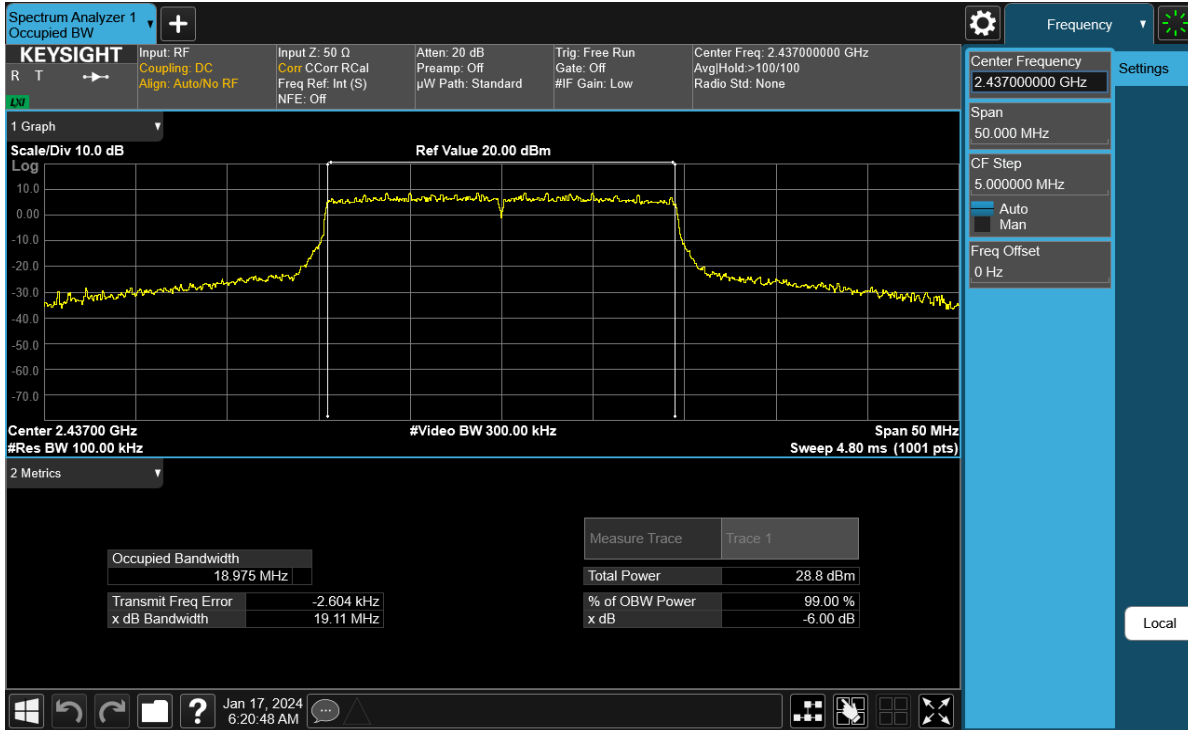
Plot 7-29. 6 dB BW and 99% OBW Plot Antenna WF8 (802.11ax (SU - 2.4GHz) – Ch. 6) – MCS9
