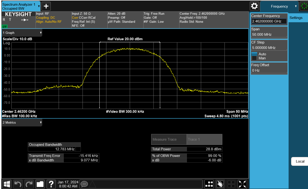
Plot 7-81. 6 dB BW and 99% OBW Plot Antenna WF9 (802.11b – Ch. 11) – 11Mbps
