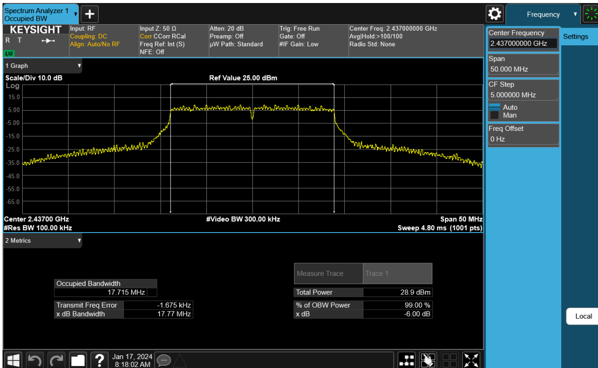
Plot 7-86. 6 dB BW and 99% OBW Plot Antenna WF9 (802.11n (2.4GHz) – Ch. 6) – MCS7
