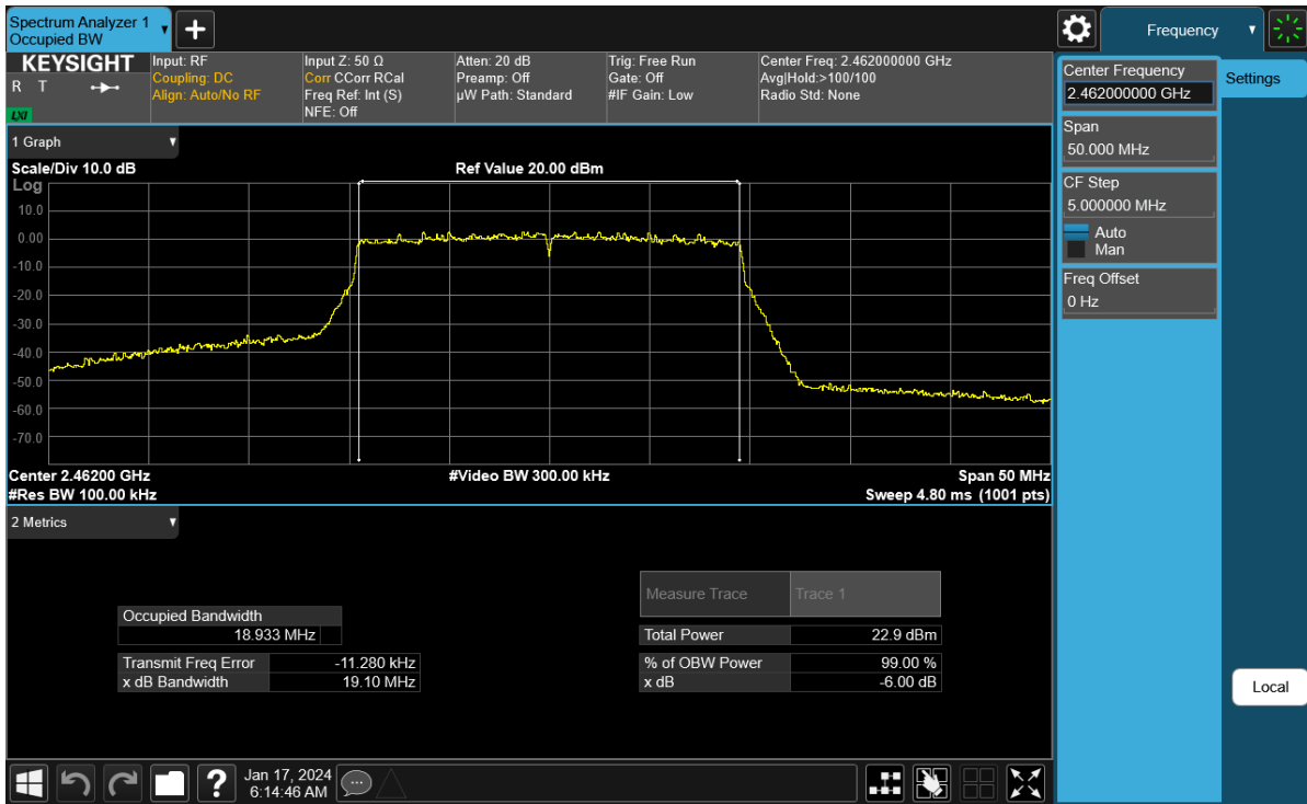
Plot 7-18. 6 dB BW and 99% OBW Plot Antenna WF8 (802.11ax (SU - 2.4GHz) - Ch. 11) - MCS4
