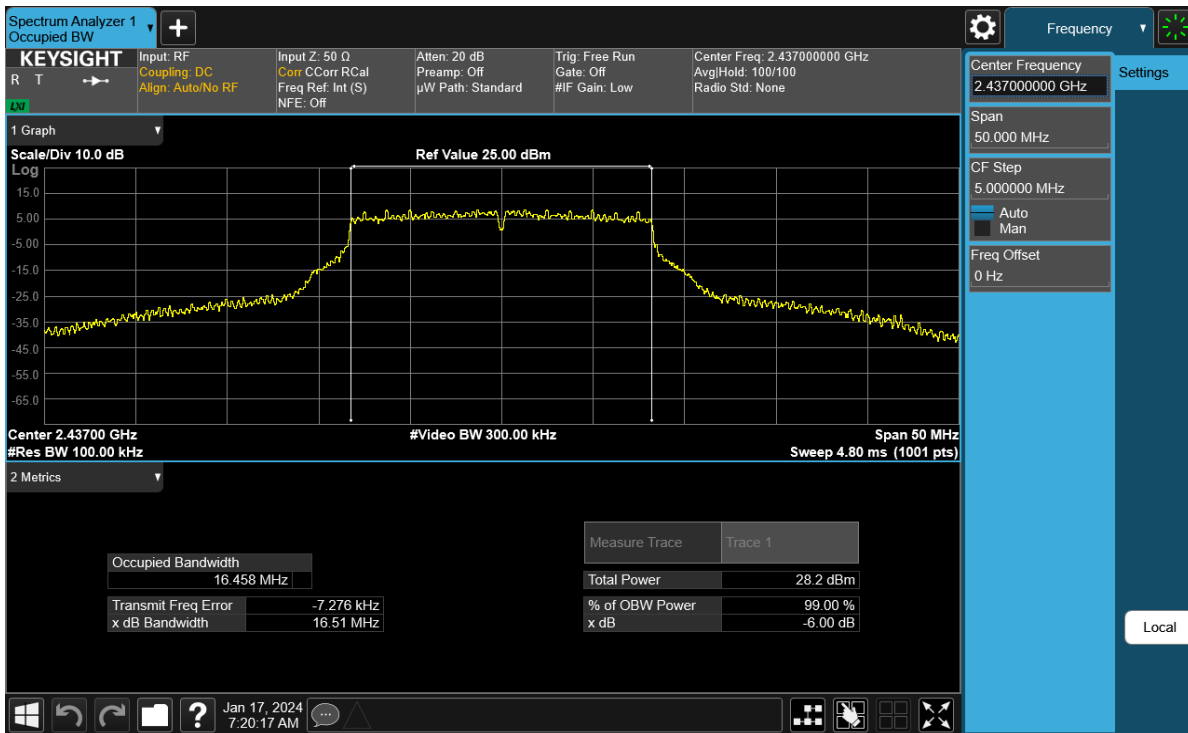
Plot 7-41. 6 dB BW and 99% OBW Plot Antenna WF7 (802.11g – Ch. 6) – 24Mbps
