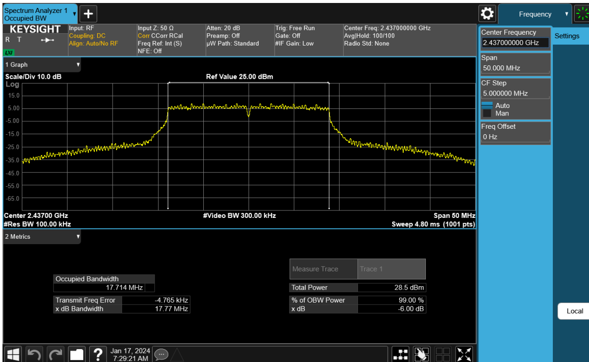
Plot 7-56. 6 dB BW and 99% OBW Plot Antenna WF7 (802.11n (2.4GHz) – Ch. 6) – MCS7
