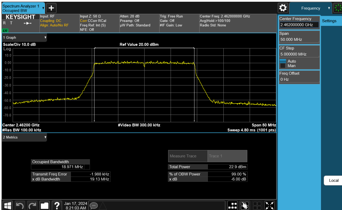
Plot 7-90. 6 dB BW and 99% OBW Plot Antenna WF9 (802.11ax (SU - 2.4GHz) – Ch. 11) – MCS9
