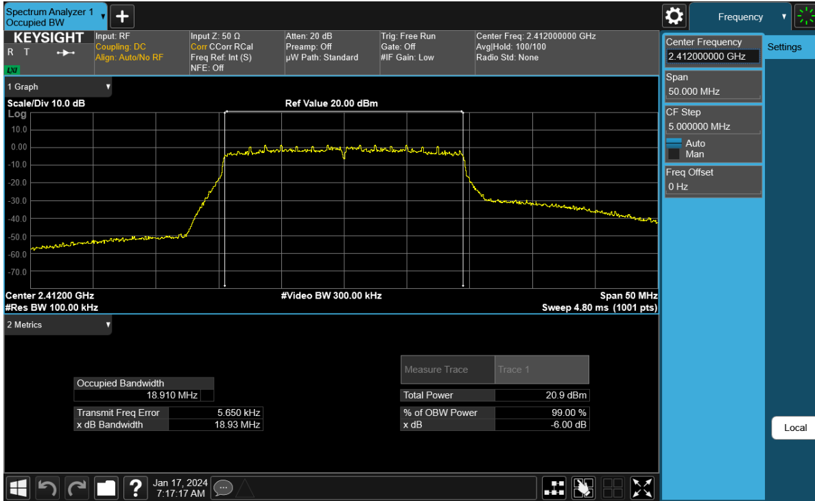
Plot 7-37. 6 dB BW and 99% OBW Plot Antenna WF7 (802.11ax (SU - 2.4GHz) – Ch. 1) – MCS2
