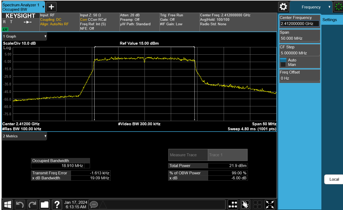
Plot 7-16. 6 dB BW and 99% OBW Plot Antenna WF8 (802.11ax (SU - 2.4GHz) - Ch. 1) - MCS4
