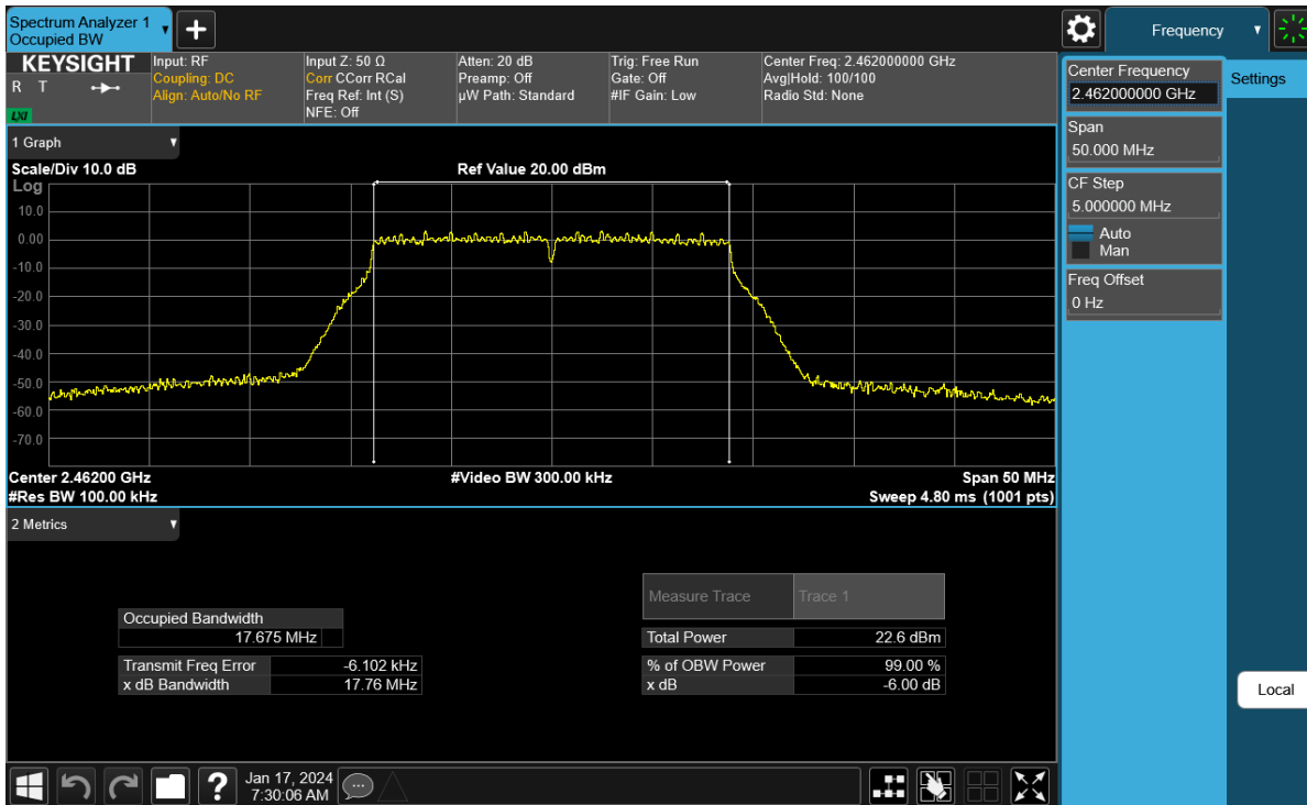
Plot 7-57. 6 dB BW and 99% OBW Plot Antenna WF7 (802.11n (2.4GHz) – Ch. 11) – MCS7
