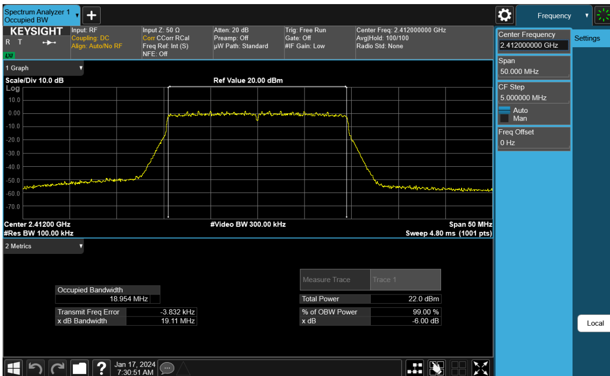
Plot 7-58. 6 dB BW and 99% OBW Plot Antenna WF7 (802.11ax (SU - 2.4GHz) – Ch. 1) – MCS9
