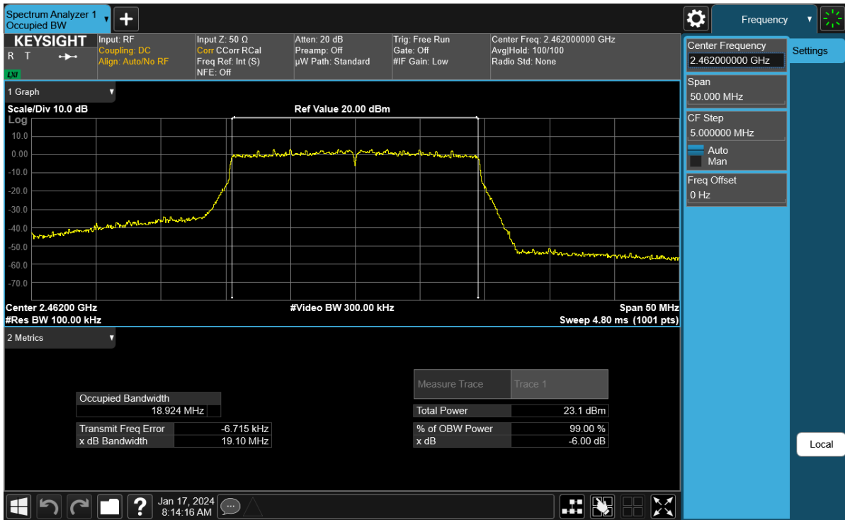
Plot 7-78. 6 dB BW and 99% OBW Plot Antenna WF9 (802.11ax (SU - 2.4GHz) - Ch. 11) - MCS4
