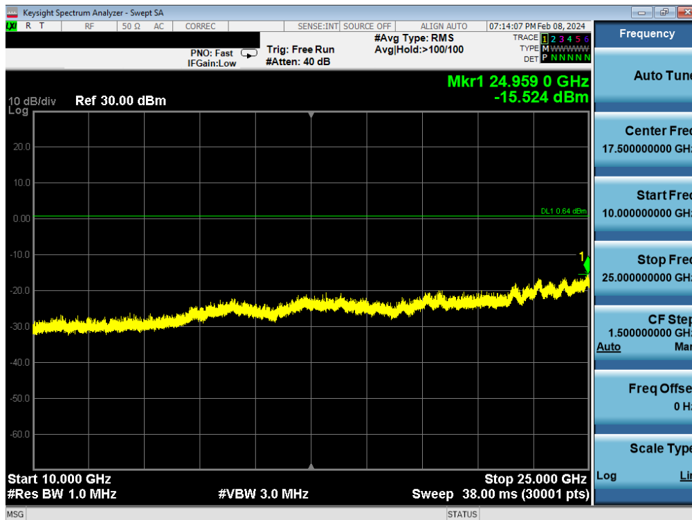
Plot 7-108. Conducted Spurious Plot Antenna WF9 (Bluetooth (LE), 1Mbps, ePA – Ch. 39)
