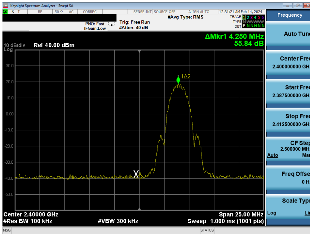
Plot 7-89. Band Edge Plot Antenna WF9 (Bluetooth (LE), 2Mbps, ePA – Ch. 1)
