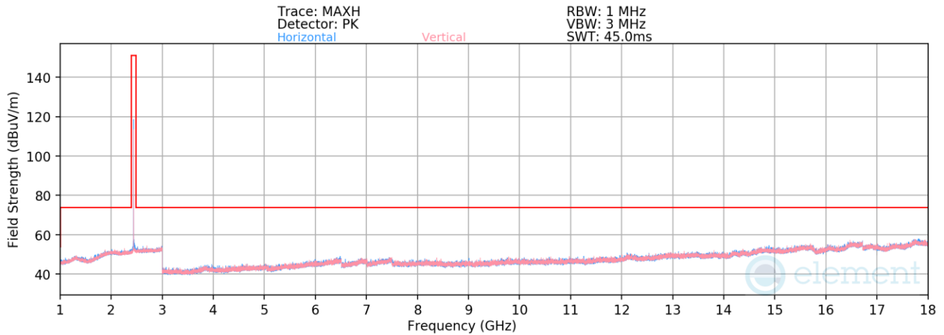
Plot 7-110. Radiated Spurious Emissions 1-18GHz Antenna WF8 (1Mbps, ePA – Ch. 19)
