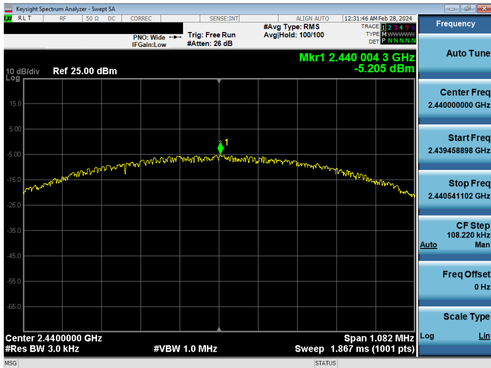
Plot 7-58. Power Spectral Density Plot Antenna WF7 (Bluetooth (LE), 1Mbps, ePA – Ch. 19)
