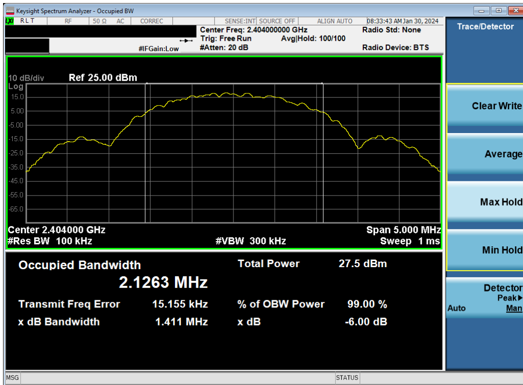
Plot 7-16. 6dB BW & 99% OBW Plot Antenna WF9 (Bluetooth (LE), 2Mbps, ePA – Ch. 1)
