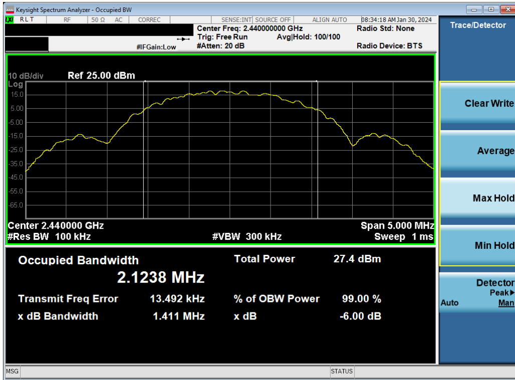
Plot 7-17. 6dB BW & 99% OBW Plot Antenna WF9 (Bluetooth (LE), 2Mbps, ePA – Ch. 19)
