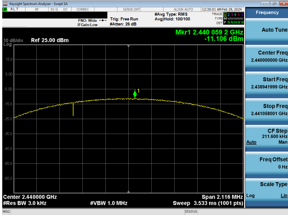
Plot 7-38. Power Spectral Density Plot Antenna WF7 (Bluetooth (LE), 2Mbps, ePA – Ch. 19)
