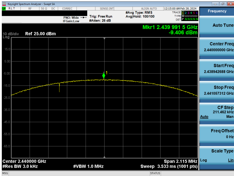
Plot 7-69. Power Spectral Density Plot Antenna WF8 (Bluetooth (LE), 2Mbps, ePA – Ch. 19)
