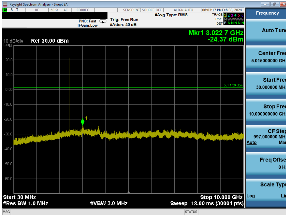
Plot 7-93. Conducted Spurious Plot Antenna WF8 (Bluetooth (LE), 1Mbps, ePA – Ch. 19)
