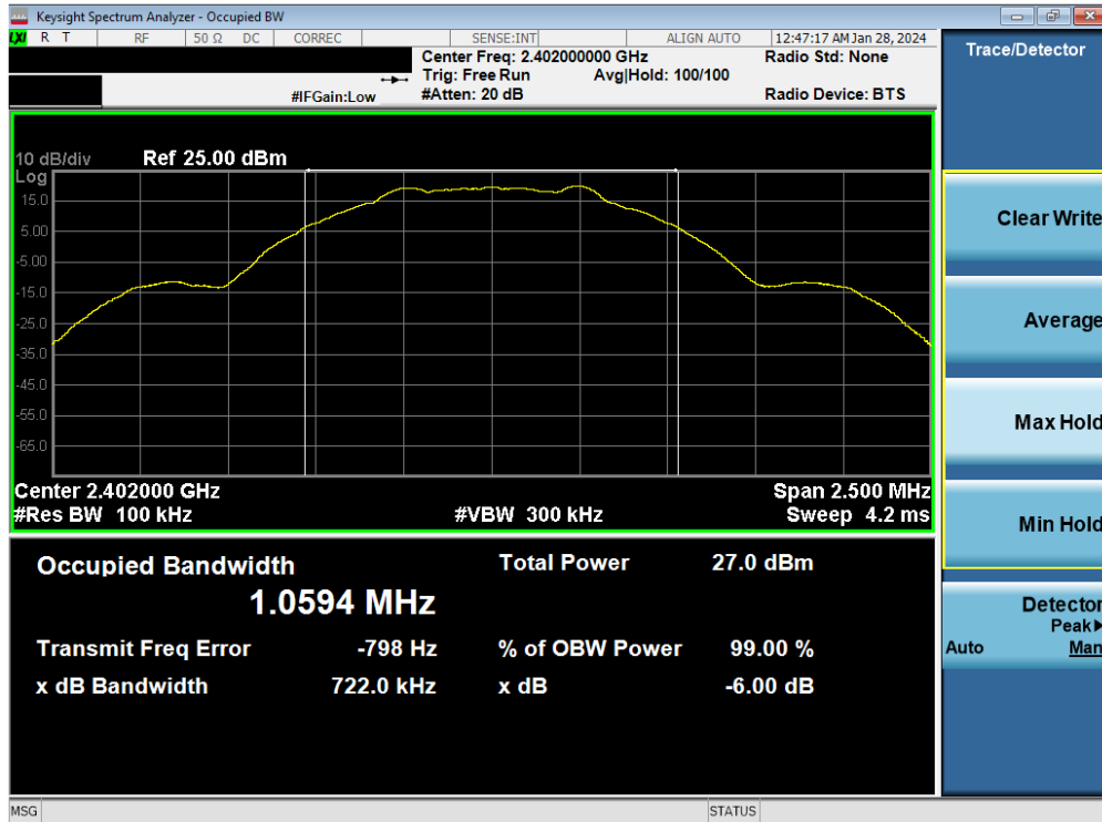
Plot 7-1. 6dB BW & 99% OBW Plot Antenna WF8 (Bluetooth (LE), 1Mbps, ePA – Ch. 0)
