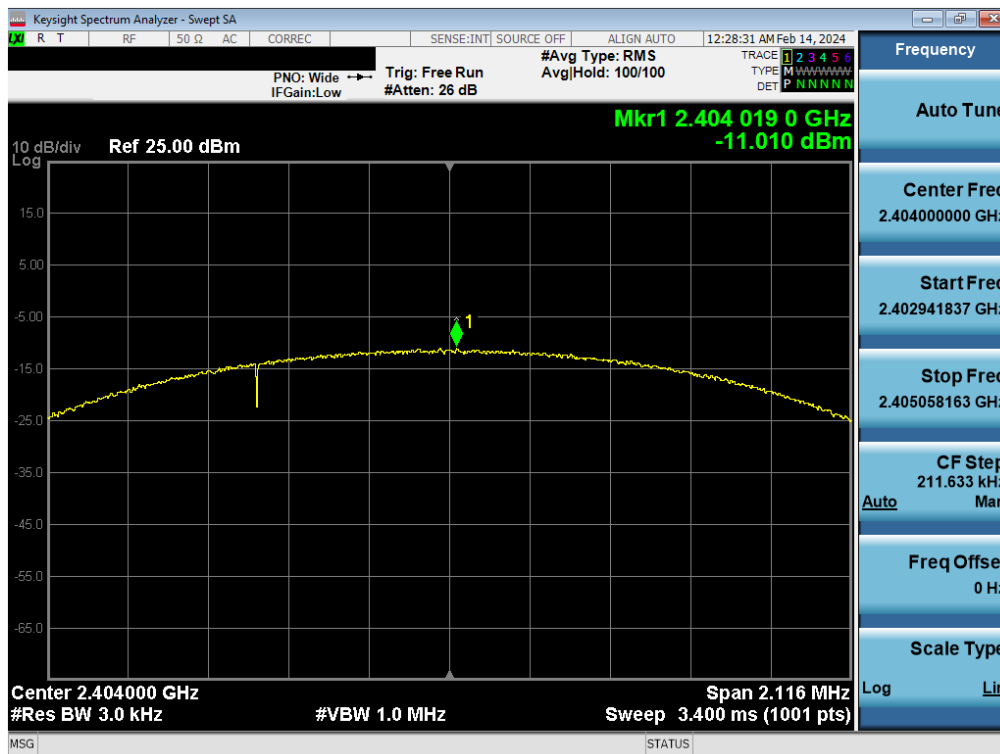
Plot 7-52. Power Spectral Density Plot Antenna WF9 (Bluetooth (LE), 2Mbps, iPA – Ch. 1)
