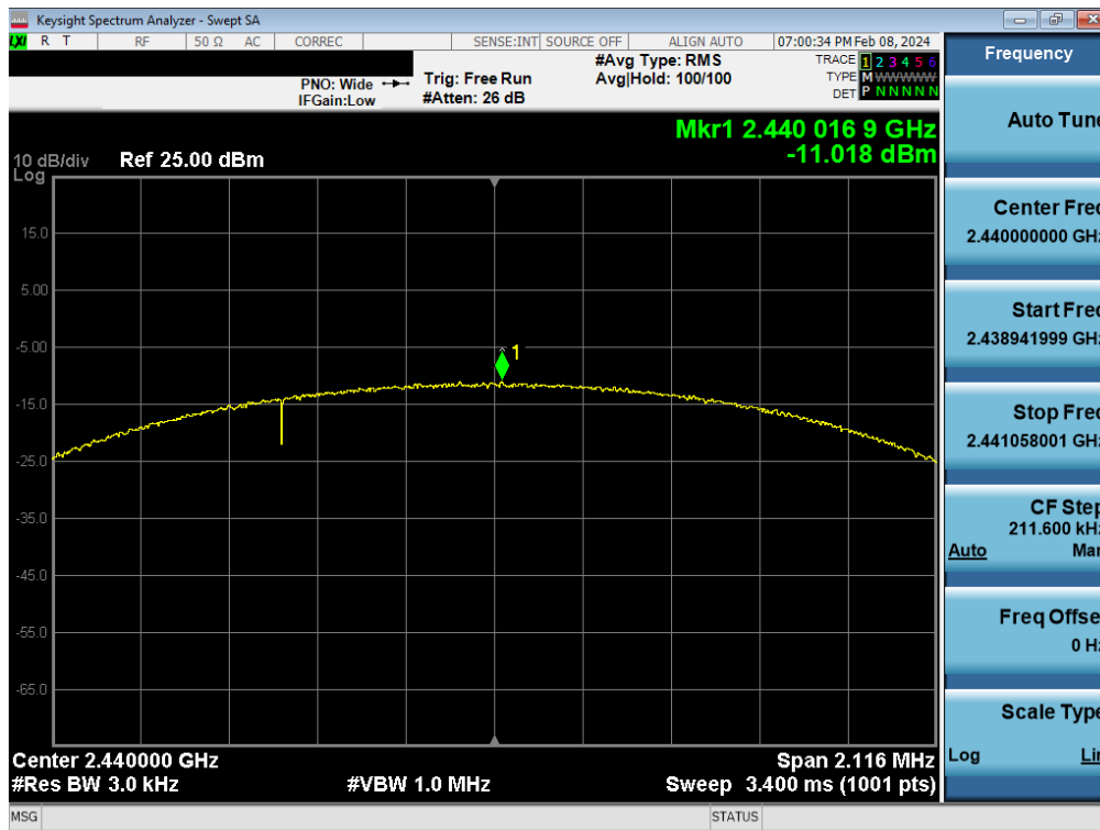
Plot 7-41. Power Spectral Density Plot Antenna WF7 (Bluetooth (LE), 2Mbps, iPA – Ch. 19)
