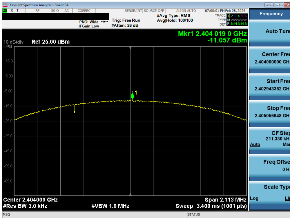
Plot 7-40. Power Spectral Density Plot Antenna WF7 (Bluetooth (LE), 2Mbps, iPA – Ch. 1)
