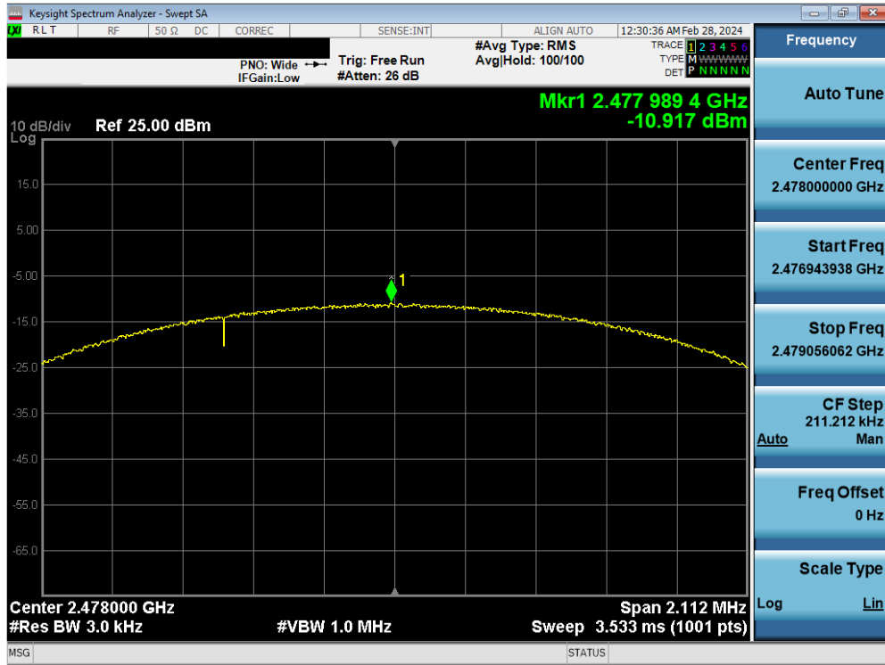
Plot 7-39. Power Spectral Density Plot Antenna WF7 (Bluetooth (LE), 2Mbps, ePA – Ch. 38)
