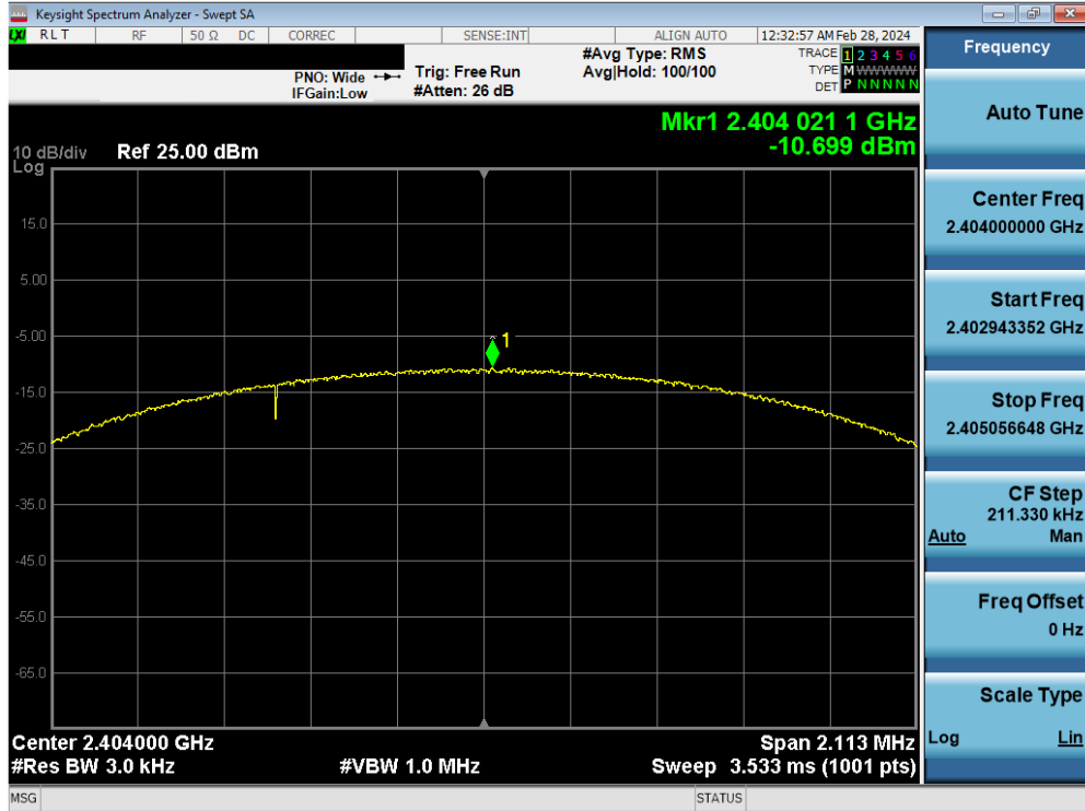
Plot 7-68. Power Spectral Density Plot Antenna WF7 (Bluetooth (LE), 2Mbps, ePA – Ch. 1)
