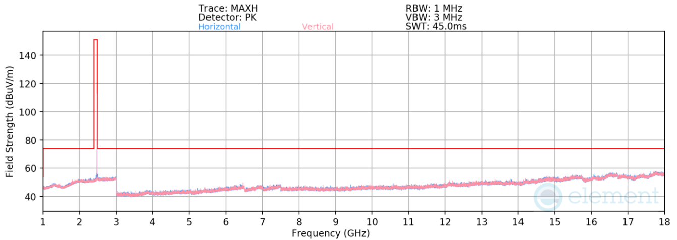
Plot 7-111. Radiated Spurious Emissions 1-18GHz Antenna WF8 (1Mbps ePA – Ch. 39)
