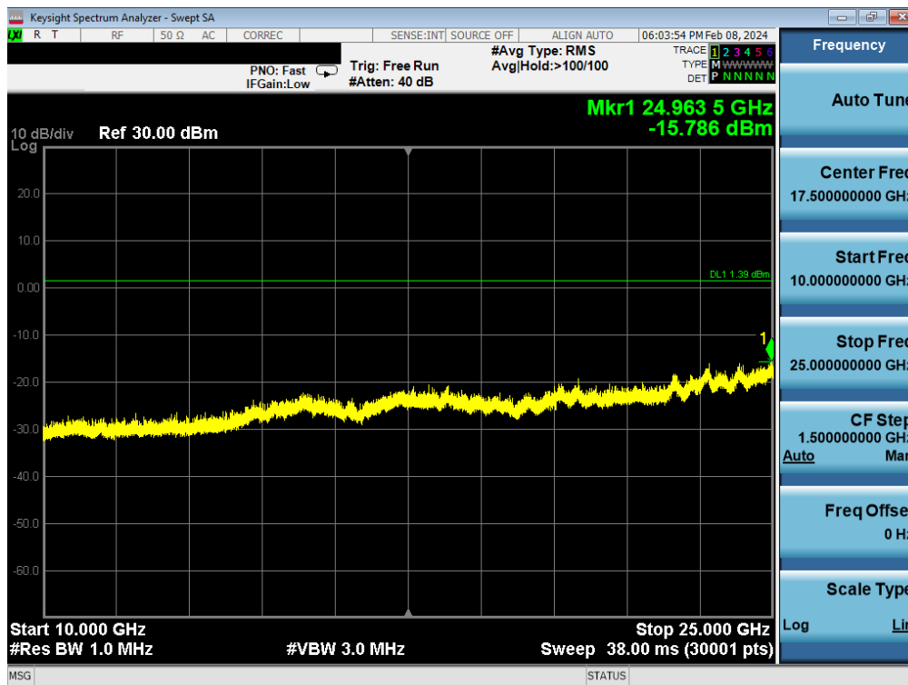
Plot 7-94. Conducted Spurious Plot Antenna WF8 (Bluetooth (LE), 1Mbps, ePA – Ch. 19)
