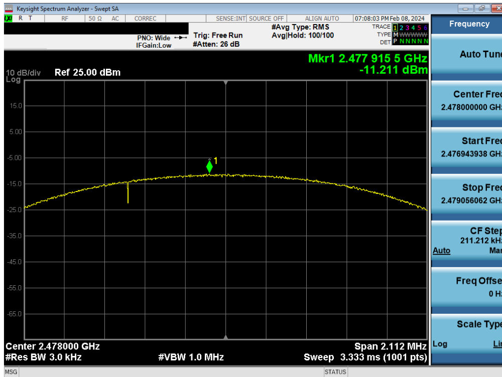
Plot 7-78. Power Spectral Density Plot Antenna WF7 (Bluetooth (LE), 2Mbps, iPA – Ch. 38)
