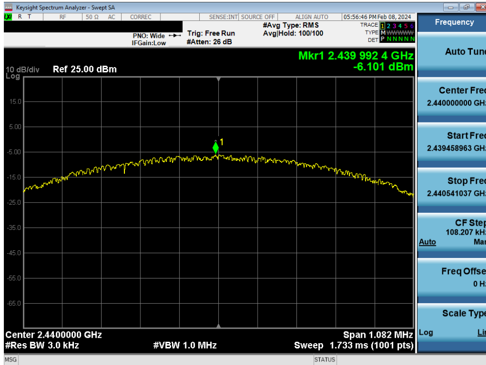
Plot 7-63. Power Spectral Density Plot Antenna WF8 (Bluetooth (LE), 1Mbps, iPA – Ch. 19)
