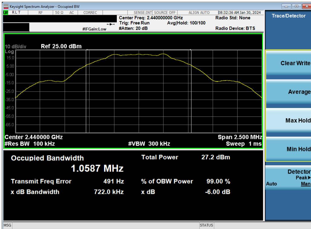
Plot 7-14. 6dB BW & 99% OBW Plot Antenna WF9 (Bluetooth (LE), 1Mbps, ePA – Ch. 19)
