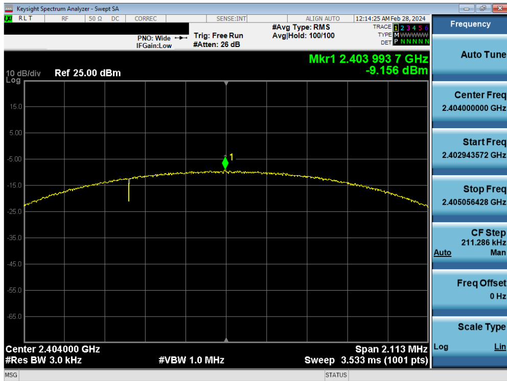
Plot 7-67. Power Spectral Density Plot Antenna WF8 (Bluetooth (LE), 2Mbps, ePA – Ch. 1)
