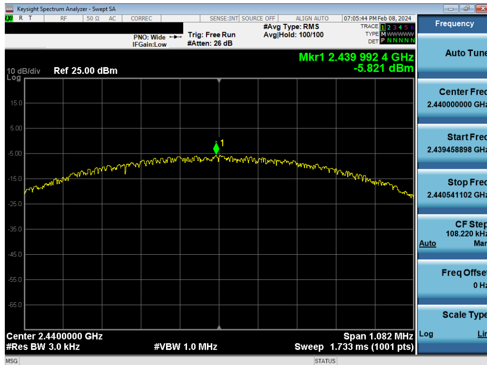
Plot 7-64. Power Spectral Density Plot Antenna WF7 (Bluetooth (LE), 1Mbps, iPA – Ch. 19)
