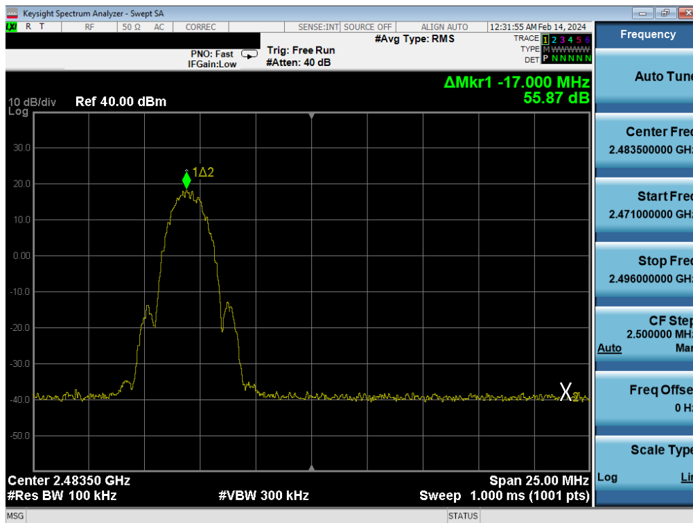
Plot 7-90. Band Edge Plot Antenna WF9 (Bluetooth (LE), 2Mbps, ePA – Ch. 38)
