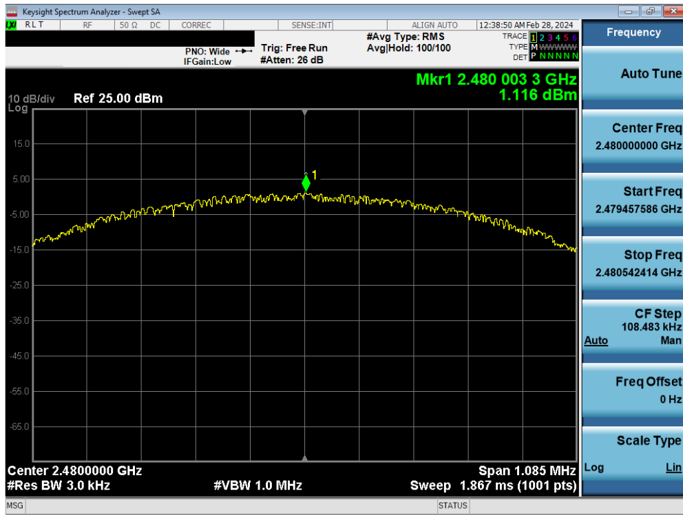
Plot 7-45. Power Spectral Density Plot Antenna WF9 (Bluetooth (LE), 1Mbps, ePA – Ch. 39)
