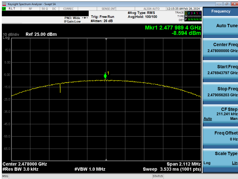
Plot 7-71. Power Spectral Density Plot Antenna WF8 (Bluetooth (LE), 2Mbps, ePA – Ch. 38)
