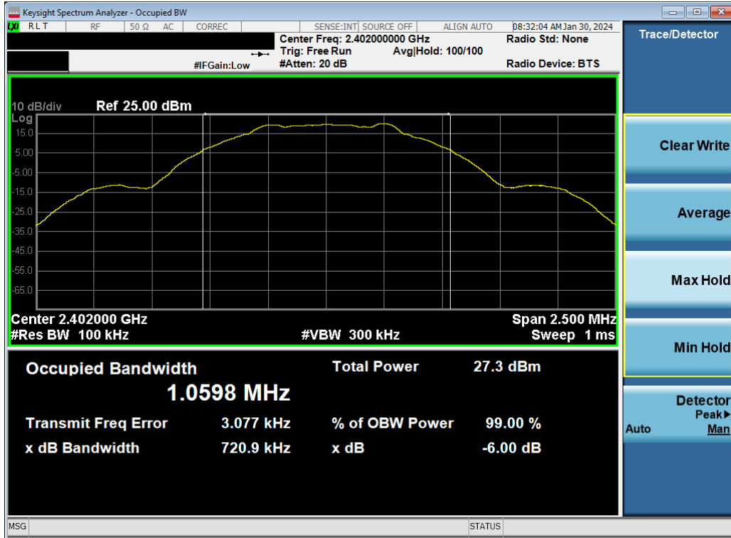
Plot 7-13. 6dB BW & 99% OBW Plot Antenna WF9 (Bluetooth (LE), 1Mbps, ePA – Ch. 0)
