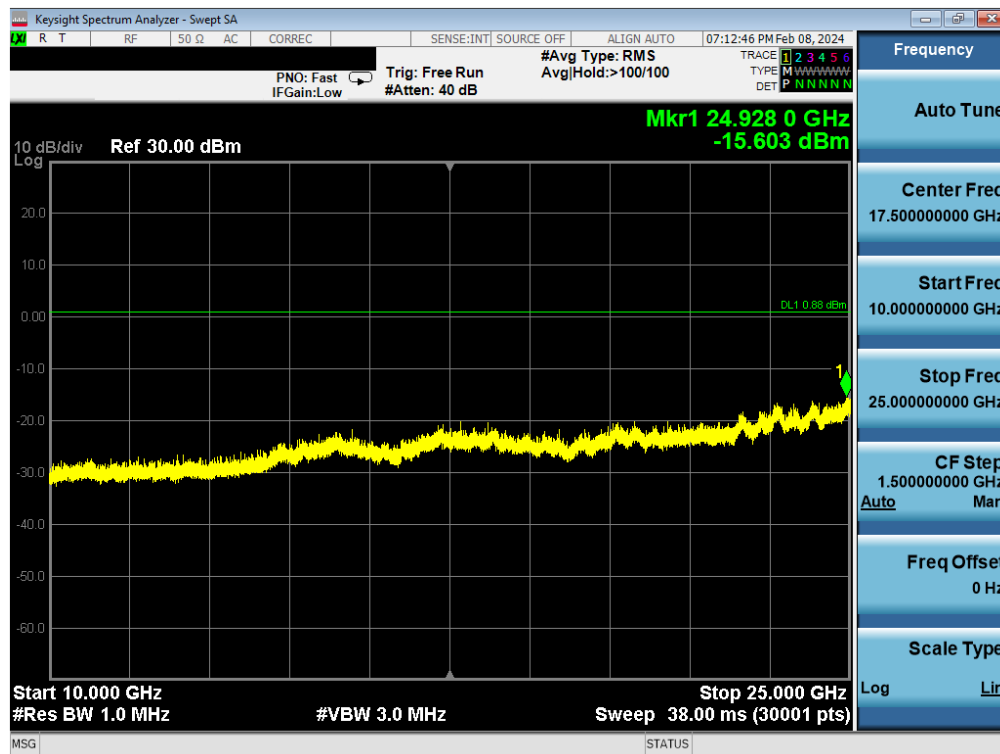
Plot 7-100. Conducted Spurious Plot Antenna WF7 (Bluetooth (LE), 1Mbps, ePA – Ch. 19)
