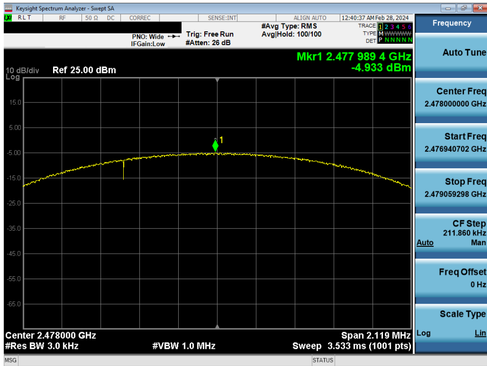
Plot 7-51. Power Spectral Density Plot Antenna WF9 (Bluetooth (LE), 2Mbps, ePA – Ch. 38)
