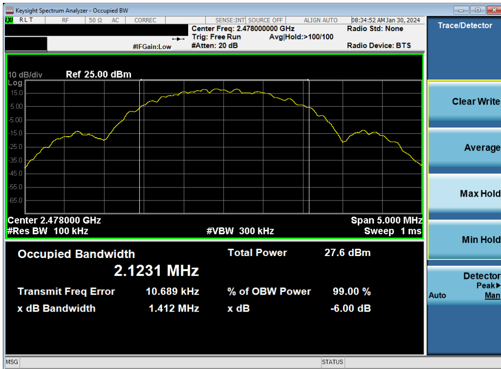
Plot 7-18. 6dB BW & 99% OBW Plot Antenna WF9 (Bluetooth (LE), 2Mbps, ePA – Ch. 38)
