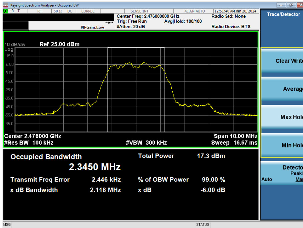
Plot 7-3. 6dB BW & 99% OBW Plot Antenna WF8 (Bluetooth (H4R), 4Mbps, ePA – Ch. 73)
