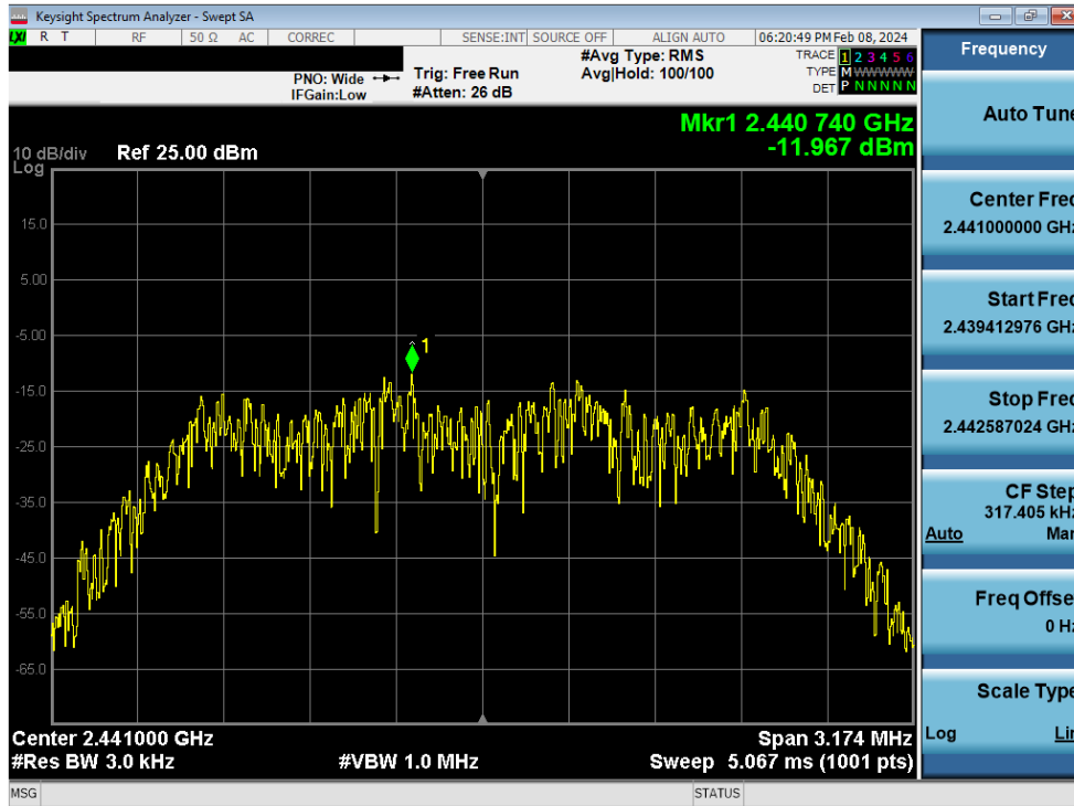
Plot 7-63. Power Spectral Density Plot TxBF Antenna WF8 (Bluetooth (HDR4), 4Mbps, iPA – Ch. 38)
