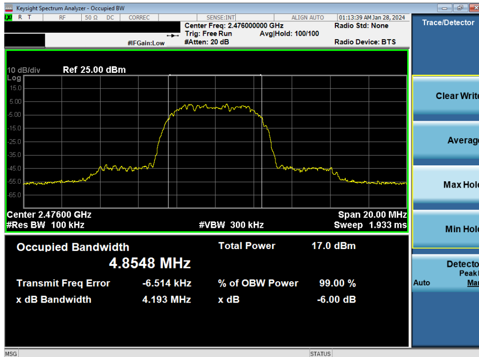
Plot 7-12. 6dB BW & 99% OBW Plot Antenna WF7 (Bluetooth (HDR8), 8Mbps, ePA – Ch. 73) Antenna WF9
