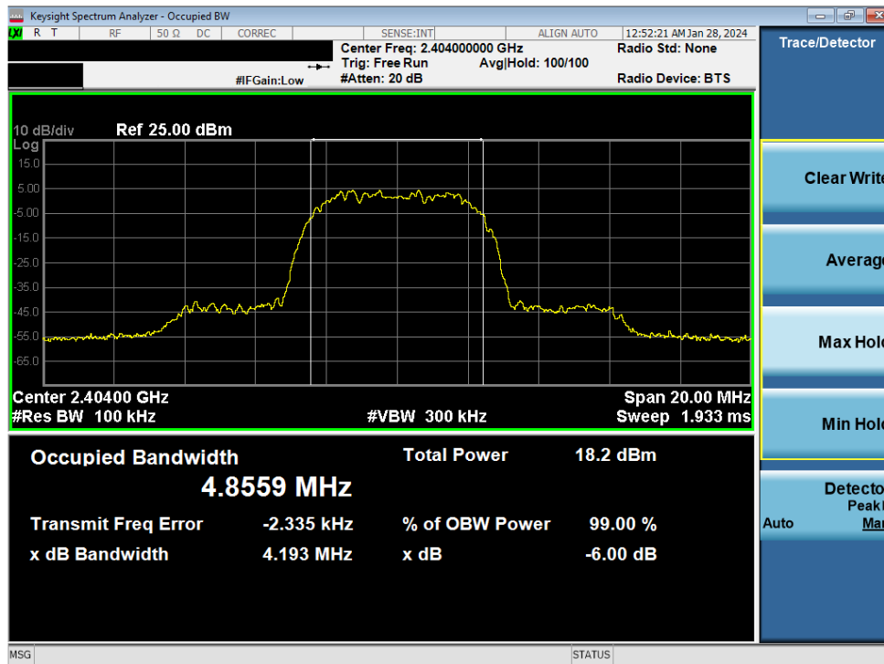
Plot 7-4. 6dB BW & 99% OBW Plot Antenna WF8 (Bluetooth (H8R), 8Mbps, ePA – Ch. 1)
