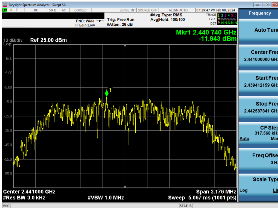
Plot 7-64. Power Spectral Density Plot TxBF Antenna WF7 (Bluetooth (HDR4), 4Mbps, iPA – Ch. 38)
