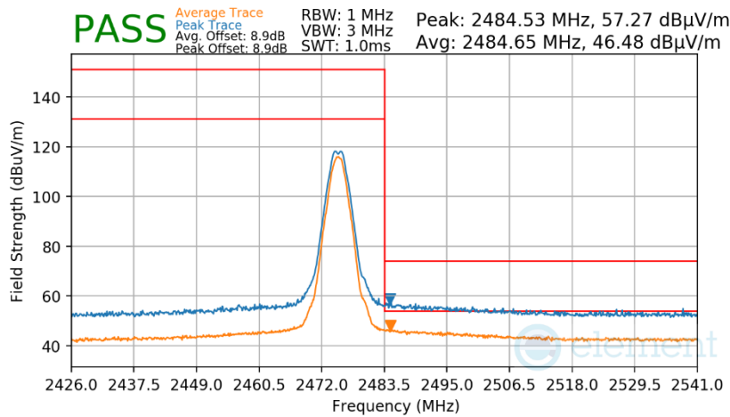
Plot 7-67. Radiated Restricted Upper Band Edge Measurement Antenna WF9
