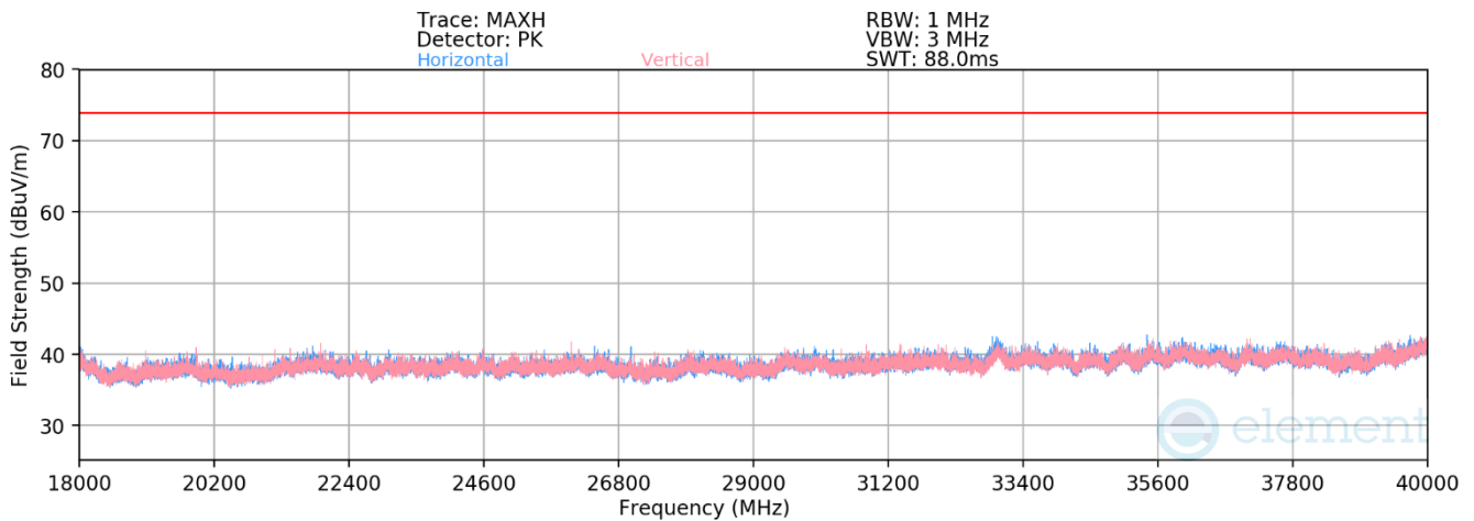
Plot 7-59. Radiated Spurious Emissions Above 18GHz Antenna WF9 (802.15.4 ePA – Ch.11)
