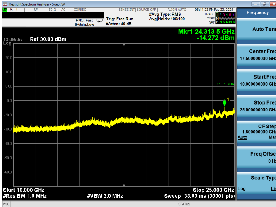
Plot 7-43. Conducted Spurious Antenna WF7 (802.15.4, ePA – Ch. 18)
