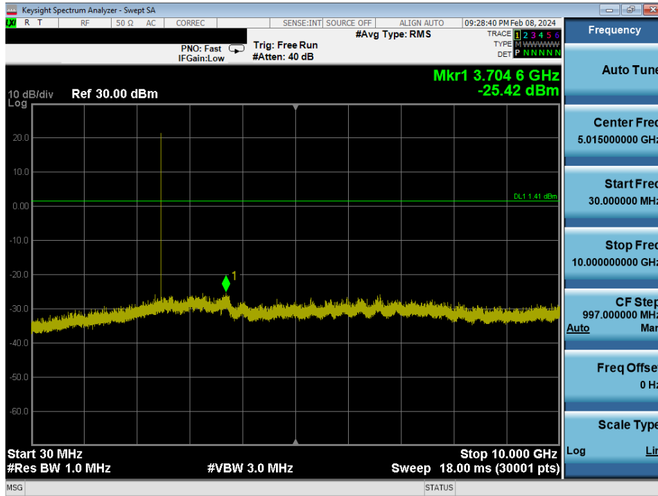
Plot 7-38. Conducted Spurious Antenna WF8 (802.15.4, ePA – Ch. 25)
