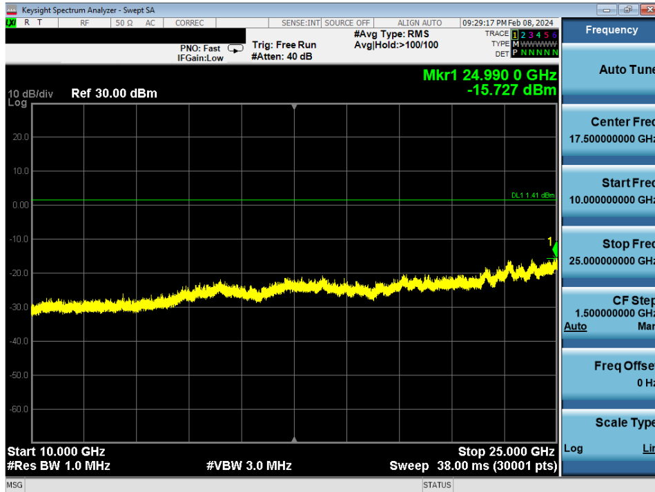
Plot 7-39. Conducted Spurious Antenna WF8 (802.15.4, ePA – Ch. 25)
