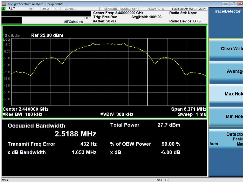
Plot 7-8. 6dB BW & 99% OBW Antenna WF9 (802.15.4, Ch. 18)
