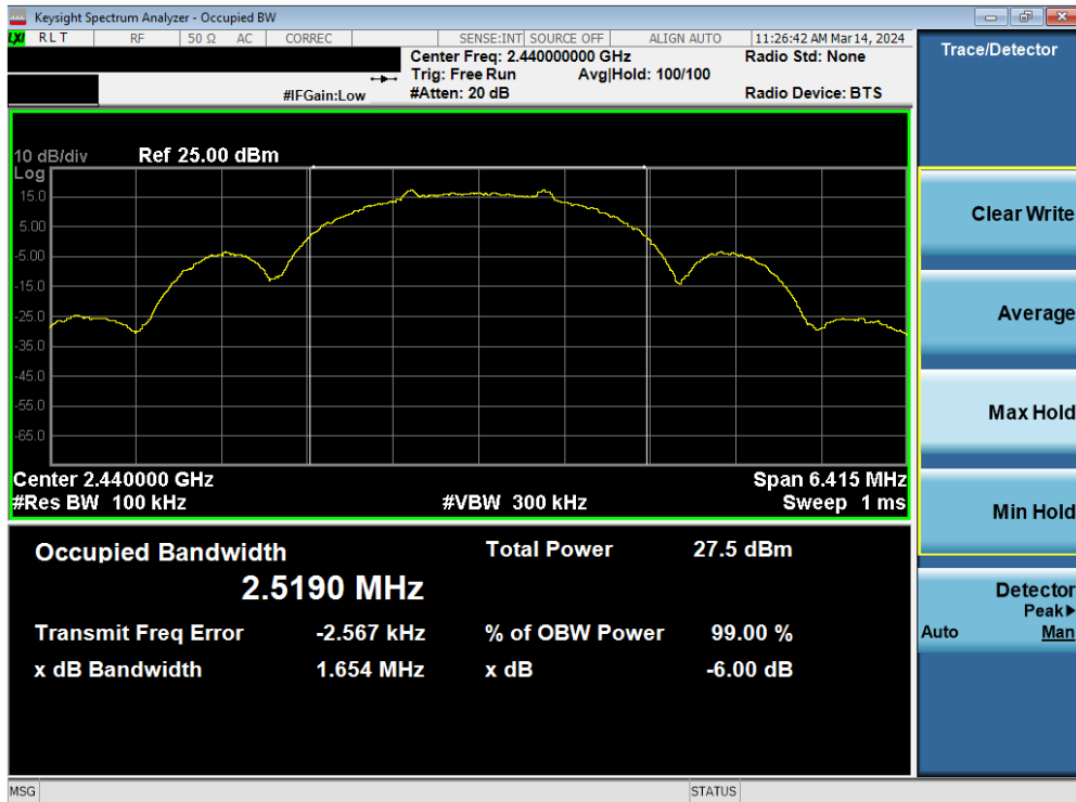
Plot 7-5. 6dB BW & 99% OBW Antenna WF7 (802.15.4, Ch. 18)
