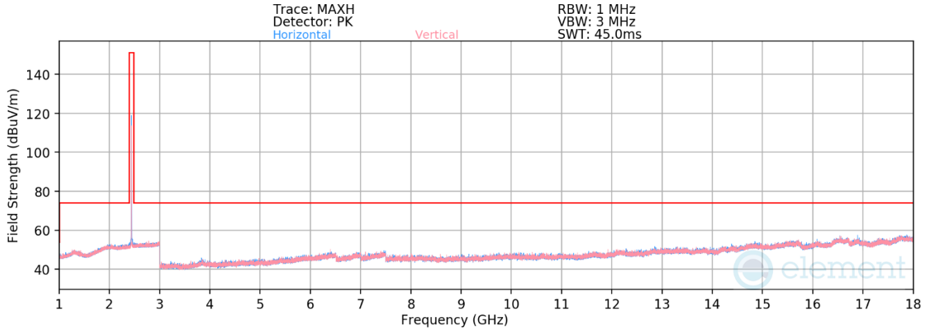
Plot 7-56. Radiated Spurious Emissions 1-18GHz Antenna WF7 (802.15.4 ePA – Ch. 18)
