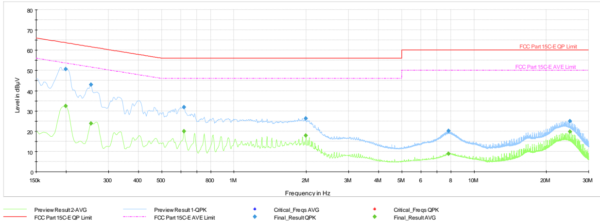
Plot 7-70. AC Line Conducted Emission with 802.15.4 Antenna WF9 (N, 250 kbps, ePA - Ch.11, with Laptop)
