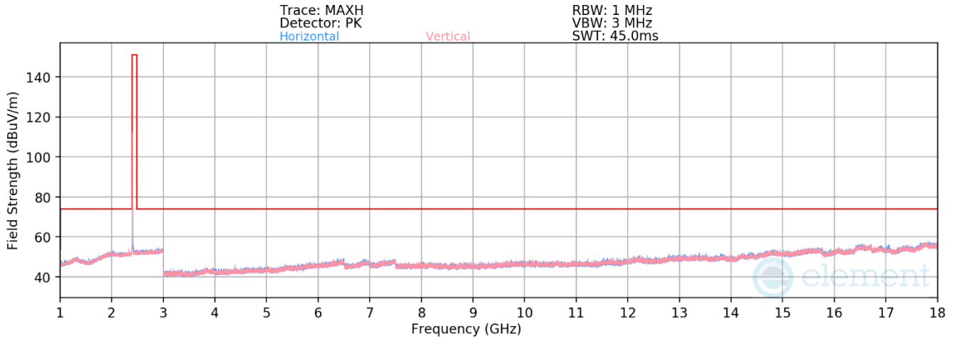
Plot 7-55. Radiated Spurious Emissions 1-18GHz Antenna WF7 (802.15.4 ePA – Ch. 11)
