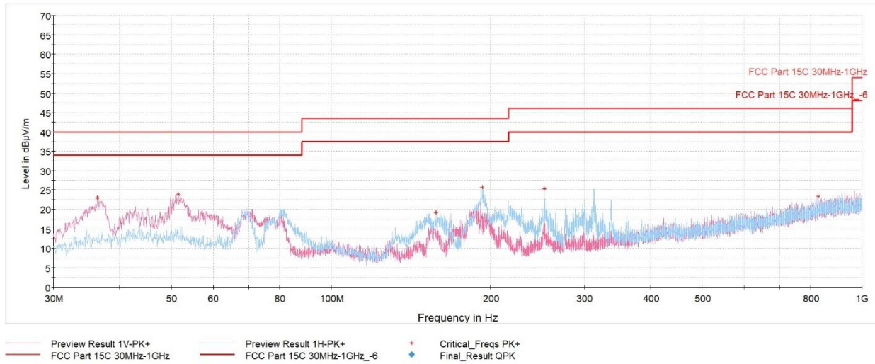
Plot 7-68. Radiated Spurious Emissions 30MHz-1GHz Antenna WF9 (250kbps, ePA - Ch.11, with AC/DC Adapter)
