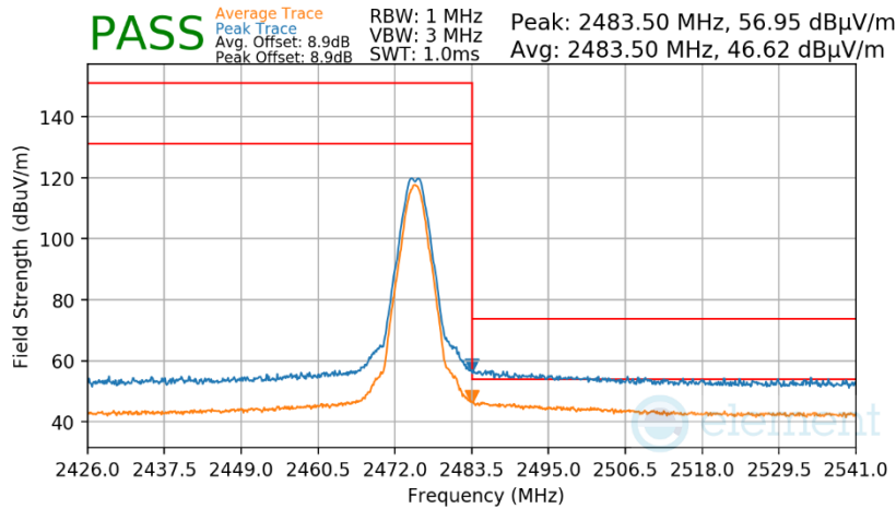
Plot 7-65. Radiated Restricted Upper Band Edge Measurement Antenna WF7
