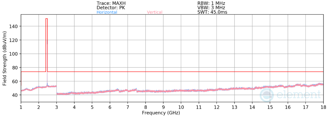
Plot 7-54. Radiated Spurious Emissions 1-18GHz Antenna WF8 (802.15.4 ePA – Ch. 25)
