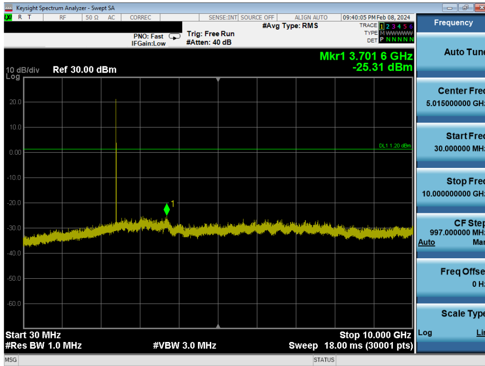
Plot 7-40. Conducted Spurious Antenna WF7 (802.15.4, ePA – Ch. 11)
