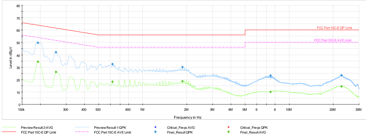
Plot 7-69. AC Line Conducted Emission with 802.15.4 Antenna WF9 (L1, 250 kbps, ePA - Ch.11, with Laptop)
