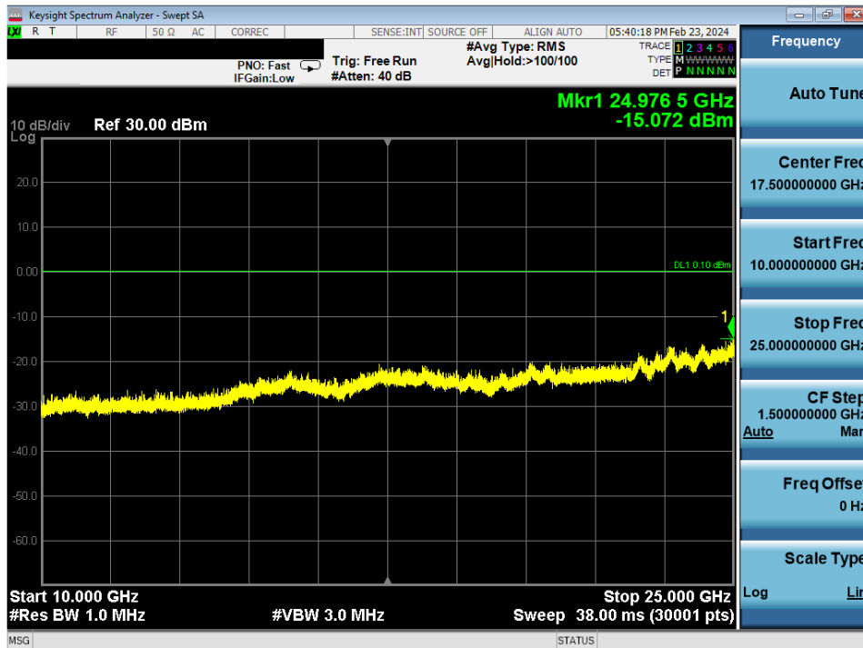
Plot 7-37. Conducted Spurious Antenna WF8 (802.15.4, ePA – Ch. 18)
