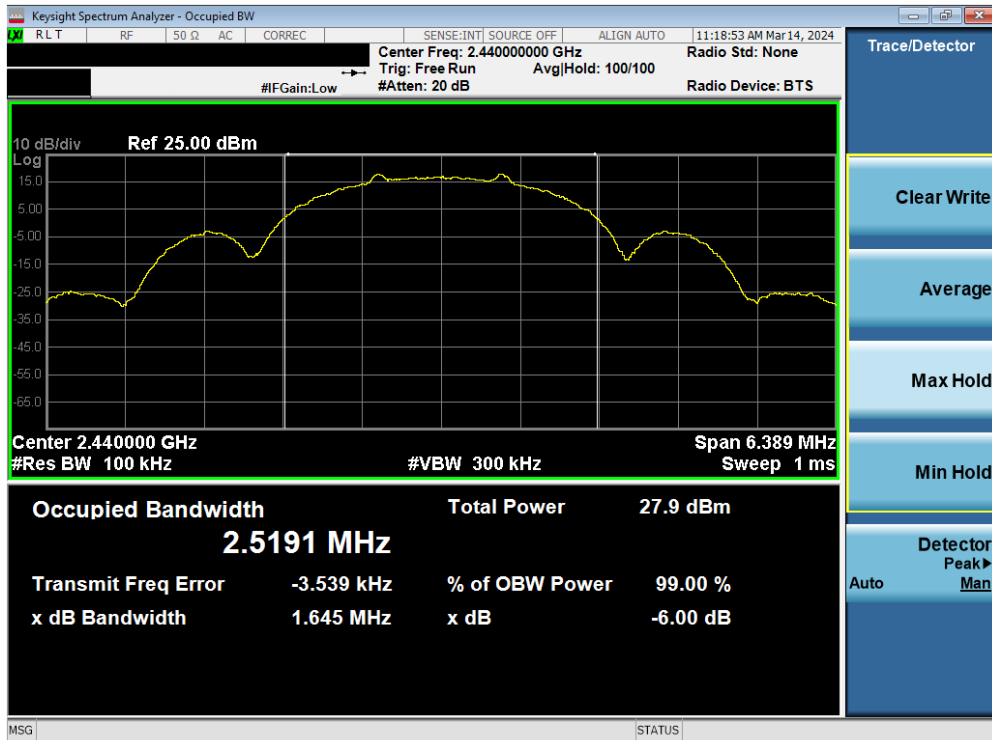
Plot 7-2. 6dB BW & 99% OBW Antenna WF8 (802.15.4, Ch. 18)
