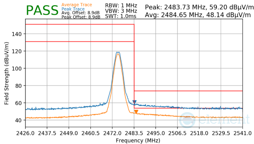
Plot 7-63. Radiated Restricted Upper Band Edge Measurement Antenna WF8
