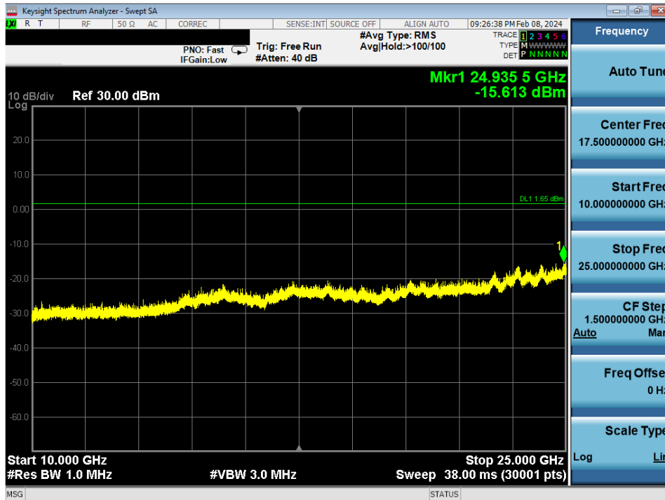
Plot 7-35. Conducted Spurious Antenna WF8 (802.15.4, ePA – Ch. 11)
