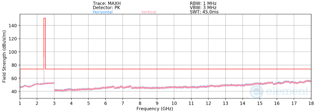
Plot 7-58. Radiated Spurious Emissions 1-18GHz Antenna WF9 (802.15.4 ePA – Ch. 11)
