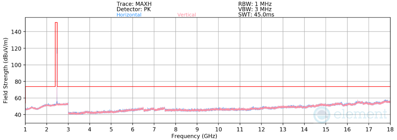
Plot 7-57. Radiated Spurious Emissions 1-18GHz Antenna WF7 (802.15.4 ePA – Ch. 25)
