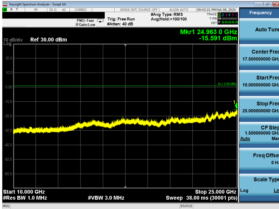
Plot 7-45. Conducted Spurious Antenna WF7 (802.15.4, ePA – Ch. 25)
