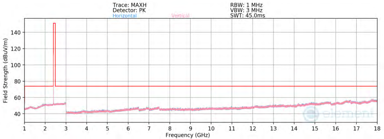
Plot 7-93. Radiated Spurious Emissions above 1GHz Antenna WF9 (BT GFSK ePA – Ch. 0)
