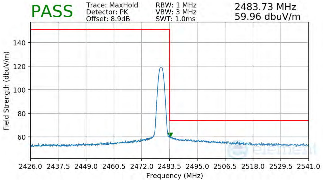
Plot 7-104. Radiated Restricted Upper Band Edge Measurement Antenna WF8
