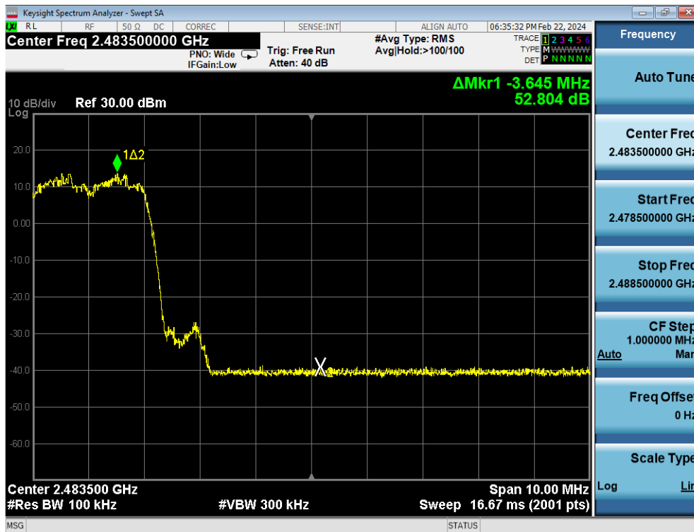
Plot 7-34. Band Edge Plot Antenna WF7 (Bluetooth with Hopping Enabled, 8DPSK, ePA)
