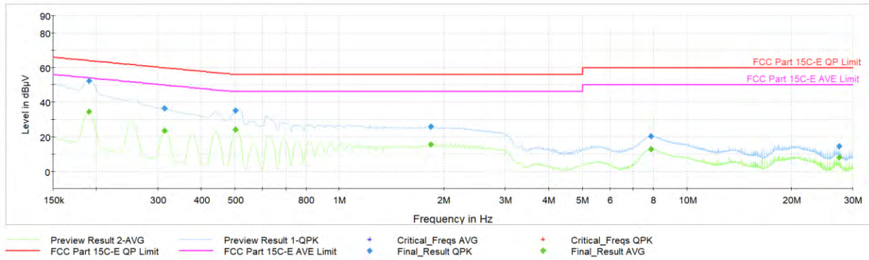
Plot 7-121. AC Line-Conducted Test Plot TxBF (N, GFSK ePA – Ch.39, with Laptop)
