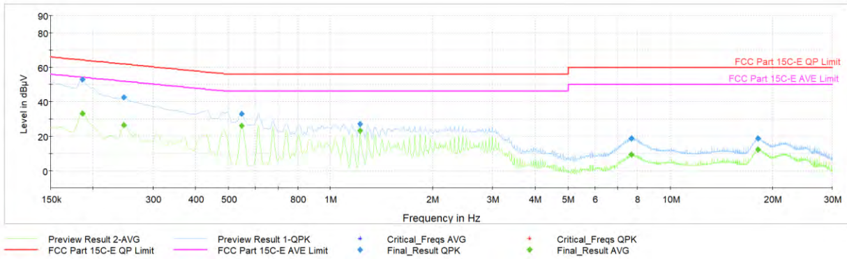
Plot 7-120. AC Line-Conducted Test Plot TxBF (L1, GFSK ePA – Ch.39, with Laptop)
