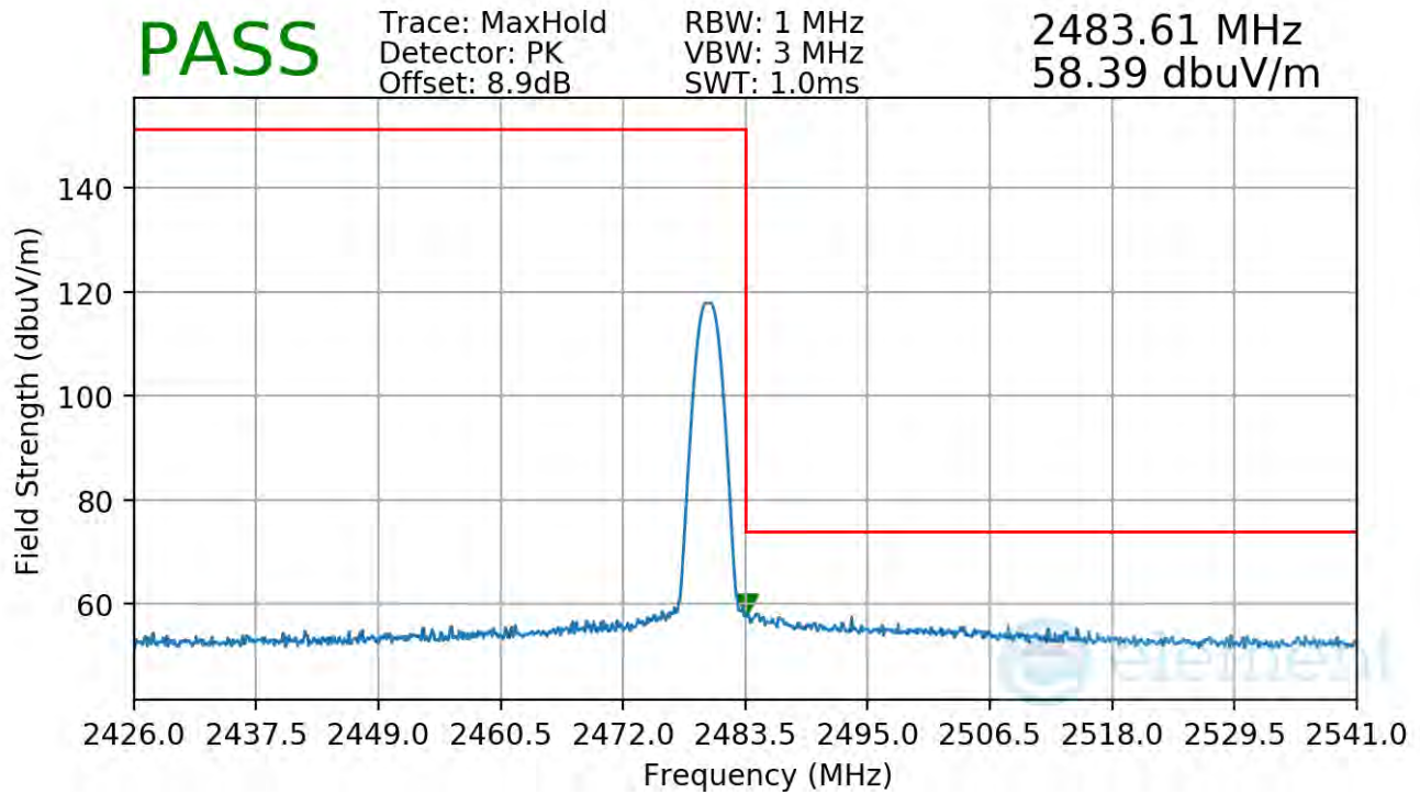
Plot 7-112. Radiated Restricted Upper Band Edge Measurement Antenna WF9
