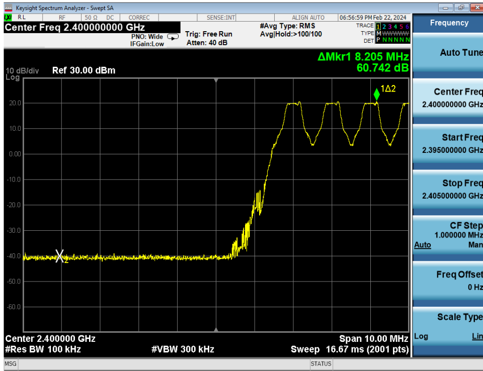
Plot 7-37. Band Edge Plot Antenna WF9 (Bluetooth with Hopping Enabled, GFSK, ePA)
