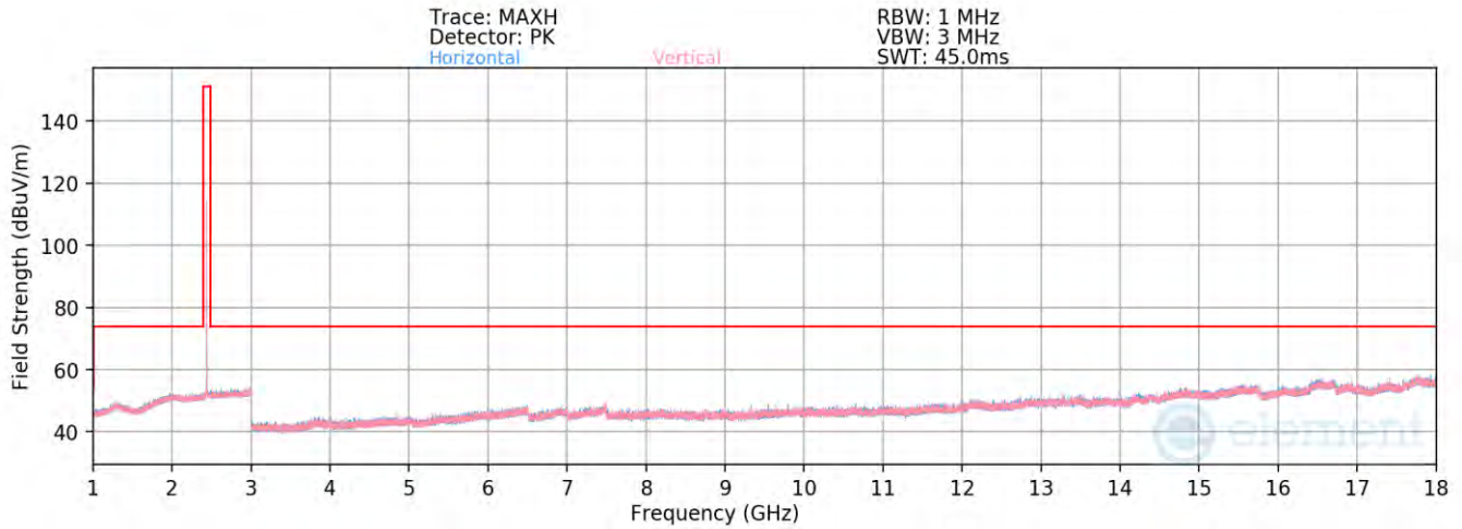
Plot 7-94. Radiated Spurious Emissions above 1GHz Antenna WF9 (BT GFSK ePA – Ch. 39)
