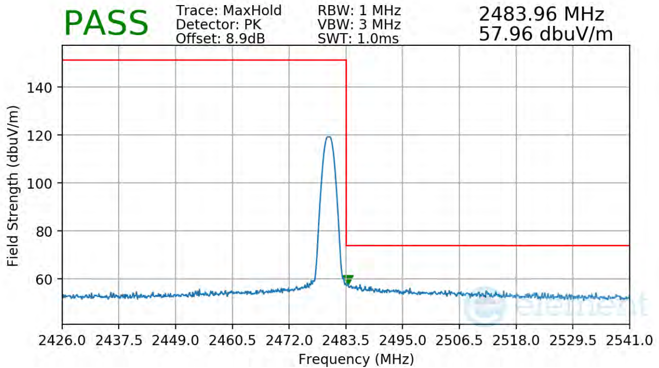
Plot 7-108. Radiated Restricted Upper Band Edge Measurement Antenna WF7
