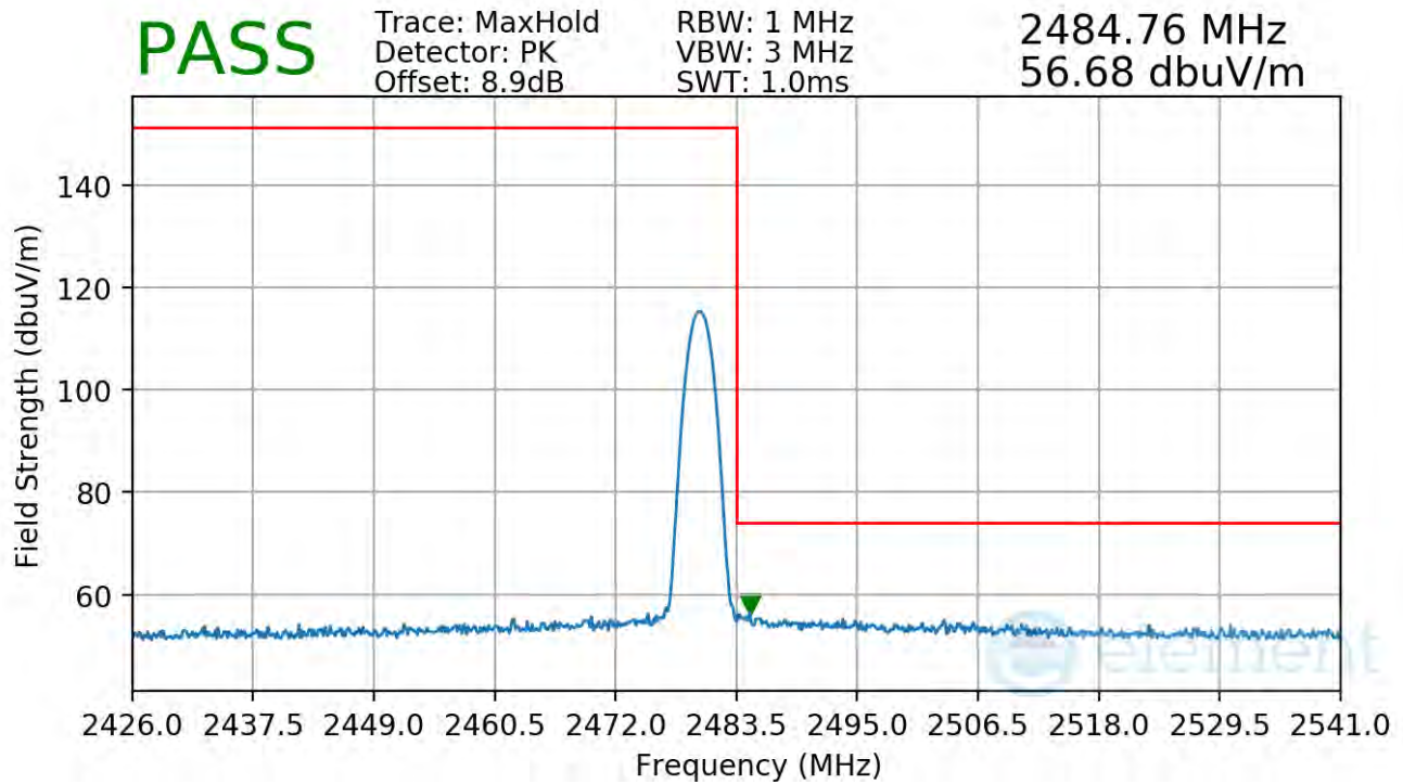
Plot 7-113. Radiated Restricted Upper Band Edge Measurement Antenna WF9
