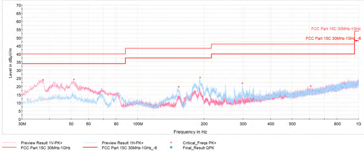
Plot 7-118. Radiated Spurious Emissions Below 1GHz TxBF (GFSK ePA – Ch.39, with AC/DC Adapter)
