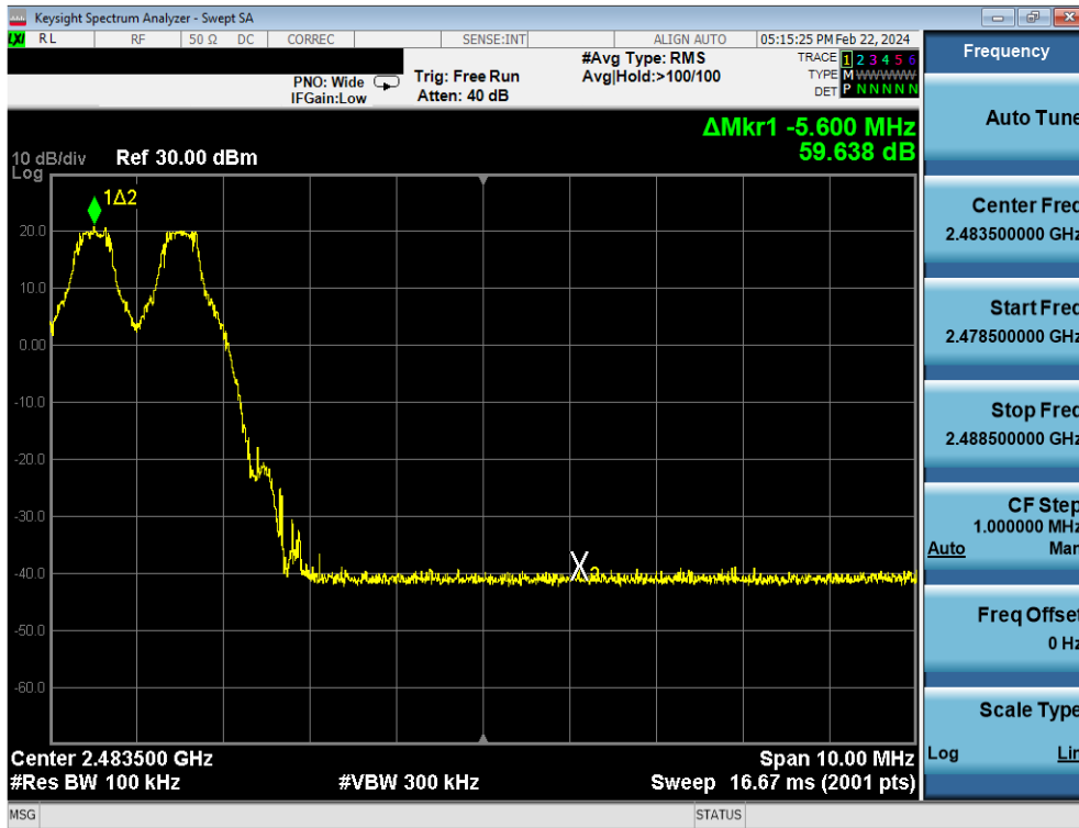
Plot 7-22. Band Edge Plot Antenna WF8 (Bluetooth with Hopping Enabled, GFSK, ePA)
