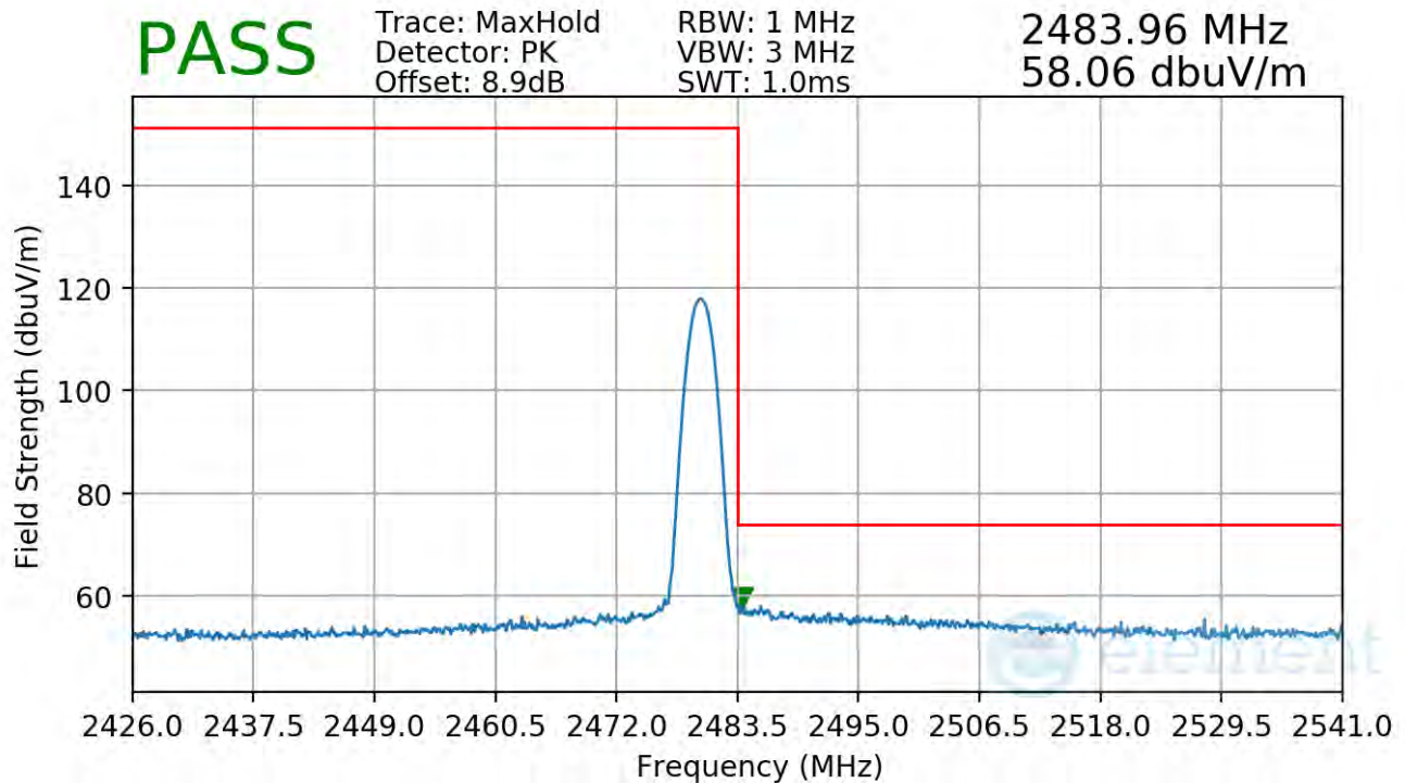
Plot 7-105. Radiated Restricted Upper Band Edge Measurement Antenna WF8
