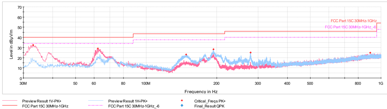
Plot 7-119. Worst Case Simultaneous Transmission Configuration
