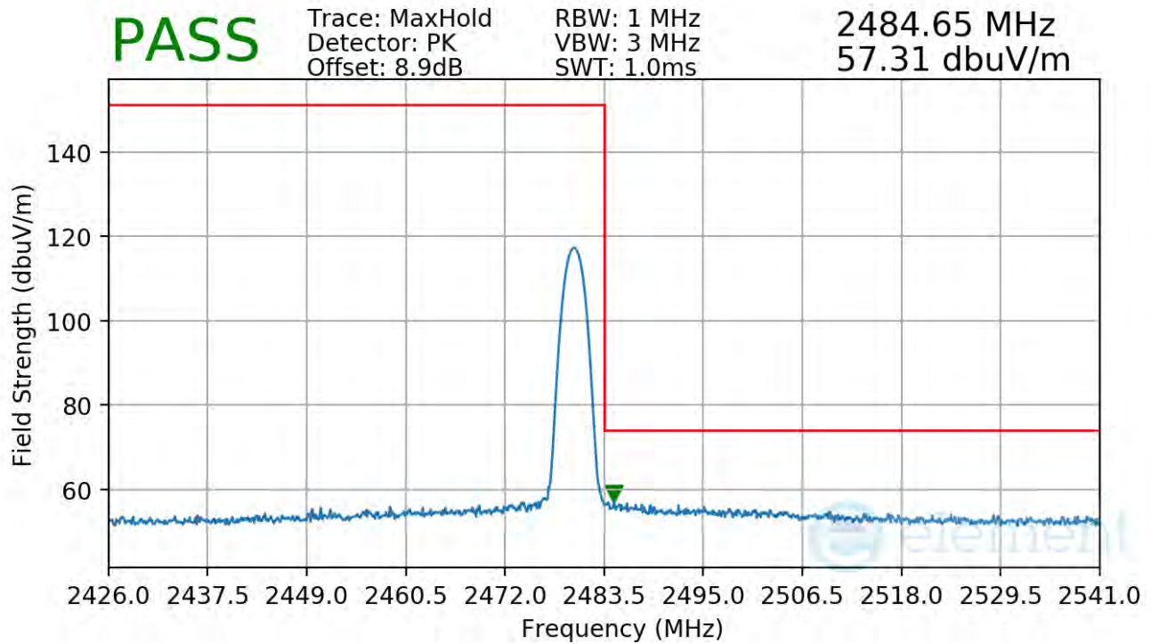
Plot 7-109. Radiated Restricted Upper Band Edge Measurement Antenna WF7
