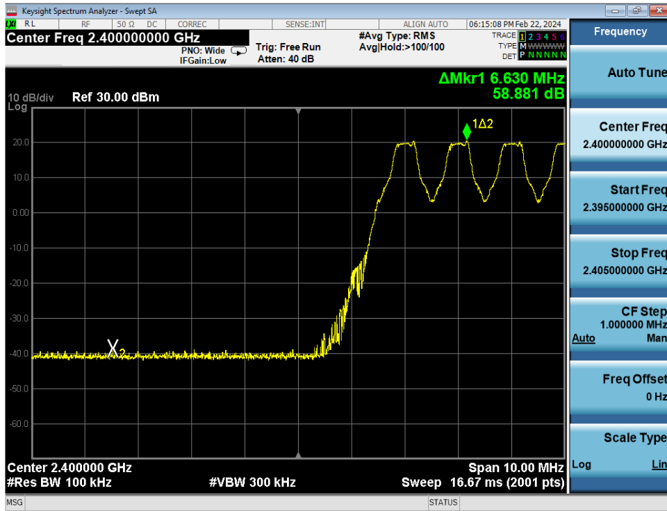
Plot 7-29. Band Edge Plot Antenna WF7 (Bluetooth with Hopping Enabled, GFSK, ePA)
