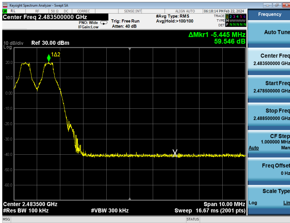
Plot 7-30. Band Edge Plot Antenna WF7 (Bluetooth with Hopping Enabled, GFSK, ePA)
