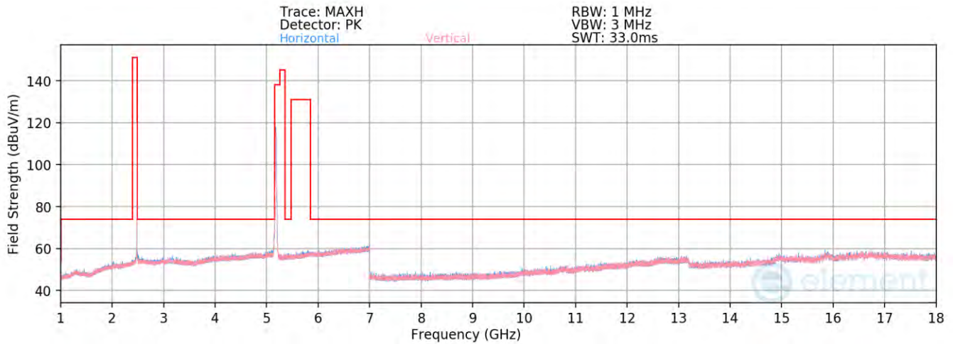
Plot 7-100. Radiated Spurious Emissions 1 – 18GHz – Simultaneous Transmission
