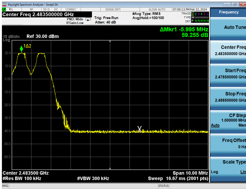
Plot 7-38. Band Edge Plot Antenna WF9 (Bluetooth with Hopping Enabled, GFSK, ePA)
