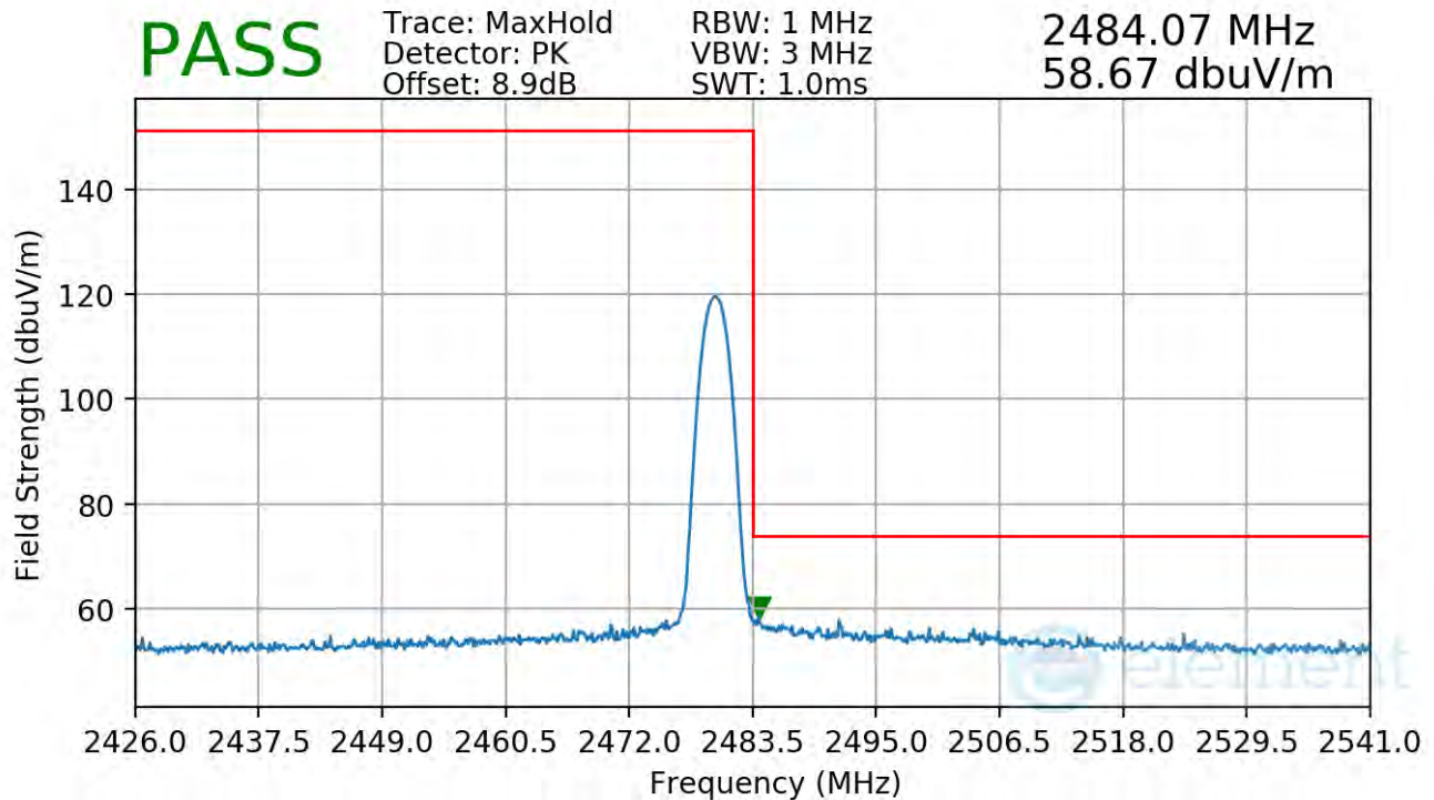
Plot 7-117. Radiated Restricted Upper Band Edge Measurement TxBF
