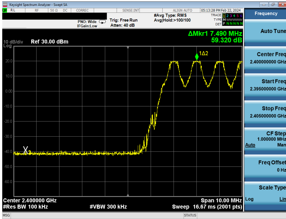
Plot 7-21. Band Edge Plot Antenna WF8 (Bluetooth with Hopping Enabled, GFSK, ePA)
