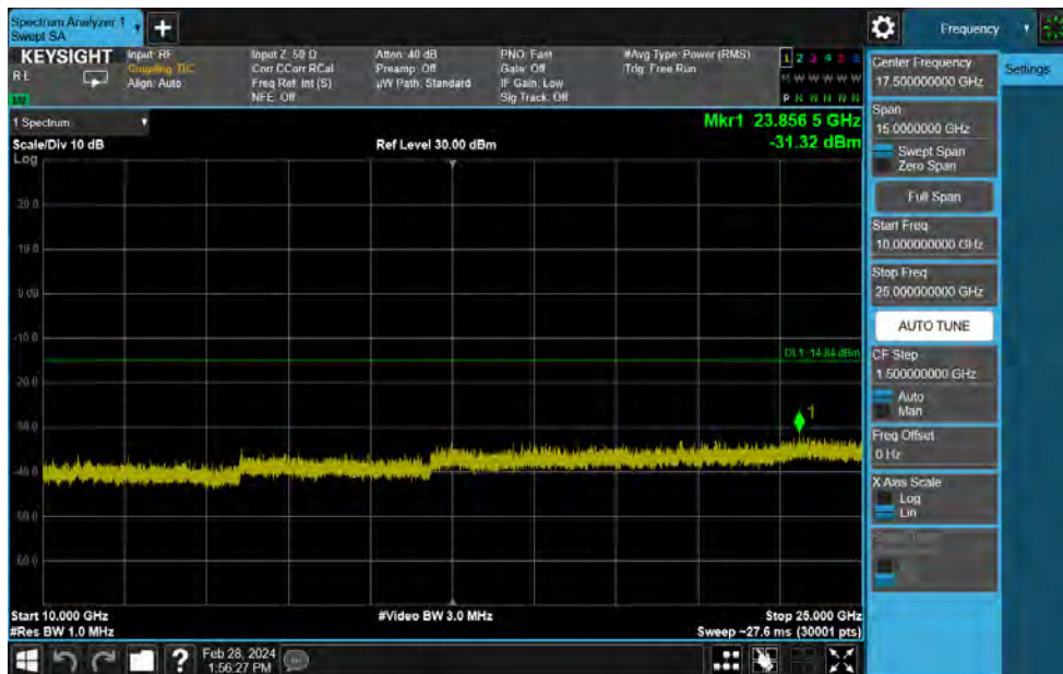
Plot 7-86. Conducted Simultaneous Tx Spurious Plot Antenna WF8 (Bluetooth + UNII)
