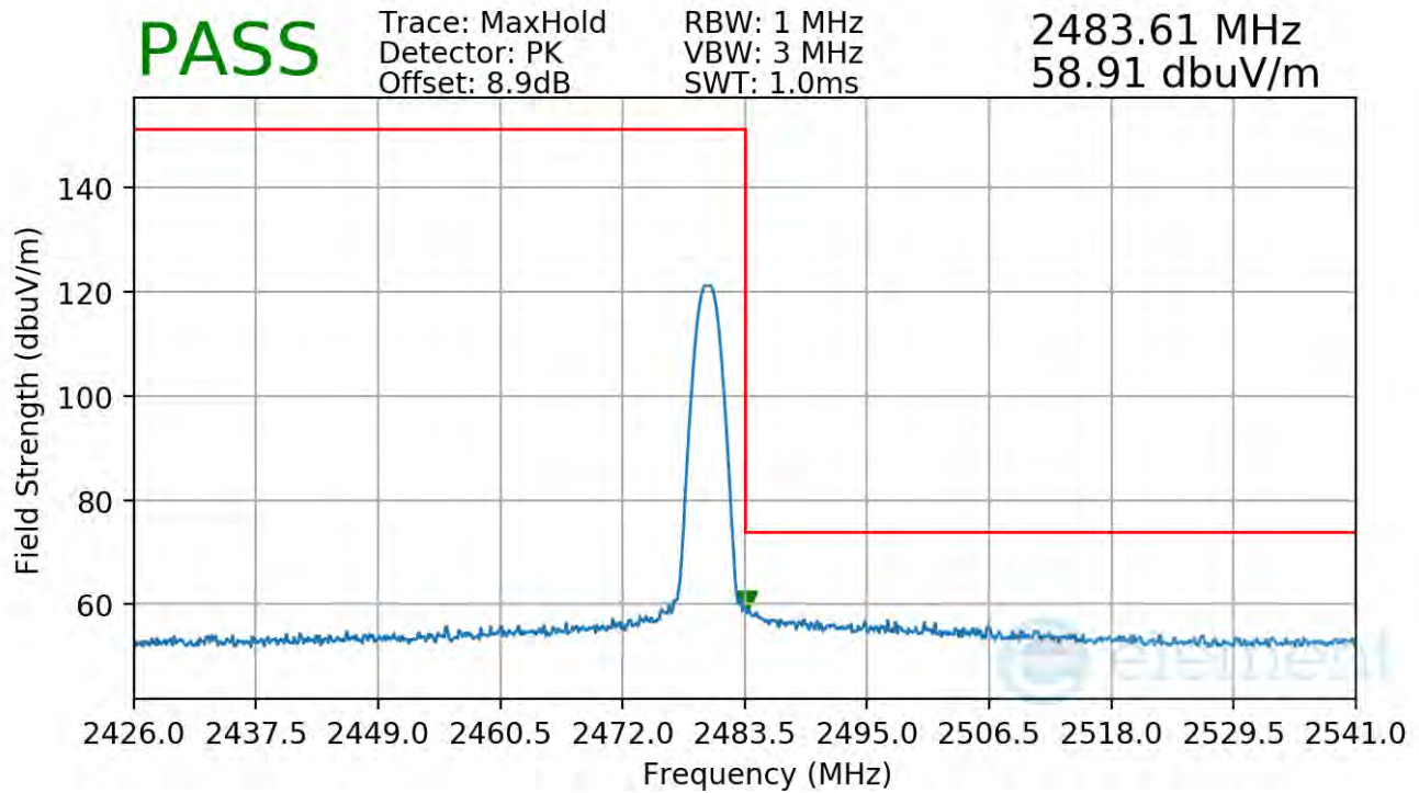
Plot 7-116. Radiated Restricted Upper Band Edge Measurement TxBF
