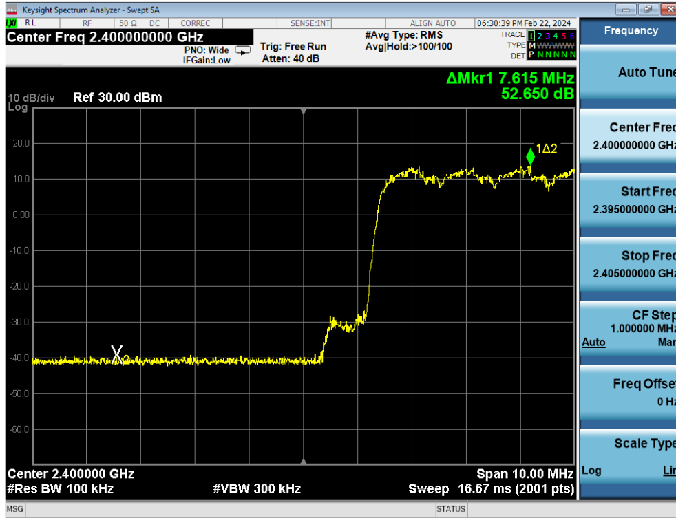
Plot 7-33. Band Edge Plot Antenna WF7 (Bluetooth with Hopping Enabled, 8DPSK, ePA)
