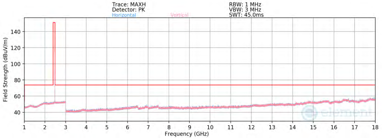
Plot 7-95. Radiated Spurious Emissions above 1GHz Antenna WF9 (BT GFSK ePA – Ch. 78)
