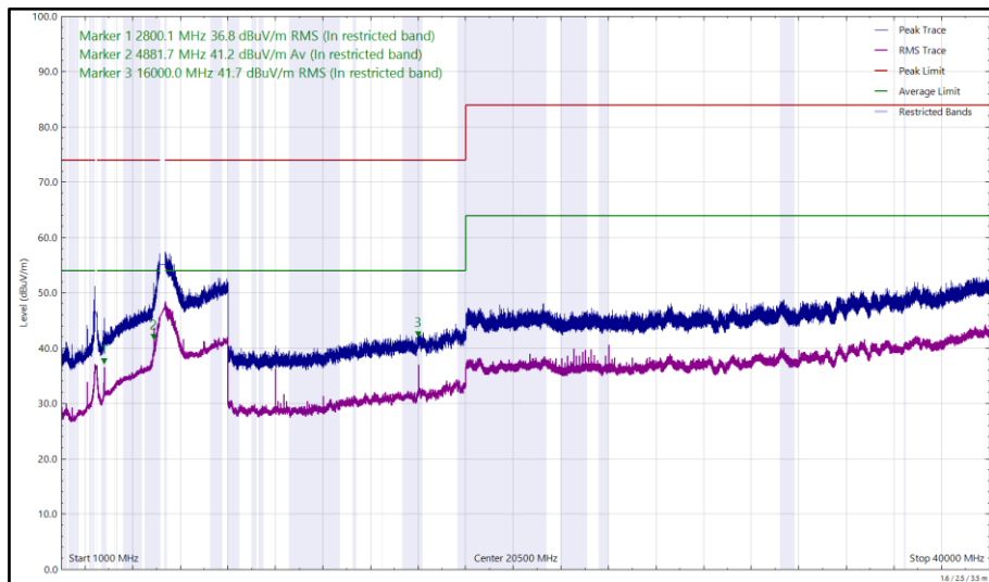
Figure 3 - U-NII-1 - 5240 MHz (CH48), VHT20, CDD, Core 0 + Core 1 and 2441 MHz (CH39), 2-DH5, ePA, Core 0 + Core 1, 1 GHz to 40 GHz, Horizontal
