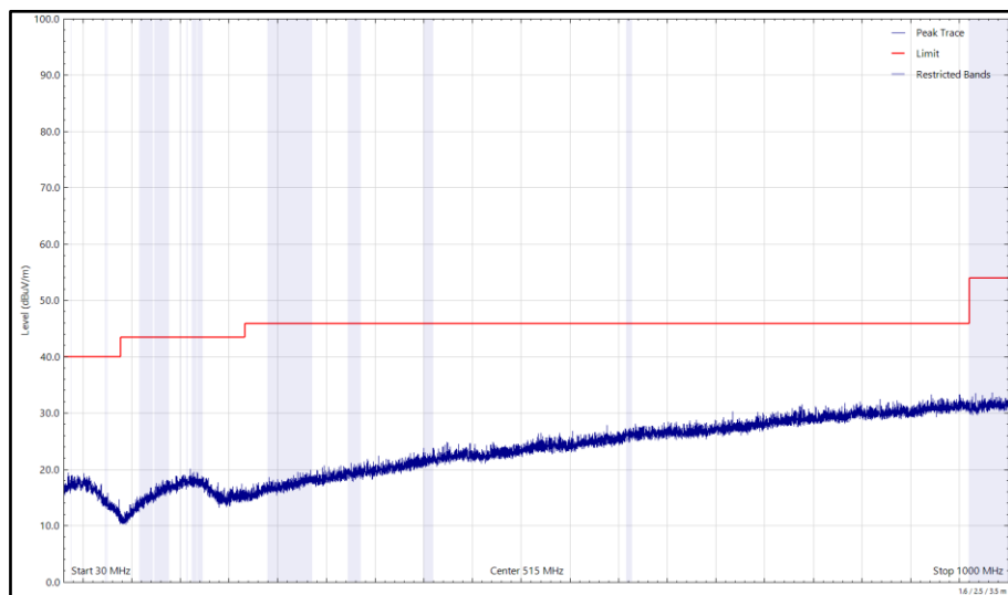
Figure 2 - U-NII-1 - 5240 MHz (CH48), VHT20, CDD, Core 0 + Core 1 and 2441 MHz (CH39), 2-DH5, ePA, Core 0 + Core 1, 30 MHz to 1 GHz, Horizontal (Peak)
