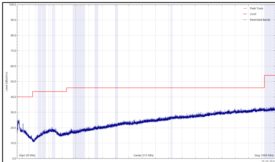
Figure 16 - U-NII-5 - 5955 MHz (CH1), HE20, SU, CDD, Core 0 + Core 1 and 2441 MHz (CH39), 2-DH5, ePA, Core 0 + Core 1, 30 MHz to 1 GHz, Vertical (Peak)
