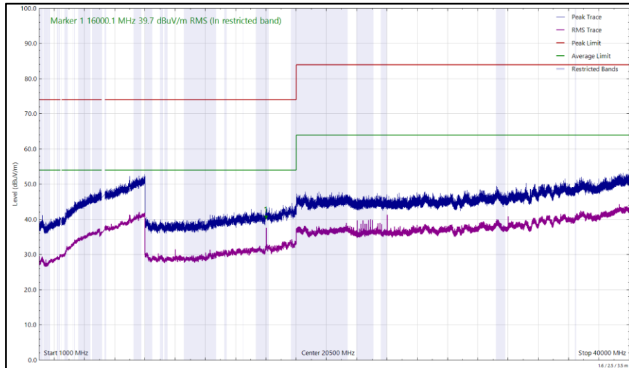
Figure 5 - U-NII-1 - 5240 MHz (CH48), VHT20, CDD, Core 0 + Core 1 and 2441 MHz (CH39), 2-DH5, ePA, Core 0 + Core 1, 1 GHz to 40 GHz, Vertical
