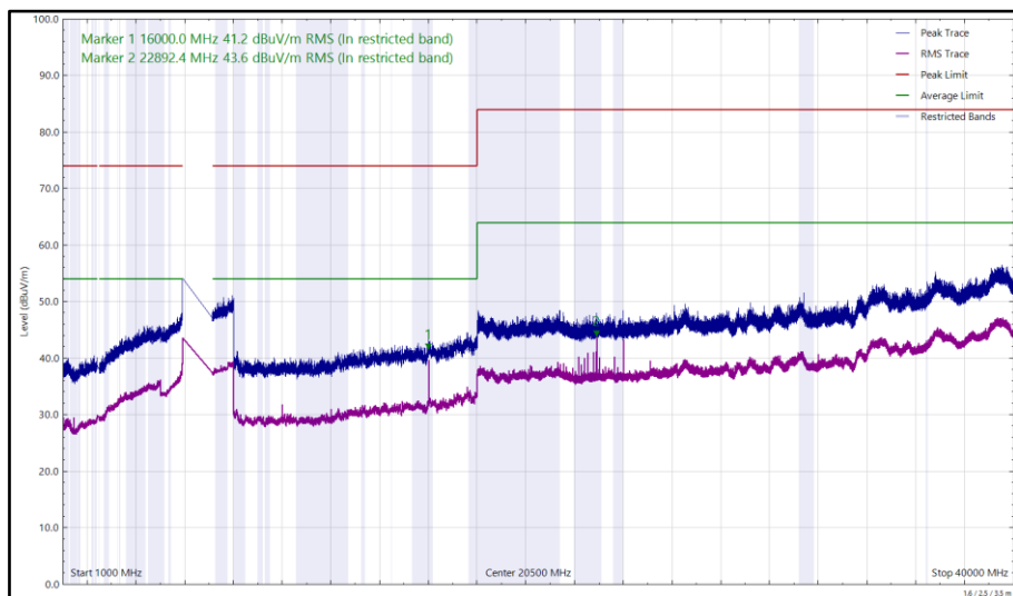
Figure 17 - U-NII-5 - 5955 MHz (CH1), HE20, SU, CDD, Core 0 + Core 1 and 2441 MHz (CH39), 2-DH5, ePA, Core 0 + Core 1, 1 GHz to 40 GHz, Vertical
