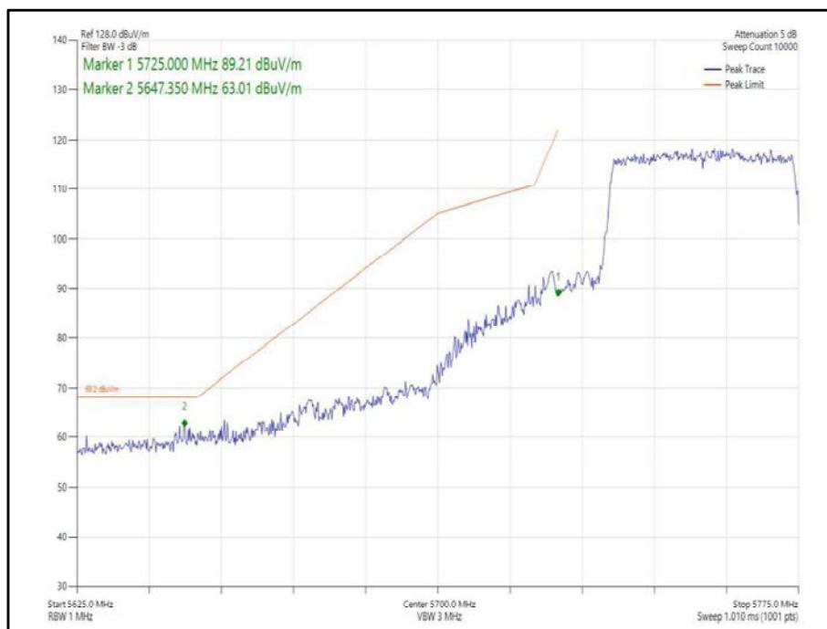
Figure 349 - 802.11ax, HE40, SU, SISO, Core 1 - 5755 MHz, Band Edge Frequency 5725 MHz
