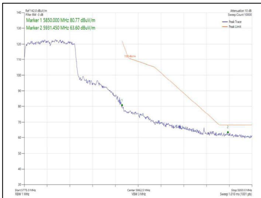
Figure 379 - 802.11ax, HE40, SU, SDM, Core 0-1 - 5795 MHz, Band Edge Frequency 5850 MHz
