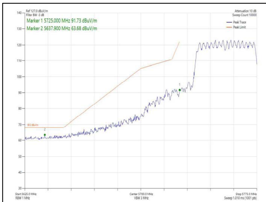
Figure 361 - 802.11ax, HE40, SU, CDD, Core 0-1 - 5755 MHz, Band Edge Frequency 5725 MHz
