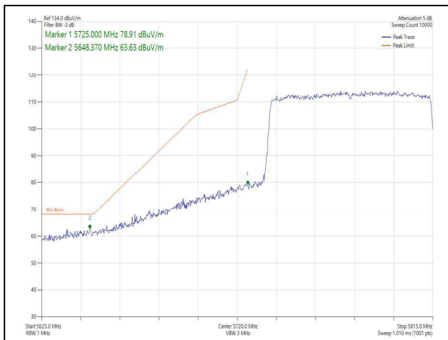
Figure 405 - 802.11ax, HE80, SU, SISO, Core 1 - 5775 MHz, Band Edge Frequency 5725 MHz
