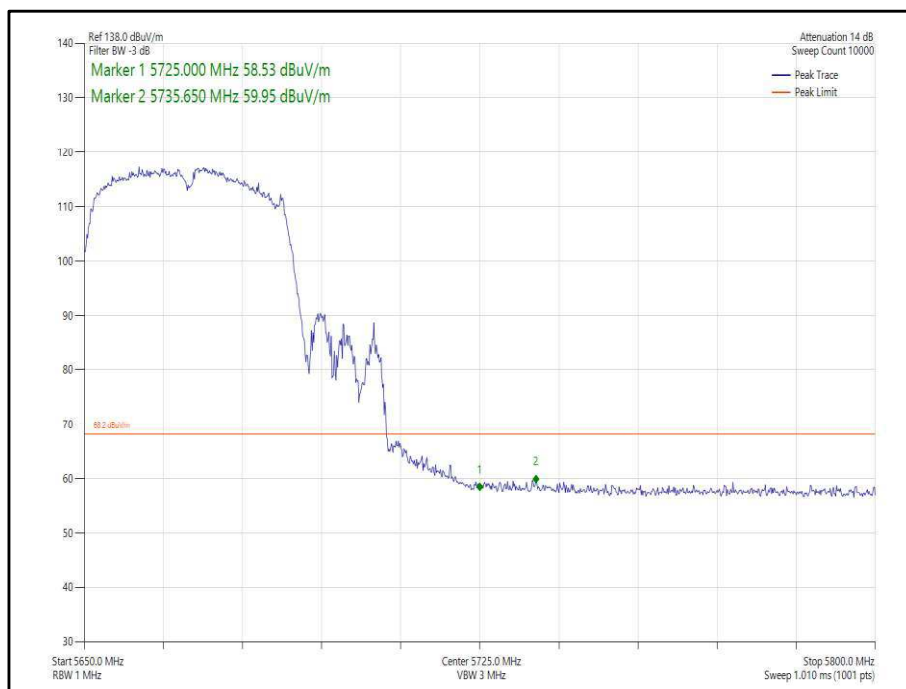
Figure 385 - 802.11n, HT40, TxBF, Core 0-1 - 5670 MHz, Band Edge Frequency 5725 MHz
