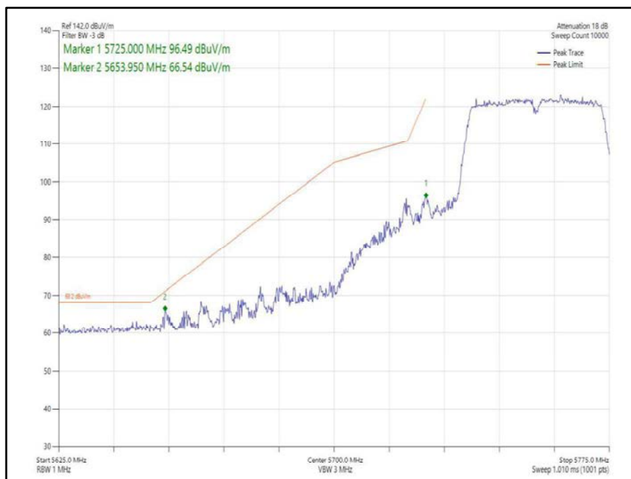
Figure 383 - 802.11ac, VHT40, TxBF, Core 0-1 - 5755 MHz, Band Edge Frequency 5725 MHz
