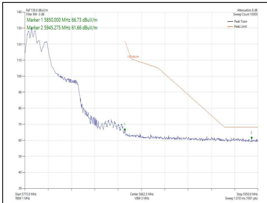
Figure 368 - 802.11ax, HE40, RU 106-53, CDD, Core 0-1 - 5795 MHz, Band Edge Frequency 5850 MHz
