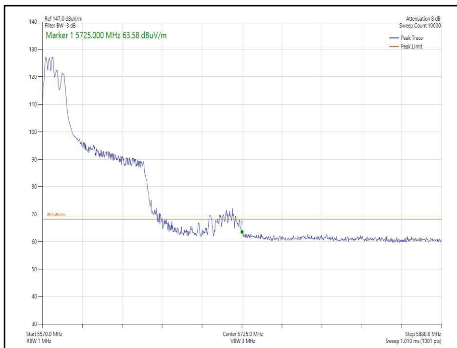
Figure 421 - 802.11ax, HE80, RU 106-53, CDD, Core 0-1 - 5610 MHz, Band Edge Frequency 5725 MHz
