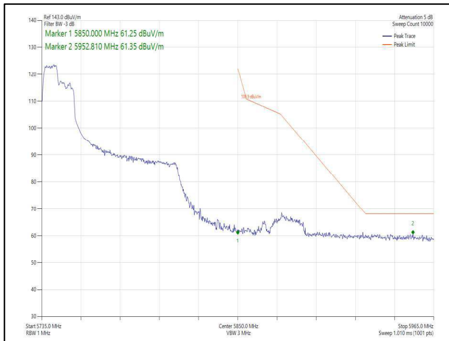
Figure 412 - 802.11ax, HE80, RU 106-53, SISO, Core 1 - 5775 MHz, Band Edge Frequency 5850 MHz
