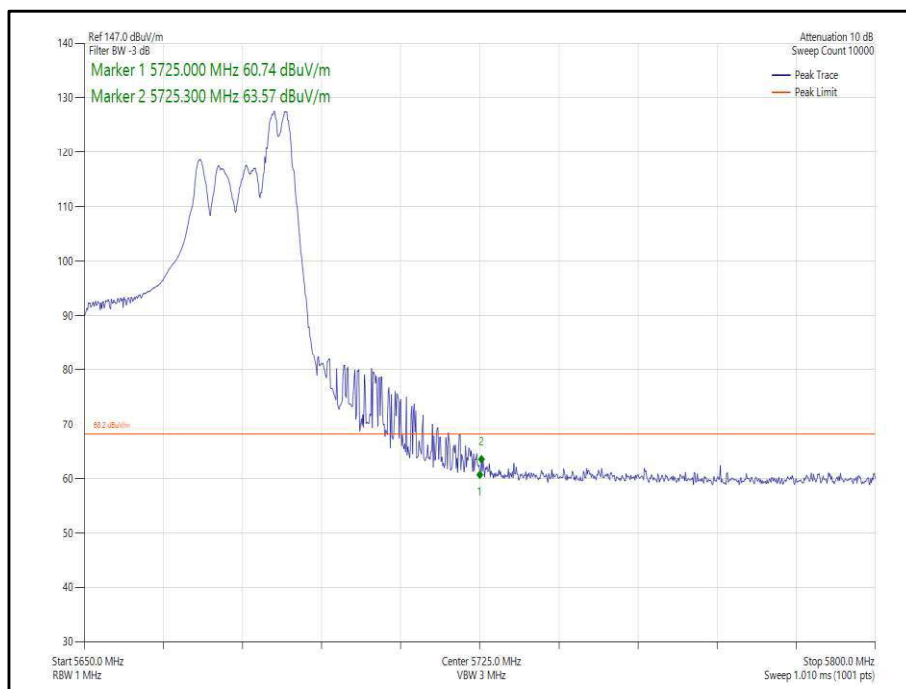
Figure 377 - 802.11ax, HE40, RU 52-44, SDM, Core 0-1 - 5670 MHz, Band Edge Frequency 5725 MHz
