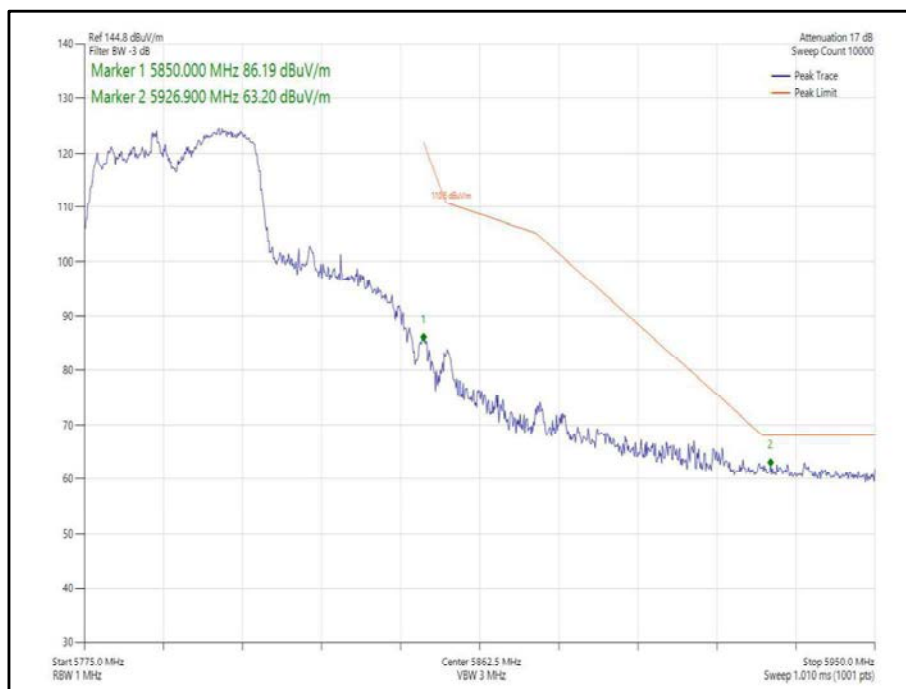
Figure 387 - 802.11n, HT40, TxBF, Core 0-1 - 5795 MHz, Band Edge Frequency 5850 MHz
