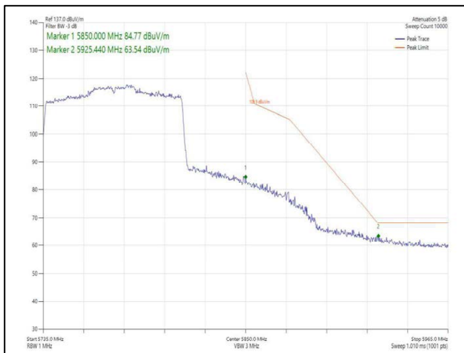
Figure 411 - 802.11ax, HE80, SU, SISO, Core 1 - 5775 MHz, Band Edge Frequency 5850 MHz
