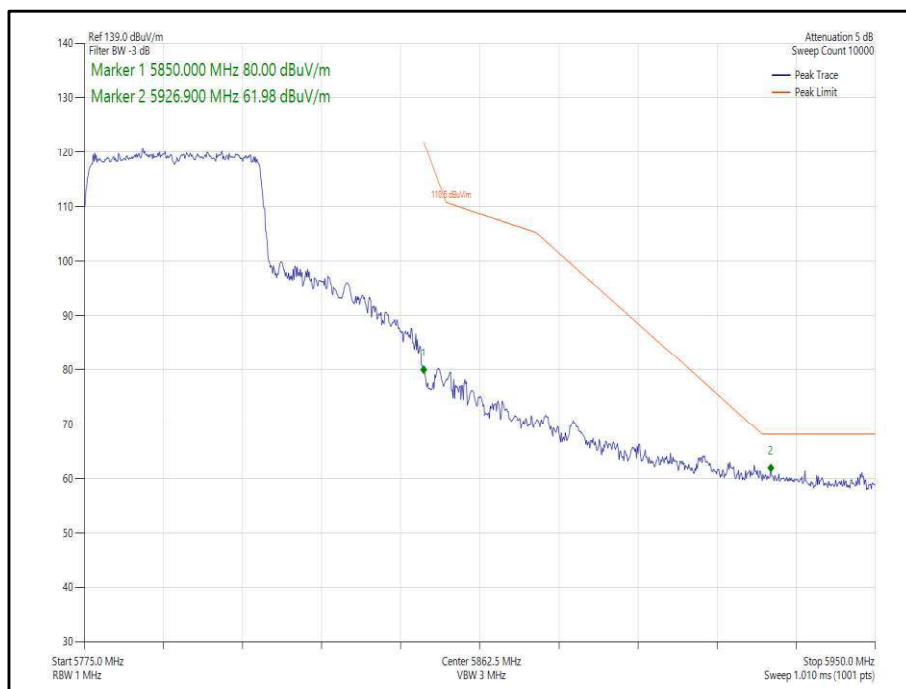
Figure 355 - 802.11ax, HE40, SU, SISO, Core 1 - 5795 MHz, Band Edge Frequency 5850 MHz
