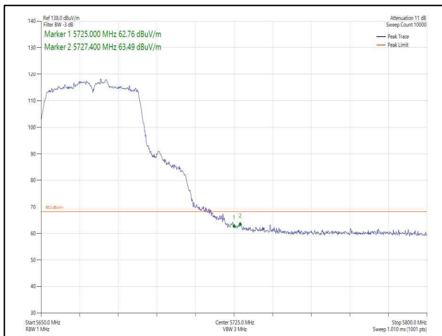
Figure 375 - 802.11n, HT40, SDM, Core 0-1 - 5670 MHz, Band Edge Frequency 5725 MHz
