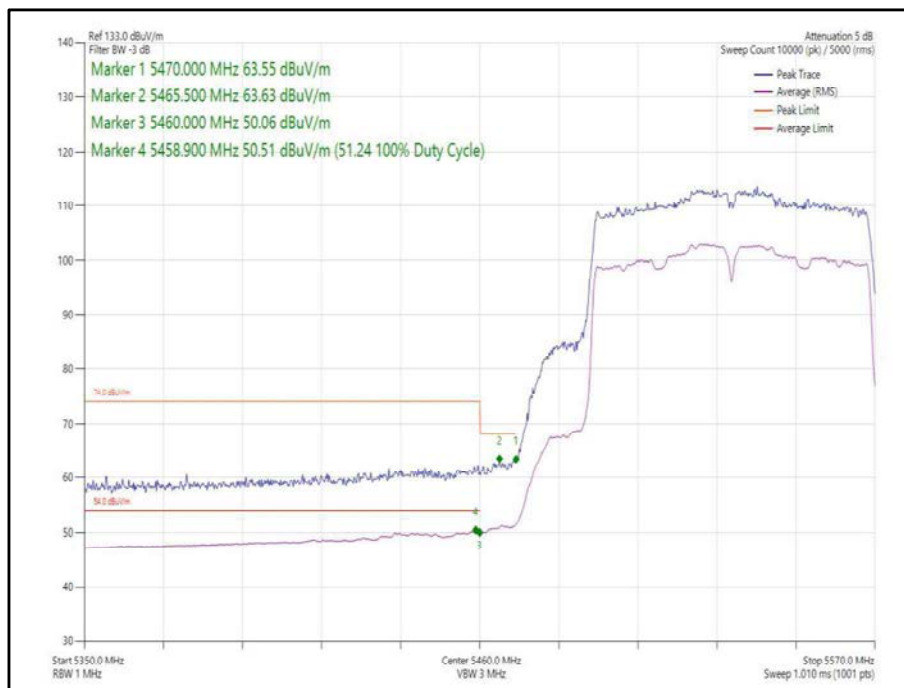
Figure 401 - 802.11ac, VHT80, SISO, Core 1 - 5530 MHz, Band Edge Frequency 5470 MHz
