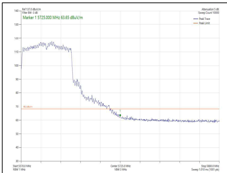
Figure 419 - 802.11ac, VHT80, CDD, Core 0-1 - 5610 MHz, Band Edge Frequency 5725 MHz
