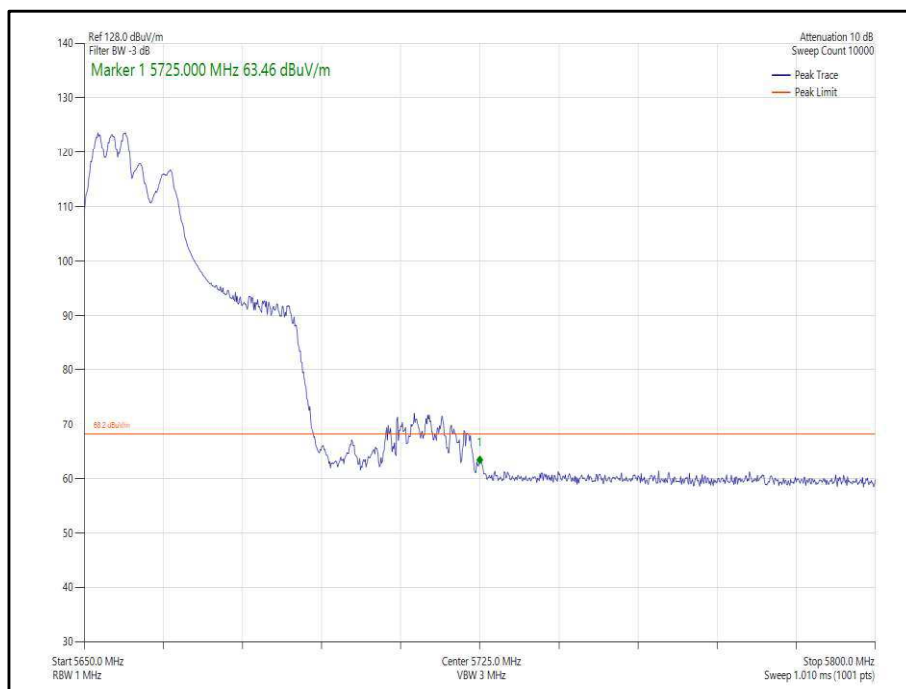
Figure 365 - 802.11ax, HE40, RU 106-53, CDD, Core 0-1 - 5670 MHz, Band Edge Frequency 5725 MHz
