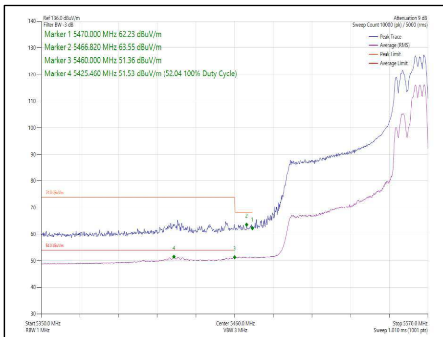
Figure 415 - 802.11ax, HE80, RU 106-60, CDD, Core 0-1 - 5530 MHz, Band Edge Frequency 5470 MHz
