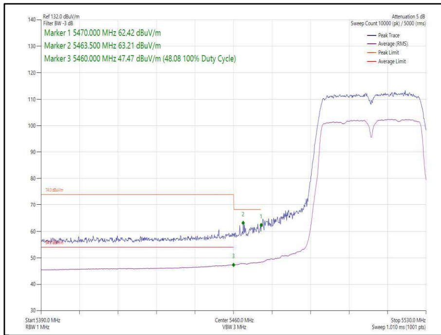
Figure 333 - 802.11n, HT40, SISO, Core 0 - 5510 MHz, Band Edge Frequency 5470 MHz
