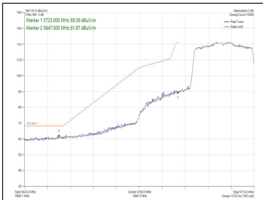
Figure 336 - 802.11n, HT40, SISO, Core 0 - 5755 MHz, Band Edge Frequency 5725 MHz
