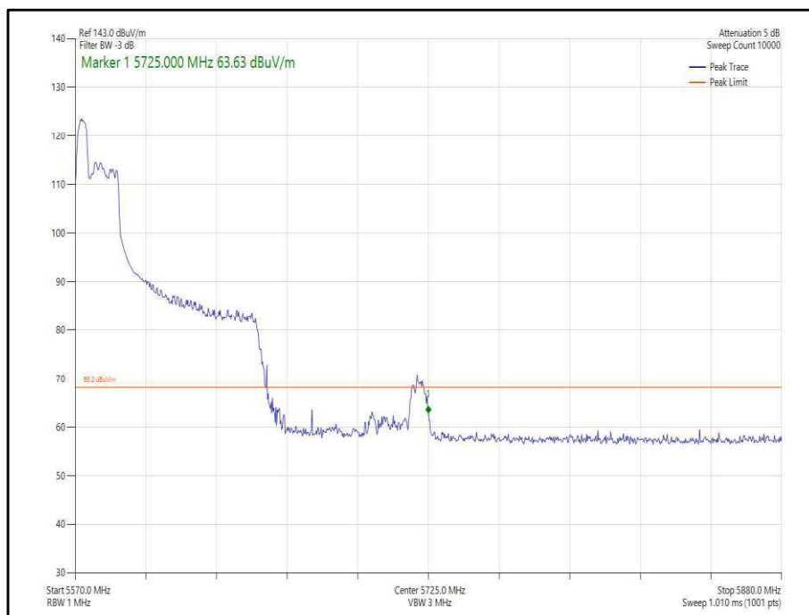
Figure 397 - 802.11ax, HE80, RU 52-37, SISO, Core 0 - 5610 MHz, Band Edge Frequency 5725 MHz
