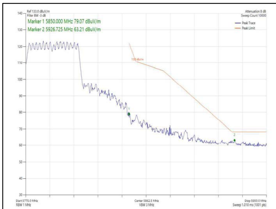
Figure 367 - 802.11ax, HE40, SU, CDD, Core 0-1 - 5795 MHz, Band Edge Frequency 5850 MHz
