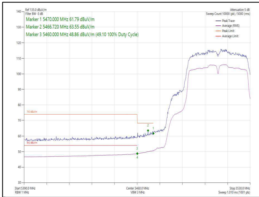
Figure 345 - 802.11n, HT40, SISO, Core 1 - 5510 MHz, Band Edge Frequency 5470 MHz
