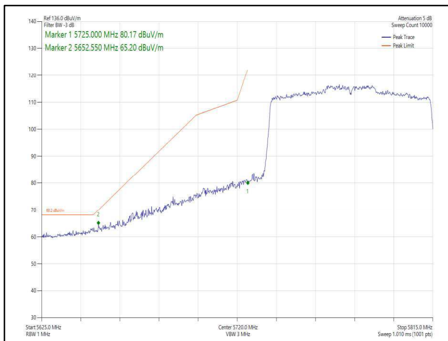
Figure 393 - 802.11ax, HE80, SU, SISO, Core 0 - 5775 MHz, Band Edge Frequency 5725 MHz
