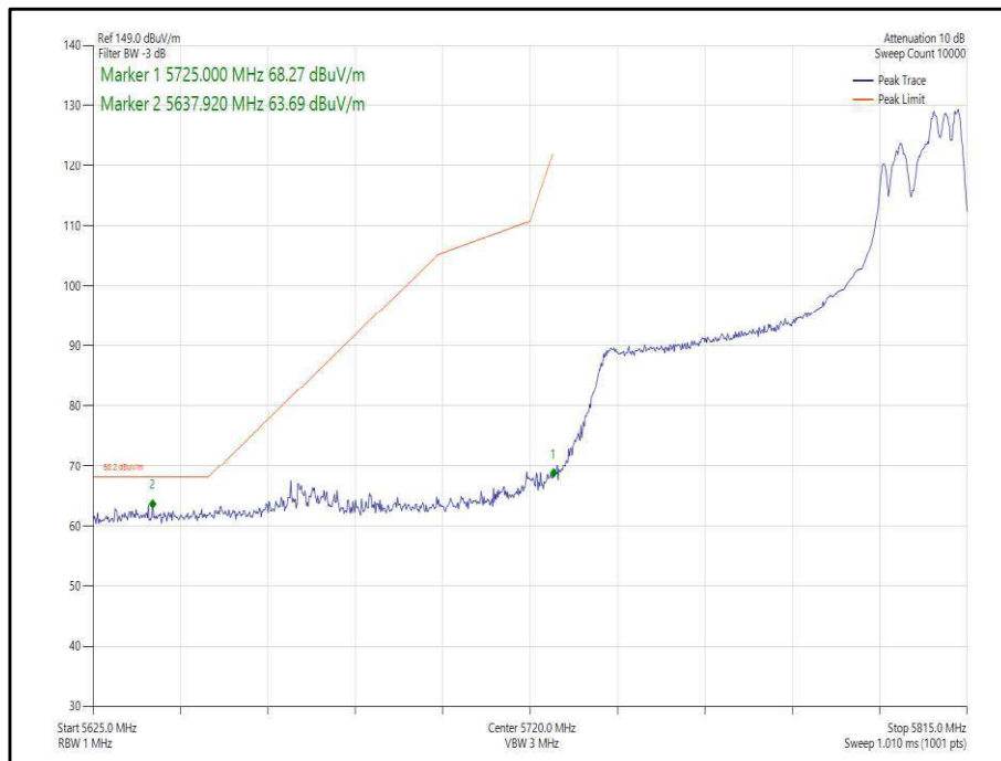
Figure 418 - 802.11ax, HE80, RU 106-60, CDD, Core 0-1 - 5775 MHz, Band Edge Frequency 5725 MHz
