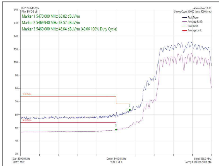
Figure 357 - 802.11n, HT40, CDD, Core 0-1 - 5510 MHz, Band Edge Frequency 5470 MHz
