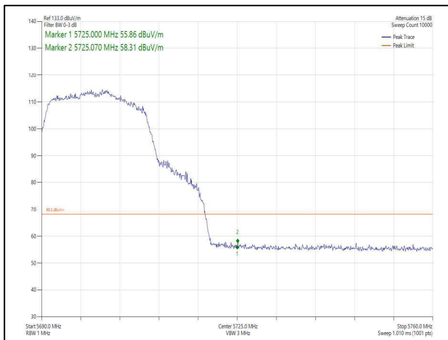
Figure 329 - 802.11ac, VHT20 TxBF, Core 0-1 - 5700 MHz, Band Edge Frequency 5725 MHz
