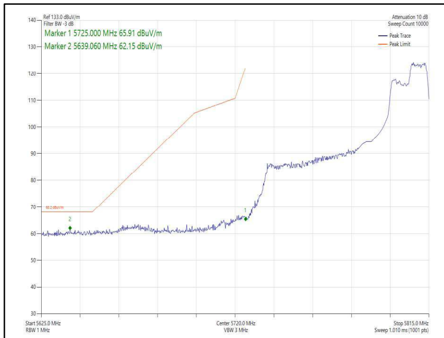
Figure 394 - 802.11ax, HE80, RU 106-60, SISO, Core 0 - 5775 MHz, Band Edge Frequency 5725 MHz
