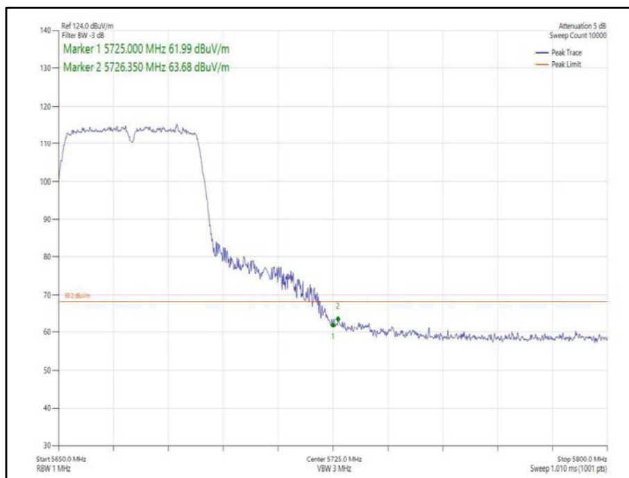
Figure 351 - 802.11n, HT40, SISO, Core 1 - 5670 MHz, Band Edge Frequency 5725 MHz
