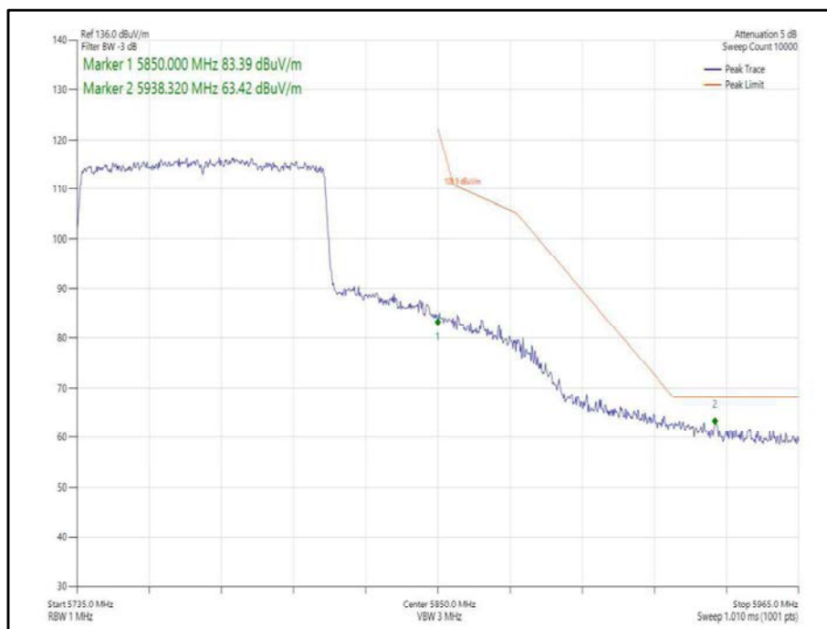
Figure 399 - 802.11ax, HE80, SU, SISO, Core 0 - 5775 MHz, Band Edge Frequency 5850 MHz
