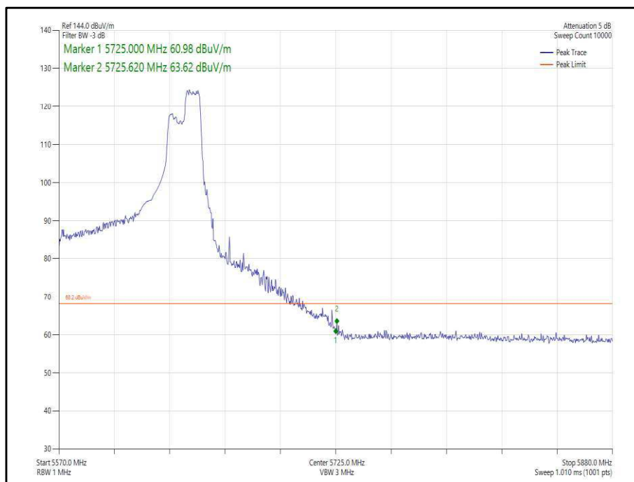
Figure 409 - 802.11ax, HE80, RU 106-60, SISO, Core 1 - 5610 MHz, Band Edge Frequency 5725 MHz
