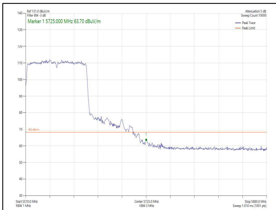
Figure 407 - 802.11ac, VHT80, SISO, Core 1 - 5610 MHz, Band Edge Frequency 5725 MHz
