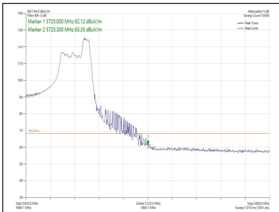
Figure 341 - 802.11ax, HE40, RU 52-44, SISO, Core 0 - 5670 MHz, Band Edge Frequency 5725 MHz
