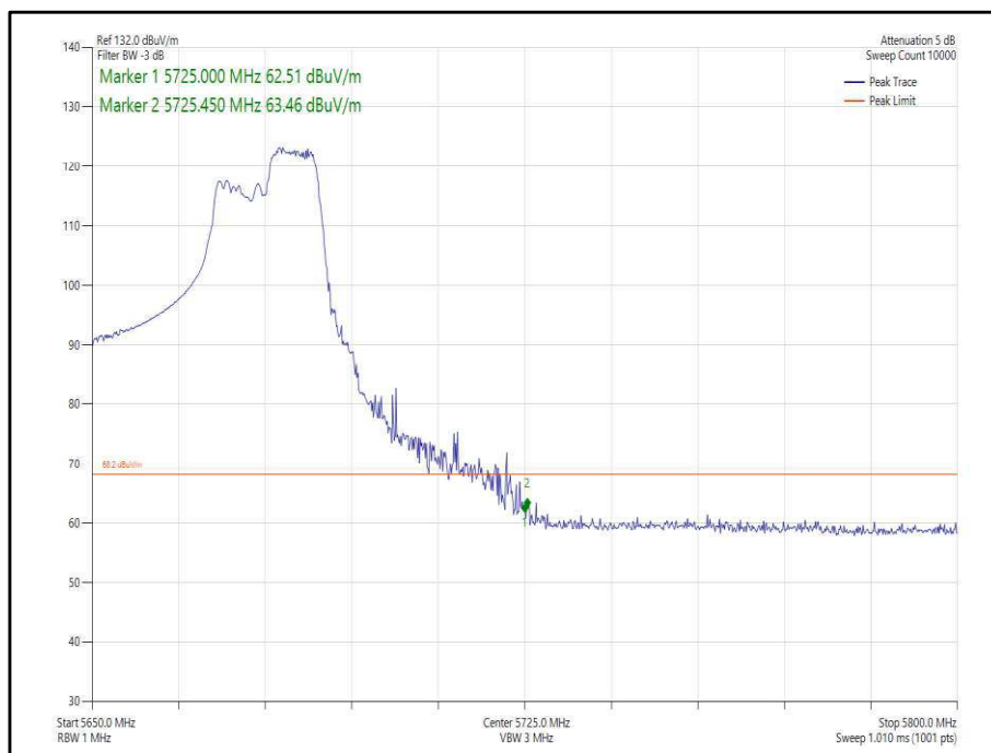
Figure 353 - 802.11ax, HE40, RU 106-56, SISO, Core 1 - 5670 MHz, Band Edge Frequency 5725 MHz
