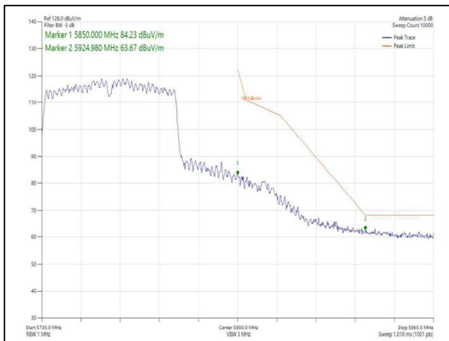
Figure 423 - 802.11ac, VHT80, CDD, Core 0-1 - 5775 MHz, Band Edge Frequency 5850 MHz
