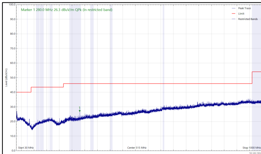
Figure 22 - U-NII-8 - 7115 MHz (CH233), HE20, SU, CDD, Core 0 + Core 1 and 2402 MHz (CH0), 2-DH5, ePA, Core 0 + Core 1, 30 MHz to 1 GHz, Horizontal (Peak)
