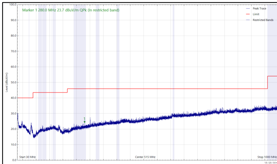
Figure 52 - 2412 MHz (CH1), HT20, Core 1 and 5162 MHz, HDR4, ePA, Core 0, 30 MHz to 1 GHz, Vertical (Peak)
