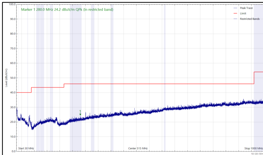
Figure 32 - U-NII-8 - 7115 MHz (CH233), HE20, SU, CDD, Core 0 + Core 1 and 2480 MHz (CH78), 2-DH5, ePA, Core 0 + Core 1, 30 MHz to 1 GHz, Vertical (Peak)
