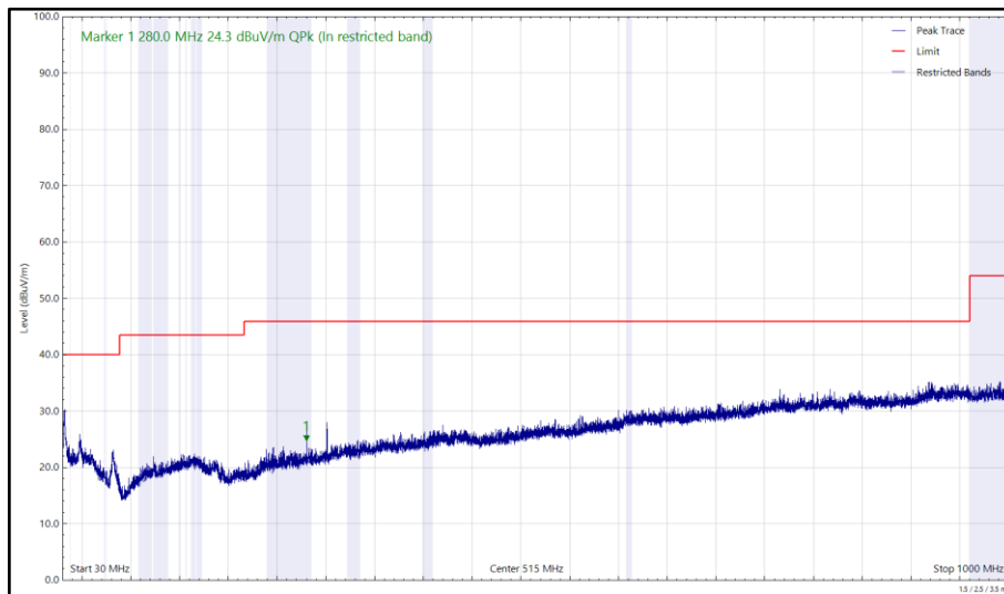
Figure 36 - 2412 MHz (CH1), HT20, Core 0 and 5162 MHz, HDR4, ePA, Core 1, 30 MHz to 1 GHz, Vertical (Peak)
