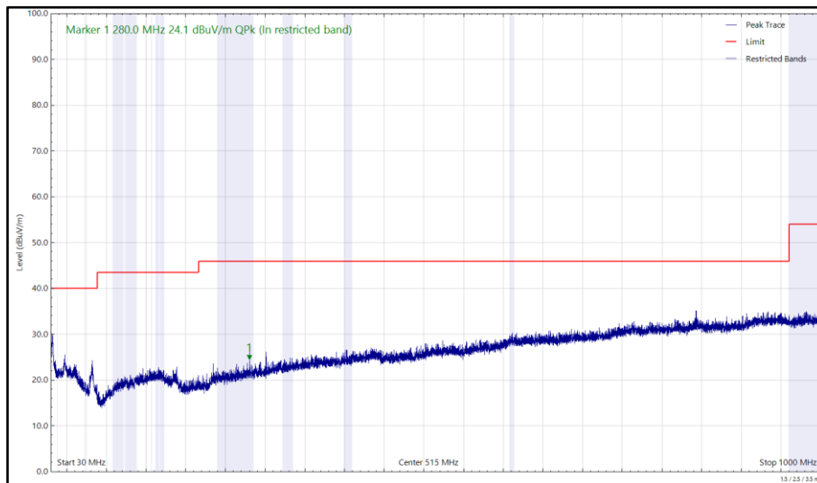
Figure 40 - 2472 MHz (CH13), HT20, Core 0 and 5162 MHz, HDR4, ePA, Core 1, 30 MHz to 1 GHz, Vertical (Peak)
