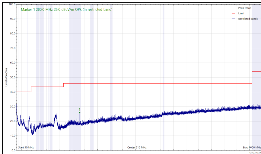
Figure 12 - U-NII-1 - 5200 MHz (CH40), VHT20, CDD, Core 0 + Core 1 and 2480 MHz (CH78), 2DH5, ePA, Core 0 + Core 1, 30 MHz to 1 GHz, Vertical (Peak)
