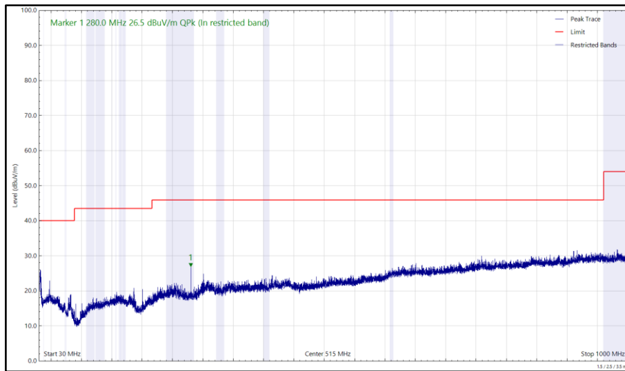
Figure 14 - U-NII-2C - 5680 MHz (CH136), VHT20, CDD, Core 0 + Core 1 and 2402 MHz (CH0), 2DH5, ePA, Core 0 + Core 1, 30 MHz to 1 GHz, Horizontal (Peak)
