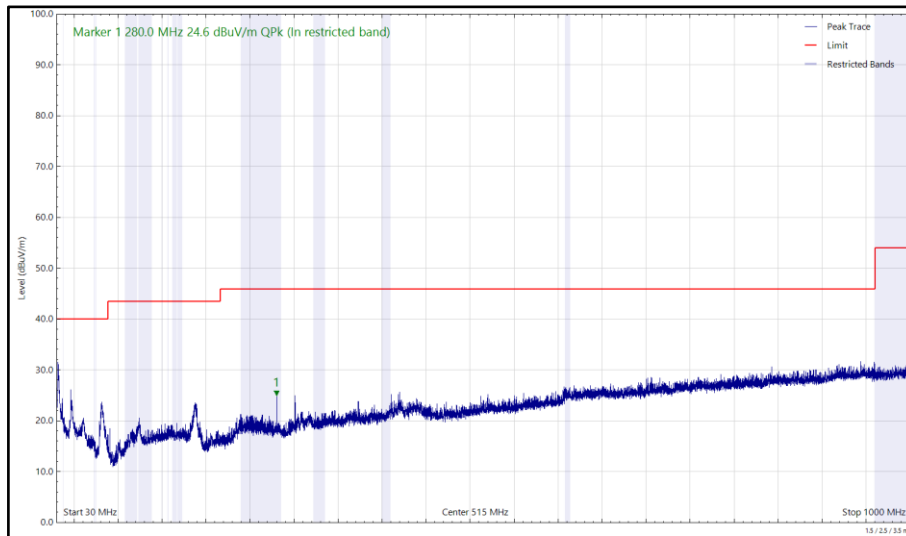
Figure 4 - U-NII-1 - 5200 MHz (CH40), VHT20, CDD, Core 0 + Core 1 and 2402 MHz (CH0), 2DH5, ePA, Core 0 + Core 1, 30 MHz to 1 GHz, Vertical (Peak)
