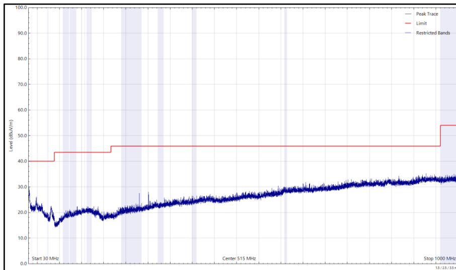
Figure 64 - 2472 MHz (CH13), HT20, Core 1 and 5844 MHz, HDR4, ePA, Core 0, 30 MHz to 1 GHz, Vertical (Peak)
