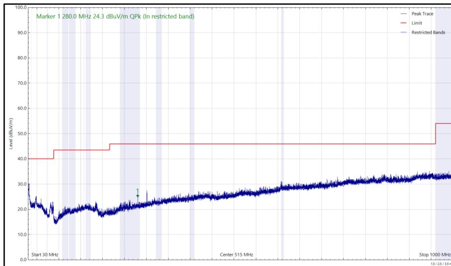
Figure 44 - 2412 MHz (CH1), HT20, Core 0 and 5844 MHz, HDR4, ePA, Core 1, 30 MHz to 1 GHz, Vertical (Peak)
