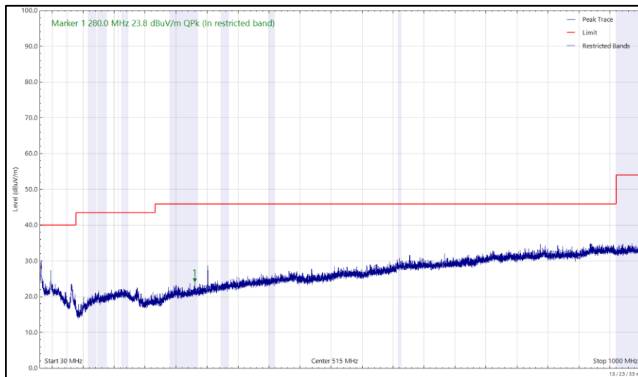
Figure 56 - 2472 MHz (CH13), HT20, Core 1 and 5162 MHz, HDR4, ePA, Core 0, 30 MHz to 1 GHz, Vertical (Peak)
