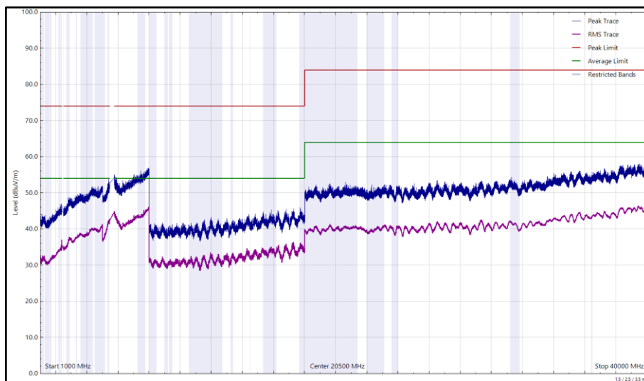
Figure 15 - U-NII-2C - 5680 MHz (CH136), VHT20, CDD, Core 0 + Core 1 and 2402 MHz (CH0), 2DH5, ePA, Core 0 + Core 1, 1 GHz to 40 GHz, Horizontal
