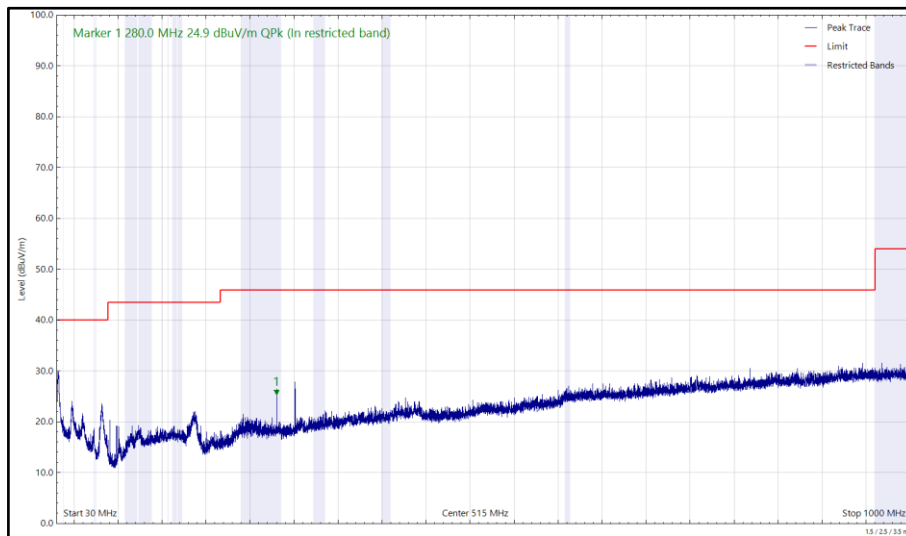
Figure 8 - U-NII-2C – 5680 MHz (CH136), VHT20, CDD, Core 0 + Core 1 and 2480 MHz (CH78), 2DH5, ePA, Core 0 + Core 1, 30 MHz to 1 GHz, Vertical (Peak)
