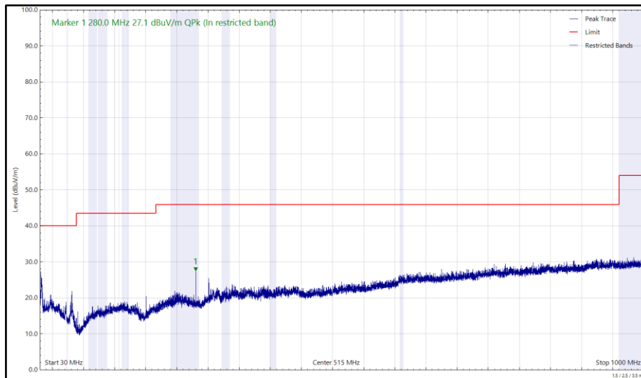
Figure 2 - U-NII-1 – 5200 MHz (CH40), VHT20, CDD, Core 0 + Core 1 and 2402 MHz (CH0), 2DH5, ePA, Core 0 + Core 1, 30 MHz to 1 GHz, Horizontal (Peak)
