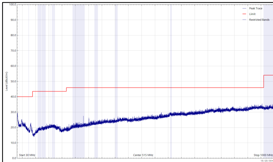
Figure 60 - 2412 MHz (CH1), HT20, Core 1 and 5844 MHz, HDR4, ePA, Core 0, 30 MHz to 1 GHz, Vertical (Peak)
