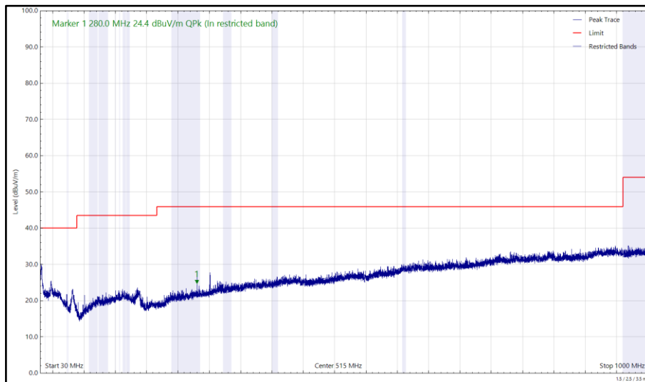
Figure 24 - U-NII-8 - 7115 MHz (CH233), HE20, SU, CDD, Core 0 + Core 1 and 2402 MHz (CH0), 2-DH5, ePA, Core 0 + Core 1, 30 MHz to 1 GHz, Vertical (Peak)
