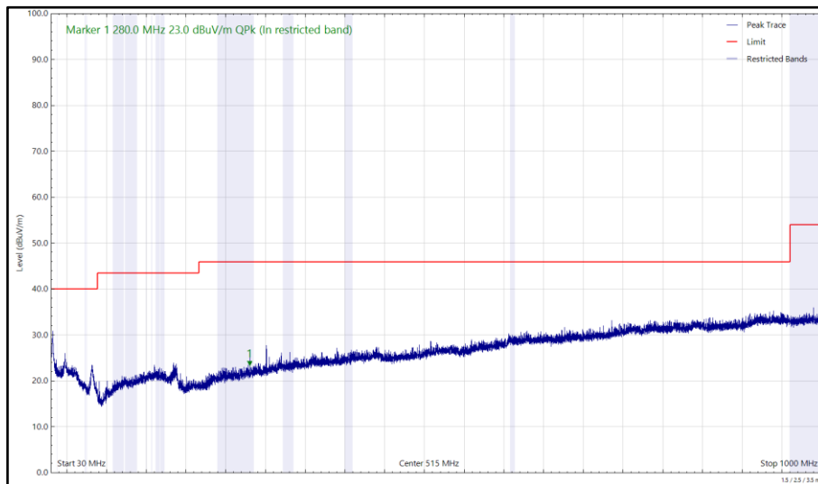
Figure 28 - U-NII-5 - 5955 MHz (CH1), HE20, SU, CDD, Core 0 + Core 1 and 2480 MHz (CH78), 2-DH5, ePA, Core 0 + Core 1, 30 MHz to 1 GHz, Vertical (Peak)
