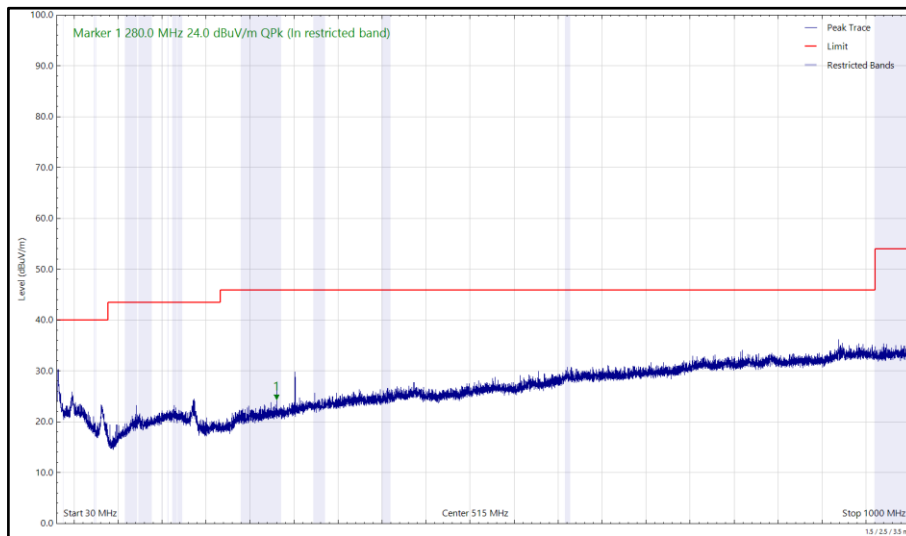
Figure 20 - U-NII-5 - 5955 MHz (CH1), HE20, SU, CDD, Core 0 + Core 1 and 2402 MHz (CH0), 2-DH5, ePA, Core 0 + Core 1, 30 MHz to 1 GHz, Vertical (Peak)
