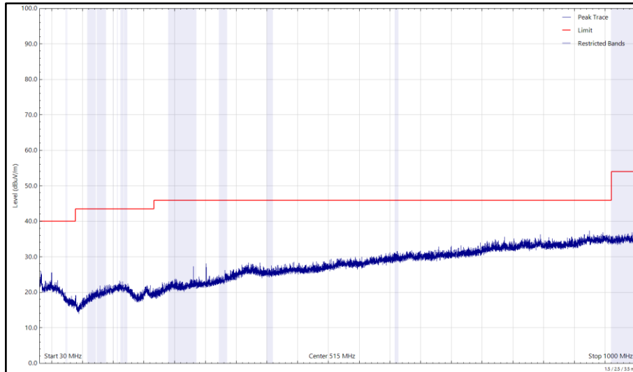
Figure 6 - U-NII-1 - 5200 MHz (CH40), VHT20, CDD, Core 0 + Core 1 and 2402 MHz (CH0), 2-DH5, ePA, Core 0 + Core 1, 30 MHz to 1 GHz, Horizontal (Peak)
