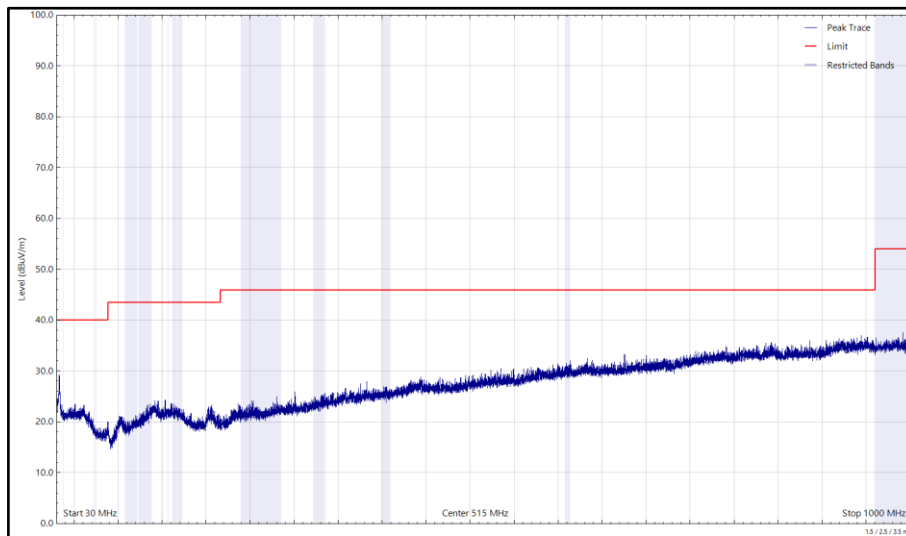
Figure 16 - U-NII-1 - 5200 MHz (CH40), VHT20, CDD, Core 0 + Core 1 and 2480 MHz (CH78), 2-DH5, ePA, Core 0 + Core 1, 30 MHz to 1 GHz, Vertical (Peak)
