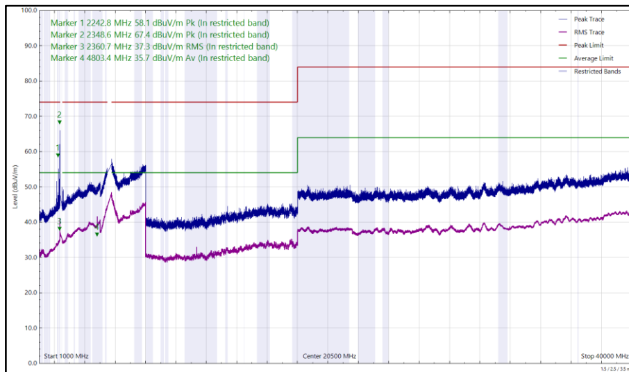
Figure 5 - U-NII-2C - 5680 MHz (CH136), VHT20, CDD, Core 0 + Core 1 and 2402 MHz (CH0), 2-DH5, ePA, Core 0 + Core 1, 1 GHz to 40 GHz, Vertical
