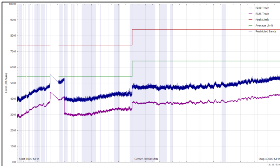
Figure 27 - U-NII-5 - 5955 MHz (CH1), HE20, SU, CDD, Core 0 + Core 1 and 2480 MHz (CH78), 2-DH5, ePA, Core 0 + Core 1, 1 GHz to 40 GHz, Horizontal
