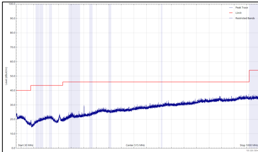
Figure 14 - U-NII-1 - 5200 MHz (CH40), VHT20, CDD, Core 0 + Core 1 and 2480 MHz (CH78), 2-DH5, ePA, Core 0 + Core 1, 30 MHz to 1 GHz, Horizontal (Peak)
