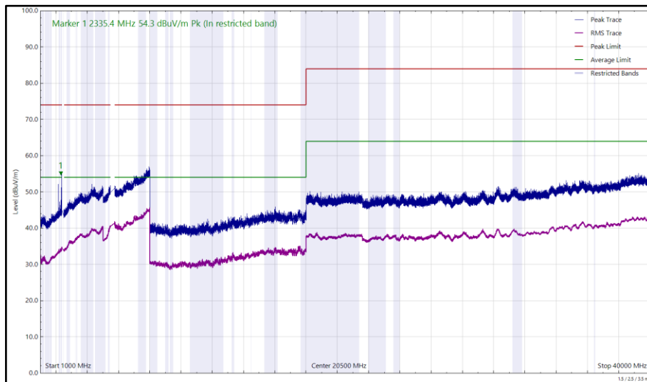
Figure 3 - U-NII-2C - 5680 MHz (CH136), VHT20, CDD, Core 0 + Core 1 and 2402 MHz (CH0), 2-DH5, ePA, Core 0 + Core 1, 1 GHz to 40 GHz, Horizontal
