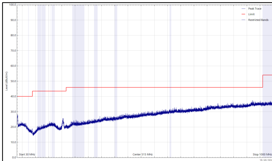
Figure 2 - U-NII-2C - 5680 MHz (CH136), VHT20, CDD, Core 0 + Core 1 and 2402 MHz (CH0), 2-DH5, ePA, Core 0 + Core 1, 30 MHz to 1 GHz, Horizontal (Peak)
