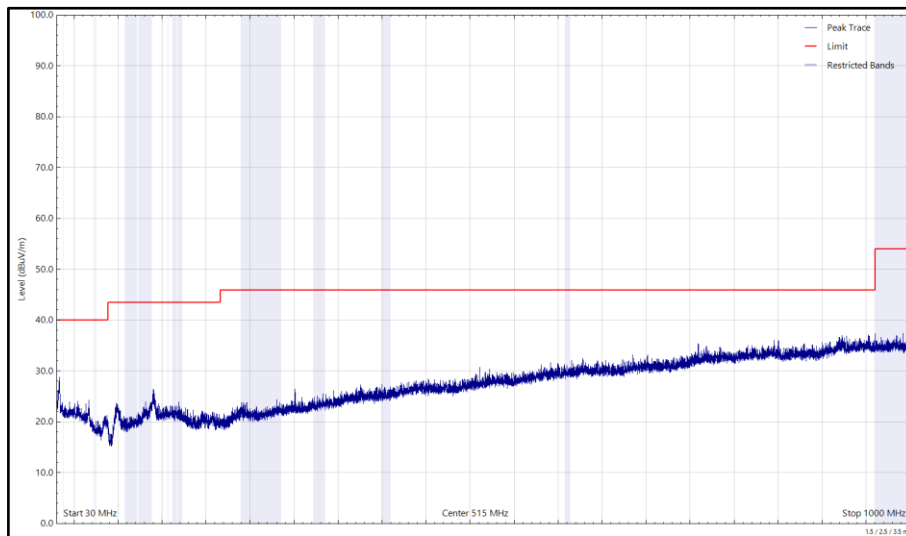
Figure 12 - U-NII-2C - 5680 MHz (CH136), VHT20, CDD, Core 0 + Core 1 and 2480 MHz (CH78), 2-DH5, ePA, Core 0 + Core 1, 30 MHz to 1 GHz, Vertical (Peak)
