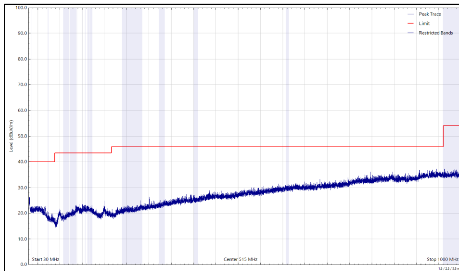
Figure 8 - U-NII-1 - 5200 MHz (CH40), VHT20, CDD, Core 0 + Core 1 and 2402 MHz (CH0), 2-DH5, ePA, Core 0 + Core 1, 30 MHz to 1 GHz, Vertical (Peak)
