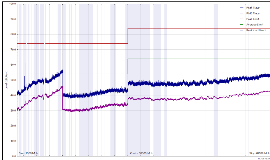
Figure 7 - U-NII-1 - 5200 MHz (CH40), VHT20, CDD, Core 0 + Core 1 and 2402 MHz (CH0), 2-DH5, ePA, Core 0 + Core 1, 1 GHz to 40 GHz, Horizontal
