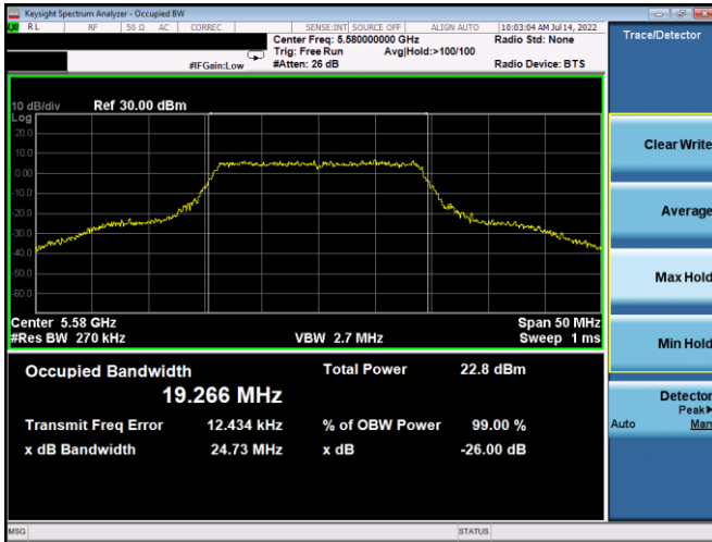
Plot 7-8. 26dB BW & 99% OBW (20MHz BW 802.11n – Ch. 116, MCS0)
