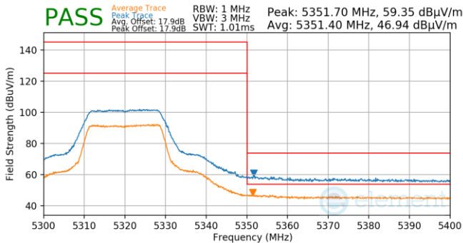
Plot 7-44. FCM (Pk & Avg, Ch.64, 802.11n, MCS7)
