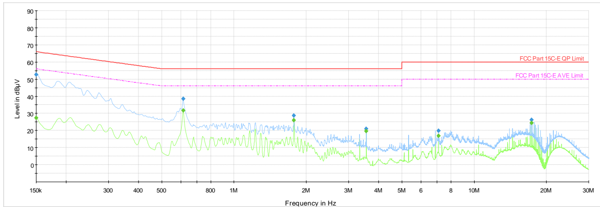
Plot 7-58. AC Line Conducted Plot with 802.11n– Ch.40 (L1), with Laptop & Magnetic Charger
