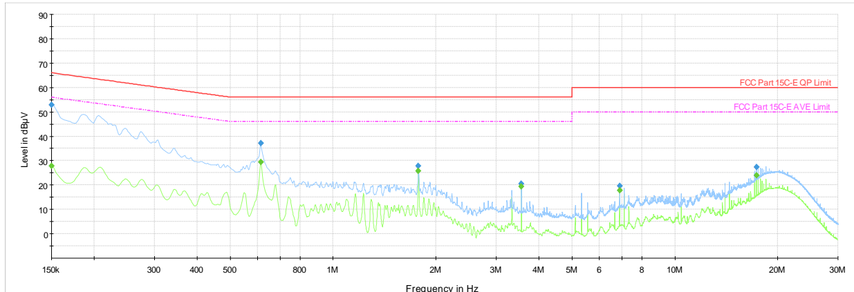
Plot 7-59. AC Line Conducted Plot with 802.11n– Ch.40 (N), with Laptop & Magnetic Charger
