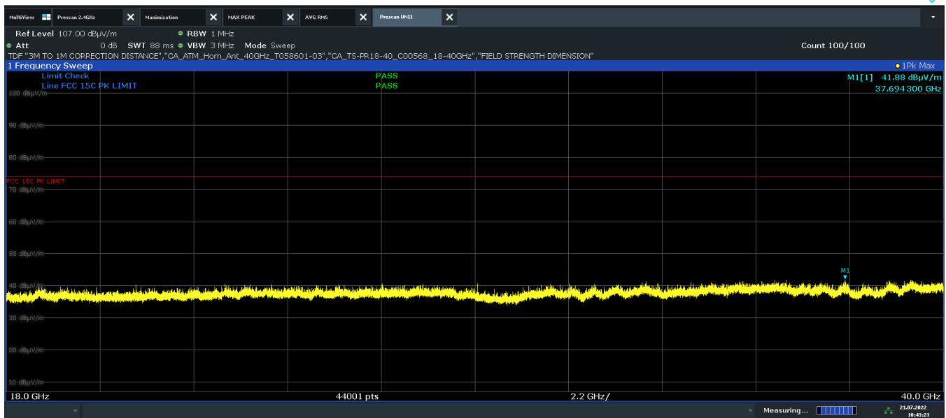
Plot 7-28. Radiated Spurious Emissions 18GHz-40GHz V Polarity (802.11n – Ch. 40)
