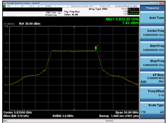
Plot 7-24. PSD (20MHz BW 802.11n – Ch. 165, MCS0)
