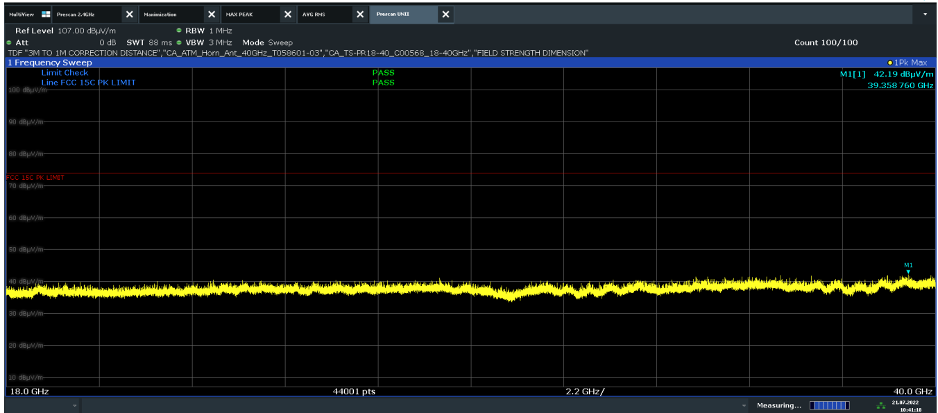
Plot 7-27. Radiated Spurious Emissions 18GHz-40GHz H Polarity (802.11n – Ch. 40)
