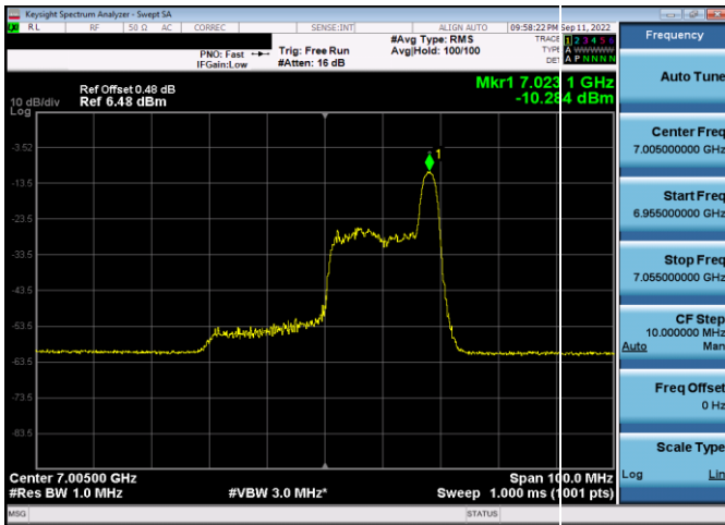
Plot 7-366. Power Spectral Density Plot SDM Antenna 4a (40MHz 802.11ax RU26 (UNII Band 8) – Ch. 211)
