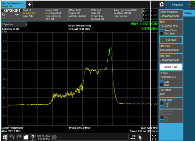
Plot 7-365. Power Spectral Density Plot SDM Antenna 5b (40MHz 802.11ax RU26 (UNII Band 8) – Ch. 211)
