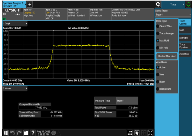
Plot 7-26. 26dB & 99% Bandwidth Plot Antenna 5b (80MHz 802.11ax RU996 (UNII Band 6) – Ch. 103)
