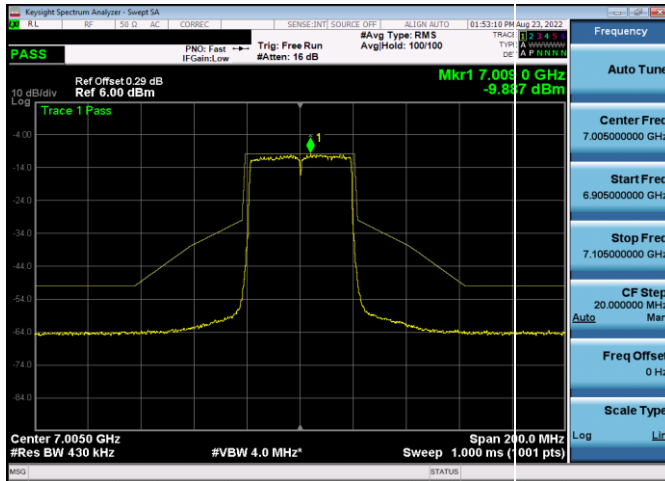
Plot 7-362. In-Band Emission Plot Antenna 5b (40MHz 802.11ax (UNII Band 8) – Ch. 211, MCS2)
