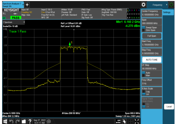
Plot 7-369. In-Band Emission Plot Antenna 5b (160MHz 802.11ax (UNII Band 5) – Ch. 47, MCS4)
