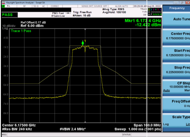
Plot 7-365. In-Band Emission Plot Antenna 5b (20MHz 802.11a (UNII Band 5) – Ch. 45, MCS4)
