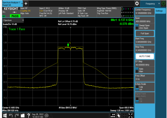
Plot 7-368. In-Band Emission Plot Antenna 5b (80MHz 802.11ax (UNII Band 5) – Ch. 39, MCS4)
