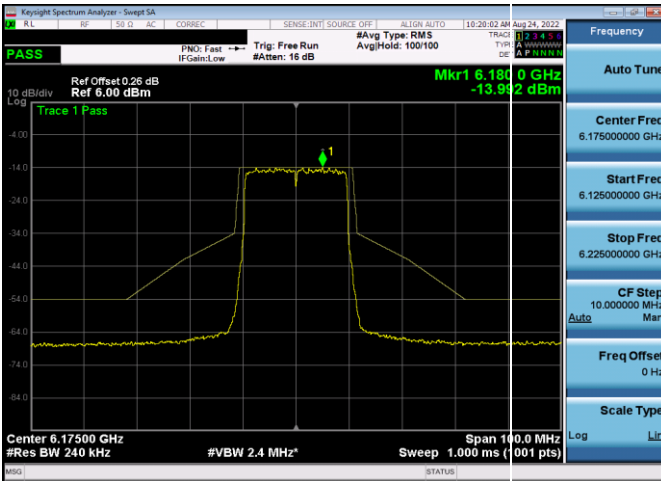
Plot 7-366. In-Band Emission Plot Antenna 5b (20MHz 802.11ax (UNII Band 5) – Ch. 45, MCS4)
