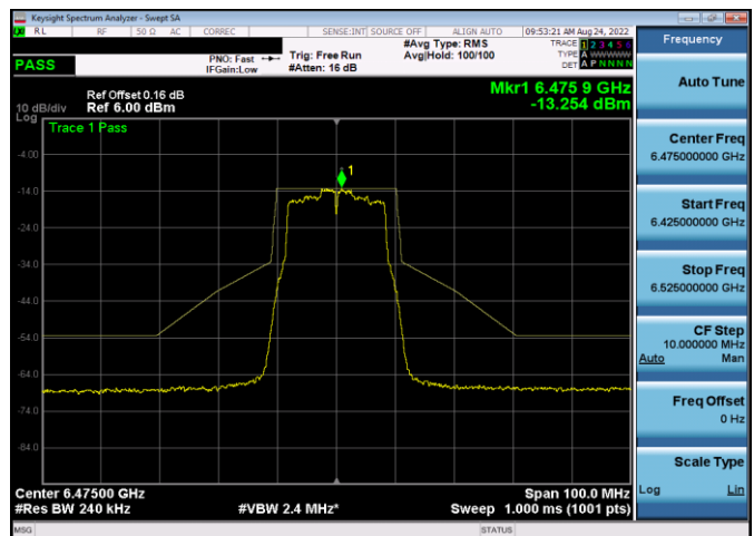
Plot 7-370. In-Band Emission Plot Antenna 5b (20MHz 802.11a (UNII Band 6) – Ch. 105, MCS4)
