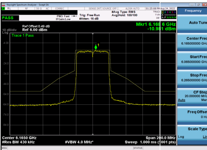
Plot 7-367. In-Band Emission Plot Antenna 5b (40MHz 802.11ax (UNII Band 5) – Ch. 43, MCS4)
