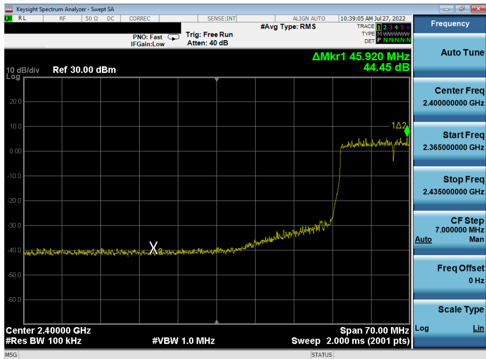
Plot 7-414. Band Edge Plot Antenna 2a (802.11ax (SU - 2.4GHz) – Ch. 5) – MCS5
