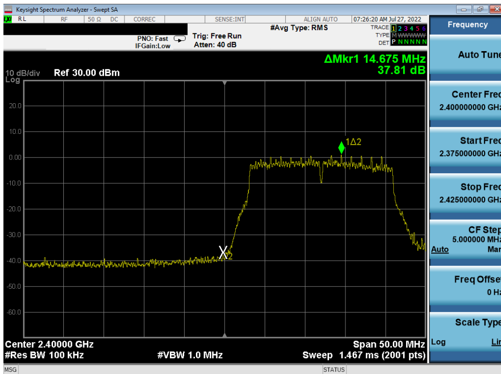
Plot 7-347. Band Edge Plot Antenna 2a (802.11n (2.4GHz) – Ch. 1) – MCS3
