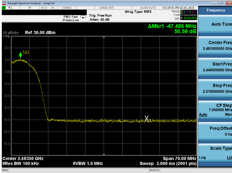
Plot 7-377. Band Edge Plot Antenna 2a (802.11b – Ch. 9) – 11Mbps
