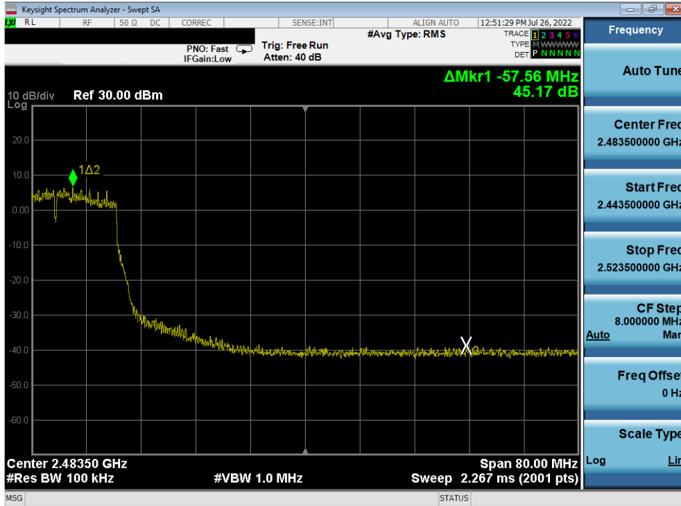
Plot 7-354. Band Edge Plot Antenna 2a (802.11n (2.4GHz) – Ch. 8) – MCS3
