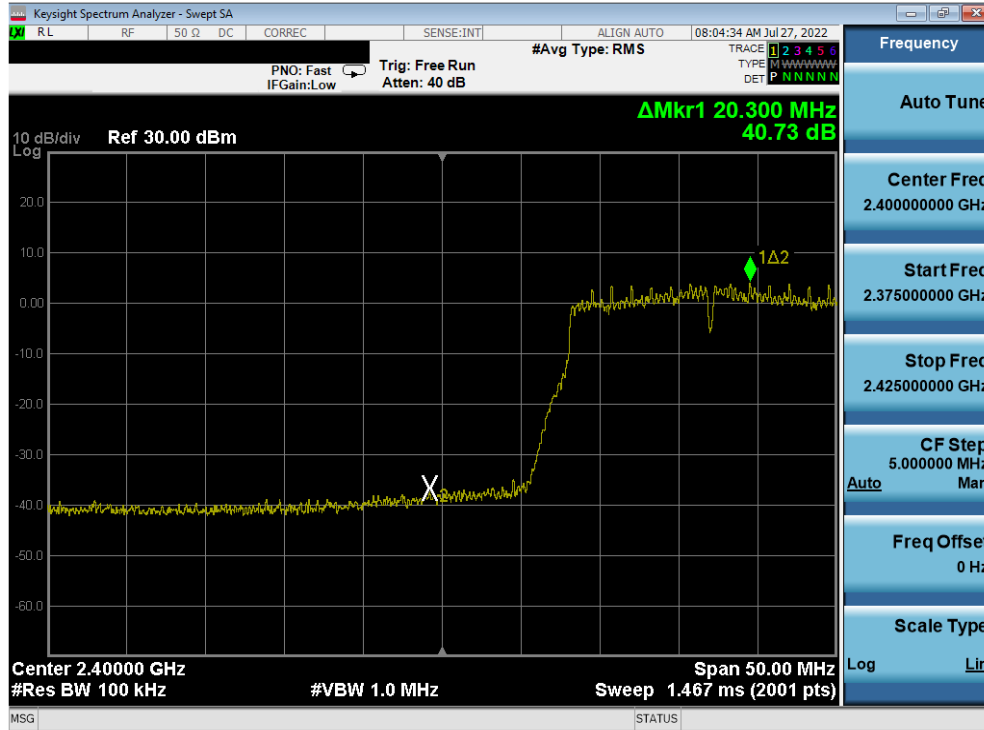
Plot 7-348. Band Edge Plot Antenna 2a (802.11n (2.4GHz) – Ch. 2) – MCS3
