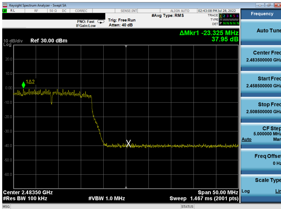
Plot 7-408. Band Edge Plot Antenna 2a (802.11n (2.4GHz) – Ch. 12) – MCS5
