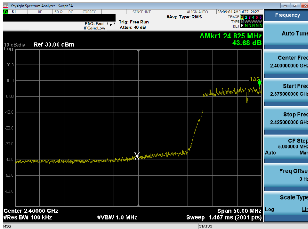
Plot 7-349. Band Edge Plot Antenna 2a (802.11n (2.4GHz) – Ch. 3) – MCS3
