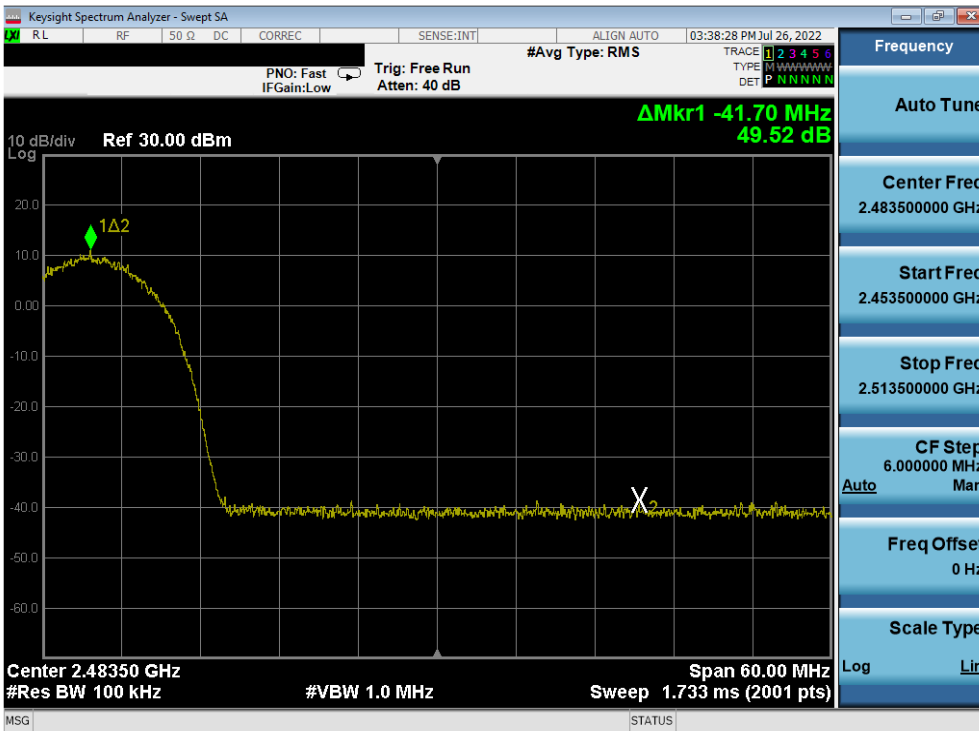
Plot 7-378. Band Edge Plot Antenna 2a (802.11b – Ch. 10) – 11Mbps
