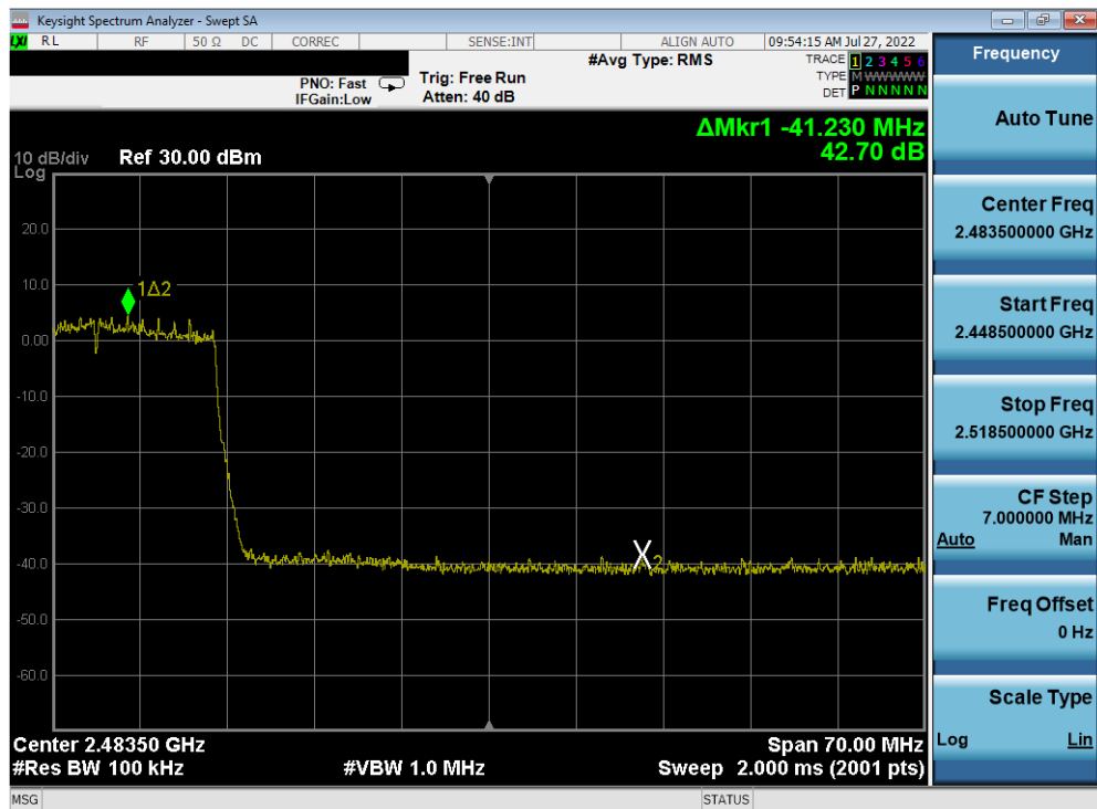
Plot 7-369. Band Edge Plot Antenna 2a (802.11ax (SU - 2.4GHz) – Ch. 9) – MCS3
