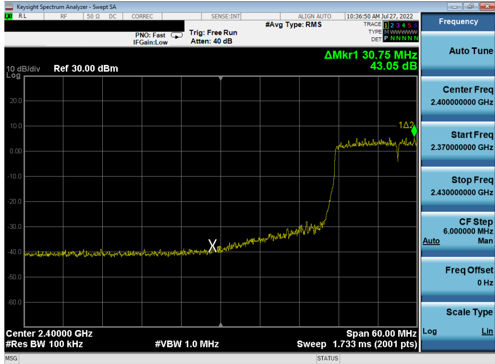
Plot 7-413. Band Edge Plot Antenna 2a (802.11ax (SU - 2.4GHz) – Ch. 4) – MCS5
