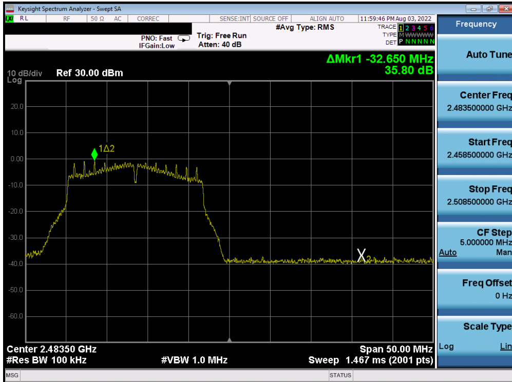
Plot 7-346. Band Edge Plot Antenna 2a (802.11g – Ch. 13) – 18Mbps
