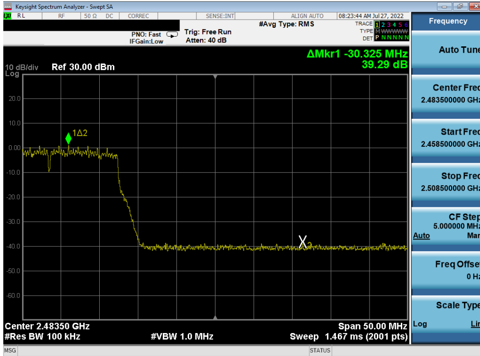
Plot 7-407. Band Edge Plot Antenna 2a (802.11n (2.4GHz) – Ch. 11) – MCS5
