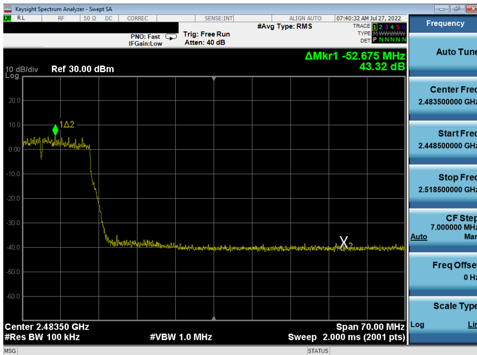
Plot 7-355. Band Edge Plot Antenna 2a (802.11n (2.4GHz) – Ch. 9) – MCS3
