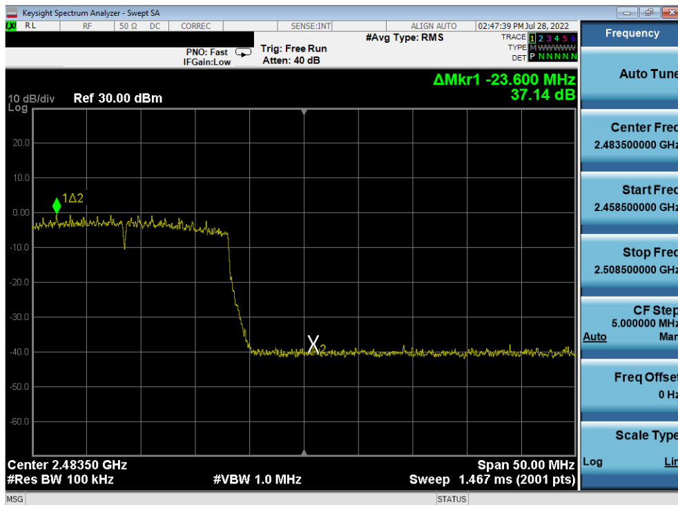
Plot 7-422. Band Edge Plot Antenna 2a (802.11ax (SU - 2.4GHz) – Ch. 12) – MCS5
