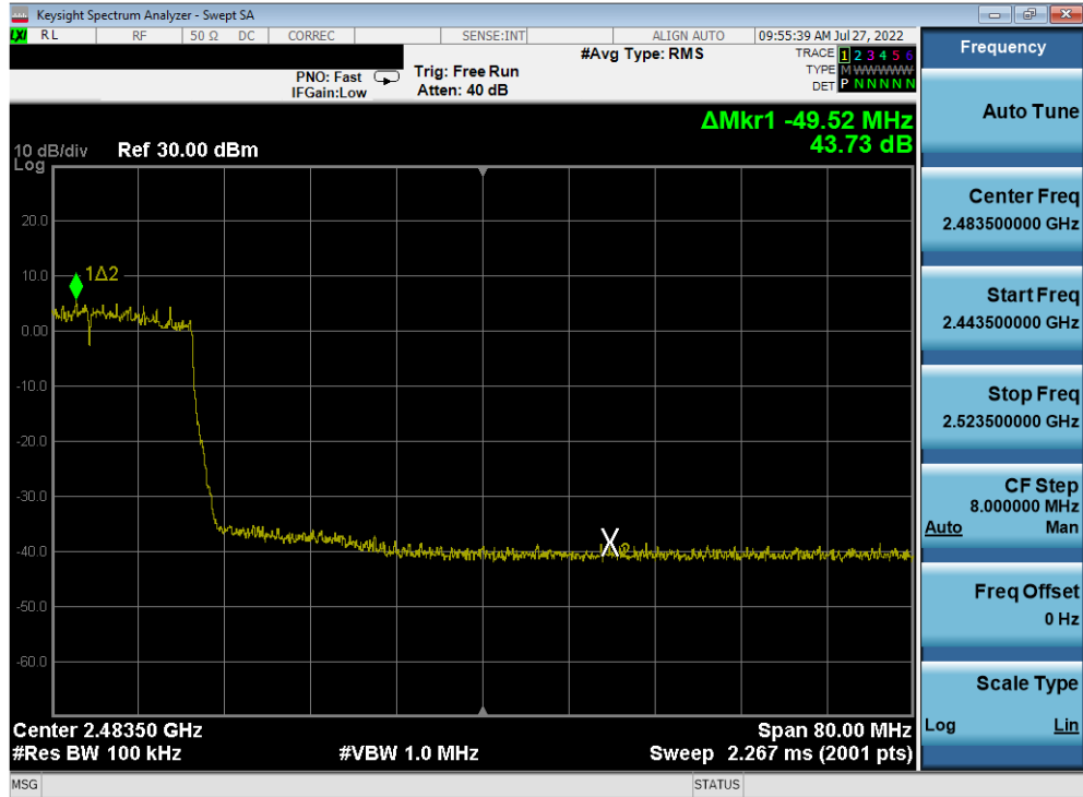
Plot 7-368. Band Edge Plot Antenna 2a (802.11ax (SU - 2.4GHz) – Ch. 8) – MCS3
