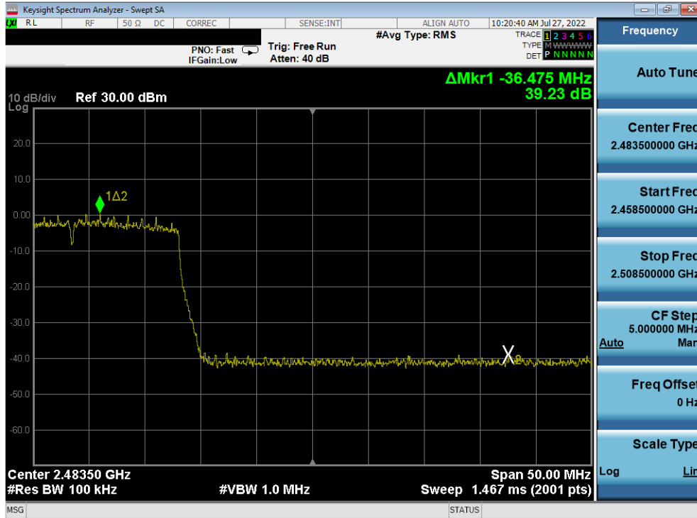
Plot 7-421. Band Edge Plot Antenna 2a (802.11ax (SU - 2.4GHz) – Ch. 11) – MCS5
