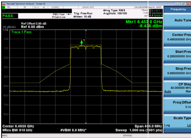
Plot 7-534. In-Band Emission Plot SDM Antenna 4a (80MHz 802.11ax (UNII Band 6) – Ch. 103, MCS11)
