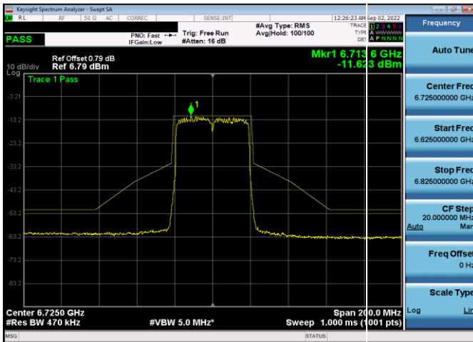
Plot 7-540. In-Band Emission Plot SDM Antenna 4a (40MHz 802.11ax (UNII Band 7) – Ch. 155, MCS11)
