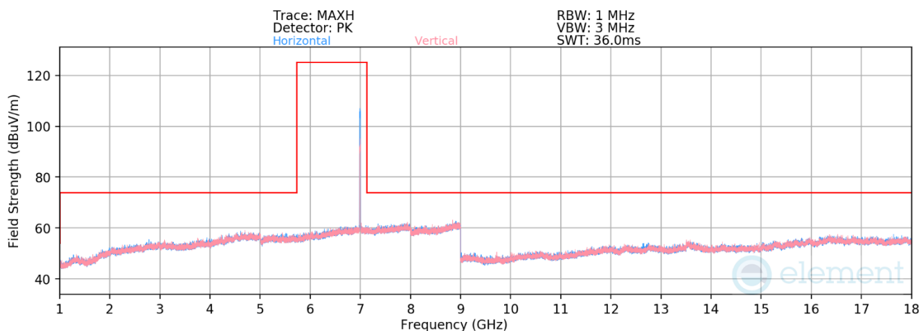
Plot 7-4. Radiated Spurious Emissions above 1GHz SDM (802.11ax – Ch. 209, MCS2)
