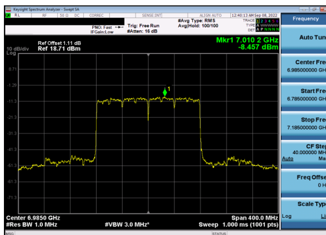
Plot 7-336. Power Spectral Density Plot SDM Antenna 4a (160MHz 802.11ax (UNII Band 8) – Ch. 207, MCS11)
